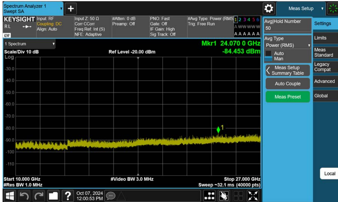
NR30_5 M_Conducted Spurious(Above10 G)_Low_BPSK_1RB
