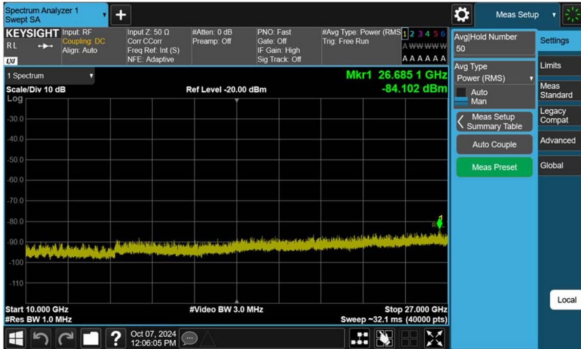
NR30_5 M_Conducted Spurious(Above10 G)_High_BPSK_1RB
