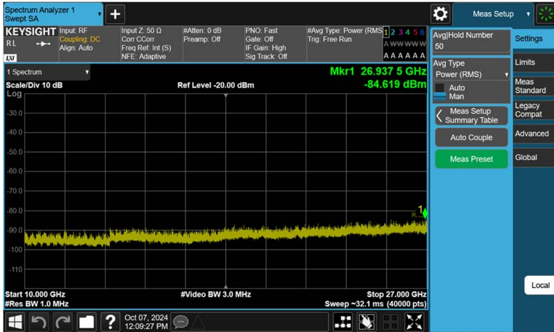
NR30_10 M_Conducted Spurious(Above10 G)_Mid_BPSK_1RB
