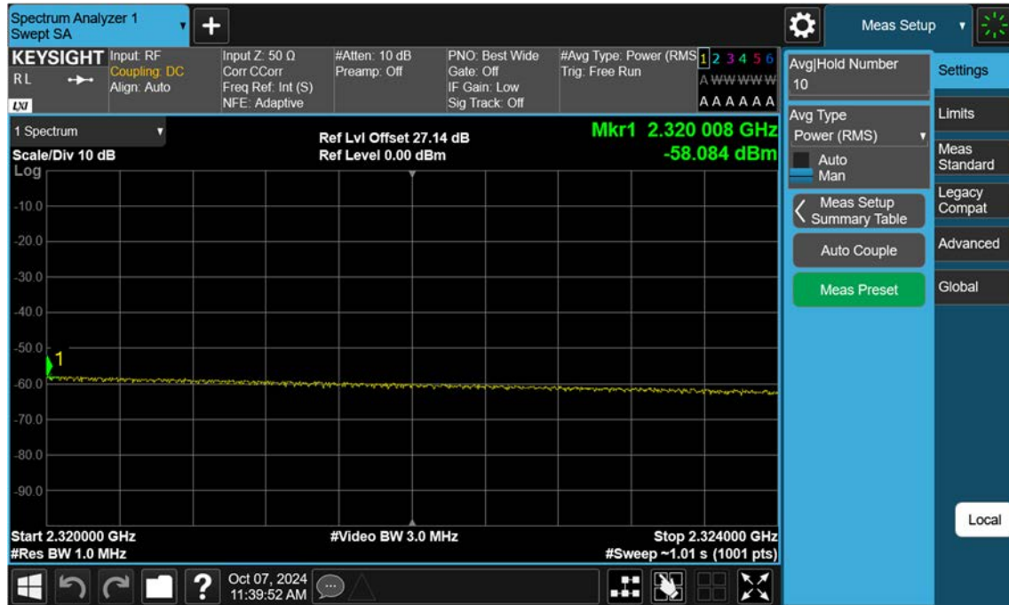
NR30_5 M_Band Edge(2320MHz-2324MHz)_Mid_BPSK_1RB
