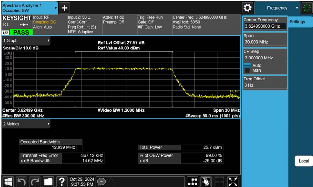
Sub6 n48. Occupied Bandwidth Plot (15 MHz Ch.641666 16-QAM RB 36)
