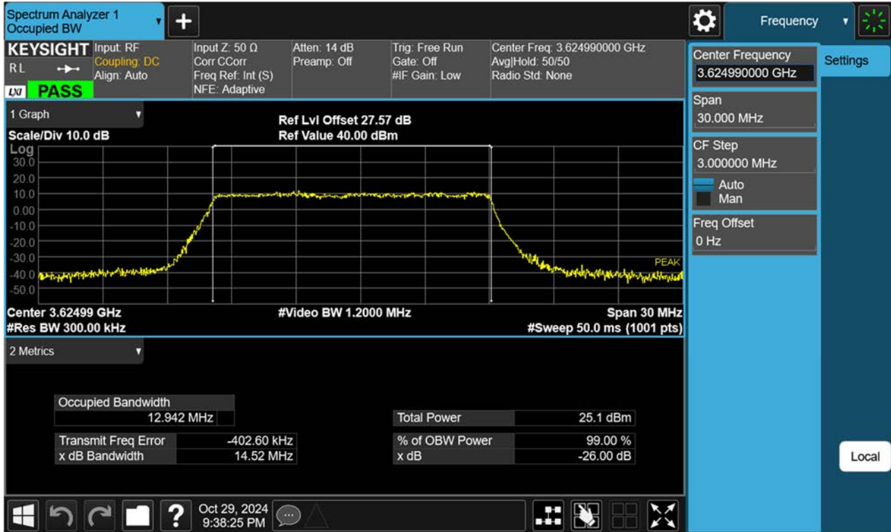
Sub6 n48. Occupied Bandwidth Plot (15 MHz Ch.641666 64-QAM RB 36)
