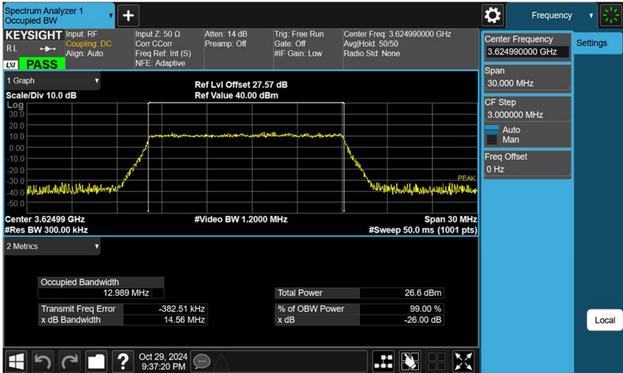
Sub6 n48. Occupied Bandwidth Plot (15 MHz Ch. 641666 QPSK RB 36)
