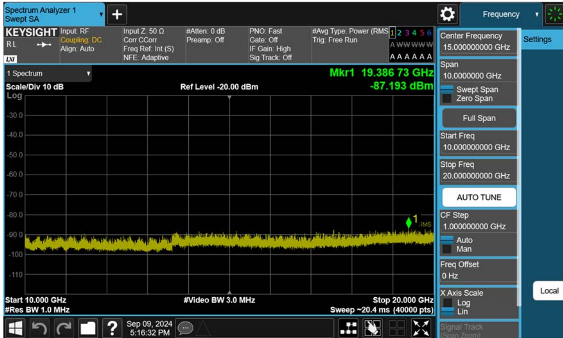
NR66_35 M_Conducted Spurious(Above10 G)_High_BPSK_1RB
