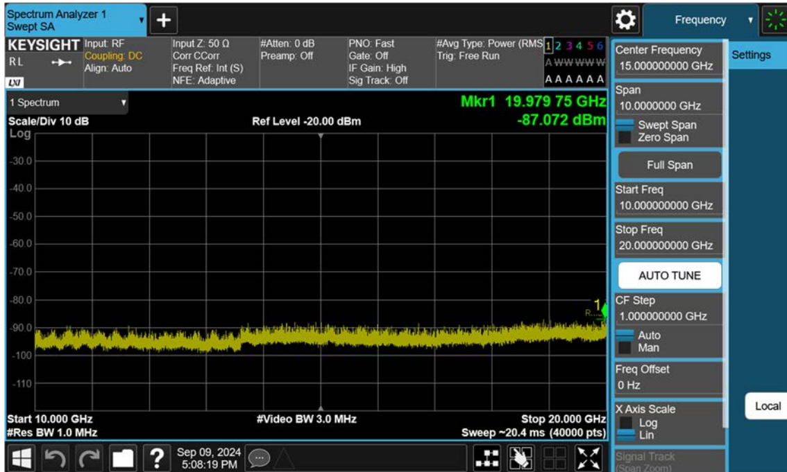
NR66_30 M_Conducted Spurious(Above10 G)_High_BPSK_1RB
