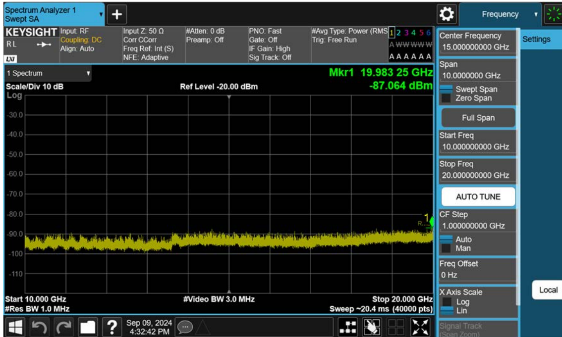
NR66_15 M_Conducted Spurious(Above10 G)_High_BPSK_1RB
