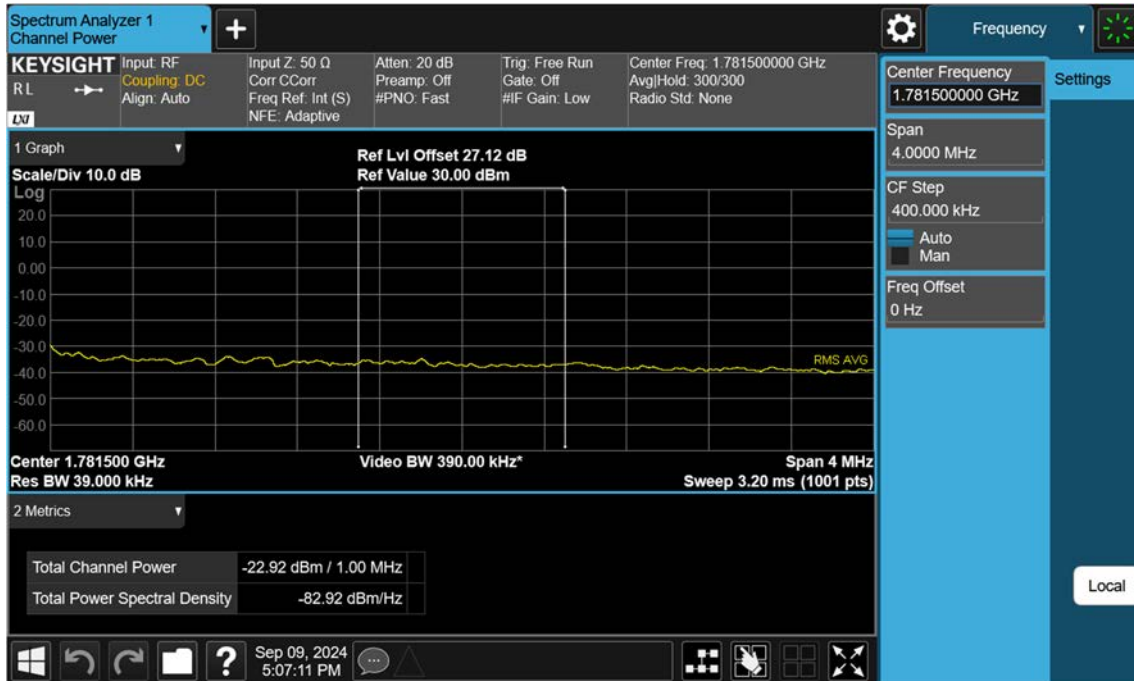
NR66_30 M_Extended Band Edge_High_BPSK_FullRB
