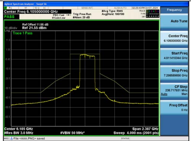
Bandwidth 320M, Ch. 31(6105 MHz) 3x996T RU104
