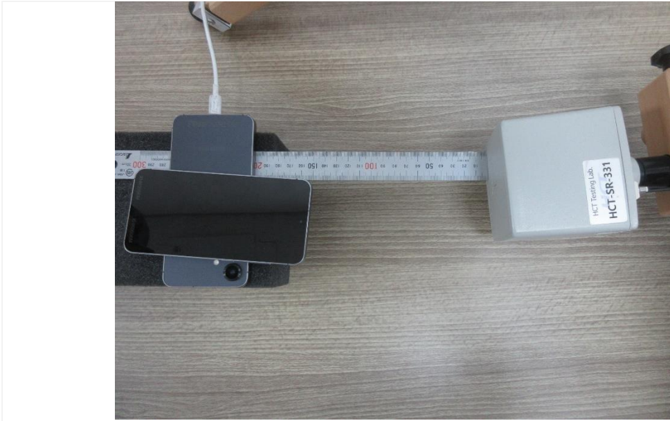
Edge 4 + TA : 20 cm (The distance between the DUT and the probe is 20 cm.)
