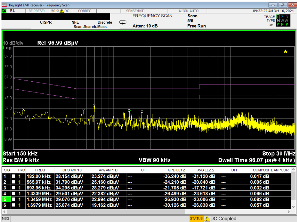
Plot 7-107. Line Conducted Plot with 802.11a UNII Band 7 (L1) with WCP
