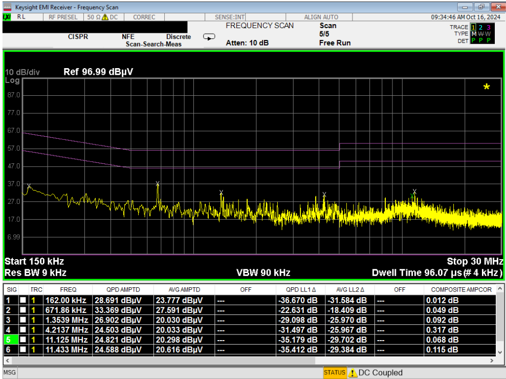
Plot 7-108. Line Conducted Plot with 802.11a UNII Band 7 (N) with WCP
