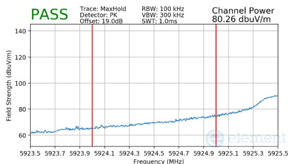
Plot 7-84. Radiated Lower Band Edge Plot MIMO (Peak – UNII Band 5)
