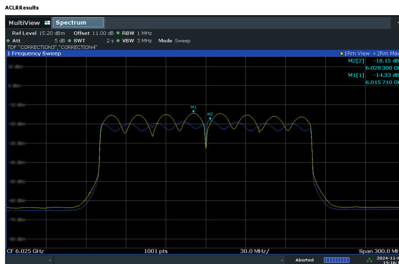
Plot 7-74. Power Spectral Density Plot – ANT1 (160MHz Bandwidth, RSSI level at -38dBm (yellow) and -34dBm (blue))
