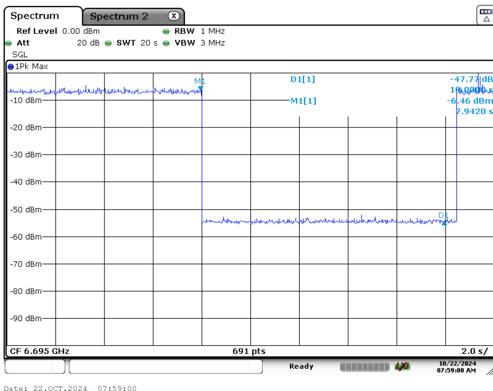
Plot 7-67. Contention Based Protocol Timing Plot (20MHz (UNII Band 7) – Ch. 149)
