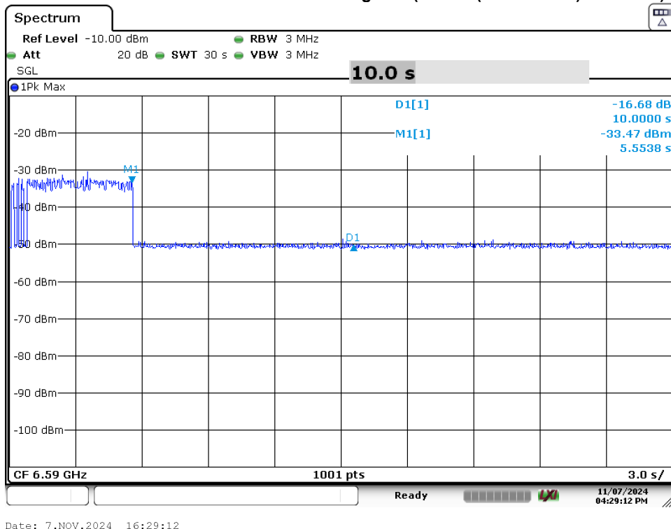
Plot 7-68. Contention Based Protocol Timing Plot (320MHz (UNII Band 7) – Ch. 175 Low)
