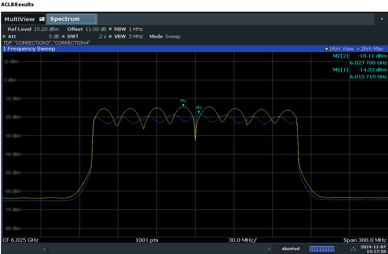
Plot 7-76. Power Spectral Density Plot – ANT1 (160MHz Bandwidth, RSSI level at -38dBm (yellow) and -18dBm (blue))
