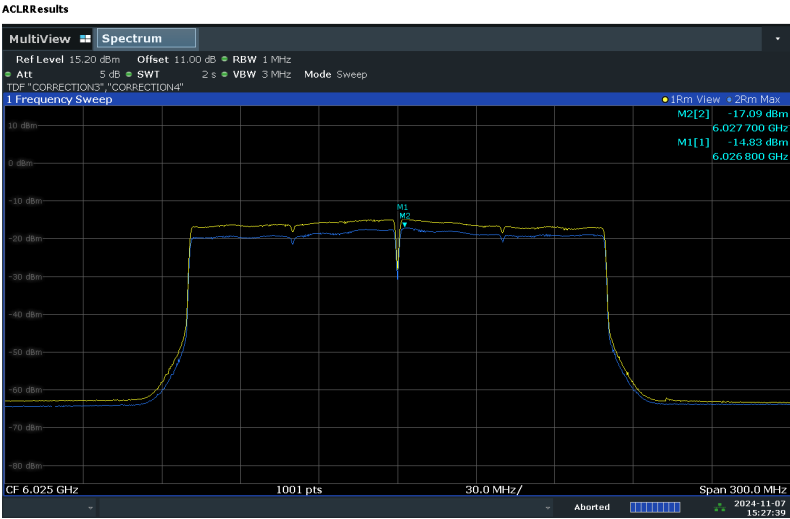
Plot 7-77. Power Spectral Density Plot – ANT2 (160MHz Bandwidth, RSSI level at -38dBm (yellow) and -18dBm (blue))
