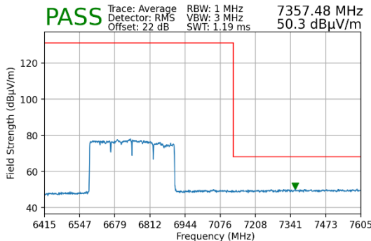
Plot 7-99. Radiated Upper Band Edge Plot MIMO (Average – UNII Band 7)
