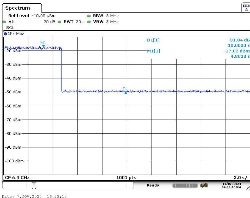
Plot 7-70. Contention Based Protocol Timing Plot (320MHz (UNII Band 7) – Ch. 175 High)
