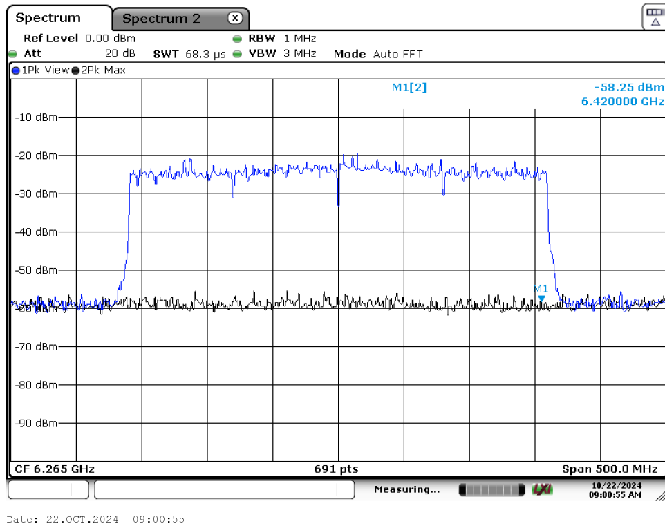
Plot 7-73. CBP 320MHz Channel - Injection Upper Edge – [6420 MHz]
