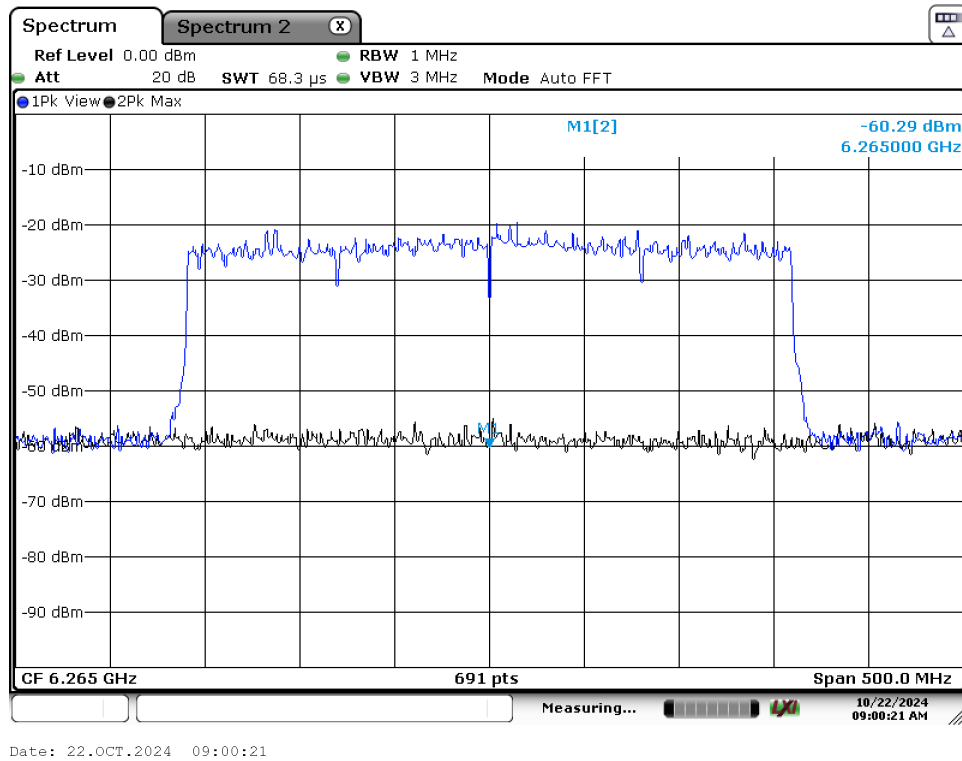
Plot 7-72. CBP 320MHz Channel - Injection Center – [6265 MHz]
