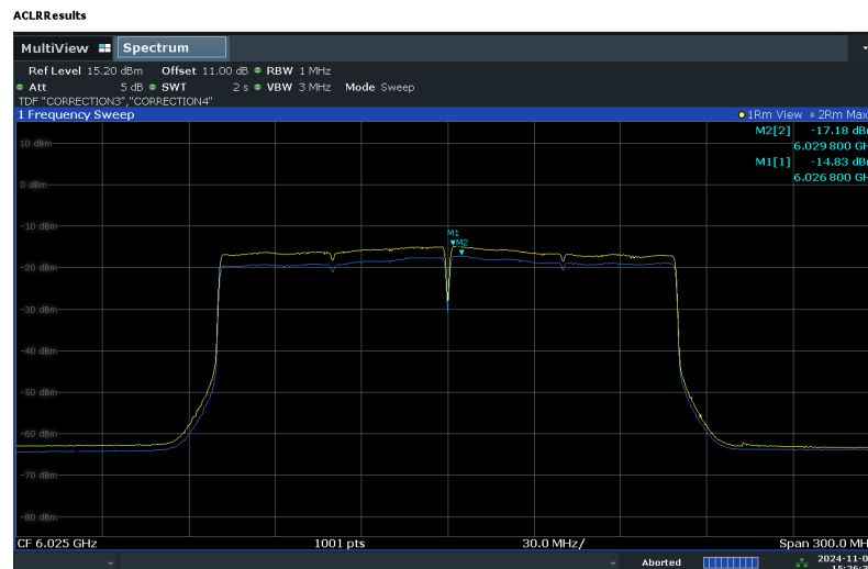
Plot 7-75. Power Spectral Density Plot – ANT2 (160MHz Bandwidth, RSSI level at -38dBm (yellow) and -34dBm (blue))
