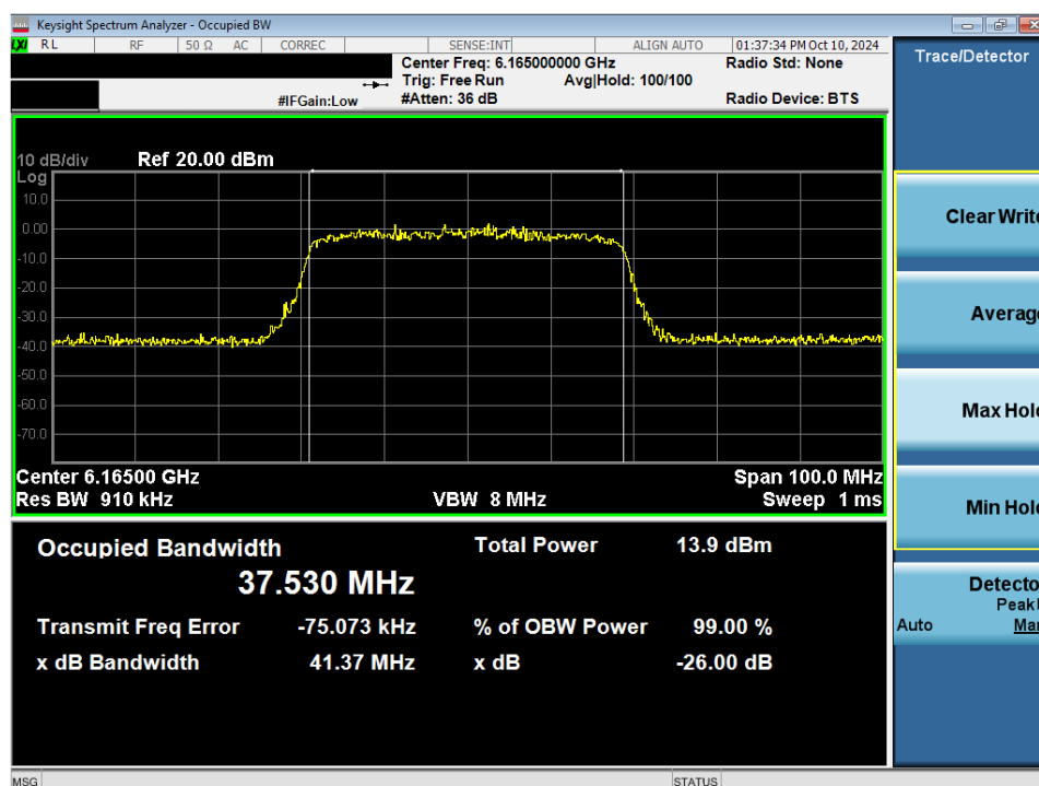
Plot 7-32. 26dB Bandwidth Plot MIMO ANT2 (40MHz 802.11ax/be (Full Tones) (UNII Band 5) – Ch. 43) - VLP
