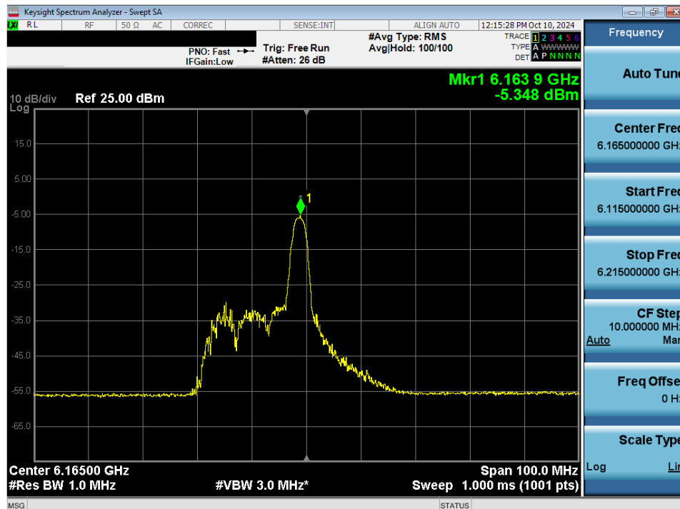
Plot 7-51. Power Spectral Density Plot MIMO ANT2 (40MHz 802.11ax/be (26 Tones) (UNII Band 5) – Ch. 43) - VLP
