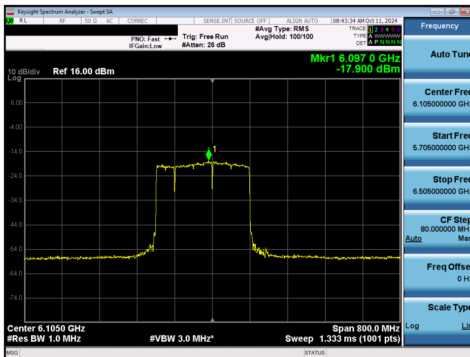
Plot 7-44. Power Spectral Density Plot MIMO ANT1 (320MHz 802.11be (UNII Band 5) – Ch. 31) VLP
