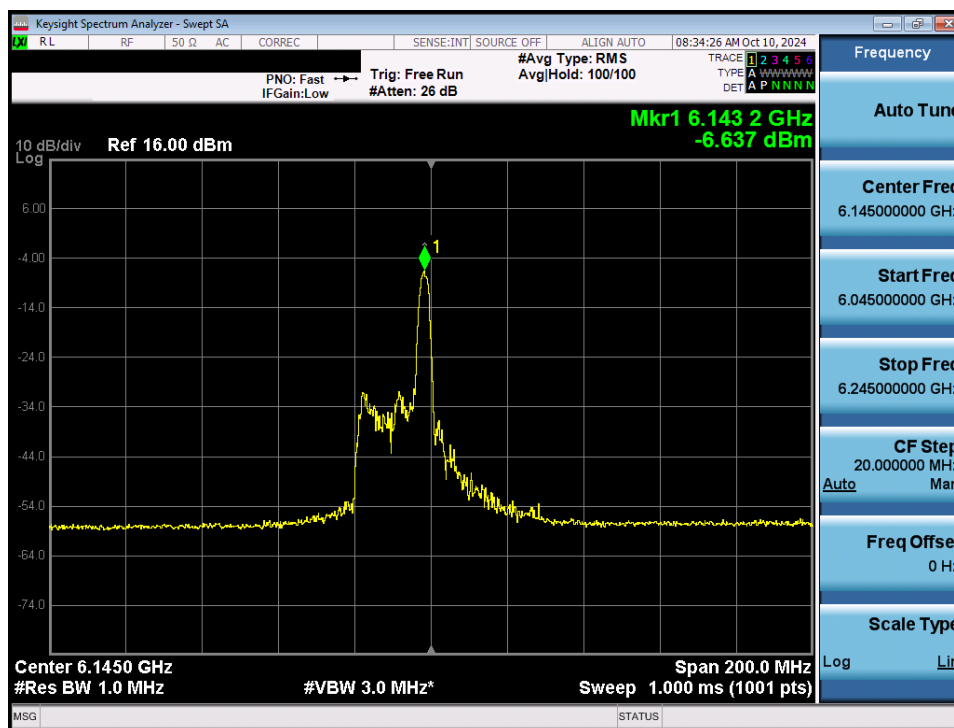
Plot 7-38. Power Spectral Density Plot MIMO ANT1 (80MHz 802.11ax/be (26 Tones) (UNII Band 5) – Ch. 39) - VLP
