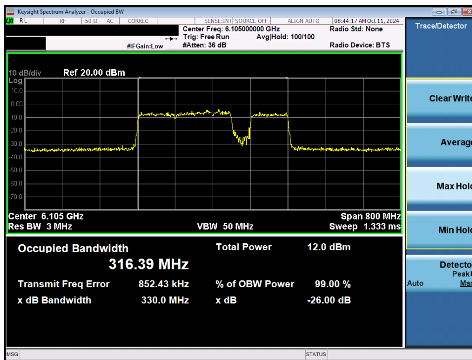
Plot 7-16. 26dB Bandwidth Plot MIMO ANT1 (320MHz 802.11be (3*996+484 Tones) (UNII Band 5) – Ch. 31) VLP
