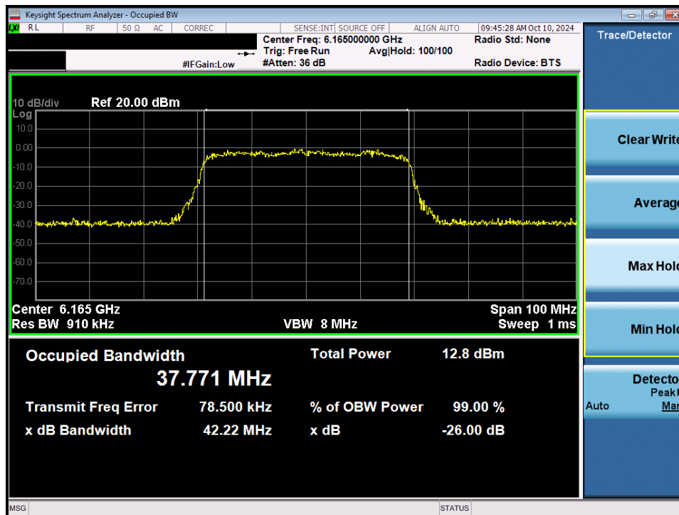
Plot 7-18. 26dB Bandwidth Plot MIMO ANT1 (40MHz 802.11ax/be (Full Tones) (UNII Band 5) – Ch. 43) - VLP
