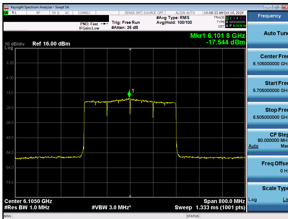
Plot 7-49. Power Spectral Density Plot MIMO ANT1 (320MHz 802.11be (Full Tones) (UNII Band 5) – Ch. 31) - VLP
