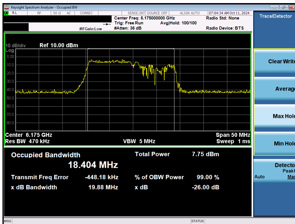
Plot 7-13. 26dB Bandwidth Plot MIMO ANT1 (20MHz 802.11be (106+26 Tones) (UNII Band 5) – Ch. 45) - VLP
