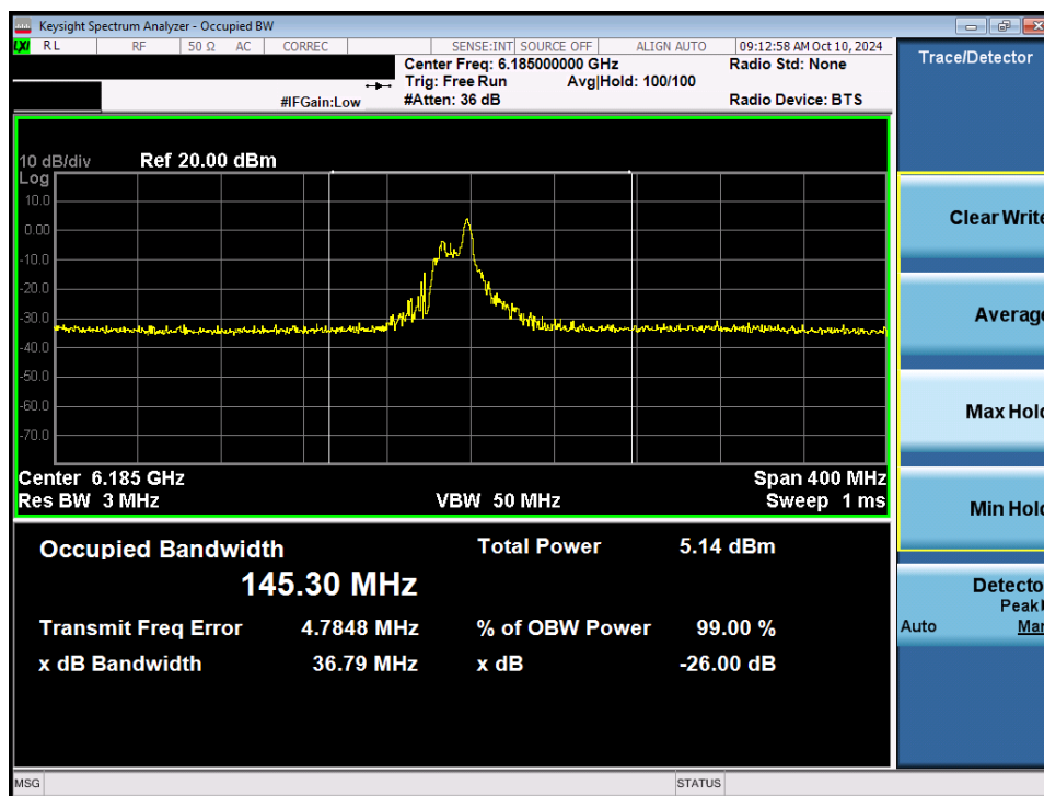
Plot 7-11. 26dB Bandwidth Plot MIMO ANT1 (160MHz 802.11ax/be (26 Tones) (UNII Band 5) – Ch. 47) - VLP
