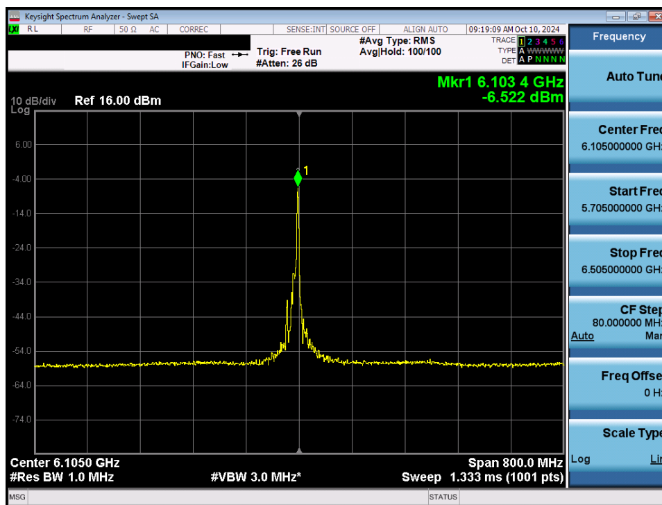
Plot 7-40. Power Spectral Density Plot MIMO ANT1 (320MHz 802.11be (26 Tones) (UNII Band 5) – Ch. 31) - VLP
