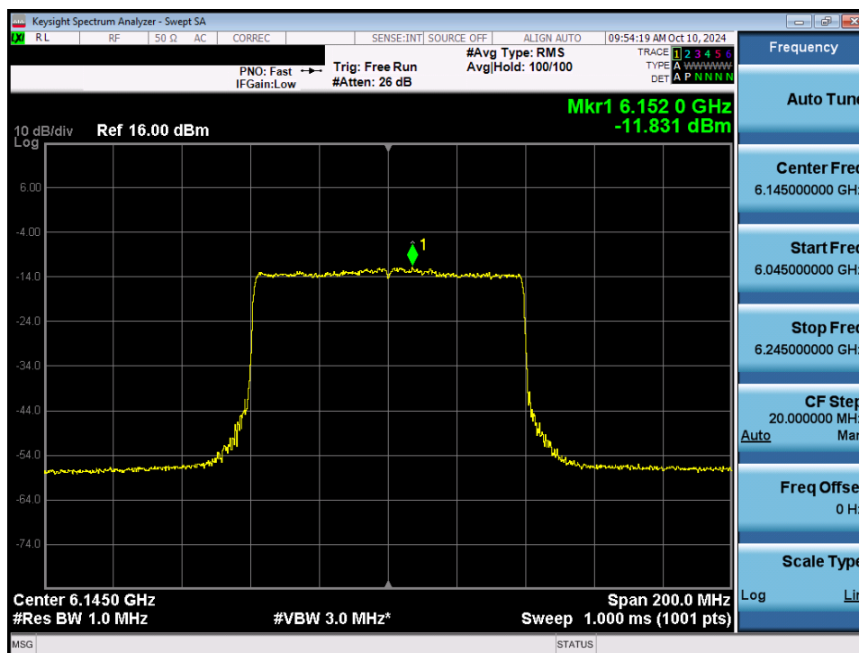
Plot 7-47. Power Spectral Density Plot MIMO ANT1 (80MHz 802.11ax/be (Full Tones) (UNII Band 5) – Ch. 39) - VLP
