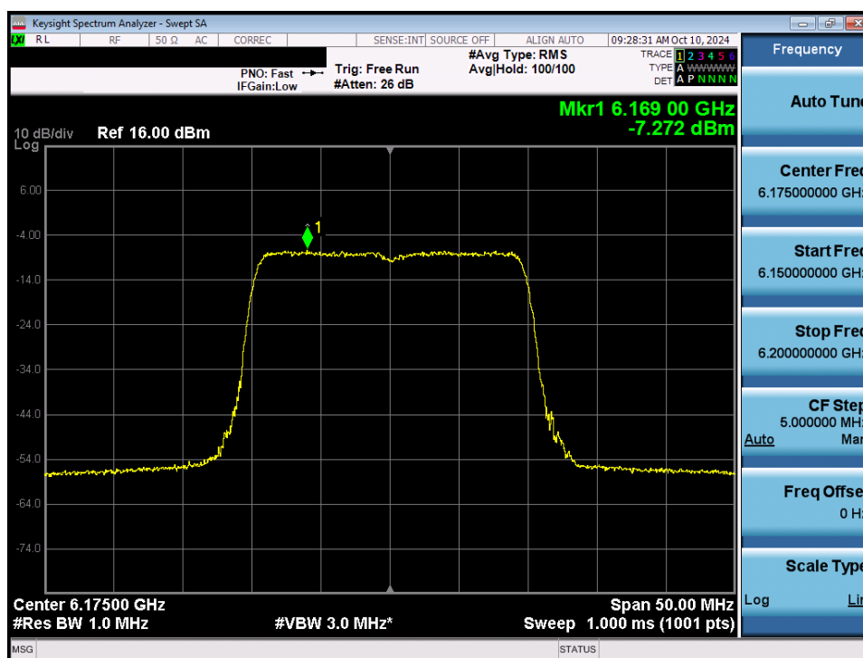
Plot 7-45. Power Spectral Density Plot MIMO ANT1 (20MHz 802.11ax/be (Full Tones) (UNII Band 5) – Ch. 45) - VLP
