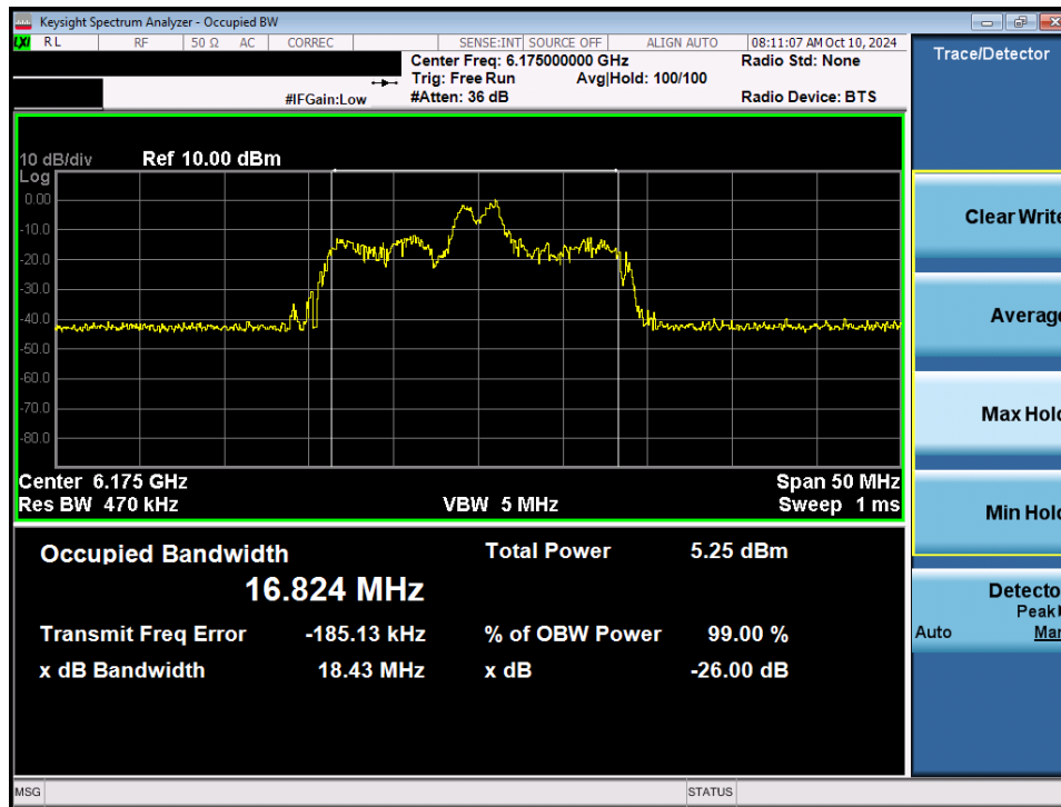
Plot 7-8. 26dB Bandwidth Plot MIMO ANT1 (20MHz 802.11ax/be (26 Tones) (UNII Band 5) – Ch. 45) - VLP
