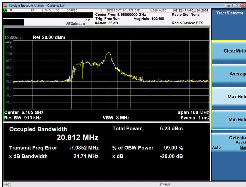
Plot 7-9. 26dB Bandwidth Plot MIMO ANT1 (40MHz 802.11ax/be (26 Tones) (UNII Band 5) – Ch. 43) - VLP
