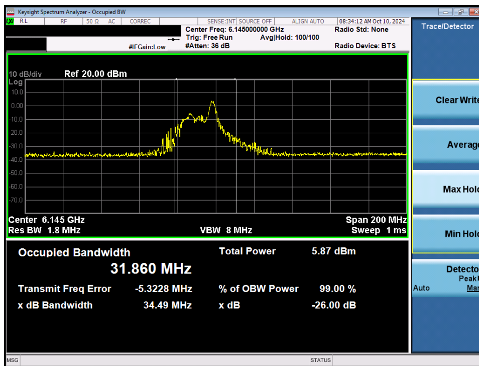
Plot 7-10. 26dB Bandwidth Plot MIMO ANT1 (80MHz 802.11ax/be (26 Tones) (UNII Band 5) – Ch. 39) - VLP
