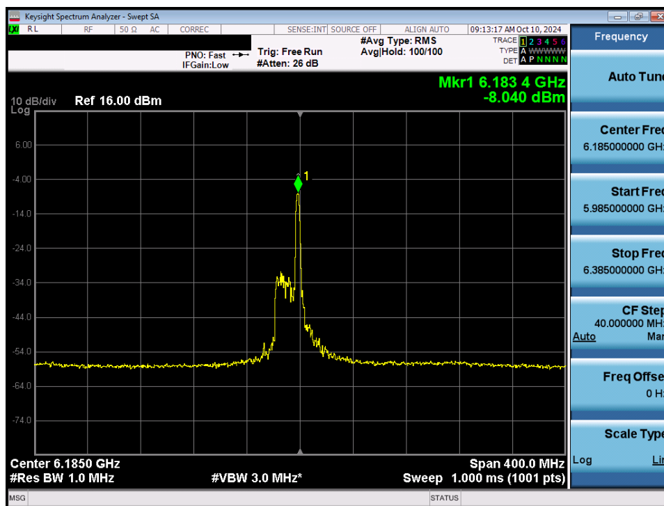
Plot 7-39. Power Spectral Density Plot MIMO ANT1 (160MHz 802.11ax/be (26 Tones) (UNII Band 5) – Ch. 47) - VLP
