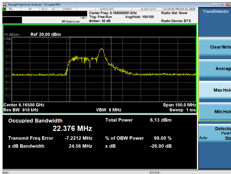
Plot 7-23. 26dB Bandwidth Plot MIMO ANT2 (40MHz 802.11ax/be (26 Tones) (UNII Band 5) – Ch. 43) - VLP
