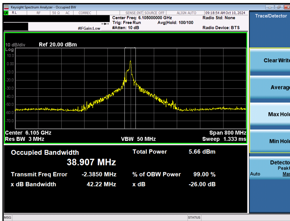
Plot 7-12. 26dB Bandwidth Plot MIMO ANT1 (320MHz 802.11be (26 Tones) (UNII Band 5) – Ch. 31) - VLP
