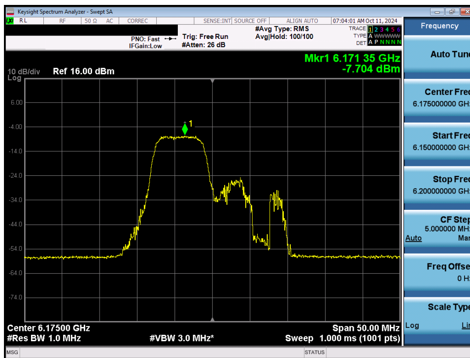
Plot 7-41. Power Spectral Density Plot MIMO ANT1 (20MHz 802.11be (52+26 Tones) (UNII Band 5) – Ch. 45) - VLP
