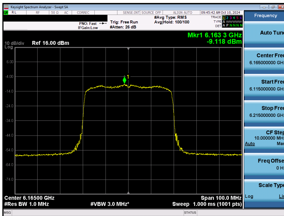
Plot 7-46. Power Spectral Density Plot MIMO ANT1 (40MHz 802.11ax/be (Full Tones) (UNII Band 5) – Ch. 43) - VLP
