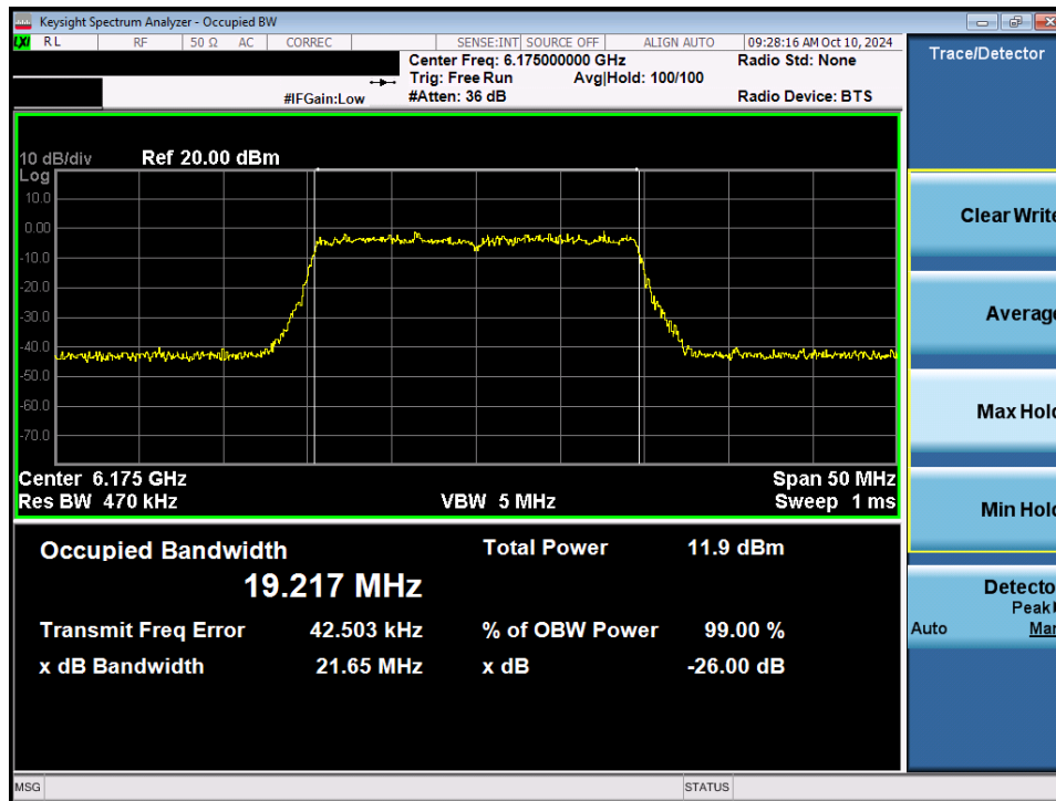
Plot 7-17. 26dB Bandwidth Plot MIMO ANT1 (20MHz 802.11ax/be (Full Tones) (UNII Band 5) – Ch. 45) - VLP
