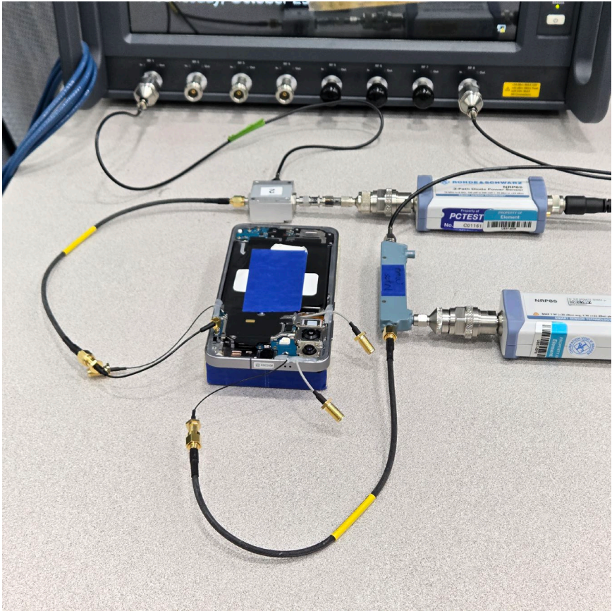
Test Setup Photo 6 – Conducted Test Setup (Figure 5-1c)
