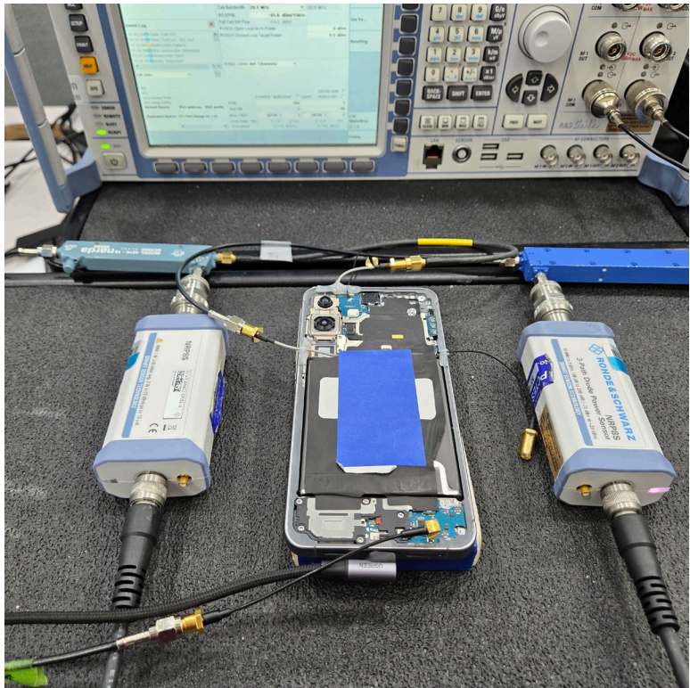
Test Setup Photo 9 – Conducted Test Setup (Figure 5-1e)
