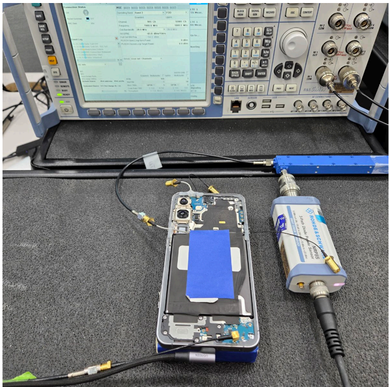
Test Setup Photo 8 – Conducted Test Setup (Figure 5-1d)
