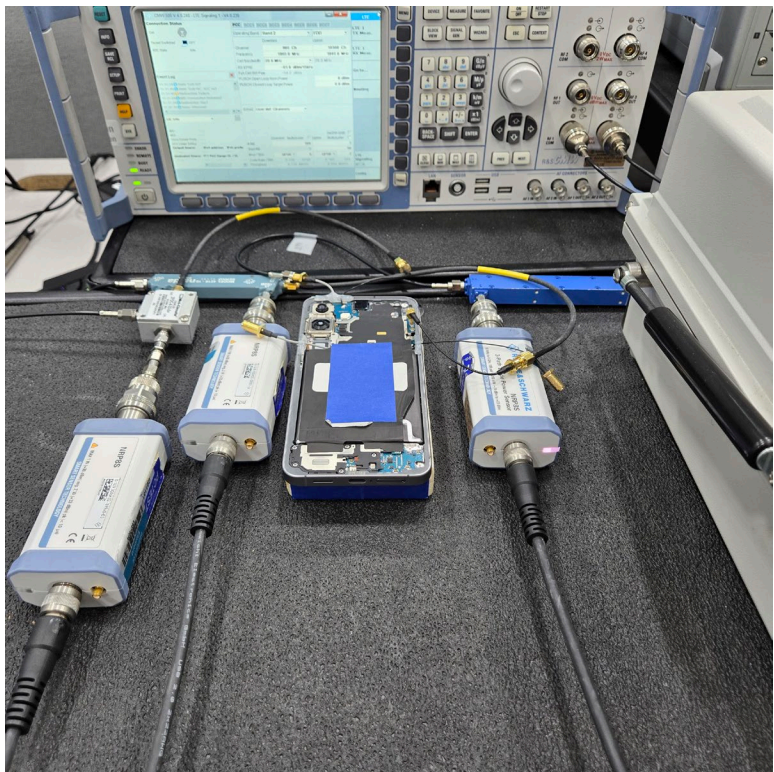
Test Setup Photo 10 – Conducted Test Setup (Figure 5-1f)
