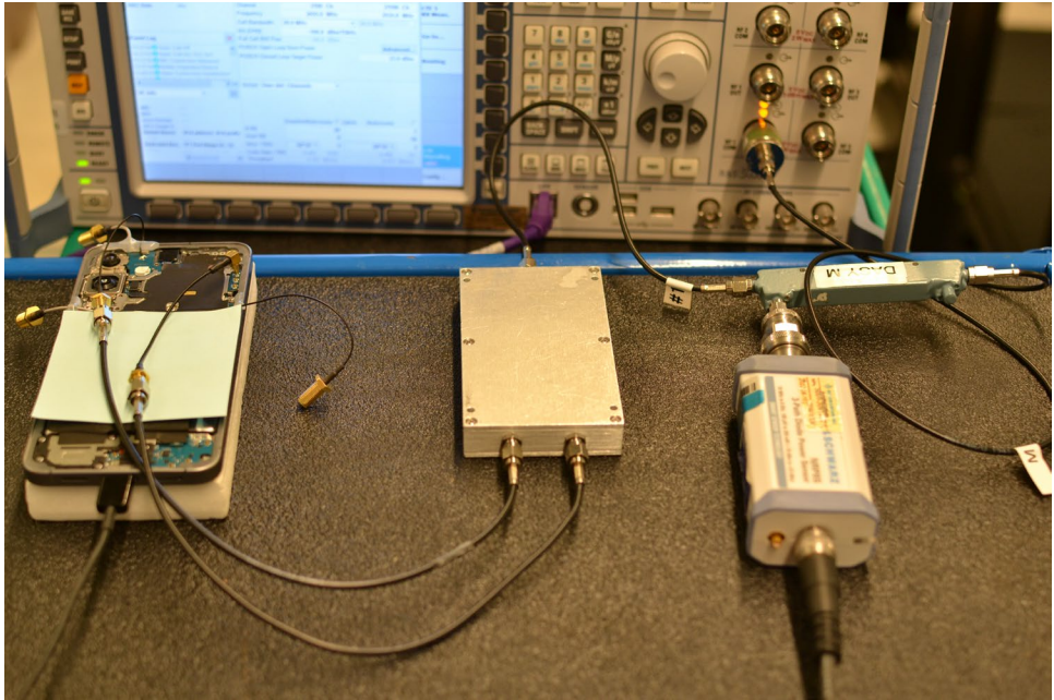
Test Setup Photo 5 – Conducted Test Setup (Figure 5-1b)
