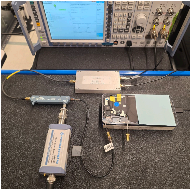
Test Setup Photo 11 – Conducted Test Setup (Figure 5-1g)
