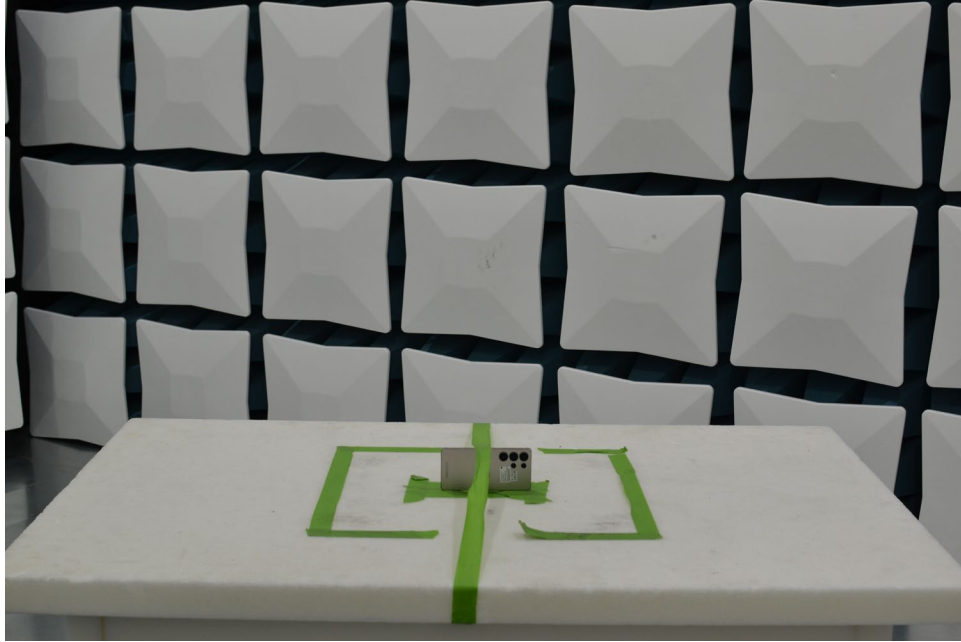
Figure 7. Test Setup – Y Position – 30MHz-1GHz
