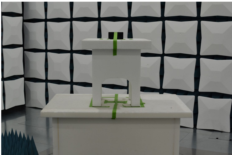
Figure 2. Test Setup – Y Position – 1GHz-40GHz
