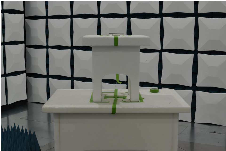
Figure 5. Test Setup – Wireless Charging Pad – 1GHz-40GHz
