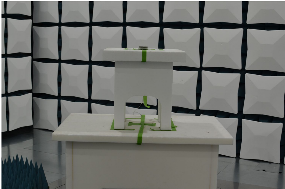
Figure 4. Test Setup – Wireless Charging Pad – 1GHz-40GHz
