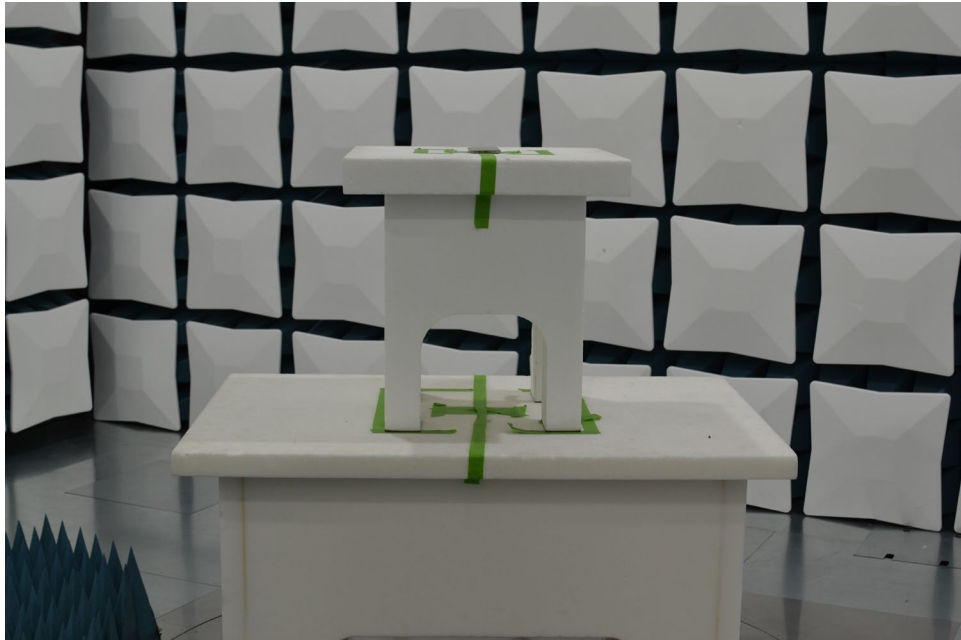
Figure 1. Test Setup – X Position – 1GHz-40GHz
