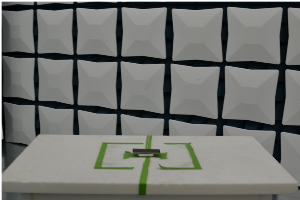
Figure 10. Test Setup – Wireless Charging Pad – 30MHz-1GHz
