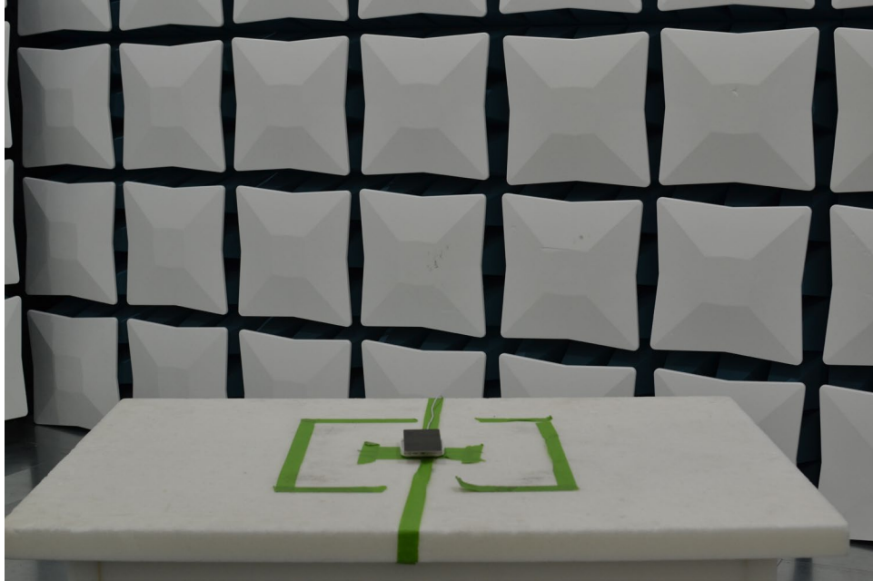
Figure 9. Test Setup – Wireless Charging Pad – 30MHz-1GHz
