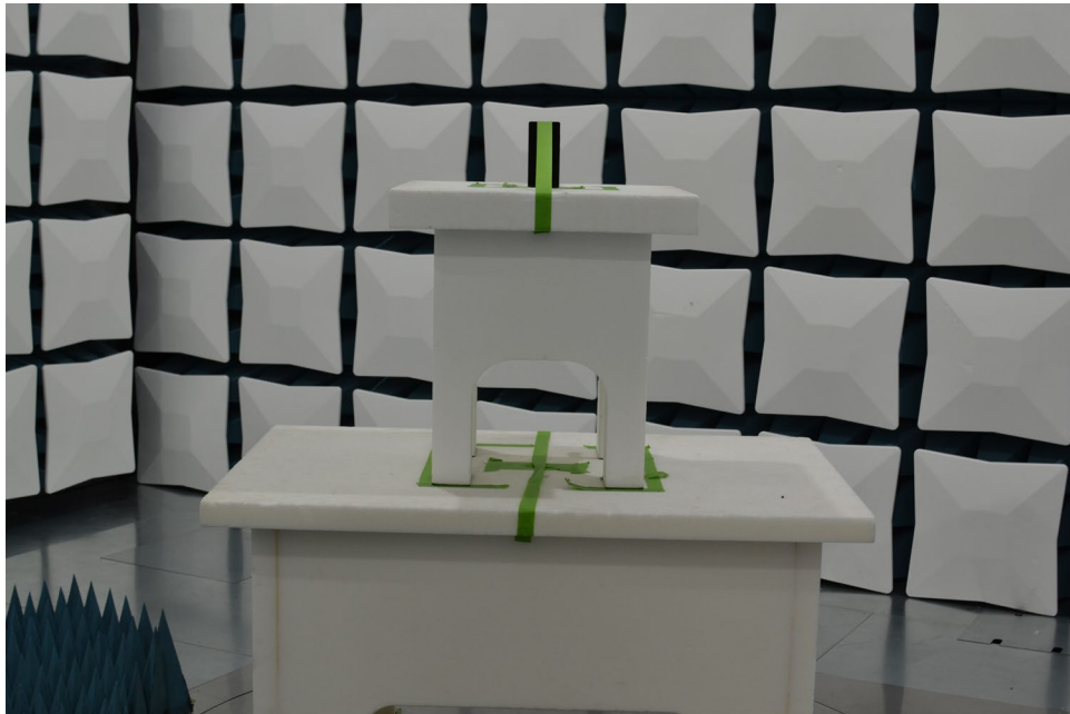
Figure 3. Test Setup – Z Position – 1GHz-40GHz
