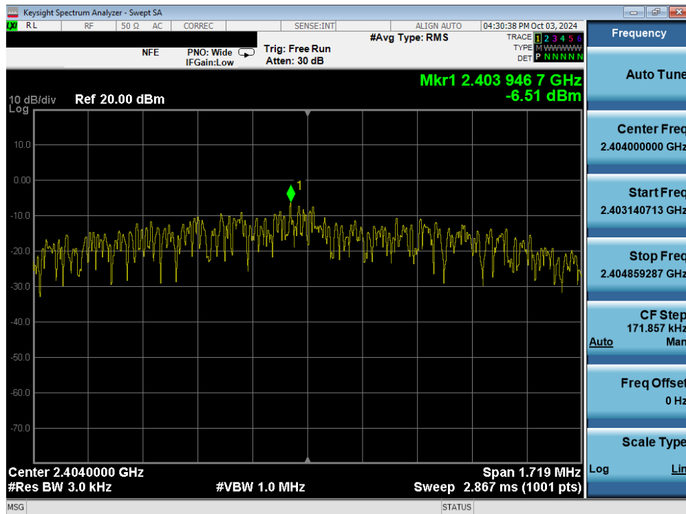
Plot 7-106. Power Spectral Density Plot (Bluetooth (LE), 2Mbps – Ch. 1) – Dual Ant 2
