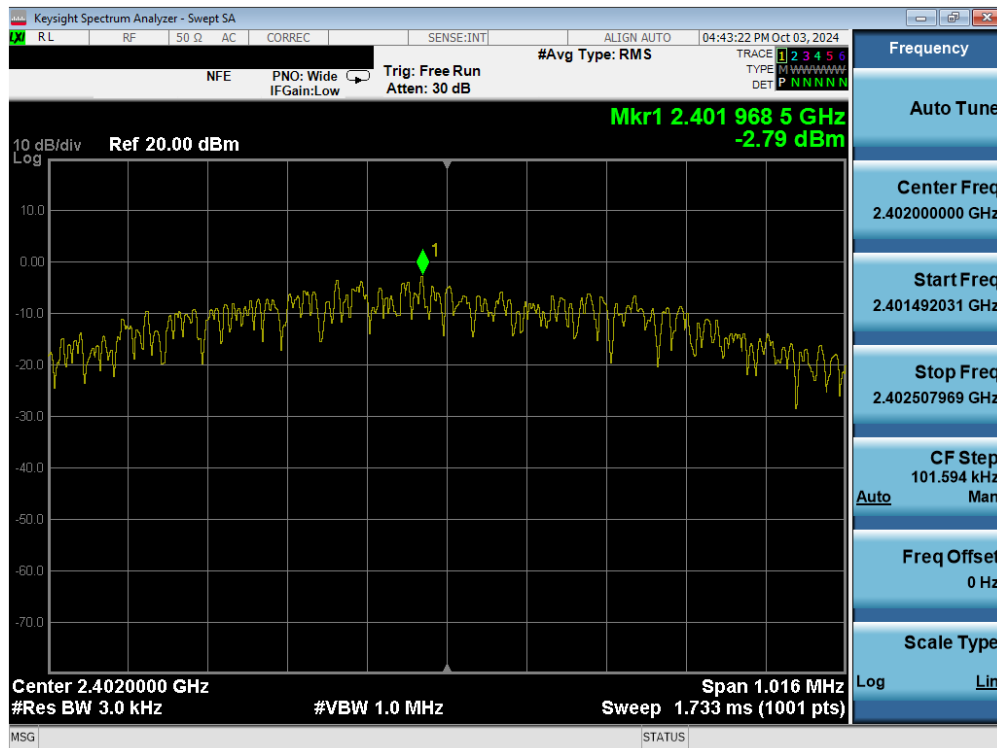
Plot 7-97. Power Spectral Density Plot (Bluetooth (LE), 1Mbps – Ch. 0) – Dual Ant 1
