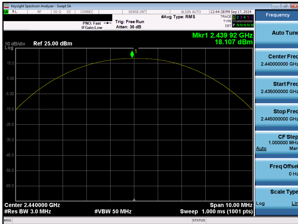
Plot 7-44. Peak Power Plot (Bluetooth (LE), 1Mbps – Ch. 19) – Ant 1
