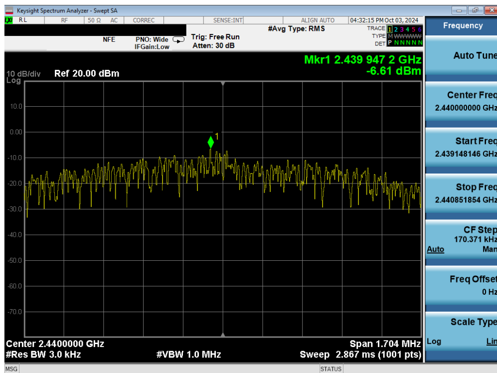
Plot 7-107. Power Spectral Density Plot (Bluetooth (LE), 2Mbps – Ch. 19) – Dual Ant 2
