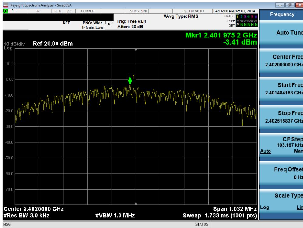
Plot 7-103. Power Spectral Density Plot (Bluetooth (LE), 1Mbps – Ch. 0) – Dual Ant 2
