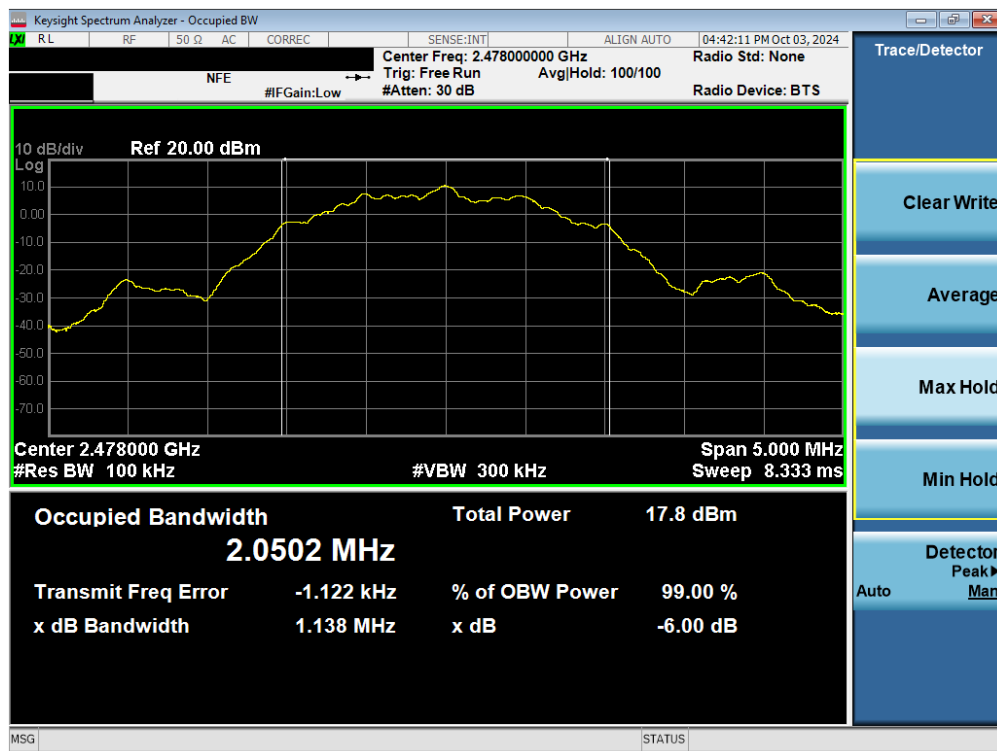
Plot 7-30. 6dB Bandwidth Plot (Bluetooth (LE), 2Mbps – Ch. 38) – Dual Ant 1
