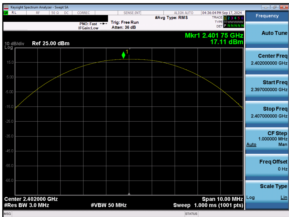
Plot 7-55. Peak Power Plot (Bluetooth (LE), 1Mbps – Ch. 0) – Ant 2
