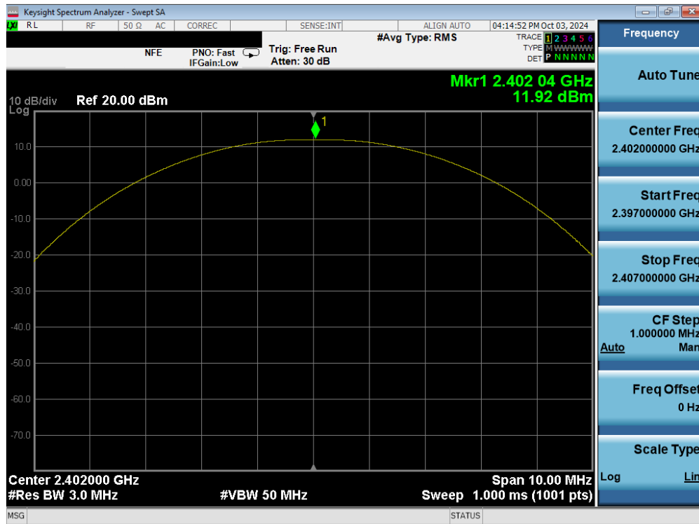
Plot 7-67. Peak Power Plot (Bluetooth (LE), 1Mbps – Ch. 0) – Daul Ant 2
