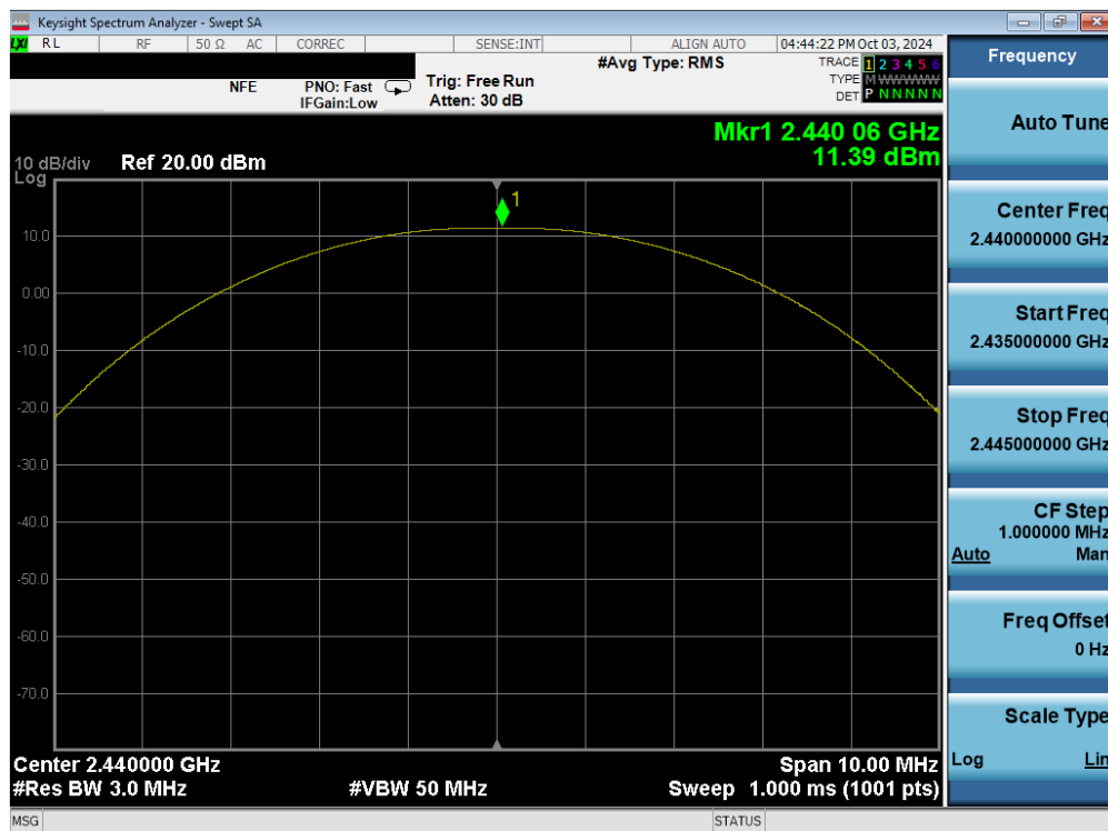
Plot 7-62. Peak Power Plot (Bluetooth (LE), 1Mbps – Ch. 19) – Daul Ant 1
