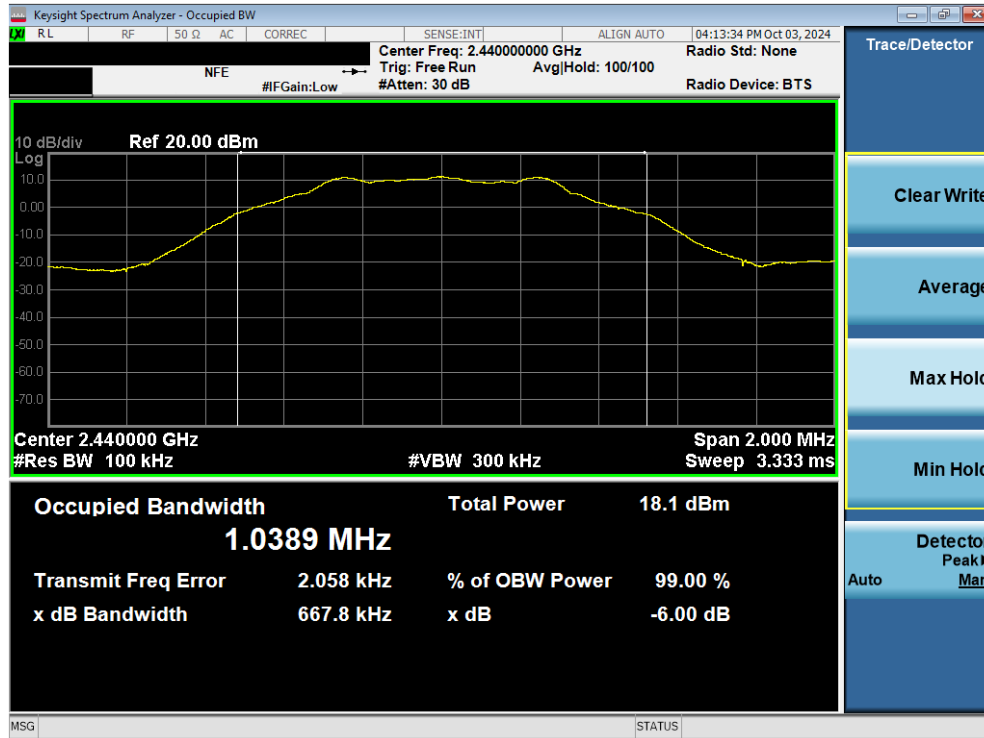
Plot 7-32. 6dB Bandwidth Plot (Bluetooth (LE), 1Mbps – Ch. 19) – Dual Ant 2
