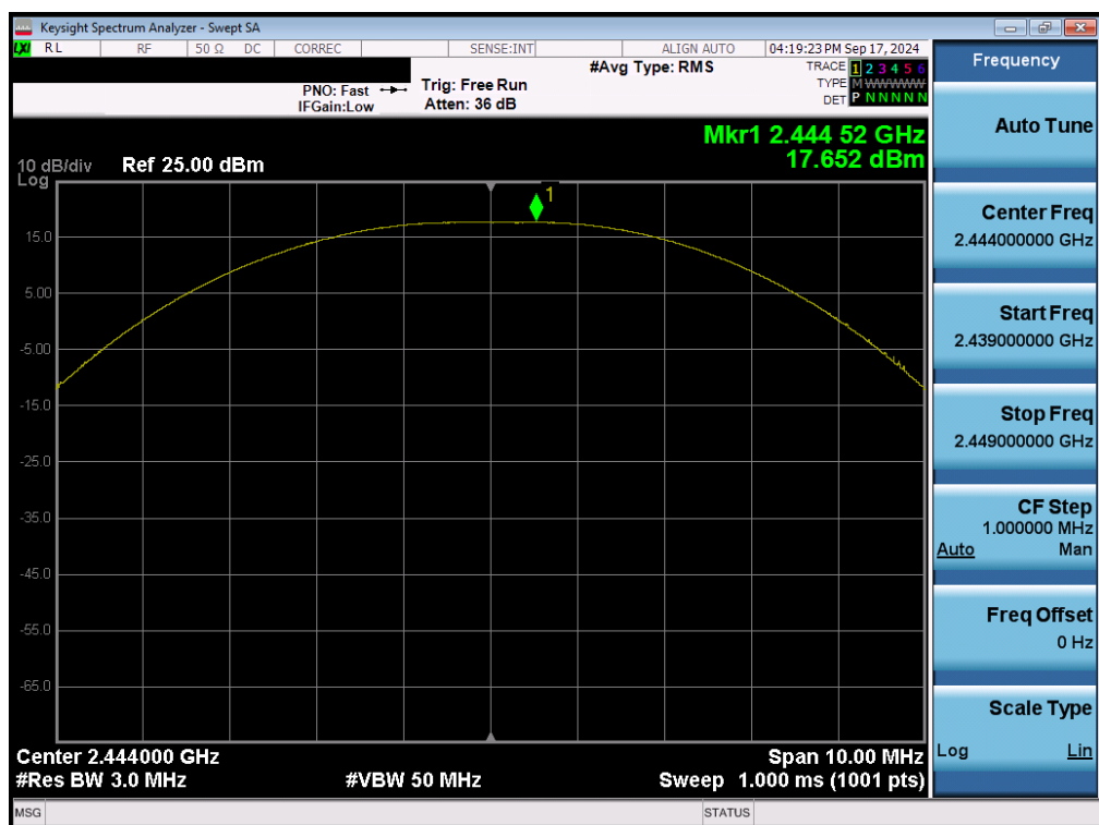
Plot 7-59. Peak Power Plot (Bluetooth (LE), 2Mbps – Ch. 19) – Ant 2
