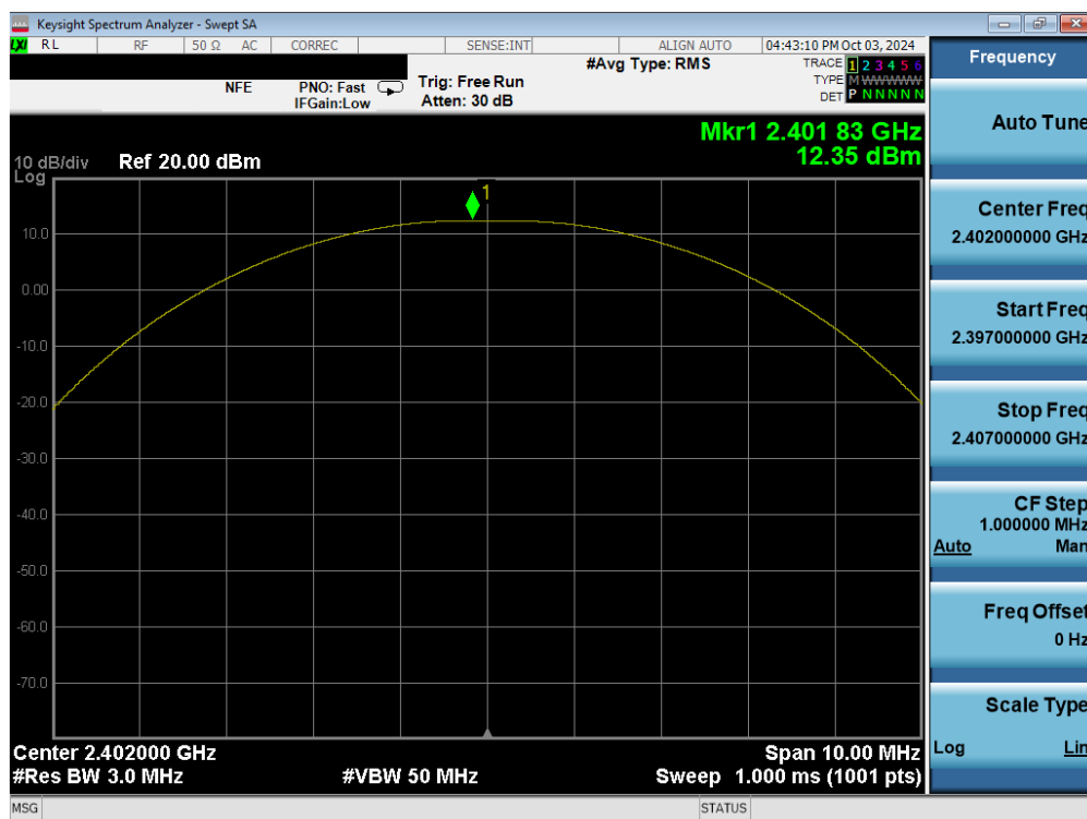
Plot 7-61. Peak Power Plot (Bluetooth (LE), 1Mbps – Ch. 0) – Daul Ant 1
