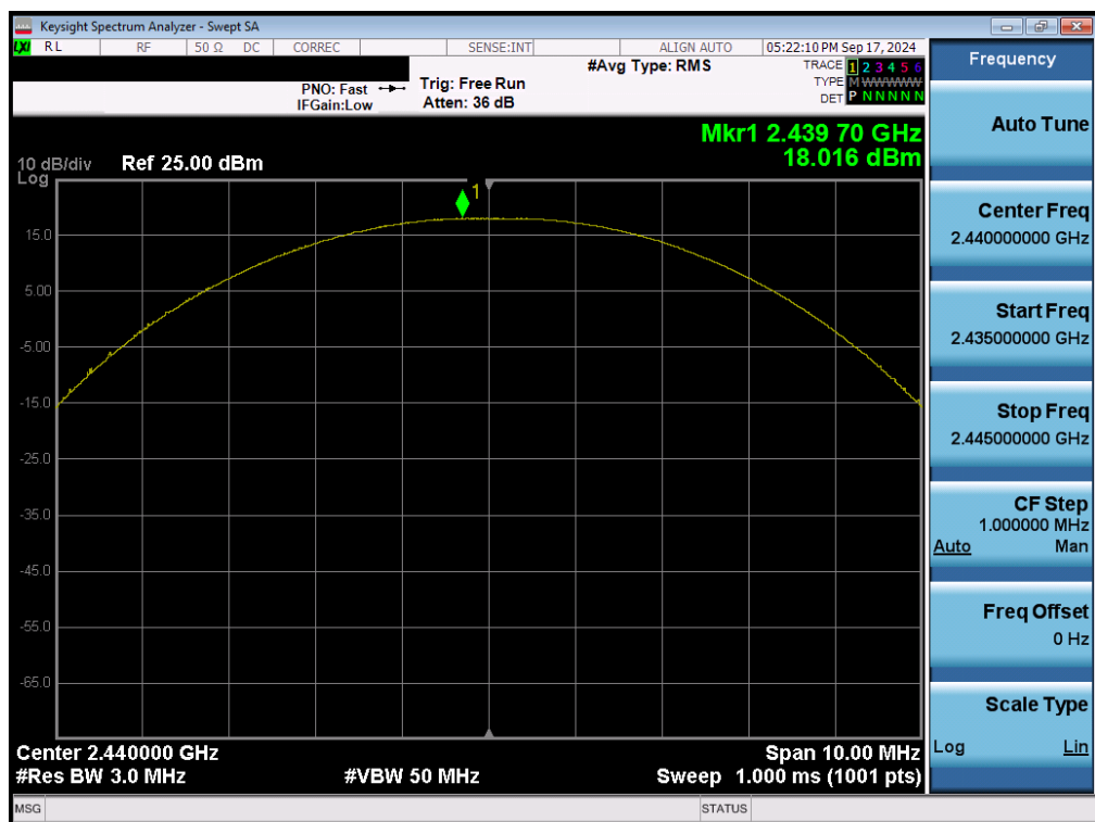
Plot 7-56. Peak Power Plot (Bluetooth (LE), 1Mbps – Ch. 19) – Ant 2
