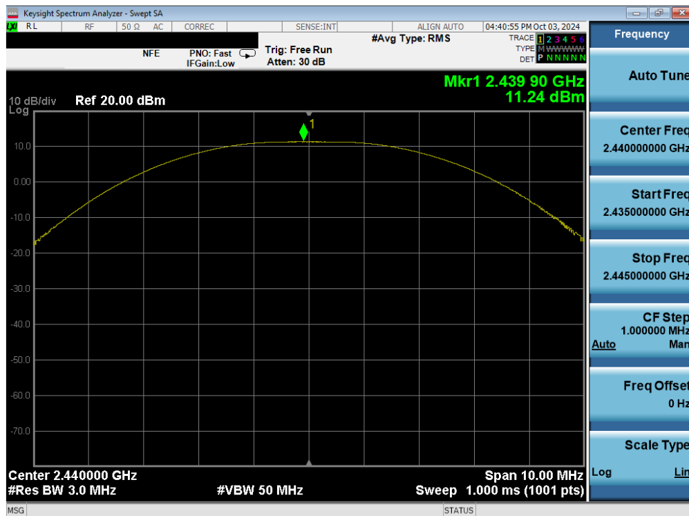
Plot 7-65. Peak Power Plot (Bluetooth (LE), 2Mbps – Ch. 19) – Daul Ant 1
