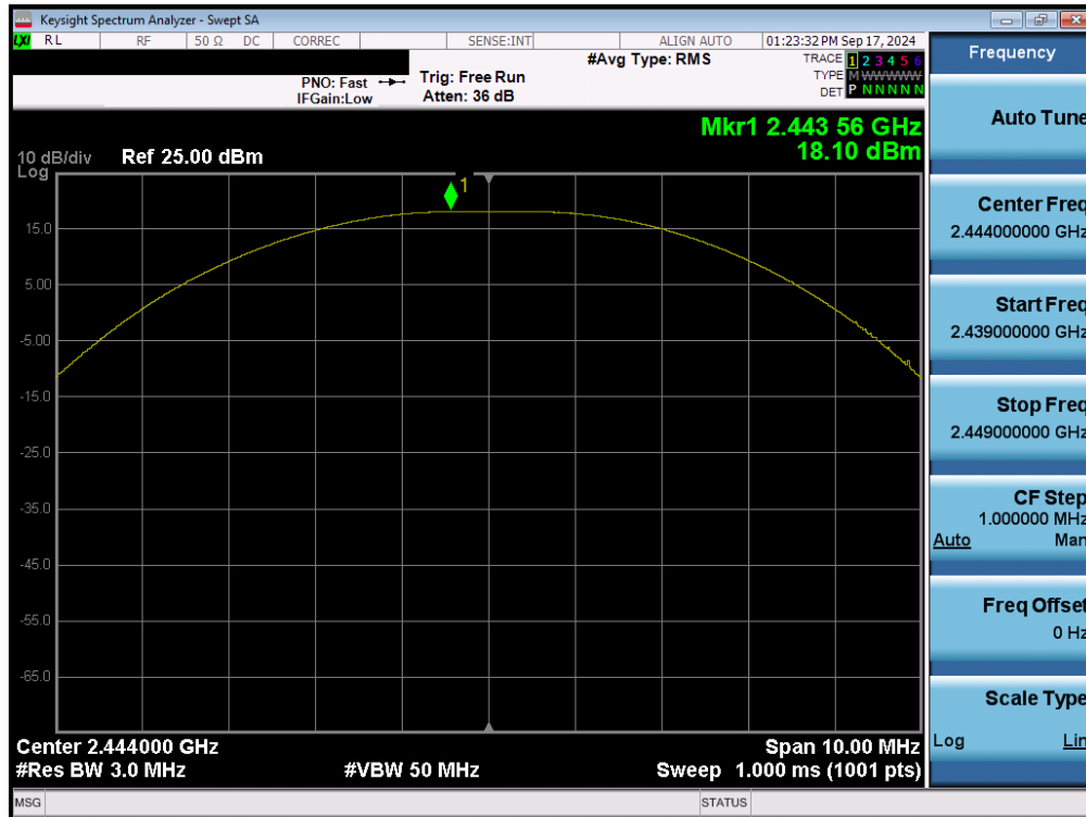
Plot 7-47. Peak Power Plot (Bluetooth (LE), 2Mbps – Ch. 19) – Ant 1
