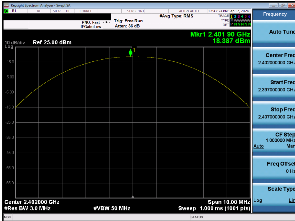
Plot 7-43. Peak Power Plot (Bluetooth (LE), 1Mbps – Ch. 0) – Ant 1
