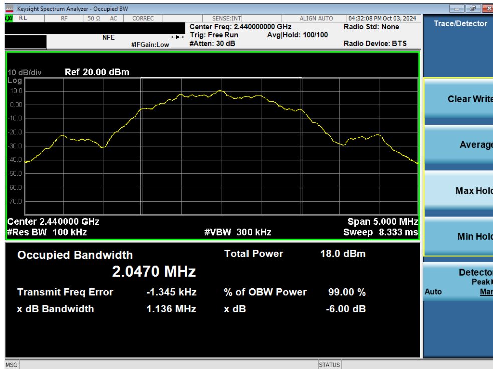
Plot 7-35. 6dB Bandwidth Plot (Bluetooth (LE), 2Mbps – Ch. 19) – Dual Ant 2
