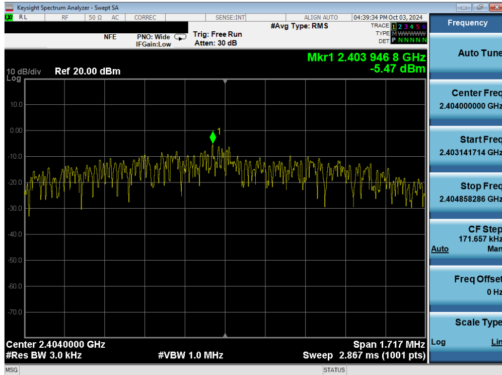
Plot 7-100. Power Spectral Density Plot (Bluetooth (LE), 2Mbps – Ch. 1) – Dual Ant 1
