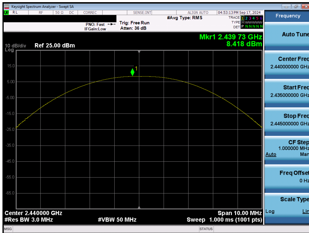
Plot 7-50. Peak Power Plot (Bluetooth (LE), 125kbps – Ch. 19) – Ant 2
