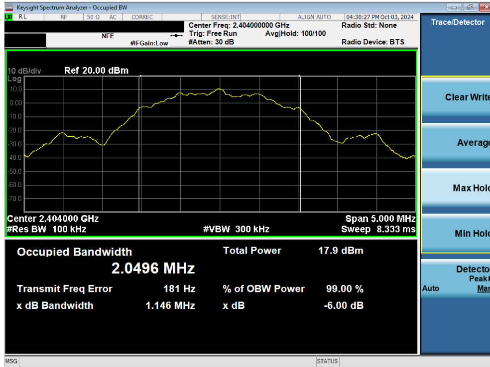
Plot 7-34. 6dB Bandwidth Plot (Bluetooth (LE), 2Mbps – Ch. 1) – Dual Ant 2
