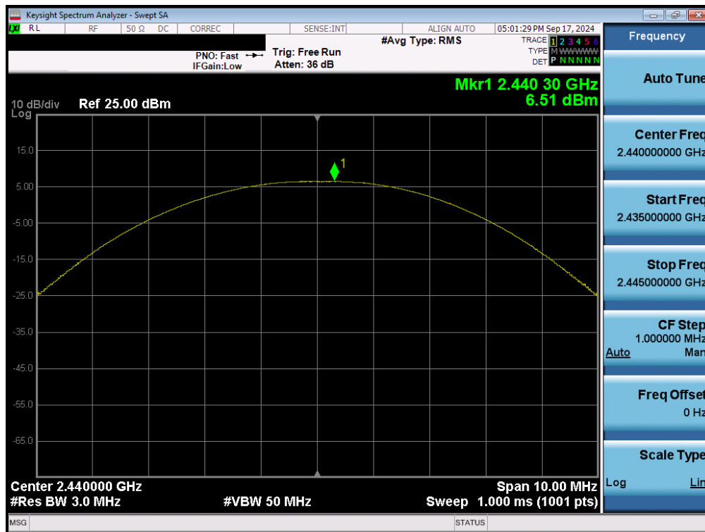
Plot 7-38. Peak Power Plot (Bluetooth (LE), 125kbps – Ch. 19) – Ant 1
