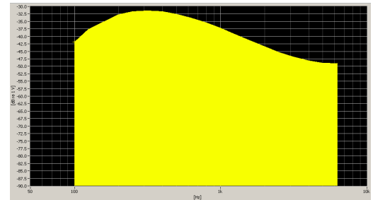
Figure 4-3 Spectral Characteristic of full P.50
