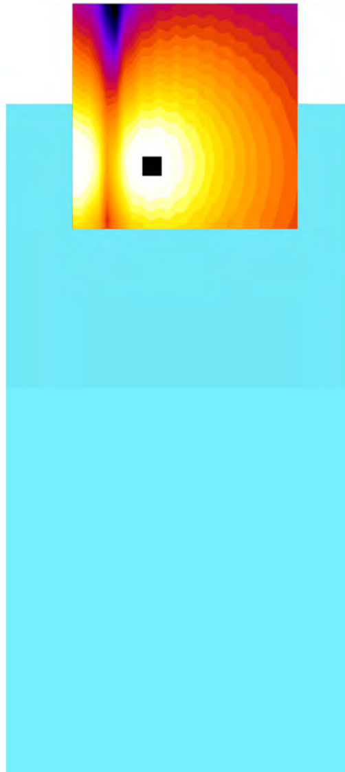
Figure 10-1 T-Coil Scan Overlay Magnetic Field Distributions
