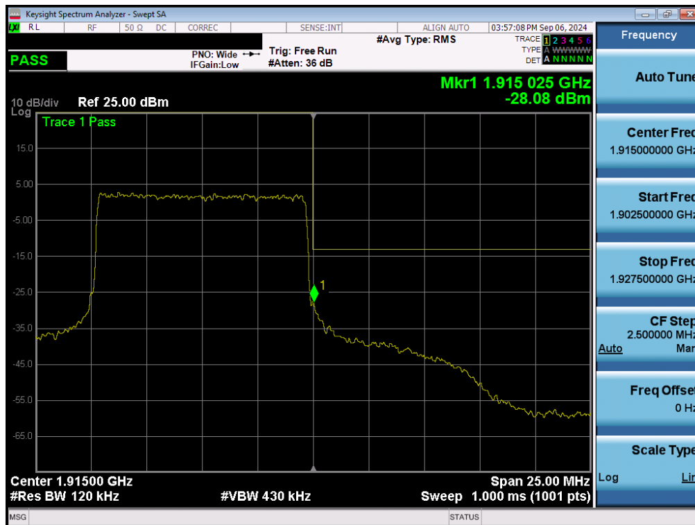
Plot 7-158. Upper Band Edge Plot (NR Band n25 - 10MHz QPSK - Full RB - Ant2)
