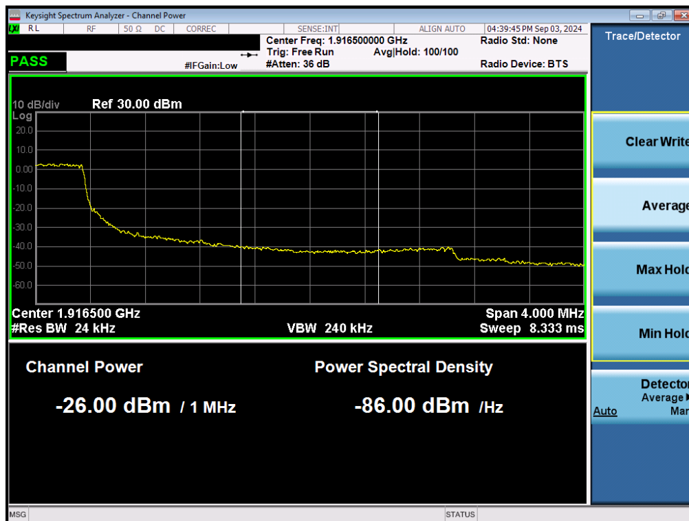
Plot 7-141. Extended Upper Band Edge Plot (LTE Band 25 - 3MHz QPSK – Full RB - Ant1)
