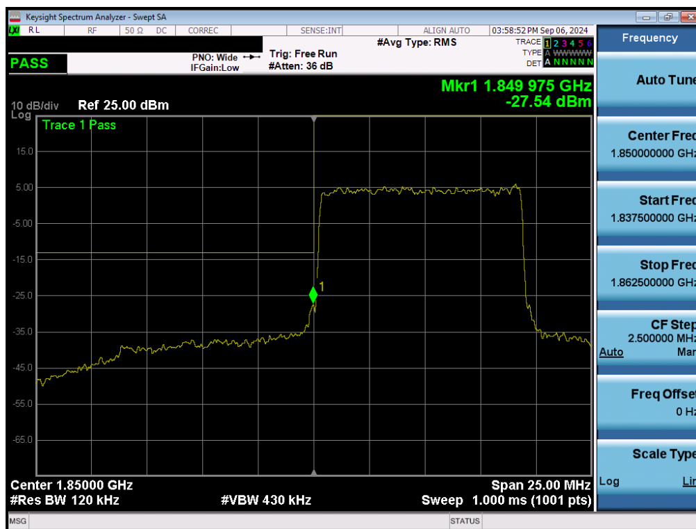
Plot 7-154. Lower Band Edge Plot (NR Band n25/2 - 10MHz QPSK – Full RB - Ant2)
