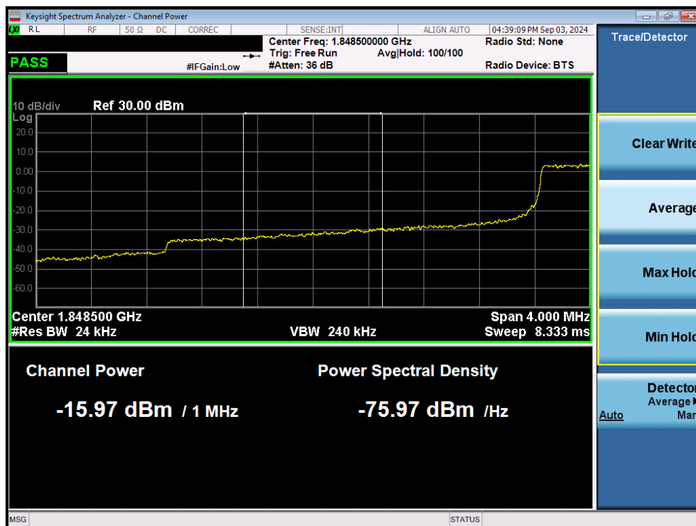
Plot 7-137. Extended Lower Band Edge Plot (LTE Band 25/2 - 3MHz QPSK – Full RB - Ant1)
