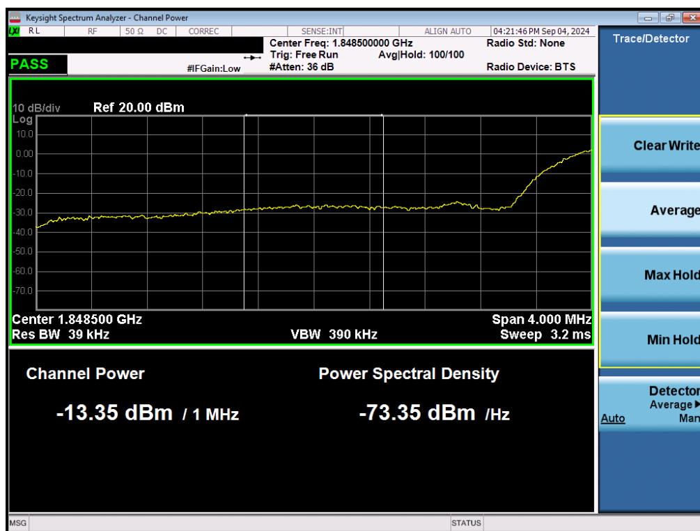
Plot 7-133. Extended Lower Band Edge Plot (WCDMA PCS – Ch. 9262 - Ant1)
