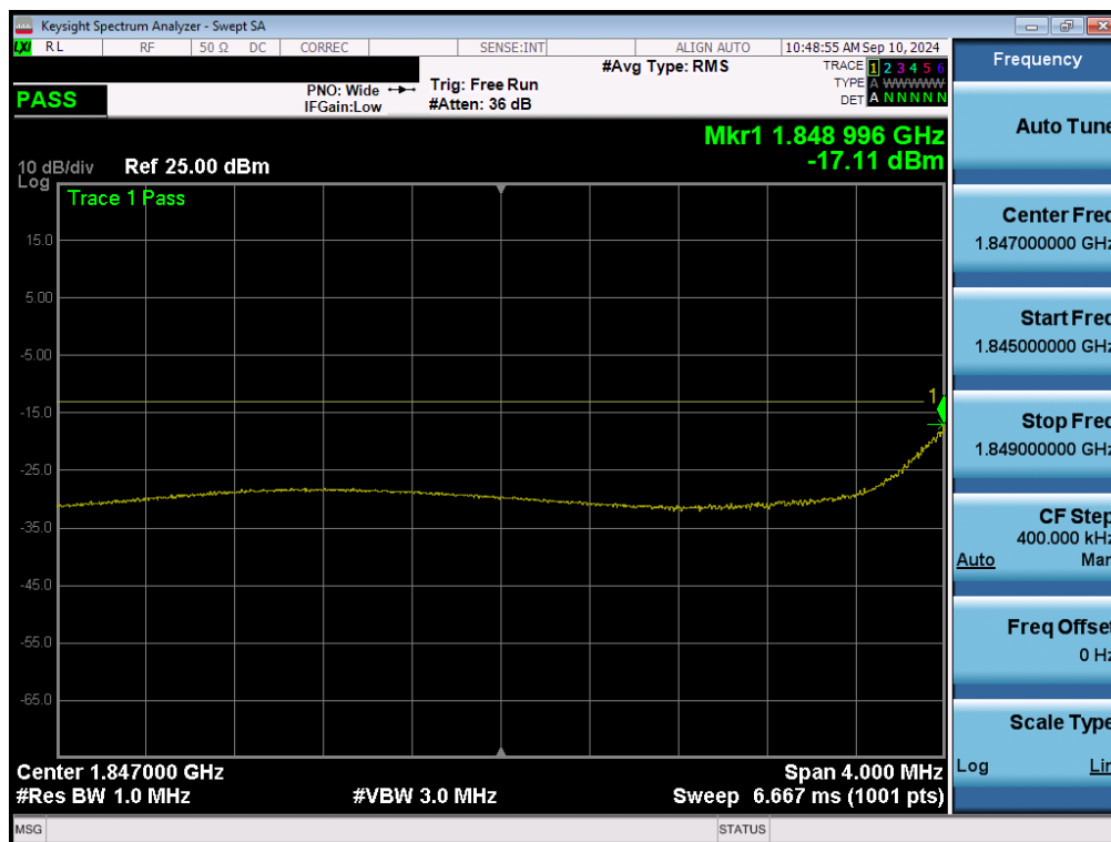
Plot 7-149. Extended Lower Band Edge Plot (NR Band n25/2 - 10MHz QPSK – Full RB - Ant1)
