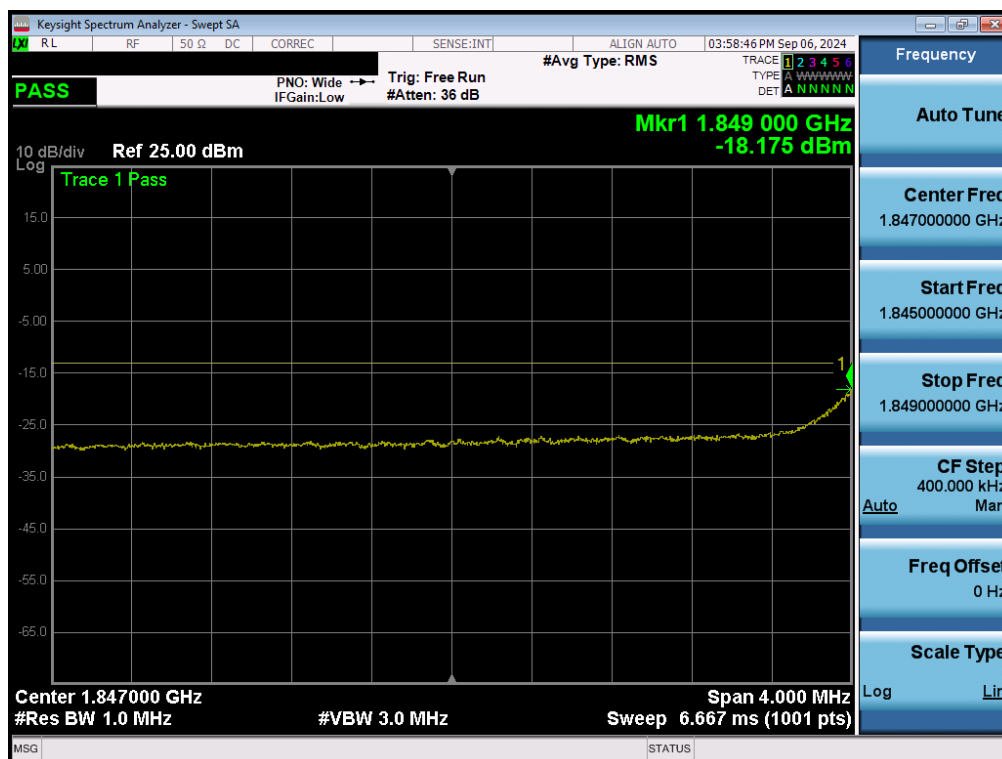
Plot 7-155. Extended Lower Band Edge Plot (NR Band n25/2 - 10MHz QPSK – Full RB - Ant2)
