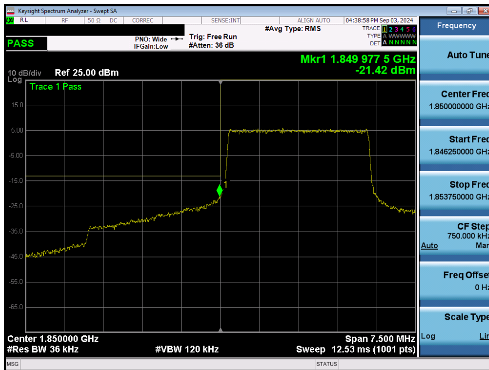
Plot 7-136. Lower Band Edge Plot (LTE Band 25/2 - 3MHz QPSK – Full RB - Ant1)
