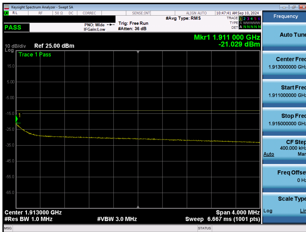
Plot 7-151. Extended Upper Band Edge Plot (NR Band n2 - 10MHz QPSK – Full RB - Ant1)
