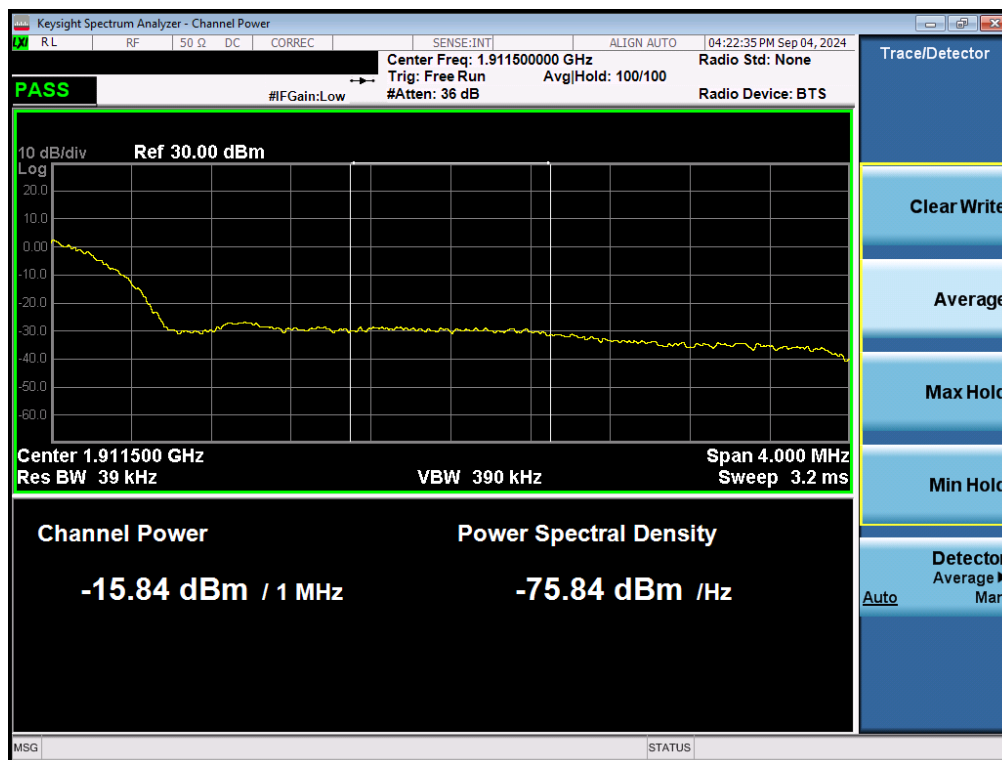
Plot 7-135. Extended Upper Band Edge Plot (WCDMA PCS – Ch. 9538 - Ant1)
