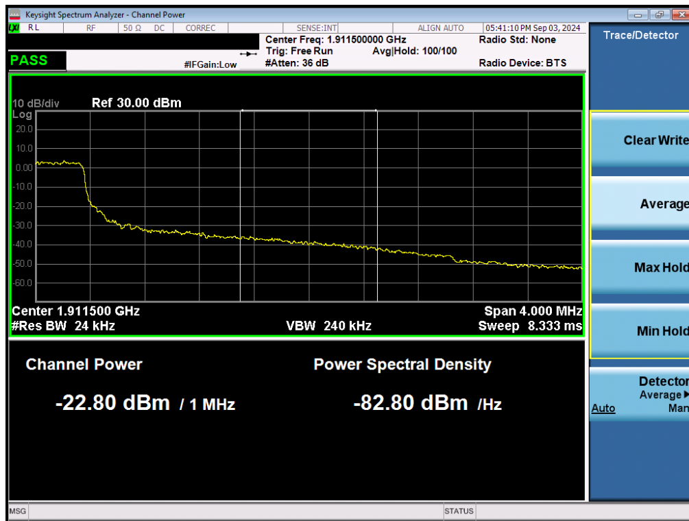
Plot 7-145. Extended Upper Band Edge Plot (LTE Band 2 - 3MHz QPSK – Full RB - Ant2)
