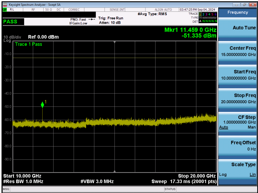
Plot 7-84. Conducted Spurious Plot (GPRS Ch. 810 - Ant1)
