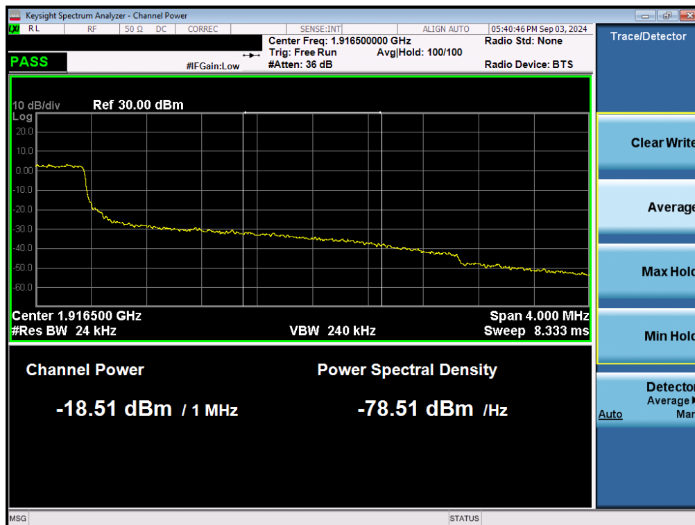
Plot 7-147. Extended Upper Band Edge Plot (LTE Band 25 - 3MHz QPSK – Full RB - Ant2)
