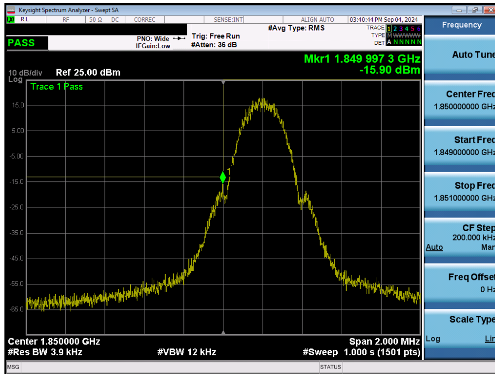
Plot 7-130. Lower Band Edge Plot (GPRS PCS – Ch. 512 - Ant1)
