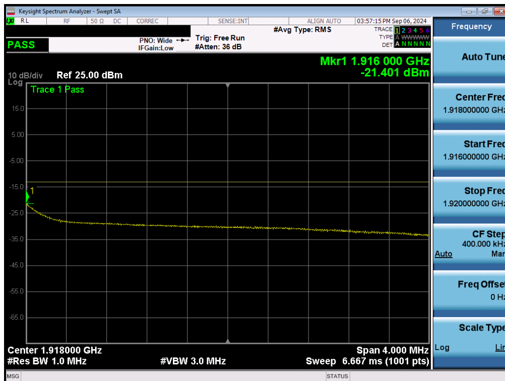
Plot 7-159. Extended Upper Band Edge Plot (NR Band n25 - 10MHz QPSK - Full RB - Ant2)
