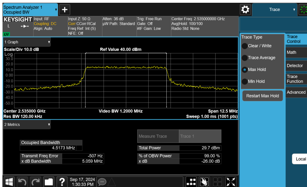
Plot 7-29. Occupied Bandwidth Plot (LTE Band 7 - 5MHz QPSK - Full RB - Ant F)
