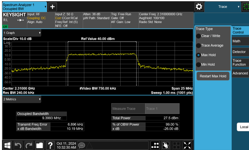
Plot 7-41. Occupied Bandwidth Plot (NR Band n30 - 10MHz 16-QAM - Full RB - Ant F)
