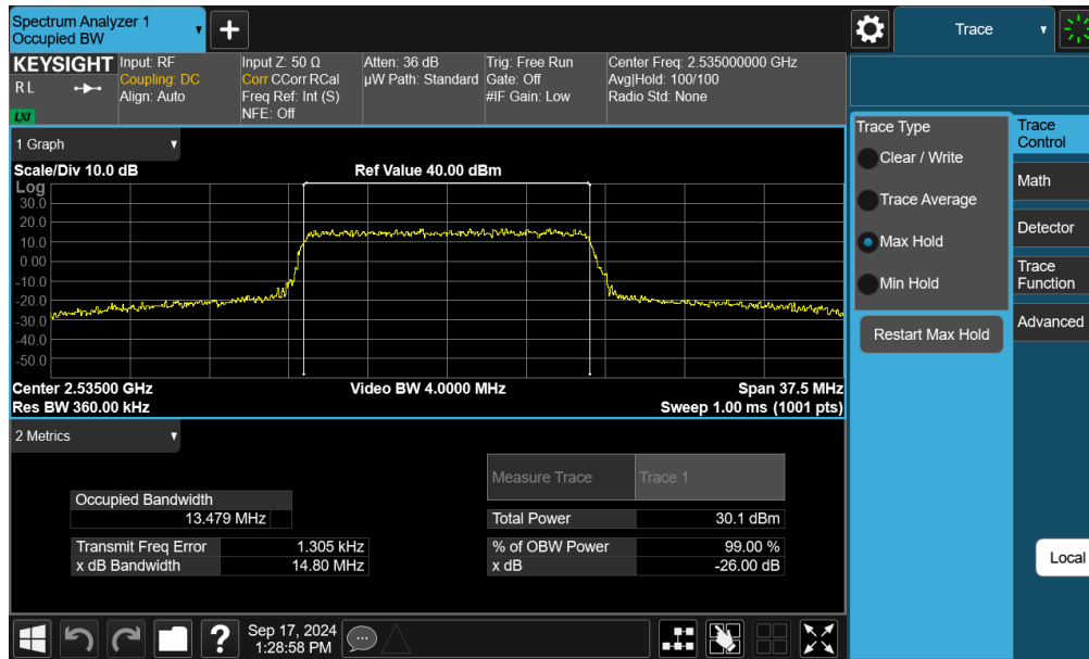
Plot 7-25. Occupied Bandwidth Plot (LTE Band 7 - 15MHz QPSK - Full RB - Ant F)
