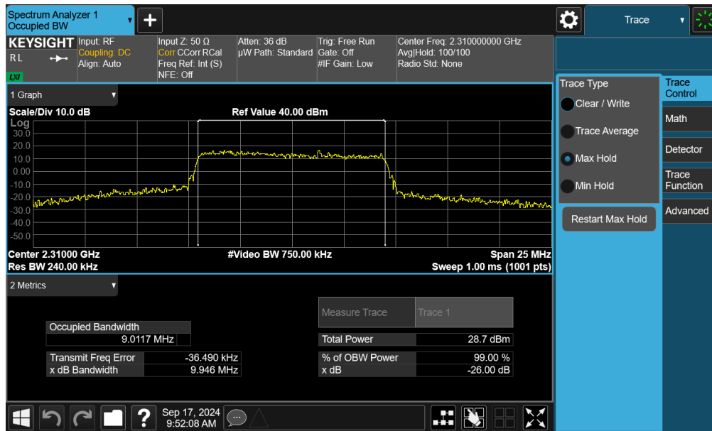
Plot 7-20. Occupied Bandwidth Plot (LTE Band 30 - 10MHz 16-QAM - Full RB - Ant F)
