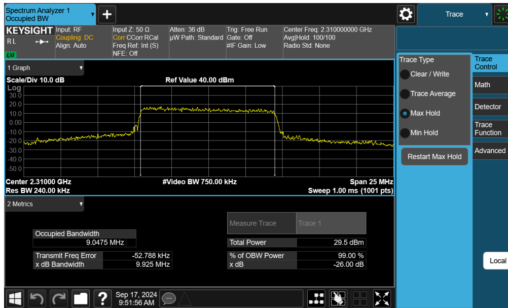
Plot 7-19. Occupied Bandwidth Plot (LTE Band 30 - 10MHz QPSK - Full RB - Ant F – Ant F)
