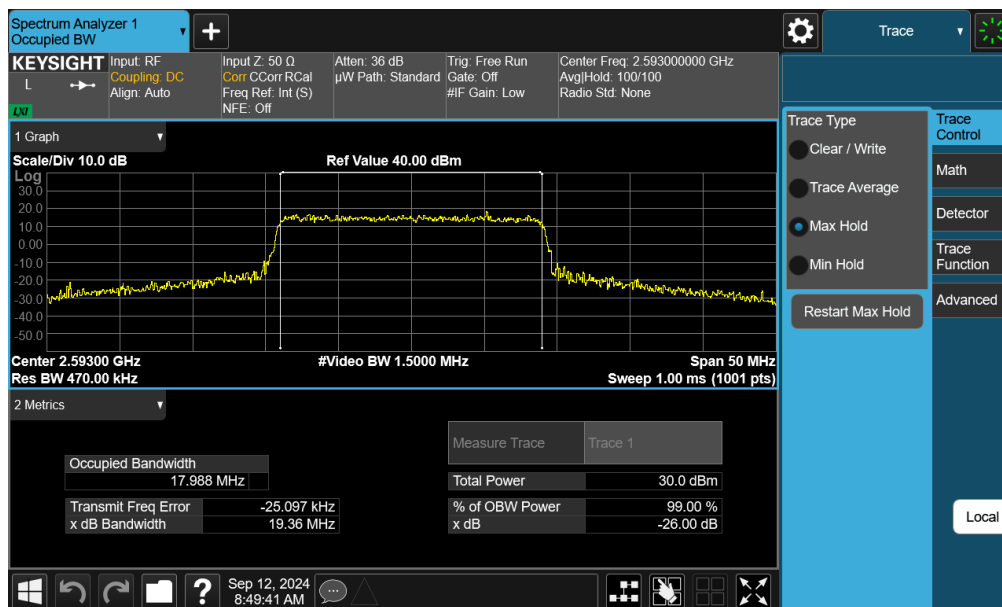
Plot 7-32. Occupied Bandwidth Plot (LTE Band 41(PC3)/38 - 20MHz 16-QAM - Full RB - Ant F)
