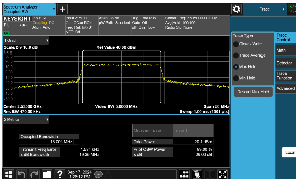
Plot 7-24. Occupied Bandwidth Plot (LTE Band 7 - 20MHz 16-QAM - Full RB - Ant F)
