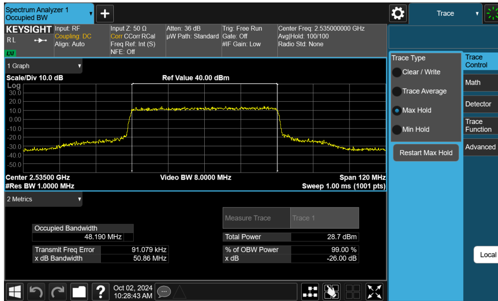
Plot 7-47. Occupied Bandwidth Plot (NR Band n7 - 50MHz 16-QAM - Full RB - Ant F)
