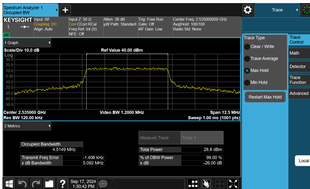
Plot 7-30. Occupied Bandwidth Plot (LTE Band 7 - 5MHz 16-QAM - Full RB - Ant F)
