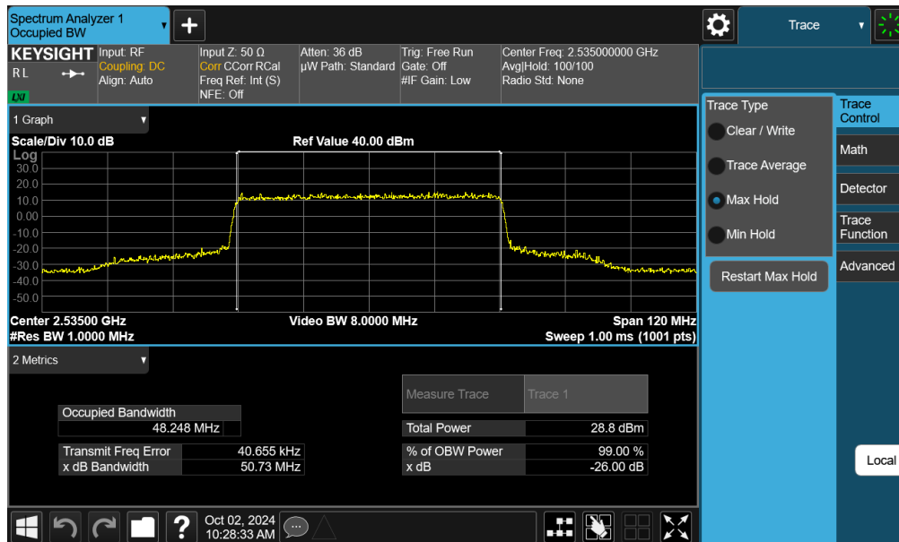
Plot 7-46. Occupied Bandwidth Plot (NR Band n7 - 50MHz QPSK - Full RB - Ant F)
