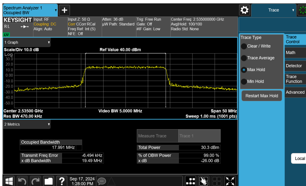
Plot 7-23. Occupied Bandwidth Plot (LTE Band 7 - 20MHz QPSK - Full RB - Ant F)
