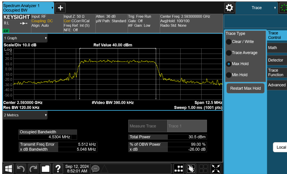
Plot 7-37. Occupied Bandwidth Plot (LTE Band 41(PC3)/38 - 5MHz QPSK - Full RB - Ant F)
