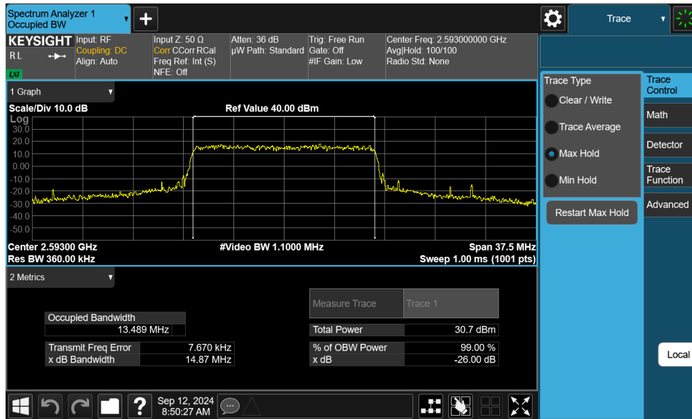
Plot 7-33. Occupied Bandwidth Plot (LTE Band 41(PC3)/38 - 15MHz QPSK - Full RB - Ant F)
