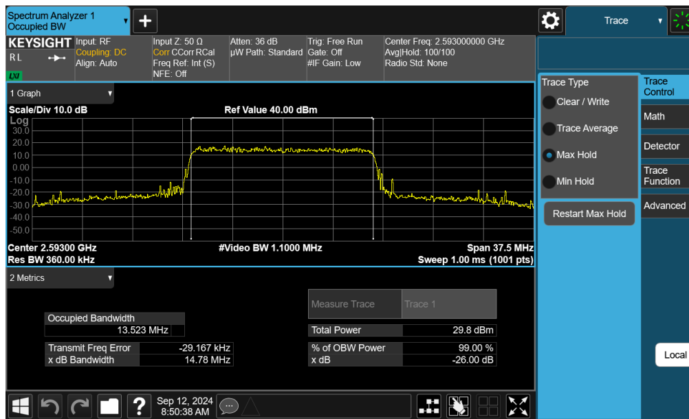
Plot 7-34. Occupied Bandwidth Plot (LTE Band 41(PC3)/38 - 15MHz 16-QAM - Full RB - Ant F)
