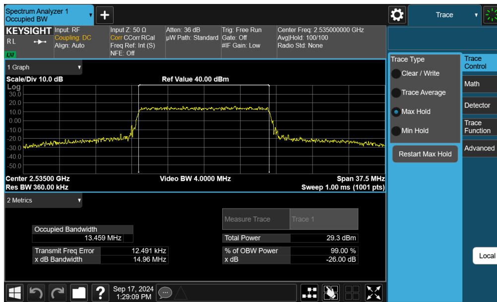
Plot 7-26. Occupied Bandwidth Plot (LTE Band 7 - 15MHz 16-QAM - Full RB - Ant F)
