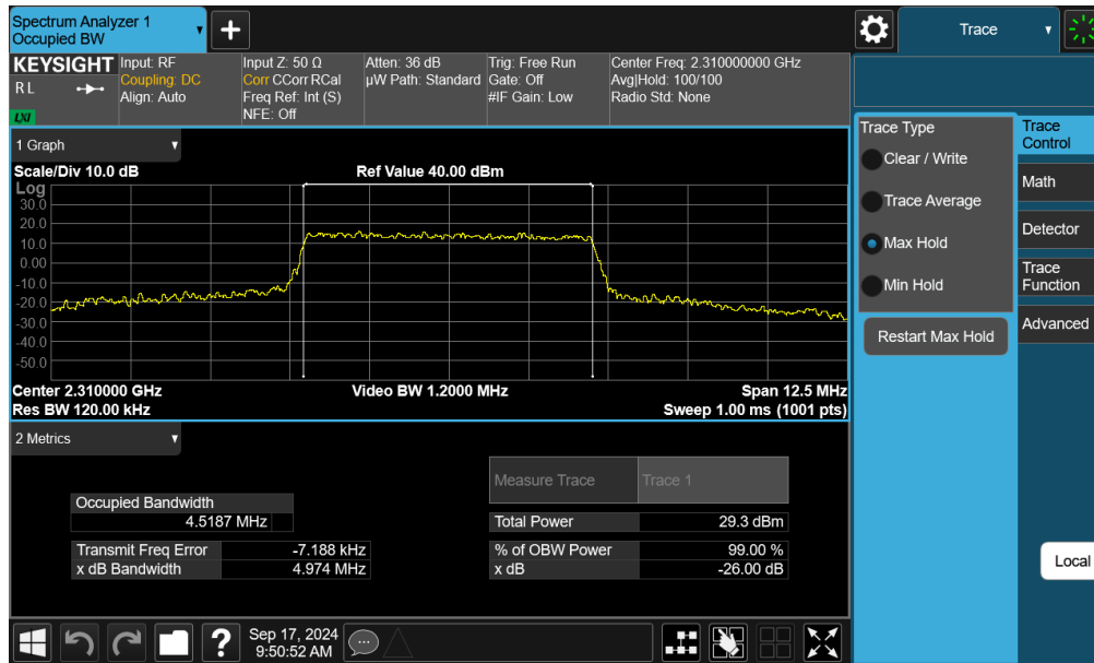
Plot 7-21. Occupied Bandwidth Plot (LTE Band 30 - 5MHz QPSK - Full RB - Ant F)
