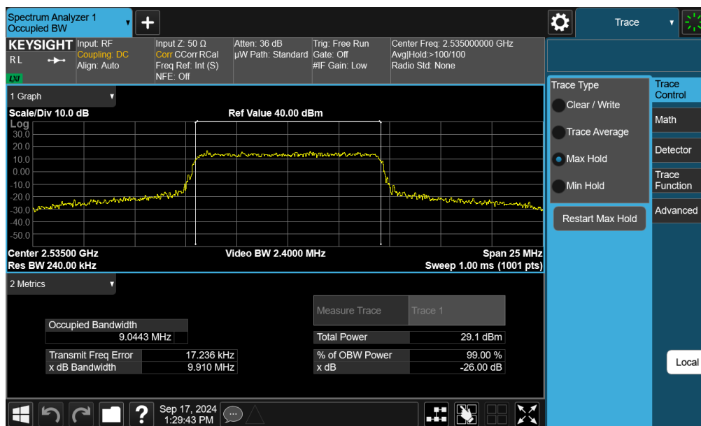
Plot 7-28. Occupied Bandwidth Plot (LTE Band 7 - 10MHz 16-QAM - Full RB - Ant F)
