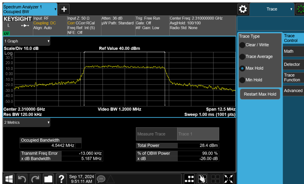
Plot 7-22. Occupied Bandwidth Plot (LTE Band 30 - 5MHz 16-QAM - Full RB - Ant F)
