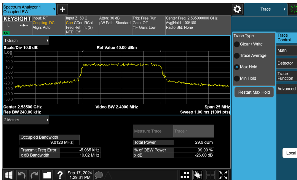
Plot 7-27. Occupied Bandwidth Plot (LTE Band 7 - 10MHz QPSK - Full RB - Ant F)
