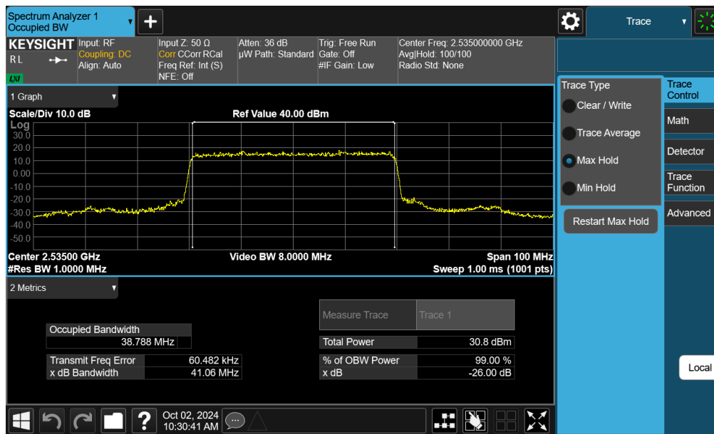
Plot 7-48. Occupied Bandwidth Plot (NR Band n7 - 40MHz \pi/2 BPSK - Full RB - Ant F)
