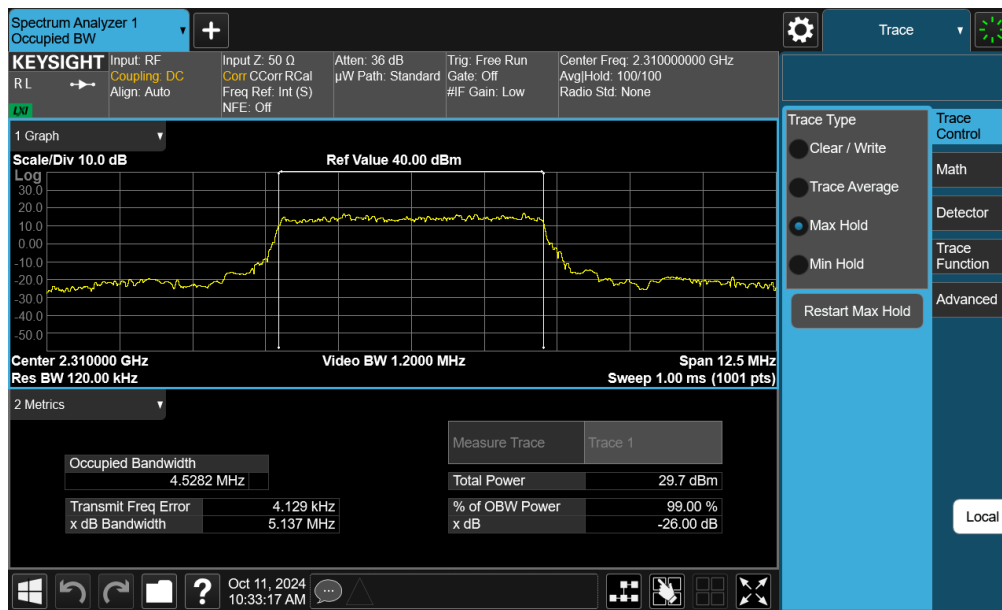
Plot 7-42. Occupied Bandwidth Plot (NR Band n30 - 5MHz \pi/2 BPSK - Full RB - Ant F)
