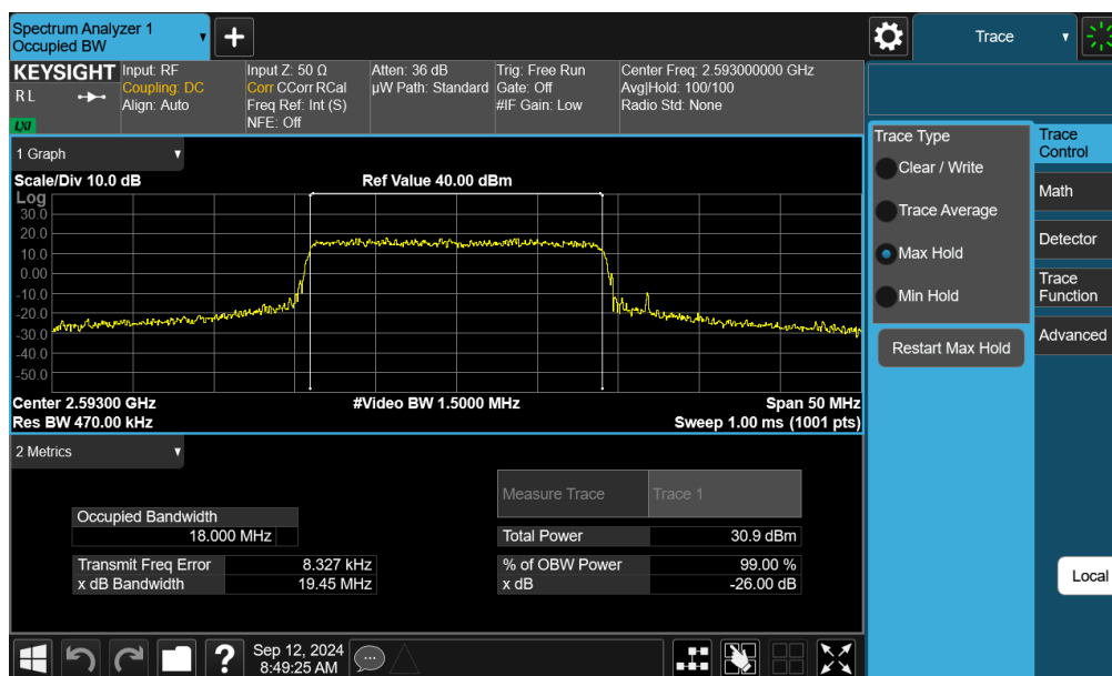
Plot 7-31. Occupied Bandwidth Plot (LTE Band 41(PC3)/38 - 20MHz QPSK - Full RB - Ant F)
