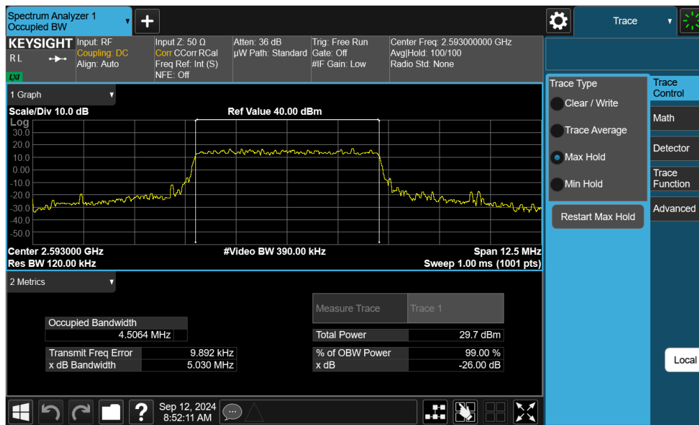
Plot 7-38. Occupied Bandwidth Plot (LTE Band 41(PC3)/38 - 5MHz 16-QAM - Full RB - Ant F)
