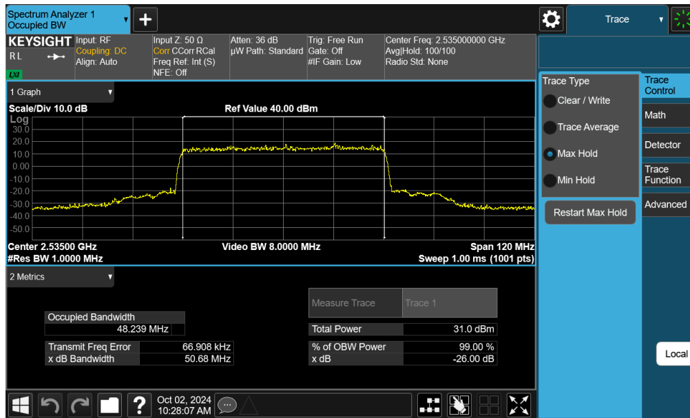
Plot 7-45. Occupied Bandwidth Plot (NR Band n7 - 50MHz \pi/2 BPSK - Full RB - Ant F)
