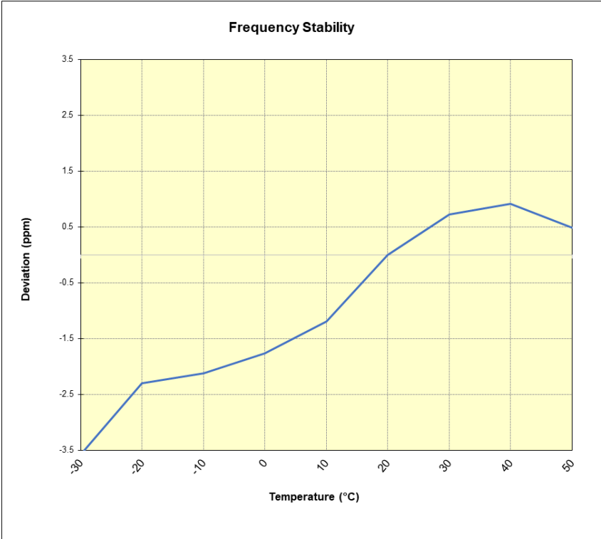
Plot 7-382. NR Band n30 Frequency Stability Chart
