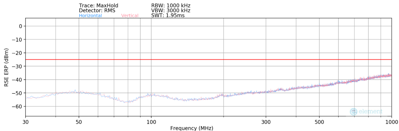
Plot 7-376. Radiated Spurious Plot (NR Band n41 – Ant E)
