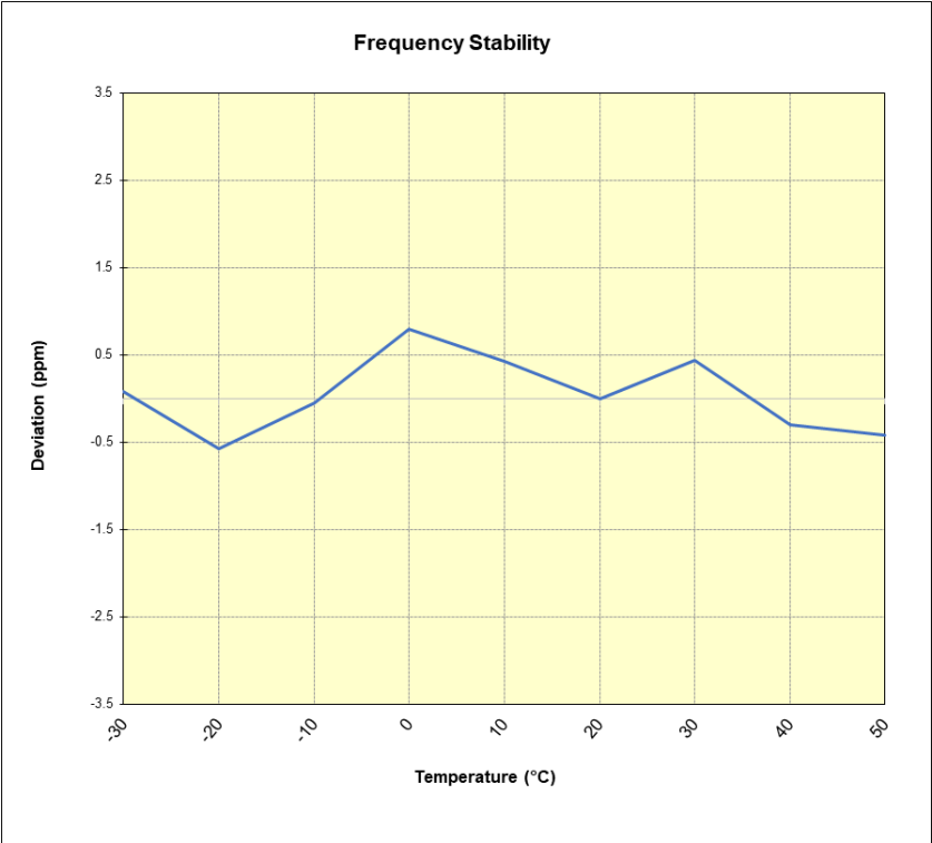
Plot 7-379. LTE Band 30 Frequency Stability Chart
