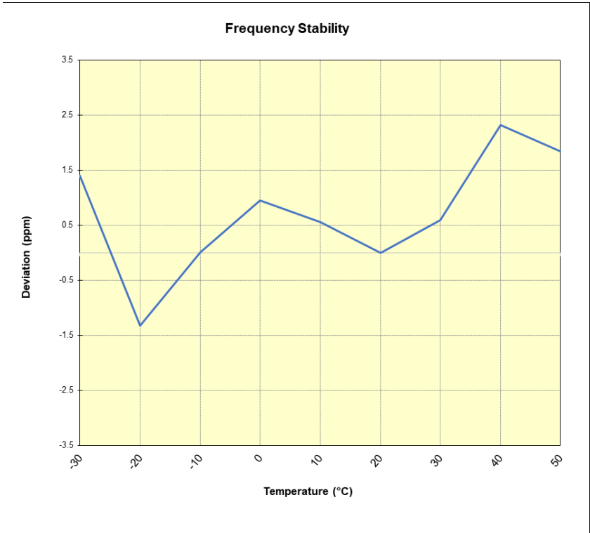
Plot 7-381. LTE Band 41(PC2) Frequency Stability Chart
