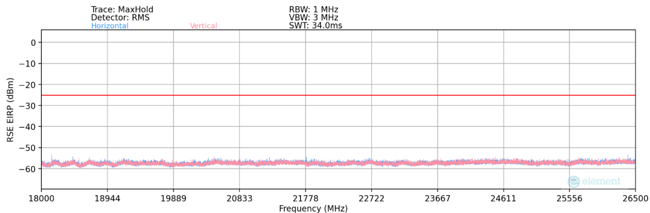
Plot 7-378. Radiated Spurious Plot (NR Band n41 – Ant E)
