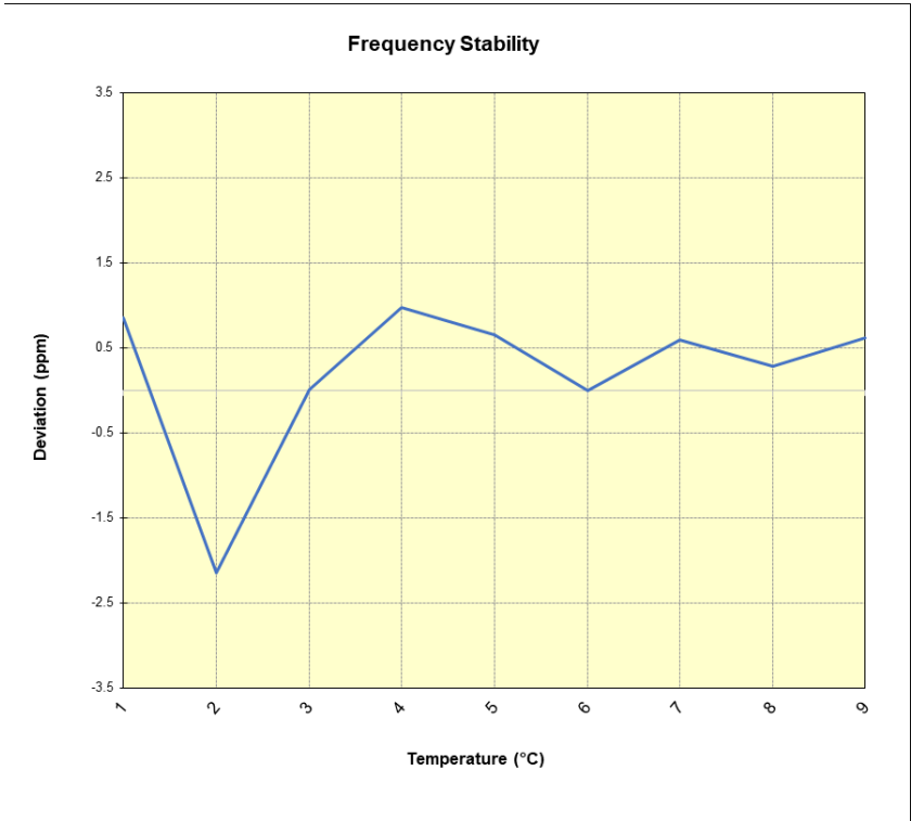
Plot 7-380. LTE Band 7 Frequency Stability Chart
