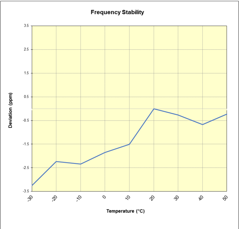
Plot 7-383. NR Band n7 Frequency Stability Chart
