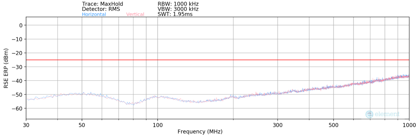
Plot 7-373. Radiated Spurious Plot (NR Band n41 – Ant D)
