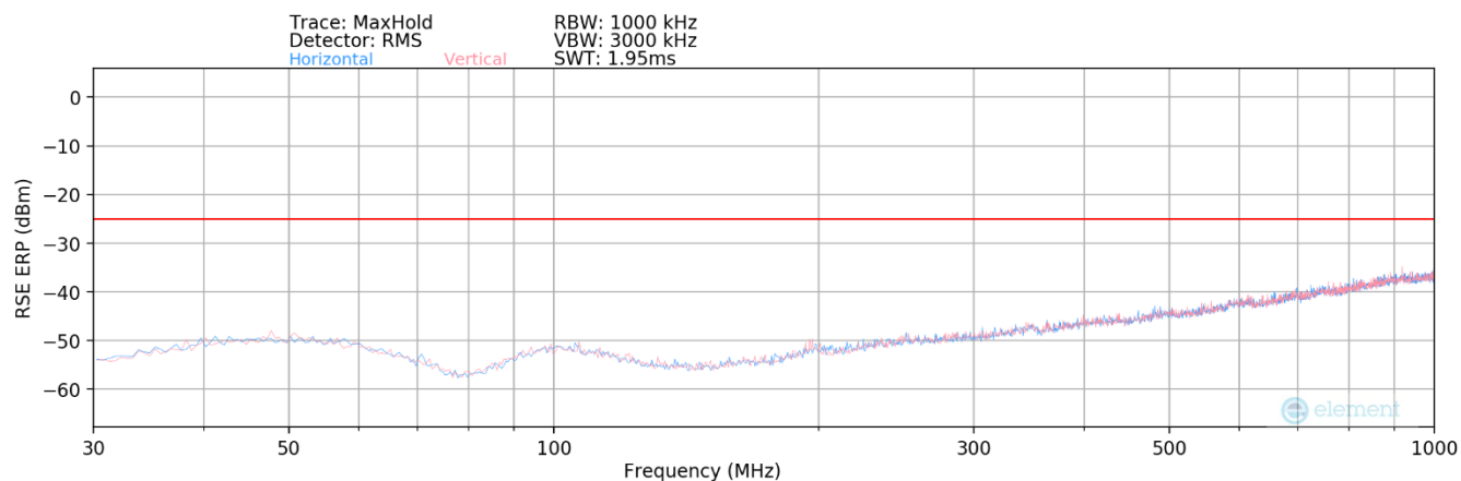
Plot 7-364. Radiated Spurious Plot (NR Band n41 – Ant F)
