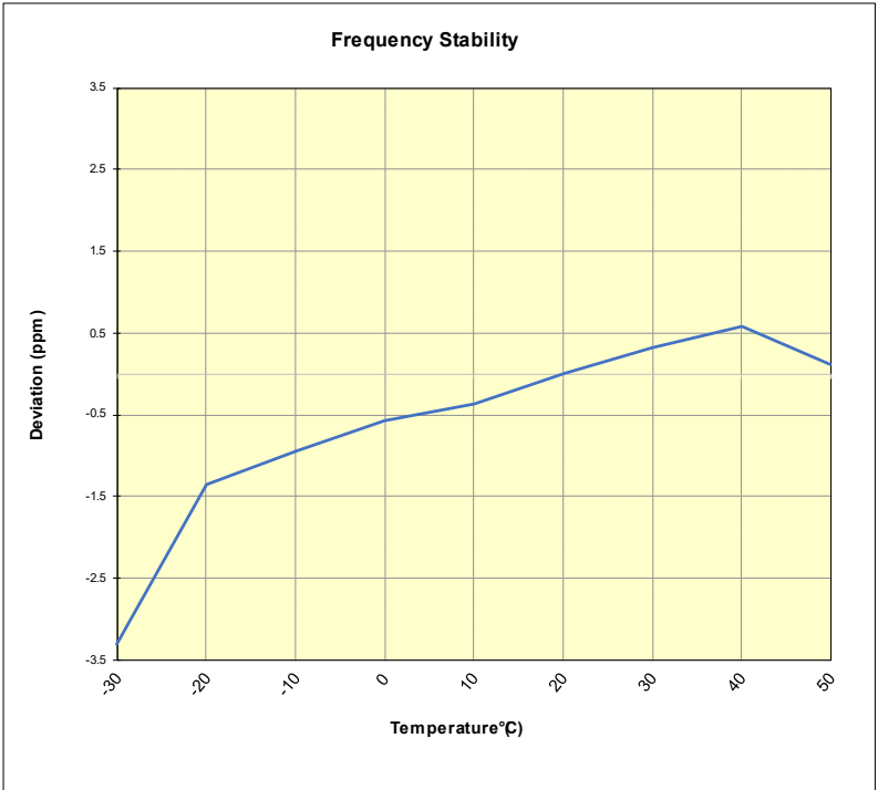
Plot 7-384. NR Band n7 Frequency Stability Chart
