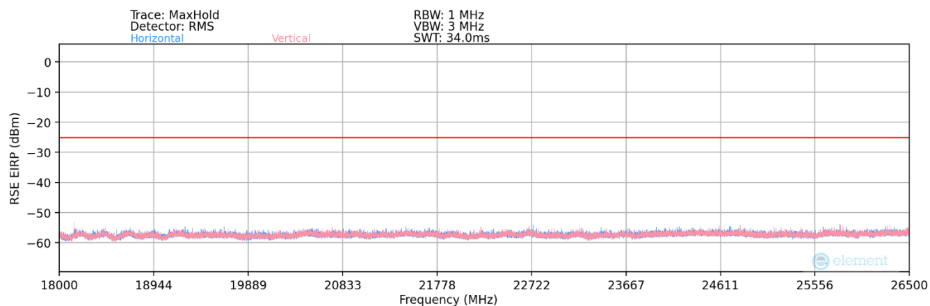
Plot 7-366. Radiated Spurious Plot (NR Band n41 – Ant F)
