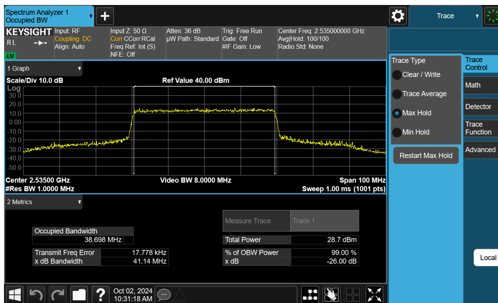
Plot 7-50. Occupied Bandwidth Plot (NR Band n7 - 40MHz 16-QAM - Full RB - Ant F)
