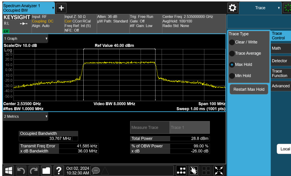
Plot 7-53. Occupied Bandwidth Plot (NR Band n7 - 35MHz 16-QAM - Full RB - Ant F)
