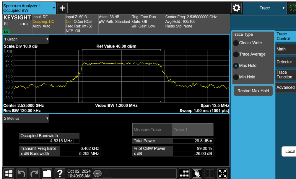
Plot 7-69. Occupied Bandwidth Plot (NR Band n7 - 5MHz \pi/2 BPSK - Full RB - Ant F)
