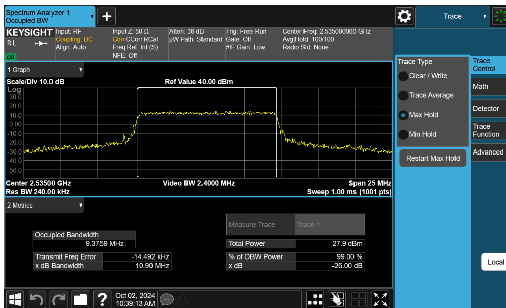
Plot 7-68. Occupied Bandwidth Plot (NR Band n7 - 10MHz 16-QAM - Full RB - Ant F)
