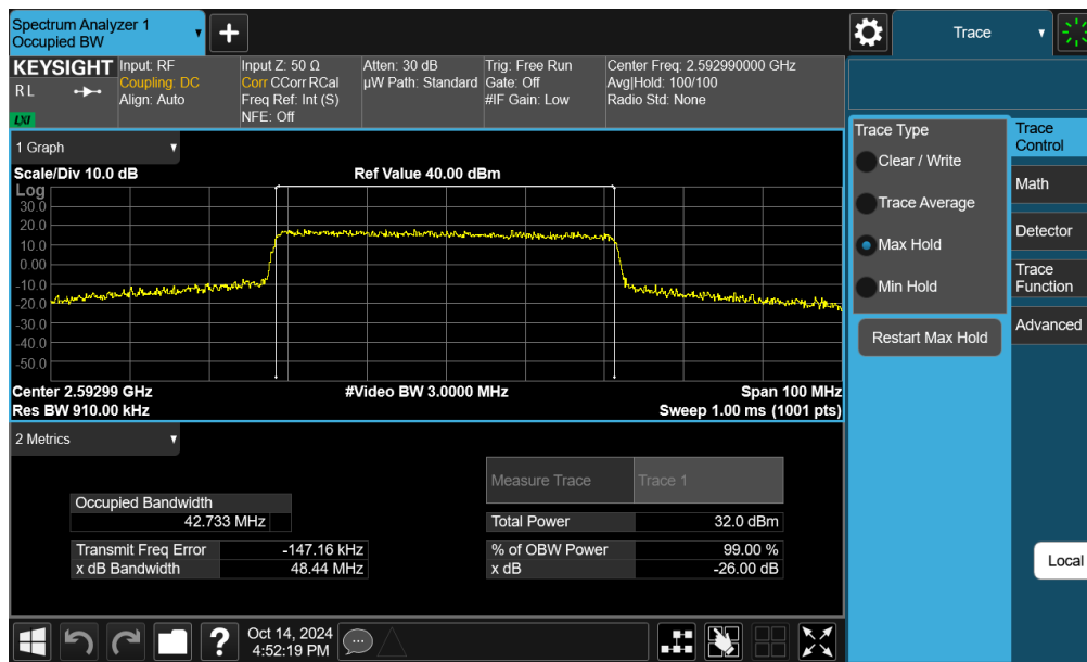
Plot 7-91. Occupied Bandwidth Plot (NR Band n41 - 45MHz QPSK - Full RB - Ant F)
