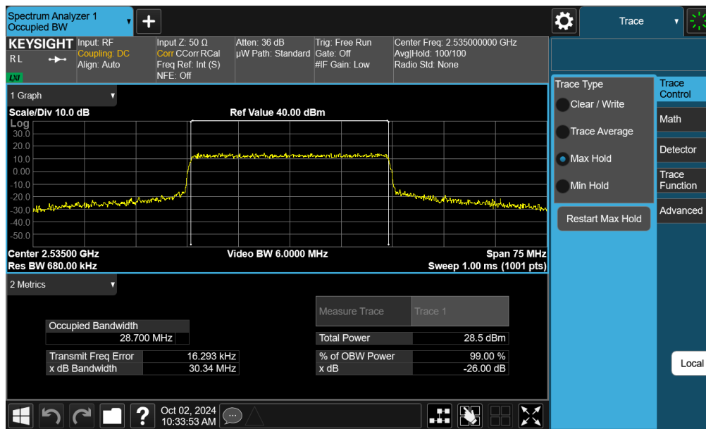
Plot 7-56. Occupied Bandwidth Plot (NR Band n7 - 30MHz 16-QAM - Full RB - Ant F)
