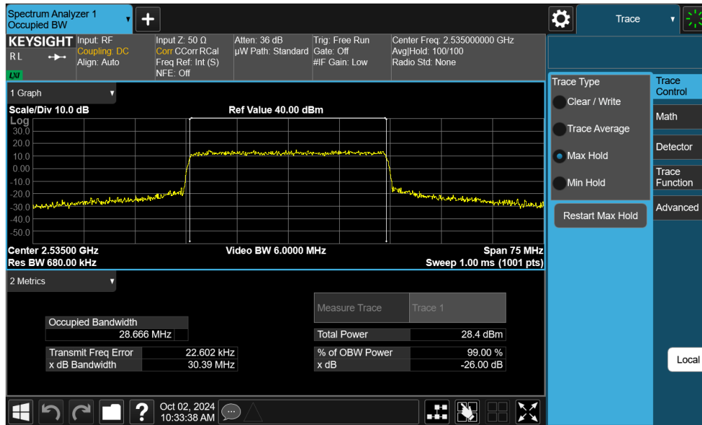
Plot 7-55. Occupied Bandwidth Plot (NR Band n7 - 30MHz QPSK - Full RB - Ant F)
