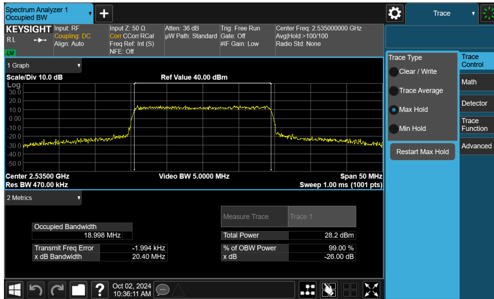
Plot 7-61. Occupied Bandwidth Plot (NR Band n7 - 20MHz QPSK - Full RB - Ant F)
