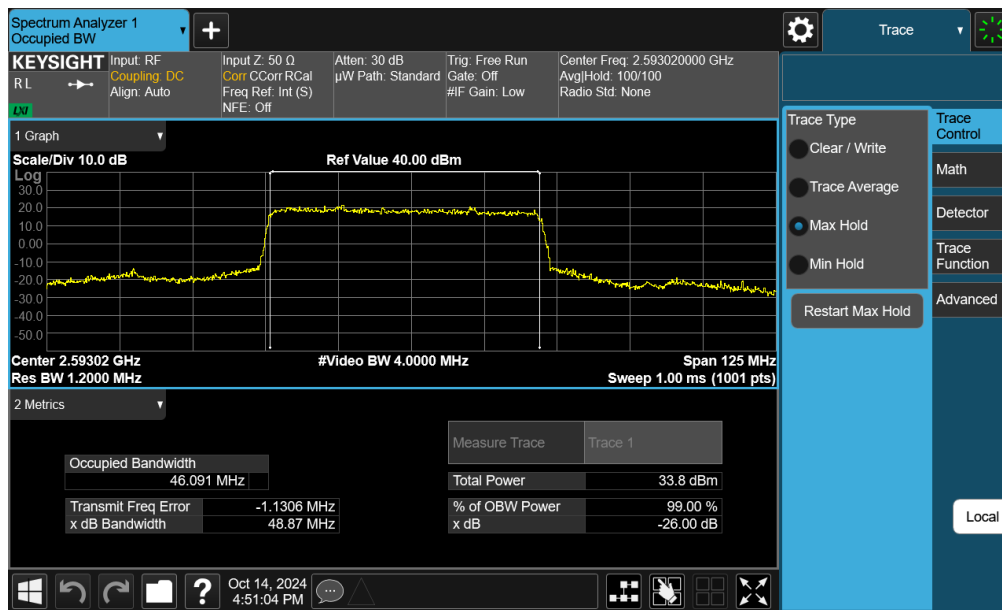
Plot 7-87. Occupied Bandwidth Plot (NR Band n41 - 50MHz \pi/2 BPSK - Full RB - Ant F)
