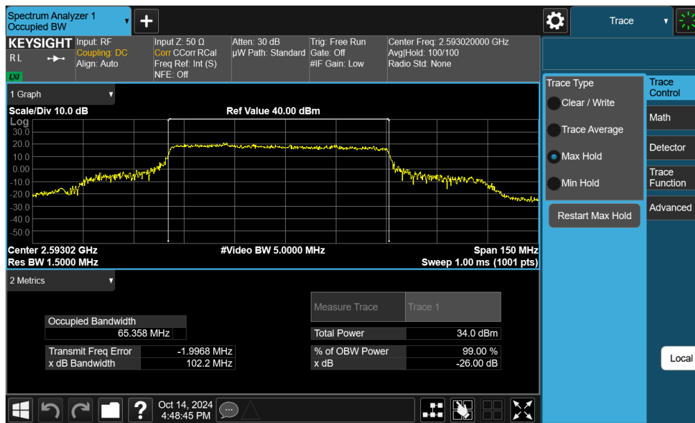
Plot 7-81. Occupied Bandwidth Plot (NR Band n41 - 70MHz 7π/2 BPSK - Full RB - Ant F)
