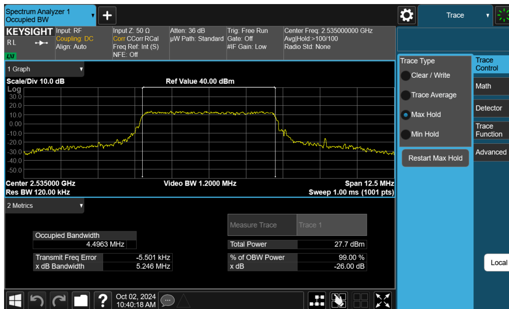
Plot 7-70. Occupied Bandwidth Plot (NR Band n7 - 5MHz QPSK - Full RB - Ant F)
