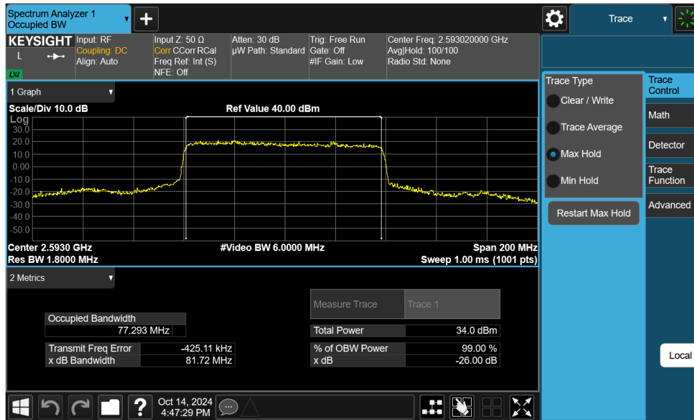
Plot 7-78. Occupied Bandwidth Plot (NR Band n41 - 80MHz \pi/2 BPSK - Full RB - Ant F)
