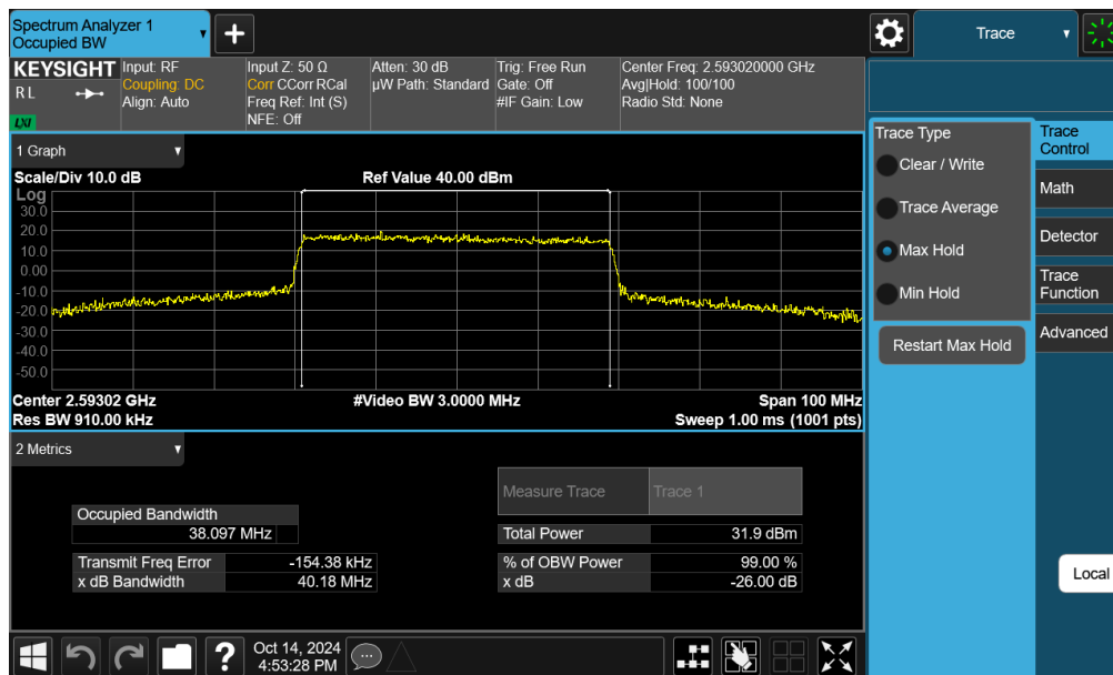
Plot 7-95. Occupied Bandwidth Plot (NR Band n41 - 40MHz 16-QAM - Full RB - Ant F)
