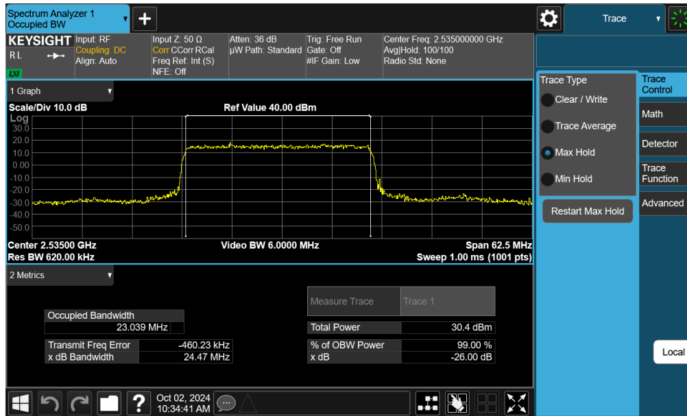
Plot 7-57. Occupied Bandwidth Plot (NR Band n7 - 25MHz \pi/2 BPSK - Full RB - Ant F)
