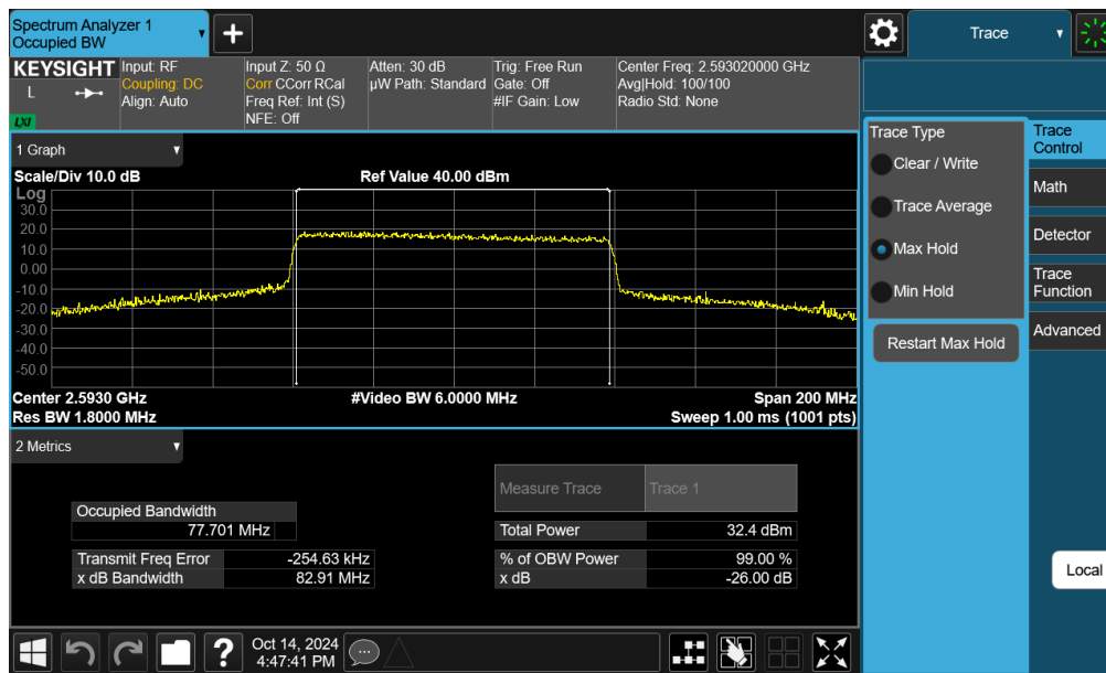
Plot 7-79. Occupied Bandwidth Plot (NR Band n41 - 80MHz QPSK - Full RB - Ant F)
