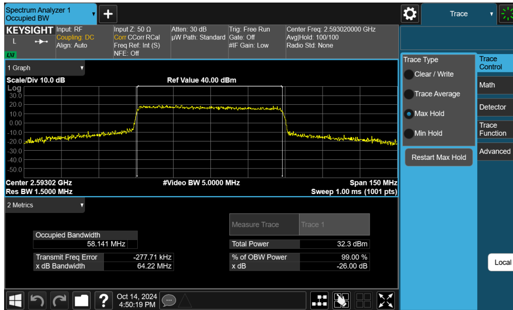
Plot 7-86. Occupied Bandwidth Plot (NR Band n41 - 60MHz 16-QAM - Full RB - Ant F)
