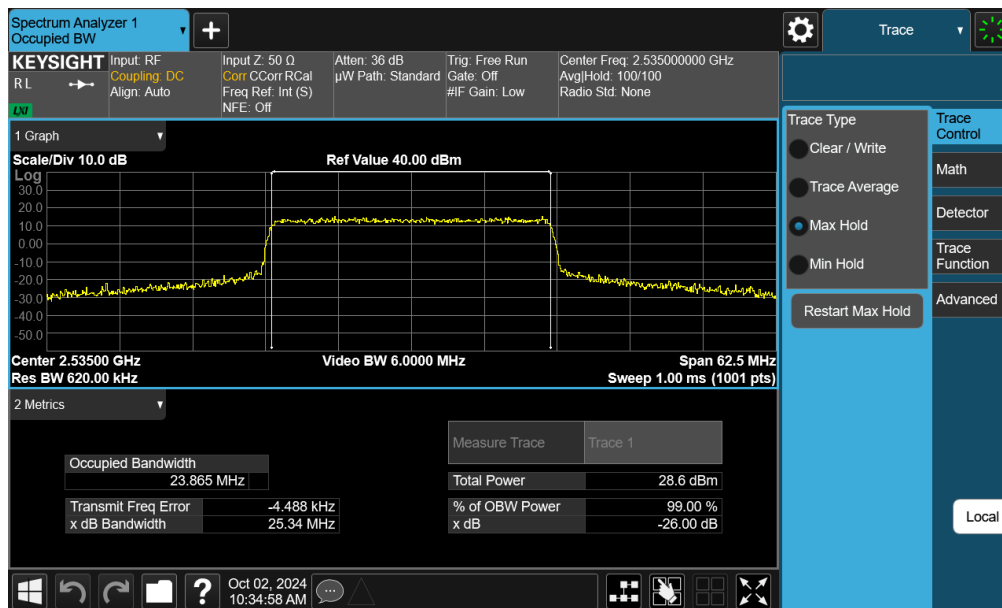
Plot 7-58. Occupied Bandwidth Plot (NR Band n7 - 25MHz QPSK - Full RB - Ant F)
