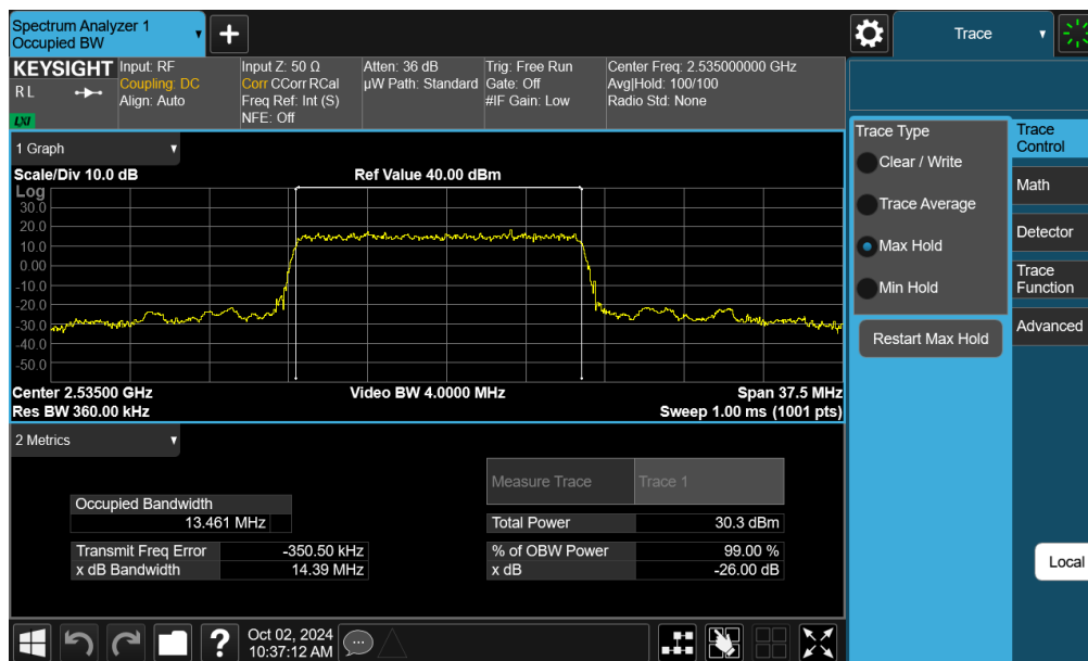
Plot 7-63. Occupied Bandwidth Plot (NR Band n7 - 15MHz \pi/2 BPSK - Full RB - Ant F)
