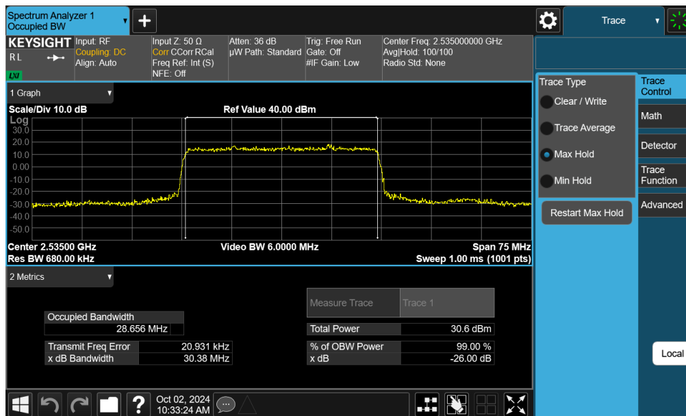
Plot 7-54. Occupied Bandwidth Plot (NR Band n7 - 30MHz \pi/2 BPSK - Full RB - Ant F)
