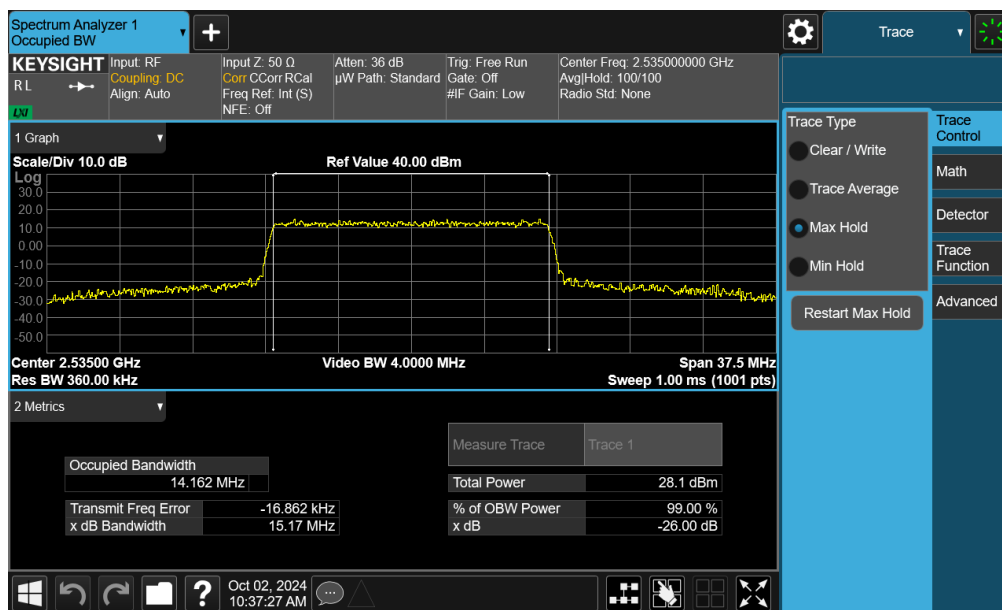
Plot 7-64. Occupied Bandwidth Plot (NR Band n7 - 15MHz QPSK - Full RB - Ant F)
