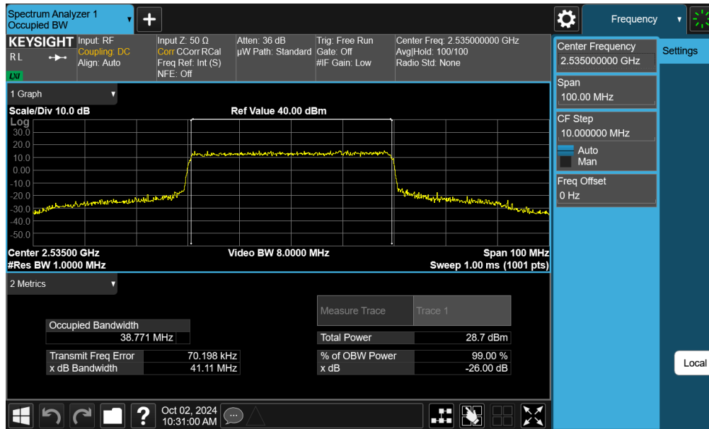
Plot 7-49. Occupied Bandwidth Plot (NR Band n7 - 40MHz QPSK - Full RB - Ant F)
