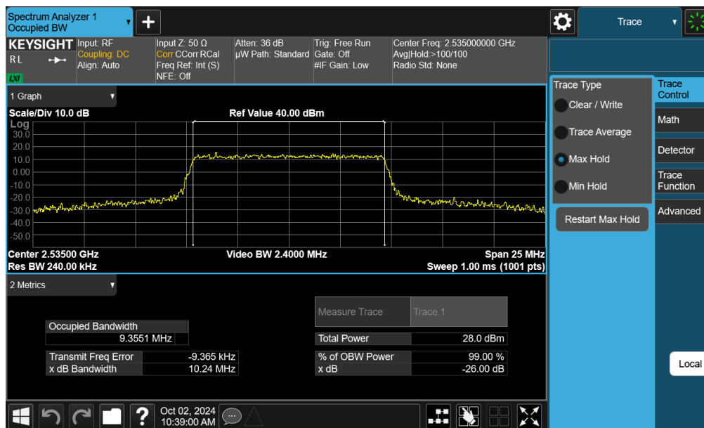
Plot 7-67. Occupied Bandwidth Plot (NR Band n7 - 10MHz QPSK - Full RB - Ant F)
