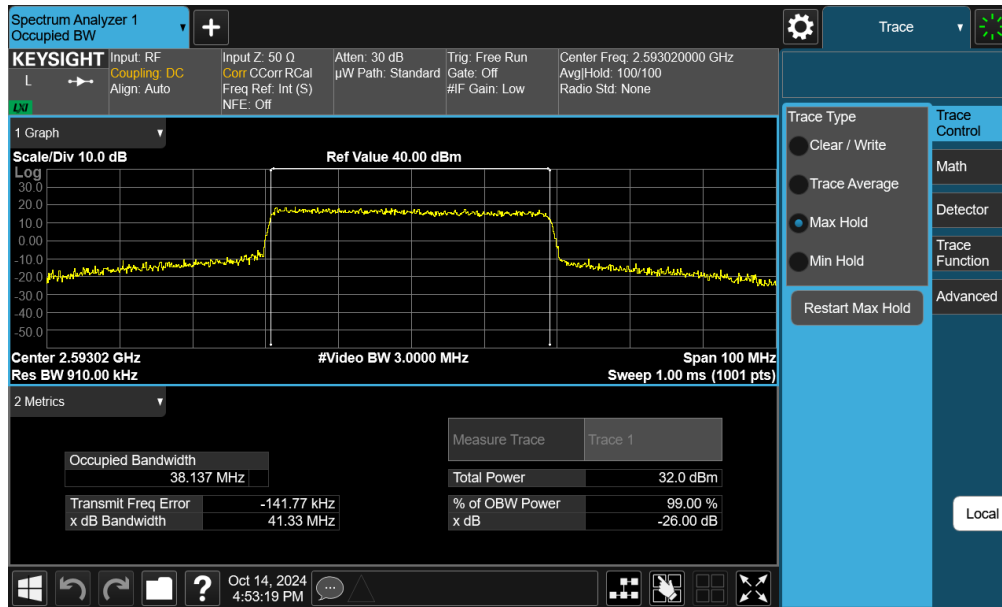
Plot 7-94. Occupied Bandwidth Plot (NR Band n41 - 40MHz QPSK - Full RB - Ant F)
