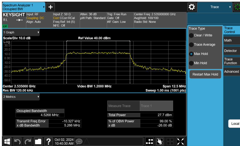
Plot 7-71. Occupied Bandwidth Plot (NR Band n7 - 5MHz 16-QAM - Full RB - Ant F)
