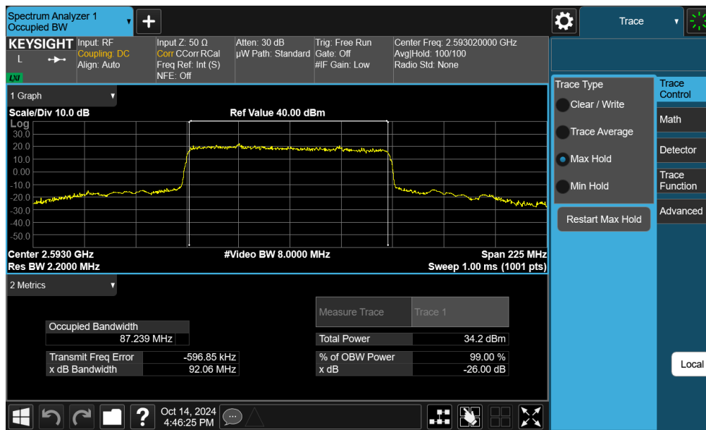
Plot 7-75. Occupied Bandwidth Plot (NR Band n41 - 90MHz \pi/2 BPSK - Full RB - Ant F)
