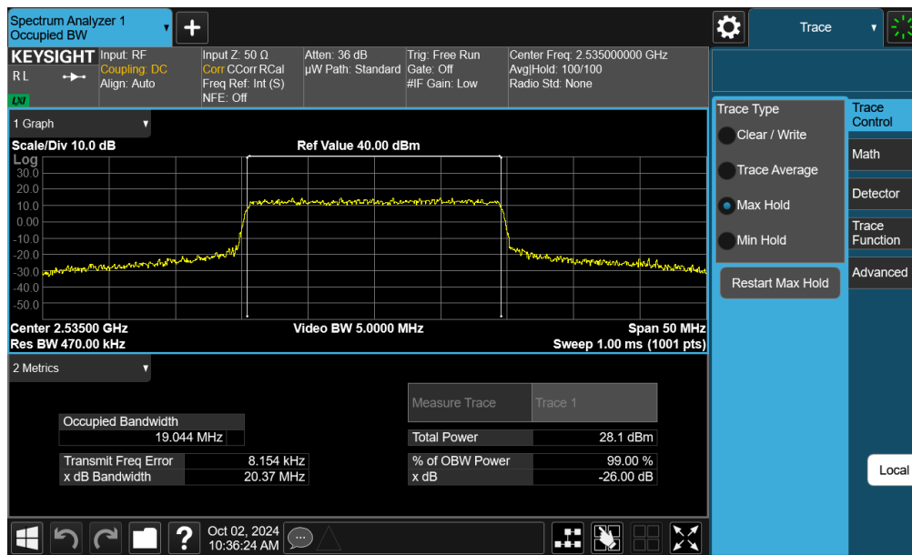
Plot 7-62. Occupied Bandwidth Plot (NR Band n7 - 20MHz 16-QAM - Full RB - Ant F)
