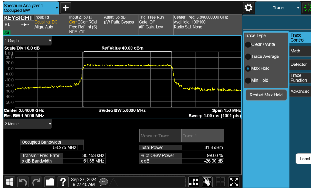
Plot 7-59. Occupied Bandwidth Plot (NR Band n77 C-band - 60MHz 16-QAM - Full RB - Ant F)
