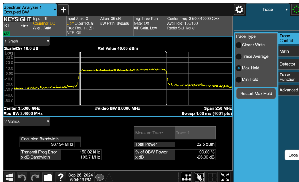
Plot 7-83. Occupied Bandwidth Plot (NR Band n77 DoD - 100MHz 16-QAM - Full RB - Ant C)
