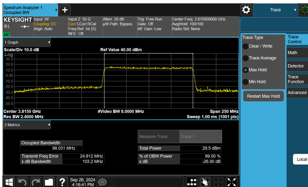
Plot 7-92. Occupied Bandwidth Plot (NR Band n77 DoD - 100MHz 16-QAM - Full RB - Ant I)
