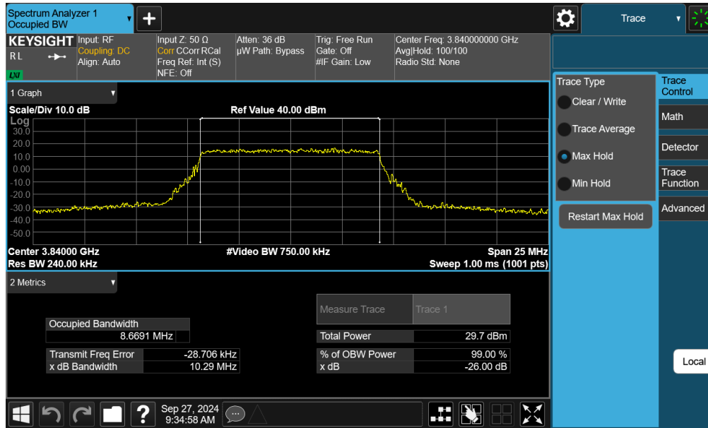
Plot 7-79. Occupied Bandwidth Plot (NR Band n77 C-band - 10MHz QPSK - Full RB - Ant F)
