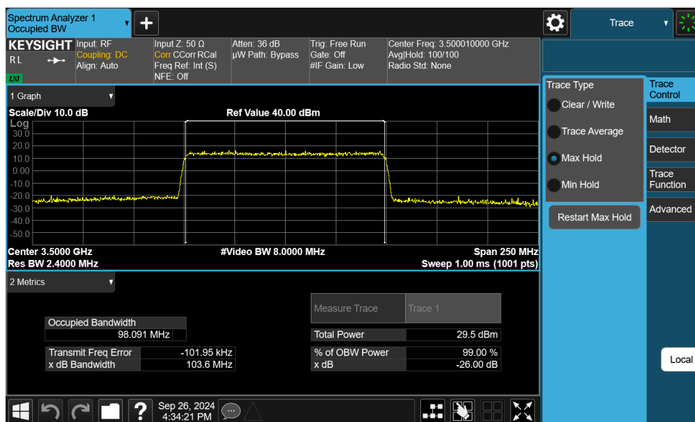
Plot 7-89. Occupied Bandwidth Plot (NR Band n77 DoD - 100MHz 16-QAM - Full RB - Ant I)
