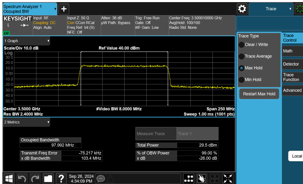
Plot 7-88. Occupied Bandwidth Plot (NR Band n77 DoD - 100MHz QPSK - Full RB - Ant I)
