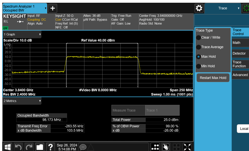
Plot 7-86. Occupied Bandwidth Plot (NR Band n77 DoD - 100MHz 16-QAM - Full RB - Ant C)
