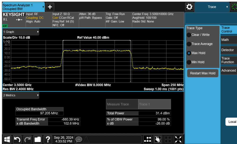
Plot 7-87. Occupied Bandwidth Plot (NR Band n77 DoD - 100MHz \pi/2 BPSK - Full RB - Ant I)
