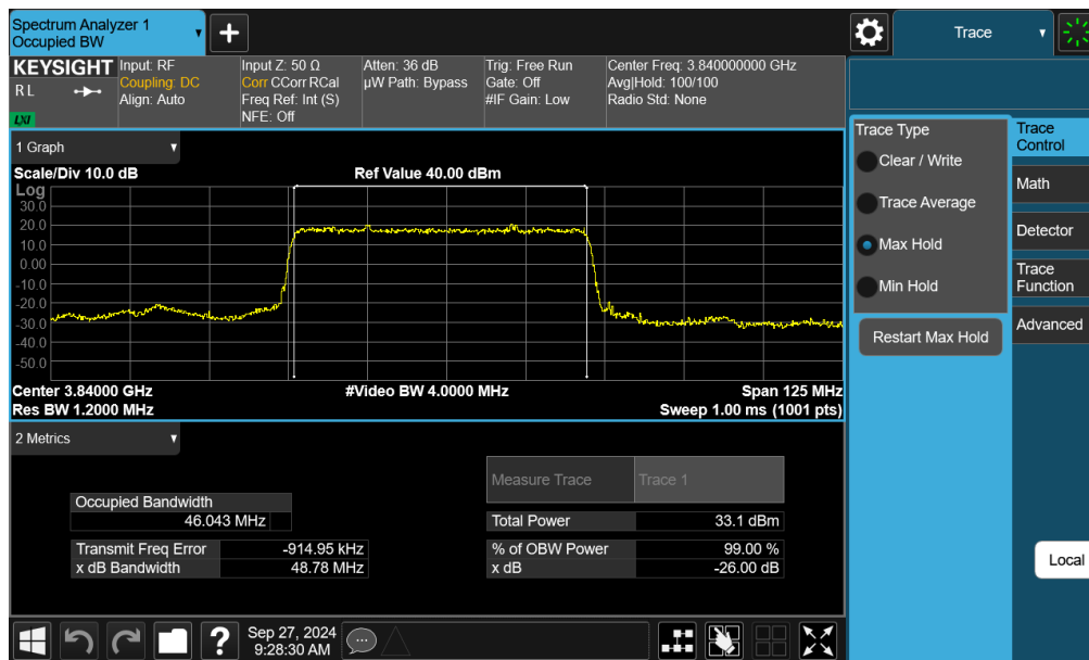
Plot 7-60. Occupied Bandwidth Plot (NR Band n77 C-band - 50MHz \pi/2 BPSK - Full RB - Ant F)
