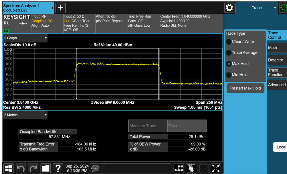
Plot 7-85. Occupied Bandwidth Plot (NR Band n77 DoD - 100MHz QPSK - Full RB - Ant C)
