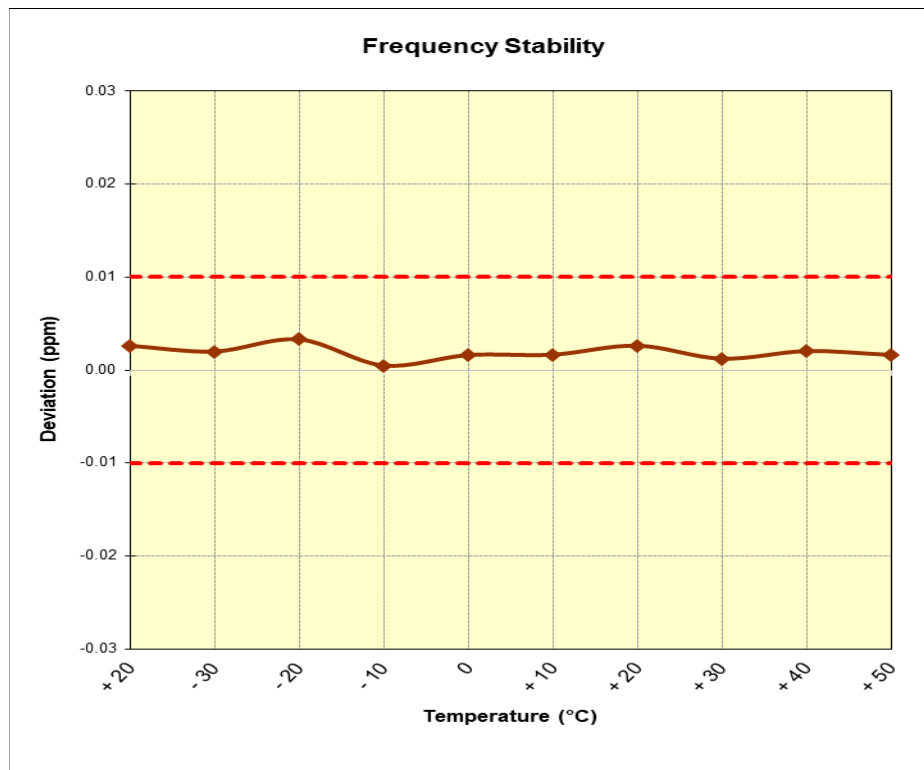
Figure 7-3. Frequency Stability Plot
