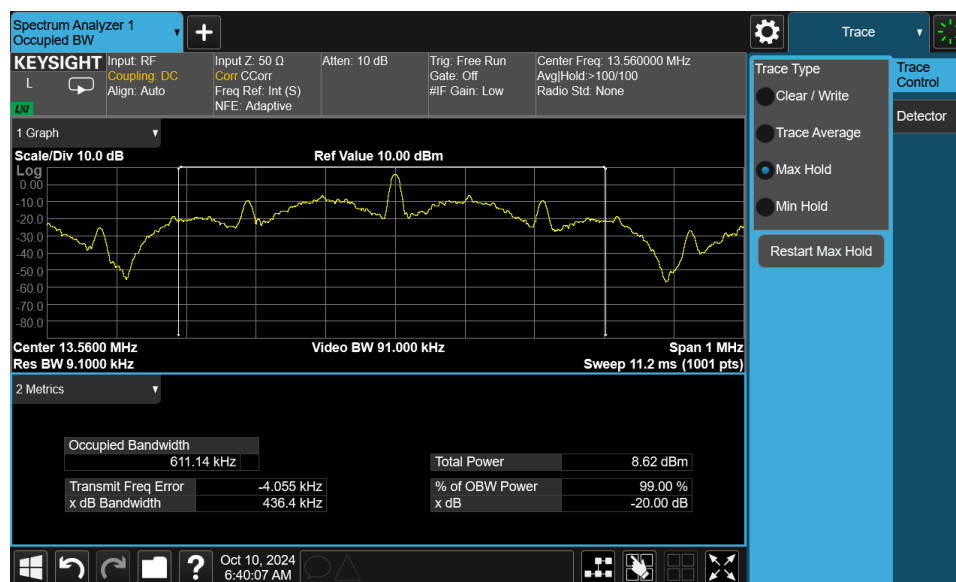
Figure 7-2. Occupied Bandwidth Plot
