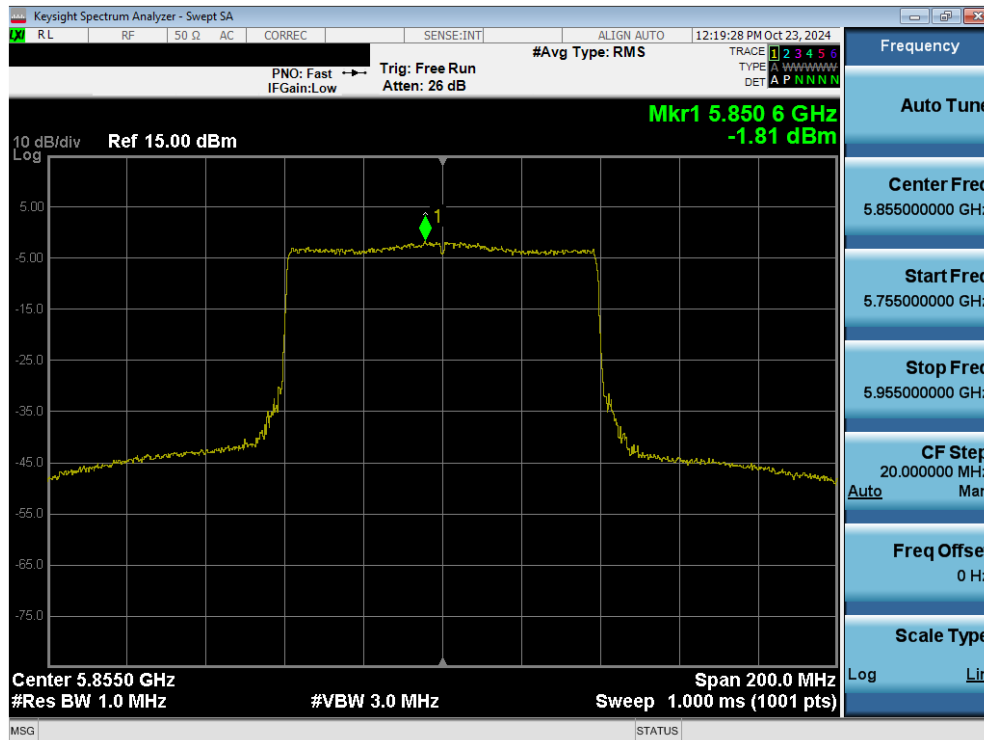
Plot 7-116. Power Spectral Density Plot MIMO ANT2 (80MHz 802.11ax/be (UNII Band 3/4) – Ch. 171)
