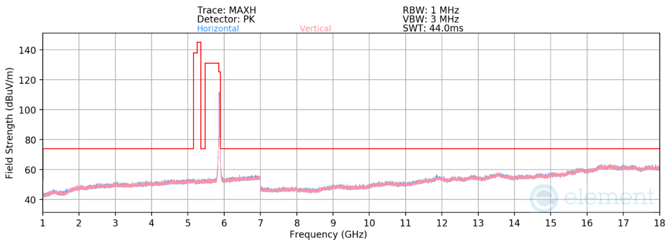
Plot 7-126. Radiated Spurious Plot above 1GHz MIMO (802.11ax – UNII Band 4 Ch. 173)
