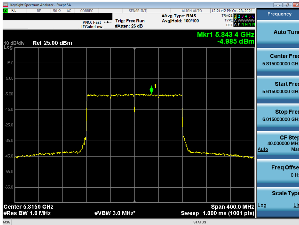
Plot 7-118. Power Spectral Density Plot MIMO ANT2 (160MHz 802.11ax/be (UNII Band 3/4) – Ch. 163)
