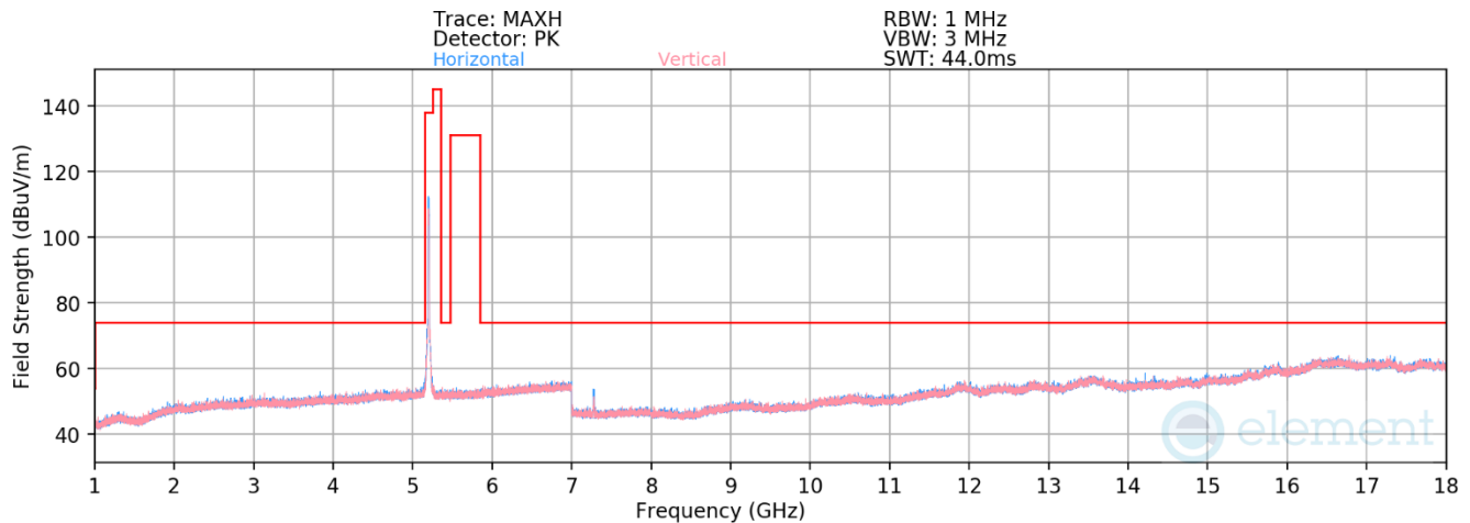
Plot 7-122. Radiated Spurious Plot above 1GHz MIMO (802.11ax – UNII Band 1 Ch. 40)
