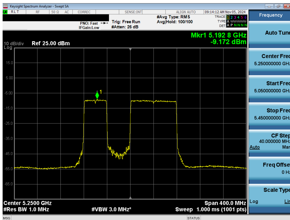
Plot 7-101. Power Spectral Density Plot MIMO ANT2 (160MHz 802.11be (40MHz Puncture) (UNII Band 1/2A) – Ch. 50)
