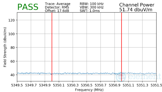
Plot 7-155. Radiated Upper Band Edge Plot MIMO (Average – UNII Band 2A)
