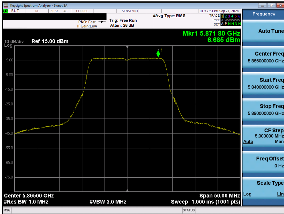
Plot 7-110. Power Spectral Density Plot MIMO ANT2 (20MHz 802.11a (UNII Band 4) – Ch.173)
