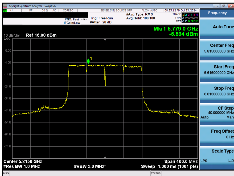
Plot 7-87. Power Spectral Density Plot MIMO ANT1 (160MHz 802.11ac (UNII Band 3/4) – Ch. 163)
