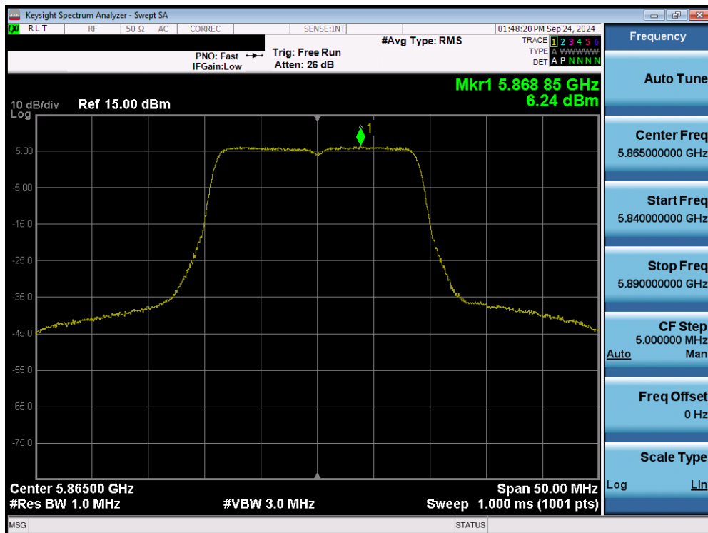
Plot 7-111. Power Spectral Density Plot MIMO ANT2 (20MHz 802.11n (UNII Band 4) – Ch.173)
