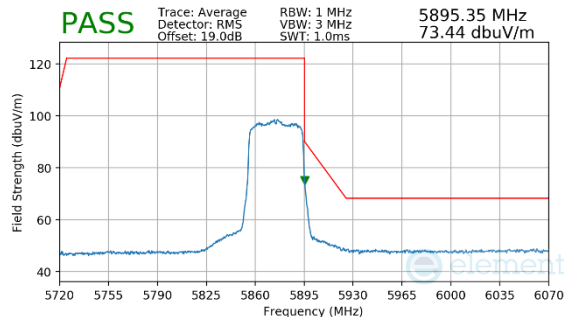
Plot 7-151. Radiated Upper Band Edge Plot MIMO (Average – UNII Band 4)
