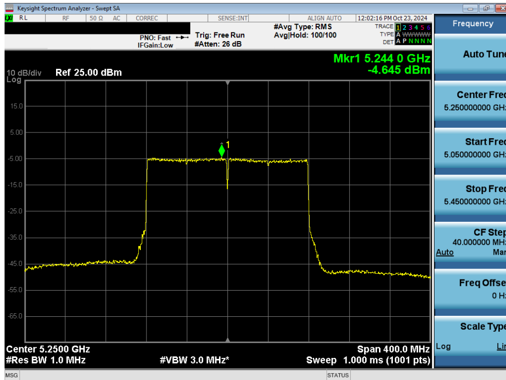
Plot 7-99. Power Spectral Density Plot MIMO ANT2 (160MHz 802.11ax/be (UNII Band 1/2A) – Ch. 50)
