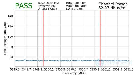
Plot 7-156. Radiated Upper Band Edge Plot MIMO (Peak – UNII Band 2A)
