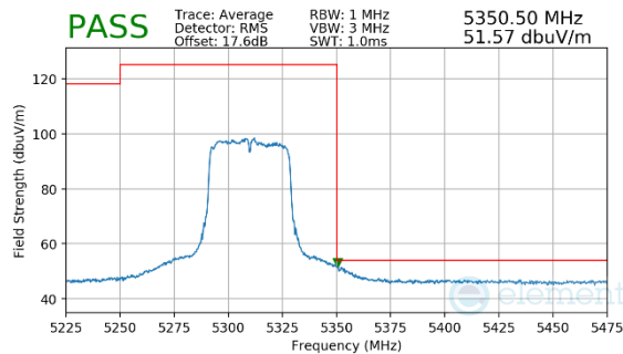
Plot 7-145. Radiated Upper Band Edge Plot MIMO (Average – UNII Band 2A)
