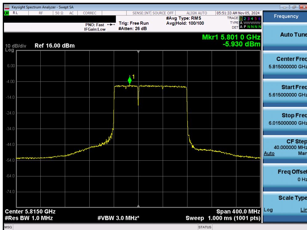
Plot 7-90. Power Spectral Density Plot MIMO ANT1 (160MHz 802.11be (40MHz Puncture) (UNII Band 3/4) – Ch. 163)
