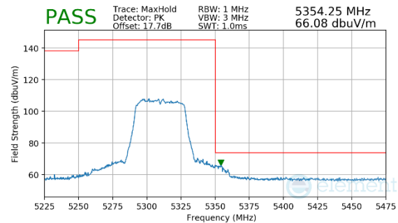
Plot 7-146. Radiated Upper Band Edge Plot MIMO (Peak – UNII Band 2A)
