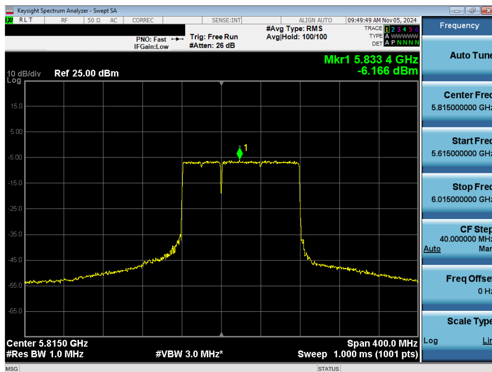
Plot 7-120. Power Spectral Density Plot MIMO ANT2 (160MHz 802.11be (40MHz Puncture) (UNII Band 3/4) – Ch. 163)
