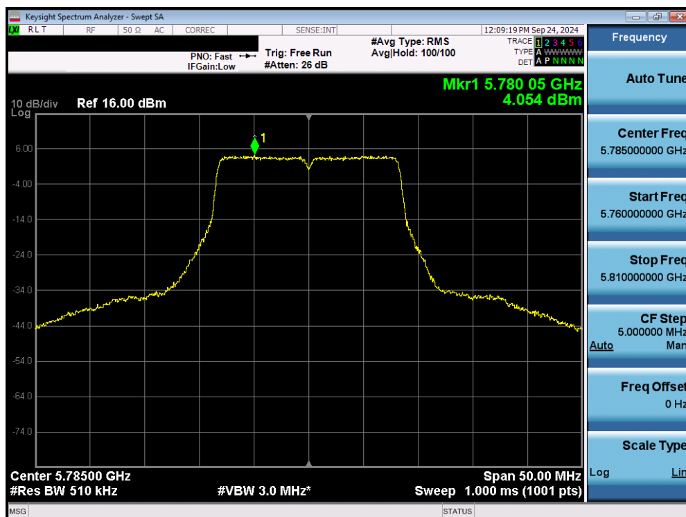
Plot 7-102. Power Spectral Density Plot MIMO ANT2 (20MHz 802.11a (UNII Band 3) – Ch.157)
