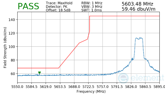
Plot 7-140. Radiated Lower Band Edge Plot MIMO (Peak – UNII Band 4)
