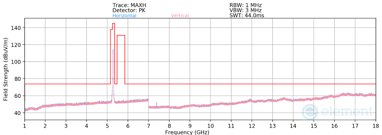
Plot 7-123. Radiated Spurious Plot above 1GHz MIMO (802.11ax – UNII Band 2A Ch. 56)
