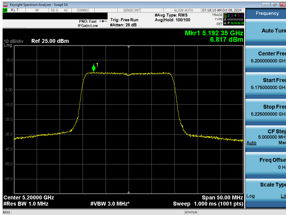
Plot 7-93. Power Spectral Density Plot MIMO ANT2 (20MHz 802.11ax/be (UNII Band 1) – Ch. 40)
