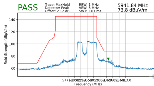
Plot 7-172. Radiated Upper Band Edge Plot MIMO (Peak – UNII Band 4)
