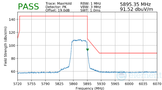
Plot 7-152. Radiated Upper Band Edge Plot MIMO (Peak – UNII Band 4)
