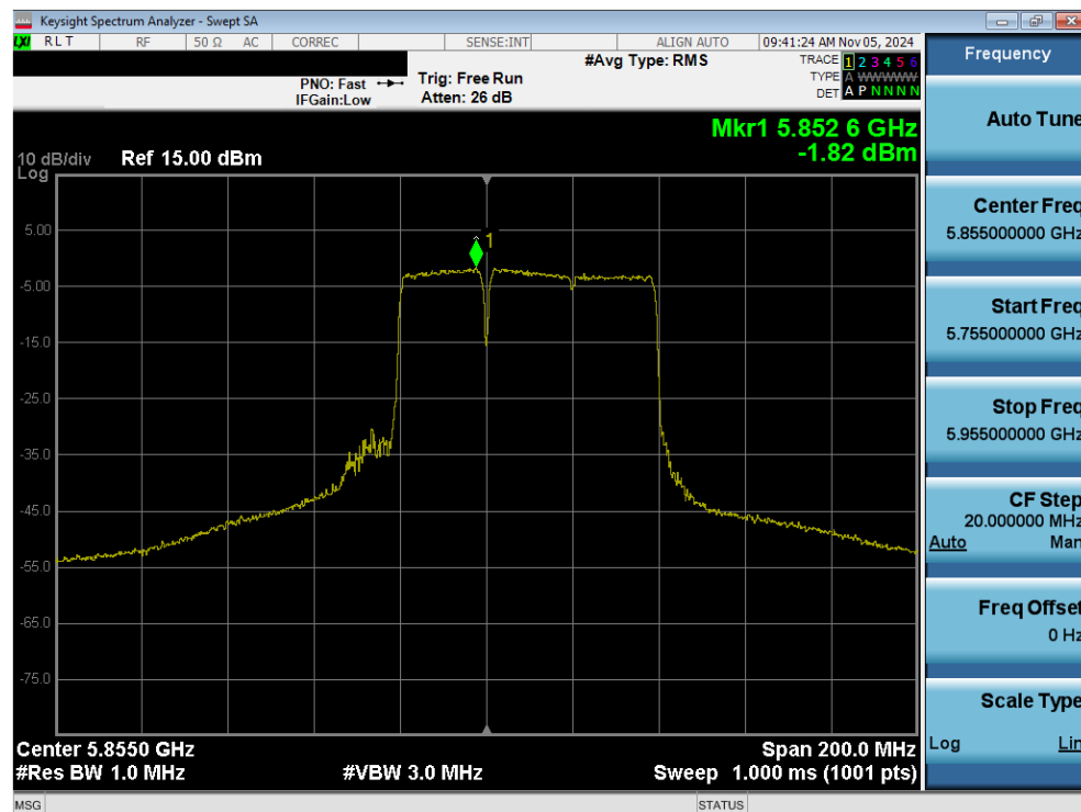
Plot 7-119. Power Spectral Density Plot MIMO ANT2 (80MHz 802.11be (20MHz Puncture) (UNII Band 3/4) – Ch. 171)
