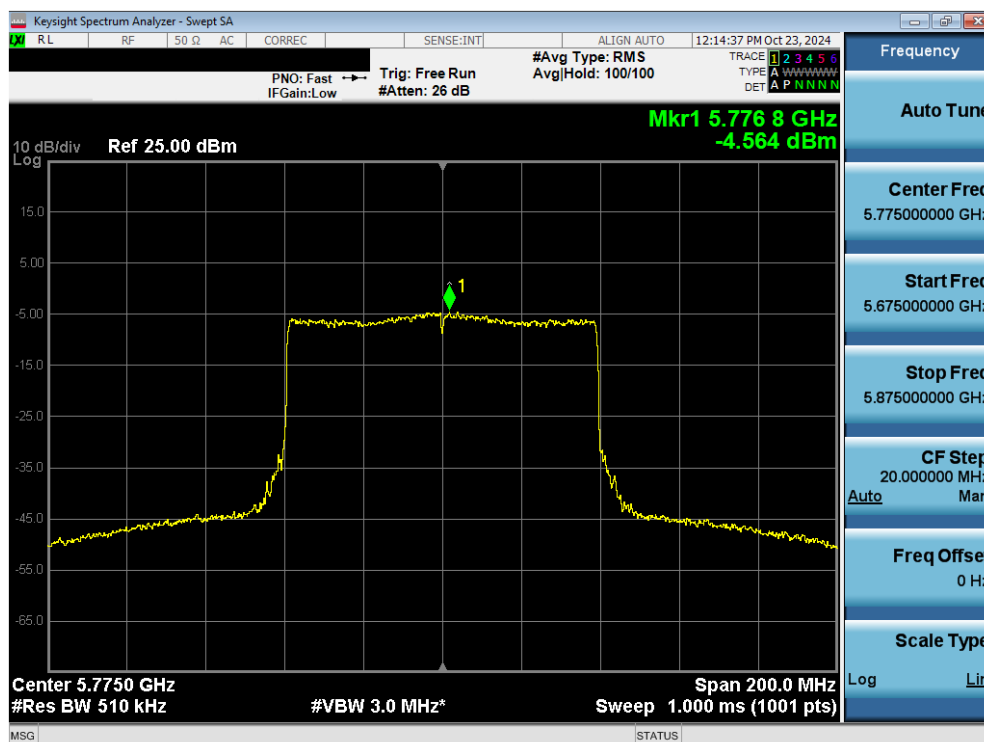
Plot 7-108. Power Spectral Density Plot MIMO ANT2 (80MHz 802.11ax/be (UNII Band 3) – Ch. 155)
