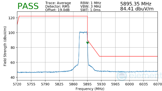
Plot 7-141. Radiated Upper Band Edge Plot MIMO (Average – UNII Band 4)
