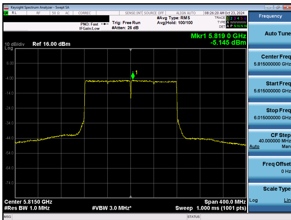
Plot 7-88. Power Spectral Density Plot MIMO ANT1 (160MHz 802.11ax/be (UNII Band 3/4) – Ch. 163)
