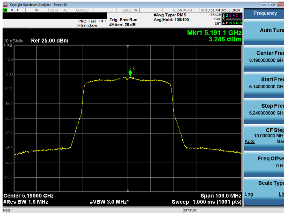
Plot 7-95. Power Spectral Density Plot MIMO ANT2 (40MHz 802.11ax/be (UNII Band 1) – Ch. 38)
