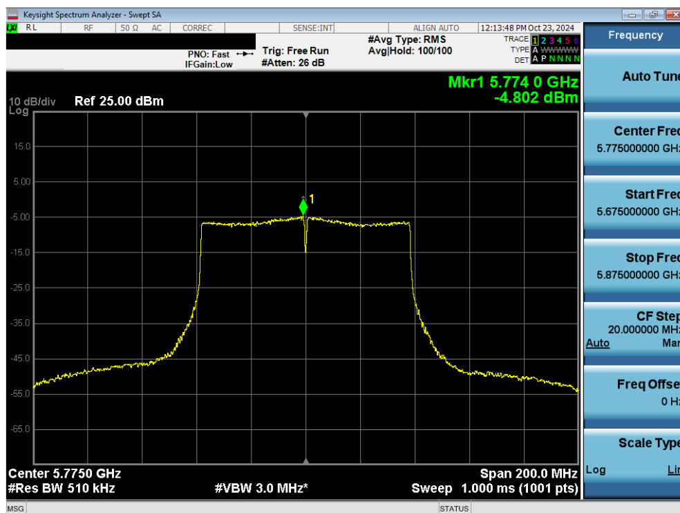
Plot 7-107. Power Spectral Density Plot MIMO ANT2 (80MHz 802.11ac (UNII Band 3) – Ch. 155)
