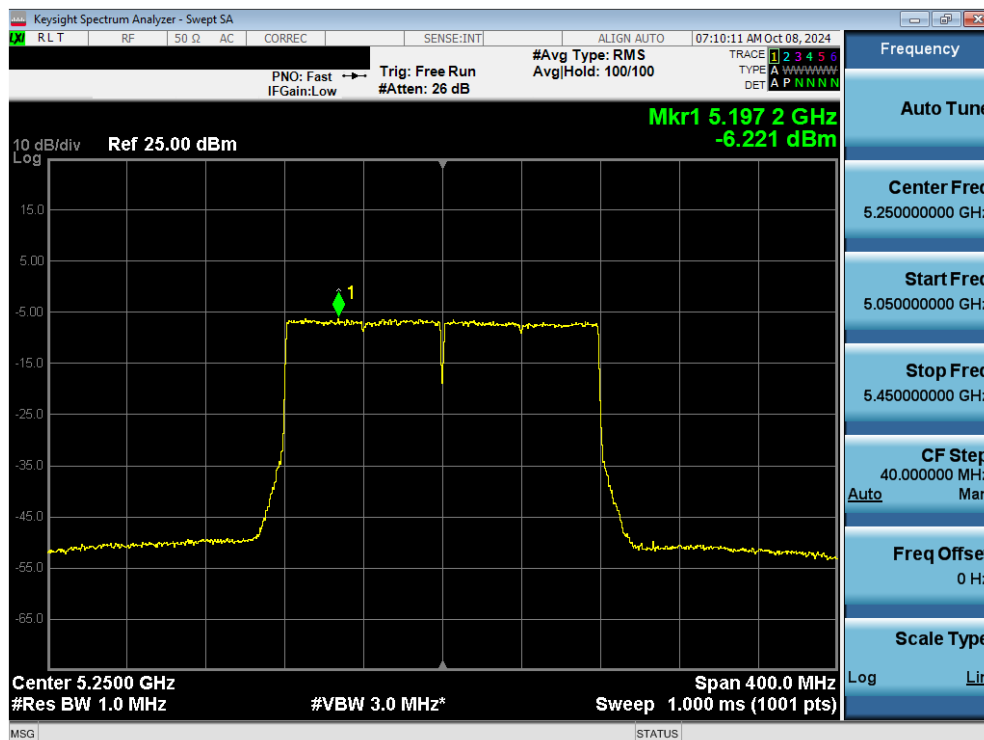
Plot 7-98. Power Spectral Density Plot MIMO ANT2 (160MHz 802.11ac (UNII Band 1/2A) – Ch. 50)
