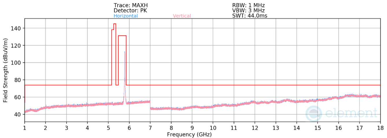
Plot 7-125. Radiated Spurious Plot above 1GHz MIMO (802.11ax – UNII Band 3 Ch. 157)
