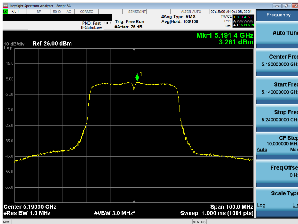
Plot 7-94. Power Spectral Density Plot MIMO ANT2 (40MHz 802.11n (UNII Band 1) – Ch. 38)
