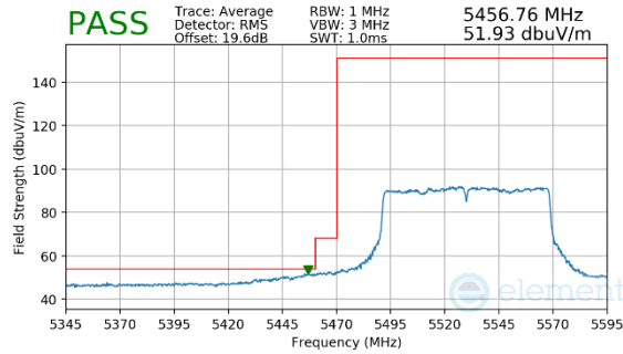
Plot 7-157. Radiated Lower Band Edge Plot MIMO (Average – UNII Band 2C)
