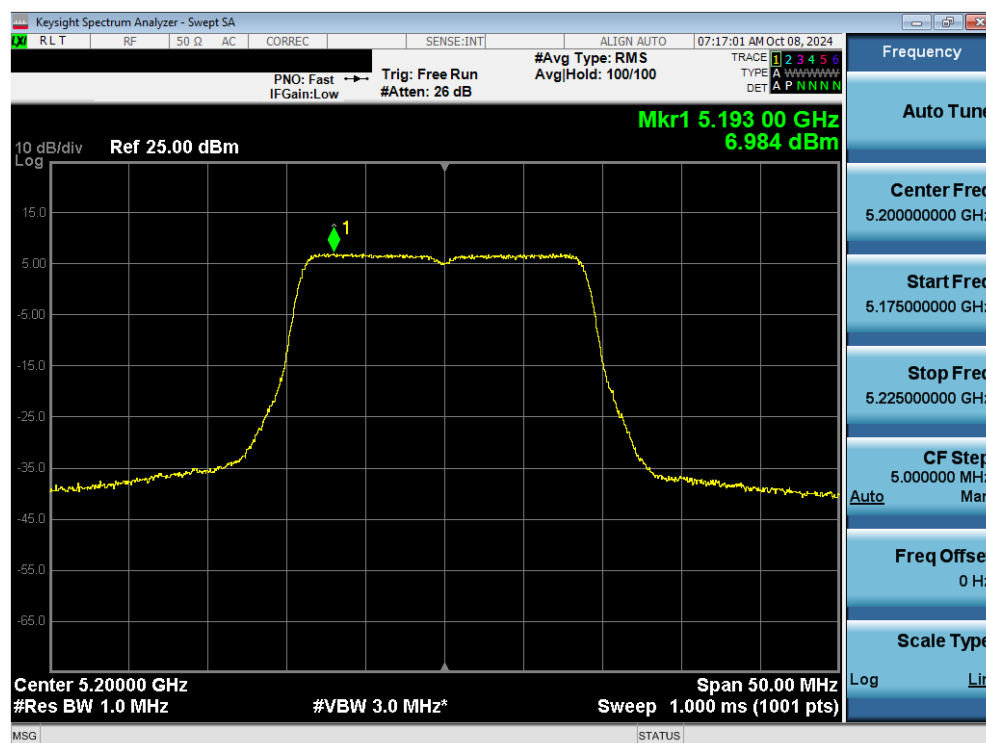
Plot 7-92. Power Spectral Density Plot MIMO ANT2 (20MHz 802.11n (UNII Band 1) – Ch. 40)
