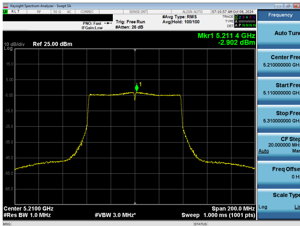
Plot 7-96. Power Spectral Density Plot MIMO ANT2 (80MHz 802.11ac (UNII Band 1) – Ch. 42)
