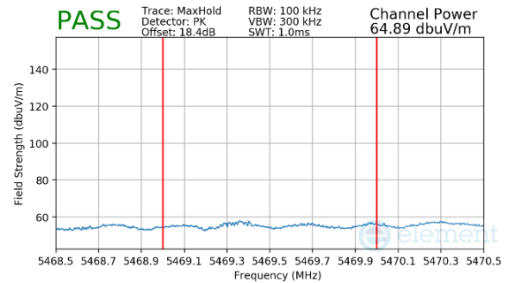
Plot 7-138. Radiated Lower Band Edge Plot MIMO (Peak – UNII Band 2C)
