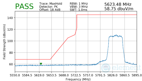
Plot 7-150. Radiated Lower Band Edge Plot MIMO (Peak – UNII Band 4)
