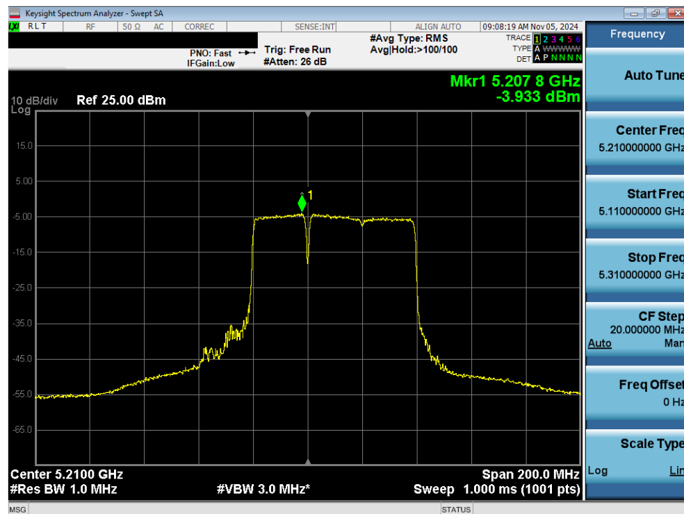
Plot 7-100. Power Spectral Density Plot MIMO ANT2 (80MHz 802.11be (20MHz Puncture) (UNII Band 1) – Ch. 42)
