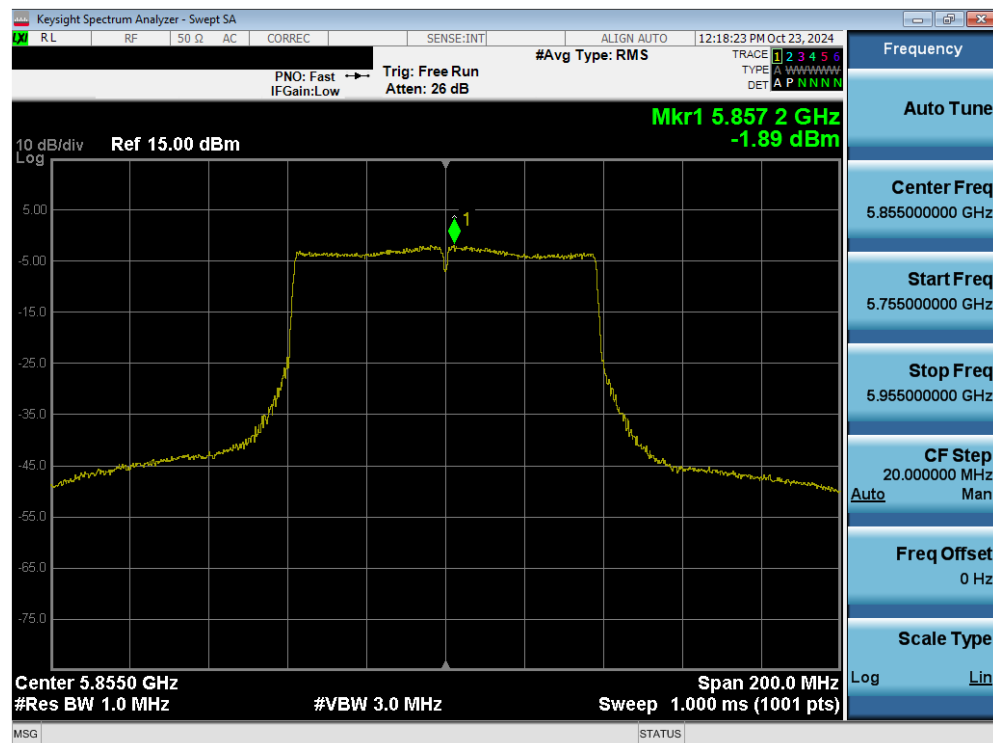
Plot 7-115. Power Spectral Density Plot MIMO ANT2 (80MHz 802.11ac (UNII Band 3/4) – Ch. 171)
