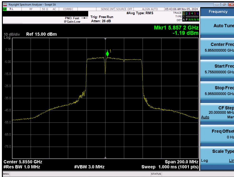
Plot 7-89. Power Spectral Density Plot MIMO ANT1 (80MHz 802.11be (20MHz Puncture) (UNII Band 3/4) – Ch. 171)
