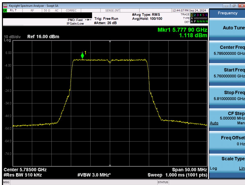
Plot 7-104. Power Spectral Density Plot MIMO ANT2 (20MHz 802.11ax/be (UNII Band 3) – Ch.157)
