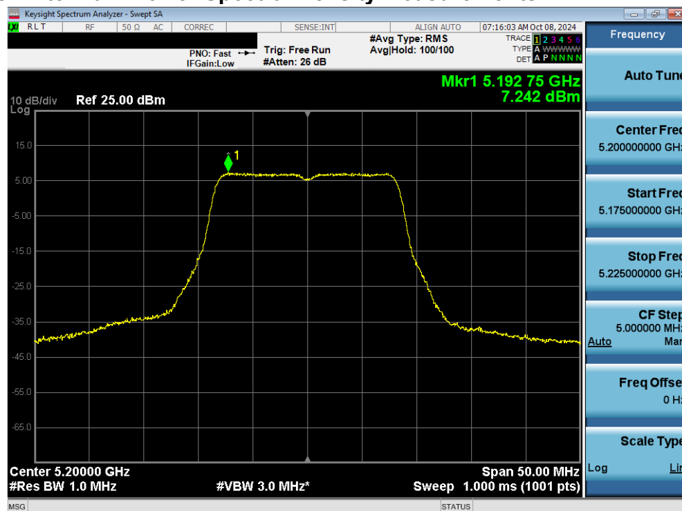
Plot 7-91. Power Spectral Density Plot MIMO ANT2 (20MHz 802.11a (UNII Band 1) – Ch. 40)
