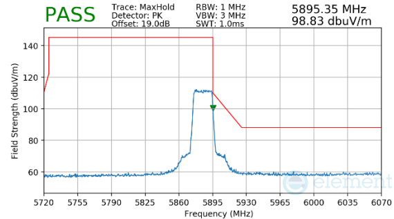
Plot 7-142. Radiated Upper Band Edge Plot MIMO (Peak – UNII Band 4)
