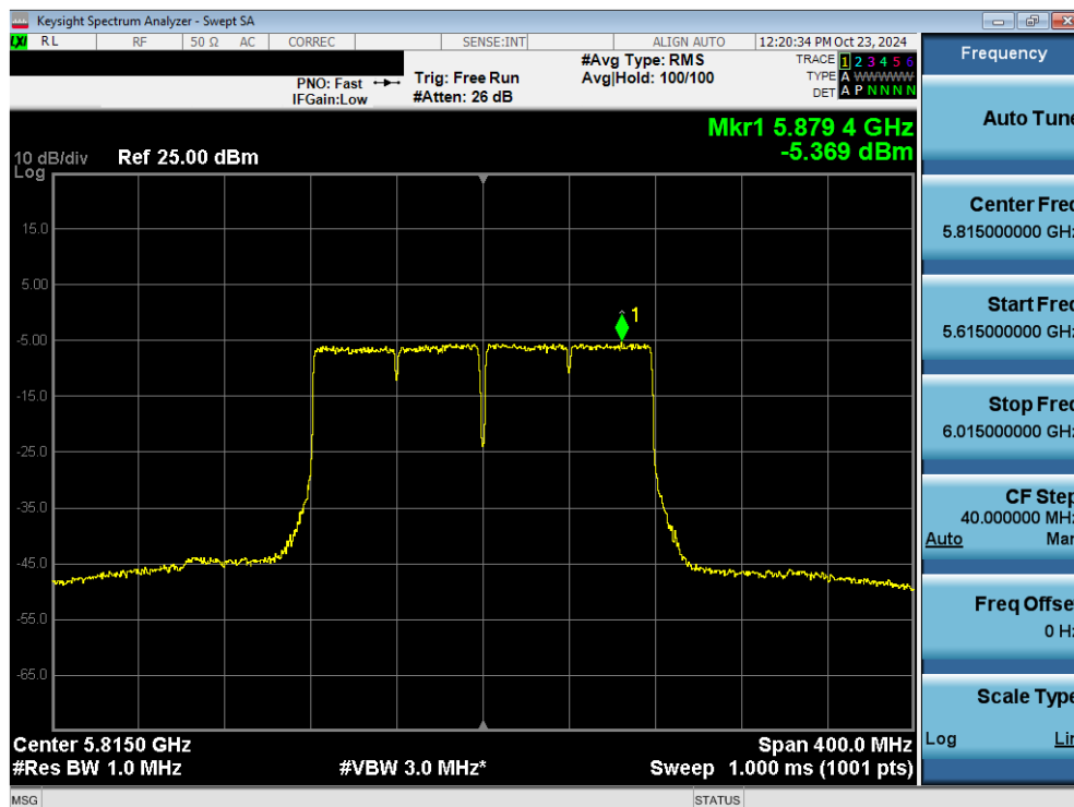
Plot 7-117. Power Spectral Density Plot MIMO ANT2 (160MHz 802.11ac (UNII Band 3/4) – Ch. 163)
