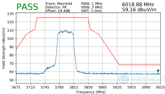
Plot 7-149. Radiated Upper Band Edge Plot MIMO (Peak – UNII Band 3)
