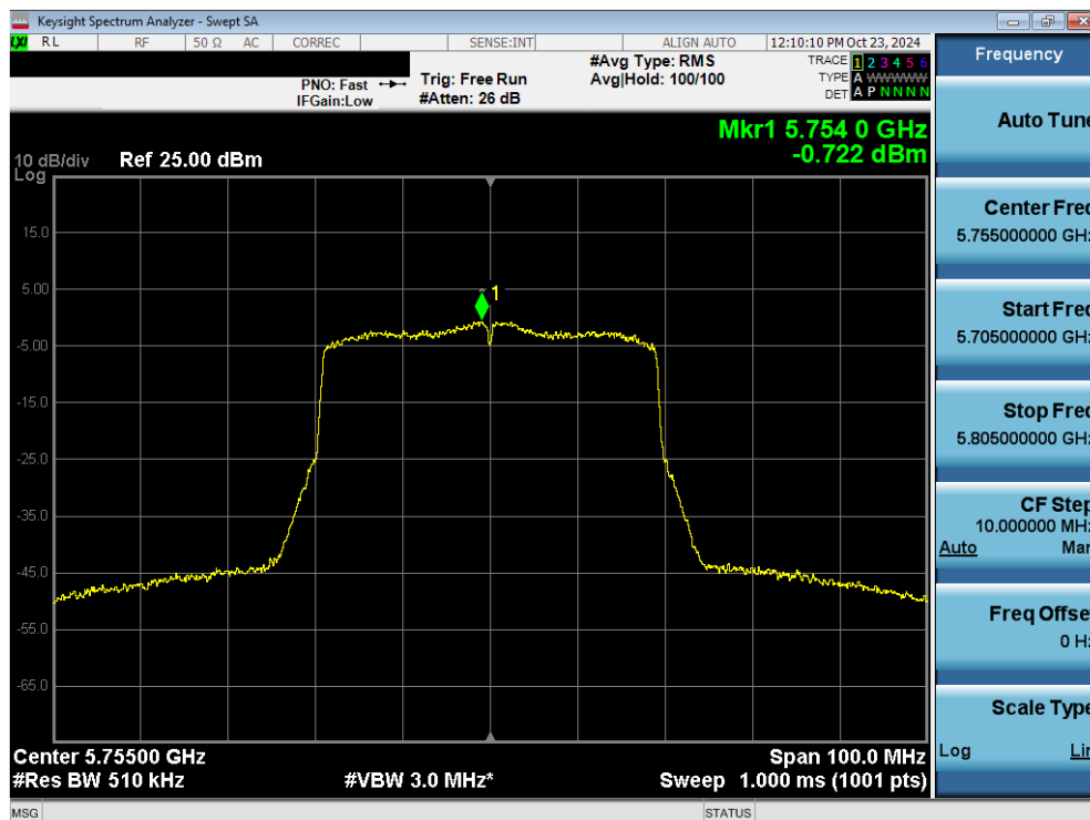
Plot 7-106. Power Spectral Density Plot MIMO ANT2 (40MHz 802.11ax/be (UNII Band 3) – Ch. 151)
