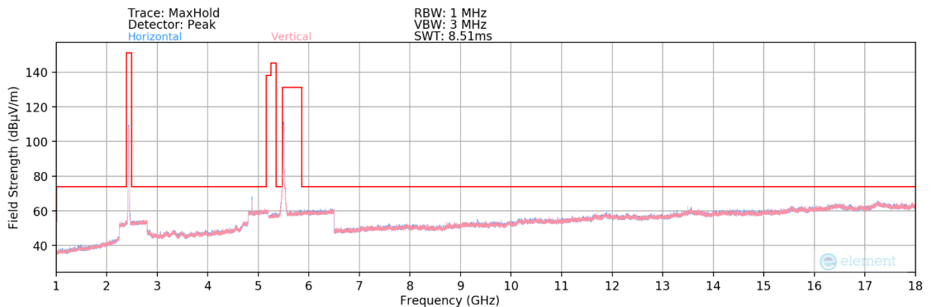
Plot 7-130. Radiated Spurious Plot above 1GHz MIMO 802.11b (2.4GHz – Ch.6) + MIMO 802.11a (5GHz – Ch.100)
