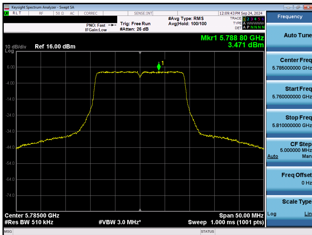
Plot 7-103. Power Spectral Density Plot MIMO ANT2 (20MHz 802.11n (UNII Band 3) – Ch.157)
