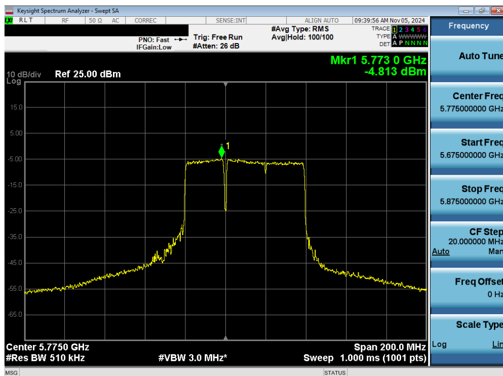
Plot 7-109. Power Spectral Density Plot MIMO ANT2 (80MHz 802.11be (20MHz Puncture) (UNII Band 3) – Ch. 155)
