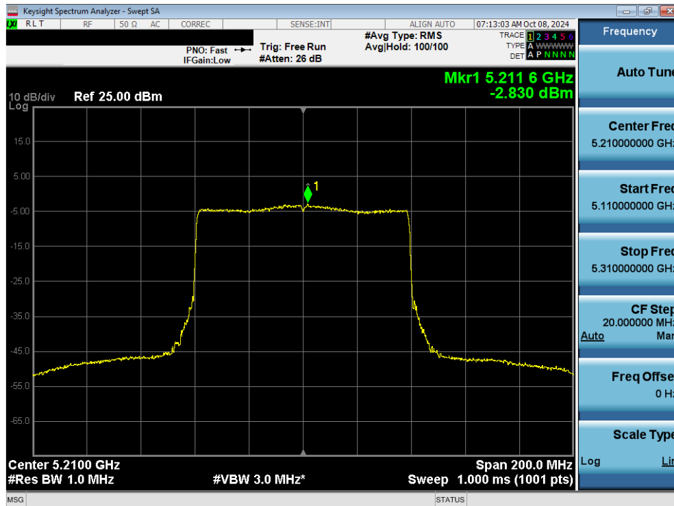
Plot 7-97. Power Spectral Density Plot MIMO ANT2 (80MHz 802.11ax/be (UNII Band 1) – Ch. 42)
