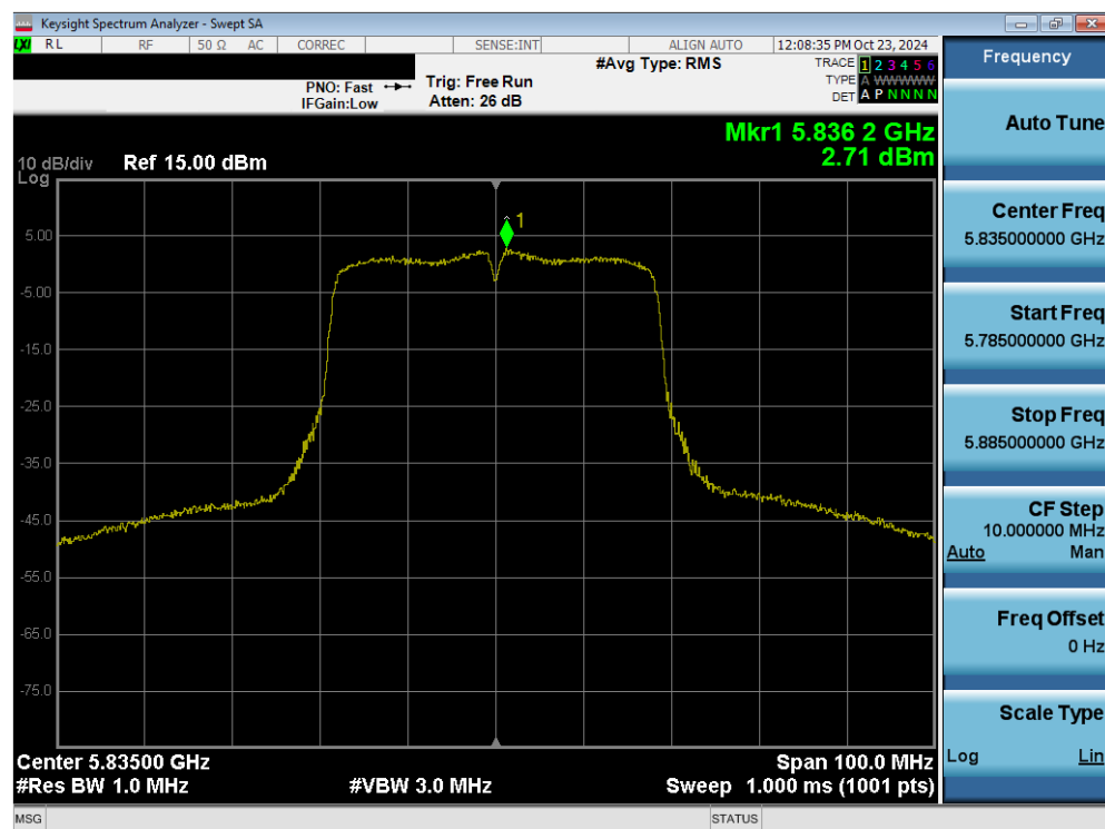
Plot 7-113. Power Spectral Density Plot MIMO ANT2 (40MHz 802.11n (UNII Band 3/4) – Ch. 167)
