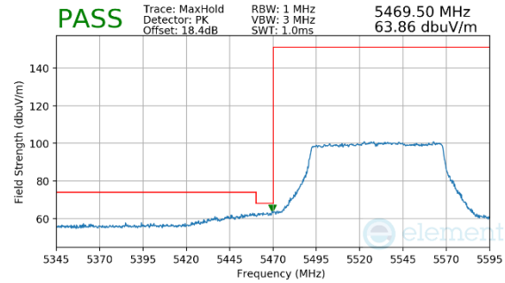
Plot 7-158. Radiated Lower Band Edge Plot MIMO (Peak – UNII Band 2C)
