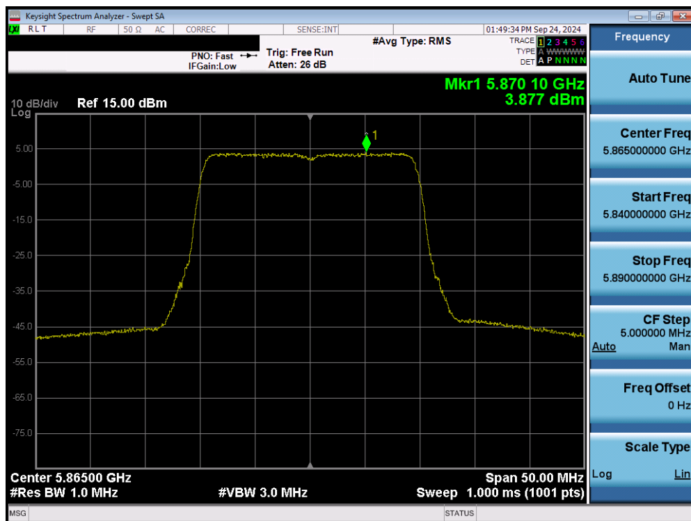
Plot 7-112. Power Spectral Density Plot MIMO ANT2 (20MHz 802.11ax/be (UNII Band 4) – Ch.173)
