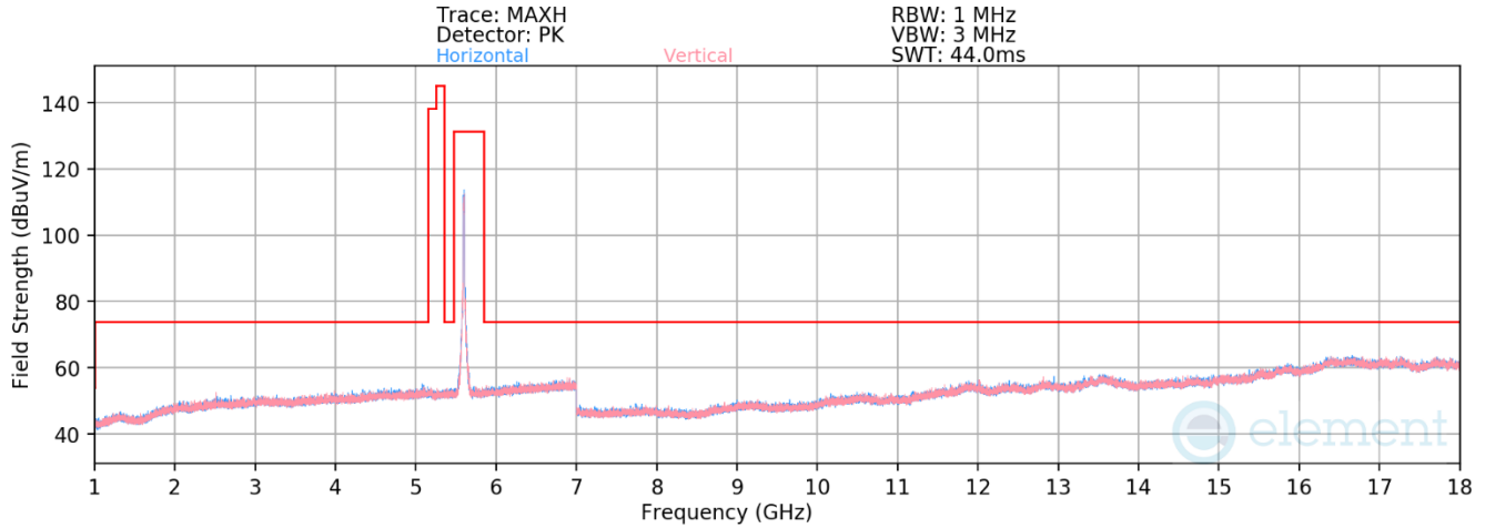
Plot 7-124. Radiated Spurious Plot above 1GHz MIMO (802.11ax – UNII Band 2C Ch. 120)
