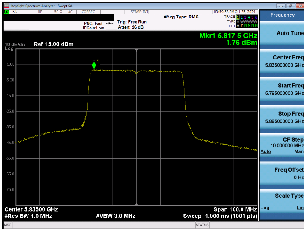
Plot 7-114. Power Spectral Density Plot MIMO ANT2 (40MHz 802.11ax/be (UNII Band 3/4) – Ch. 167)
