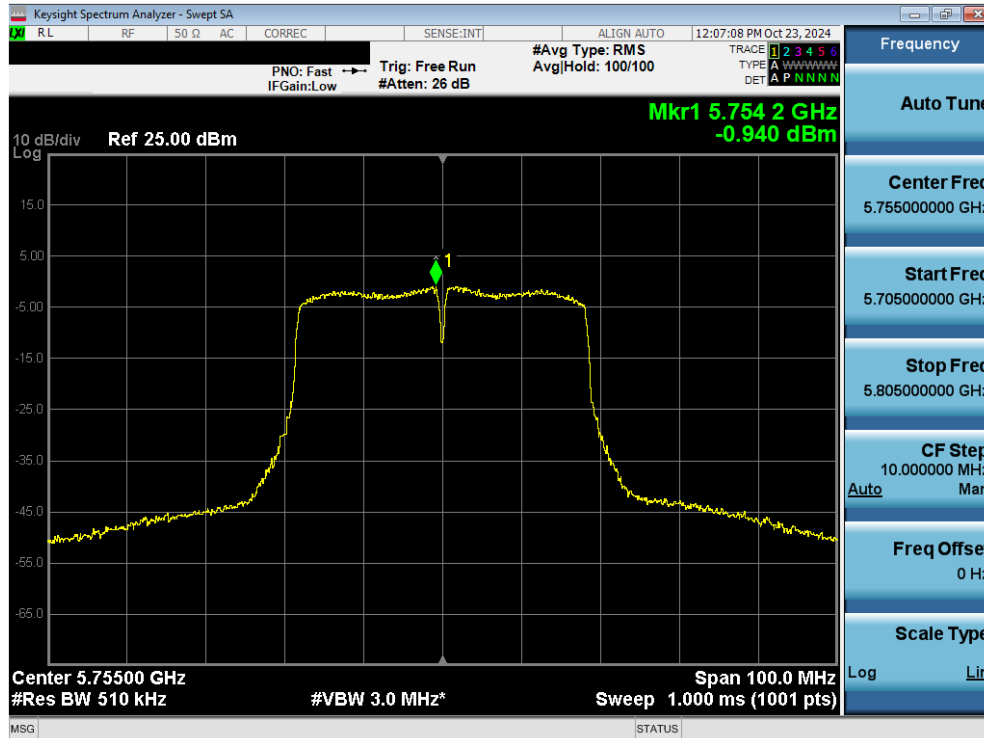
Plot 7-105. Power Spectral Density Plot MIMO ANT2 (40MHz 802.11n (UNII Band 3) – Ch. 151)
