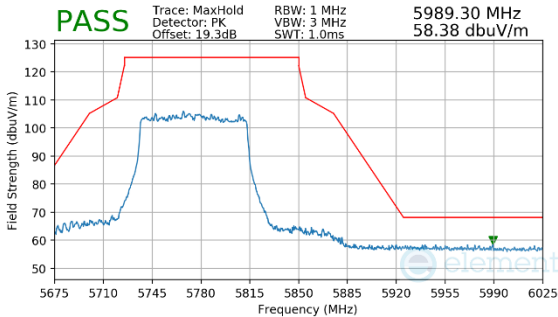
Plot 7-159. Radiated Upper Band Edge Plot MIMO (Peak – UNII Band 3)
