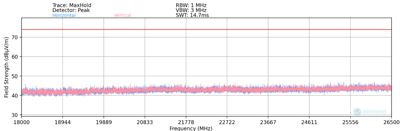
Plot 7-127. Radiated Spurious Plot 18GHz – 26.5GHz MIMO (802.11ax)
