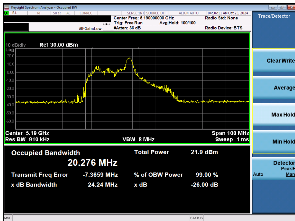
Plot 7-2. 26dB Bandwidth Plot MIMO ANT1 (40MHz 802.11ax/be (26 Tones) (UNII Band 1) – Ch. 38)
