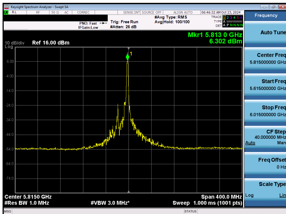
Plot 7-80. Power Spectral Density Plot MIMO ANT1 (160MHz 802.11ax/be (26 Tones) (UNII Band 3/4) – Ch. 163)
