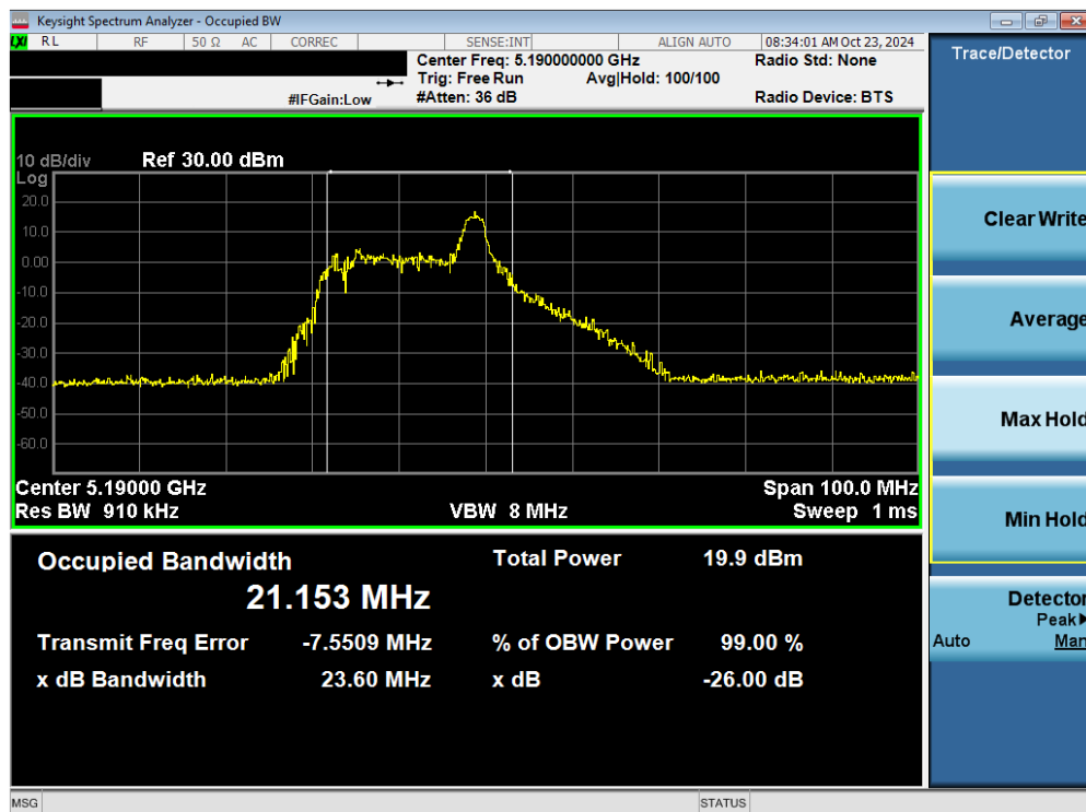
Plot 7-13. 26dB Bandwidth Plot MIMO ANT2 (40MHz 802.11ax/be (26 Tones) (UNII Band 1) – Ch. 38)
