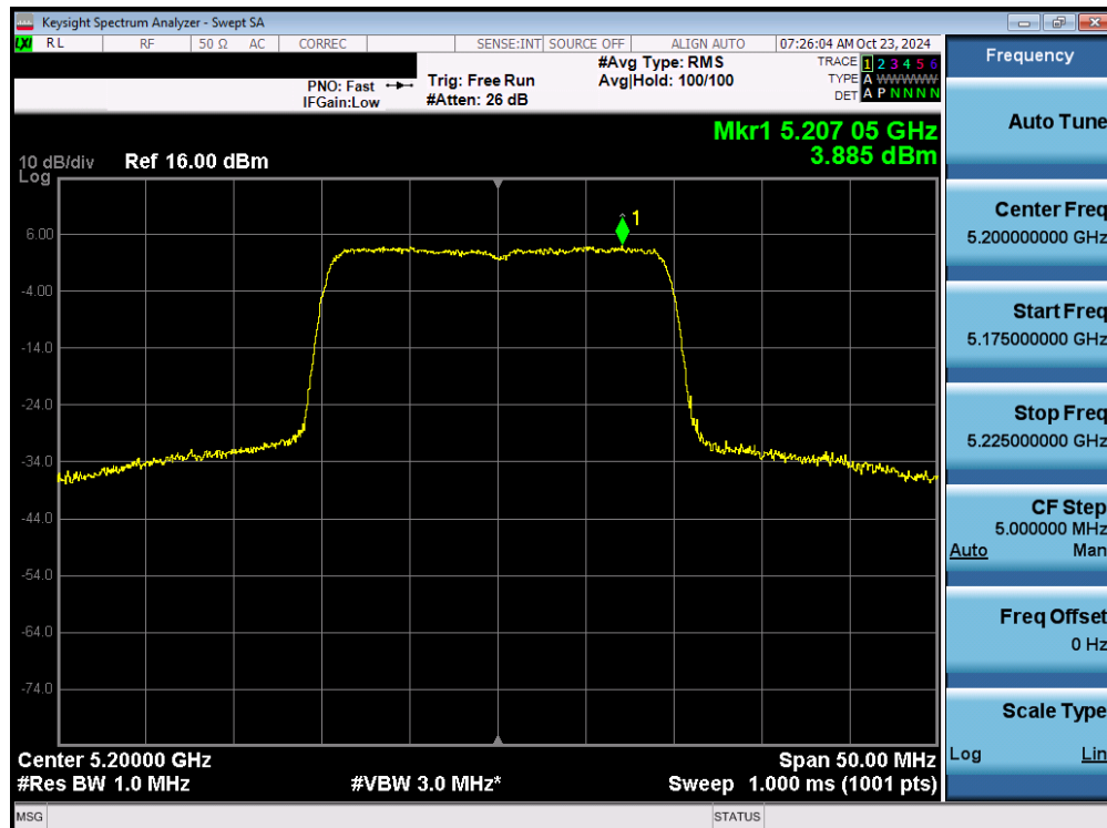
Plot 7-68. Power Spectral Density Plot MIMO ANT1 (20MHz 802.11ax/be (Full Tones) (UNII Band 1) – Ch. 40)
