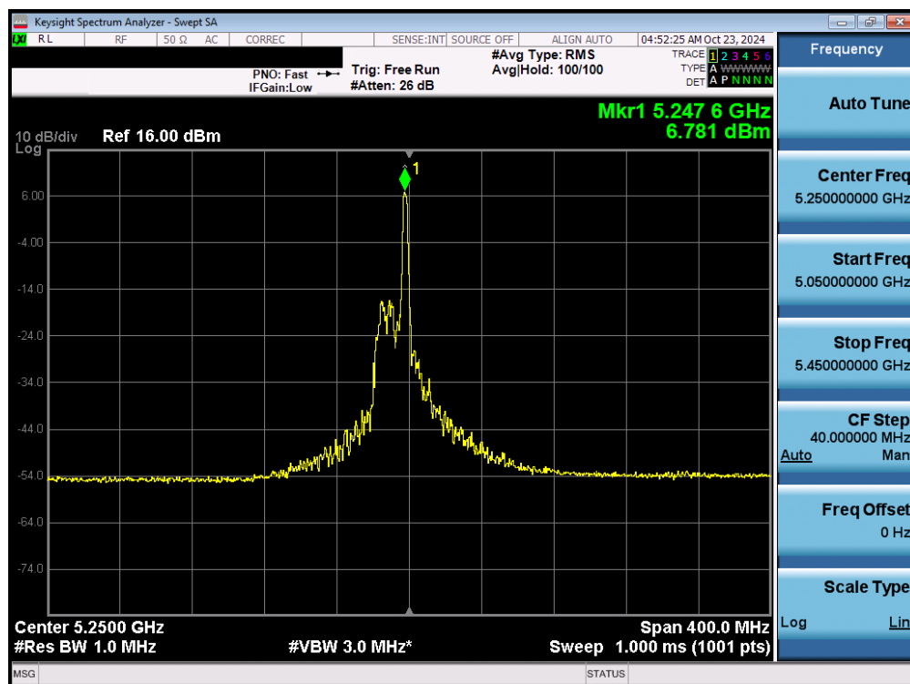
Plot 7-64. Power Spectral Density Plot MIMO ANT1 (160MHz 802.11ax/be (26 Tones) (UNII Band 1/2A) – Ch. 50)
