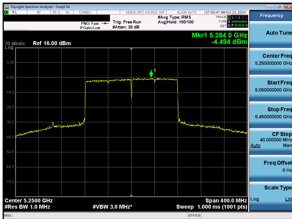
Plot 7-71. Power Spectral Density Plot MIMO ANT1 (160MHz 802.11ax/be (Full Tones) (UNII Band 1/2A) – Ch. 50)
