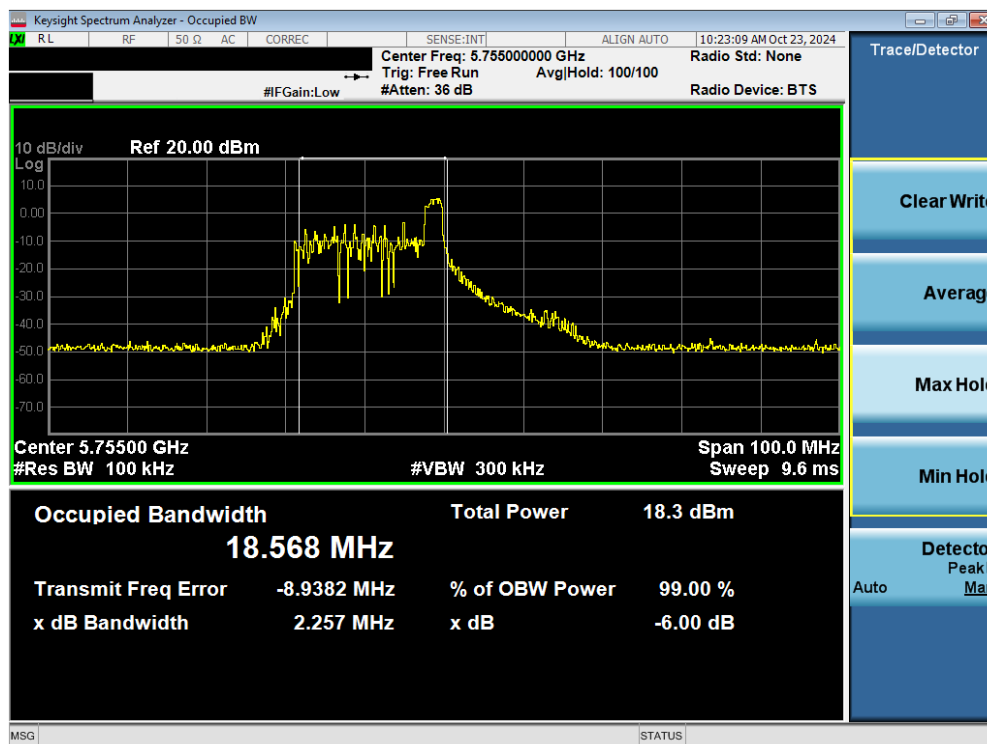
Plot 7-43. 6dB Bandwidth Plot MIMO ANT2 (40MHz 802.11ax/be (26 Tones) (UNII Band 3) – Ch. 151)
