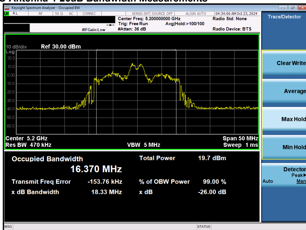
Plot 7-1. 26dB Bandwidth Plot MIMO ANT1 (20MHz 802.11ax/be (26 Tones) (UNII Band 1) – Ch. 40)
