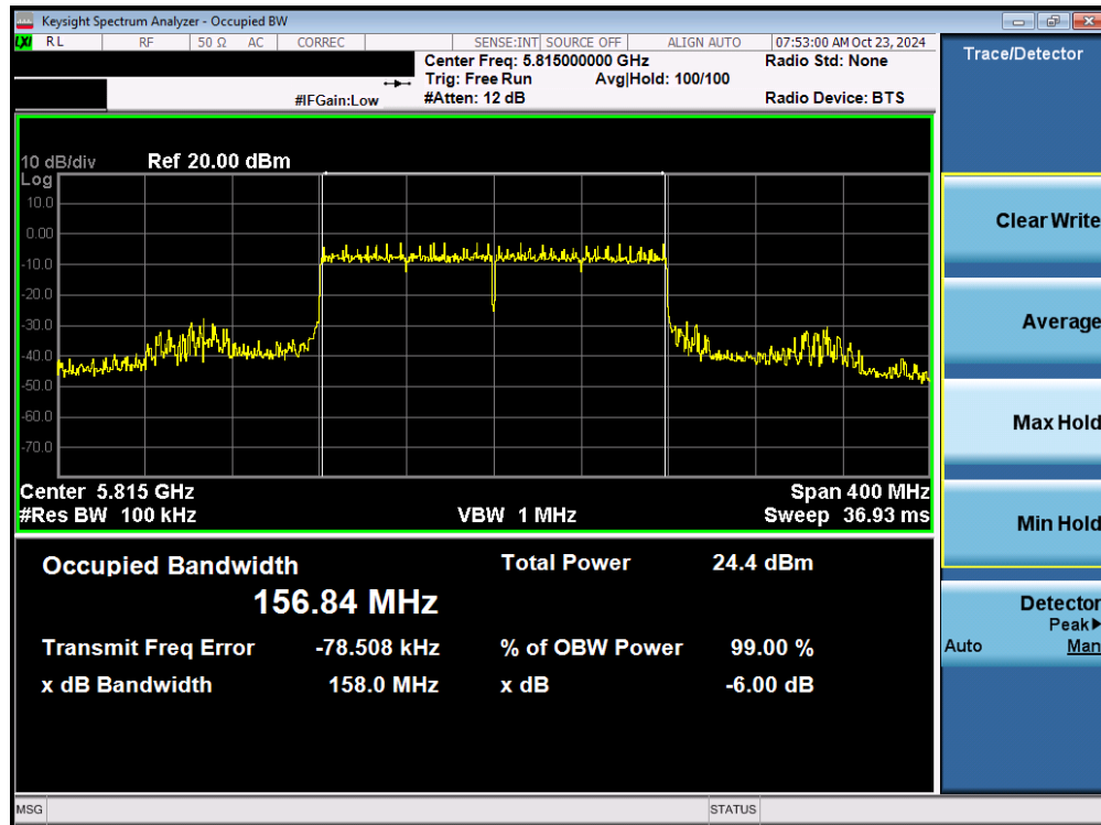
Plot 7-41. 6dB Bandwidth Plot MIMO ANT1 (160MHz 802.11ax/be (Full Tones) (UNII Band 3/4) – Ch. 163)
