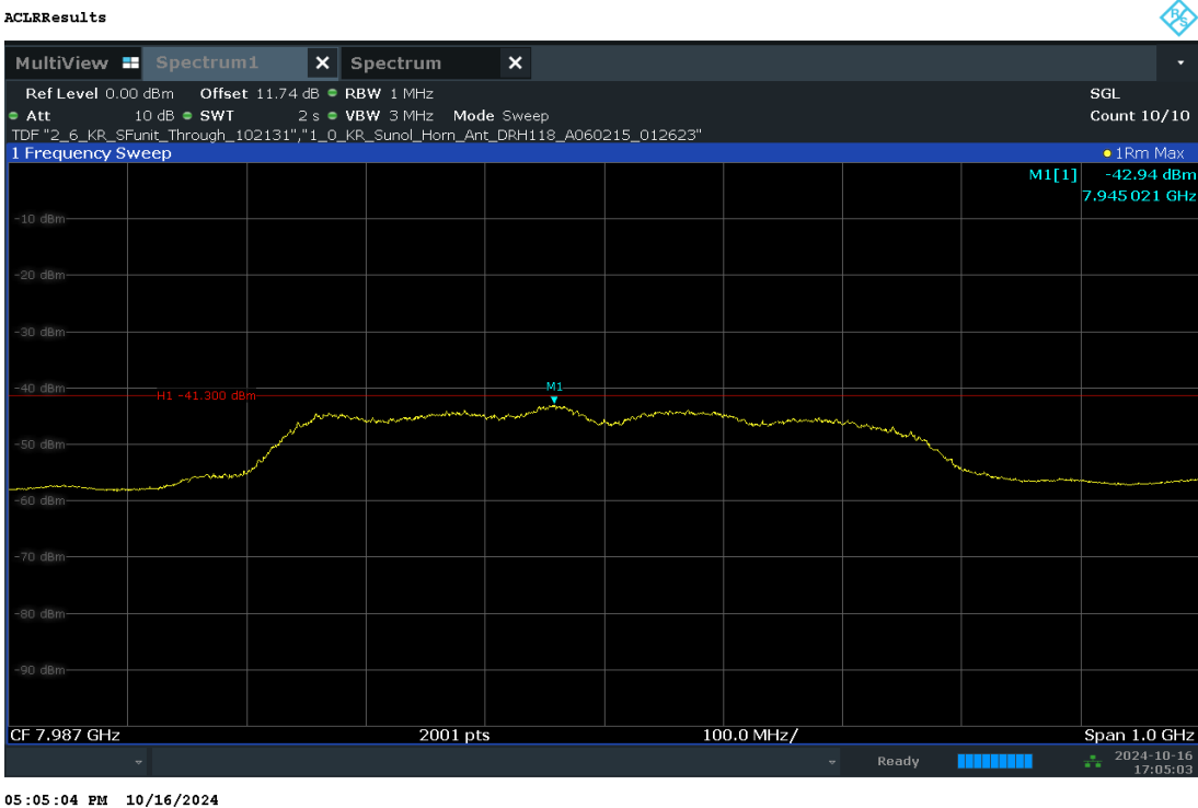
Plot 7-35. UWB Average Power Measurement - CH.9 – BPRF
