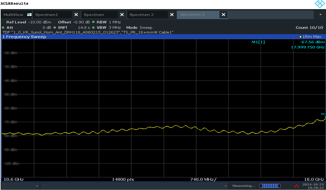
Plot 7-46. Radiated Spurious Pre-Scan 10600 - 18000 MHz - CH.9
