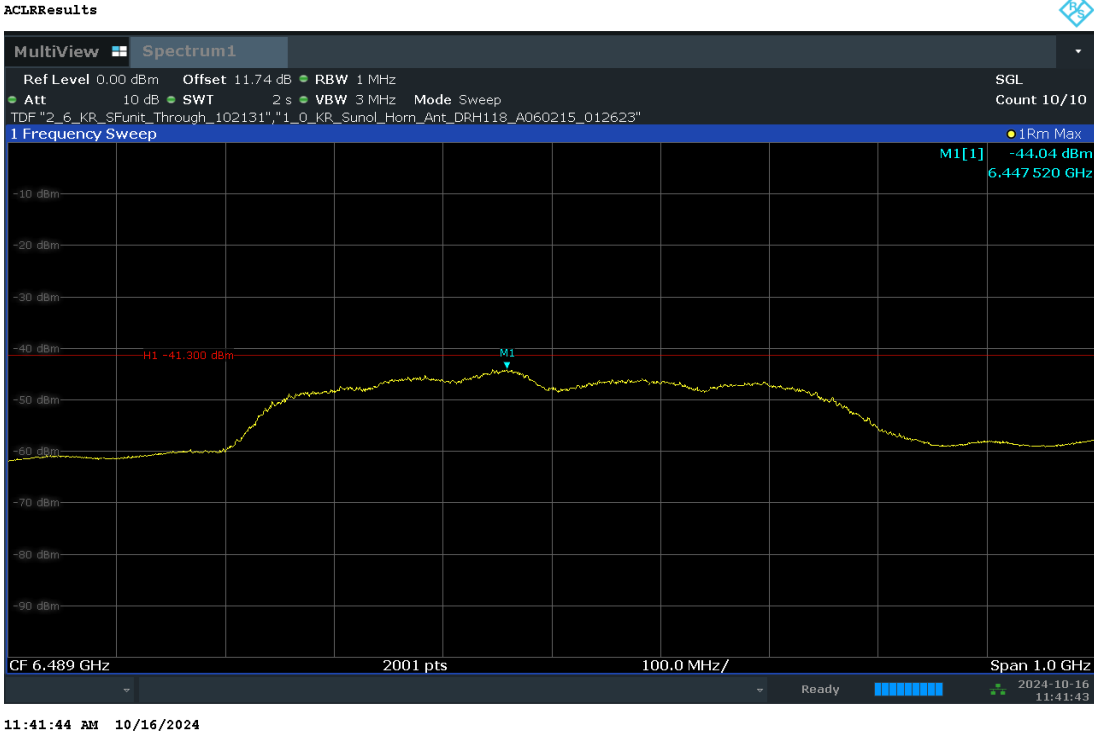
Plot 7-34. UWB Average Power Measurement - CH.5 – BPRF
