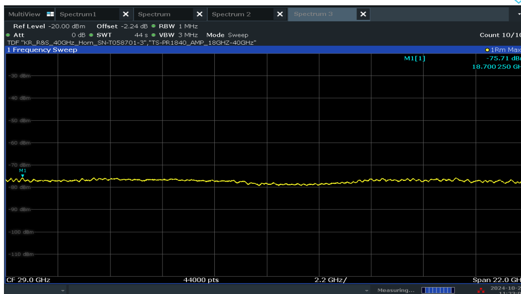
Plot 7-44. Radiated Spurious Pre-Scan 18 – 40 GHz - CH.5
