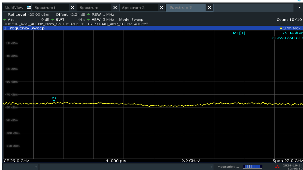
Plot 7-49. Radiated Spurious Pre-Scan 18 – 40 GHz - CH.9
