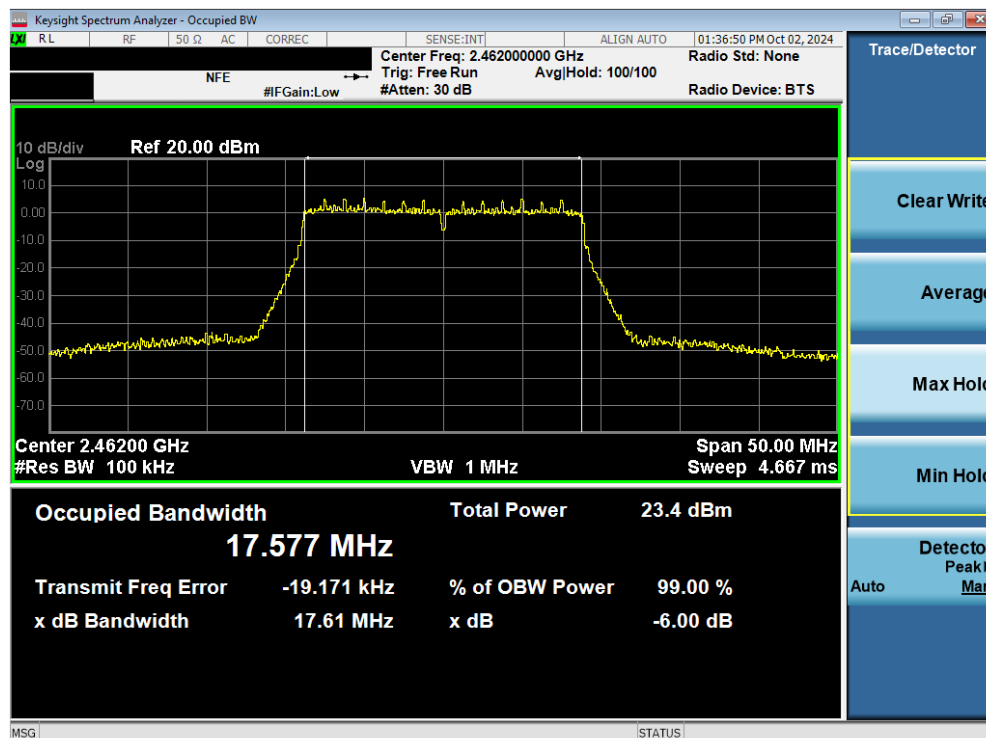
Plot 7-30. 6dB Bandwidth Plot (802.11ax/be (2.4GHz) – Ch. 11) MIMO ANT2
