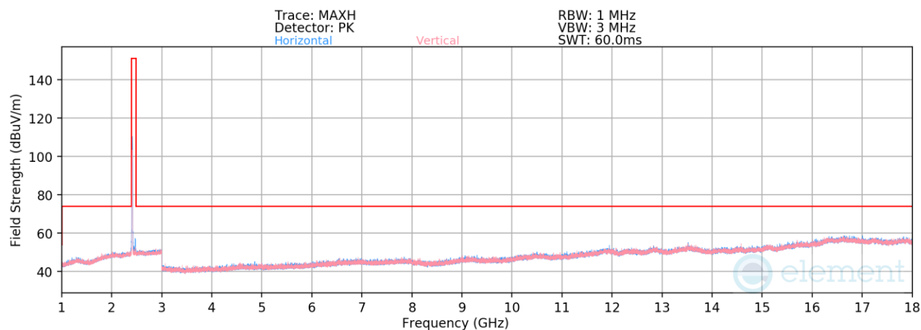
Plot 7-94. Radiated Spurious Plot above 1GHz (802.11b – Ch. 1) MIMO
