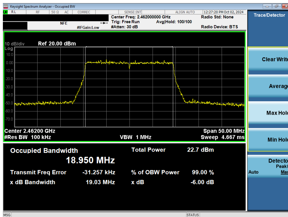
Plot 7-15. 6dB Bandwidth Plot (802.11ax/be (2.4GHz) – Ch. 11) MIMO ANT1
