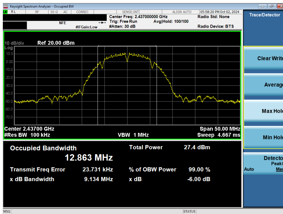
Plot 7-17. 6dB Bandwidth Plot (802.11b – Ch. 6) MIMO ANT2
