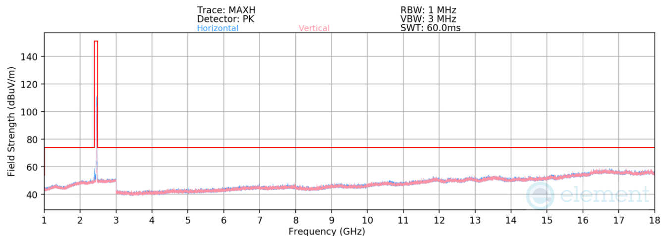
Plot 7-96. Radiated Spurious Plot above 1GHz (802.11b – Ch. 11) MIMO
