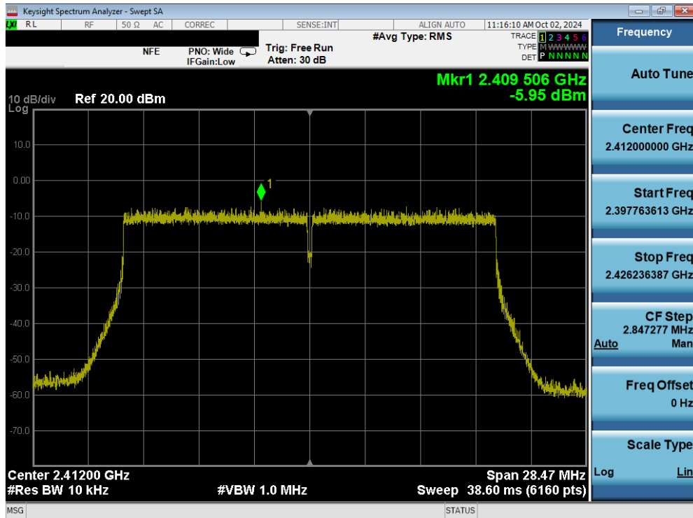
Plot 7-43. Power Spectral Density Plot (802.11ax/be (2.4GHz) – Ch. 1) MIMO ANT1
