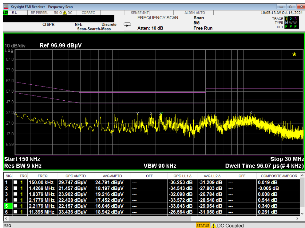
Plot 7-105. Line Conducted Plot with 802.11b (N) - WCP
