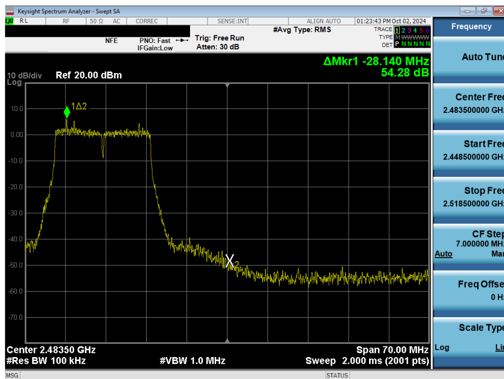
Plot 7-64. Band Edge Plot (802.11g – Ch. 11) MIMO ANT1
