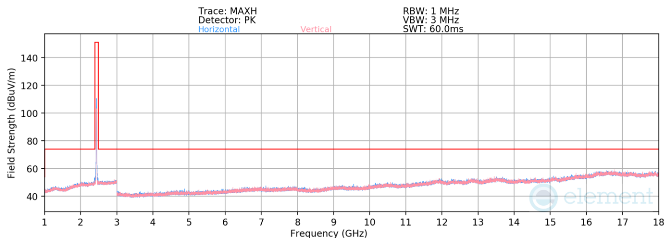
Plot 7-95. Radiated Spurious Plot above 1GHz (802.11b – Ch. 6) MIMO
