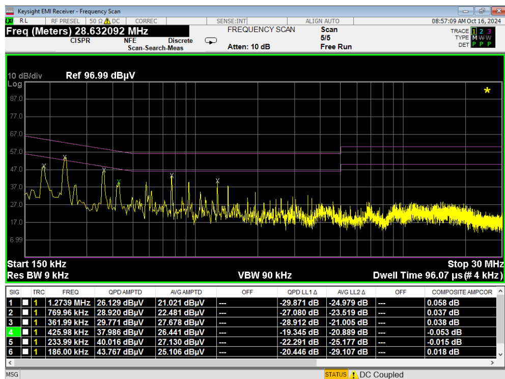
Plot 7-102. Line Conducted Plot with 802.11b (L1)
