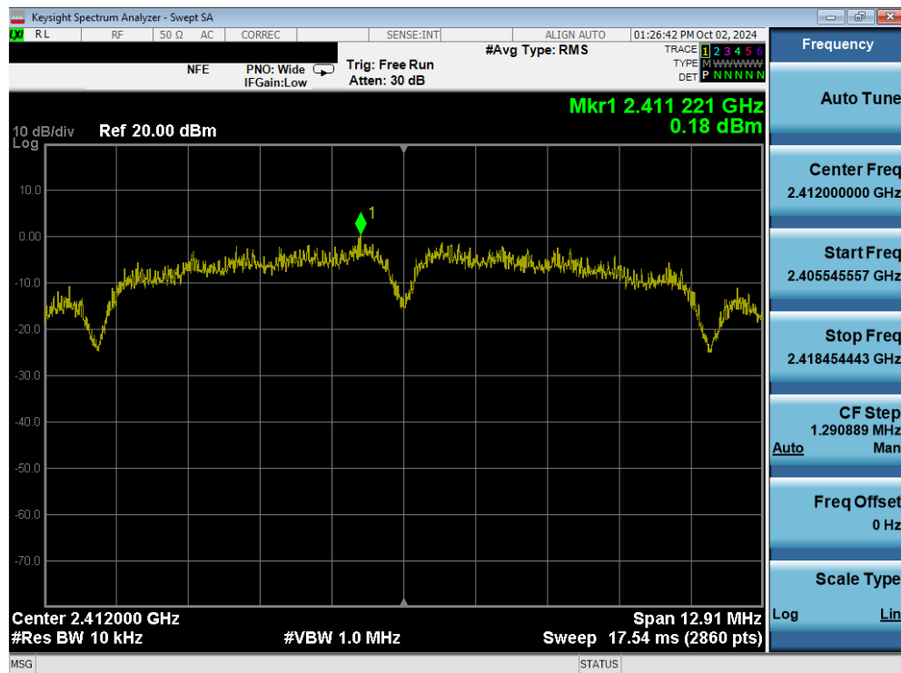
Plot 7-31. Power Spectral Density Plot (802.11b – Ch. 1) MIMO ANT1
