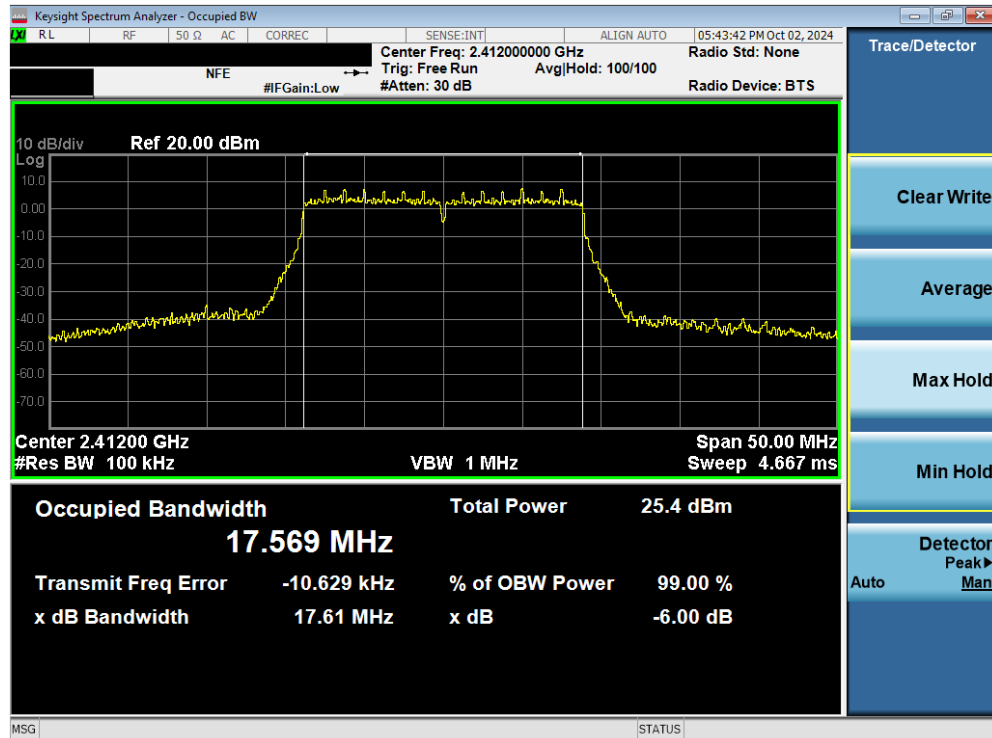
Plot 7-22. 6dB Bandwidth Plot (802.11n (2.4GHz) – Ch. 1) MIMO ANT2
