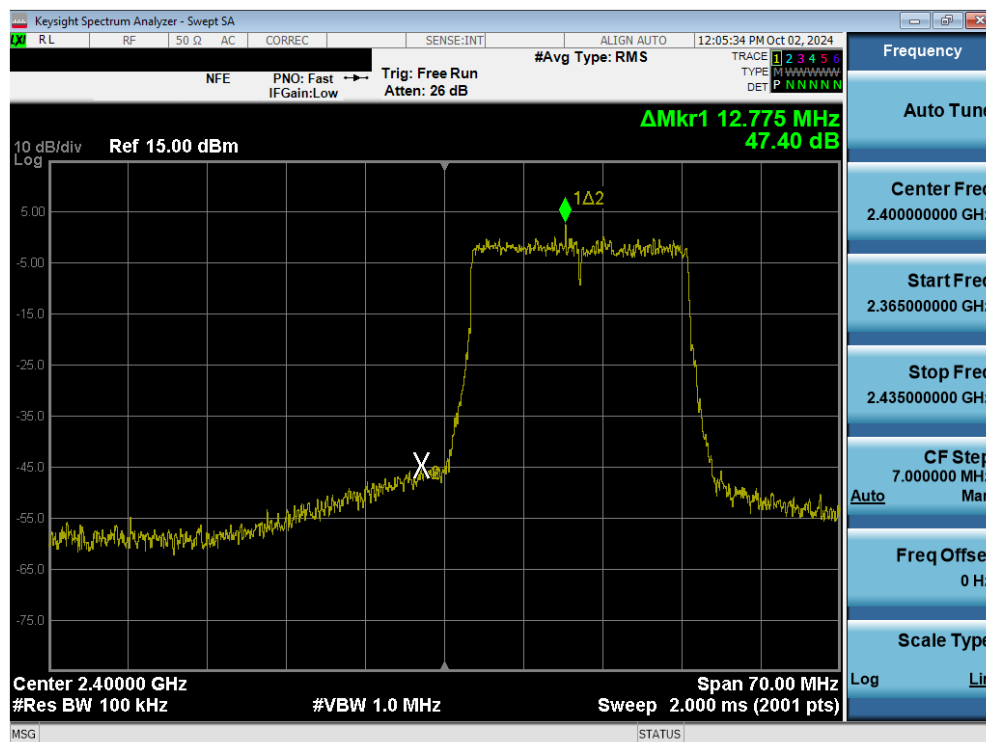
Plot 7-69. Band Edge Plot (802.11ax/be (2.4GHz) – Ch. 1) MIMO ANT1
