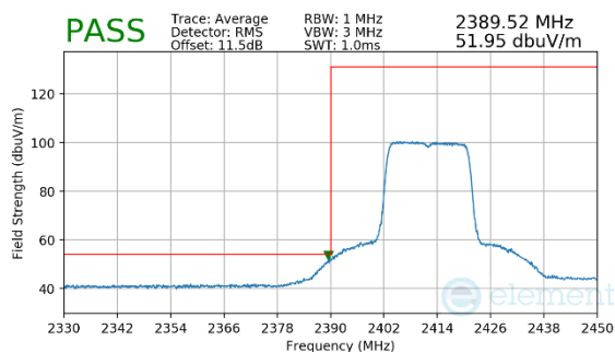
Plot 7-98. Radiated Restricted Lower Band Edge Measurement (Average)
