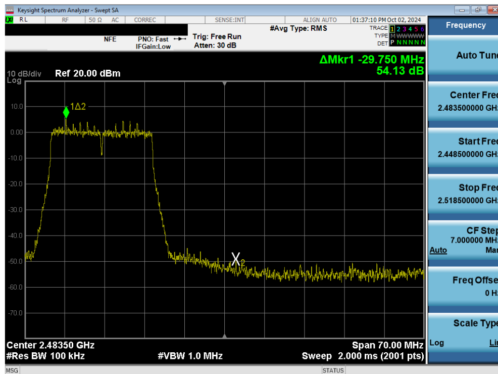
Plot 7-80. Band Edge Plot (802.11ax/be (2.4GHz) – Ch. 11) MIMO ANT2
