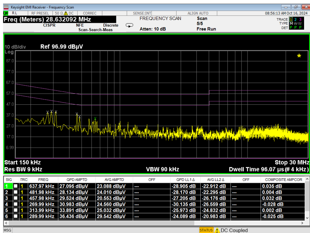
Plot 7-103. Line Conducted Plot with 802.11b (N)
