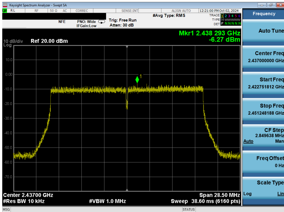
Plot 7-44. Power Spectral Density Plot (802.11ax/be (2.4GHz) – Ch. 6) MIMO ANT1
