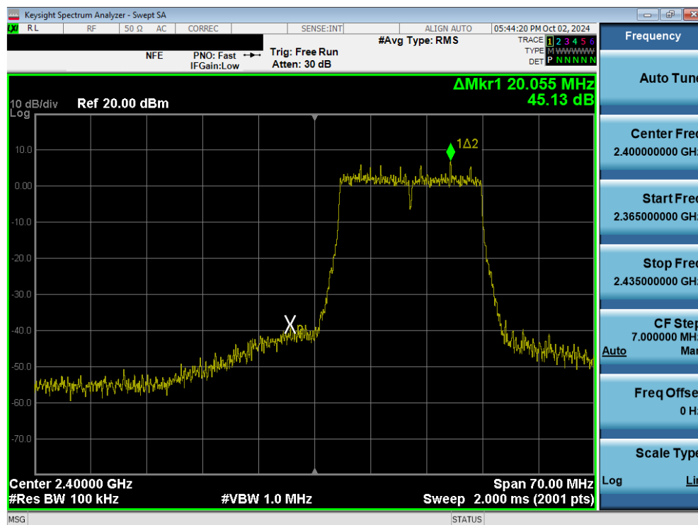
Plot 7-75. Band Edge Plot (802.11n (2.4GHz) – Ch. 1) MIMO ANT2
