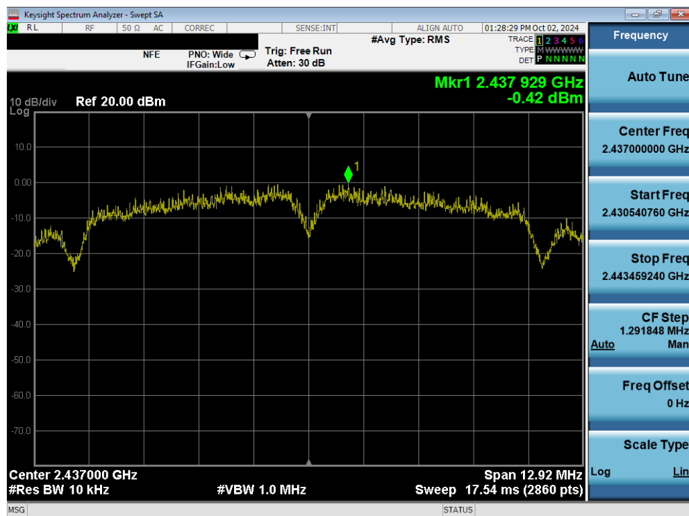
Plot 7-32. Power Spectral Density Plot (802.11b – Ch. 6) MIMO ANT1
