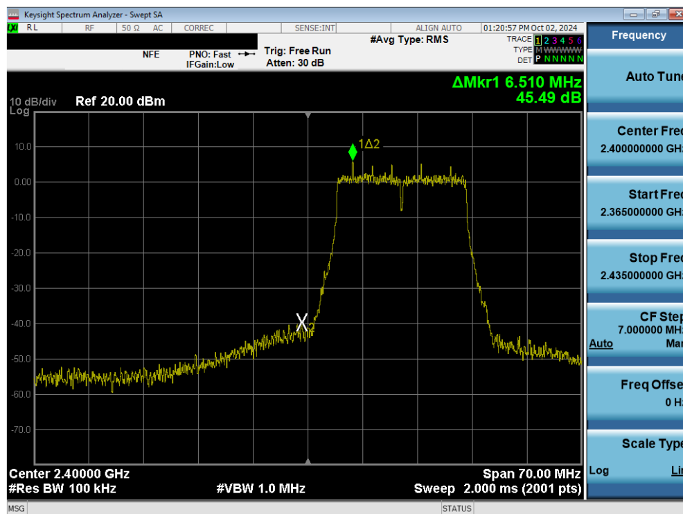
Plot 7-63. Band Edge Plot (802.11g– Ch. 1) MIMO ANT1
