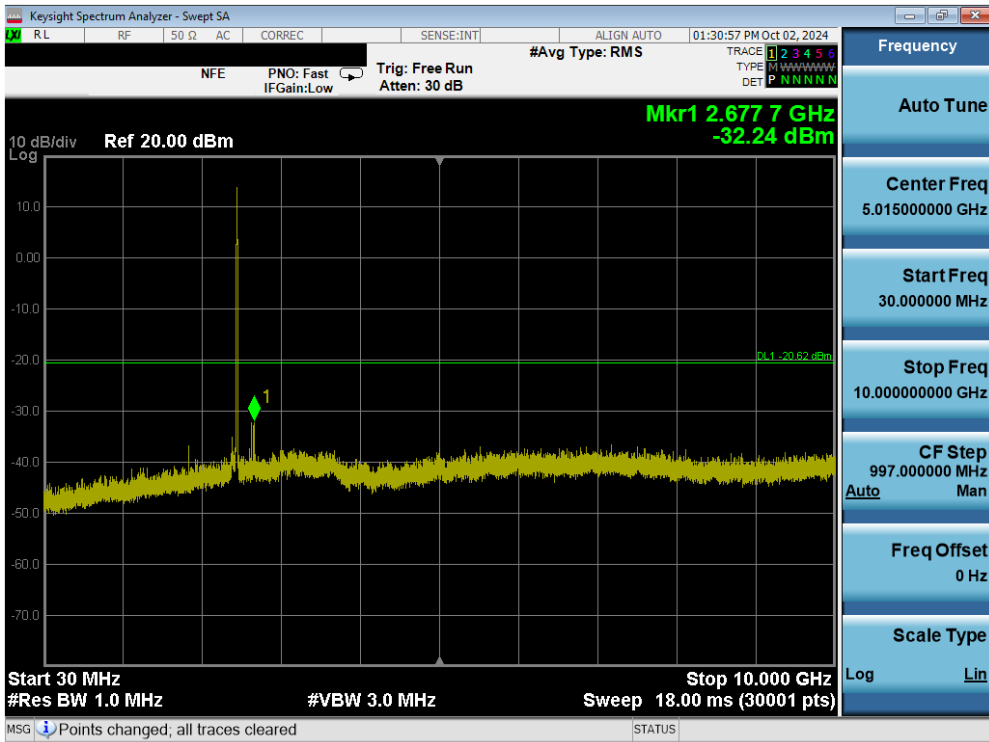
Plot 7-85. Conducted Spurious Plot (802.11b – Ch. 11) MIMO ANT1
