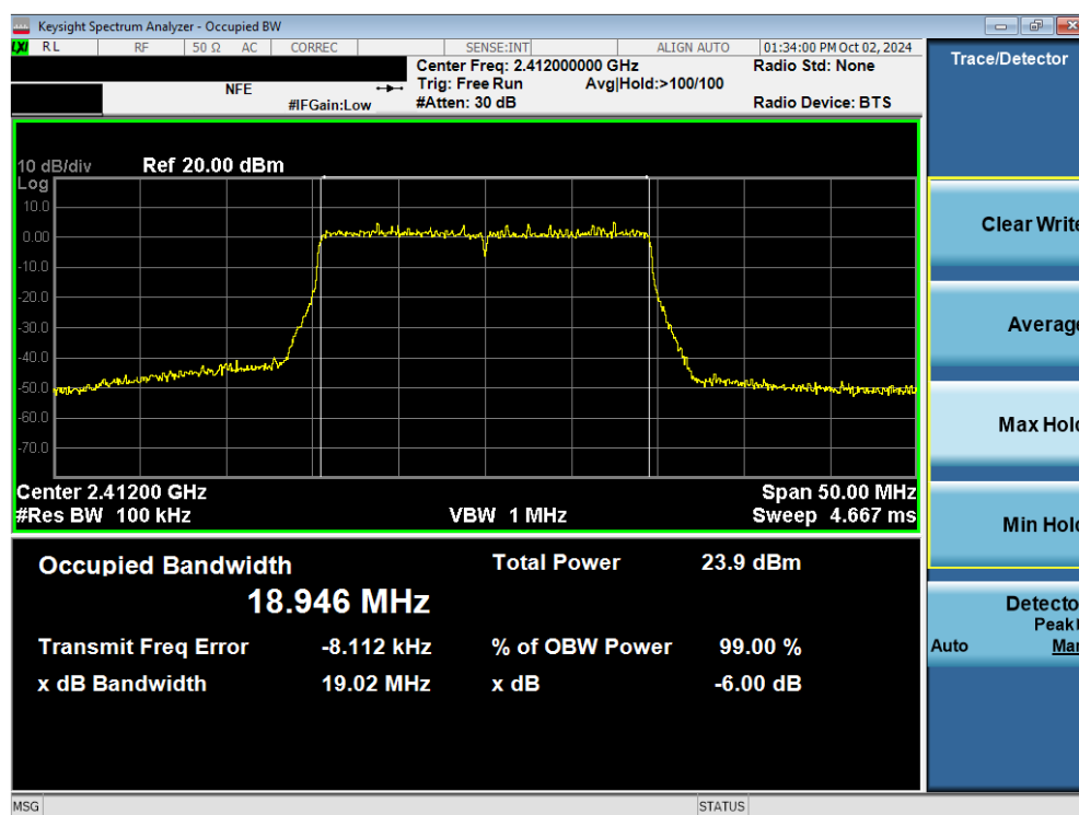
Plot 7-28. 6dB Bandwidth Plot (802.11ax/be (2.4GHz) – Ch. 1) MIMO ANT2
