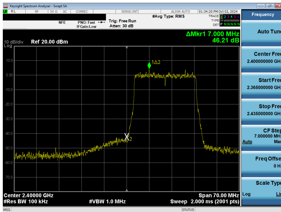
Plot 7-79. Band Edge Plot (802.11ax/be (2.4GHz) – Ch. 1) MIMO ANT2
