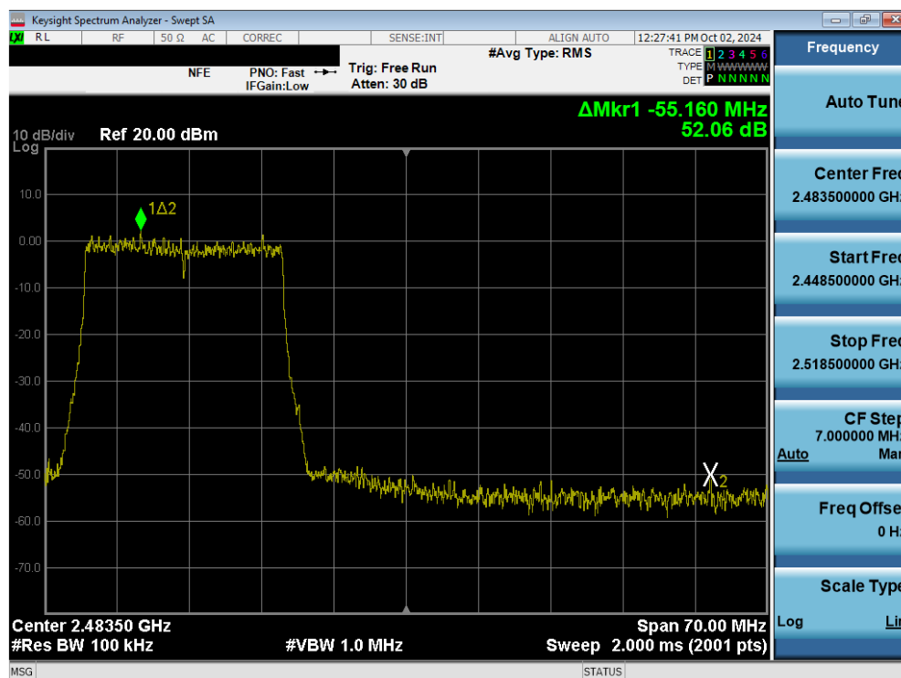
Plot 7-70. Band Edge Plot (802.11ax/be (2.4GHz) – Ch. 11) MIMO ANT1
