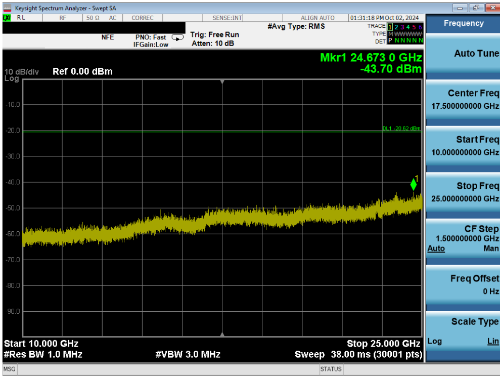
Plot 7-86. Conducted Spurious Plot (802.11b – Ch. 11) MIMO ANT1
