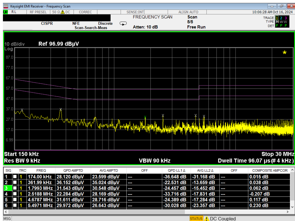
Plot 7-104. Line Conducted Plot with 802.11b (L1) - WCP
