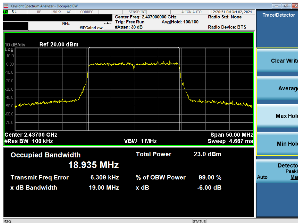
Plot 7-14. 6dB Bandwidth Plot (802.11ax/be (2.4GHz) – Ch. 6) MIMO ANT1
