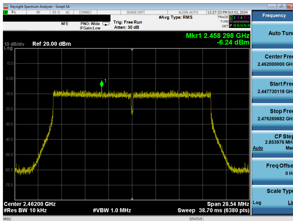
Plot 7-45. Power Spectral Density Plot (802.11ax/be (2.4GHz) – Ch. 11) MIMO ANT1
