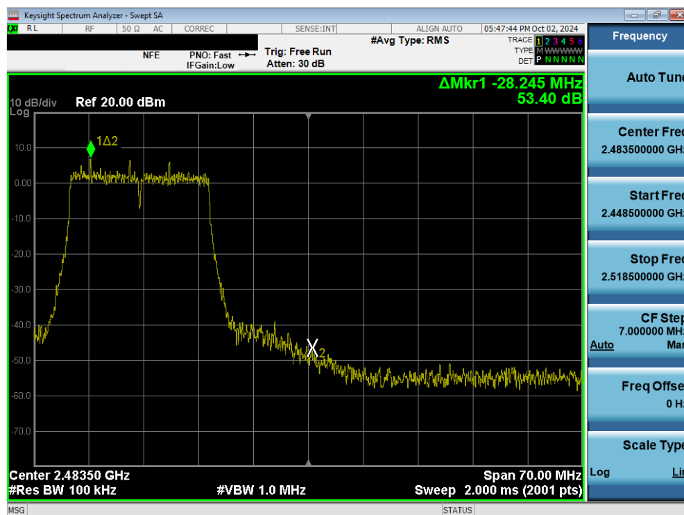
Plot 7-76. Band Edge Plot (802.11n (2.4GHz) – Ch. 11) MIMO ANT2
