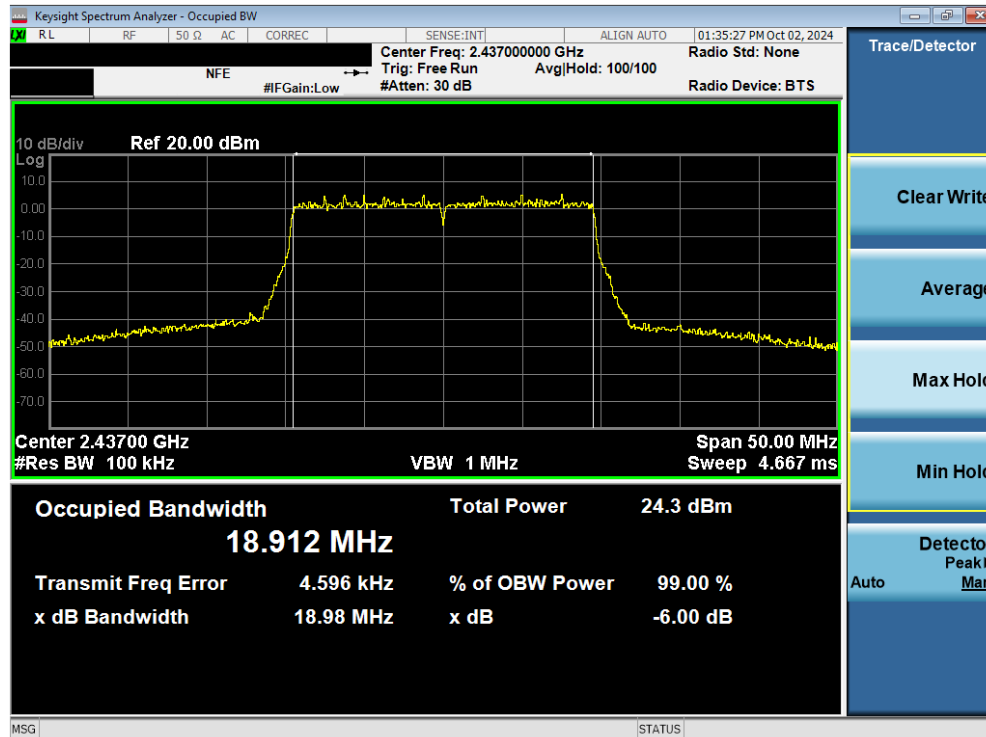
Plot 7-29. 6dB Bandwidth Plot (802.11ax/be (2.4GHz) – Ch. 6) MIMO ANT2
