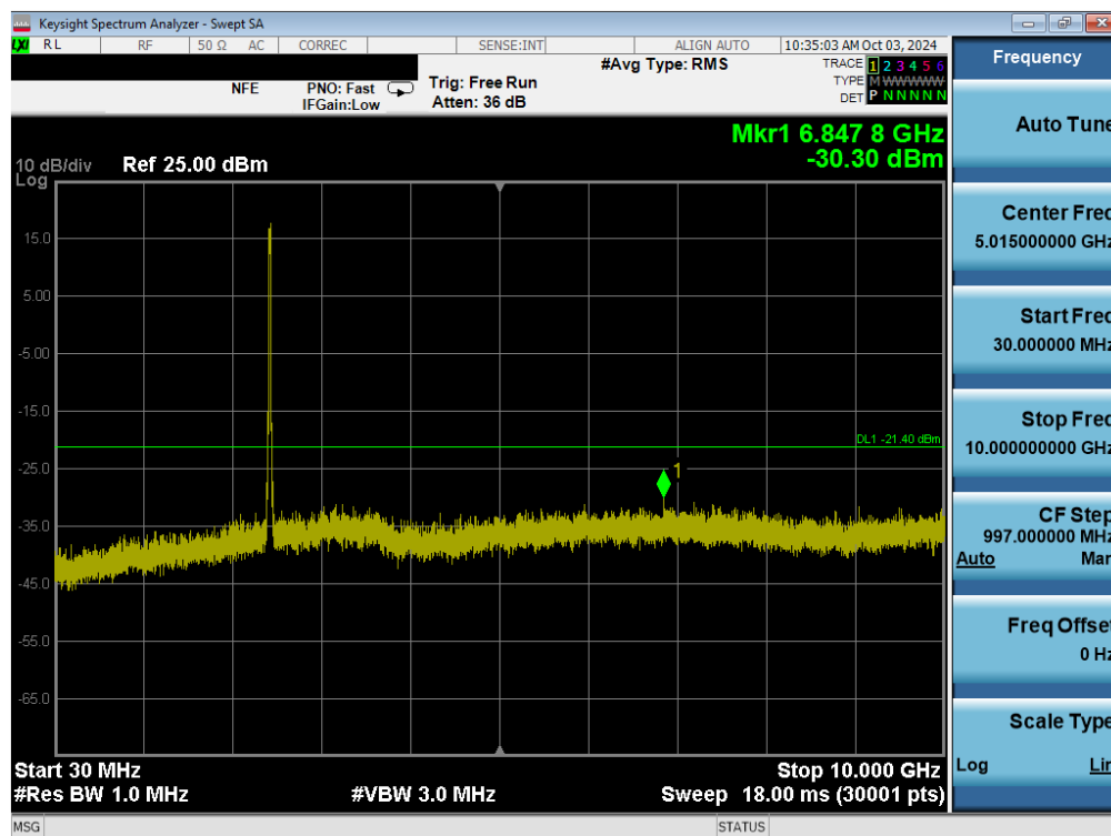
Plot 7-53. Conducted Spurious Plot MIMO ANT2 (802.11ax/be OFDMA – 242 Tones – Ch. 6)
