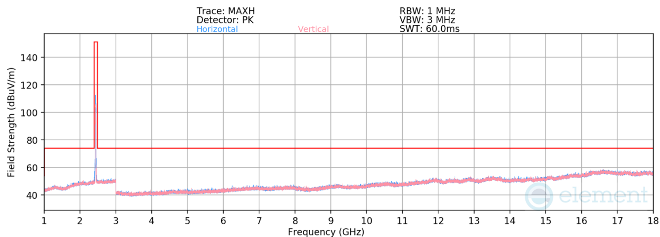
Plot 7-58. Radiated Spurious Plot above 1GHz MIMO (802.11ax/be OFDMA – 26 Tones – Ch. 6)
