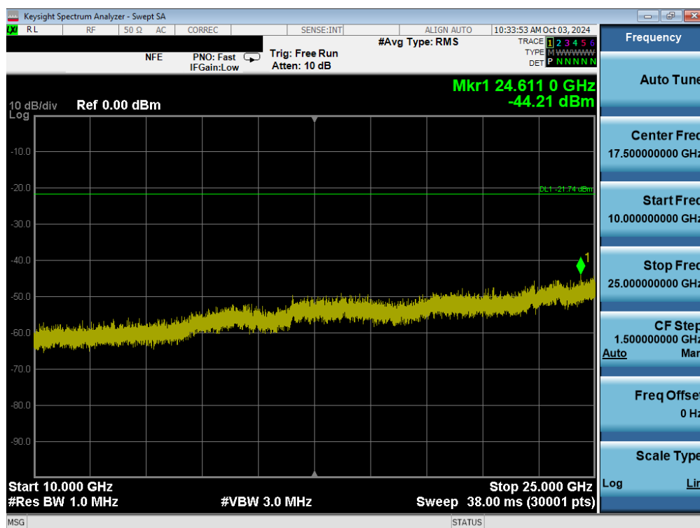
Plot 7-52. Conducted Spurious Plot MIMO ANT2 (802.11ax/be OFDMA – 242 Tones – Ch. 1)
