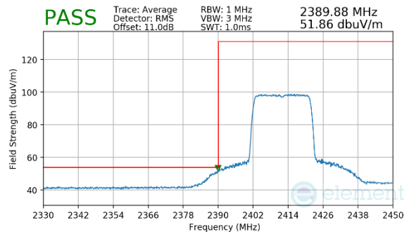
Plot 7-69. Radiated Restricted Lower Band Edge Measurement MIMO (Average – 242 Tones)
