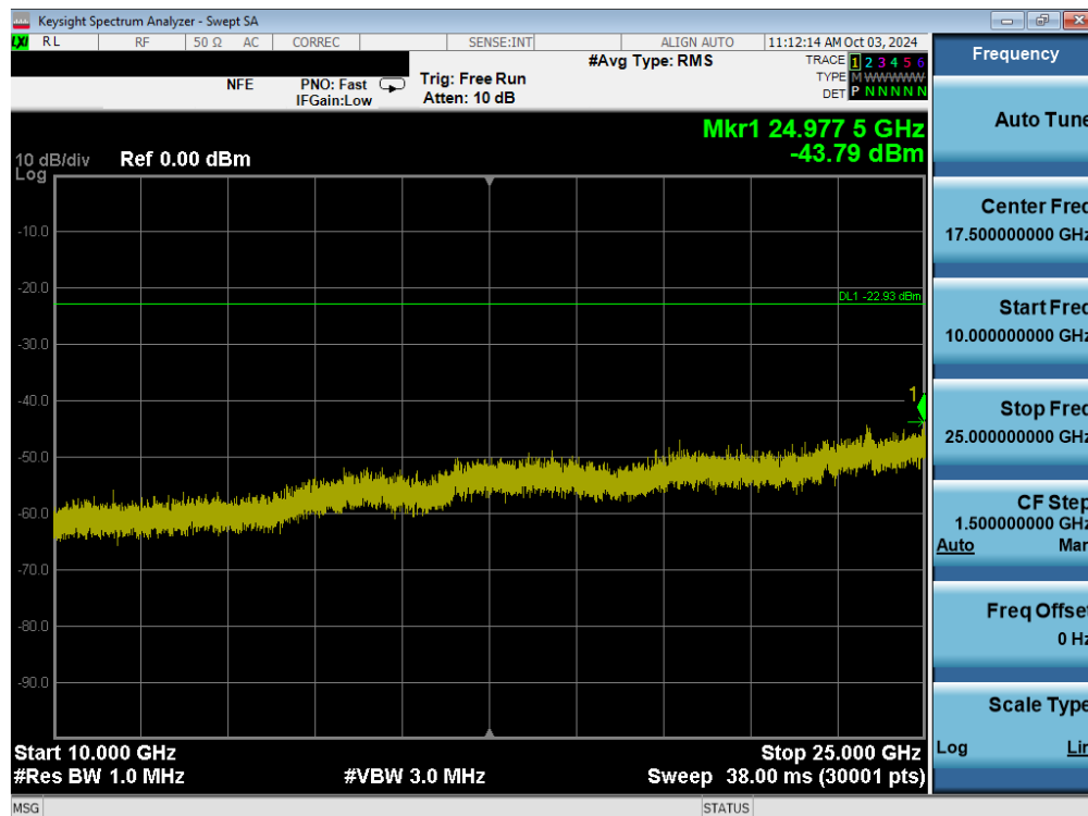
Plot 7-44. Conducted Spurious Plot MIMO ANT1 (802.11ax/be OFDMA – 242 Tones – Ch. 11)
