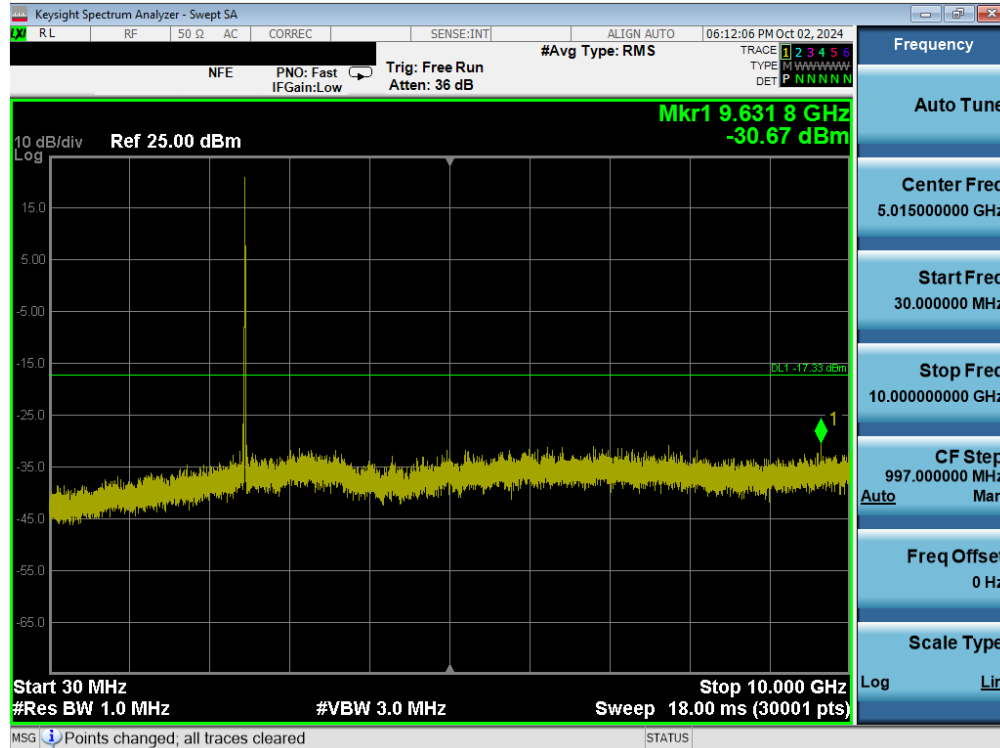
Plot 7-49. Conducted Spurious Plot MIMO ANT2 (802.11ax/be OFDMA – 26 Tones – Ch. 11)
