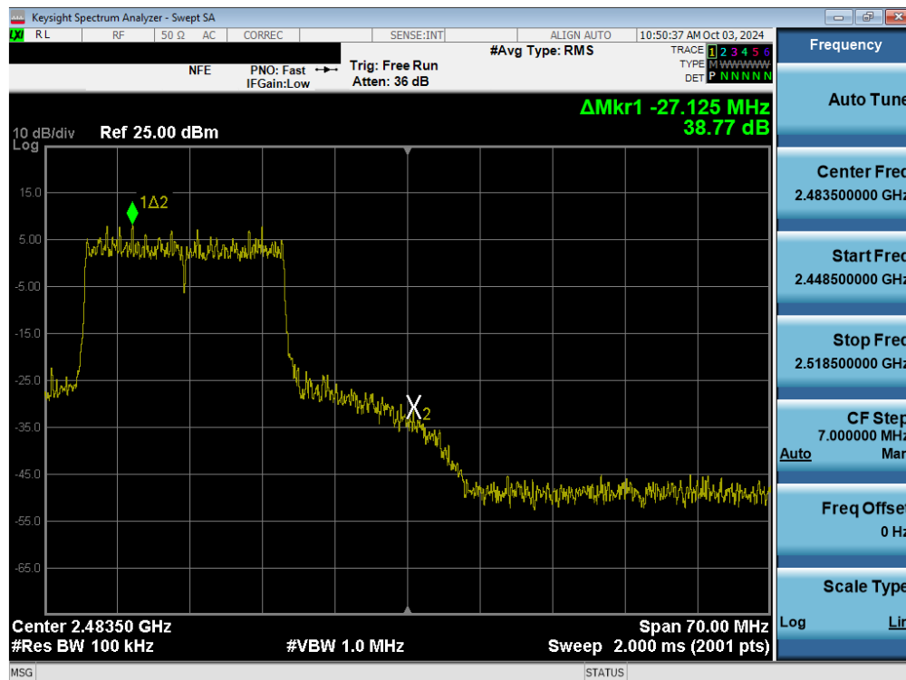
Plot 7-32. Band Edge Plot MIMO ANT2 (802.11ax/be OFDMA – 242 Tones – Ch. 11)
