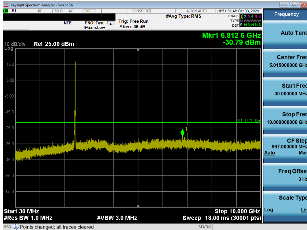
Plot 7-55. Conducted Spurious Plot MIMO ANT2 (802.11ax/be OFDMA – 242 Tones – Ch. 11)
