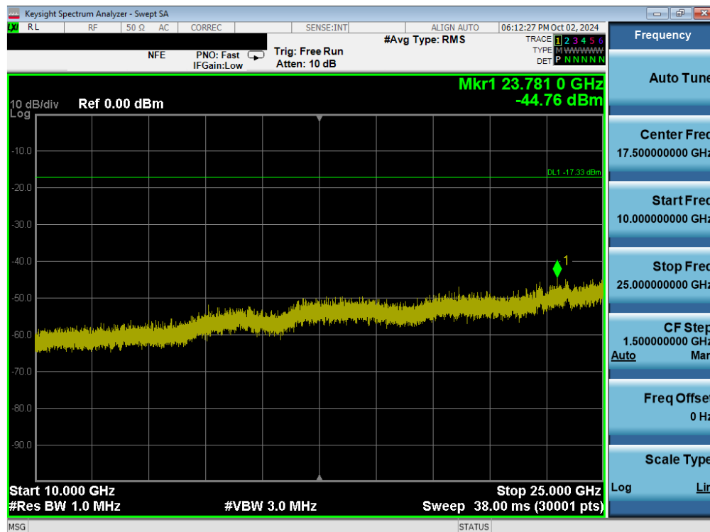
Plot 7-50. Conducted Spurious Plot MIMO ANT2 (802.11ax/be OFDMA – 26 Tones – Ch. 11)
