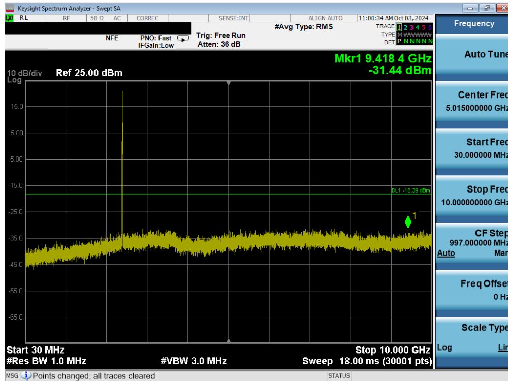
Plot 7-45. Conducted Spurious Plot MIMO ANT1 (802.11ax/be OFDMA – 26 Tones – Ch. 1)
