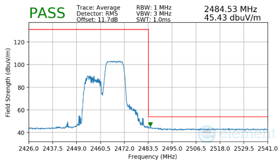
Plot 7-67. Radiated Restricted Upper Band Edge Measurement MIMO (Average – 106 Tones)
