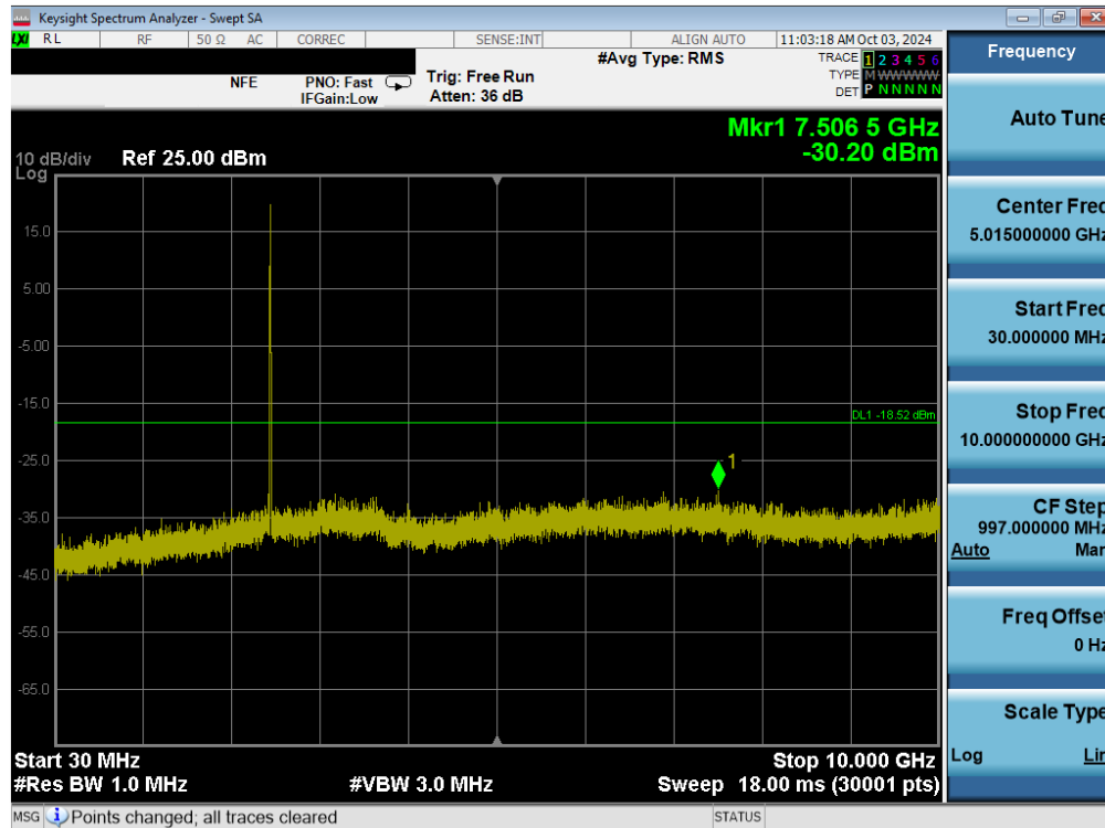
Plot 7-37. Conducted Spurious Plot MIMO ANT1 (802.11ax/be OFDMA – 26 Tones – Ch. 11)
