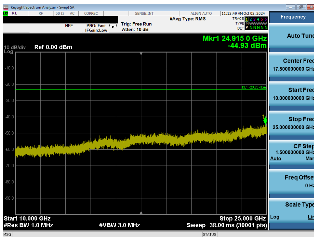
Plot 7-40. Conducted Spurious Plot MIMO ANT1 (802.11ax/be OFDMA – 242 Tones – Ch. 1)
