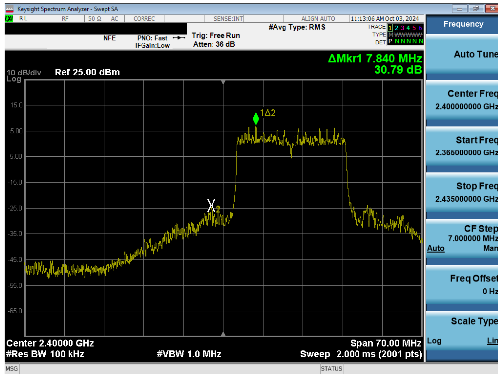
Plot 7-27. Band Edge Plot MIMO ANT1 (802.11ax/be OFDMA – 242 Tones – Ch. 1)
