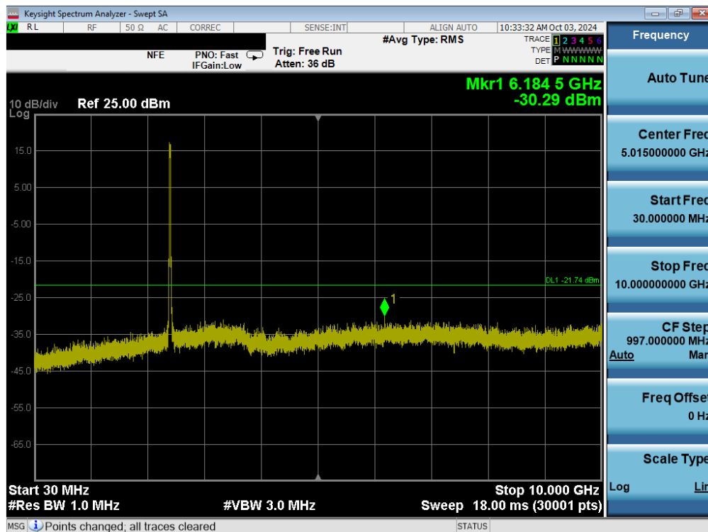
Plot 7-51. Conducted Spurious Plot MIMO ANT2 (802.11ax/be OFDMA – 242 Tones – Ch. 1)
