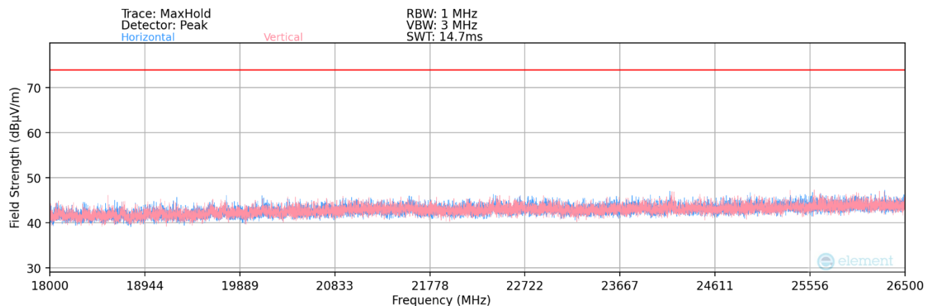
Plot 7-64. Radiated Spurious Plot above 18GHz MIMO (802.11ax/be OFDMA – 242 Tones)
