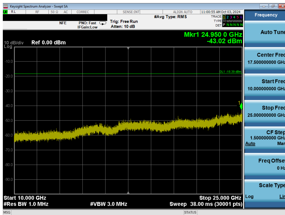
Plot 7-34. Conducted Spurious Plot MIMO ANT1 (802.11ax/be OFDMA – 26 Tones – Ch. 1)
