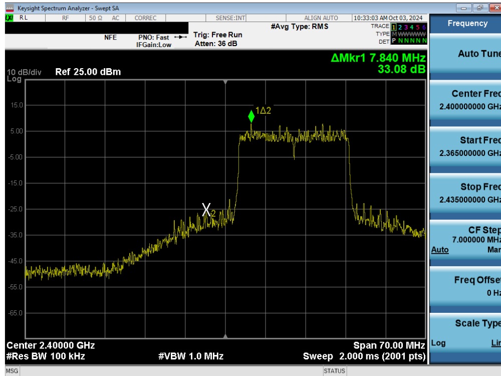
Plot 7-31. Band Edge Plot MIMO ANT2 (802.11ax/be OFDMA – 242 Tones – Ch. 1)
