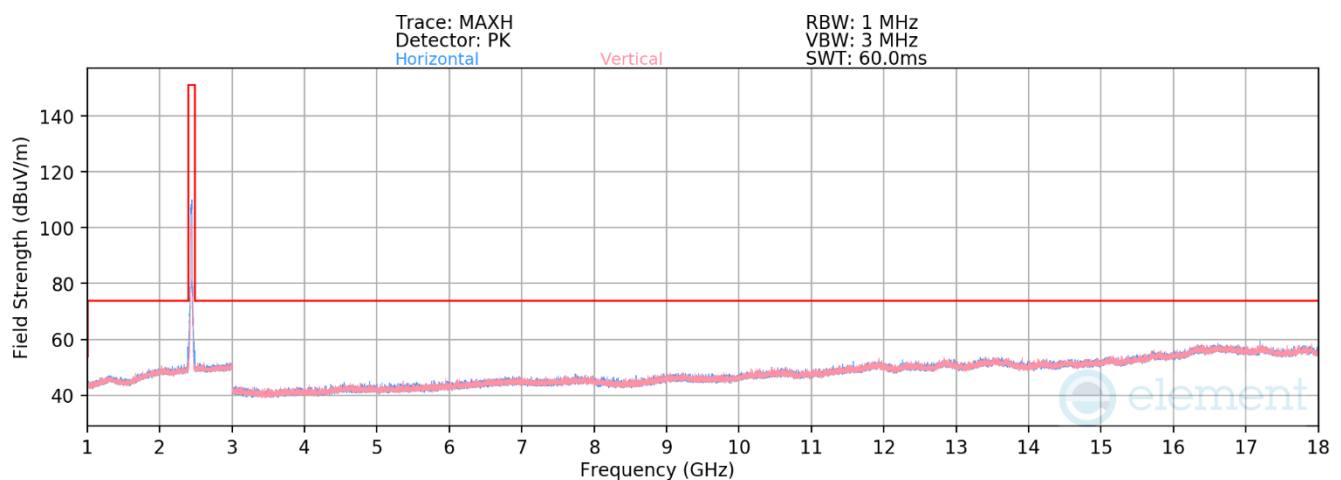
Plot 7-62. Radiated Spurious Plot above 1GHz MIMO (802.11ax/be OFDMA – 242 Tones – Ch. 6)
