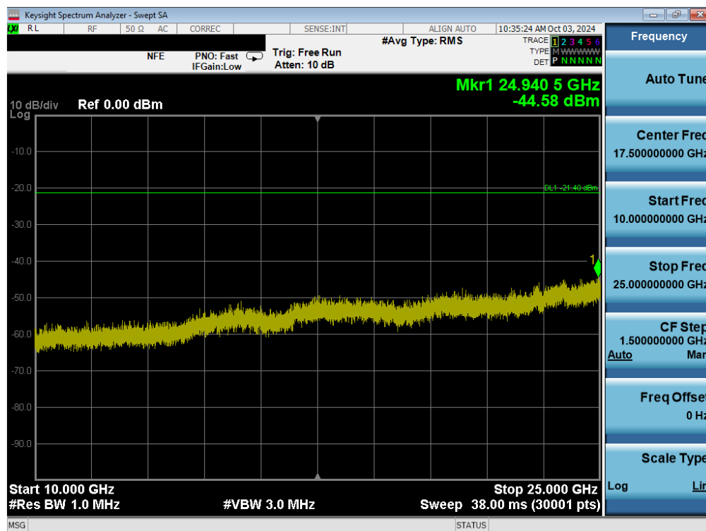
Plot 7-54. Conducted Spurious Plot MIMO ANT2 (802.11ax/be OFDMA – 242 Tones – Ch. 6)
