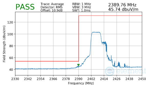
Plot 7-65. Radiated Restricted Lower Band Edge Measurement MIMO (Average – 106 Tones)
