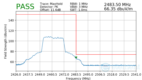
Plot 7-72. Radiated Restricted Upper Band Edge Measurement MIMO (Peak – 242 Tones)
