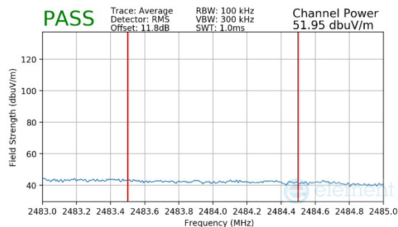
Plot 7-71. Radiated Restricted Upper Band Edge Measurement MIMO (Average – 242 Tones)
