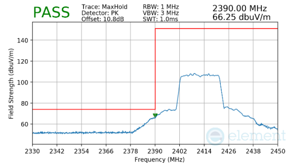
Plot 7-70. Radiated Restricted Lower Band Edge Measurement MIMO (Peak – 242 Tones)
