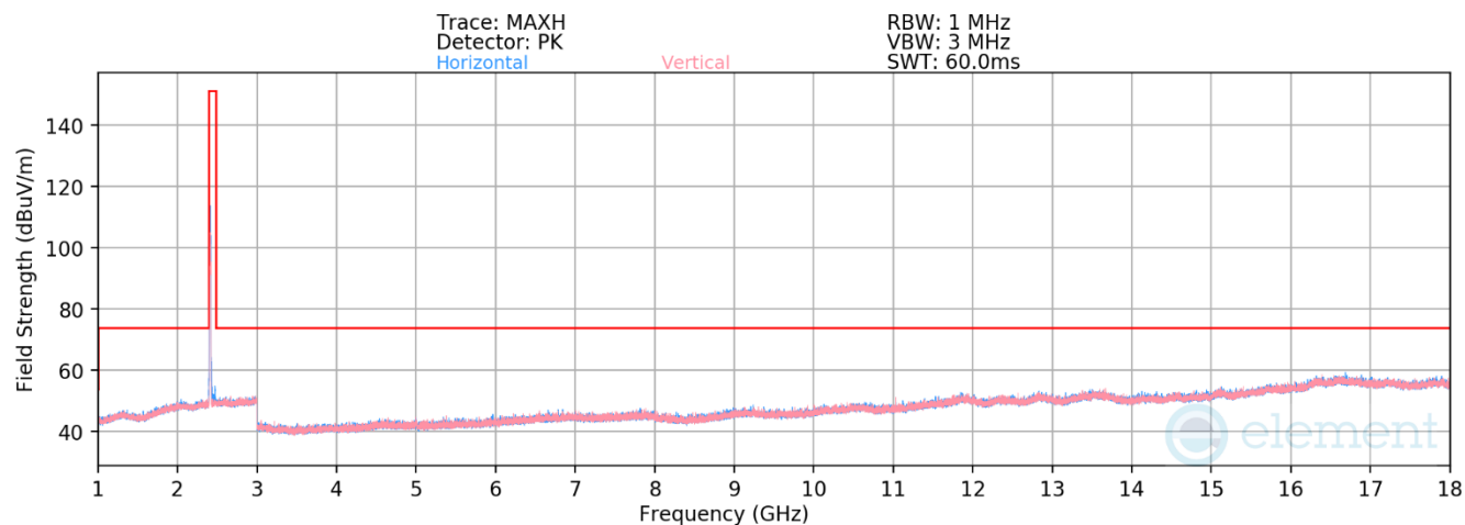
Plot 7-57. Radiated Spurious Plot above 1GHz MIMO (802.11ax/be OFDMA – 26 Tones – Ch. 1)
