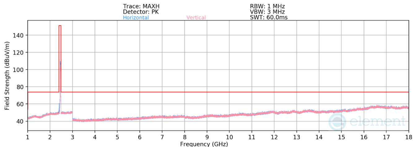
Plot 7-63. Radiated Spurious Plot above 1GHz MIMO (802.11ax/be OFDMA – 242 Tones – Ch. 11)
