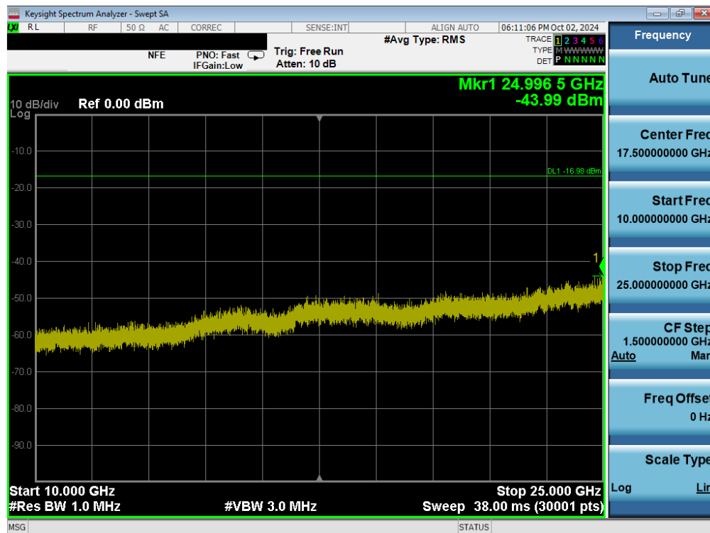
Plot 7-48. Conducted Spurious Plot MIMO ANT2 (802.11ax/be OFDMA – 26 Tones – Ch. 6)
