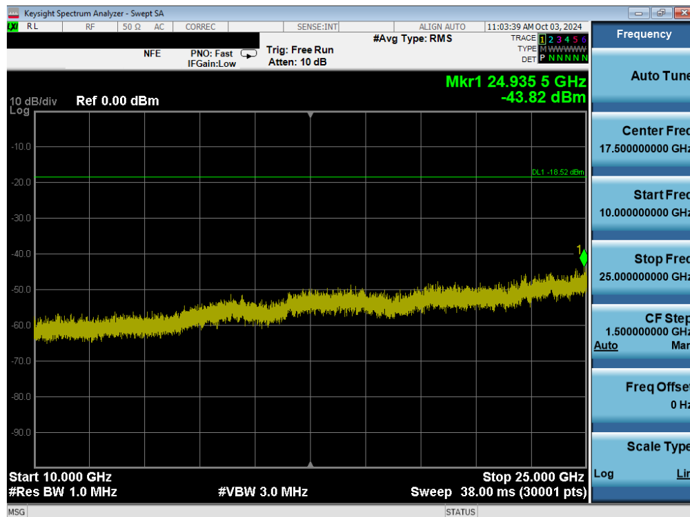
Plot 7-38. Conducted Spurious Plot MIMO ANT1 (802.11ax/be OFDMA – 26 Tones – Ch. 11)
