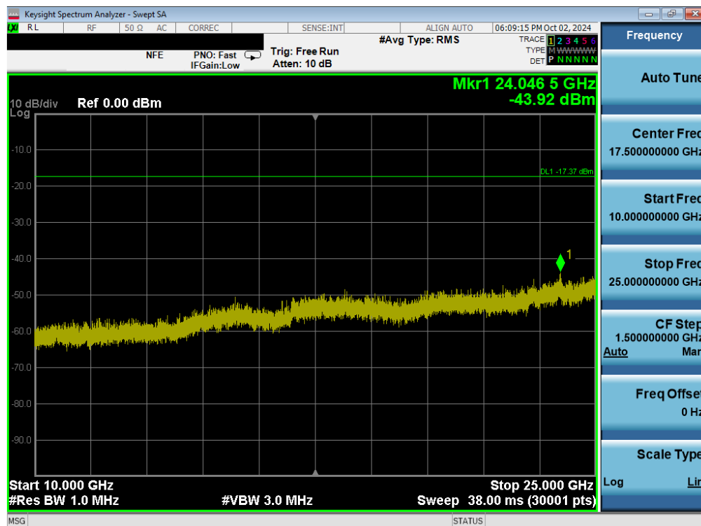
Plot 7-46. Conducted Spurious Plot MIMO ANT2 (802.11ax/be OFDMA – 26 Tones – Ch. 1)
