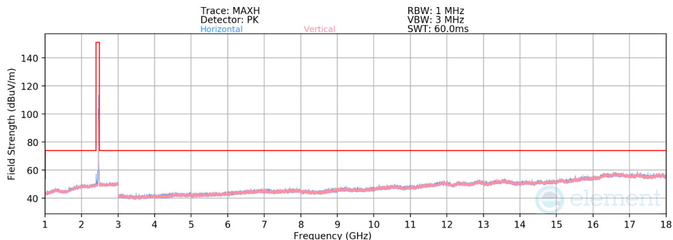
Plot 7-59. Radiated Spurious Plot above 1GHz MIMO (802.11ax/be OFDMA – 26 Tones – Ch. 11)
