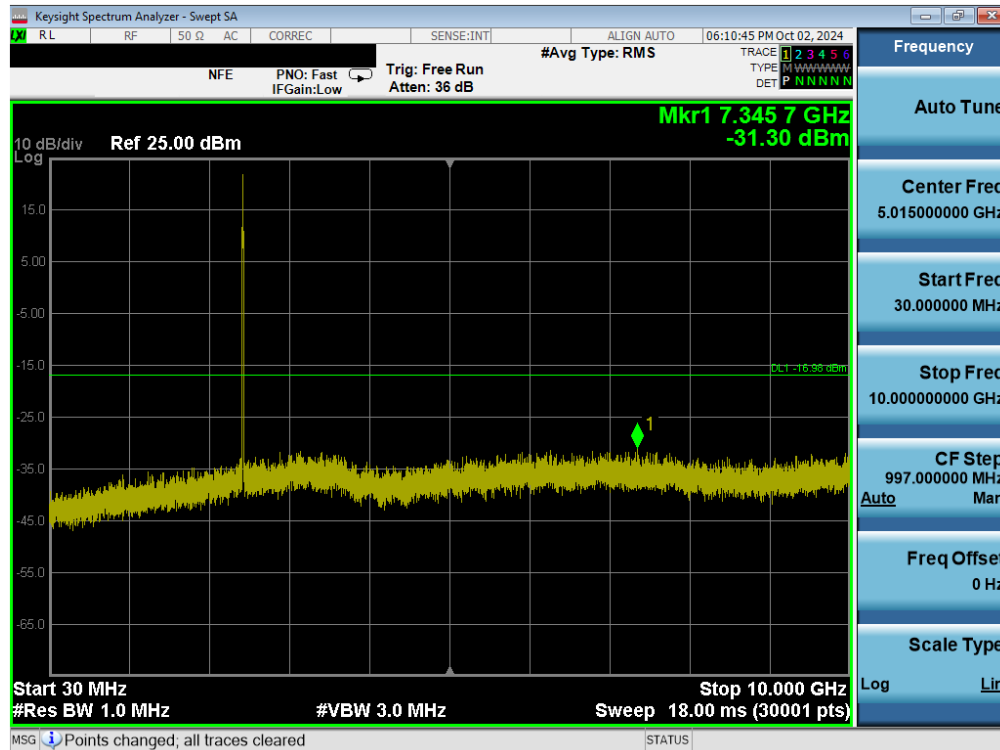
Plot 7-47. Conducted Spurious Plot MIMO ANT2 (802.11ax/be OFDMA – 26 Tones – Ch. 6)
