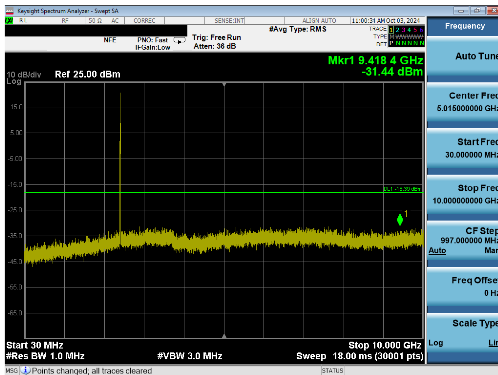
Plot 7-33. Conducted Spurious Plot MIMO ANT1 (802.11ax/be OFDMA – 26 Tones – Ch. 1)
