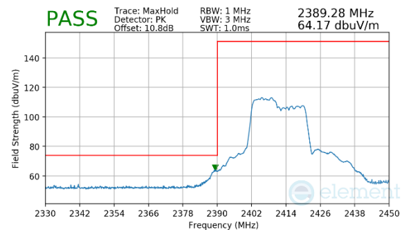
Plot 7-66. Radiated Restricted Lower Band Edge Measurement MIMO (Peak – 106 Tones)
