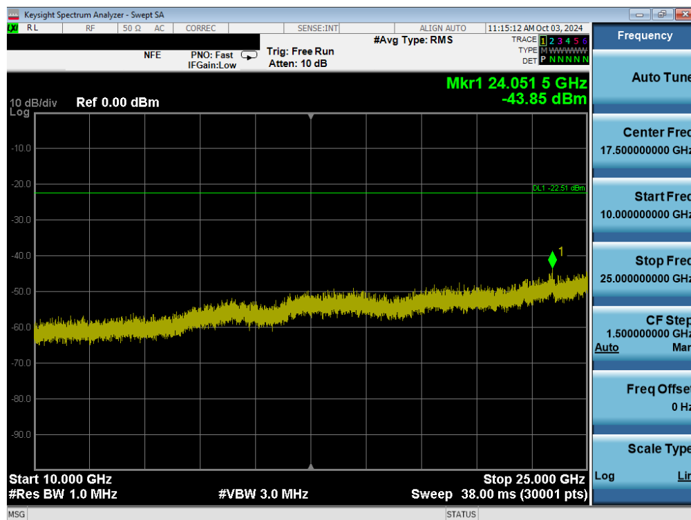
Plot 7-42. Conducted Spurious Plot MIMO ANT1 (802.11ax/be OFDMA – 242 Tones – Ch. 6)
