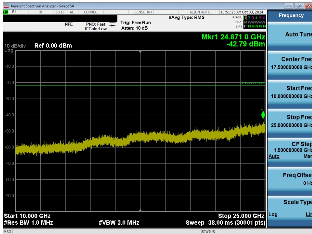
Plot 7-56. Conducted Spurious Plot MIMO ANT2 (802.11ax/be OFDMA – 242 Tones – Ch. 11)
