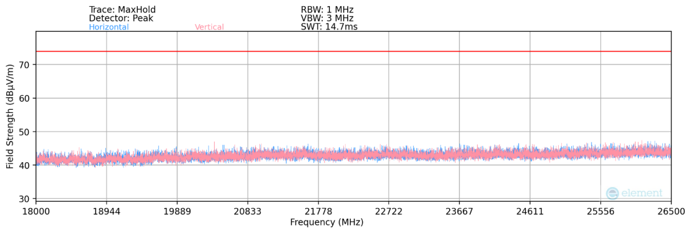
Plot 7-60. Radiated Spurious Plot above 18GHz MIMO (802.11ax/be OFDMA – 26 Tones)
