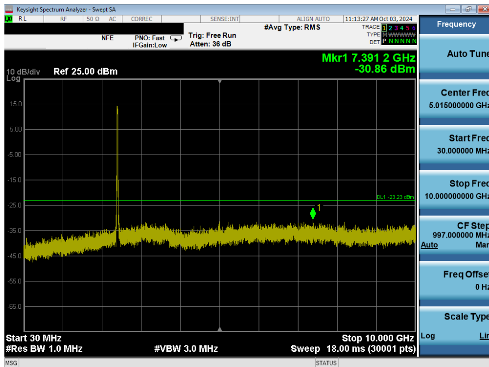
Plot 7-39. Conducted Spurious Plot MIMO ANT1 (802.11ax/be OFDMA – 242 Tones – Ch. 1)
