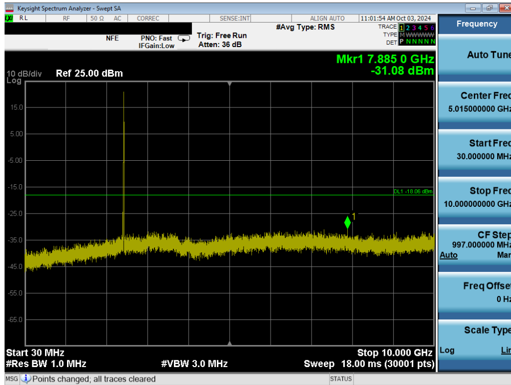
Plot 7-35. Conducted Spurious Plot MIMO ANT1 (802.11ax/be OFDMA – 26 Tones – Ch. 6)
