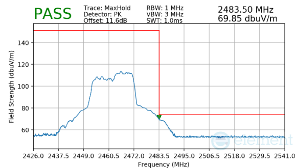
Plot 7-68. Radiated Restricted Upper Band Edge Measurement MIMO (Peak – 106 Tones)
