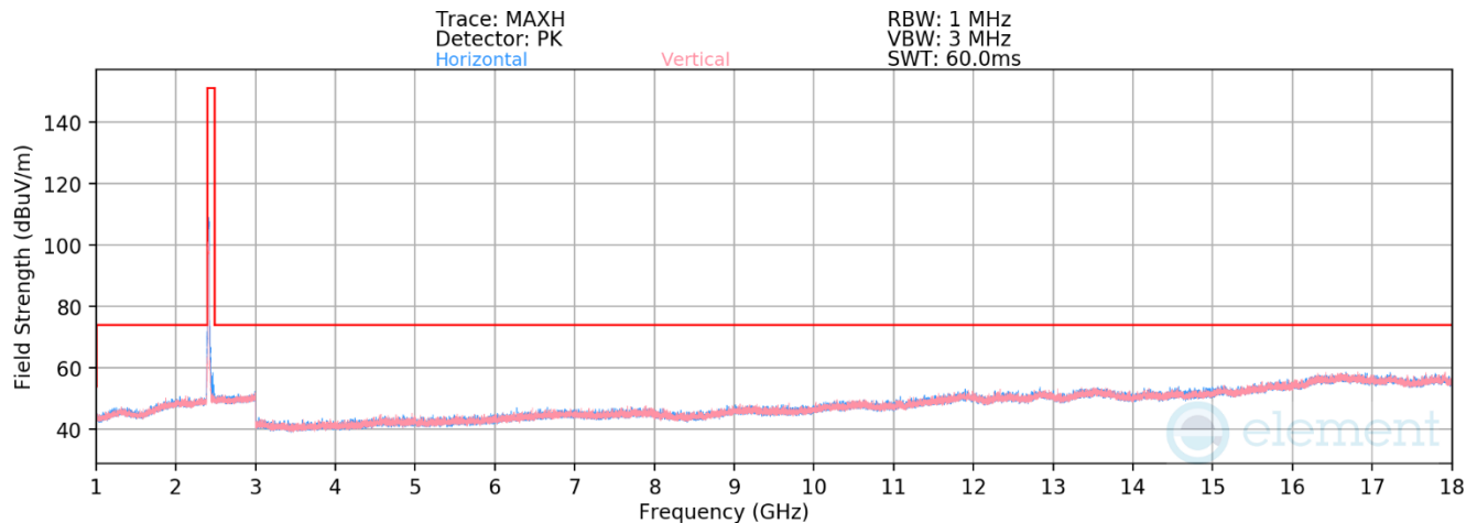
Plot 7-61. Radiated Spurious Plot above 1GHz MIMO (802.11ax/be OFDMA – 242 Tones – Ch. 1)
