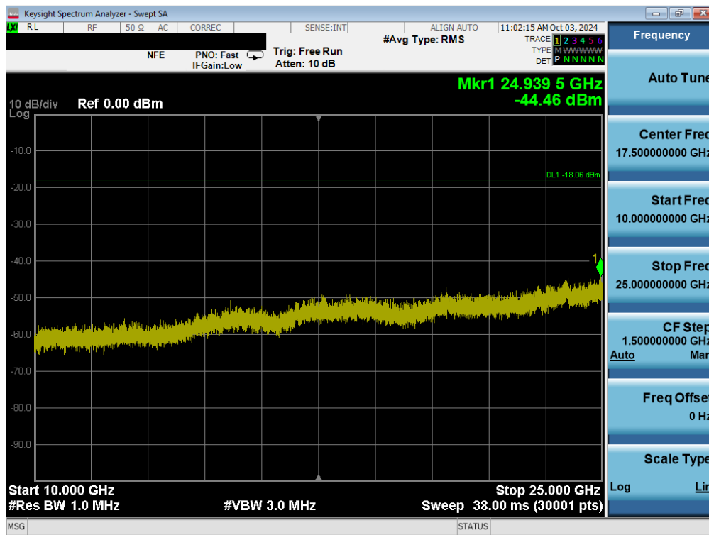
Plot 7-36. Conducted Spurious Plot MIMO ANT1 (802.11ax/be OFDMA – 26 Tones – Ch. 6)
