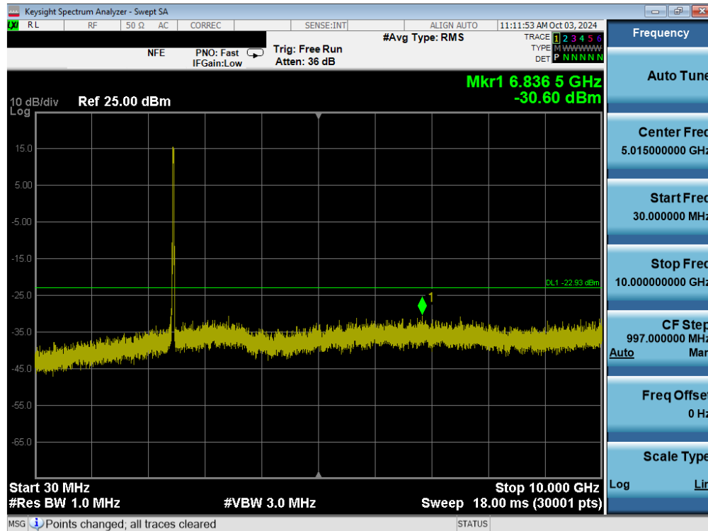
Plot 7-43. Conducted Spurious Plot MIMO ANT1 (802.11ax/be OFDMA – 242 Tones – Ch. 11)
