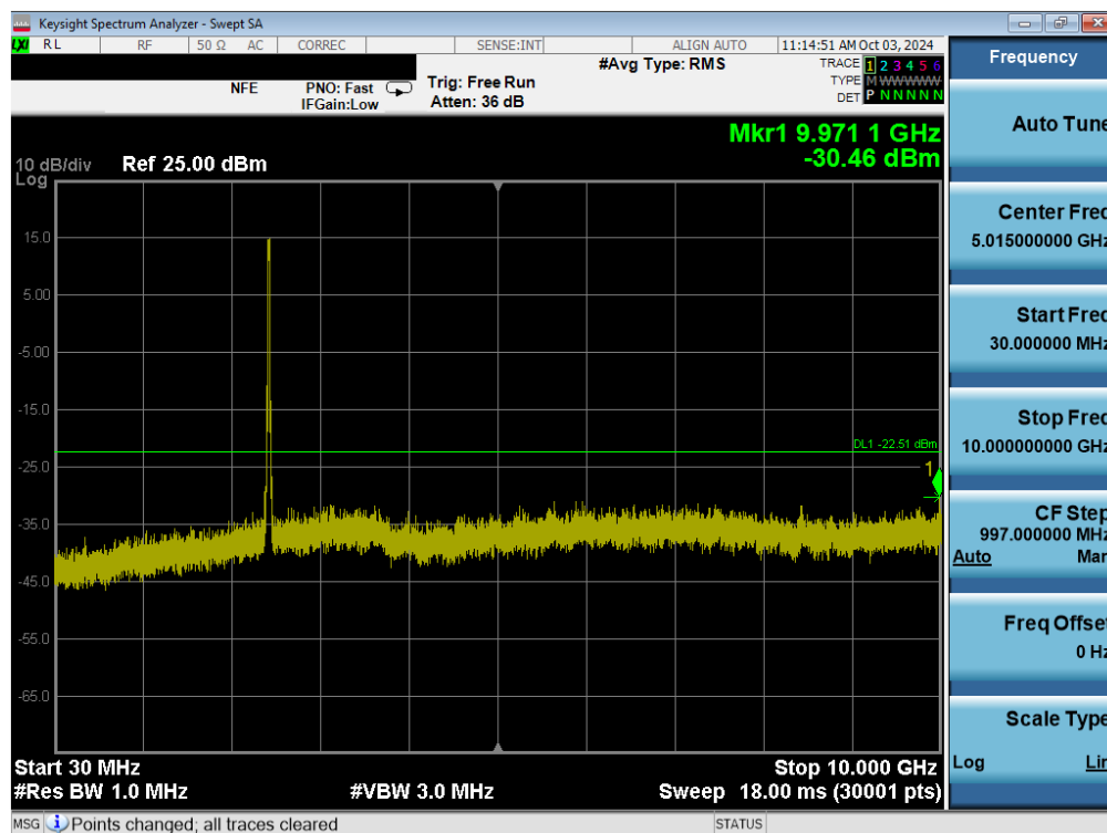
Plot 7-41. Conducted Spurious Plot MIMO ANT1 (802.11ax/be OFDMA – 242 Tones – Ch. 6)
