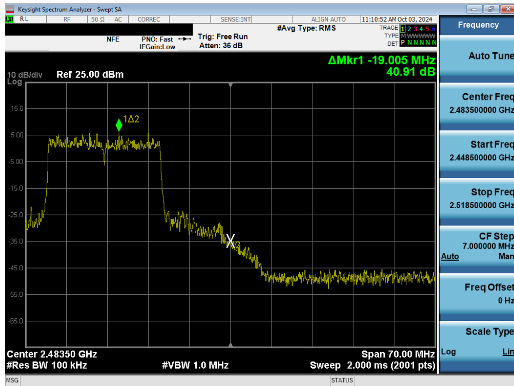
Plot 7-28. Band Edge Plot MIMO ANT1 (802.11ax/be OFDMA – 242 Tones – Ch. 11)
