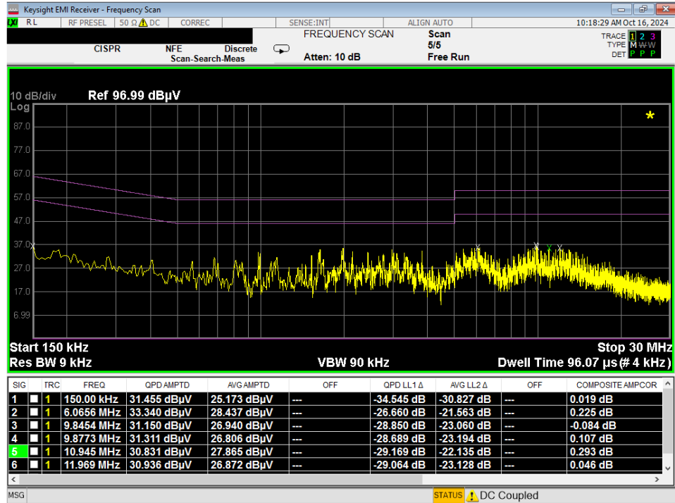
Plot 7-167. Line Conducted Plot with 802.11a UNII Band 5 (L1)
