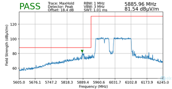
Plot 7-156. Radiated Lower Band Edge Plot MIMO (Peak – UNII Band 5)
