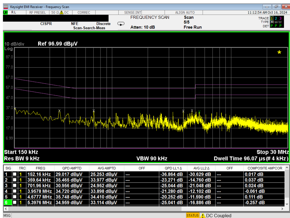
Plot 7-176. Line Conducted Plot with 802.11a UNII Band 5 (N) with WCP
