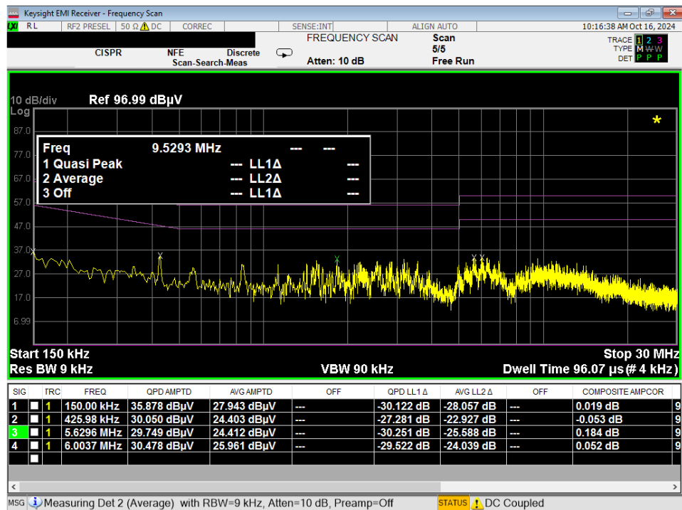
Plot 7-168. Line Conducted Plot with 802.11a UNII Band 5 (N)
