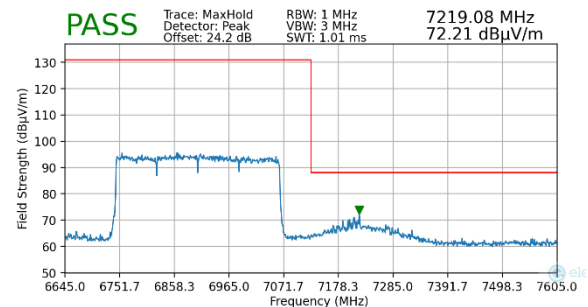
Plot 7-162. Radiated Upper Band Edge Plot MIMO (Peak – UNII Band 8)
