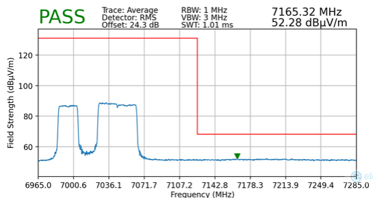
Plot 7-149. Radiated Upper Band Edge Plot MIMO (Average – UNII Band 8)
