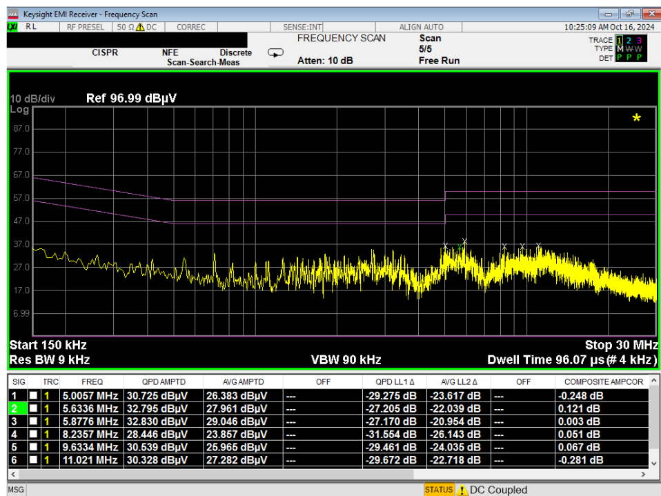
Plot 7-171. Line Conducted Plot with 802.11a UNII Band 7 (L1)
