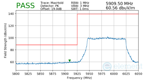
Plot 7-144. Radiated Lower Band Edge Plot MIMO (Peak – UNII Band 5)
