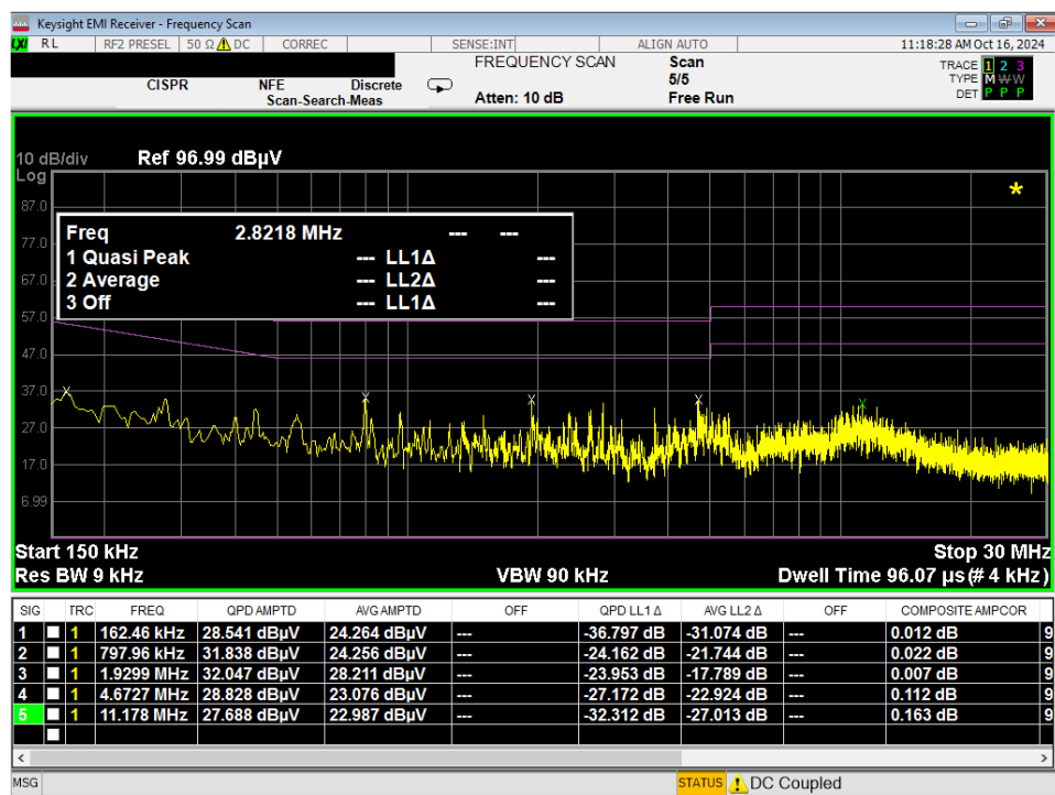
Plot 7-180. Line Conducted Plot with 802.11a UNII Band 7 (N) with WCP
