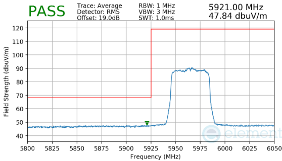
Plot 7-139. Radiated Lower Band Edge Plot MIMO (Average – UNII Band 5)
