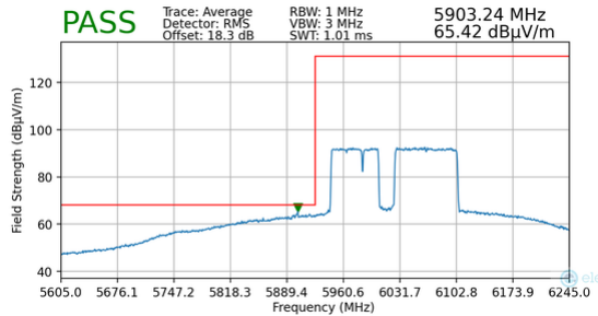
Plot 7-155. Radiated Lower Band Edge Plot MIMO (Average – UNII Band 5)
