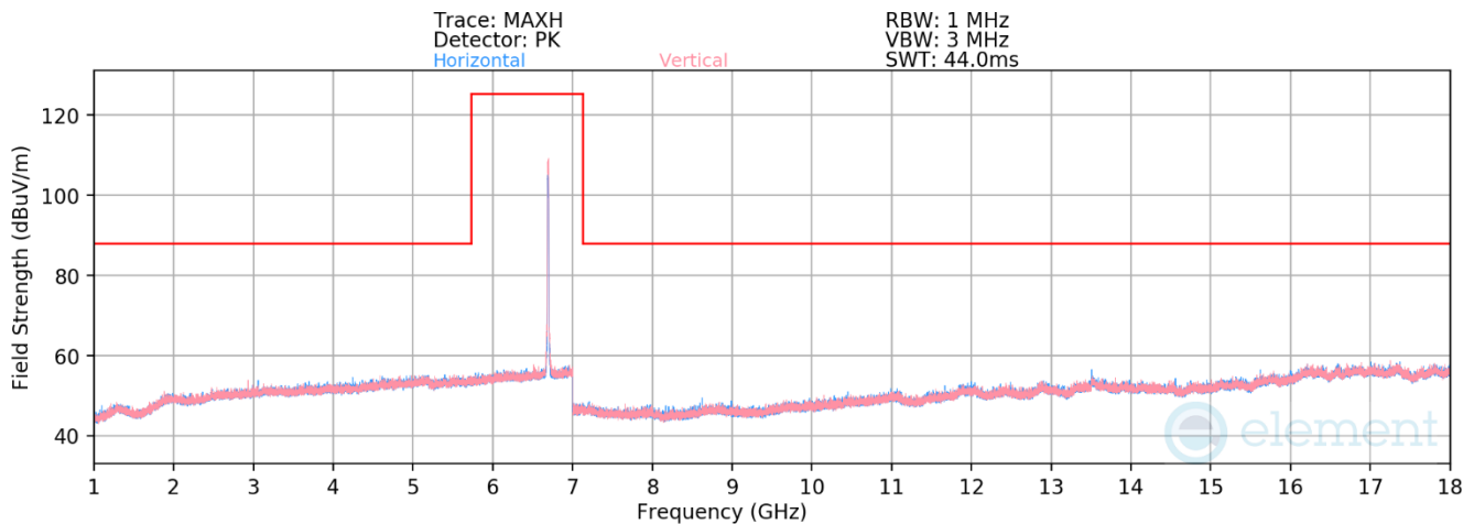
Plot 7-131. Radiated Spurious Plot 1GHz – 18GHz MIMO (802.11a – UNII Band 7 Ch. 149)
