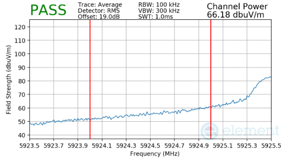
Plot 7-135. Radiated Lower Band Edge Plot MIMO (Average – UNII Band 5)
