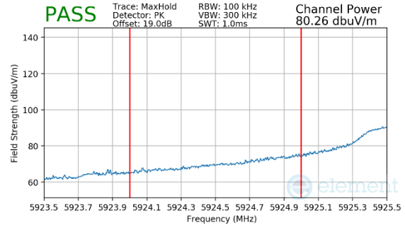
Plot 7-136. Radiated Lower Band Edge Plot MIMO (Peak – UNII Band 5)
