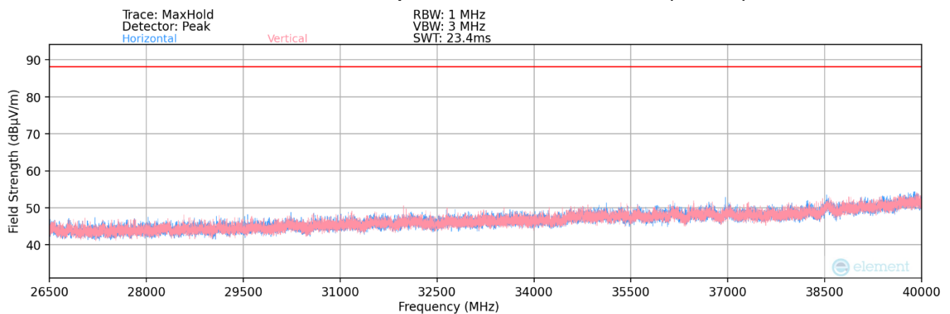
Plot 7-134. Radiated Spurious Plot 26.5GHz - 40GHz (802.11a)
