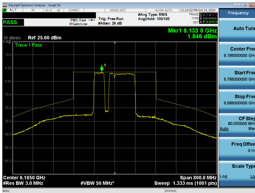
Plot 7-107. In Band Emissions Plot MIMO ANT2 (160MHz 802.11ax/be (UNII Band 5) – Ch. 47) – 20MHz Punctured - SP
