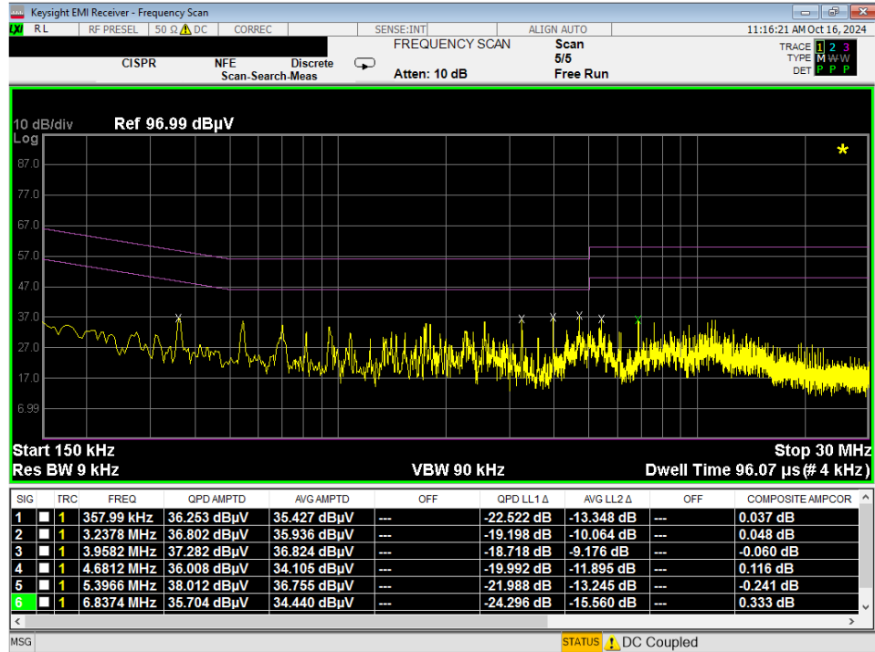
Plot 7-177. Line Conducted Plot with 802.11a UNII Band 6 (L1) with WCP
