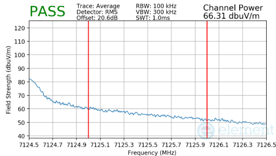
Plot 7-137. Radiated Upper Band Edge Plot MIMO (Average – UNII Band 8)
