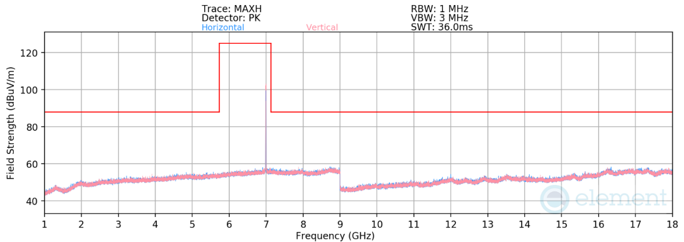
Plot 7-132. Radiated Spurious Plot 1GHz – 18GHz MIMO (802.11a – U Band 8 Ch. 209)
