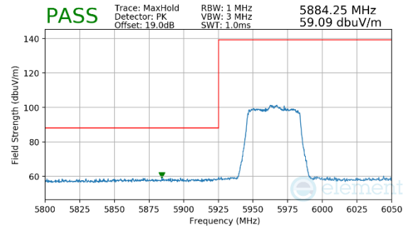
Plot 7-140. Radiated Lower Band Edge Plot MIMO (Peak – UNII Band 5)
