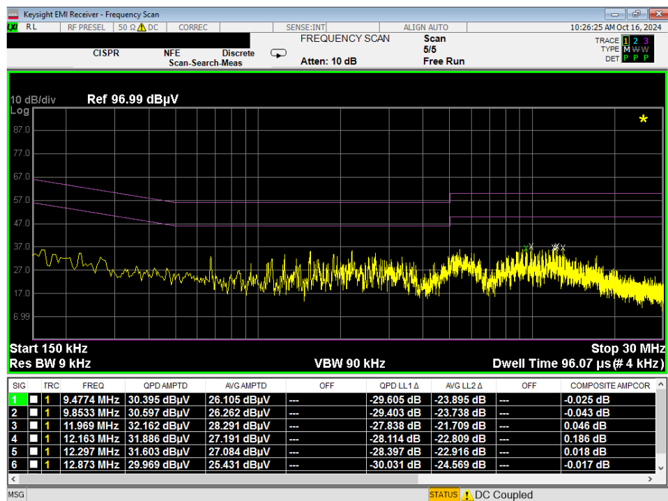
Plot 7-173. Line Conducted Plot with 802.11a UNII Band 8 (L1)
