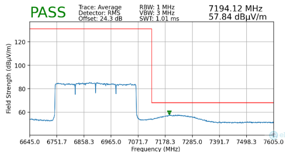
Plot 7-161. Radiated Upper Band Edge Plot MIMO (Average – UNII Band 8)
