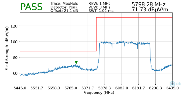
Plot 7-160. Radiated Lower Band Edge Plot MIMO (Peak – UNII Band 5)
