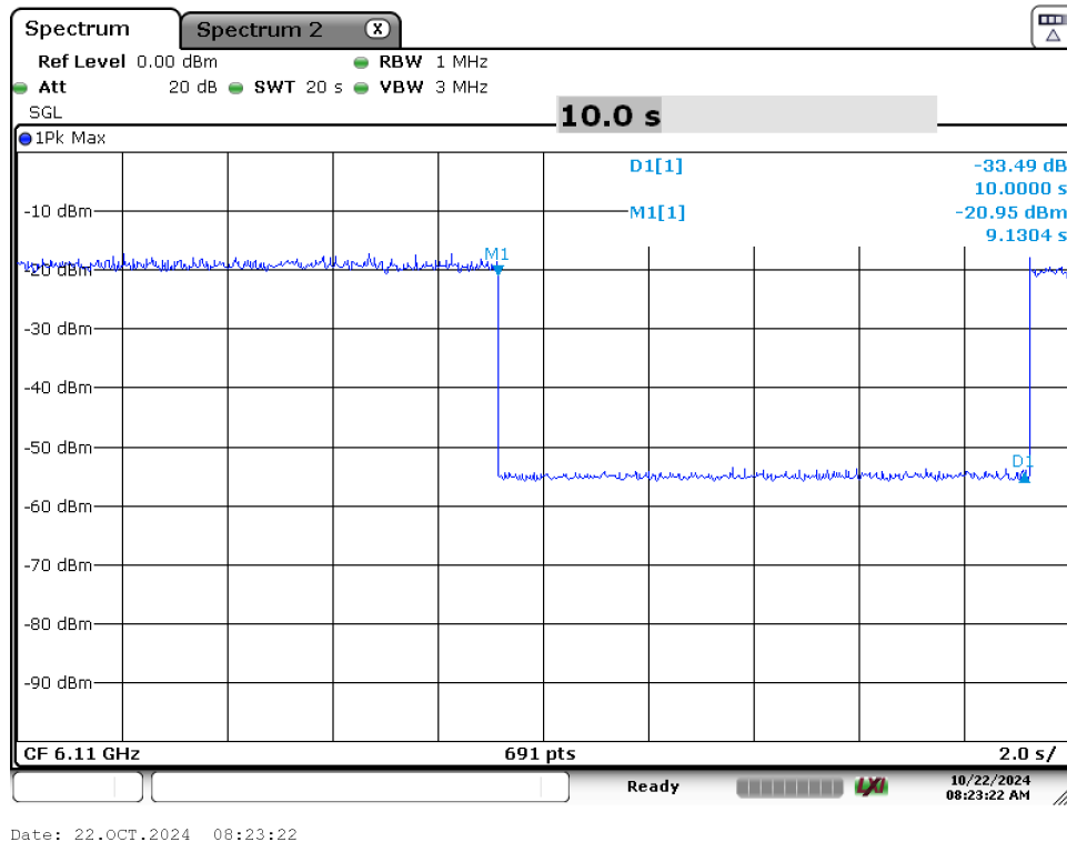
Plot 7-111. Contention Based Protocol Timing Plot (320MHz (UNII Band 5) – Ch. 31 Low)
