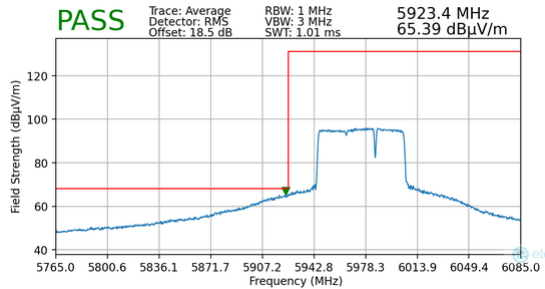
Plot 7-147. Radiated Lower Band Edge Plot MIMO (Average – UNII Band 5)
