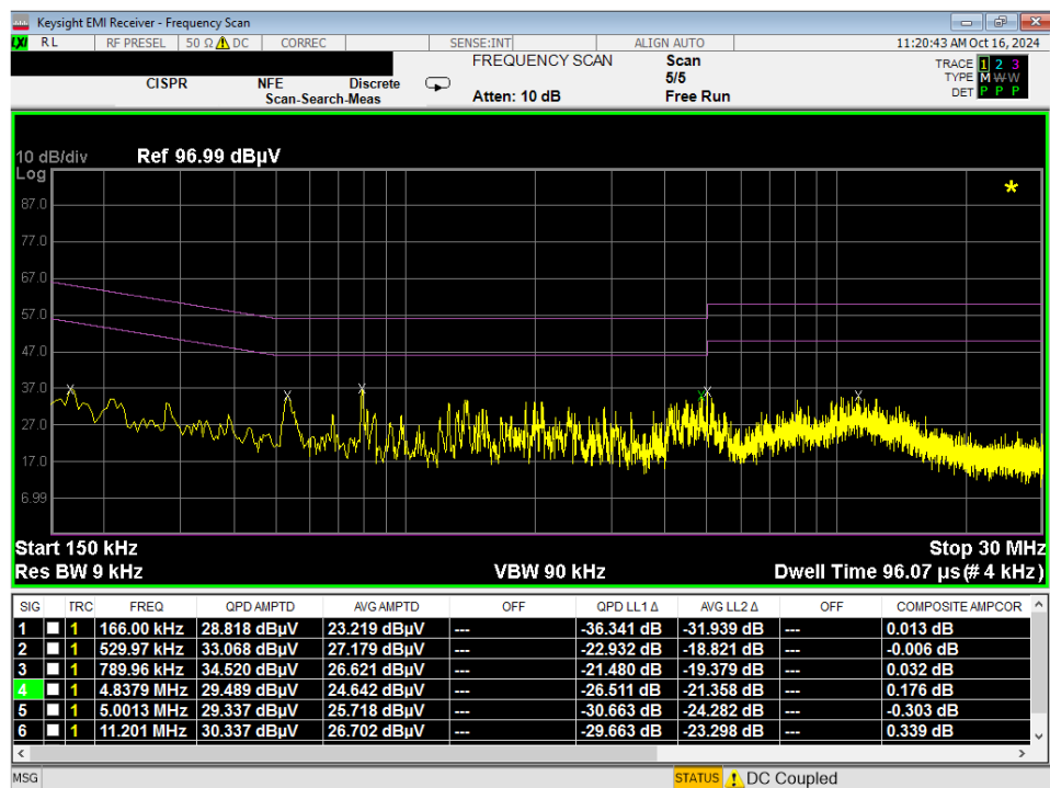
Plot 7-181. Line Conducted Plot with 802.11a UNII Band 8 (L1) with WCP
