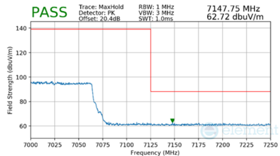
Plot 7-154. Radiated Upper Band Edge Plot MIMO (Peak – UNII Band 8)
