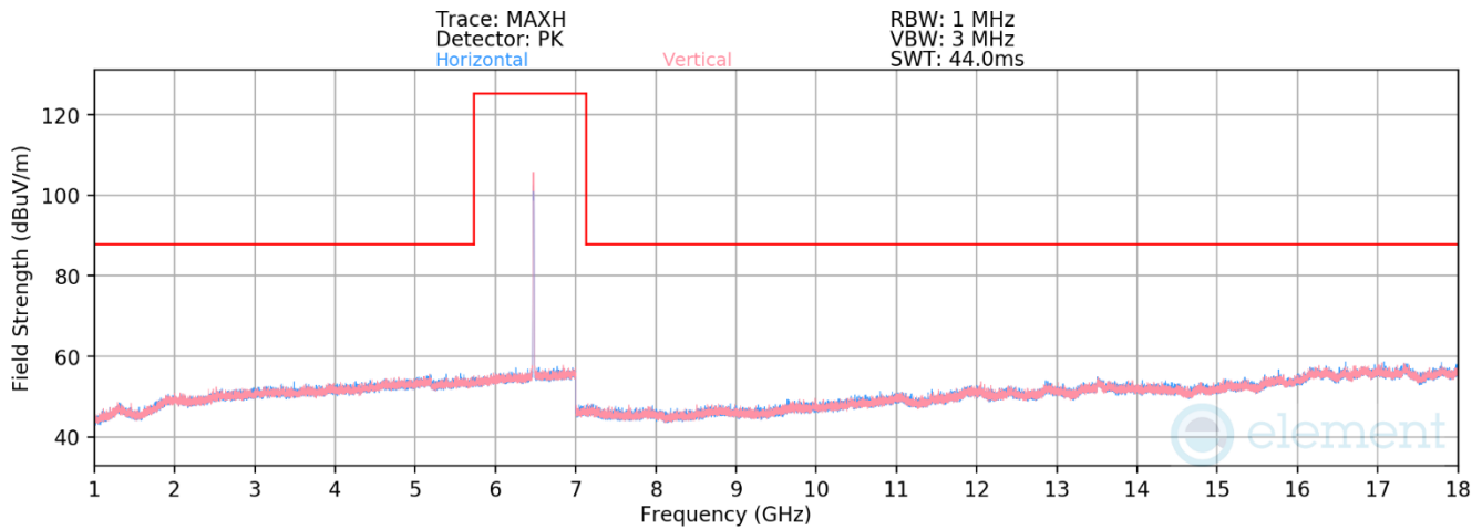
Plot 7-130. Radiated Spurious Plot 1GHz – 18GHz MIMO (802.11a – UNII Band 6 Ch. 105)
