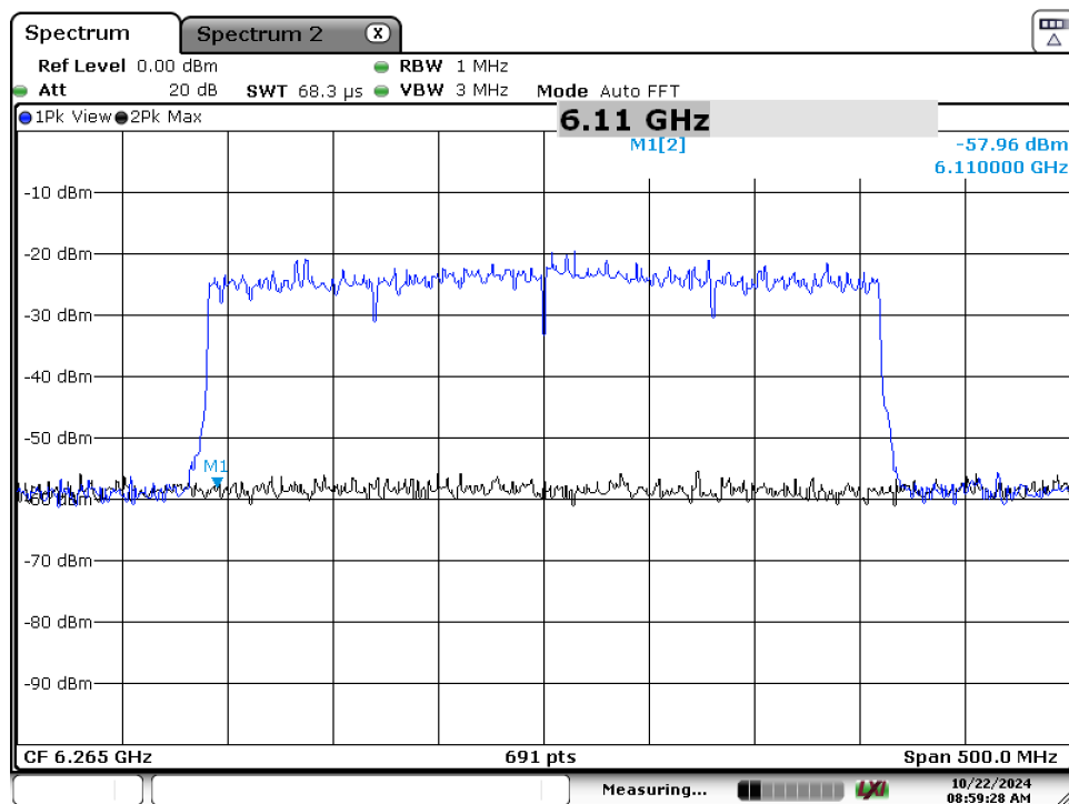
Plot 7-126. CBP 320MHz Channel - Injection Lower Edge – [6110 MHz]
