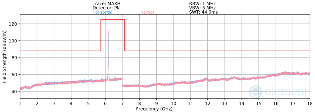
Plot 7-129. Radiated Spurious Plot 1GHz – 18GHz MIMO (802.11a – UNII Band 5 Ch. 45)
