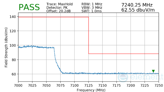
Plot 7-146. Radiated Upper Band Edge Plot MIMO (Peak – UNII Band 8)
