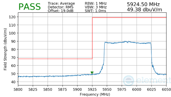
Plot 7-143. Radiated Lower Band Edge Plot MIMO (Average – UNII Band 5)
