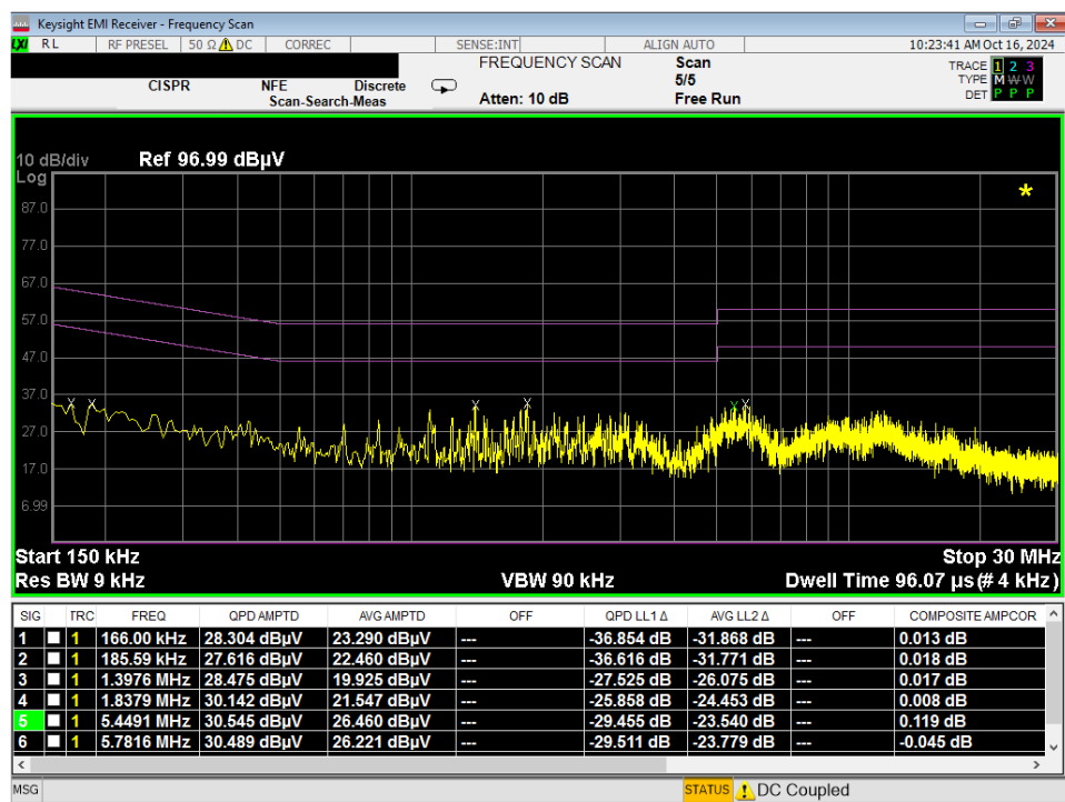
Plot 7-172. Line Conducted Plot with 802.11a UNII Band 7 (N)
