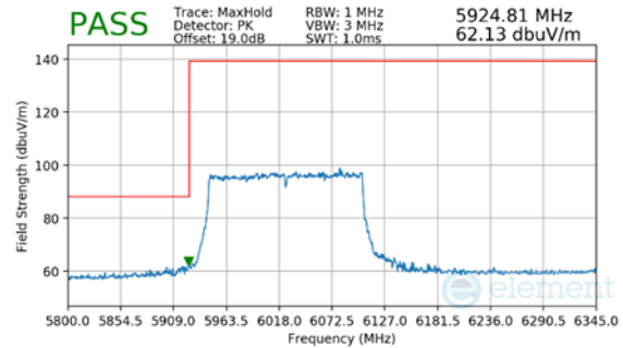
Plot 7-152. Radiated Lower Band Edge Plot MIMO (Peak – UNII Band 5)
