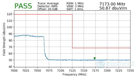
Plot 7-145. Radiated Upper Band Edge Plot MIMO (Average – UNII Band 8)
