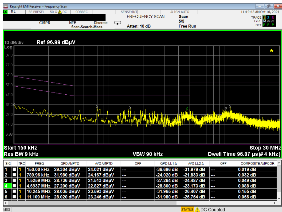
Plot 7-182. Line Conducted Plot with 802.11a UNII Band 8 (N) with WCP
