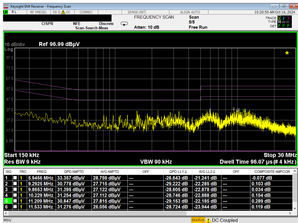
Plot 7-169. Line Conducted Plot with 802.11a UNII Band 6 (L1)
