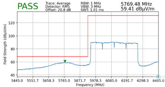
Plot 7-159. Radiated Lower Band Edge Plot MIMO (Average – UNII Band 5)
