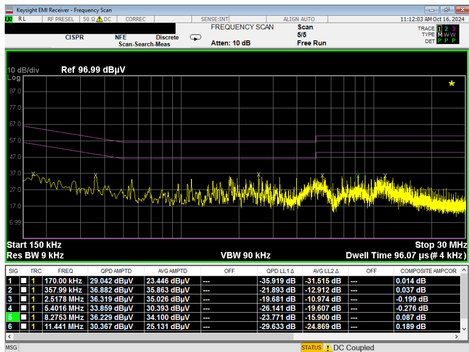
Plot 7-175. Line Conducted Plot with 802.11a UNII Band 5 (L1) with WCP
