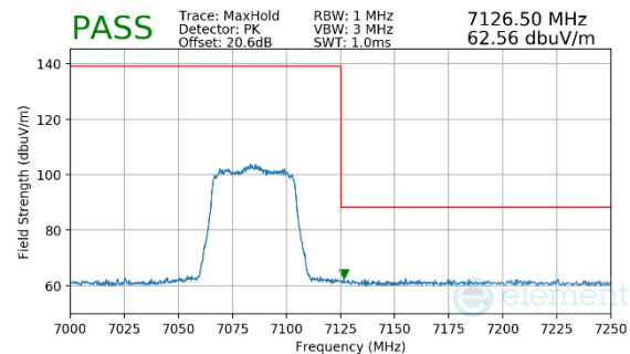
Plot 7-142. Radiated Upper Band Edge Plot MIMO (Peak – UNII Band 8)
