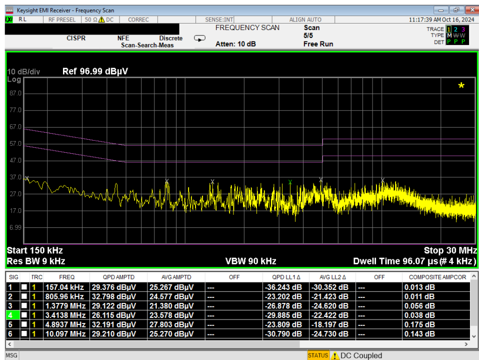
Plot 7-179. Line Conducted Plot with 802.11a UNII Band 7 (L1) with WCP
