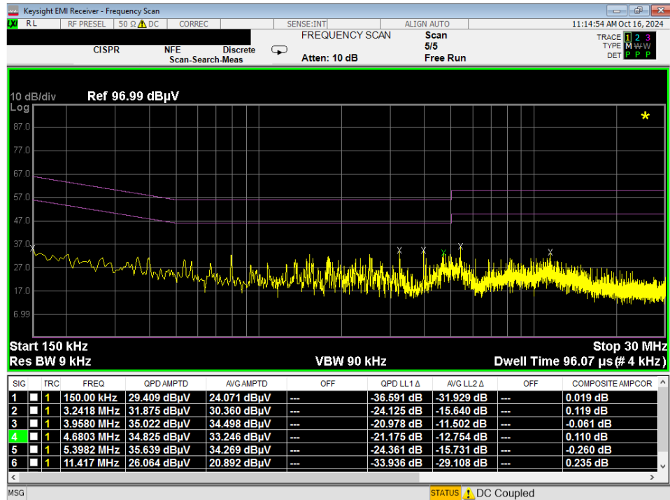
Plot 7-178. Line Conducted Plot with 802.11a UNII Band 6 (N) with WCP
