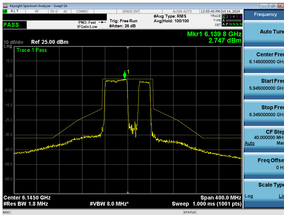
Plot 7-106. In Band Emissions Plot MIMO ANT2 (80MHz 802.11ax/be (UNII Band 5) – Ch. 39) – 20MHz Punctured - SP
