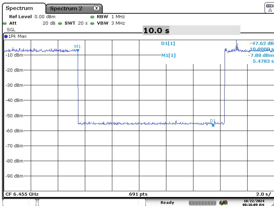
Plot 7-114. Contention Based Protocol Timing Plot (20MHz (UNII Band 6) – Ch. 101)
