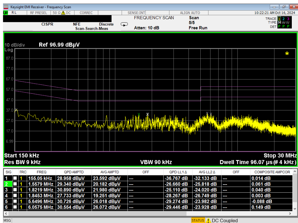
Plot 7-170. Line Conducted Plot with 802.11a UNII Band 6 (N)
