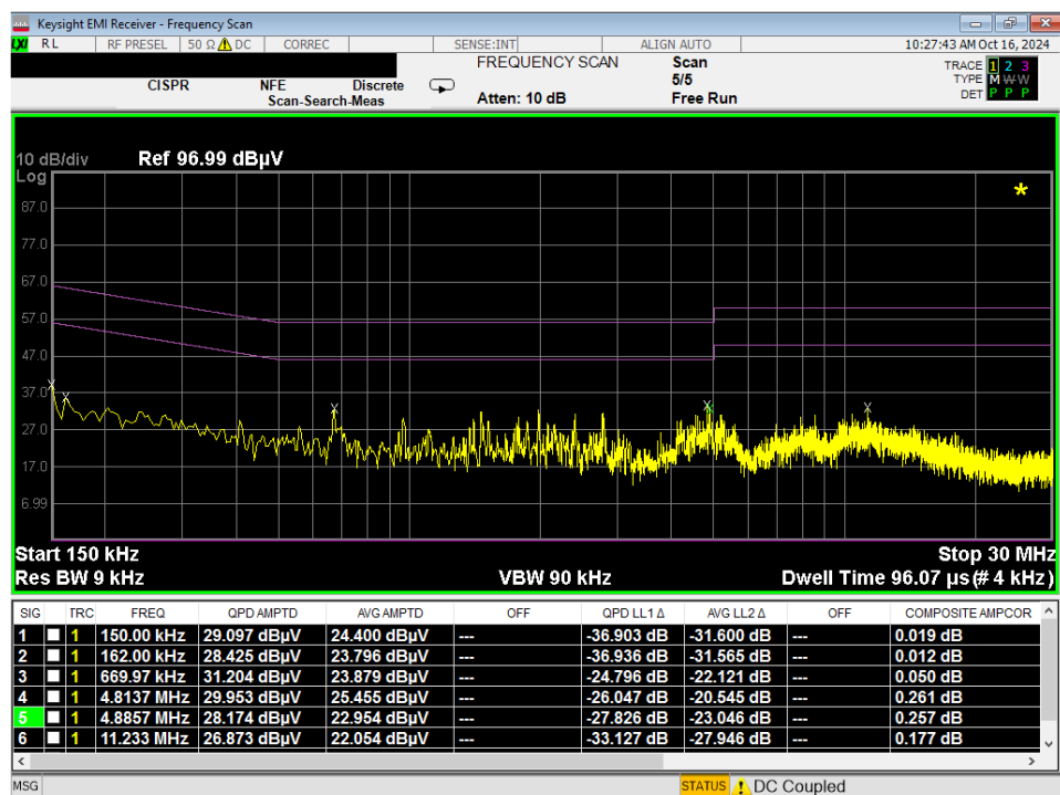
Plot 7-174. Line Conducted Plot with 802.11a UNII Band 8 (N)
