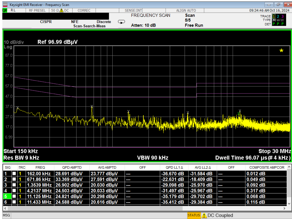
Plot 7-101. Line Conducted Plot with 802.11a UNII Band 7 (N) with WCP
