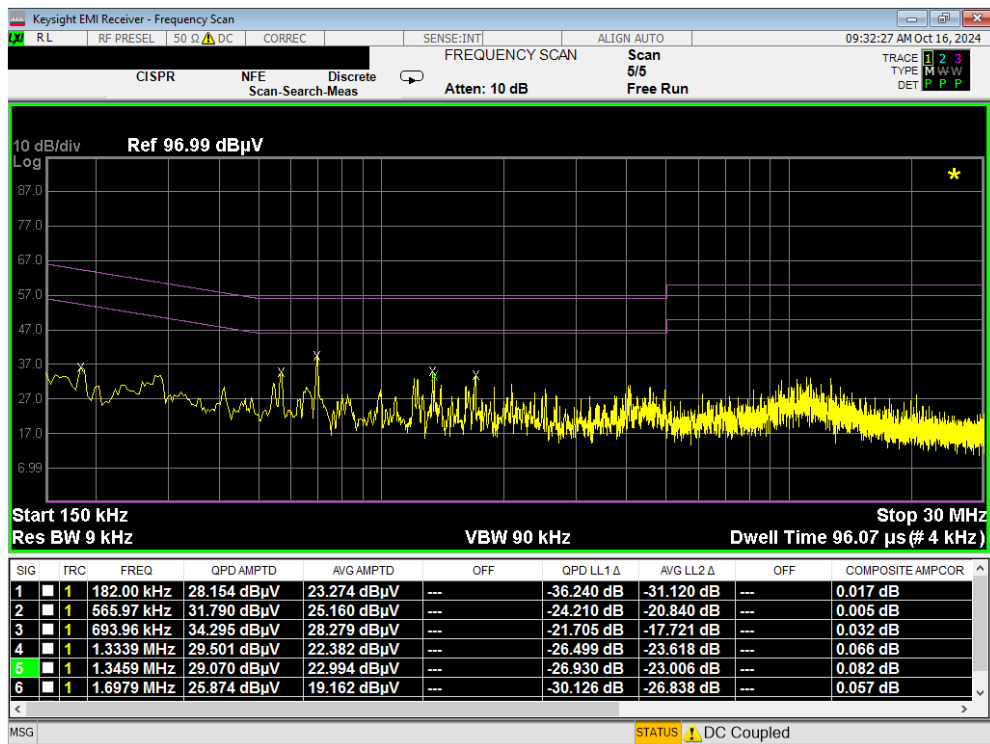
Plot 7-100. Line Conducted Plot with 802.11a UNII Band 7 (L1) with WCP
