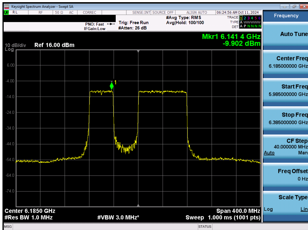
Plot 7-63. Power Spectral Density Plot MIMO ANT1 (160MHz 802.11be (996+484 Tones) (UNII Band 5) – Ch. 47) LPI
