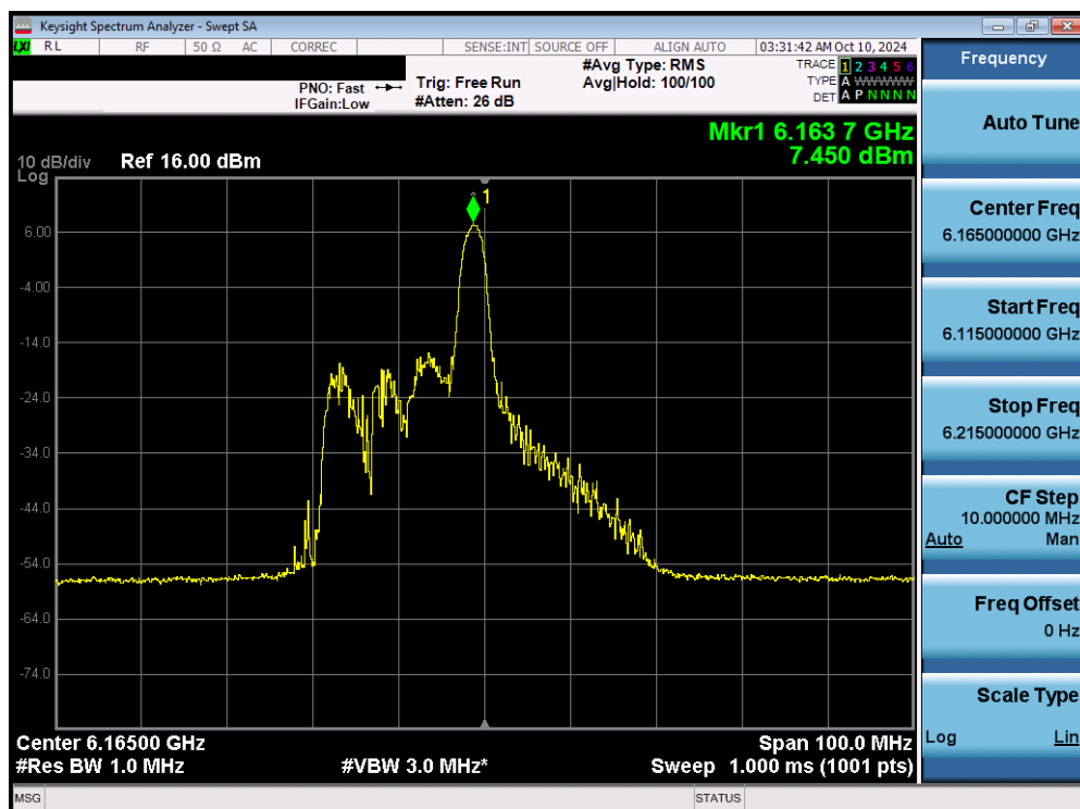
Plot 7-66. Power Spectral Density Plot MIMO ANT1 (40MHz 802.11ax/be (26 Tones) (UNII Band 5) – Ch. 43) - SP
