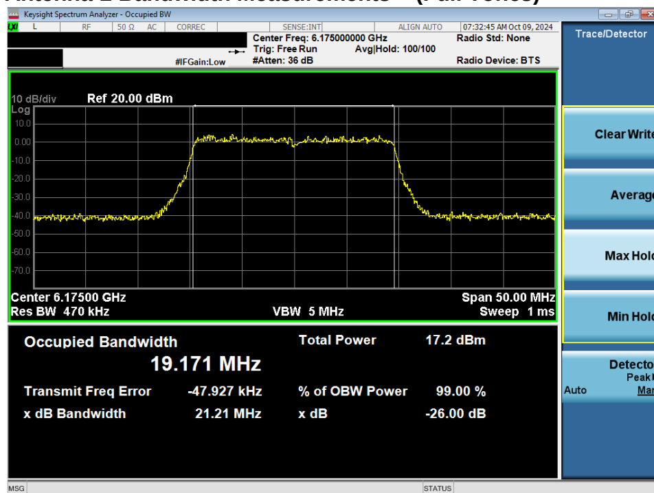
Plot 7-47. 26dB Bandwidth Plot MIMO ANT2 (20MHz 802.11ax/be (Full Tones) (UNII Band 5) – Ch. 45) - LPI
