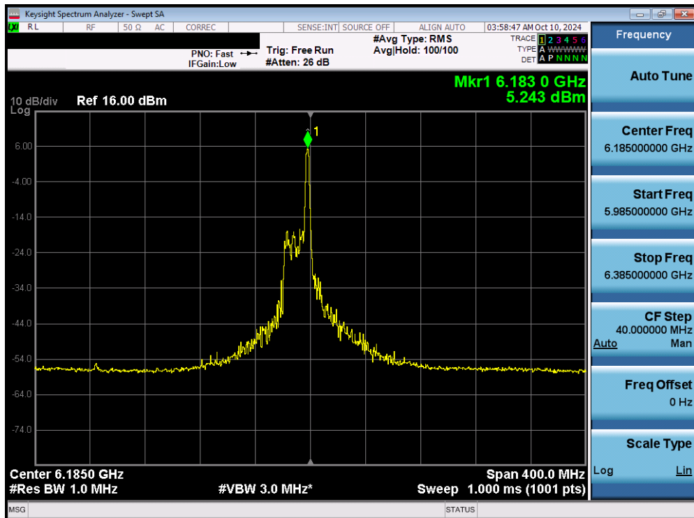
Plot 7-68. Power Spectral Density Plot MIMO ANT1 (160MHz 802.11ax/be (26 Tones) (UNII Band 5) – Ch. 47) - SP
