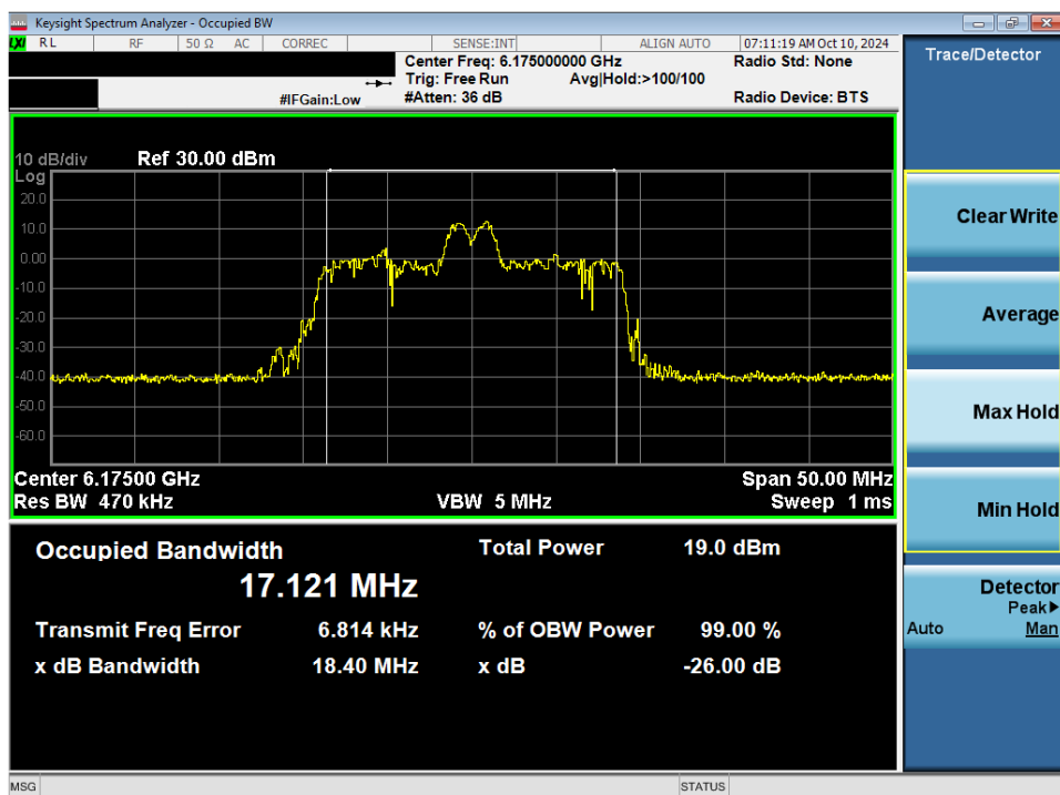
Plot 7-38. 26dB Bandwidth Plot MIMO ANT2 (20MHz 802.11ax/be (26 Tones) (UNII Band 5) – Ch. 45) - SP
