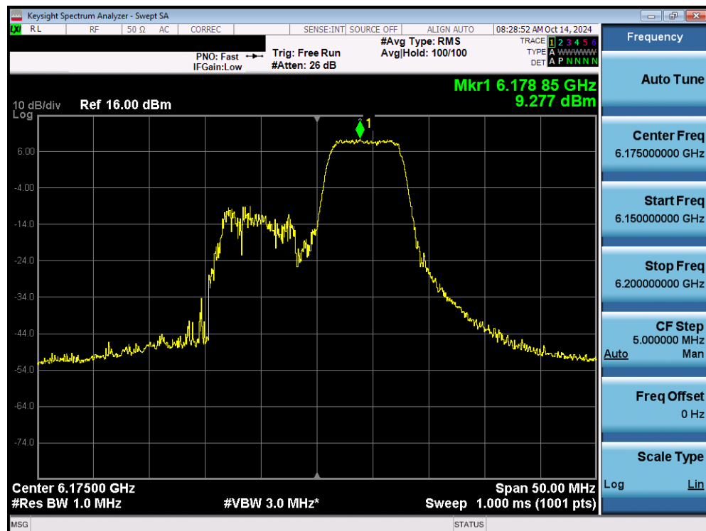
Plot 7-70. Power Spectral Density Plot MIMO ANT1 (20MHz 802.11be (52+26 Tones) (UNII Band 5) – Ch. 45) - SP
