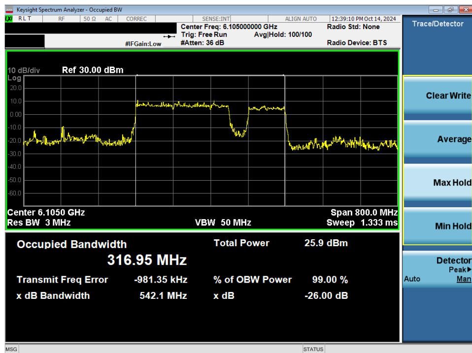
Plot 7-46. 26dB Bandwidth Plot MIMO ANT2 (320MHz 802.11be (3*996+484 Tones) (UNII Band 5) – Ch. 31) SP
