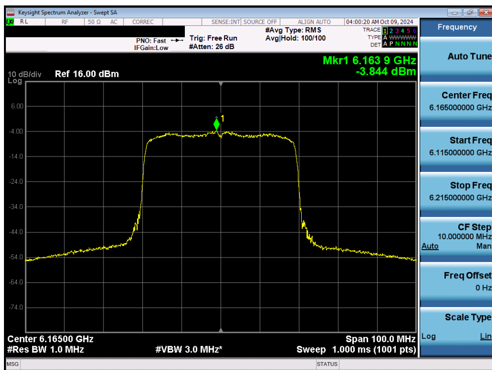
Plot 7-75. Power Spectral Density Plot MIMO ANT1 (40MHz 802.11ax/be (Full Tones) (UNII Band 5) – Ch. 43) - LPI
