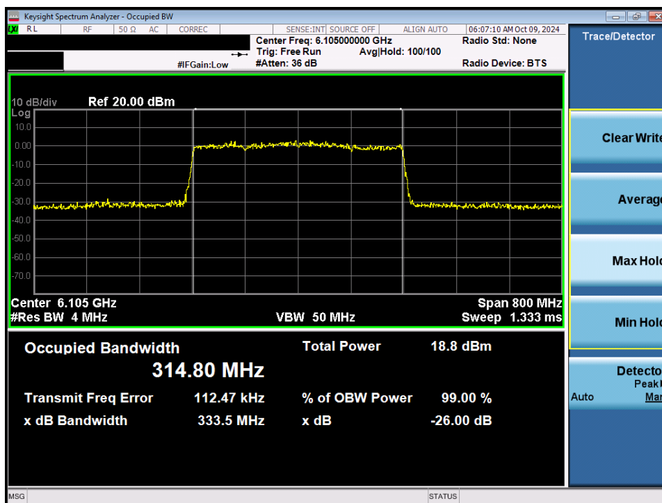
Plot 7-23. 26dB Bandwidth Plot MIMO ANT1 (320MHz 802.11be (Full Tones) (UNII Band 5) – Ch. 31) - LPI
