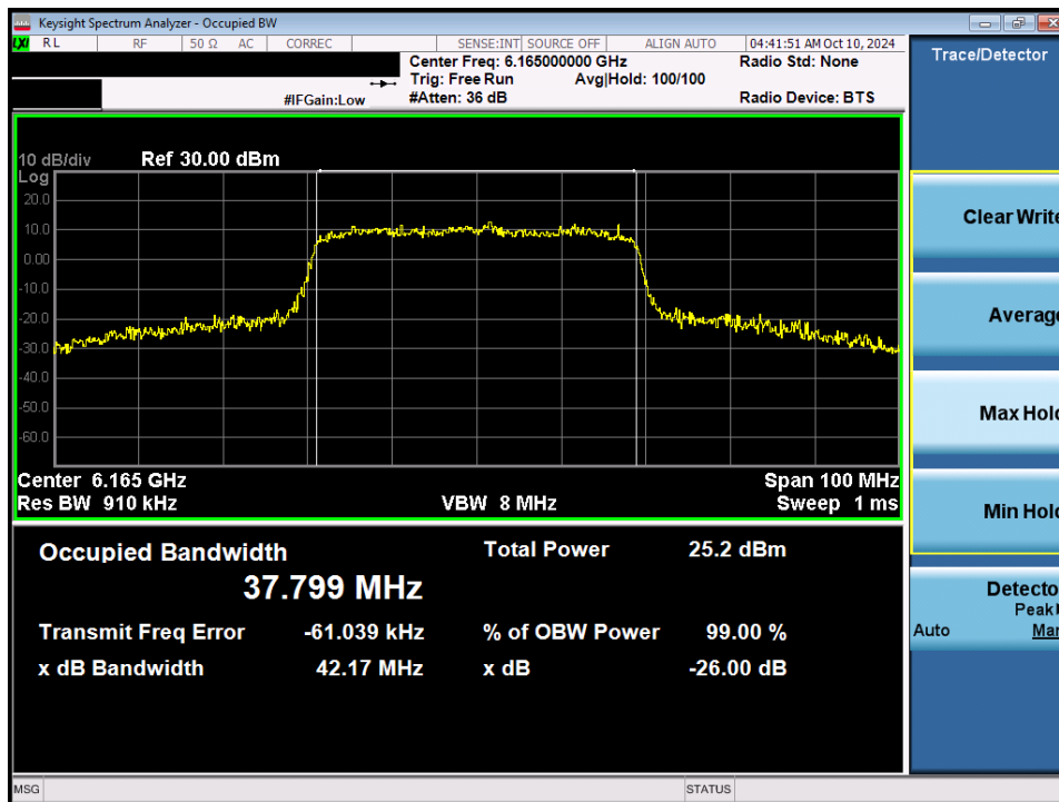
Plot 7-25. 26dB Bandwidth Plot MIMO ANT1 (40MHz 802.11ax/be (Full Tones) (UNII Band 5) – Ch. 43) - SP
