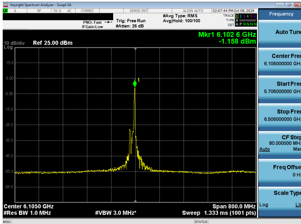
Plot 7-88. Power Spectral Density Plot MIMO ANT2 (320MHz 802.11be (26 Tones) (UNII Band 5) – Ch. 31) - LPI
