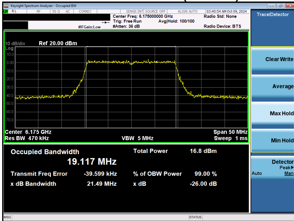
Plot 7-19. 26dB Bandwidth Plot MIMO ANT1 (20MHz 802.11ax/be (Full Tones) (UNII Band 5) – Ch. 45) - LPI
