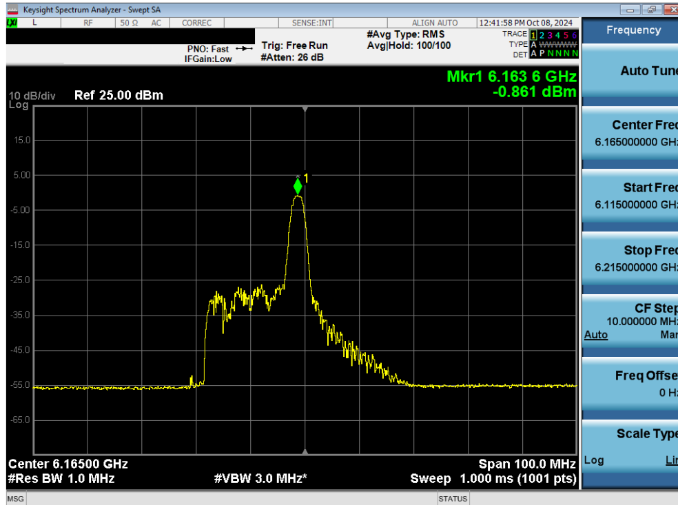
Plot 7-85. Power Spectral Density Plot MIMO ANT2 (40MHz 802.11ax/be (26 Tones) (UNII Band 5) – Ch. 43) - LPI
