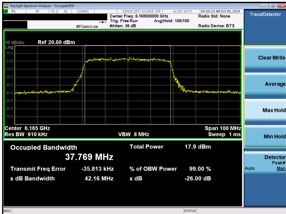
Plot 7-20. 26dB Bandwidth Plot MIMO ANT1 (40MHz 802.11ax/be (Full Tones) (UNII Band 5) – Ch. 43) - LPI
