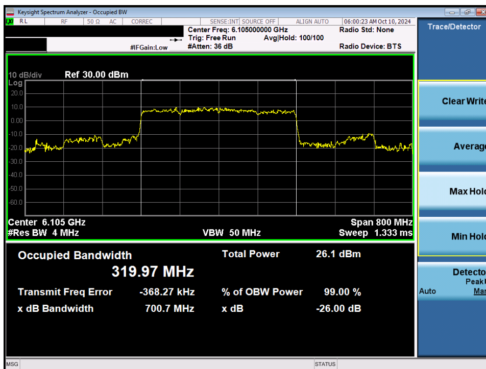
Plot 7-28. 26dB Bandwidth Plot MIMO ANT1 (320MHz 802.11be (Full Tones) (UNII Band 5) – Ch. 31) - SP
