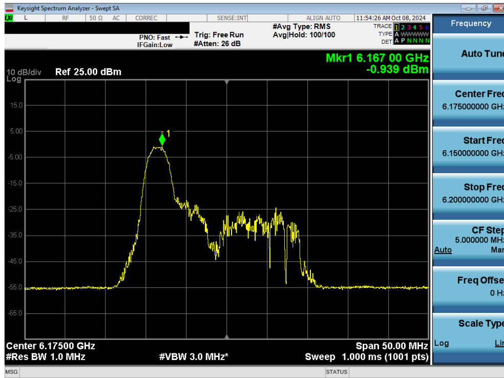
Plot 7-84. Power Spectral Density Plot MIMO ANT2 (20MHz 802.11ax/be (26 Tones) (UNII Band 5) – Ch. 45) - LPI
