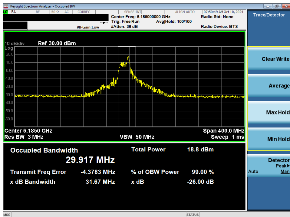
Plot 7-41. 26dB Bandwidth Plot MIMO ANT2 (160MHz 802.11ax/be (26 Tones) (UNII Band 5) – Ch. 47) - SP
