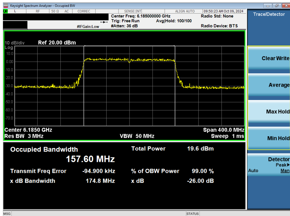
Plot 7-50. 26dB Bandwidth Plot MIMO ANT2 (160MHz 802.11ax/be (Full Tones) (UNII Band 5) – Ch. 47) - LPI
