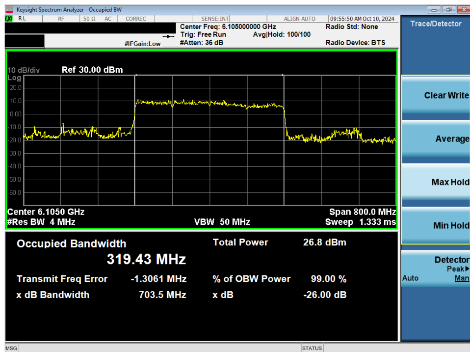
Plot 7-56. 26dB Bandwidth Plot MIMO ANT2 (320MHz 802.11be (Full Tones) (UNII Band 5) – Ch. 31) - SP
