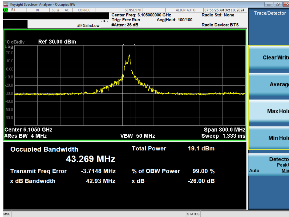
Plot 7-42. 26dB Bandwidth Plot MIMO ANT2 (320MHz 802.11be (26 Tones) (UNII Band 5) – Ch. 31) - SP
