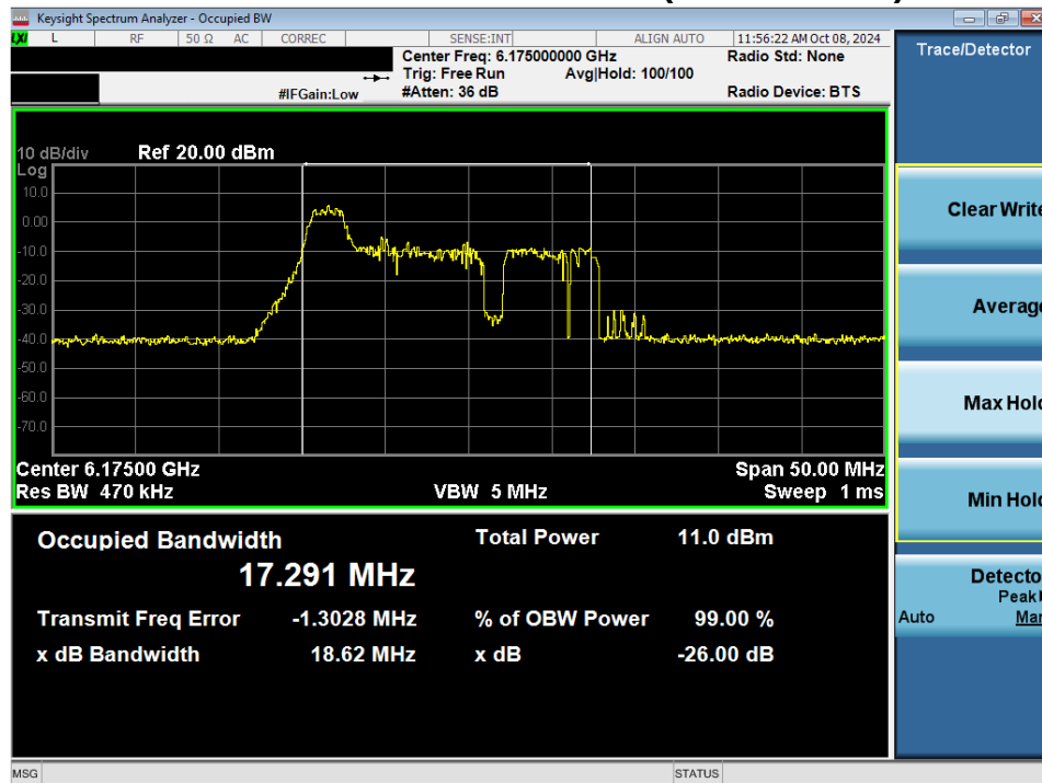
Plot 7-29. 26dB Bandwidth Plot MIMO ANT2 (20MHz 802.11ax/be (26 Tones) (UNII Band 5) – Ch. 45) - LPI
