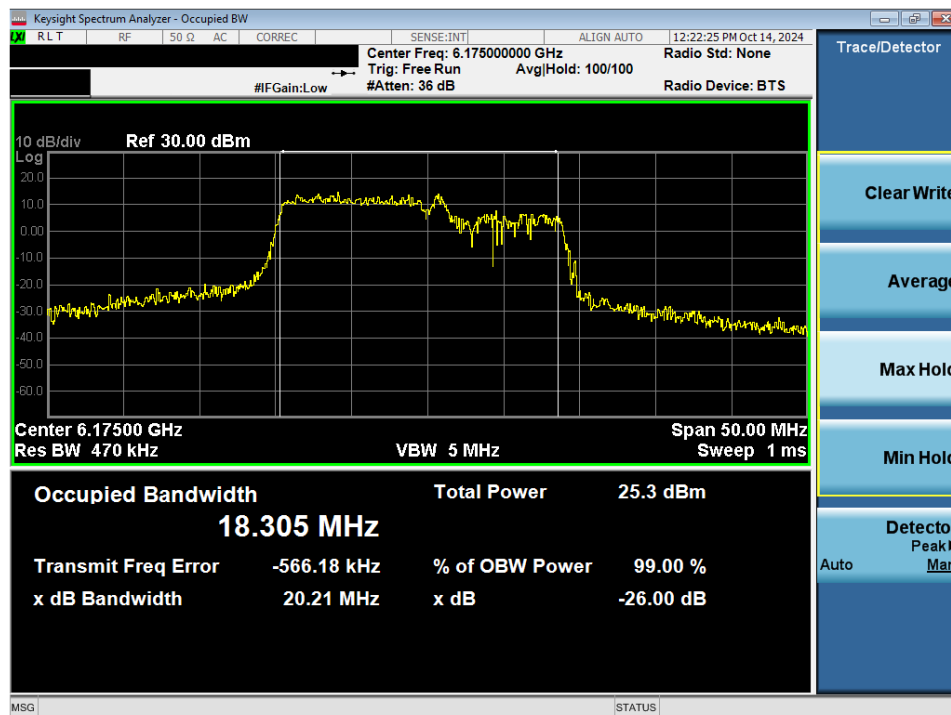
Plot 7-43. 26dB Bandwidth Plot MIMO ANT2 (20MHz 802.11be (106+26 Tones) (UNII Band 5) – Ch. 45) - SP
