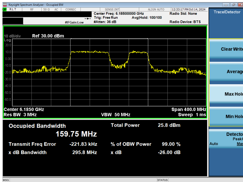
Plot 7-45. 26dB Bandwidth Plot MIMO ANT2 (160MHz 802.11be (996+484 Tones) (UNII Band 5) – Ch. 47) SP
