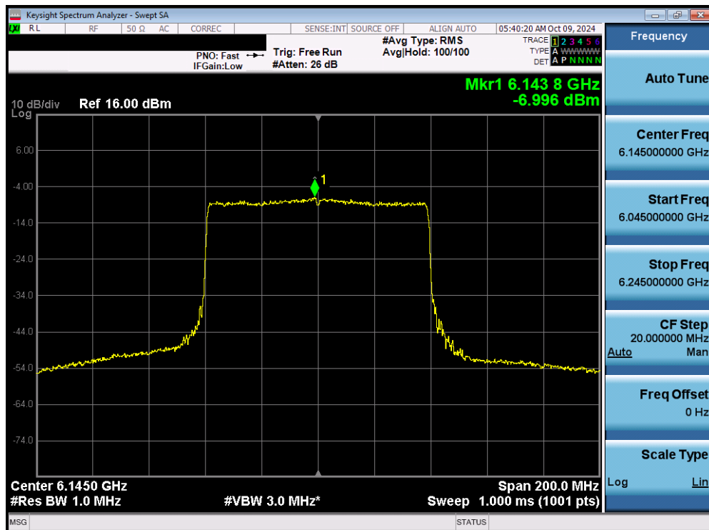
Plot 7-76. Power Spectral Density Plot MIMO ANT1 (80MHz 802.11ax/be (Full Tones) (UNII Band 5) – Ch. 39) - LPI
