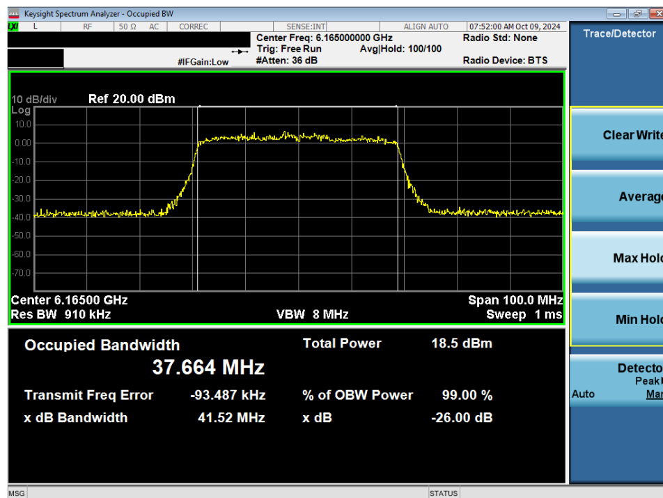
Plot 7-48. 26dB Bandwidth Plot MIMO ANT2 (40MHz 802.11ax/be (Full Tones) (UNII Band 5) – Ch. 43) - LPI
