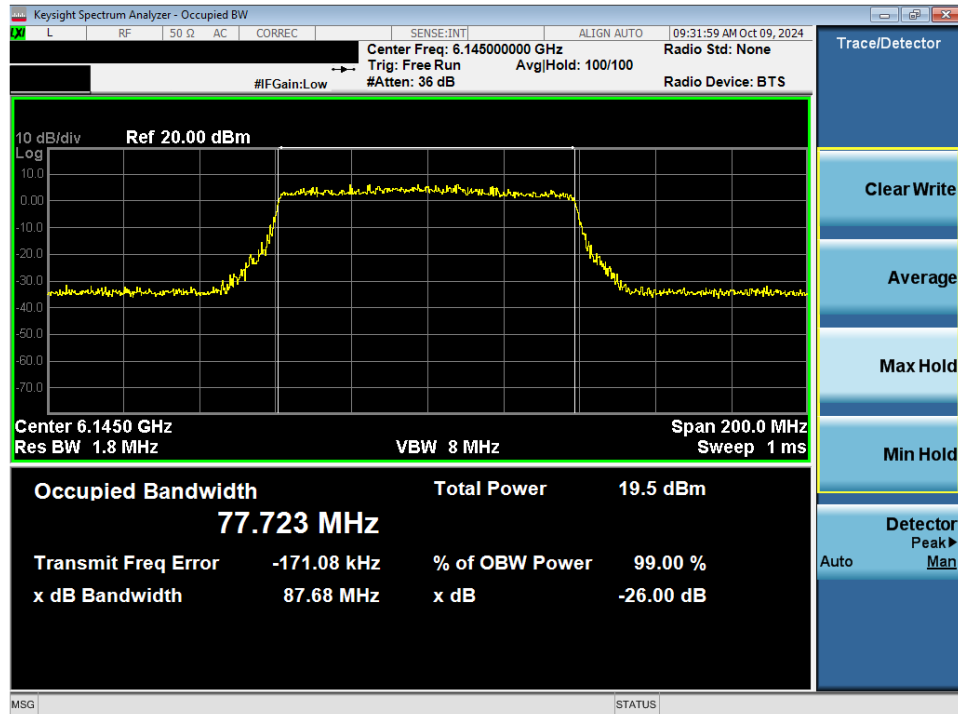
Plot 7-49. 26dB Bandwidth Plot MIMO ANT2 (80MHz 802.11ax/be (Full Tones) (UNII Band 5) – Ch. 39) - LPI
