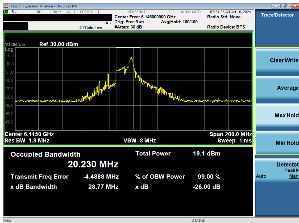
Plot 7-40. 26dB Bandwidth Plot MIMO ANT2 (80MHz 802.11ax/be (26 Tones) (UNII Band 5) – Ch. 39) - SP
