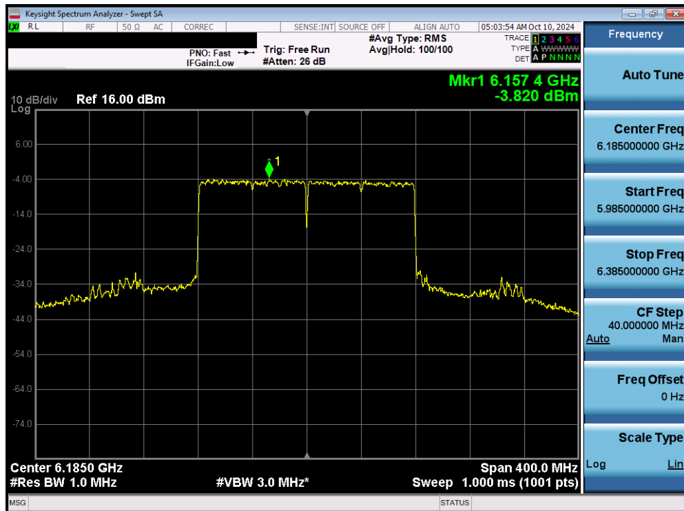
Plot 7-82. Power Spectral Density Plot MIMO ANT1 (160MHz 802.11ax/be (Full Tones) (UNII Band 5) – Ch. 47) - SP
