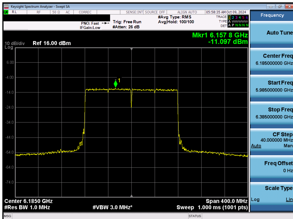
Plot 7-77. Power Spectral Density Plot MIMO ANT1 (160MHz 802.11ax/be (Full Tones) (UNII Band 5) – Ch. 47) - LPI
