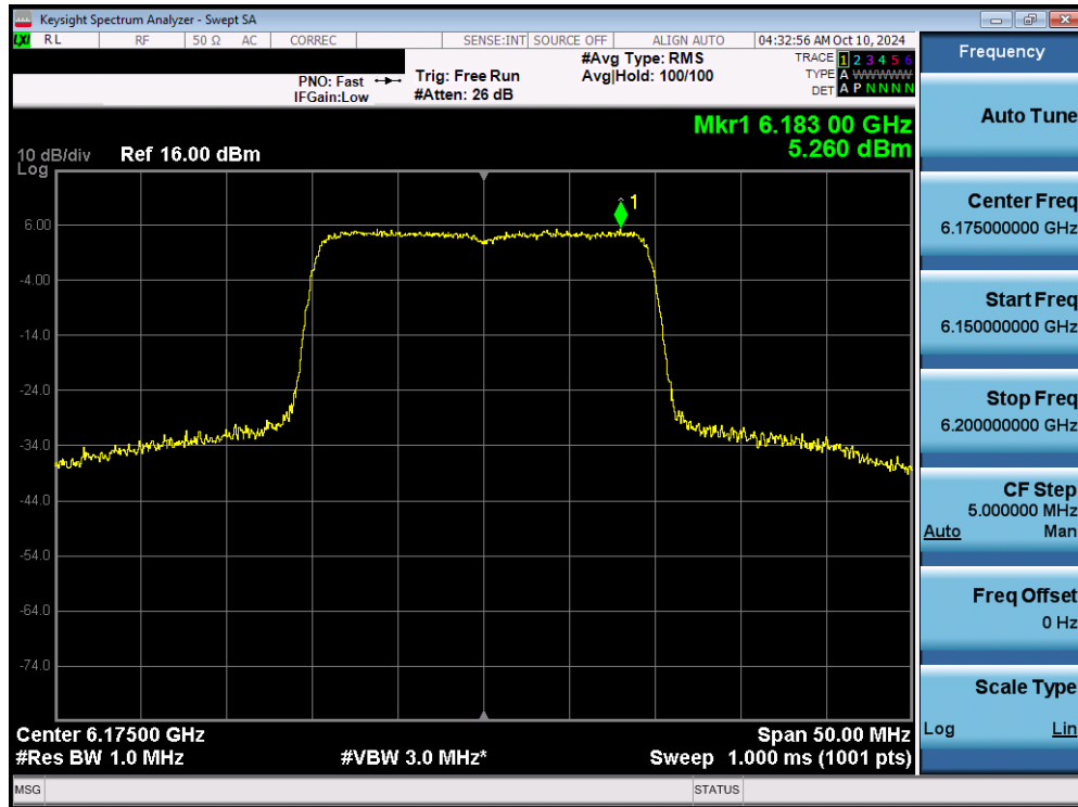
Plot 7-79. Power Spectral Density Plot MIMO ANT1 (20MHz 802.11ax/be (Full Tones) (UNII Band 5) – Ch. 45) - SP
