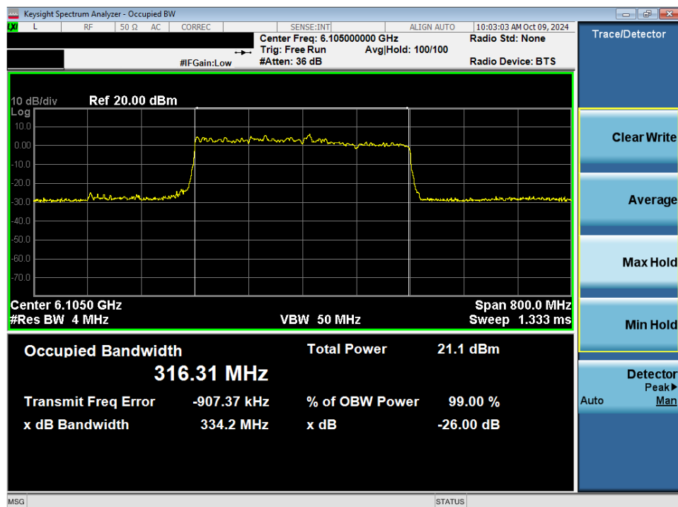
Plot 7-51. 26dB Bandwidth Plot MIMO ANT2 (320MHz 802.11be (Full Tones) (UNII Band 5) – Ch. 31) - LPI
