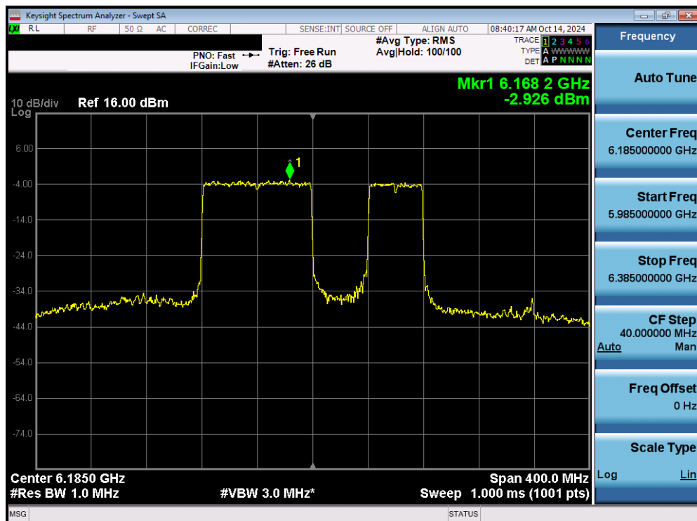
Plot 7-72. Power Spectral Density Plot MIMO ANT1 (160MHz 802.11be (996+484 Tones) (UNII Band 5) – Ch. 47) SP
