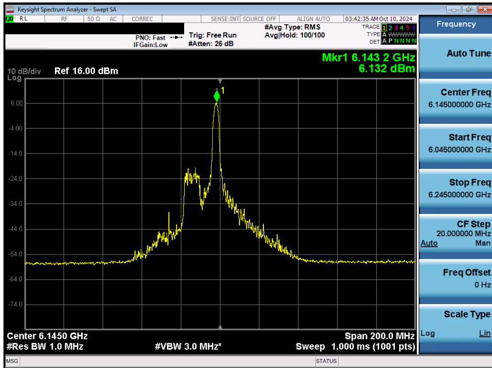
Plot 7-67. Power Spectral Density Plot MIMO ANT1 (80MHz 802.11ax/be (26 Tones) (UNII Band 5) – Ch. 39) - SP
