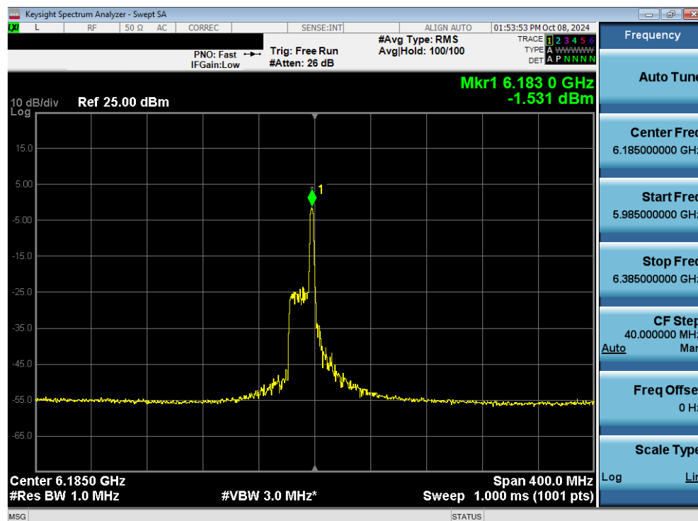
Plot 7-87. Power Spectral Density Plot MIMO ANT2 (160MHz 802.11ax/be (26 Tones) (UNII Band 5) – Ch. 47) - LPI
