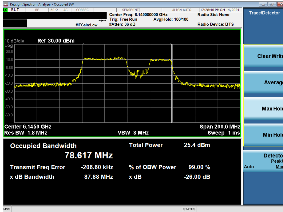
Plot 7-44. 26dB Bandwidth Plot MIMO ANT2 (80MHz 802.11be (484+242 Tones) (UNII Band 5) – Ch. 39) SP
