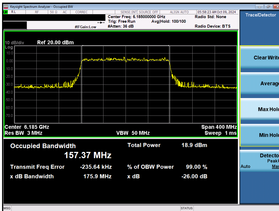
Plot 7-22. 26dB Bandwidth Plot MIMO ANT1 (160MHz 802.11ax/be (Full Tones) (UNII Band 5) – Ch. 47) - LPI
