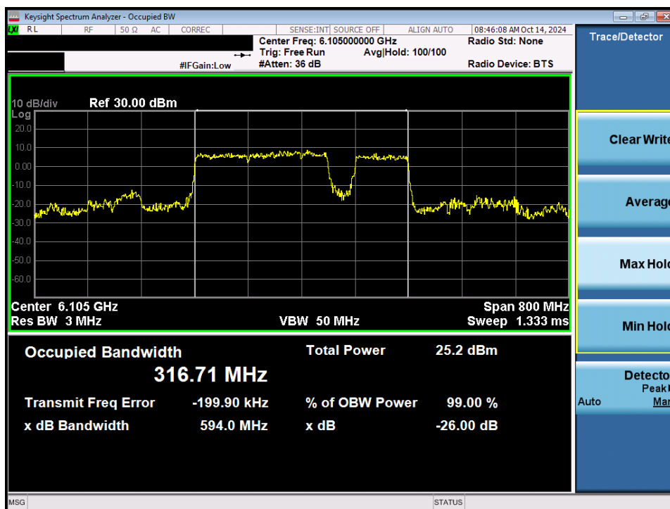
Plot 7-18. 26dB Bandwidth Plot MIMO ANT1 (320MHz 802.11be (3*996+484 Tones) (UNII Band 5) – Ch. 31) SP
