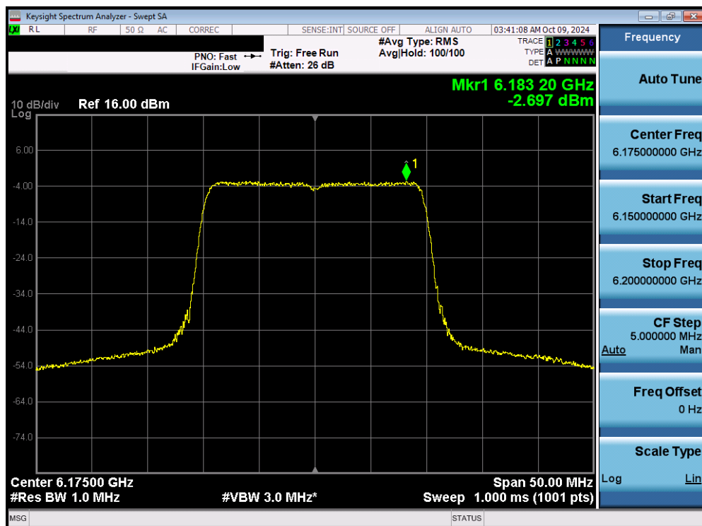
Plot 7-74. Power Spectral Density Plot MIMO ANT1 (20MHz 802.11ax/be (Full Tones) (UNII Band 5) – Ch. 45) - LPI
