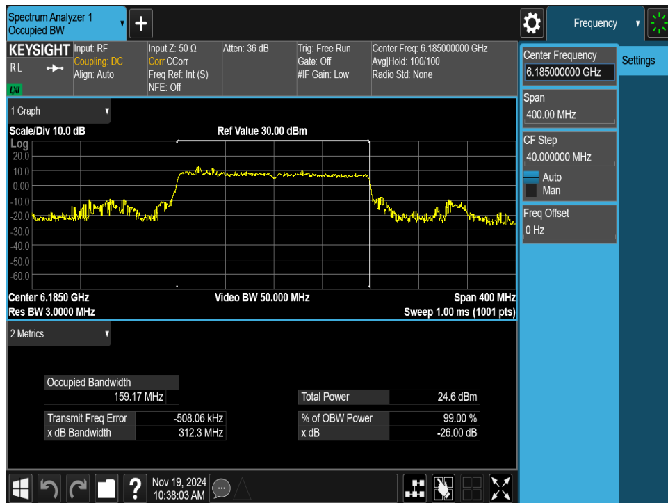
Plot 7-55. 26dB Bandwidth Plot MIMO ANT2 (160MHz 802.11ax/be (Full Tones) (UNII Band 5) – Ch. 47) - SP
