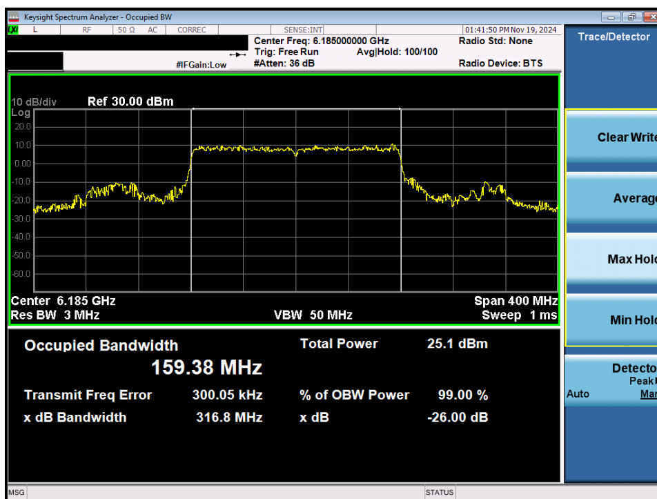
Plot 7-27. 26dB Bandwidth Plot MIMO ANT1 (160MHz 802.11ax/be (Full Tones) (UNII Band 5) – Ch. 47) - SP
