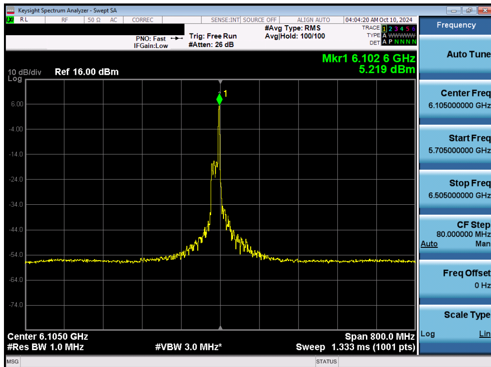
Plot 7-69. Power Spectral Density Plot MIMO ANT1 (320MHz 802.11be (26 Tones) (UNII Band 5) – Ch. 31) - SP
