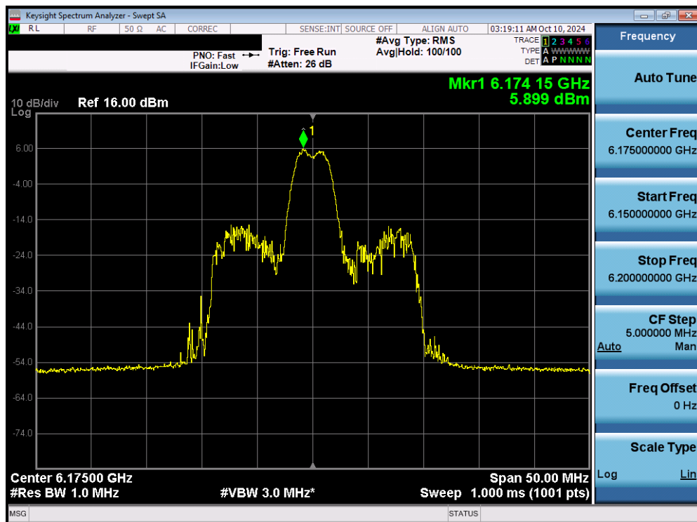
Plot 7-65. Power Spectral Density Plot MIMO ANT1 (20MHz 802.11ax/be (26 Tones) (UNII Band 5) – Ch. 45) - SP
