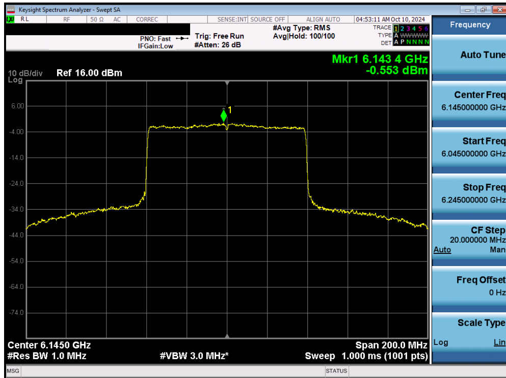
Plot 7-81. Power Spectral Density Plot MIMO ANT1 (80MHz 802.11ax/be (Full Tones) (UNII Band 5) – Ch. 39) - SP
