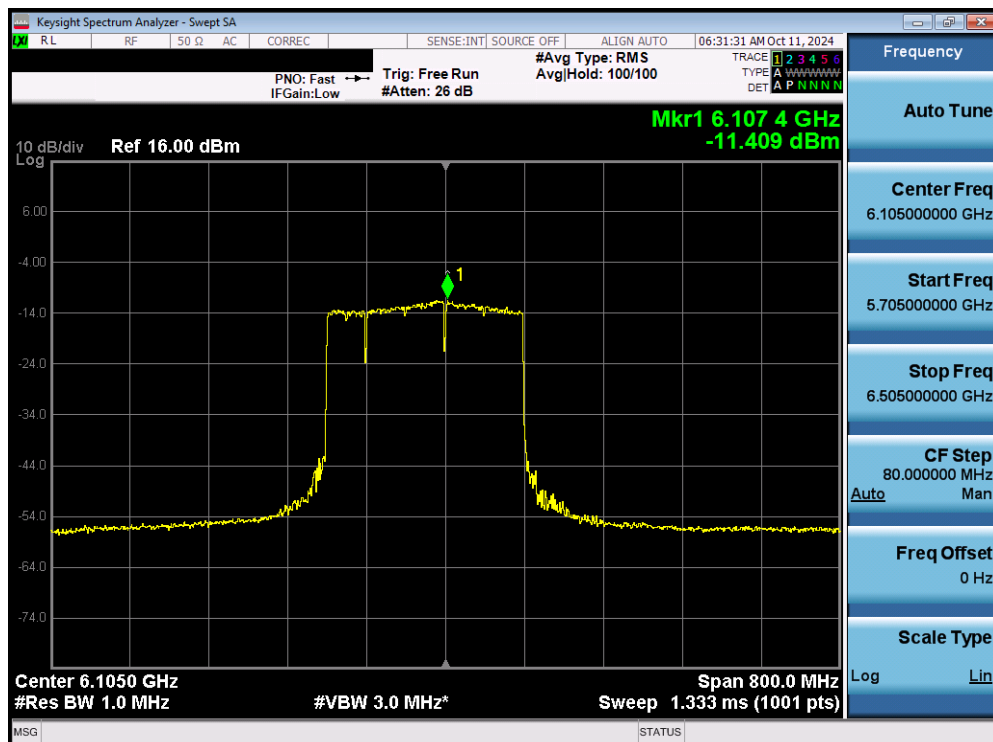
Plot 7-64. Power Spectral Density Plot MIMO ANT1 (320MHz 802.11be (UNII Band 5) – Ch. 31) LPI
