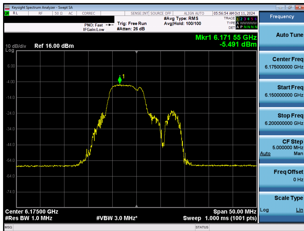
Plot 7-62. Power Spectral Density Plot MIMO ANT1 (20MHz 802.11be (52+26 Tones) (UNII Band 5) – Ch. 45) - LPI
