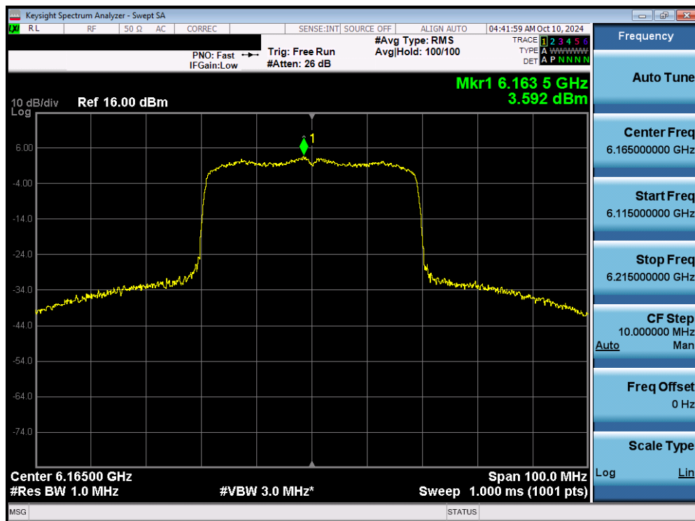
Plot 7-80. Power Spectral Density Plot MIMO ANT1 (40MHz 802.11ax/be (Full Tones) (UNII Band 5) – Ch. 43) - SP
