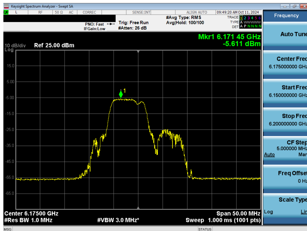
Plot 7-89. Power Spectral Density Plot MIMO ANT2 (20MHz 802.11be (52+26 Tones) (UNII Band 5) – Ch. 45) - LPI
