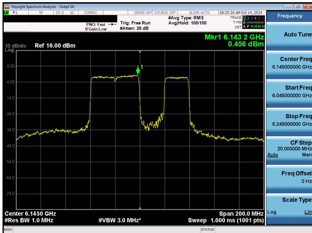
Plot 7-71. Power Spectral Density Plot MIMO ANT1 (80MHz 802.11be (484+242 Tones) (UNII Band 5) – Ch. 39) SP
