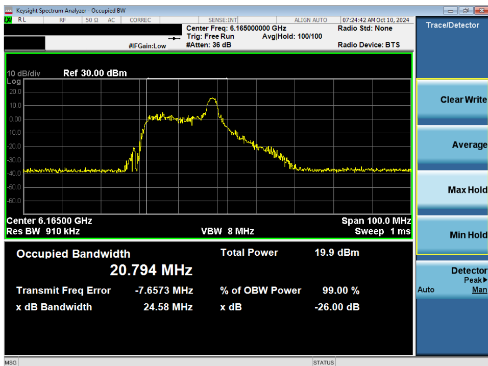
Plot 7-39. 26dB Bandwidth Plot MIMO ANT2 (40MHz 802.11ax/be (26 Tones) (UNII Band 5) – Ch. 43) - SP
