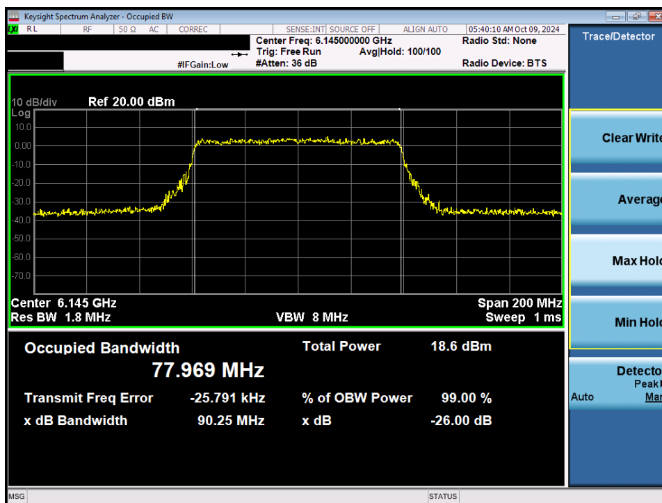
Plot 7-21. 26dB Bandwidth Plot MIMO ANT1 (80MHz 802.11ax/be (Full Tones) (UNII Band 5) – Ch. 39) - LPI
