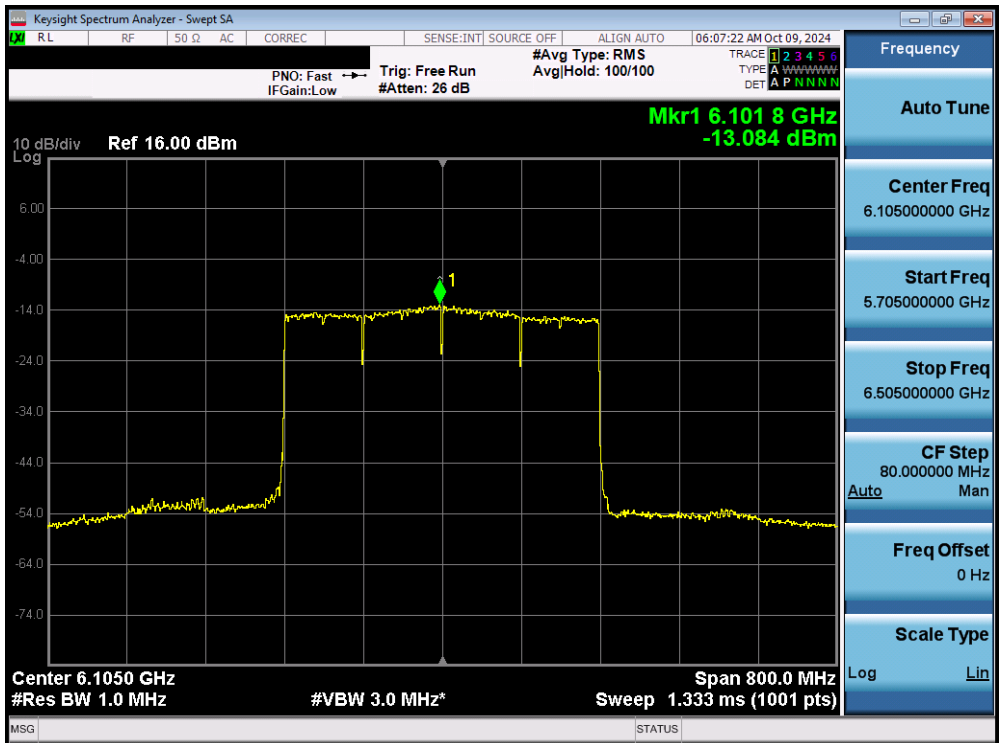
Plot 7-78. Power Spectral Density Plot MIMO ANT1 (320MHz 802.11be (Full Tones) (UNII Band 5) – Ch. 31) - LPI
