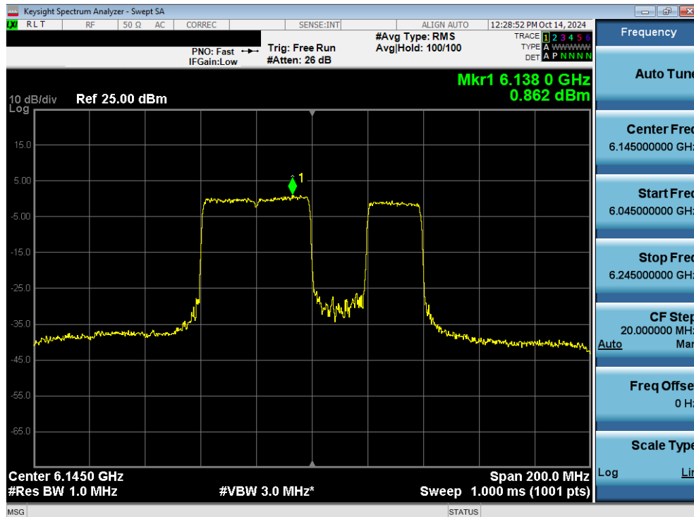
Plot 7-98. Power Spectral Density Plot MIMO ANT2 (80MHz 802.11be (484+242 Tones) (UNII Band 5) – Ch. 39) SP
