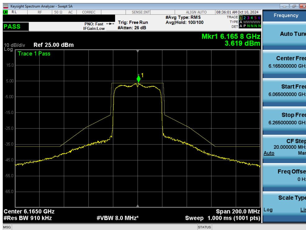
Plot 7-163. In Band Emissions Plot MIMO ANT2 (40MHz 802.11ax/be (Full Tones) (UNII Band 5) – Ch. 43) - SP
