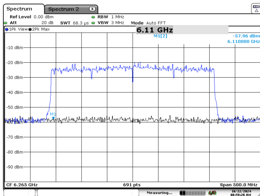
Plot 7-184. CBP 320MHz Channel - Injection Lower Edge – [6110 MHz]
