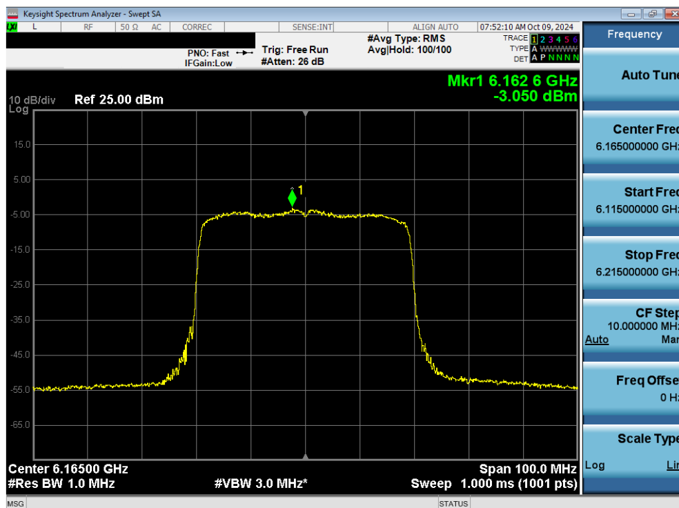
Plot 7-102. Power Spectral Density Plot MIMO ANT2 (40MHz 802.11ax/be (Full Tones) (UNII Band 5) – Ch. 43) - LPI
