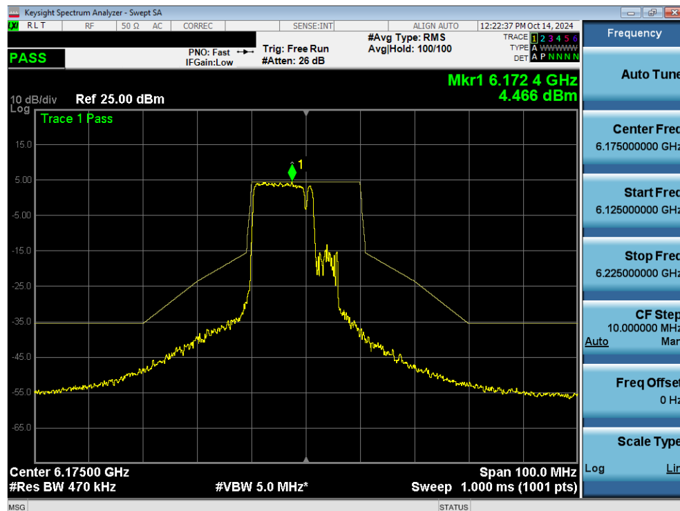
Plot 7-153. In Band Emissions Plot MIMO ANT2 (20MHz 802.11be (106+26 Tones) (UNII Band 5) – Ch. 45) - SP
