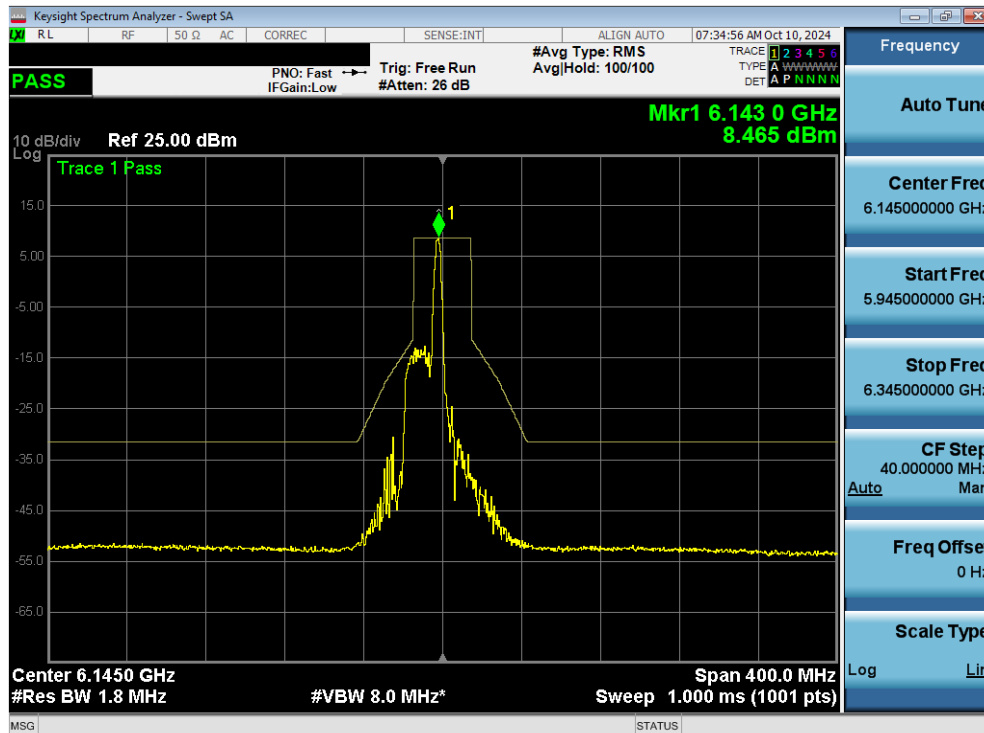
Plot 7-150. In Band Emissions Plot MIMO ANT2 (80MHz 802.11ax/be (26 Tones) (UNII Band 5) – Ch. 39) - SP
