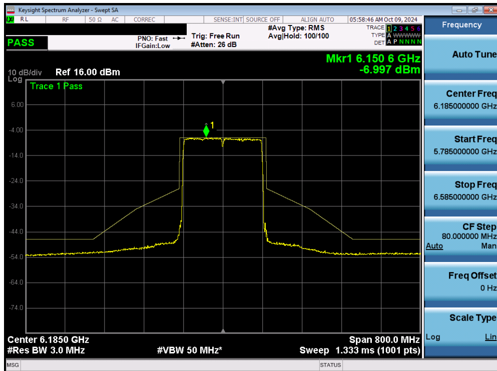
Plot 7-132. In Band Emissions Plot MIMO ANT1 (160MHz 802.11ax/be (Full Tones) (UNII Band 5) – Ch. 47) - LPI
