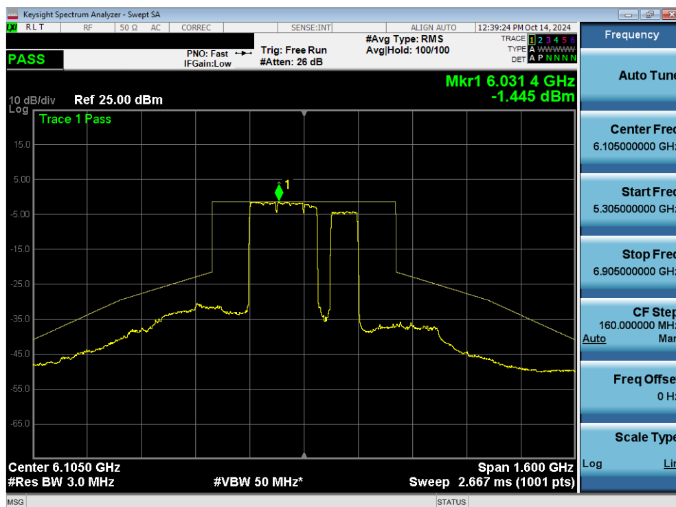
Plot 7-156. In Band Emissions Plot MIMO ANT2 (320MHz 802.11be (3*996+484 Tones) (UNII Band 5) – Ch. 31) SP
