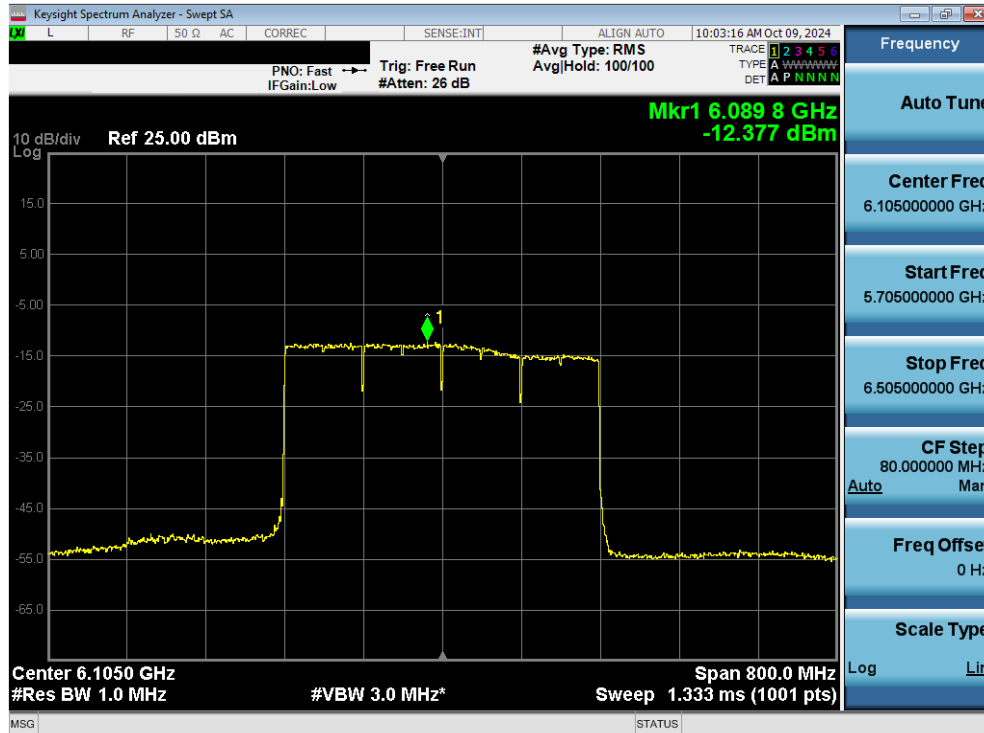
Plot 7-105. Power Spectral Density Plot MIMO ANT2 (320MHz 802.11be (Full Tones) (UNII Band 5) – Ch. 31) - LPI
