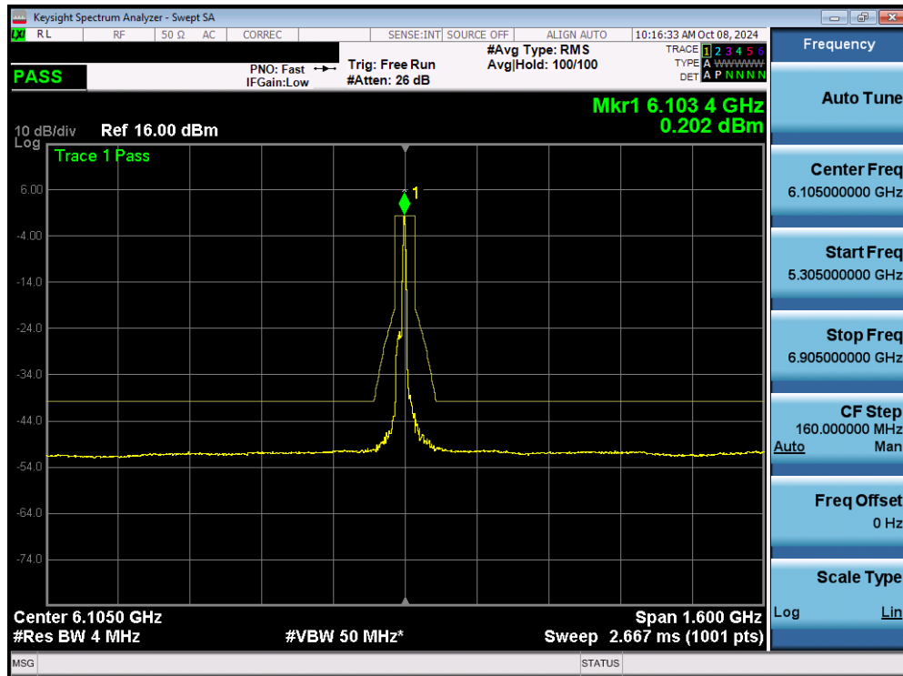
Plot 7-115. In Band Emissions Plot MIMO ANT1 (320MHz 802.11be (26 Tones) (UNII Band 5) – Ch. 31) - LPI
