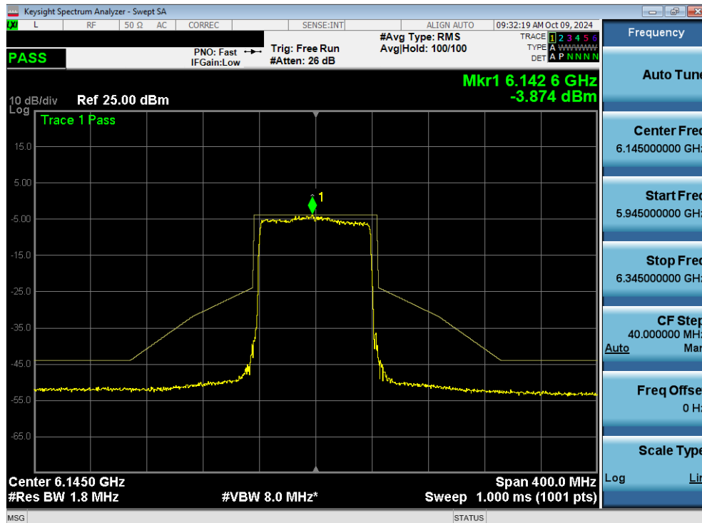
Plot 7-159. In Band Emissions Plot MIMO ANT2 (80MHz 802.11ax/be (Full Tones) (UNII Band 5) – Ch. 39) - LPI
