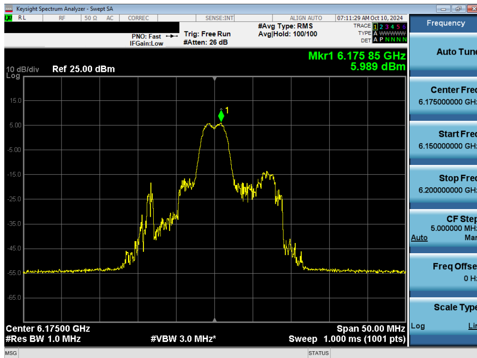
Plot 7-92. Power Spectral Density Plot MIMO ANT2 (20MHz 802.11ax/be (26 Tones) (UNII Band 5) – Ch. 45) - SP
