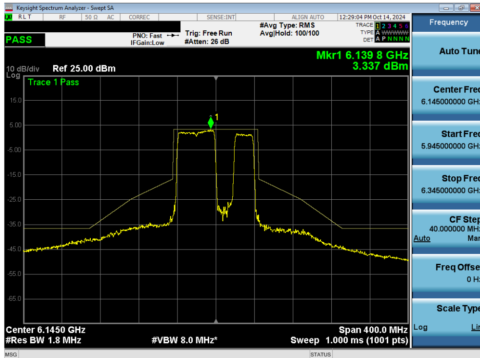
Plot 7-154. In Band Emissions Plot MIMO ANT2 (80MHz 802.11be (484+242 Tones) (UNII Band 5) – Ch. 39) SP
