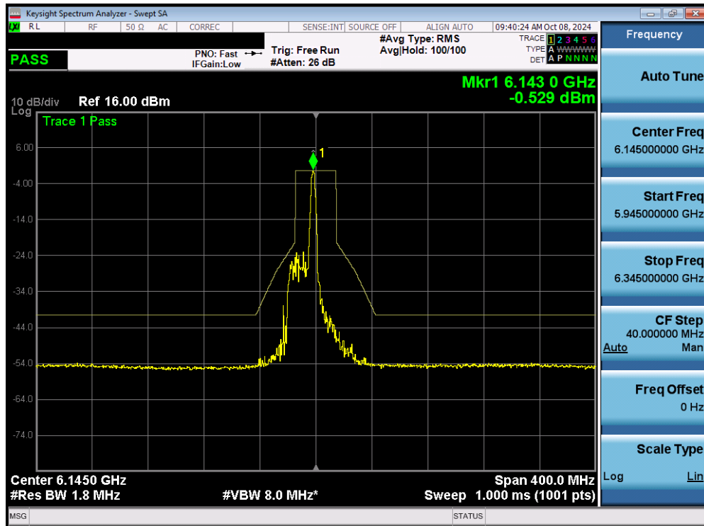
Plot 7-113. In Band Emissions Plot MIMO ANT1 (80MHz 802.11ax/be (26 Tones) (UNII Band 5) – Ch. 39) - LPI
