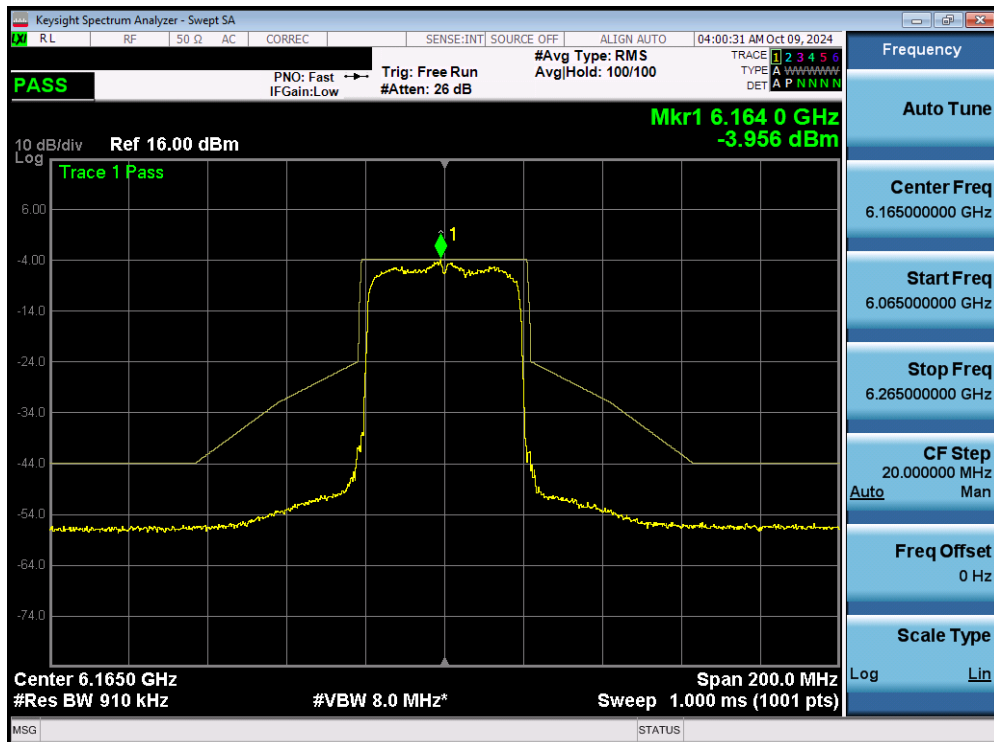
Plot 7-130. In Band Emissions Plot MIMO ANT1 (40MHz 802.11ax/be (Full Tones) (UNII Band 5) – Ch. 43) - LPI
