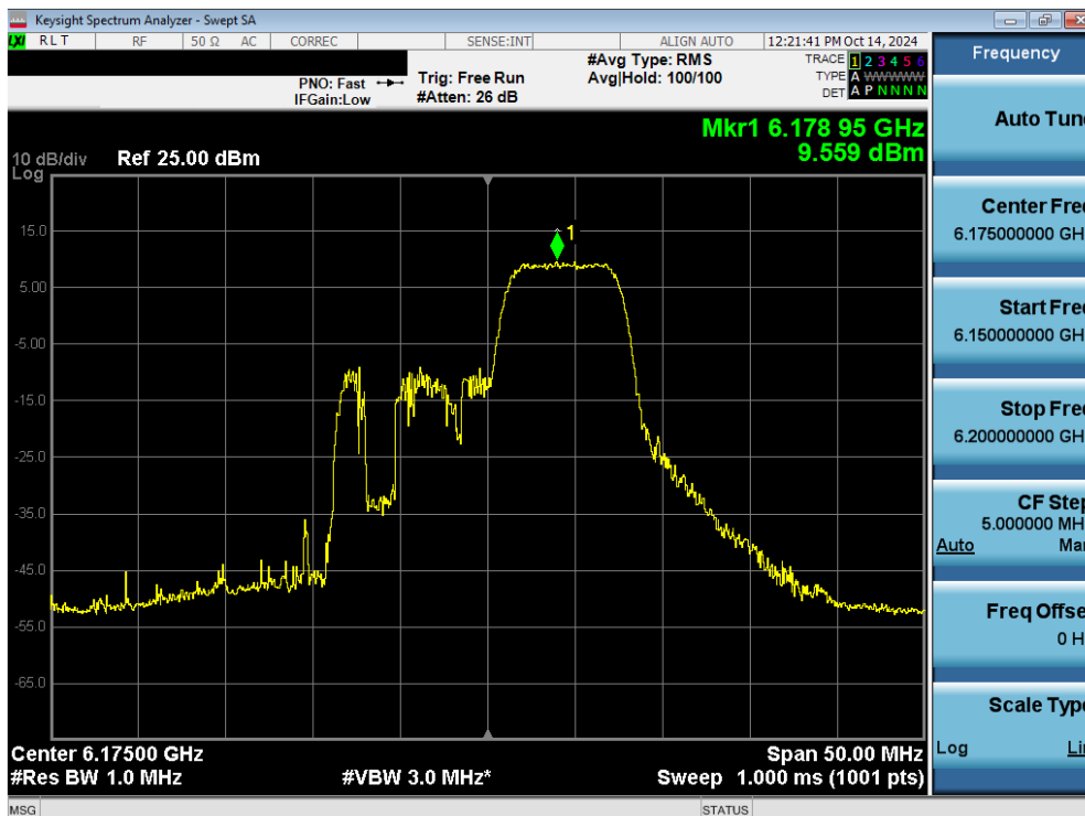
Plot 7-97. Power Spectral Density Plot MIMO ANT2 (20MHz 802.11be (52+26 Tones) (UNII Band 5) – Ch. 45) - SP
