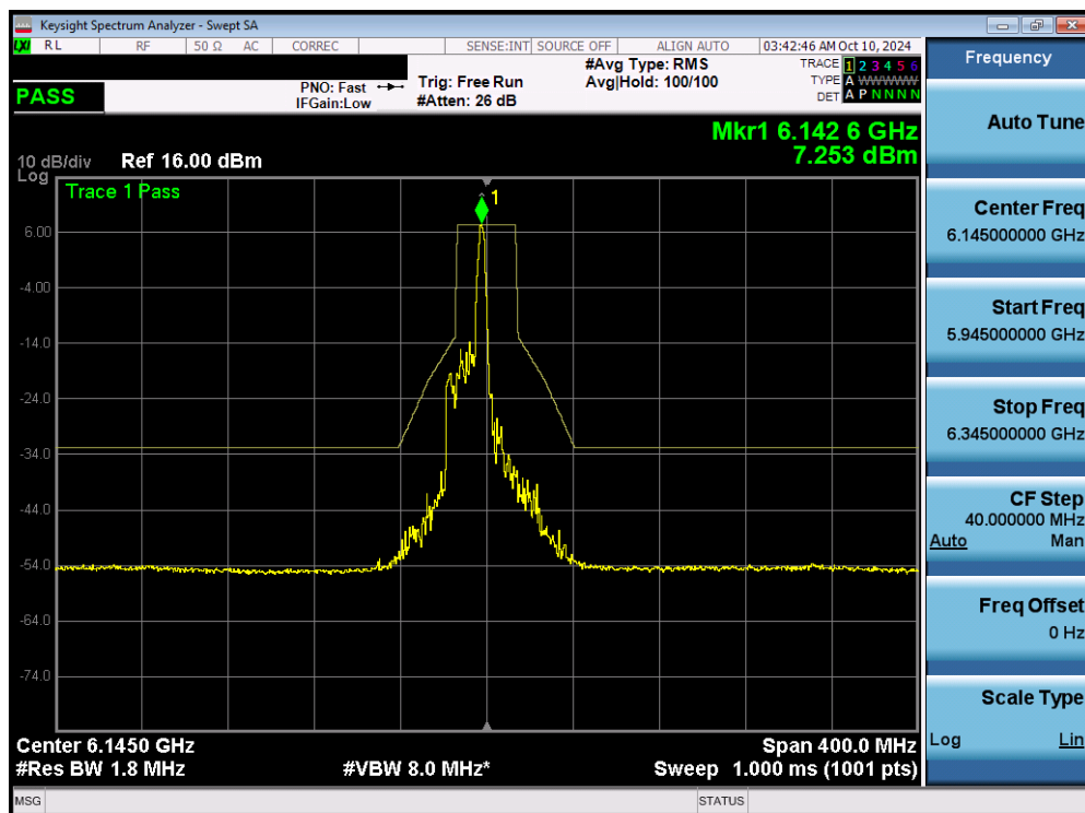
Plot 7-122. In Band Emissions Plot MIMO ANT1 (80MHz 802.11ax/be (26 Tones) (UNII Band 5) – Ch. 39) - SP
