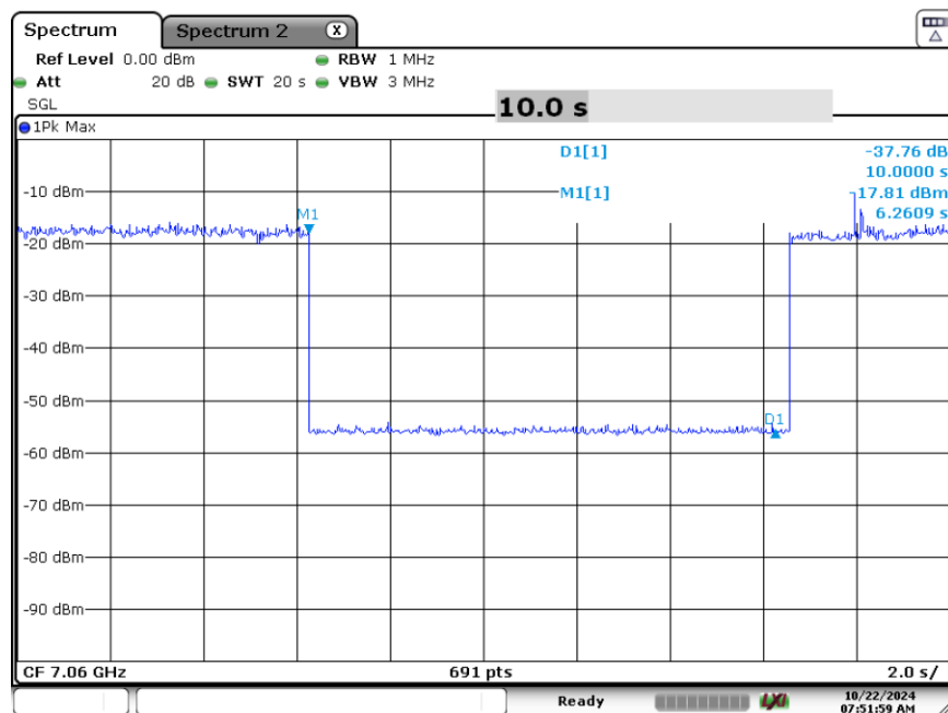
Plot 7-182. Contention Based Protocol Timing Plot (320MHz (UNII Band 8) – Ch. 191 Mid)
