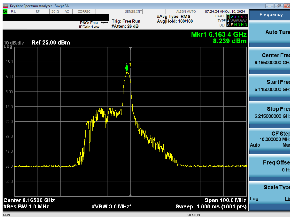
Plot 7-93. Power Spectral Density Plot MIMO ANT2 (40MHz 802.11ax/be (26 Tones) (UNII Band 5) – Ch. 43) - SP
