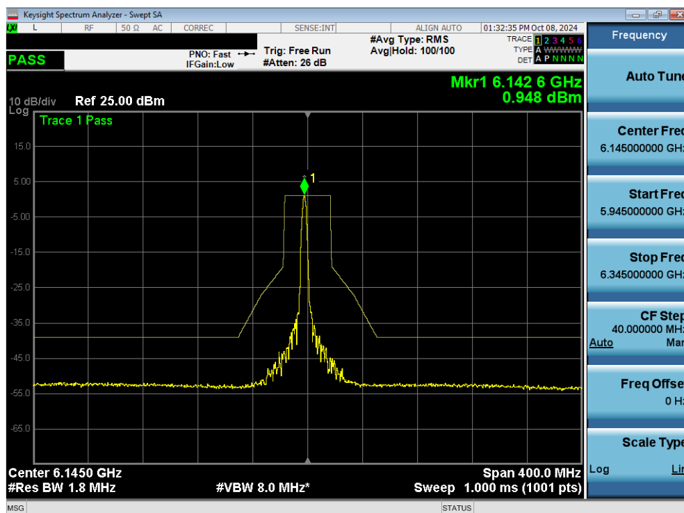
Plot 7-141. In Band Emissions Plot MIMO ANT2 (80MHz 802.11ax/be (26 Tones) (UNII Band 5) – Ch. 39) - LPI
