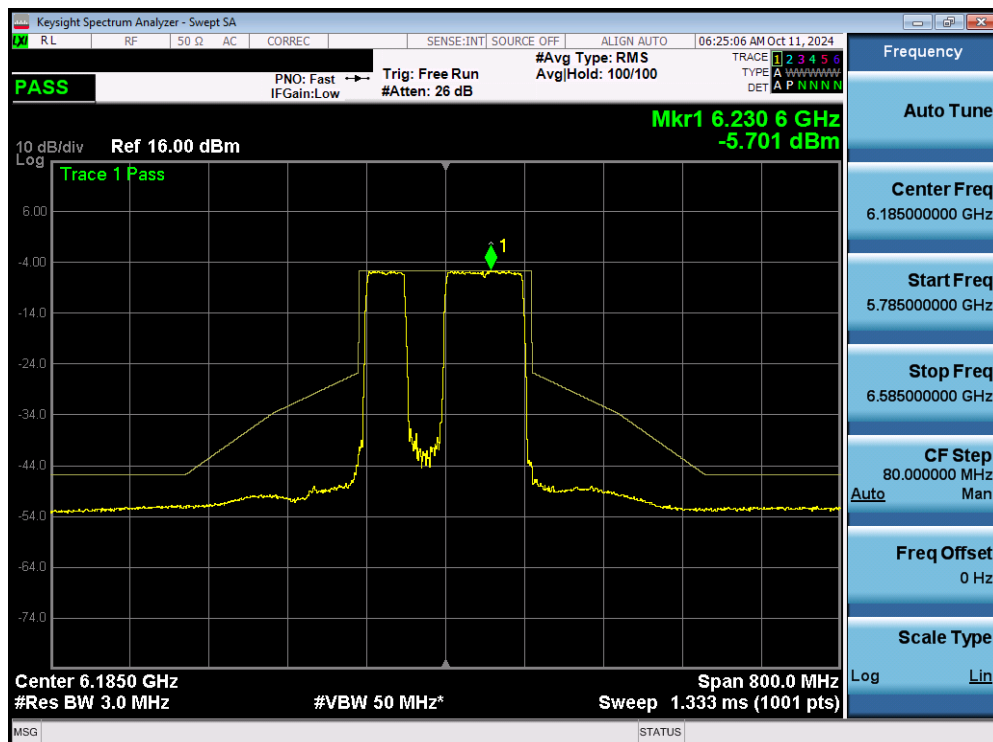
Plot 7-118. In Band Emissions Plot MIMO ANT1 (160MHz 802.11be (996+484 Tones) (UNII Band 5) – Ch. 47) LPI
