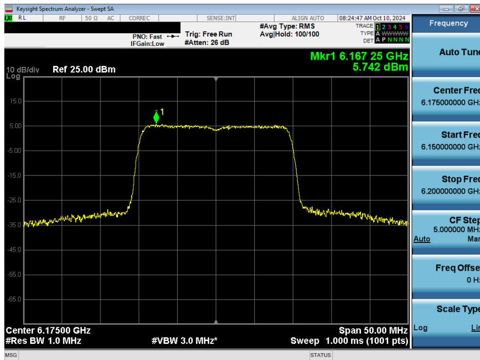
Plot 7-106. Power Spectral Density Plot MIMO ANT2 (20MHz 802.11ax/be (Full Tones) (UNII Band 5) – Ch. 45) - SP
