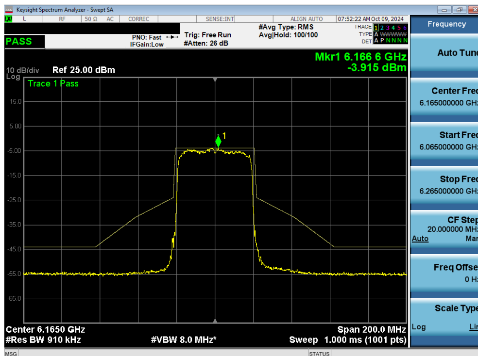
Plot 7-158. In Band Emissions Plot MIMO ANT2 (40MHz 802.11ax/be (Full Tones) (UNII Band 5) – Ch. 43) - LPI
