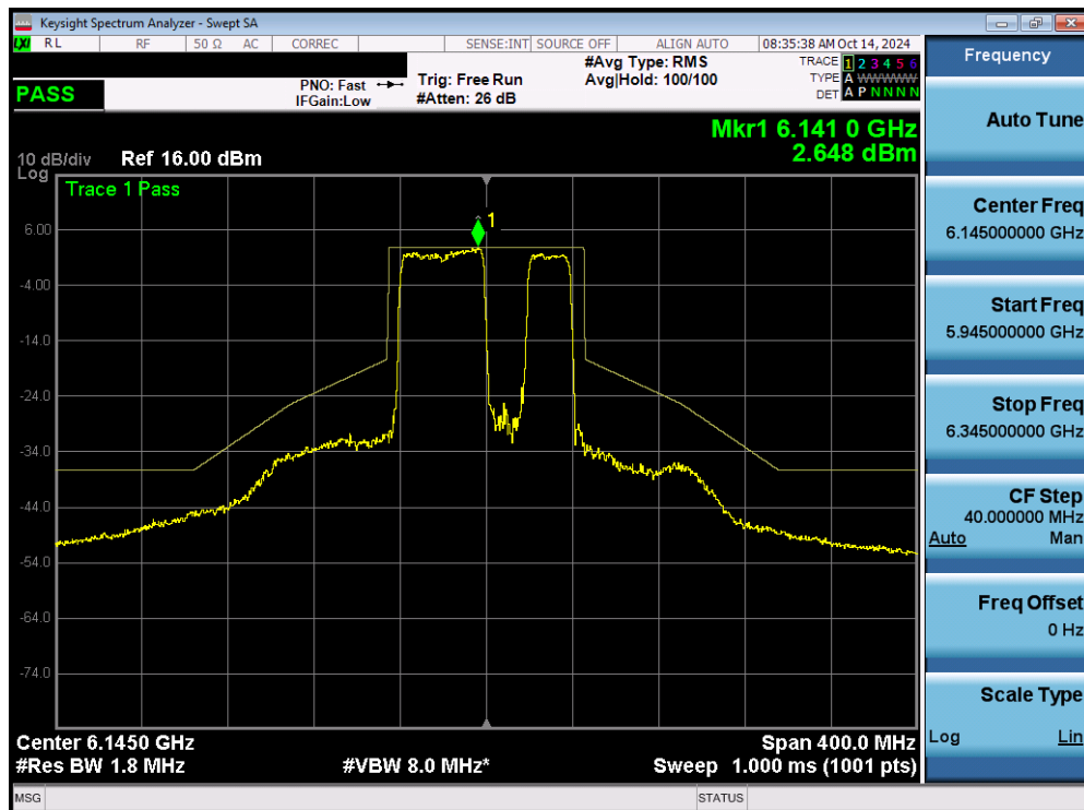
Plot 7-126. In Band Emissions Plot MIMO ANT1 (80MHz 802.11be (484+242 Tones) (UNII Band 5) – Ch. 39) SP
