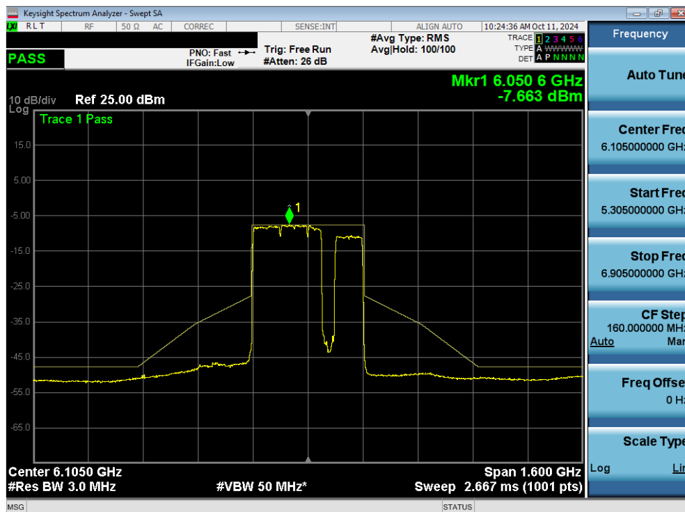
Plot 7-147. In Band Emissions Plot MIMO ANT2 (320MHz 802.11be (3*996+484 Tones) (UNII Band 5) – Ch. 31) LPI
