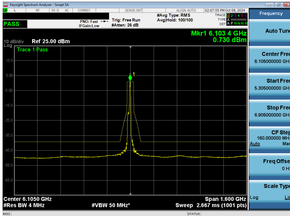
Plot 7-143. In Band Emissions Plot MIMO ANT2 (320MHz 802.11be (26 Tones) (UNII Band 5) – Ch. 31) - LPI
