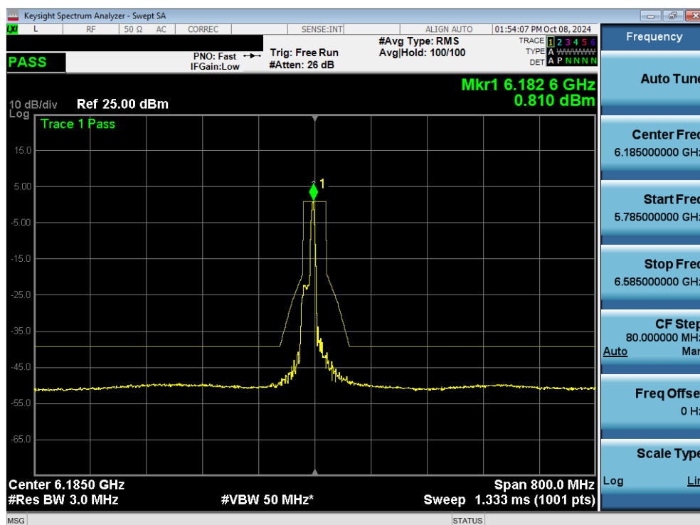
Plot 7-142. In Band Emissions Plot MIMO ANT2 (160MHz 802.11ax/be (26 Tones) (UNII Band 5) – Ch. 47) - LPI
