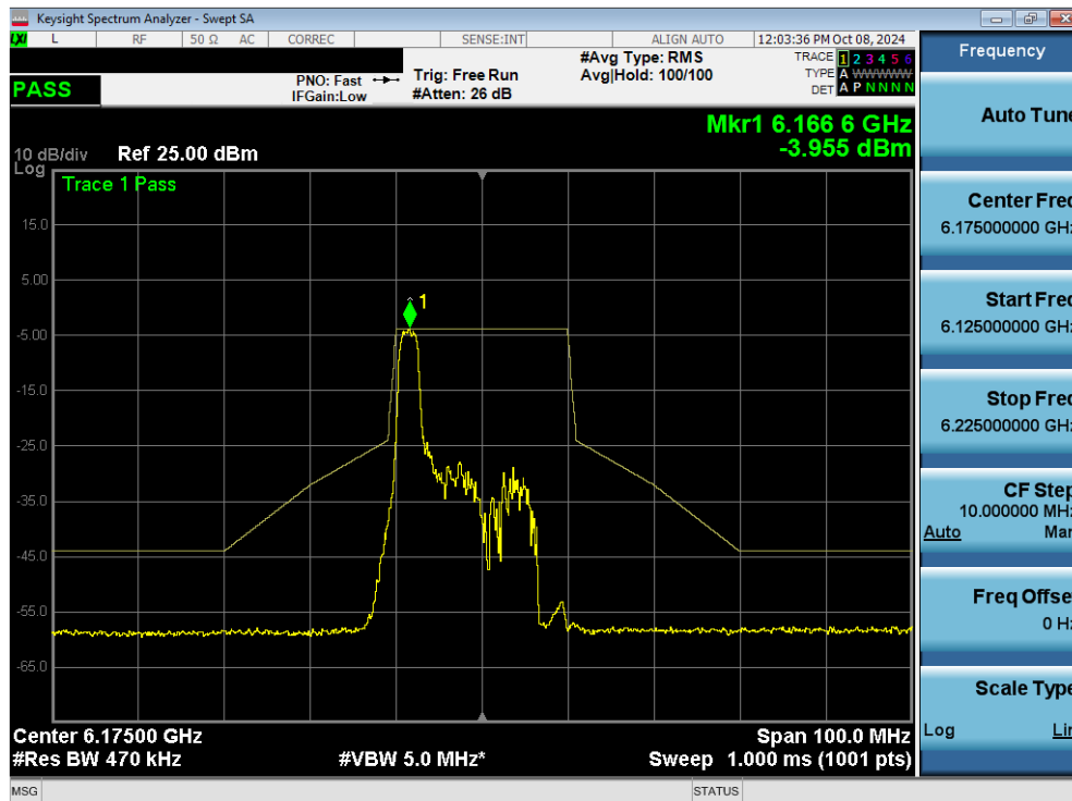
Plot 7-139. In Band Emissions Plot MIMO ANT2 (20MHz 802.11ax/be (26 Tones) (UNII Band 5) – Ch. 45) - LPI
