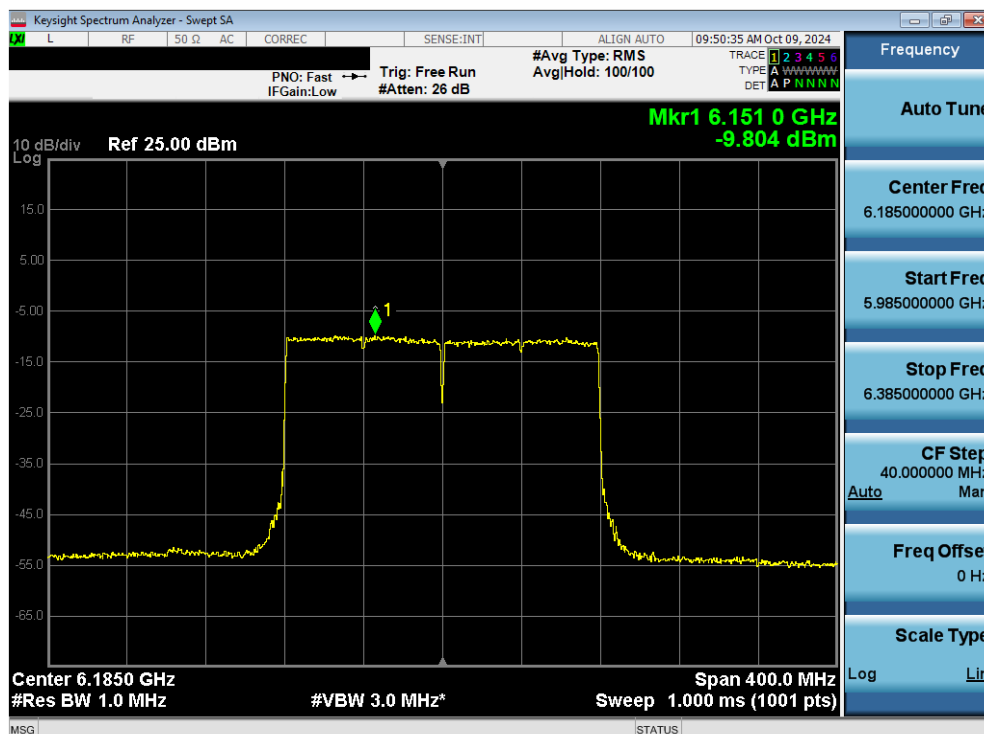
Plot 7-104. Power Spectral Density Plot MIMO ANT2 (160MHz 802.11ax/be (Full Tones) (UNII Band 5) – Ch. 47) - LPI
