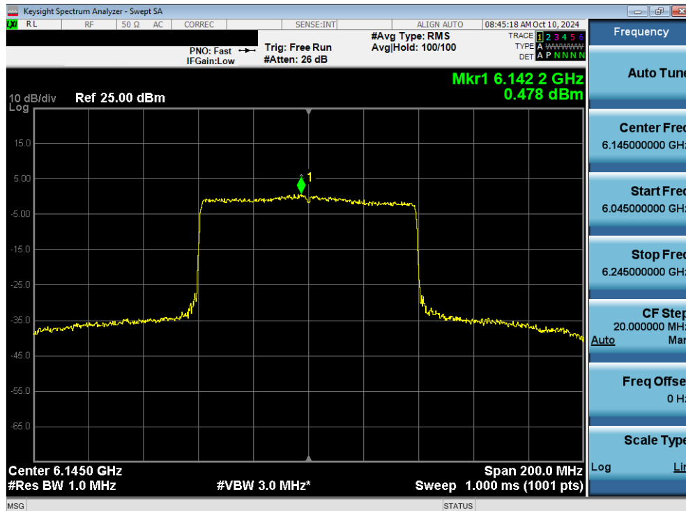
Plot 7-108. Power Spectral Density Plot MIMO ANT2 (80MHz 802.11ax/be (Full Tones) (UNII Band 5) – Ch. 39) - SP
