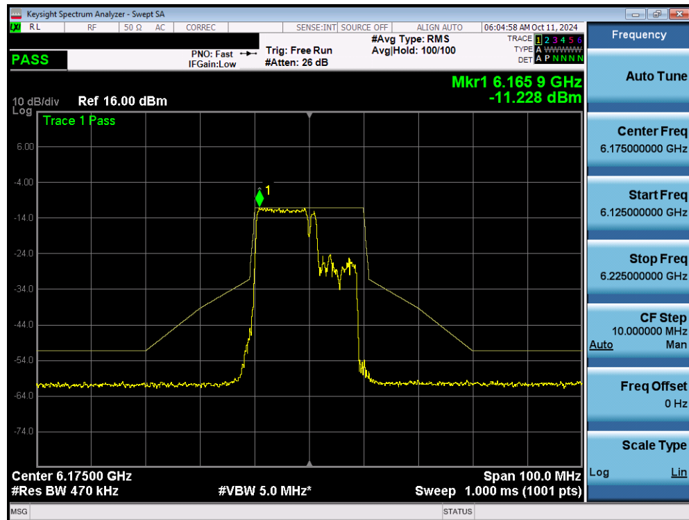
Plot 7-116. In Band Emissions Plot MIMO ANT1 (20MHz 802.11be (106+26 Tones) (UNII Band 5) – Ch. 45) - LPI
