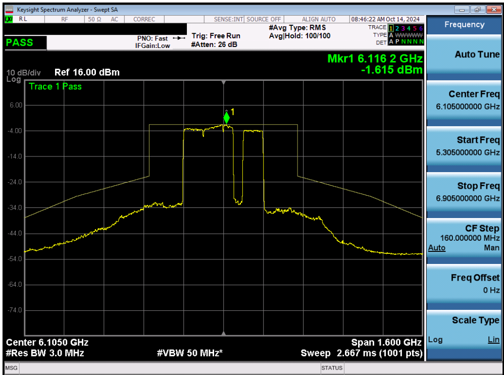
Plot 7-128. In Band Emissions Plot MIMO ANT1 (320MHz 802.11be (3*996+484 Tones) (UNII Band 5) – Ch. 31) SP
