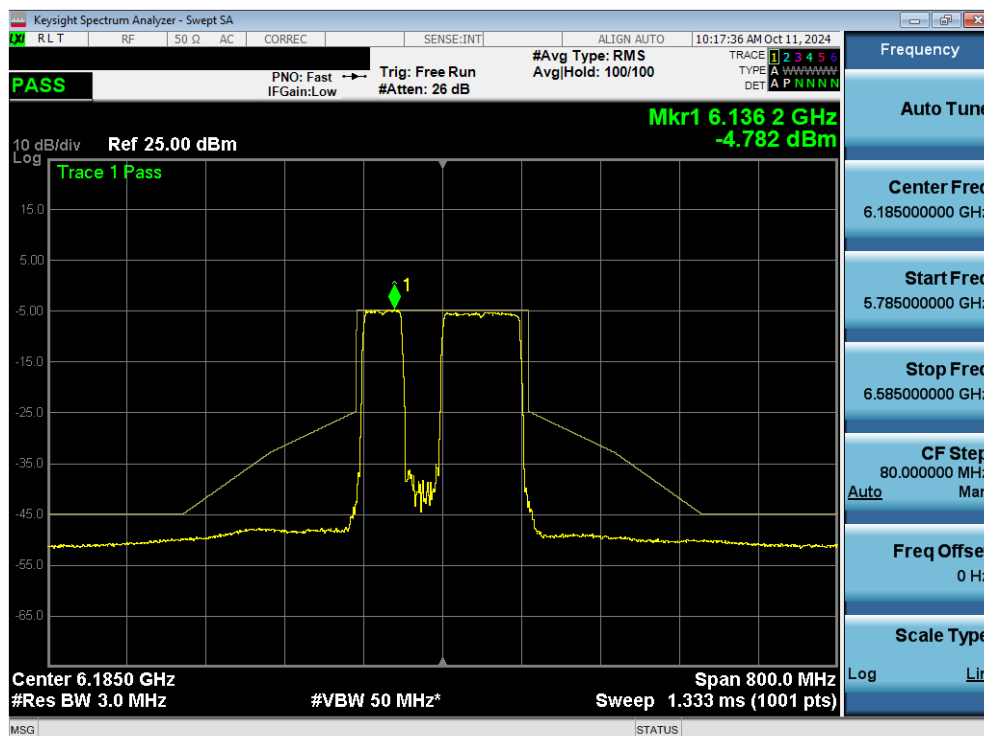
Plot 7-146. In Band Emissions Plot MIMO ANT2 (160MHz 802.11be (996+484 Tones) (UNII Band 5) – Ch. 47) LPI
