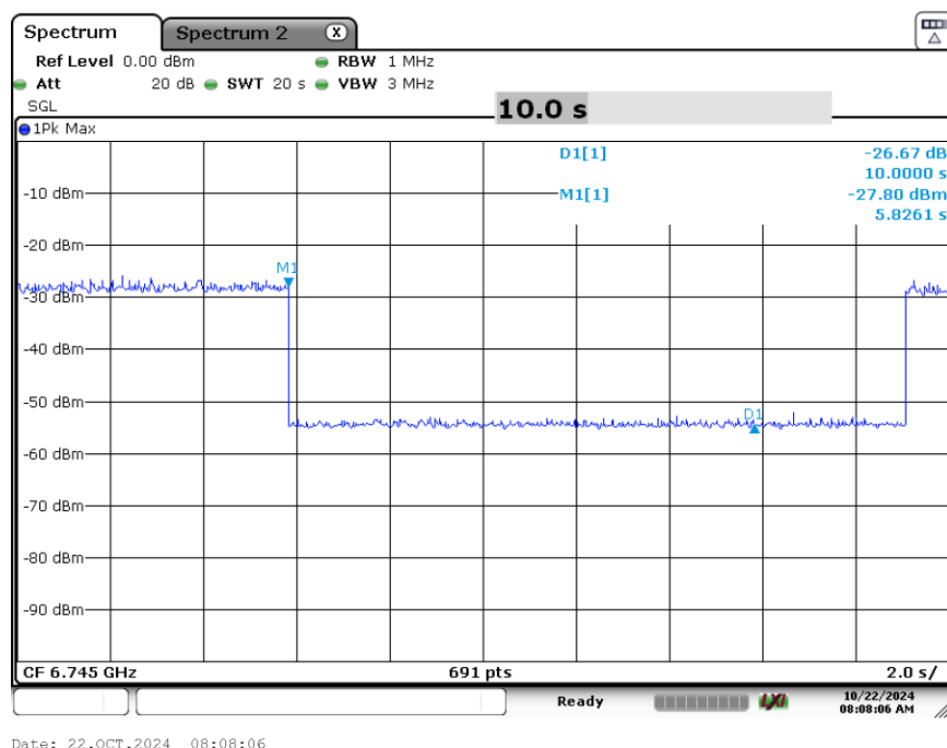
Plot 7-178. Contention Based Protocol Timing Plot (320MHz (UNII Band 7) – Ch. 159 Mid)
