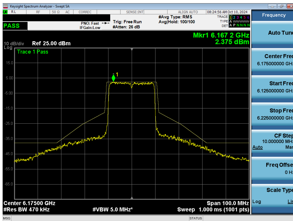
Plot 7-162. In Band Emissions Plot MIMO ANT2 (20MHz 802.11ax/be (Full Tones) (UNII Band 5) – Ch. 45) - SP
