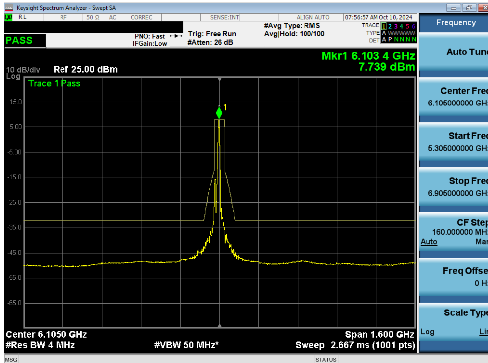
Plot 7-152. In Band Emissions Plot MIMO ANT2 (320MHz 802.11be (26 Tones) (UNII Band 5) – Ch. 31) - SP
