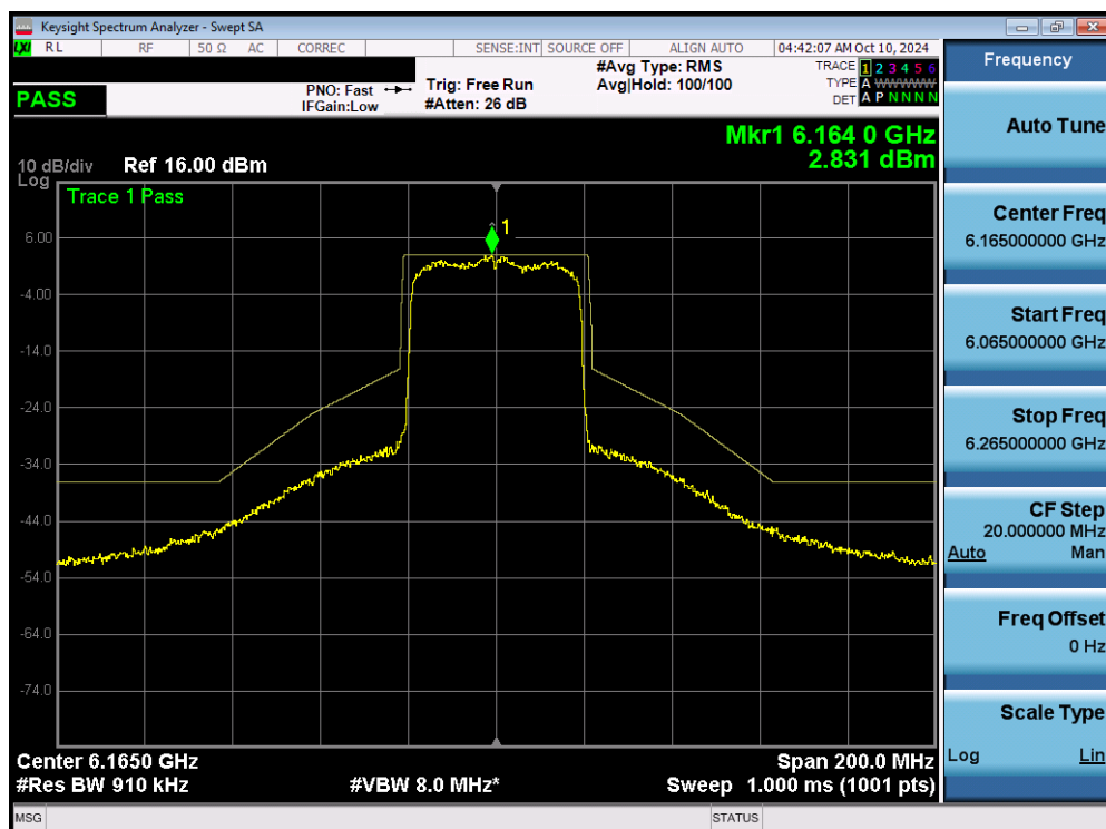
Plot 7-135. In Band Emissions Plot MIMO ANT1 (40MHz 802.11ax/be (Full Tones) (UNII Band 5) – Ch. 43) - SP
