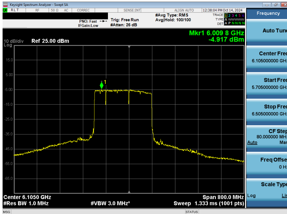
Plot 7-100. Power Spectral Density Plot MIMO ANT2 (320MHz 802.11be (UNII Band 5) – Ch. 31) SP
