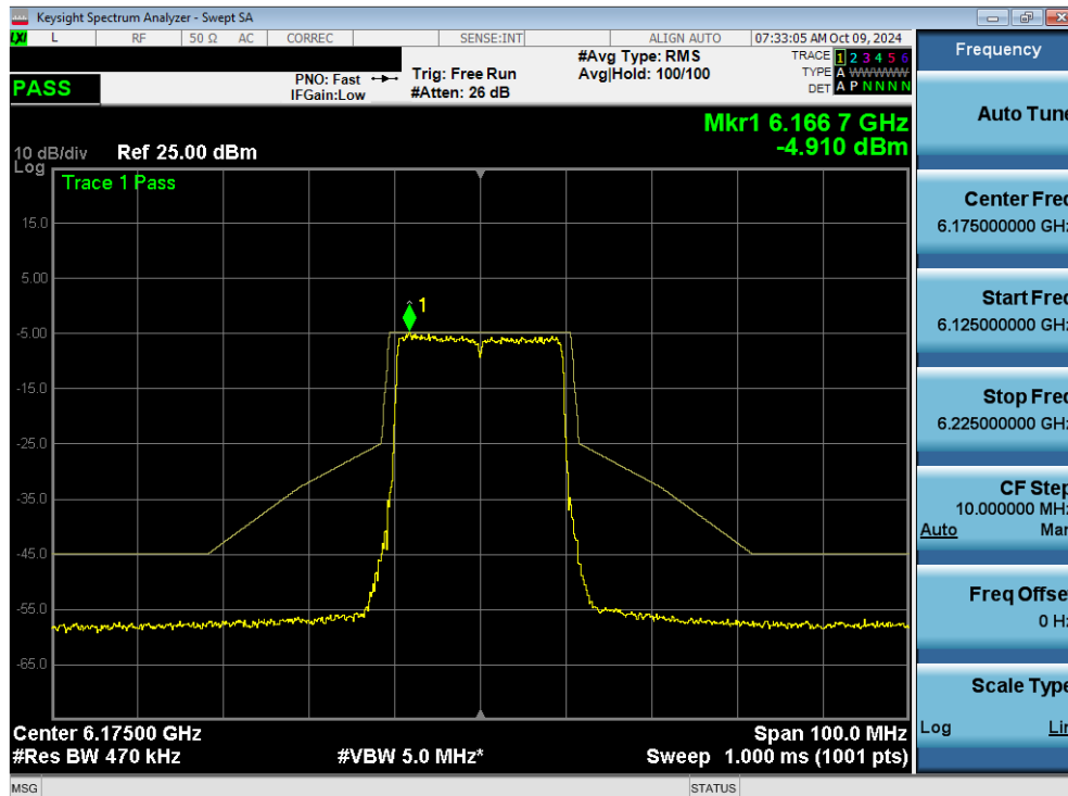
Plot 7-157. In Band Emissions Plot MIMO ANT2 (20MHz 802.11ax/be (Full Tones) (UNII Band 5) – Ch. 45) - LPI
