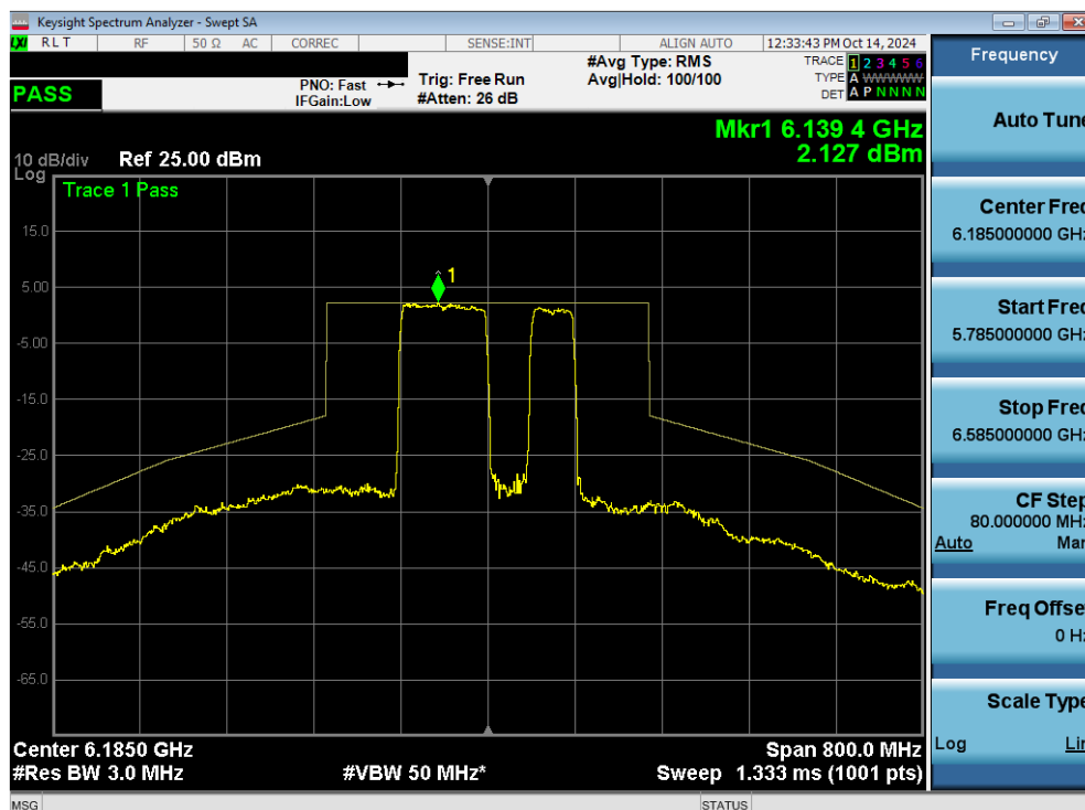
Plot 7-155. In Band Emissions Plot MIMO ANT2 (160MHz 802.11be (996+484 Tones) (UNII Band 5) – Ch. 47) SP
