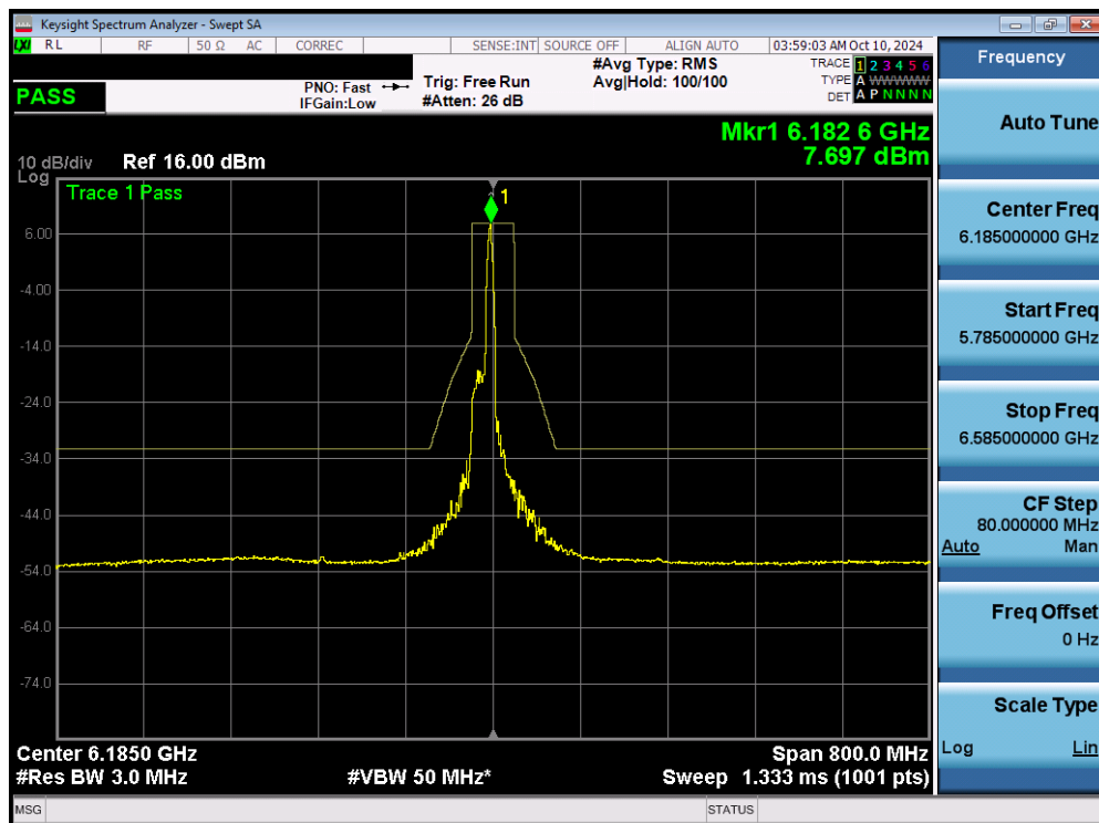
Plot 7-123. In Band Emissions Plot MIMO ANT1 (160MHz 802.11ax/be (26 Tones) (UNII Band 5) – Ch. 47) - SP
