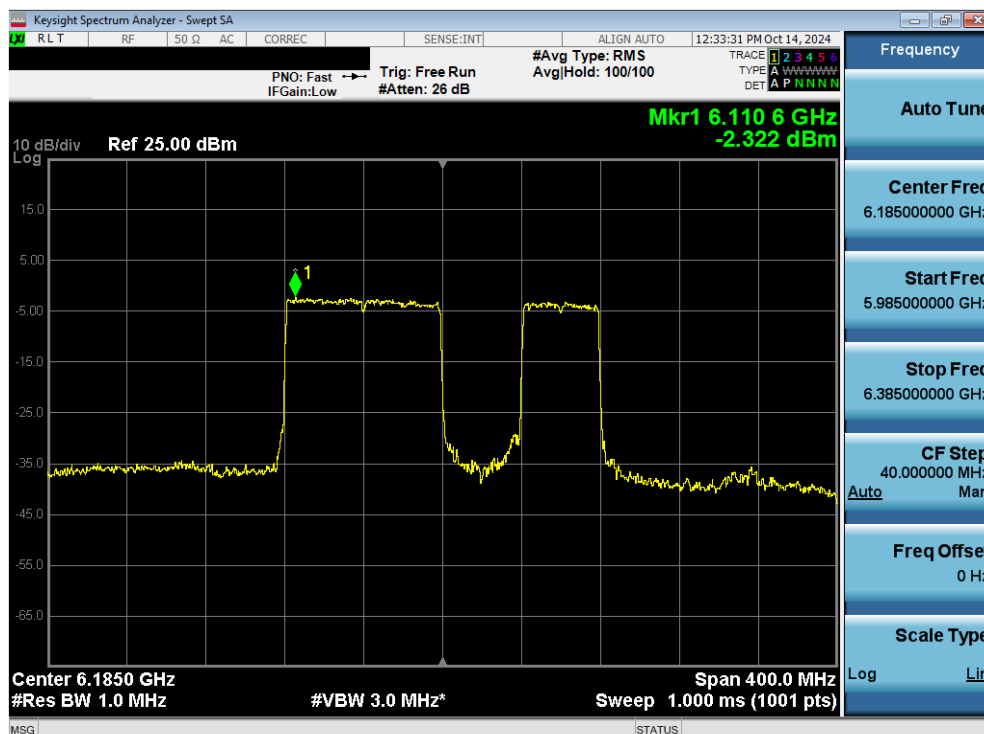
Plot 7-99. Power Spectral Density Plot MIMO ANT2 (160MHz 802.11be (996+484 Tones) (UNII Band 5) – Ch. 47) SP
