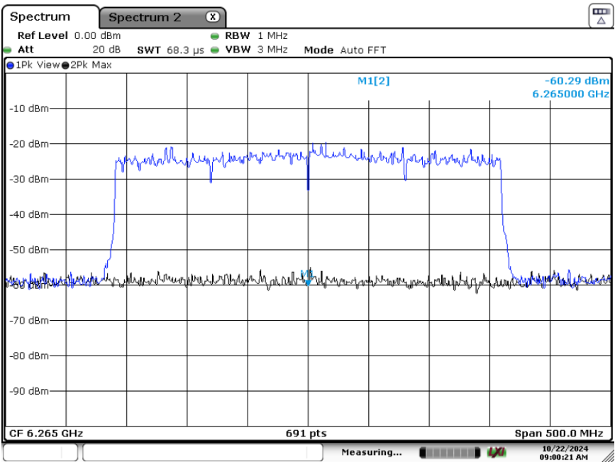
Plot 7-185. CBP 320MHz Channel - Injection Center – [6265 MHz]
