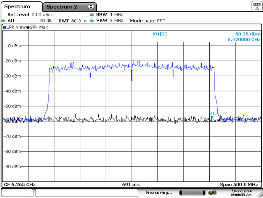
Plot 7-186. CBP 320MHz Channel - Injection Upper Edge – [6420 MHz]
