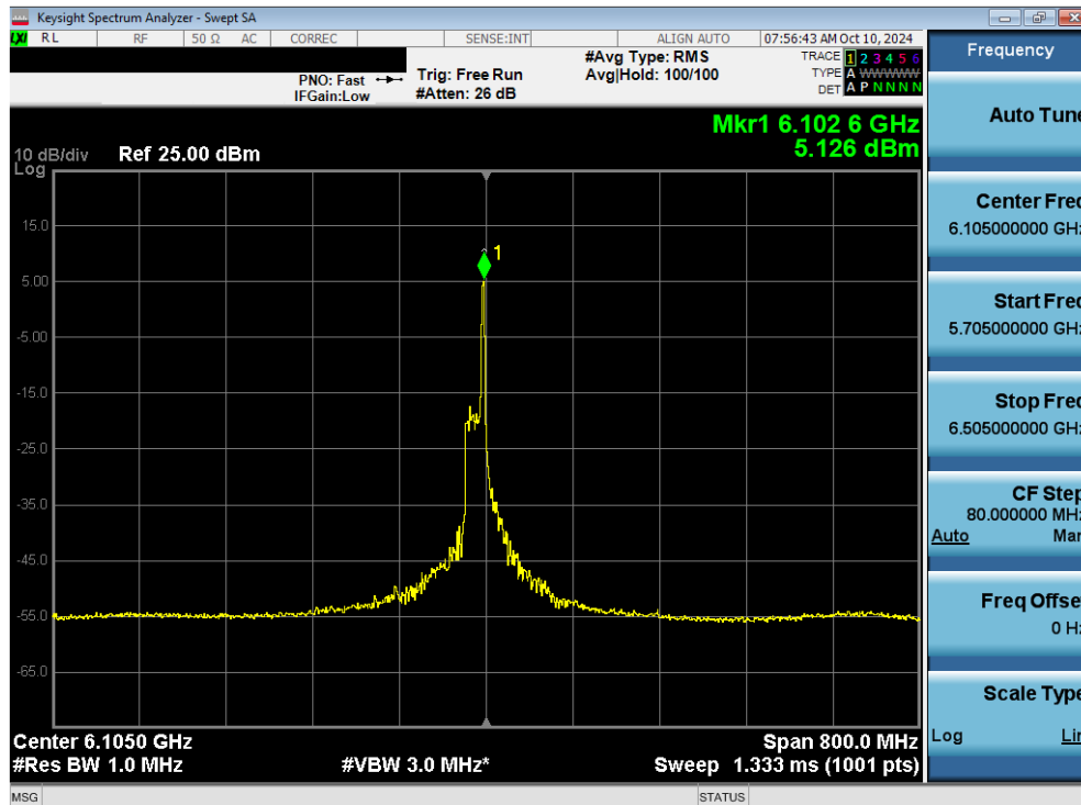
Plot 7-96. Power Spectral Density Plot MIMO ANT2 (320MHz 802.11be (26 Tones) (UNII Band 5) – Ch. 31) - SP
