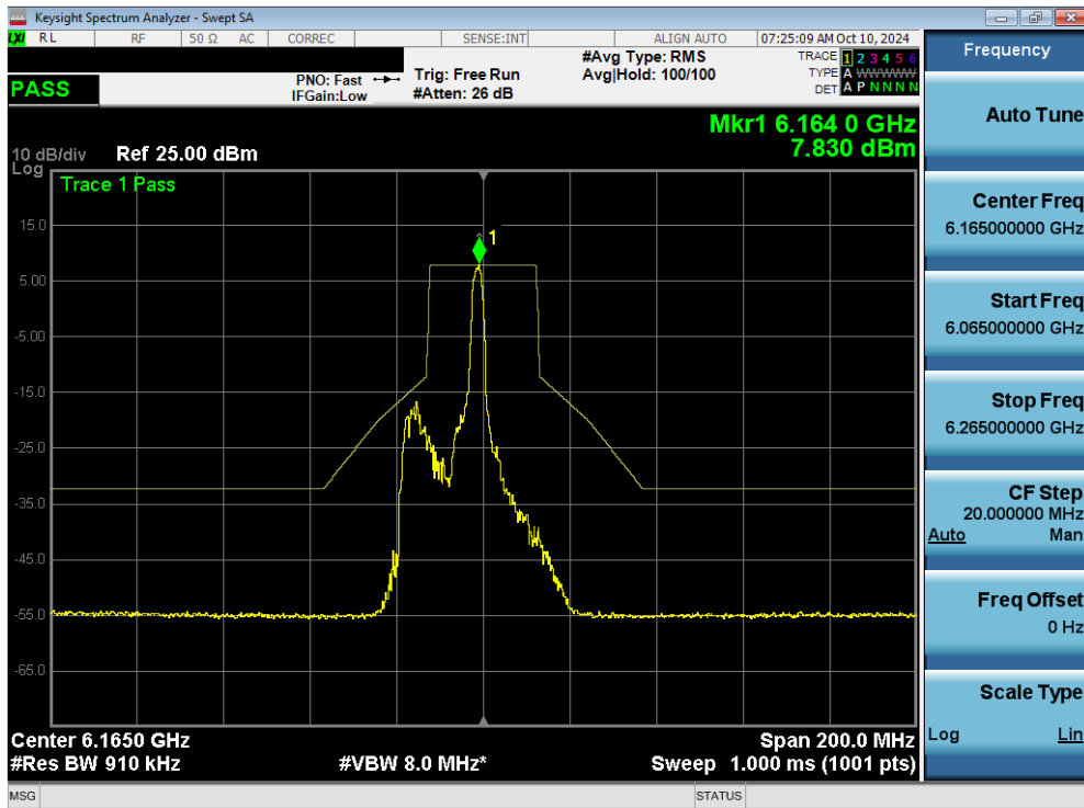
Plot 7-149. In Band Emissions Plot MIMO ANT2 (40MHz 802.11ax/be (26 Tones) (UNII Band 5) – Ch. 43) - SP
