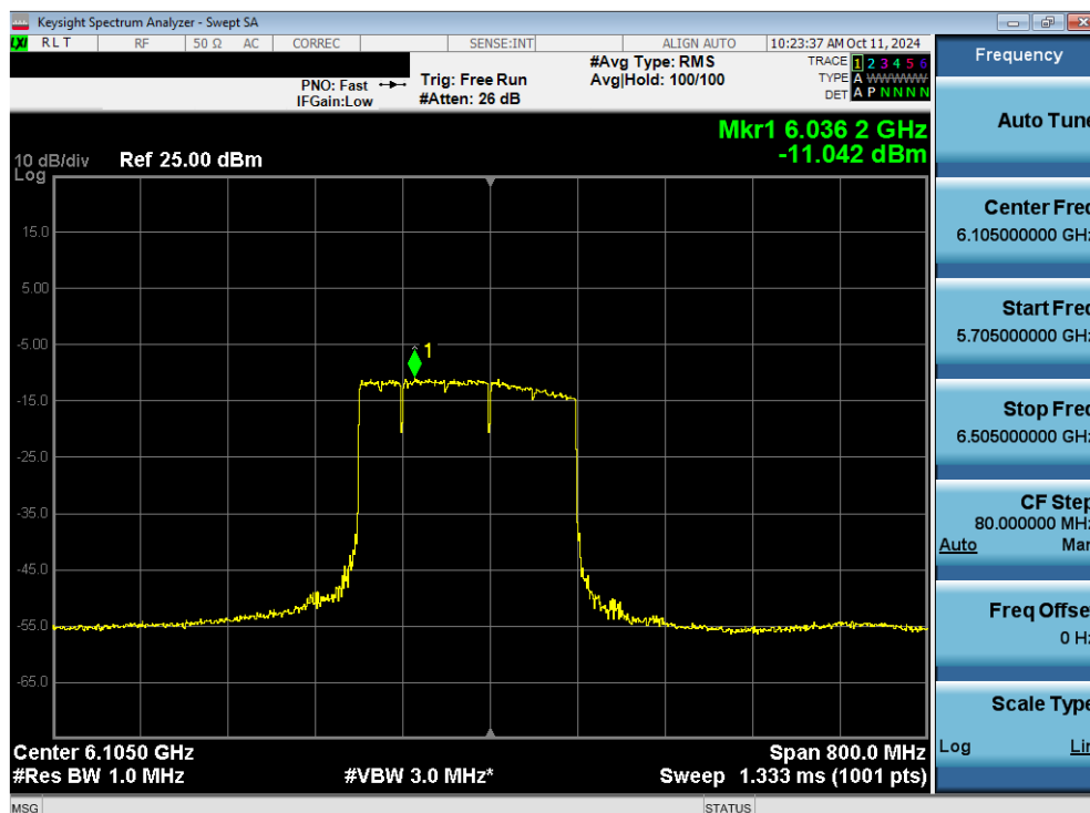
Plot 7-91. Power Spectral Density Plot MIMO ANT2 (320MHz 802.11be (UNII Band 5) – Ch. 31) LPI
