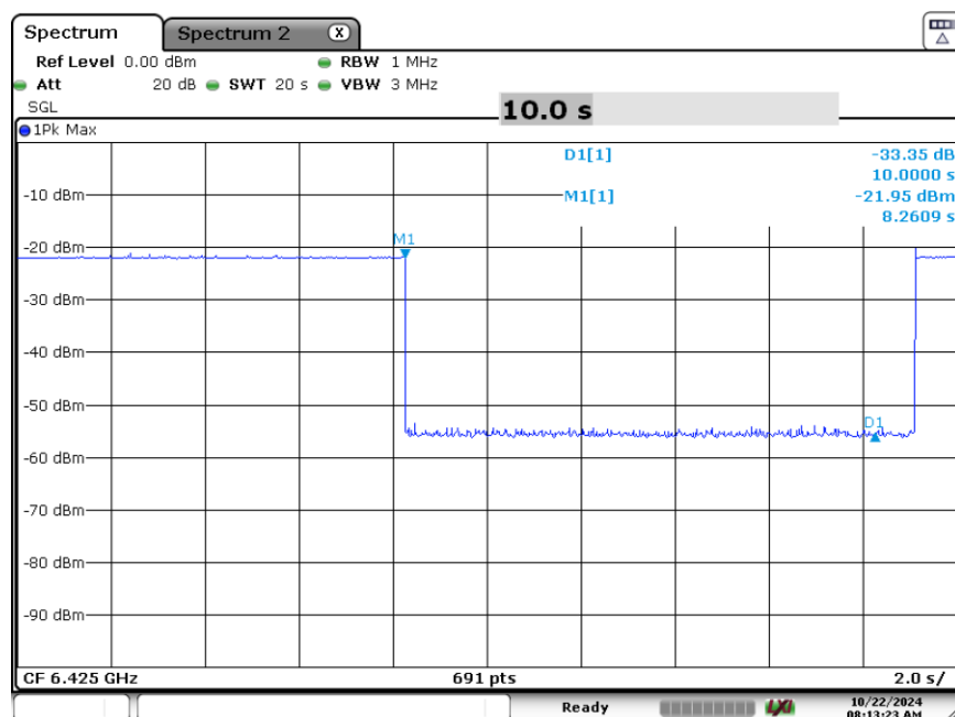
Plot 7-174. Contention Based Protocol Timing Plot (320MHz (UNII Band 6) – Ch. 95 Mid)
