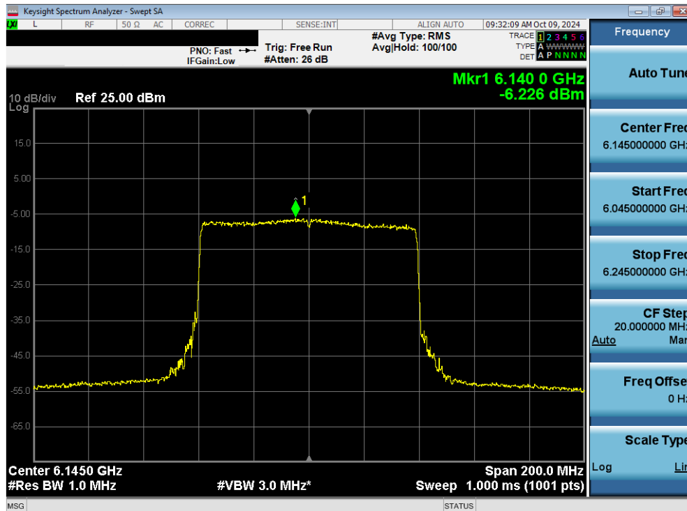
Plot 7-103. Power Spectral Density Plot MIMO ANT2 (80MHz 802.11ax/be (Full Tones) (UNII Band 5) – Ch. 39) - LPI
