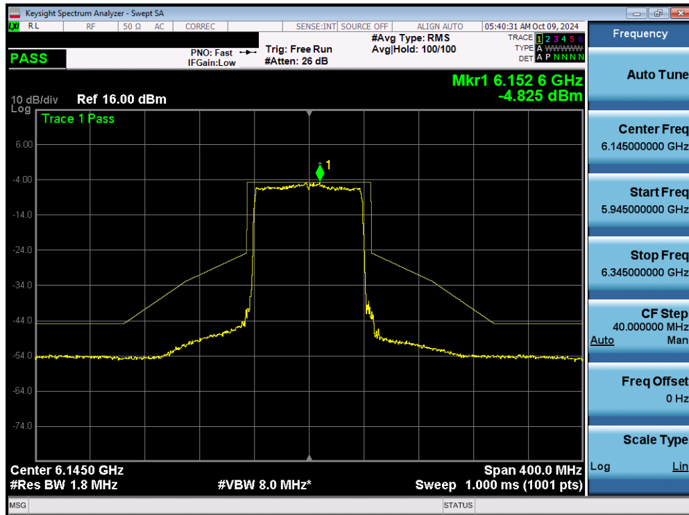
Plot 7-131. In Band Emissions Plot MIMO ANT1 (80MHz 802.11ax/be (Full Tones) (UNII Band 5) – Ch. 39) - LPI
