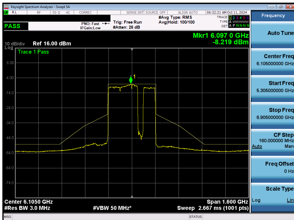
Plot 7-119. In Band Emissions Plot MIMO ANT1 (320MHz 802.11be (3*996+484 Tones) (UNII Band 5) – Ch. 31) LPI
