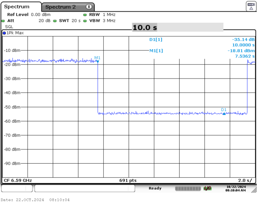
Plot 7-177. Contention Based Protocol Timing Plot (320MHz (UNII Band 7) – Ch. 159 Low)
