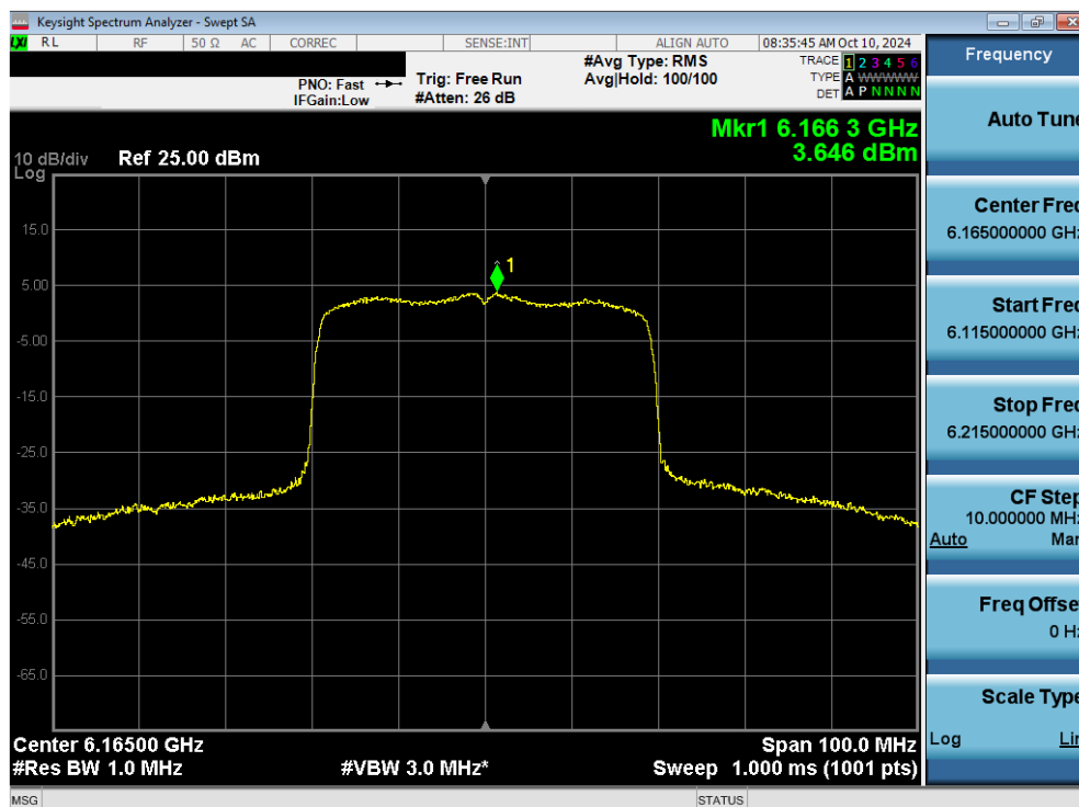
Plot 7-107. Power Spectral Density Plot MIMO ANT2 (40MHz 802.11ax/be (Full Tones) (UNII Band 5) – Ch. 43) - SP
