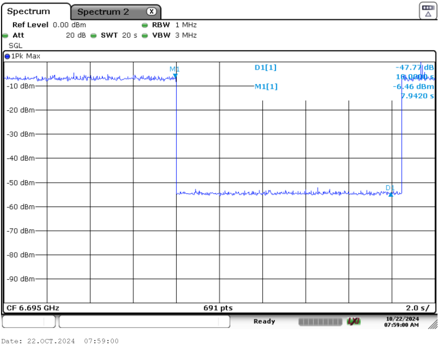
Plot 7-176. Contention Based Protocol Timing Plot (20MHz (UNII Band 7) – Ch. 149)
