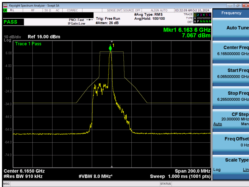
Plot 7-121. In Band Emissions Plot MIMO ANT1 (40MHz 802.11ax/be (26 Tones) (UNII Band 5) – Ch. 43) - SP
