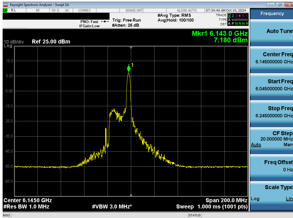
Plot 7-94. Power Spectral Density Plot MIMO ANT2 (80MHz 802.11ax/be (26 Tones) (UNII Band 5) – Ch. 39) - SP
