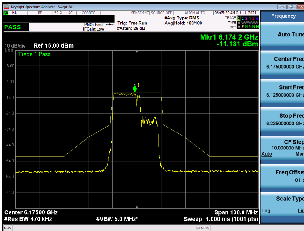
Plot 7-144. In Band Emissions Plot MIMO ANT2 (20MHz 802.11be (106+26 Tones) (UNII Band 5) – Ch. 45) - LPI
