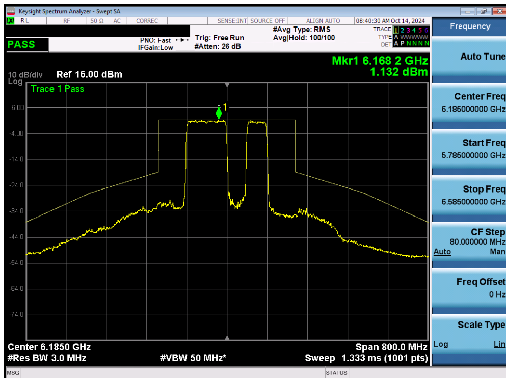
Plot 7-127. In Band Emissions Plot MIMO ANT1 (160MHz 802.11be (996+484 Tones) (UNII Band 5) – Ch. 47) SP
