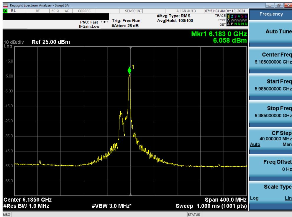
Plot 7-95. Power Spectral Density Plot MIMO ANT2 (160MHz 802.11ax/be (26 Tones) (UNII Band 5) – Ch. 47) - SP
