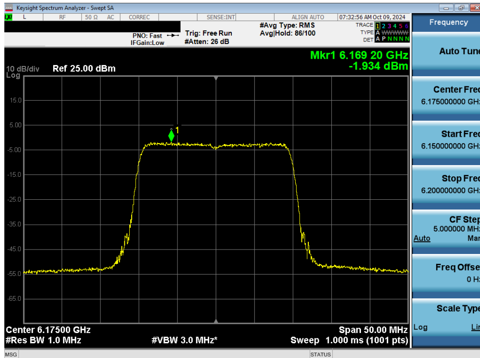
Plot 7-101. Power Spectral Density Plot MIMO ANT2 (20MHz 802.11ax/be (Full Tones) (UNII Band 5) – Ch. 45) - LPI
