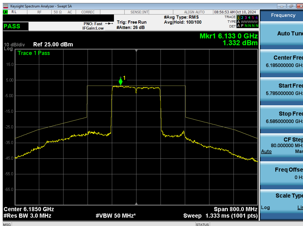
Plot 7-165. In Band Emissions Plot MIMO ANT2 (160MHz 802.11ax/be (Full Tones) (UNII Band 5) – Ch. 47) - SP
