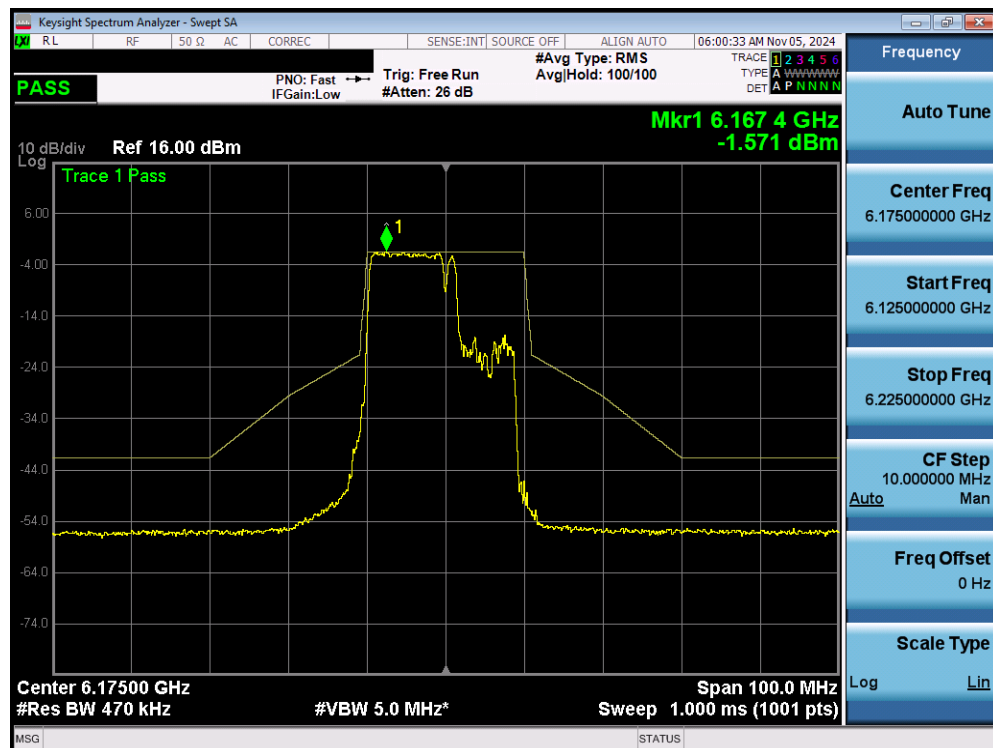
Plot 7-125. In Band Emissions Plot MIMO ANT1 (20MHz 802.11be (106+26 Tones) (UNII Band 5) – Ch. 45) - SP
