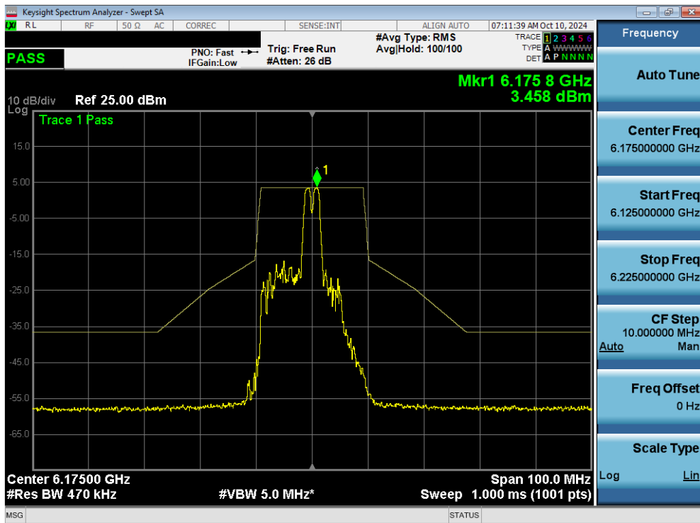
Plot 7-148. In Band Emissions Plot MIMO ANT2 (20MHz 802.11ax/be (26 Tones) (UNII Band 5) – Ch. 45) - SP
