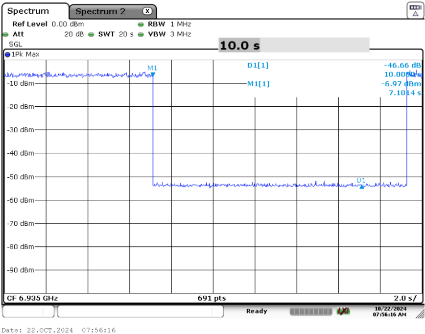
Plot 7-180. Contention Based Protocol Timing Plot (20MHz (UNII Band 8) – Ch. 197)
