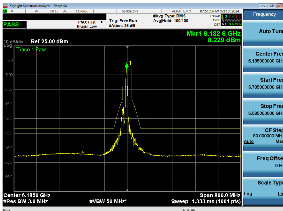
Plot 7-151. In Band Emissions Plot MIMO ANT2 (160MHz 802.11ax/be (26 Tones) (UNII Band 5) – Ch. 47) - SP
