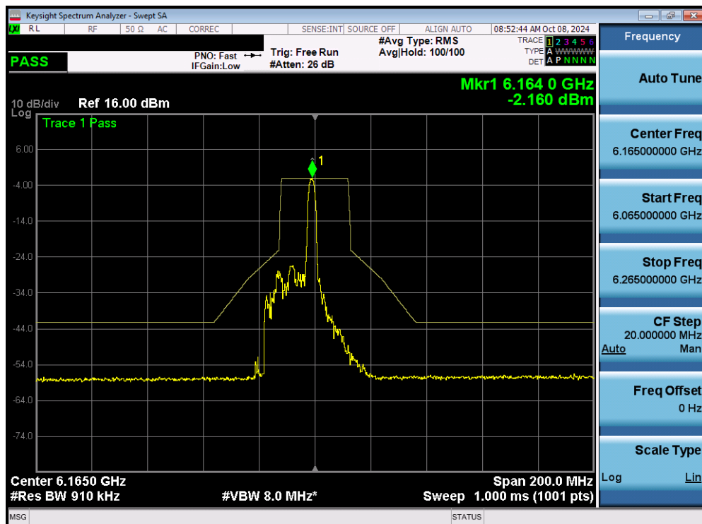
Plot 7-112. In Band Emissions Plot MIMO ANT1 (40MHz 802.11ax/be (26 Tones) (UNII Band 5) – Ch. 43) - LPI
