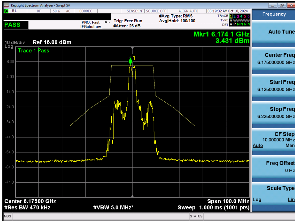
Plot 7-120. In Band Emissions Plot MIMO ANT1 (20MHz 802.11ax/be (26 Tones) (UNII Band 5) – Ch. 45) - SP
