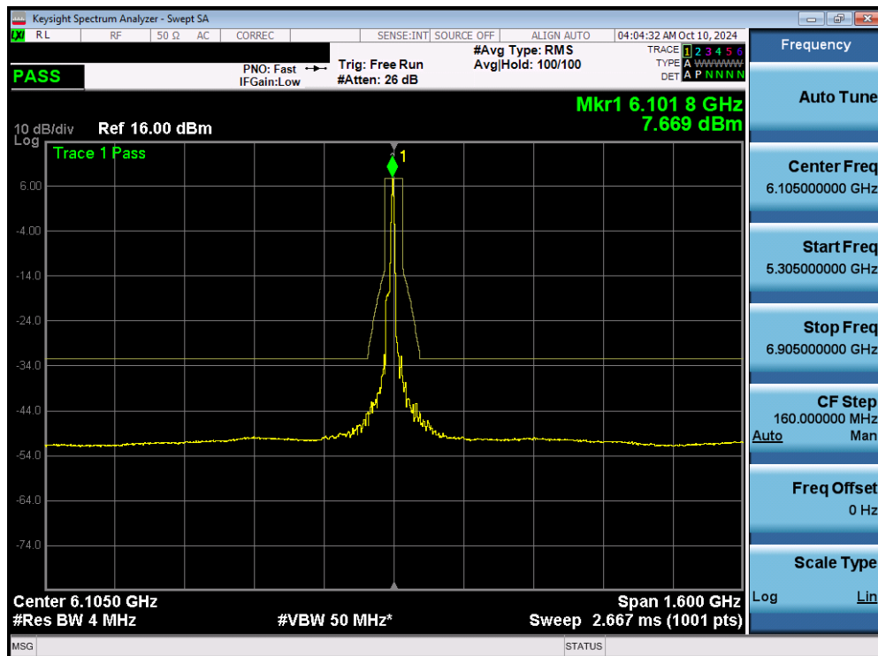
Plot 7-124. In Band Emissions Plot MIMO ANT1 (320MHz 802.11be (26 Tones) (UNII Band 5) – Ch. 31) - SP
