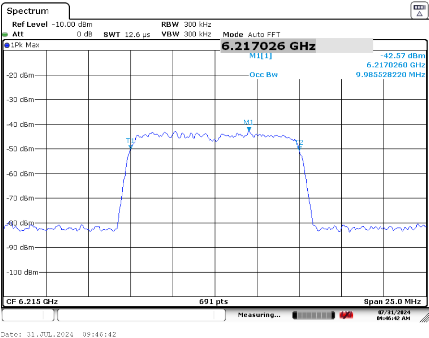
Plot 7-167. AWGN Signal (Demonstration)
