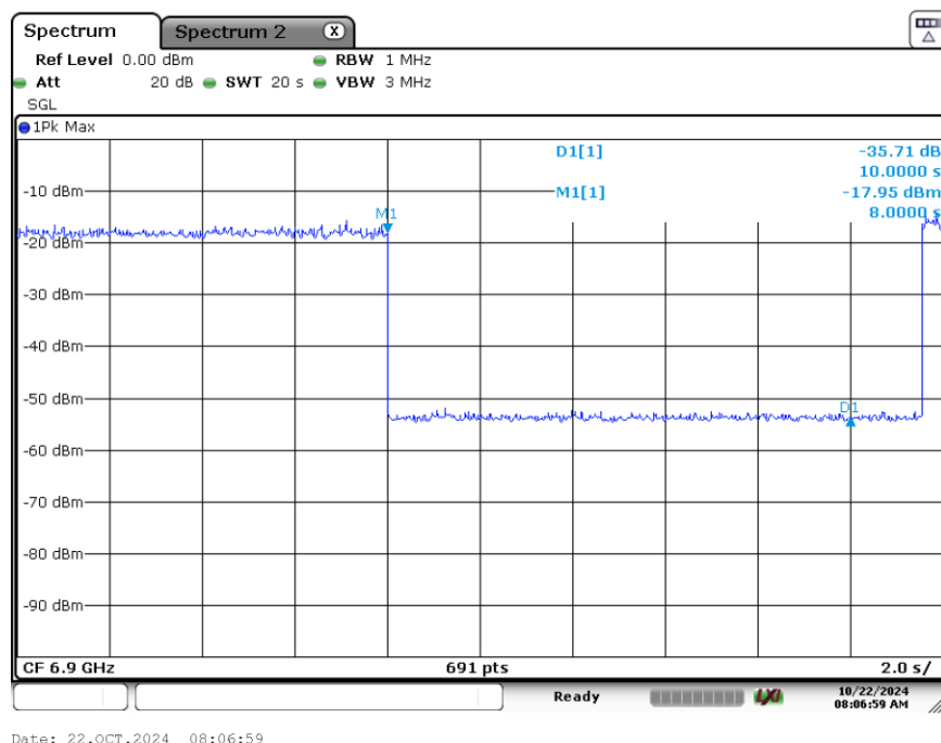
Plot 7-179. Contention Based Protocol Timing Plot (320MHz (UNII Band 7) – Ch. 159 High)
