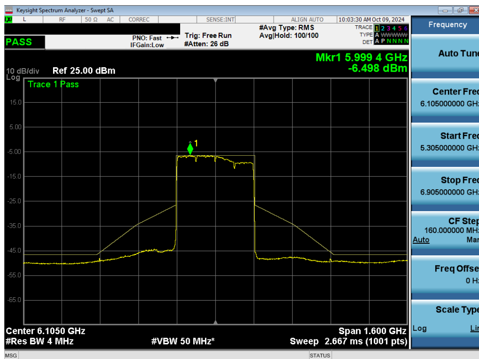
Plot 7-161. In Band Emissions Plot MIMO ANT2 (320MHz 802.11be (Full Tones) (UNII Band 5) – Ch. 31) - LPI
