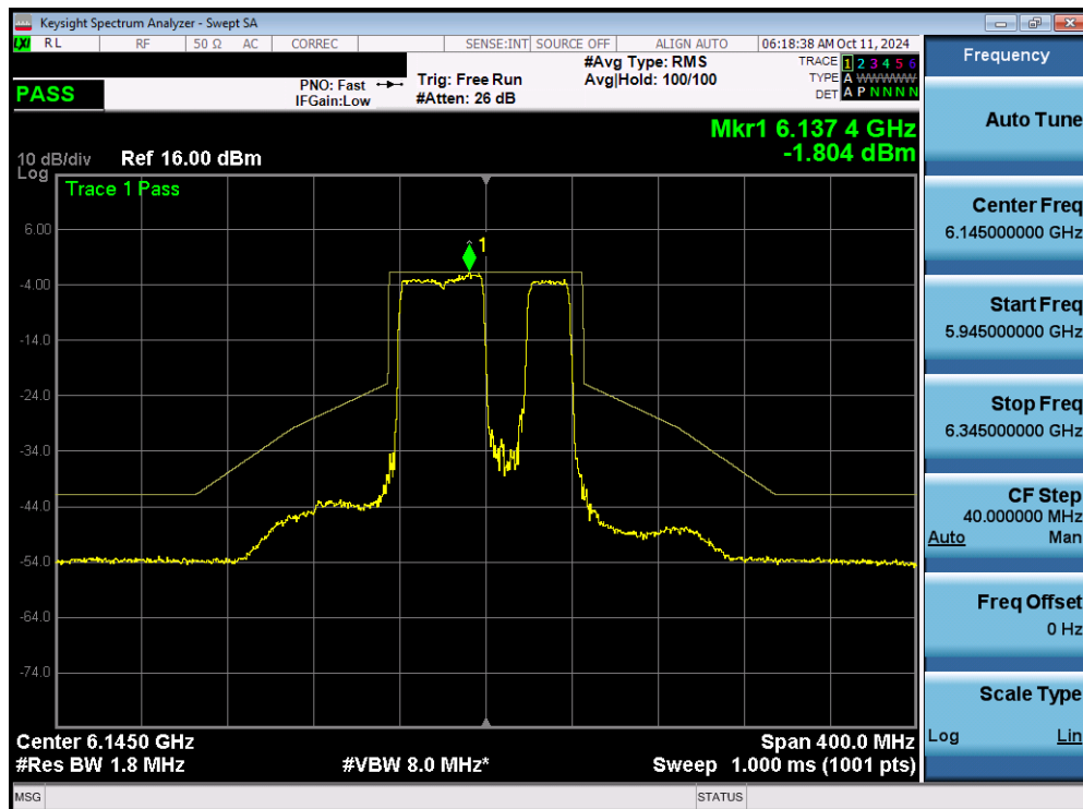
Plot 7-117. In Band Emissions Plot MIMO ANT1 (80MHz 802.11be (484+242 Tones) (UNII Band 5) – Ch. 39) LPI
