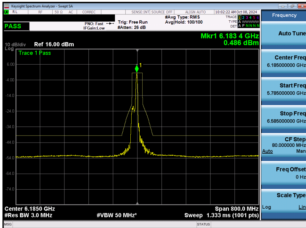
Plot 7-114. In Band Emissions Plot MIMO ANT1 (160MHz 802.11ax/be (26 Tones) (UNII Band 5) – Ch. 47) - LPI
