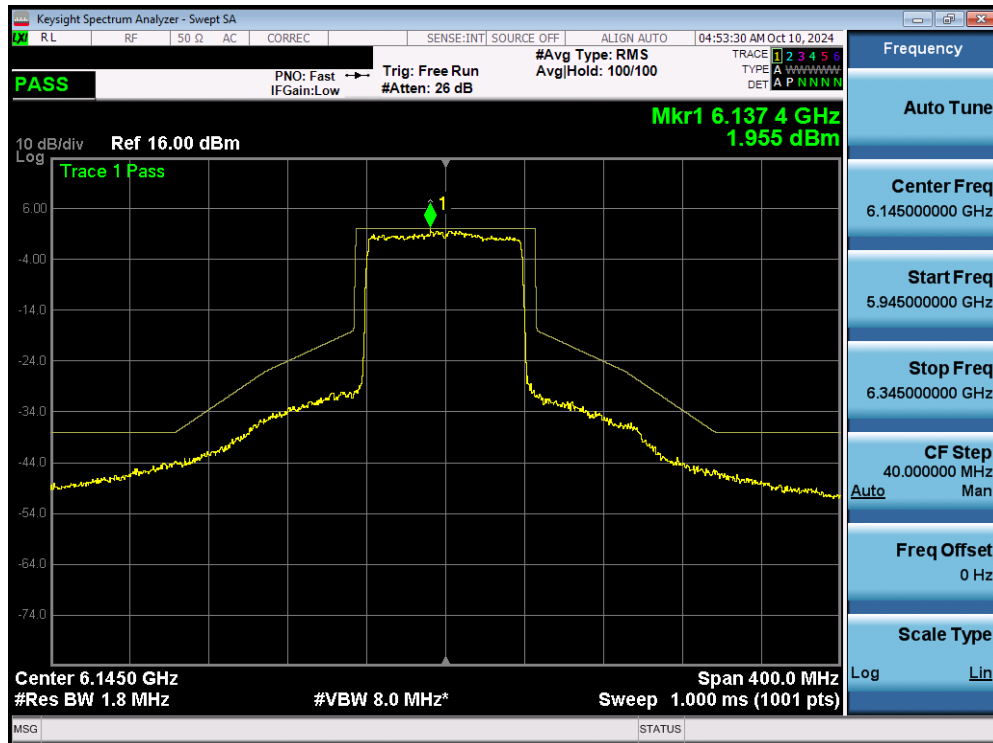
Plot 7-136. In Band Emissions Plot MIMO ANT1 (80MHz 802.11ax/be (Full Tones) (UNII Band 5) – Ch. 39) - SP
