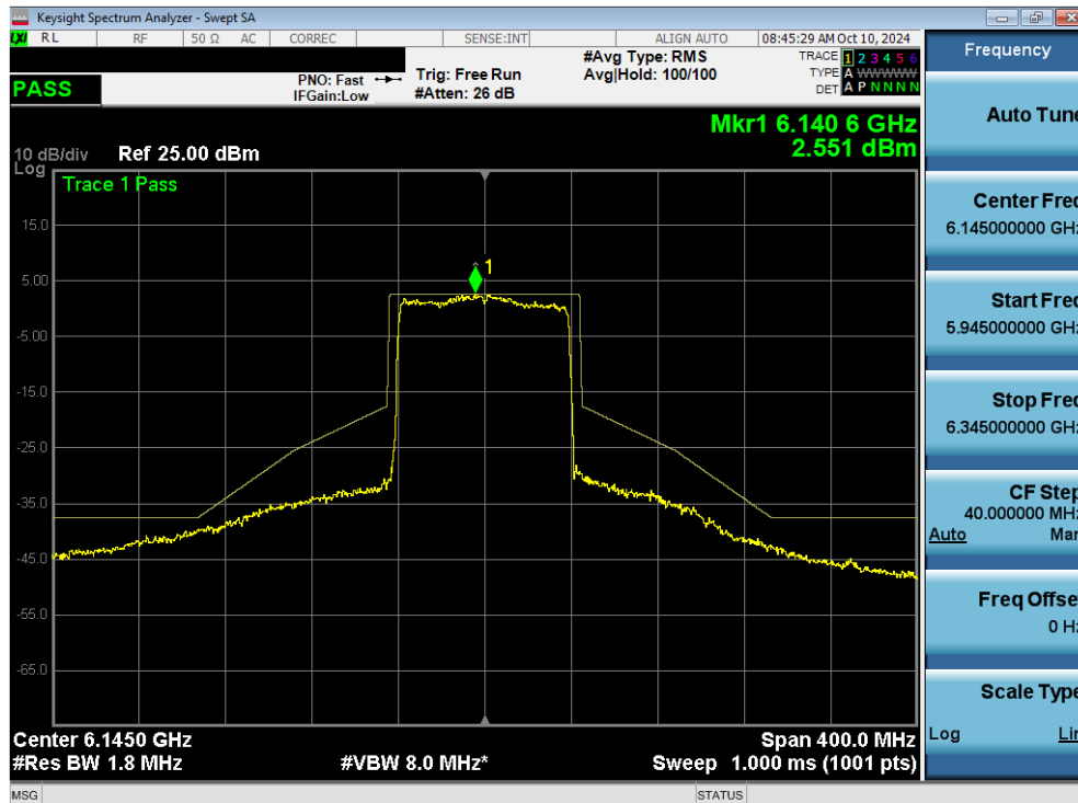
Plot 7-164. In Band Emissions Plot MIMO ANT2 (80MHz 802.11ax/be (Full Tones) (UNII Band 5) – Ch. 39) - SP
