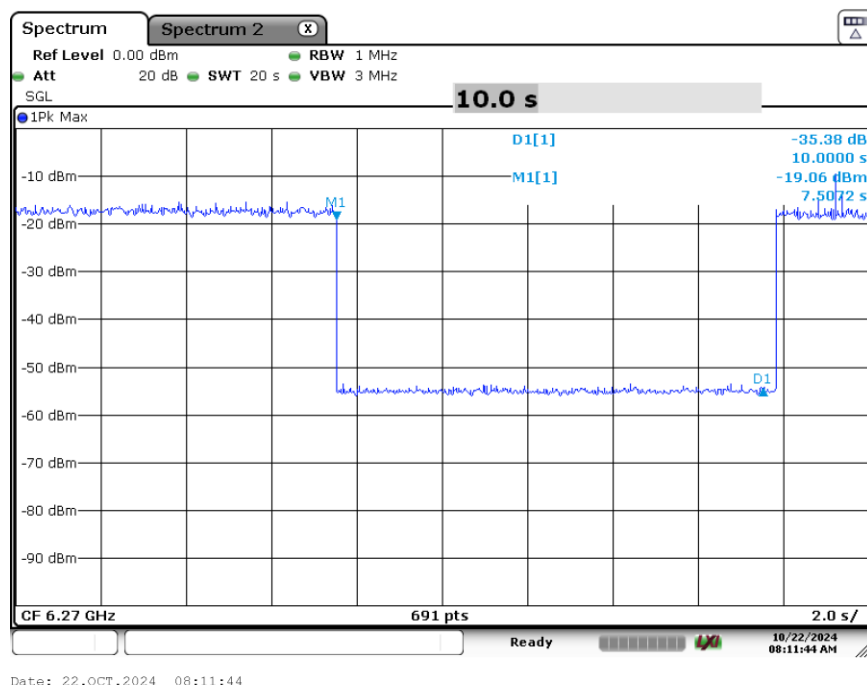
Plot 7-173. Contention Based Protocol Timing Plot (320MHz (UNII Band 6) – Ch. 95 Low)
