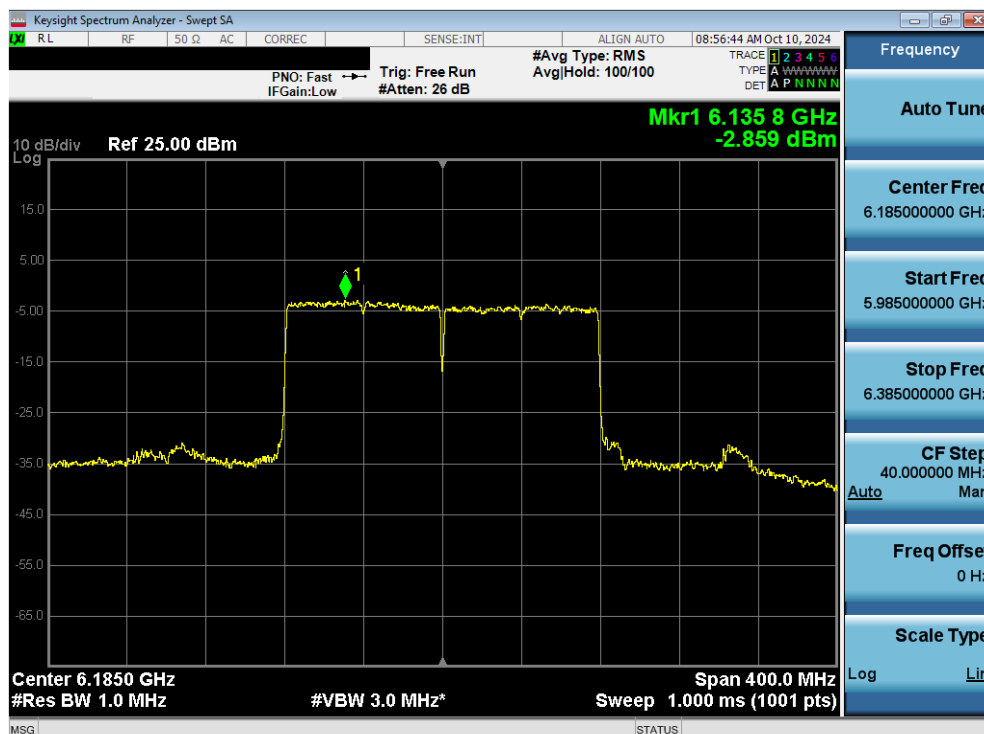
Plot 7-109. Power Spectral Density Plot MIMO ANT2 (160MHz 802.11ax/be (Full Tones) (UNII Band 5) – Ch. 47) - SP
