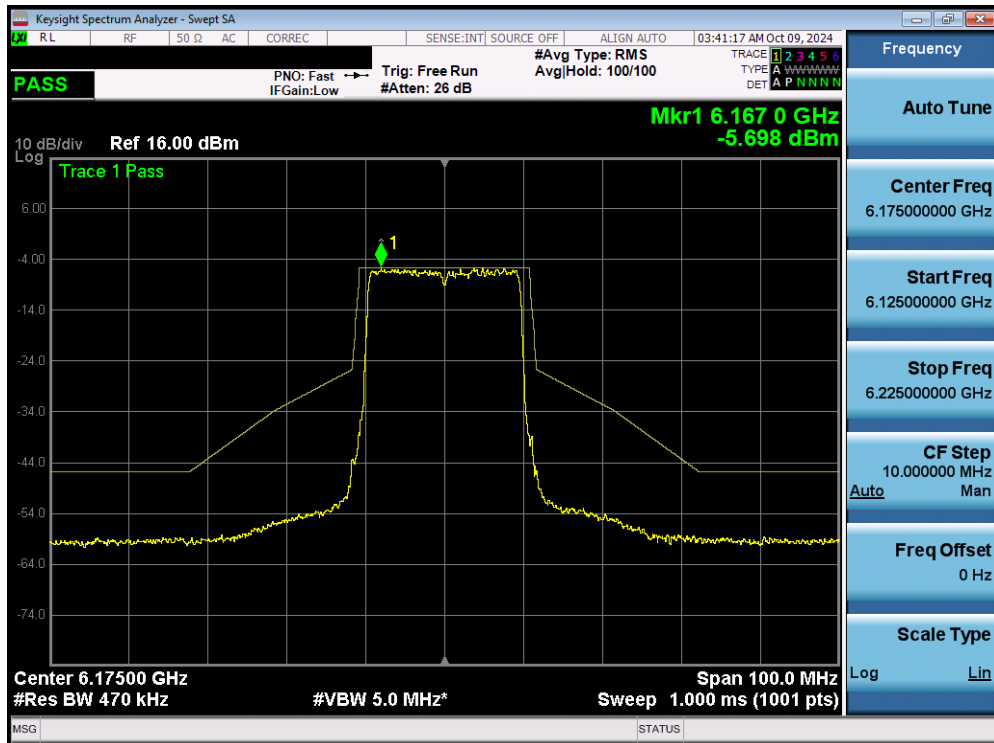
Plot 7-129. In Band Emissions Plot MIMO ANT1 (20MHz 802.11ax/be (Full Tones) (UNII Band 5) – Ch. 45) - LPI
