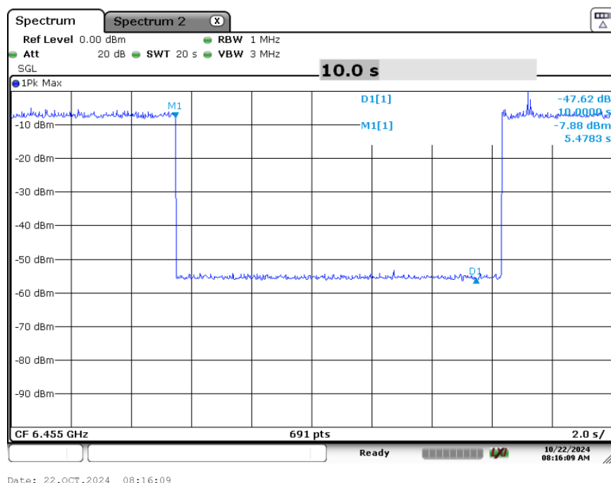
Plot 7-172. Contention Based Protocol Timing Plot (20MHz (UNII Band 6) – Ch. 101)
