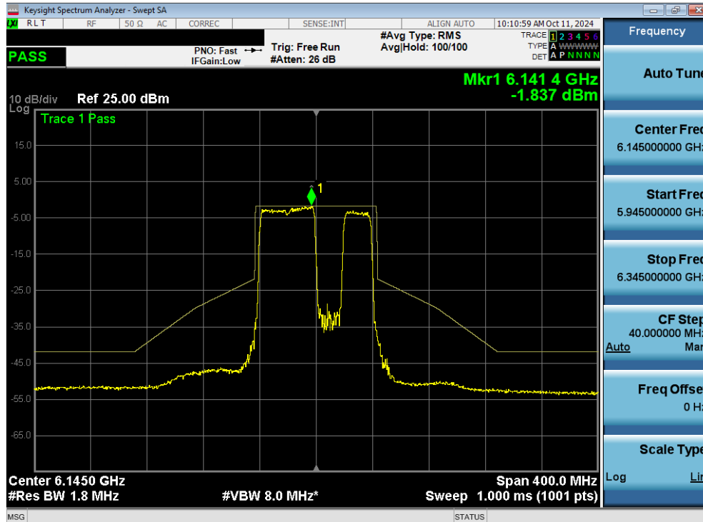
Plot 7-145. In Band Emissions Plot MIMO ANT2 (80MHz 802.11be (484+242 Tones) (UNII Band 5) – Ch. 39) (484+242 Tones) LPI
