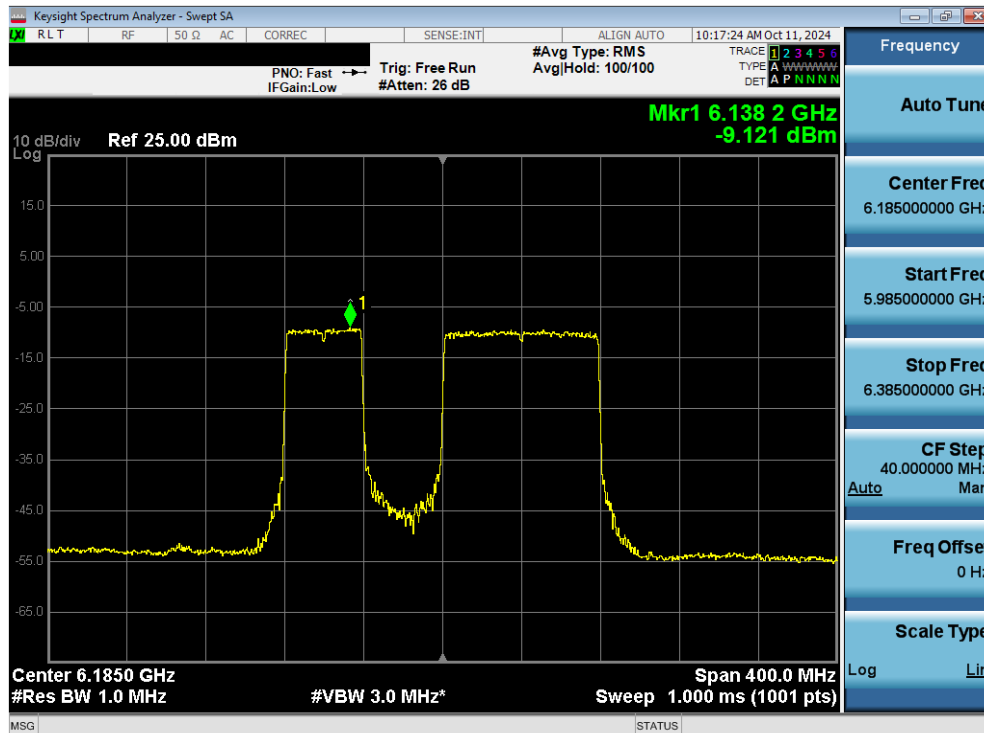
Plot 7-90. Power Spectral Density Plot MIMO ANT2 (160MHz 802.11be (996+484 Tones) (UNII Band 5) – Ch. 47) LPI
