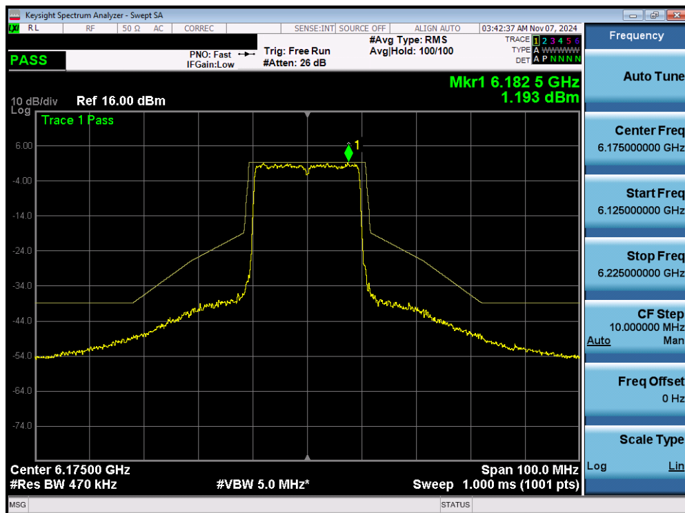
Plot 7-134. In Band Emissions Plot MIMO ANT1 (20MHz 802.11ax/be (Full Tones) (UNII Band 5) – Ch. 45) - SP
