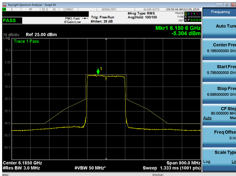
Plot 7-160. In Band Emissions Plot MIMO ANT2 (160MHz 802.11ax/be (Full Tones) (UNII Band 5) – Ch. 47) - LPI
