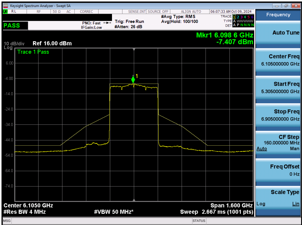
Plot 7-133. In Band Emissions Plot MIMO ANT1 (320MHz 802.11be (Full Tones) (UNII Band 5) – Ch. 31) - LPI
