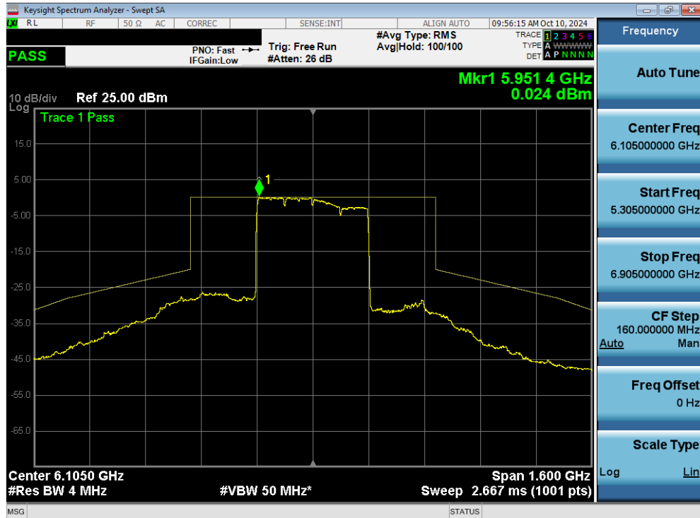
Plot 7-166. In Band Emissions Plot MIMO ANT2 (320MHz 802.11be (Full Tones) (UNII Band 5) – Ch. 31) - SP
