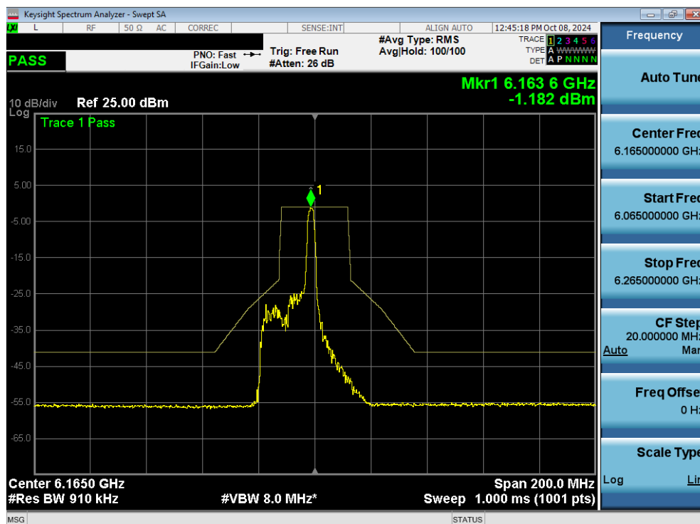
Plot 7-140. In Band Emissions Plot MIMO ANT2 (40MHz 802.11ax/be (26 Tones) (UNII Band 5) – Ch. 43) - LPI
