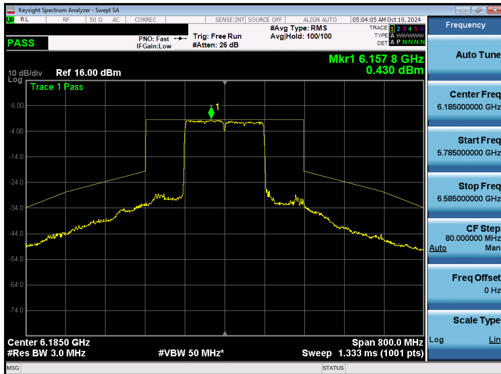
Plot 7-137. In Band Emissions Plot MIMO ANT1 (160MHz 802.11ax/be (Full Tones) (UNII Band 5) – Ch. 47) - SP
