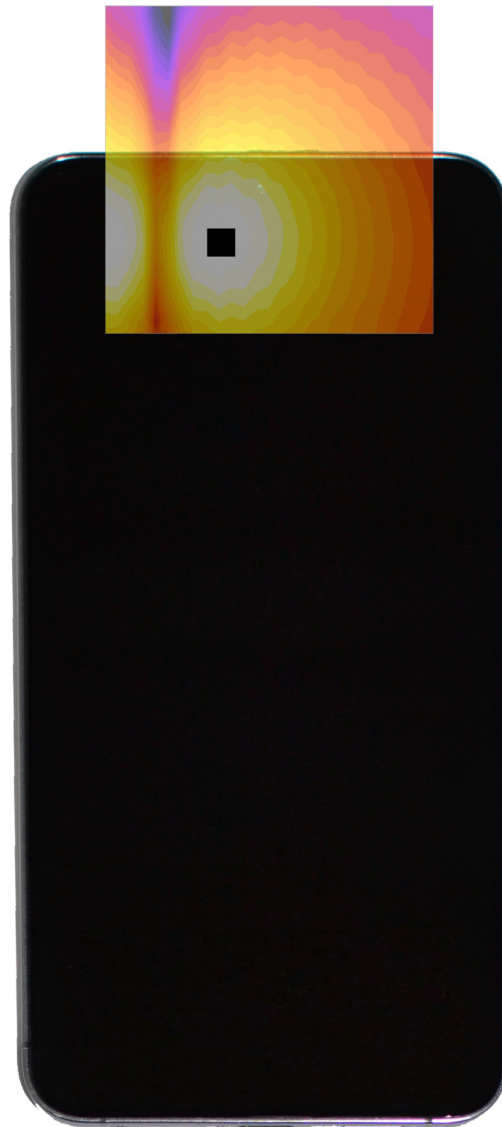
Figure 18-5 T-Coil Scan Overlay Magnetic Field Distributions
