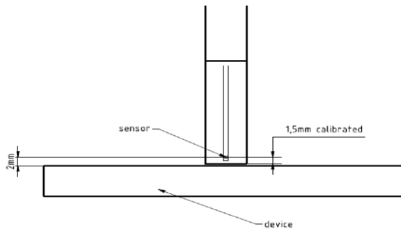
Figure C-2 EUMmWVx Probe
