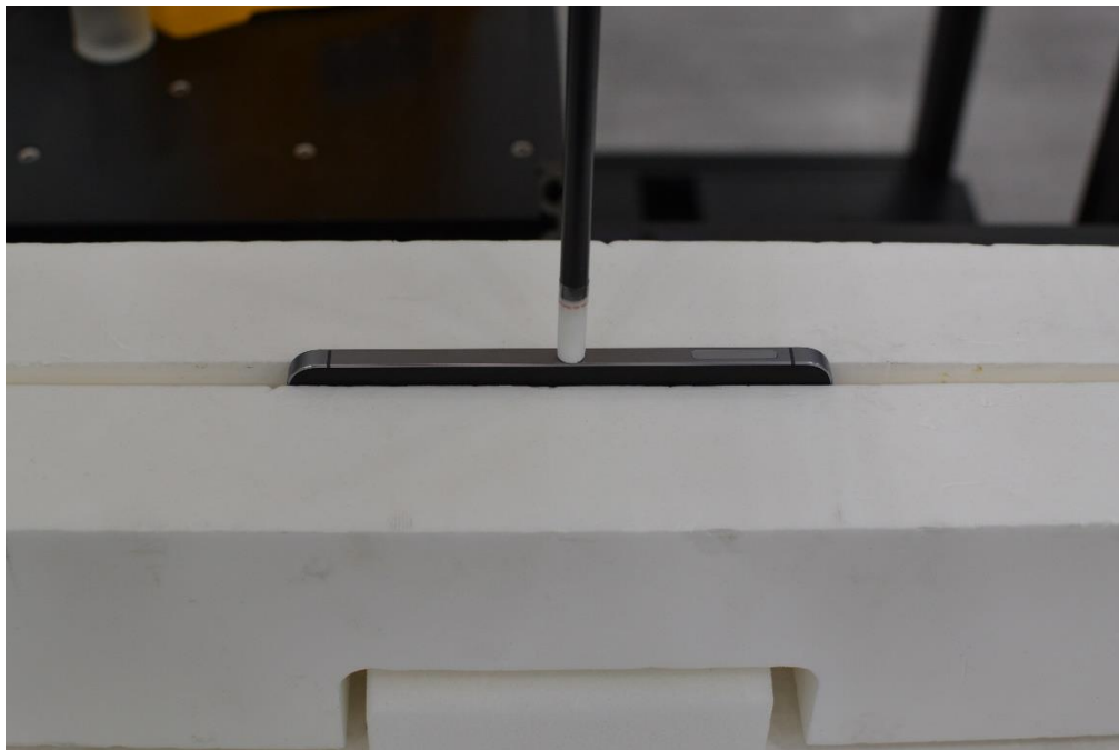
Near Field Power Density Test Setup Photo 2 – Left Side at 2 mm
