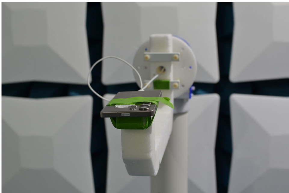
Figure 2. Test Setup – X Down Position – >18GHz
