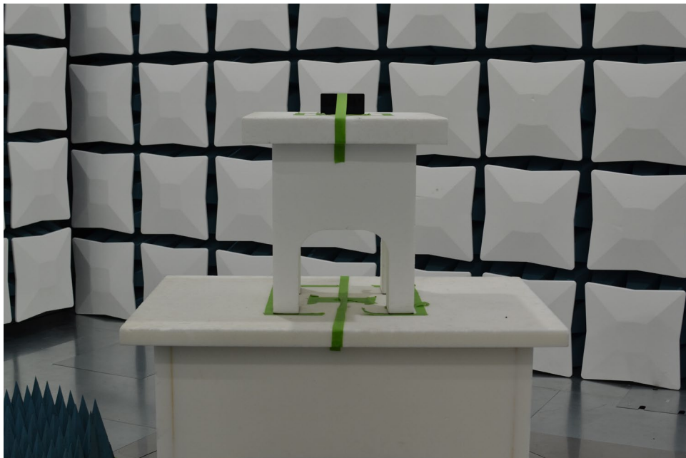
Figure 6. Test Setup – Y Position – 1GHz-40GHz
