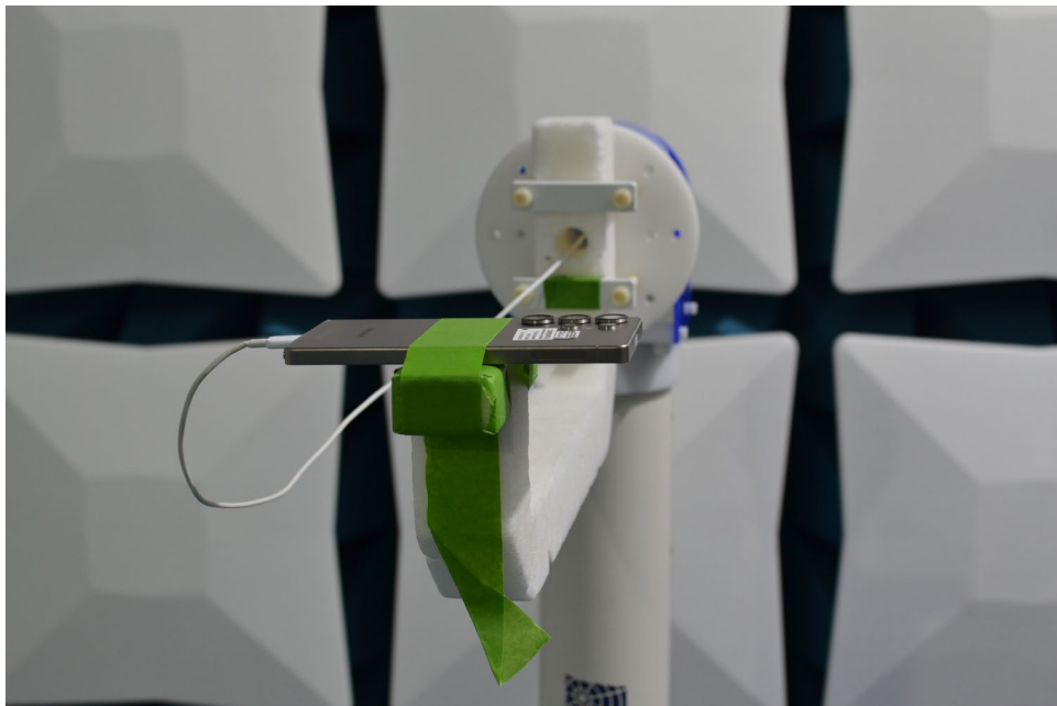
Figure 4. Test Setup – Y Down Position – >18GHz
