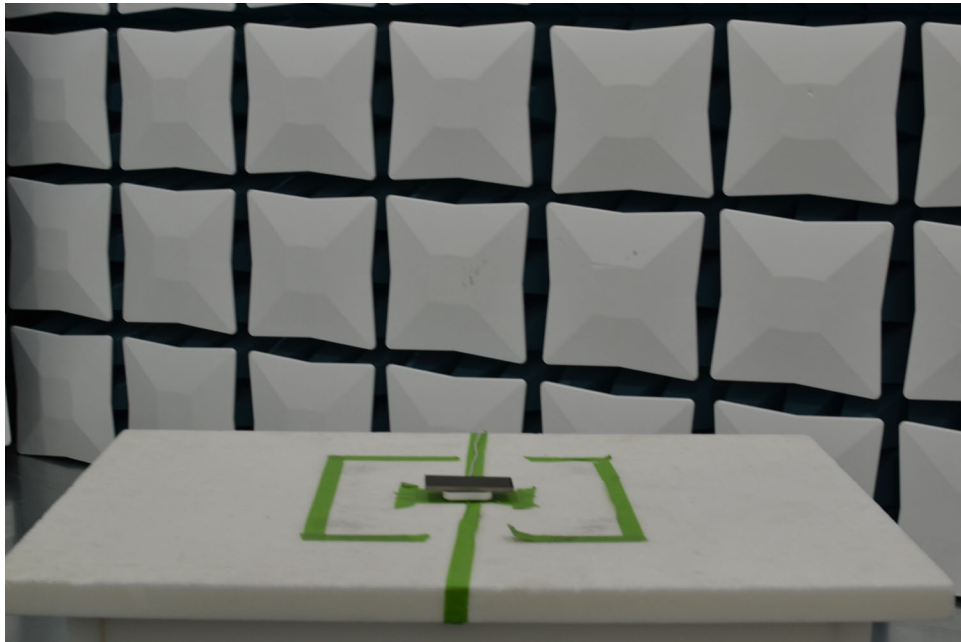
Figure 14. Test Setup – Wireless Charging Pad – 30MHz-1GHz
