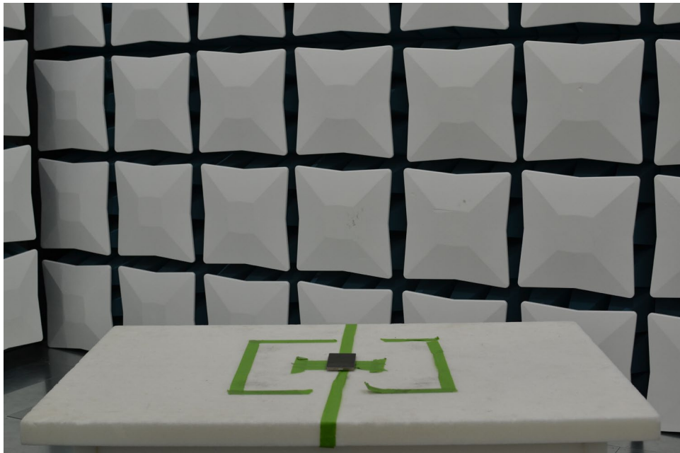
Figure 10. Test Setup – X Position – 30MHz-1GHz
