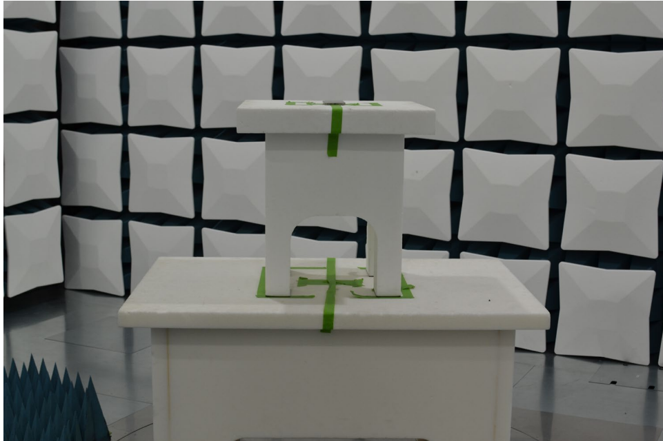
Figure 5. Test Setup – X Position – 1GHz-40GHz
