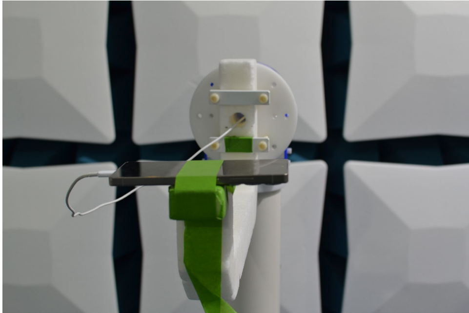
Figure 3. Test Setup – Y Position – >18GHz
