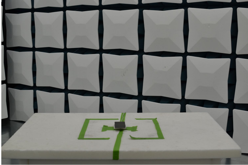
Figure 13. Test Setup – Wireless Charging Pad – 30MHz-1GHz
