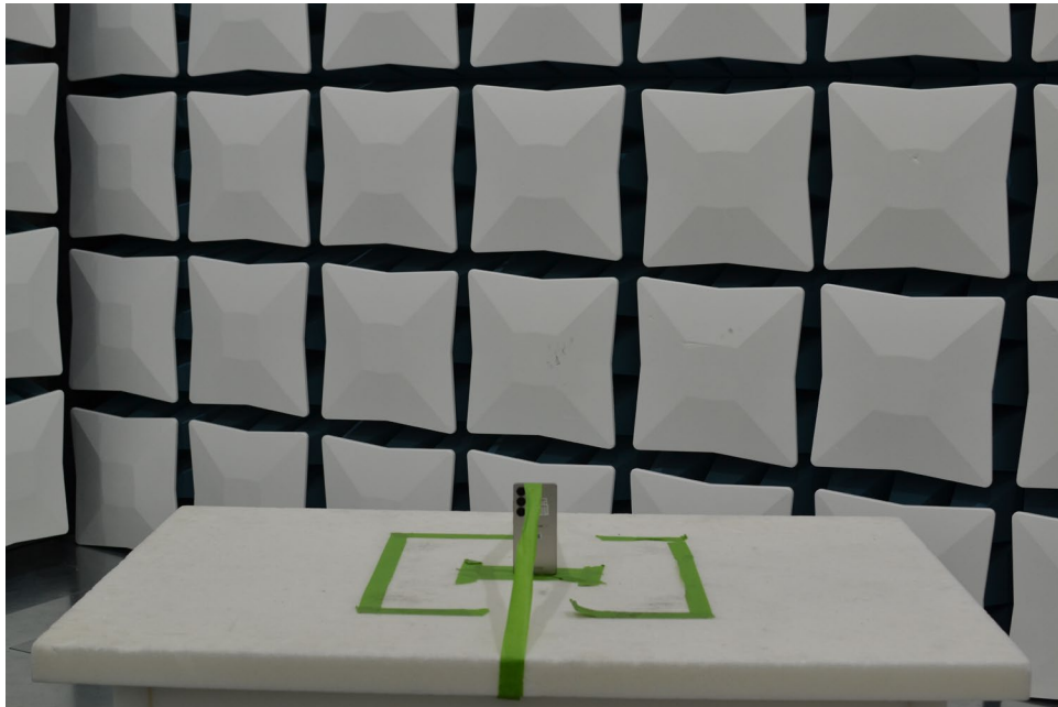
Figure 12. Test Setup – Z Position – 30MHz-1GHz
