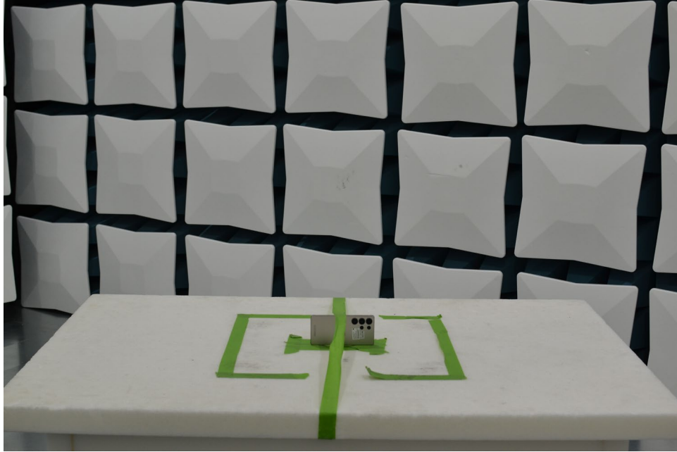
Figure 11. Test Setup – Y Position – 30MHz-1GHz
