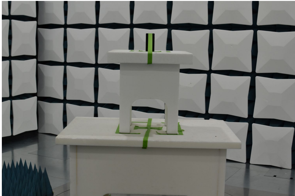
Figure 7. Test Setup – Z Position – 1GHz-40GHz
