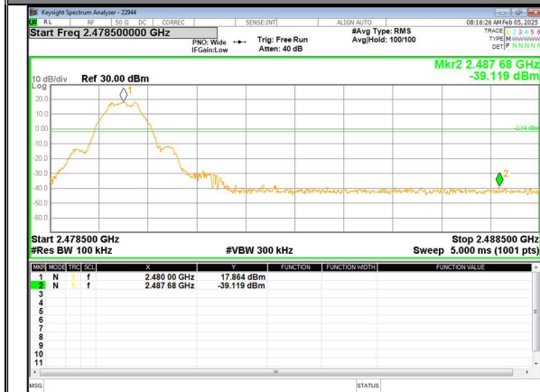
HIGH(39) CHANNEL BANDEDGE
