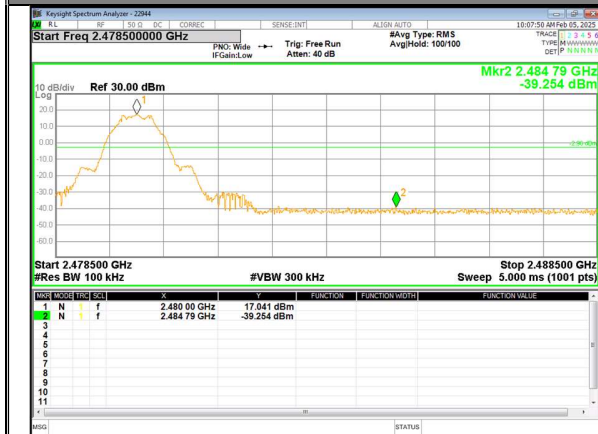
HIGH(39) CHANNEL BANDEGE
