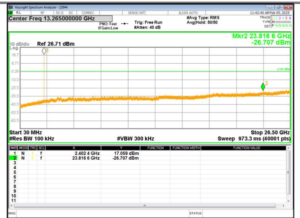
OUT-OF-BAND LOW(37) CHANNEL
