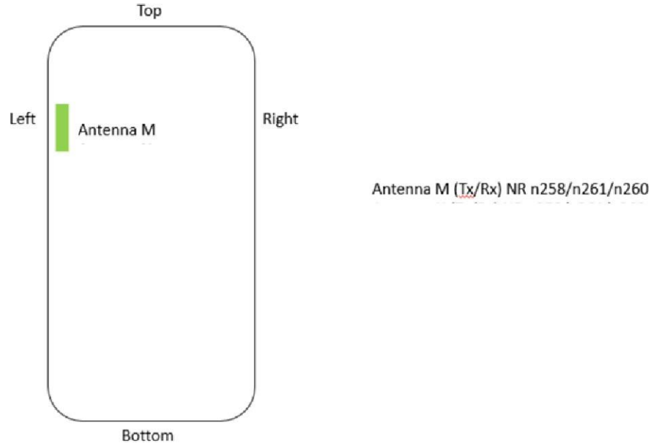
Figure 1: Location of mmW antenna module looking from Front of the DUT
