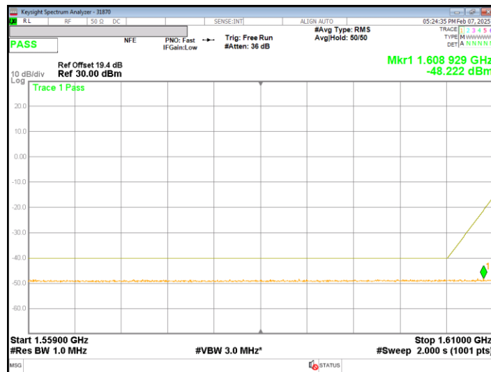
VERTICAL QPSK / 15 kHz / 6SC6 / Mid channel
