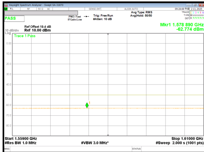
VERTICAL QPSK / 15 kHz / 6SC6 / High channel
