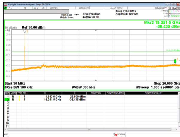
Mid channel 3.75 kHz SCS QPSK 1SC24
