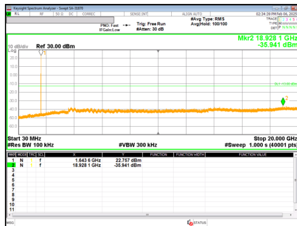
Mid channel 3.75 kHz SCS BPSK 1SC24
