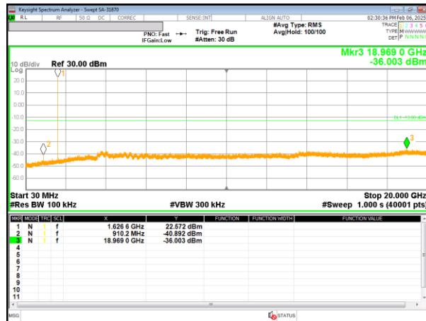
Low channel 3.75 kHz SCS BPSK 1SC24
