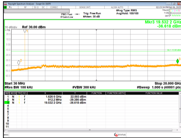
Low channel 3.75 kHz SCS QPSK 1SC24
