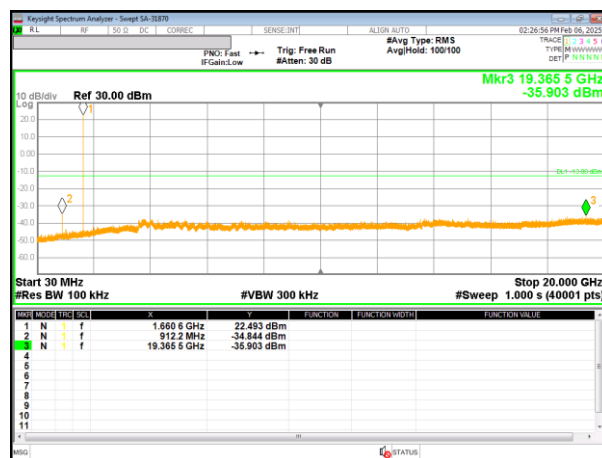
High channel 3.75 kHz SCS QPSK 1SC24
