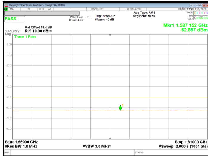
HORIZONTAL QPSK / 15 kHz / 6SC6 / High channel
