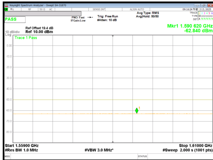
HORIZONTAL QPSK / 15 kHz / 6SC6 / Mid channel
