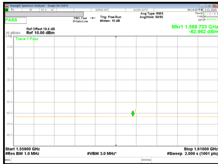
HORIZONTAL QPSK / 15 kHz / 6SC6 / Low channel
