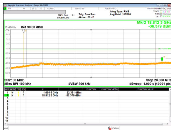
High channel 15 kHz SCS BPSK 1SC6
