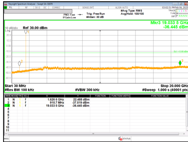
Low channel 15 kHz SCS BPSK 1SC6
