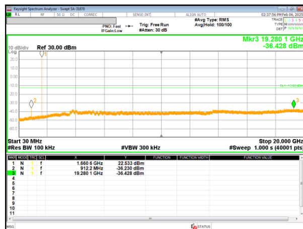
High channel 3.75 kHz SCS BPSK 1SC24
