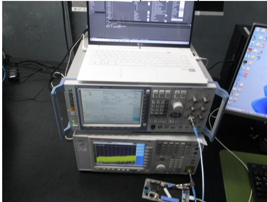
LICENSED BAND TEST PHOTO (LTE, NB NTN)
