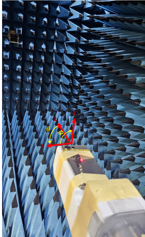
Figure 1: Geometry for SM-S938B for Radiation patterns.
