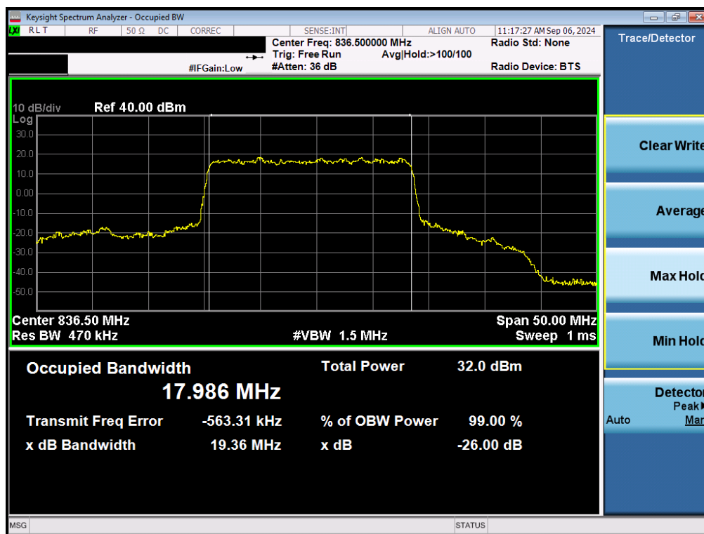
Plot 7-36. Occupied Bandwidth Plot (NR Band n5 - 20MHz \pi/2 BPSK - Full RB - Ant2)
