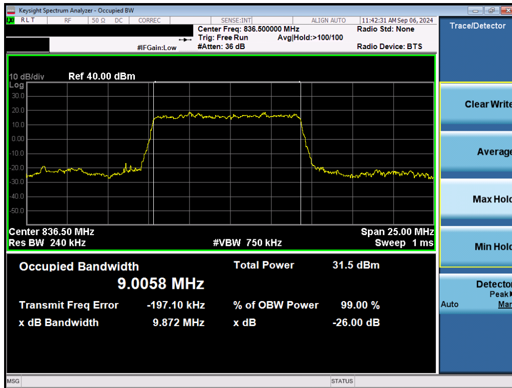
Plot 7-42. Occupied Bandwidth Plot (NR Band n5 - 10MHz \pi/2 BPSK - Full RB - Ant2)
