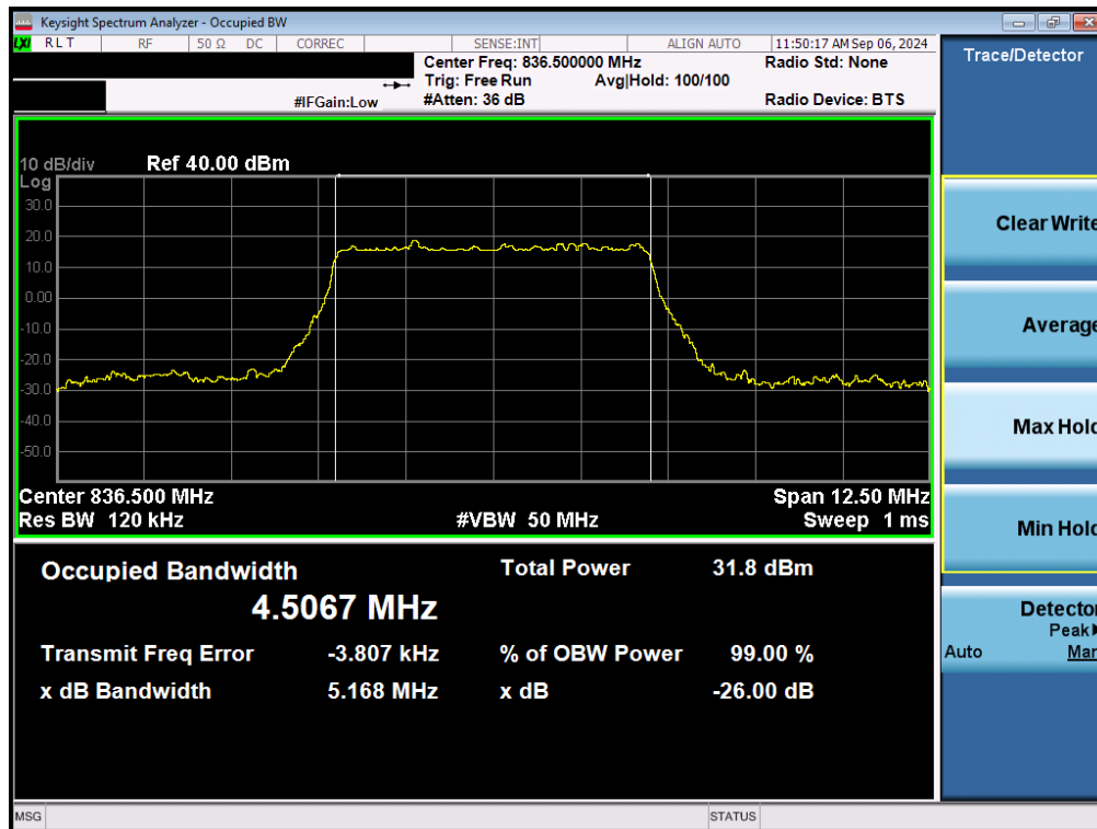
Plot 7-45. Occupied Bandwidth Plot (NR Band n5 - 5MHz \pi/2 BPSK - Full RB - Ant2)
