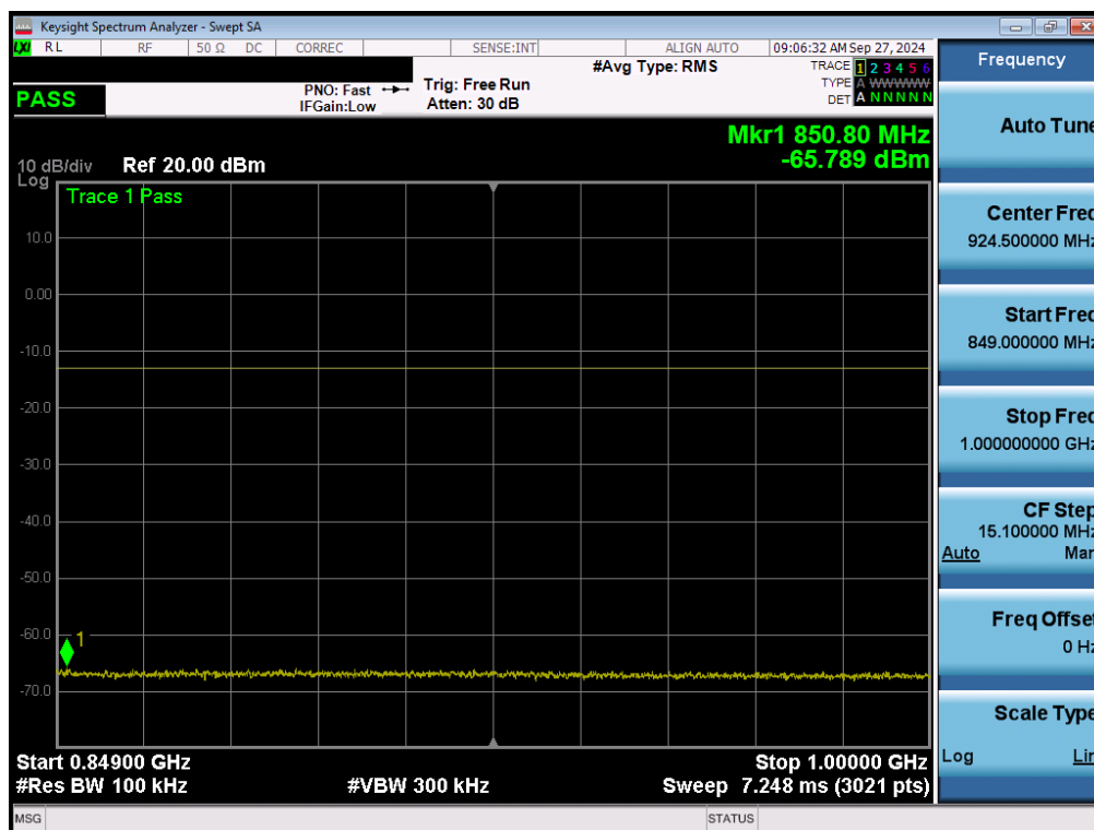
Plot 7-52. Conducted Spurious Plot (WCDMA Low – Ant1)
