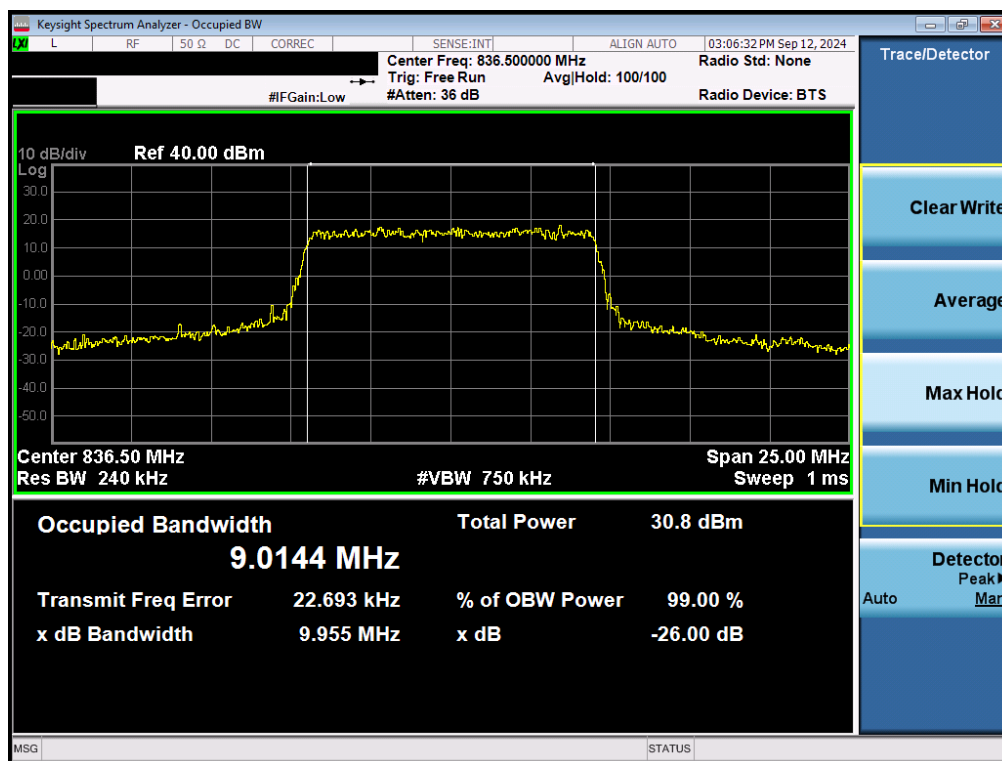
Plot 7-5. Occupied Bandwidth Plot (LTE Band 5 - 10MHz QPSK - Full RB - Ant1)
