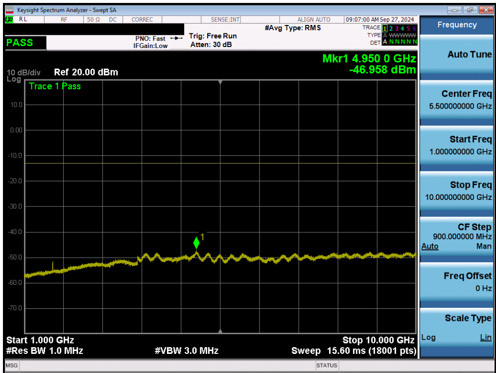
Plot 7-53. Conducted Spurious Plot (WCDMA Low – Ant1)
