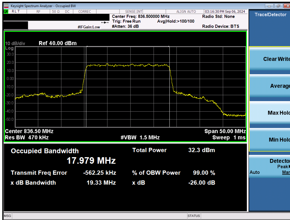
Plot 7-13. Occupied Bandwidth Plot (NR Band n5 - 20MHz \pi/2 BPSK - Full RB - Ant1)
