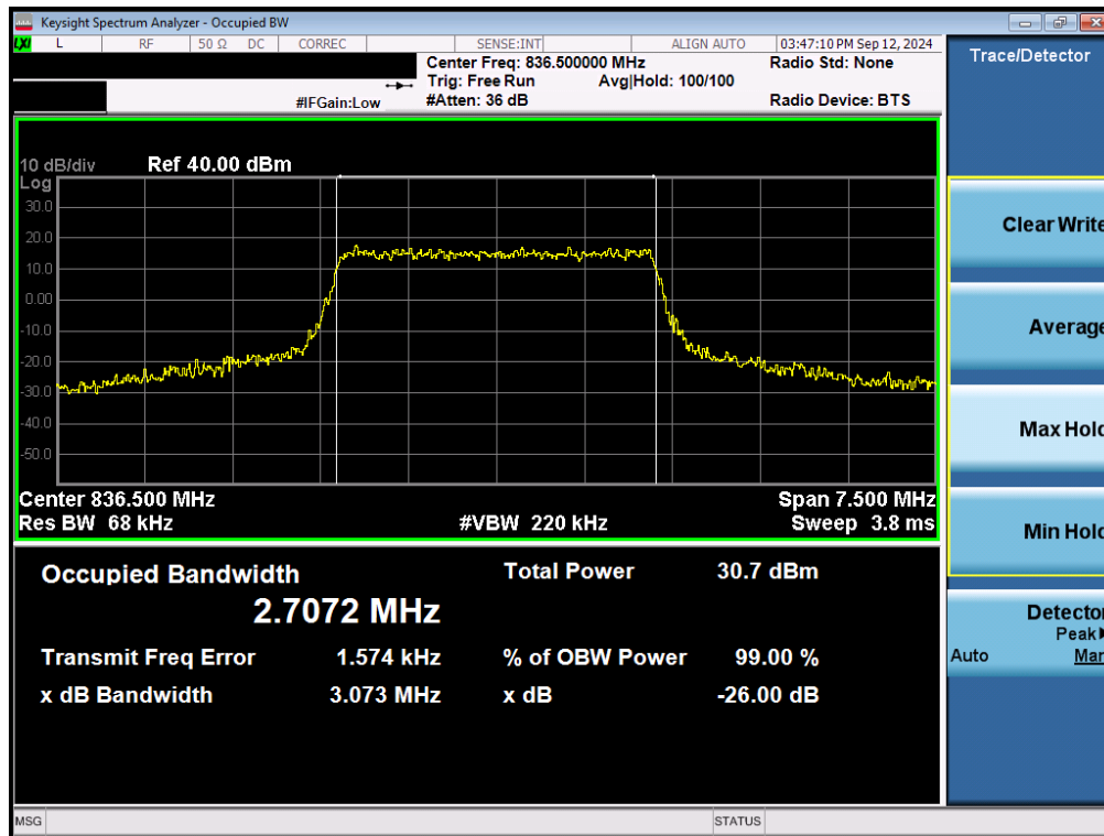
Plot 7-32. Occupied Bandwidth Plot (LTE Band 5 - 3MHz QPSK - Full RB - Ant2)
