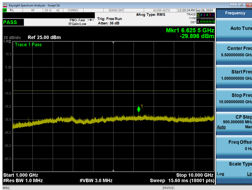
Plot 7-50. Conducted Spurious Plot (GPRS Ch. 251 – Ant1)
