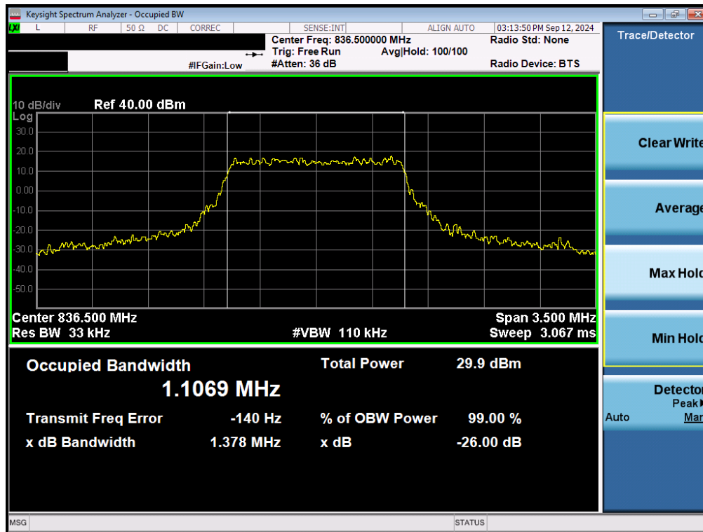
Plot 7-11. Occupied Bandwidth Plot (LTE Band 5 - 1.4MHz QPSK - Full RB - Ant1)
