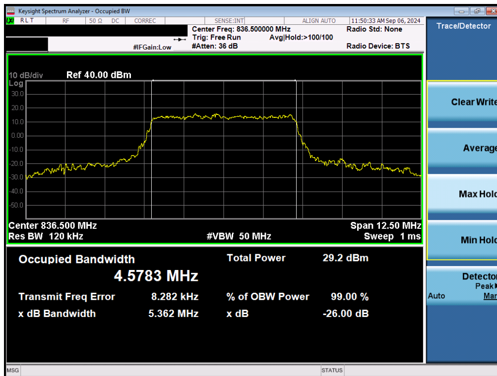
Plot 7-47. Occupied Bandwidth Plot (NR Band n5 - 5MHz 16-QAM - Full RB - ABnt2)
