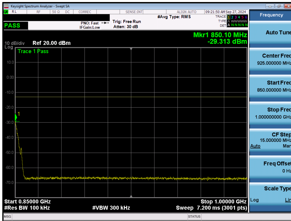
Plot 7-64. Conducted Spurious Plot (WCDMA Ch. 4233 – Ant2)
