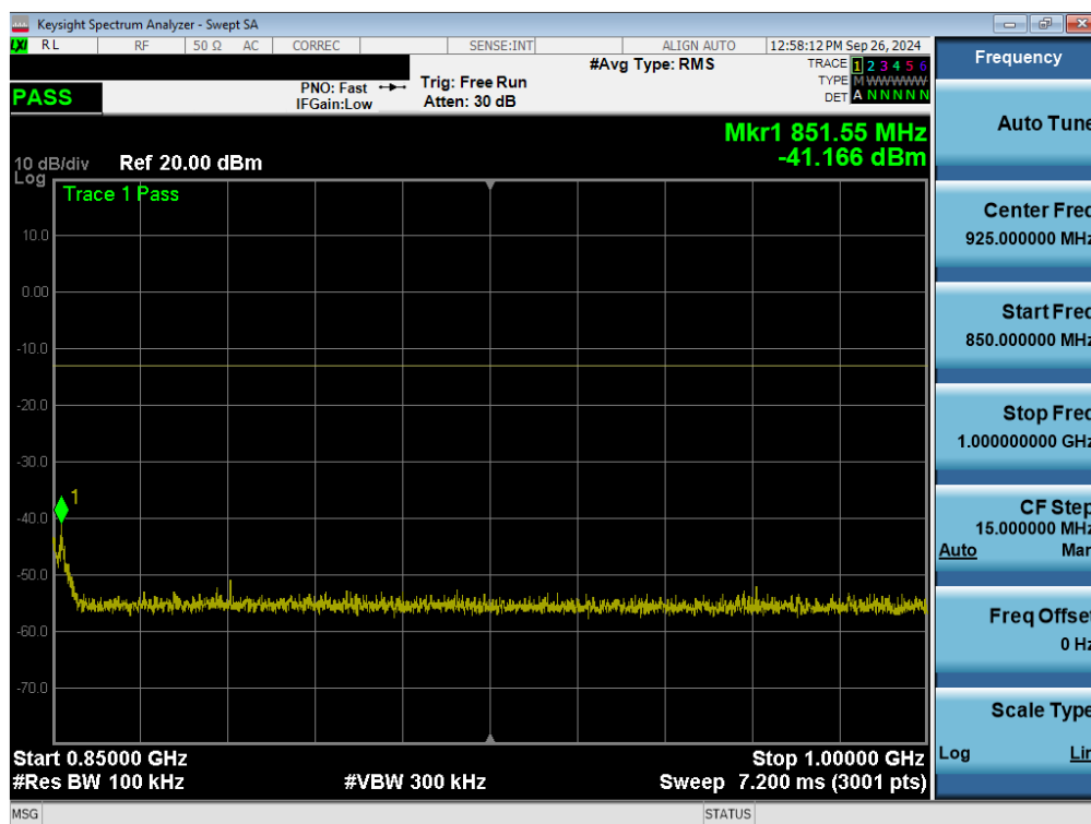
Plot 7-61. Conducted Spurious Plot (GPRS Ch. 251 – Ant2)
