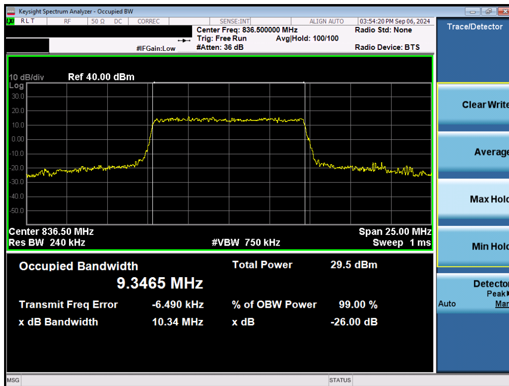
Plot 7-20. Occupied Bandwidth Plot (NR Band n5 - 10MHz QPSK - Full RB - Ant1)
