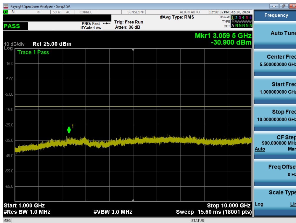
Plot 7-62. Conducted Spurious Plot (GPRS Ch. 251 – Ant2)
