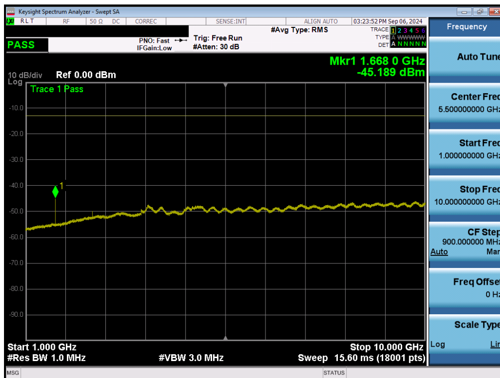
Plot 7-59. Conducted Spurious Plot (NR Band n5 - 20.0MHz - 1 RB - Low Channel - Ant1)
