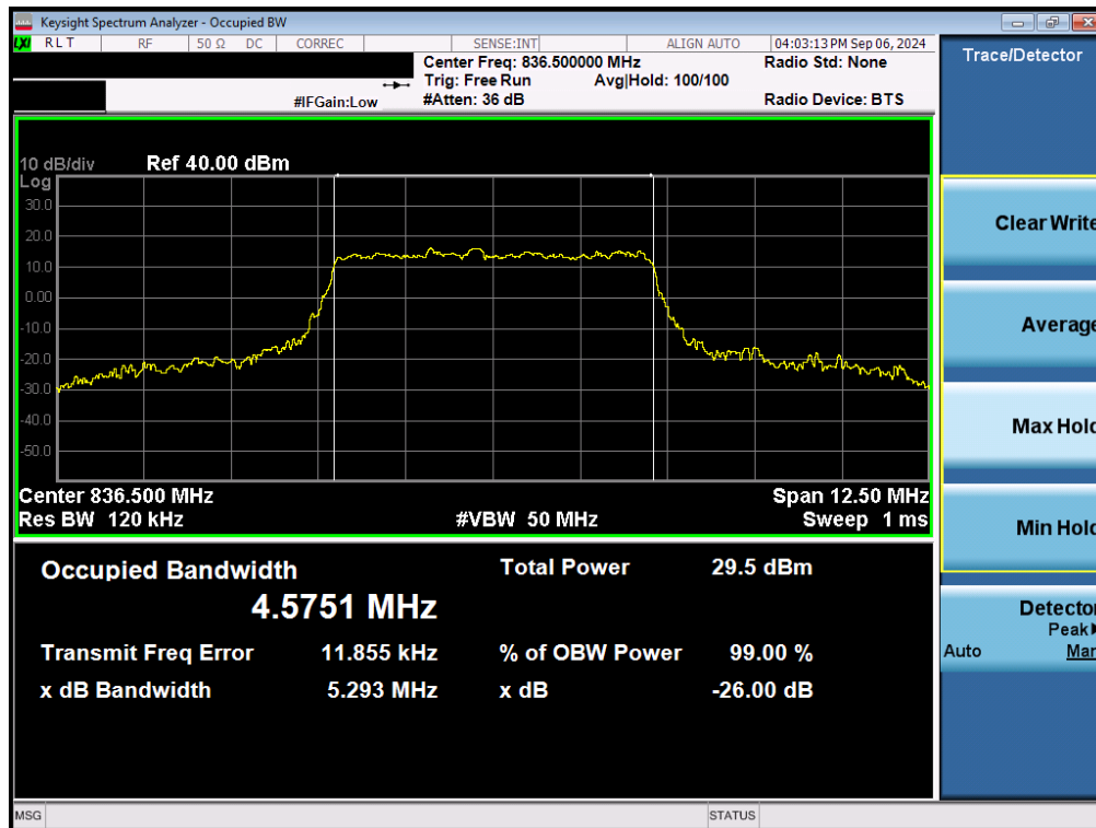
Plot 7-24. Occupied Bandwidth Plot (NR Band n5 - 5MHz 16-QAM - Full RB - Ant1)
