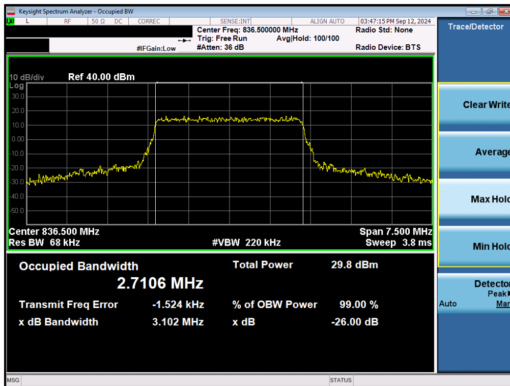
Plot 7-33. Occupied Bandwidth Plot (LTE Band 5 - 3MHz 16-QAM - Full RB - Ant2)
