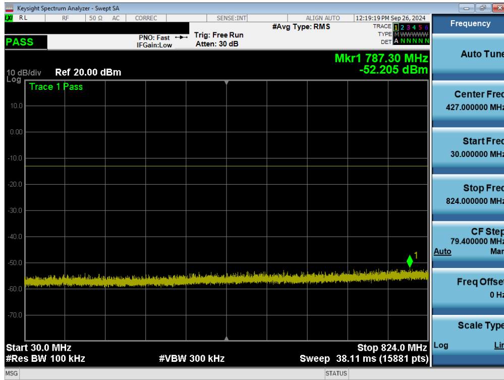
Plot 7-48. Conducted Spurious Plot (GPRS Ch. 251 – Ant1)
