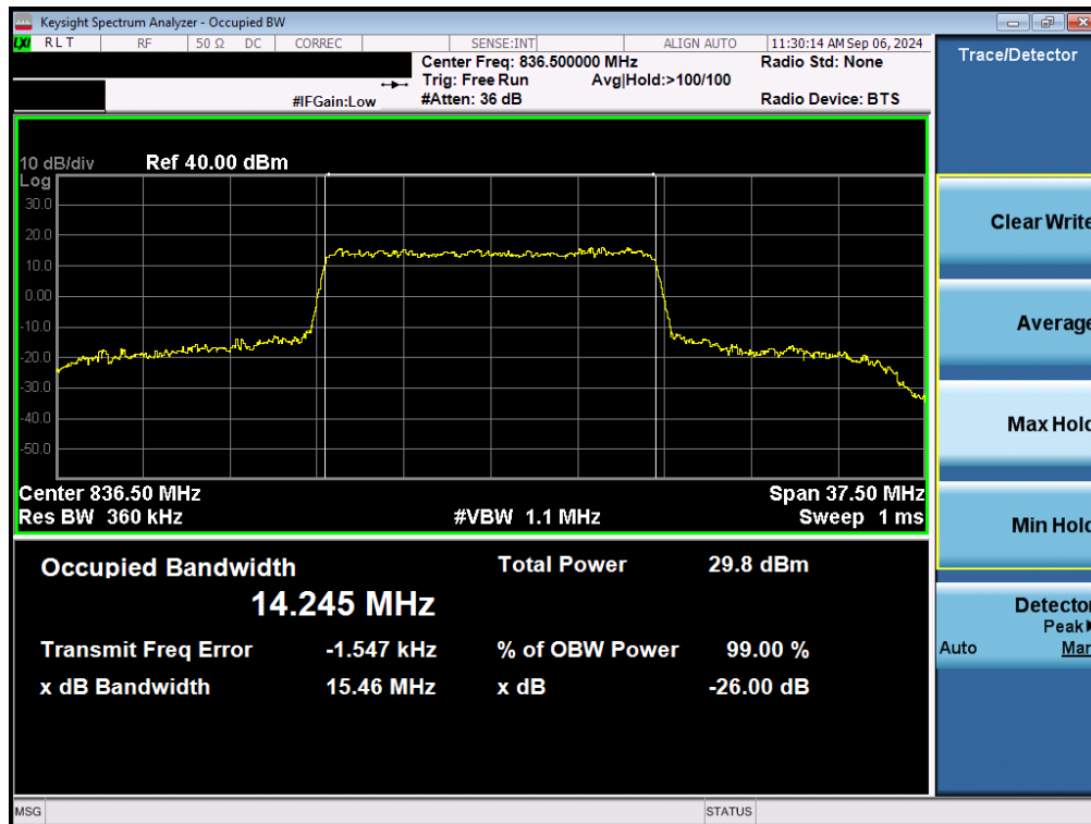
Plot 7-41. Occupied Bandwidth Plot (NR Band n5 - 15MHz 16-QAM - Full RB - Ant2)
