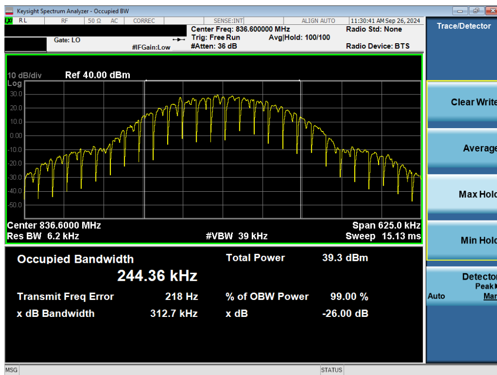
Plot 7-2. Occupied Bandwidth Plot (GPRS, Ch. 190 – Ant1)
