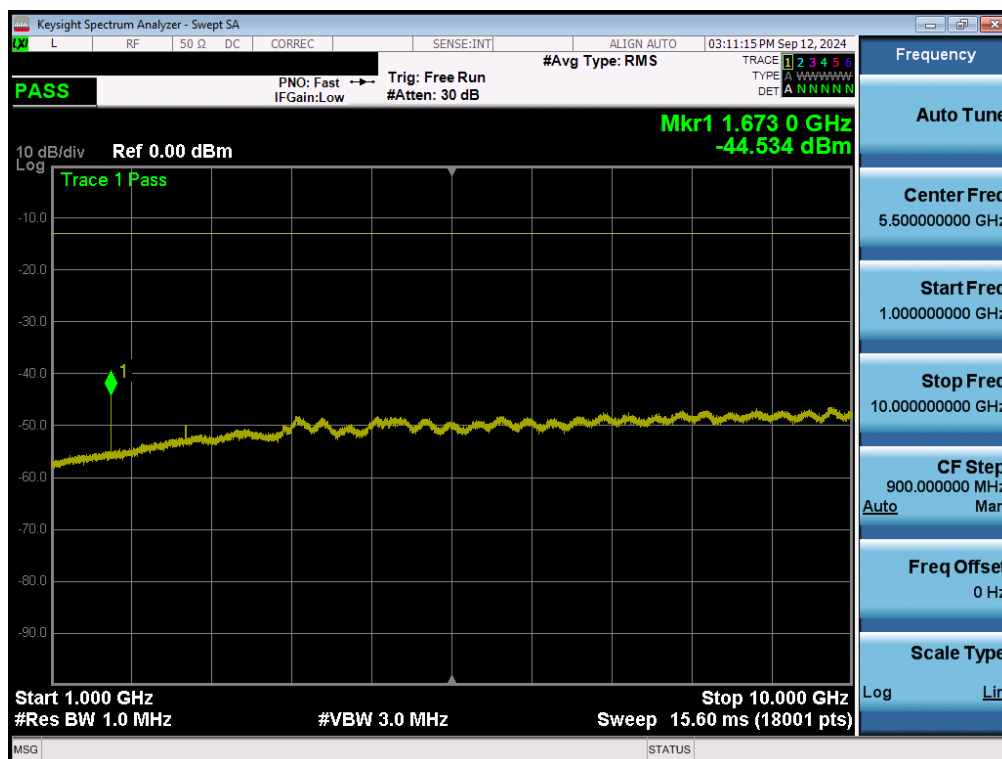
Plot 7-56. Conducted Spurious Plot (LTE Band 5 - 10MHz QPSK - 1 RB - Mid Channel – Ant1)
