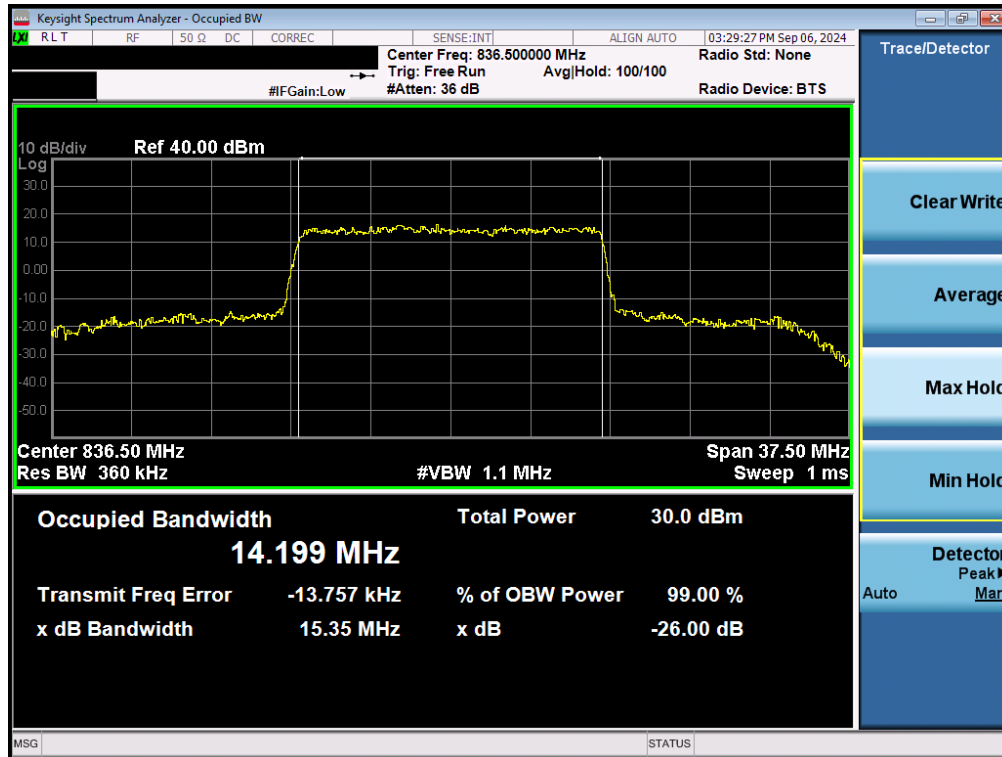
Plot 7-17. Occupied Bandwidth Plot (NR Band n5 - 15MHz QPSK - Full RB - Ant1)
