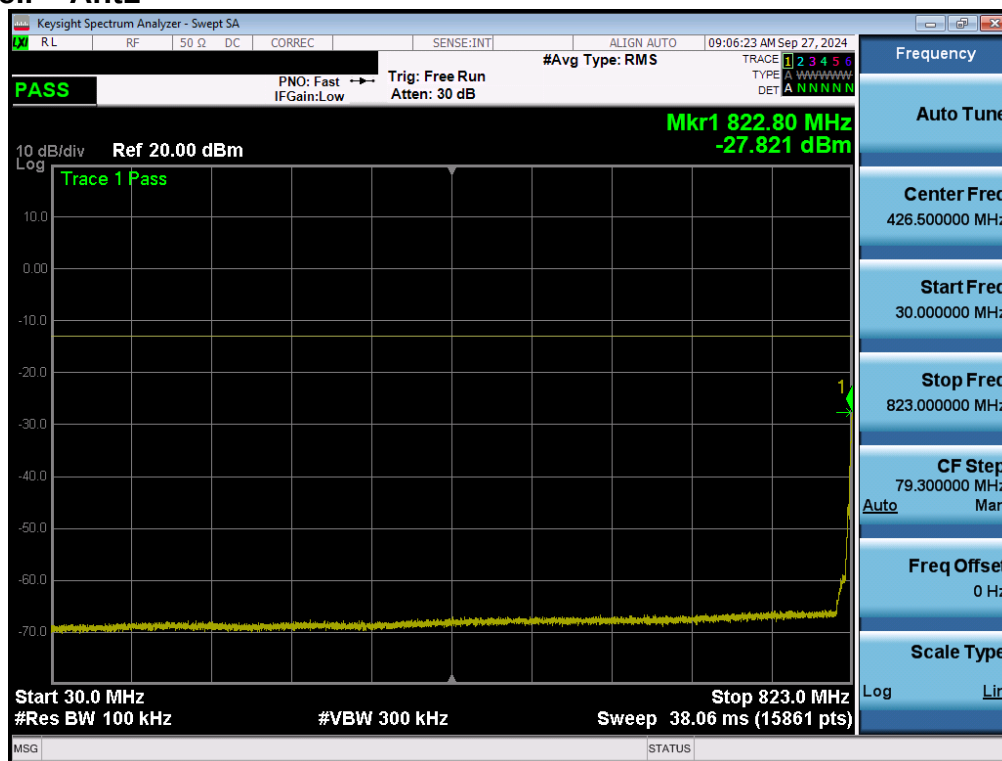
Plot 7-51. Conducted Spurious Plot (WCDMA Low – Ant1)
