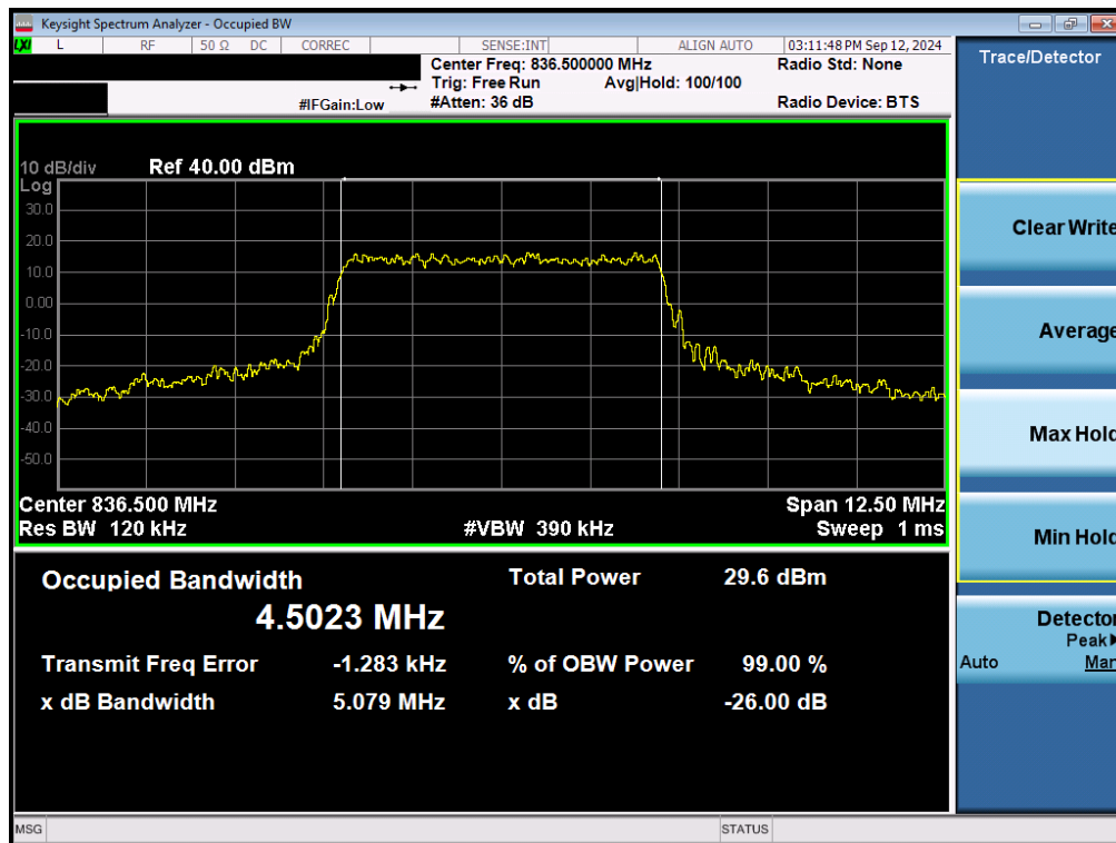
Plot 7-8. Occupied Bandwidth Plot (LTE Band 5 - 5MHz 16-QAM - Full RB - Ant1)
