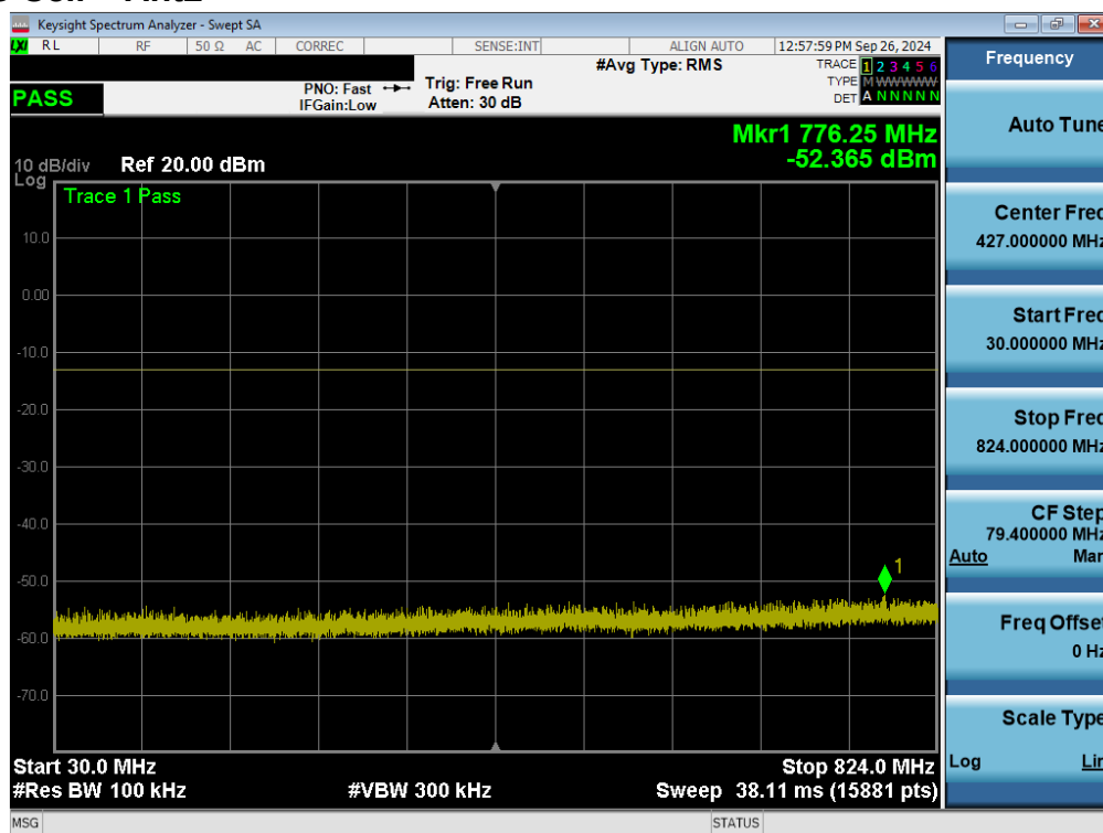
Plot 7-60. Conducted Spurious Plot (GPRS Ch. 251 – Ant2)
