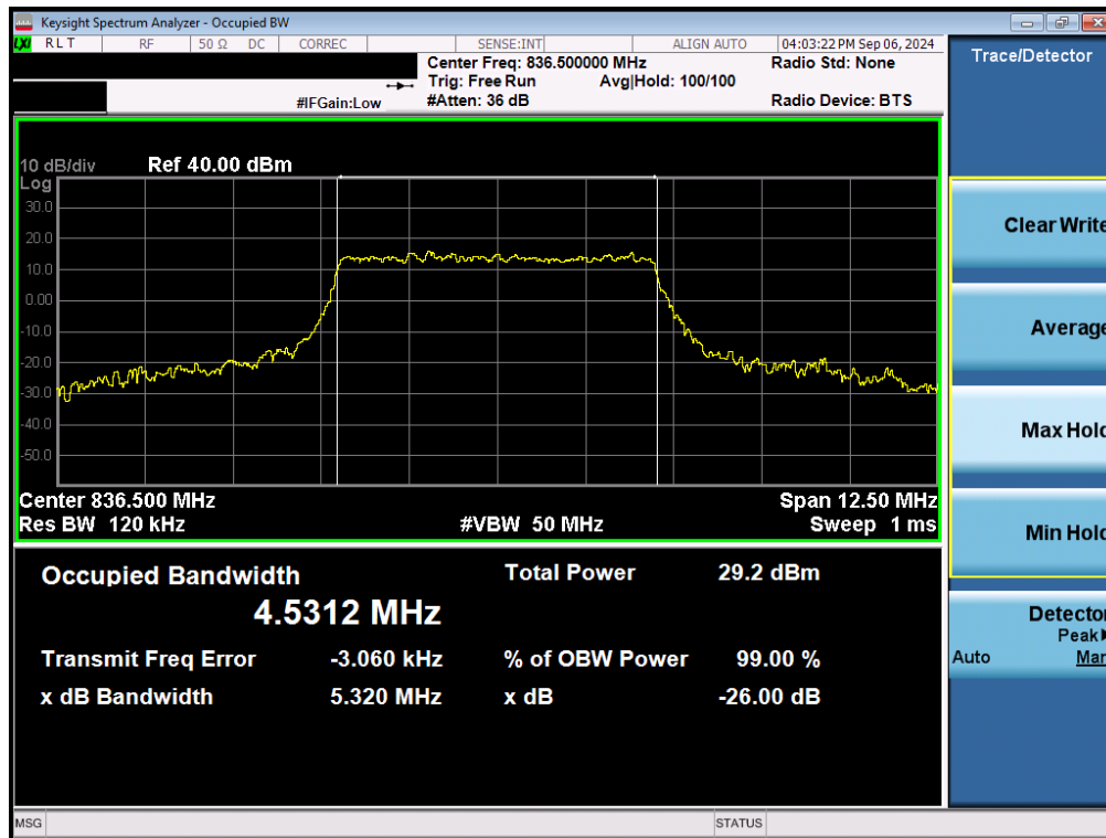
Plot 7-23. Occupied Bandwidth Plot (NR Band n5 - 5MHz QPSK - Full RB - Ant1)
