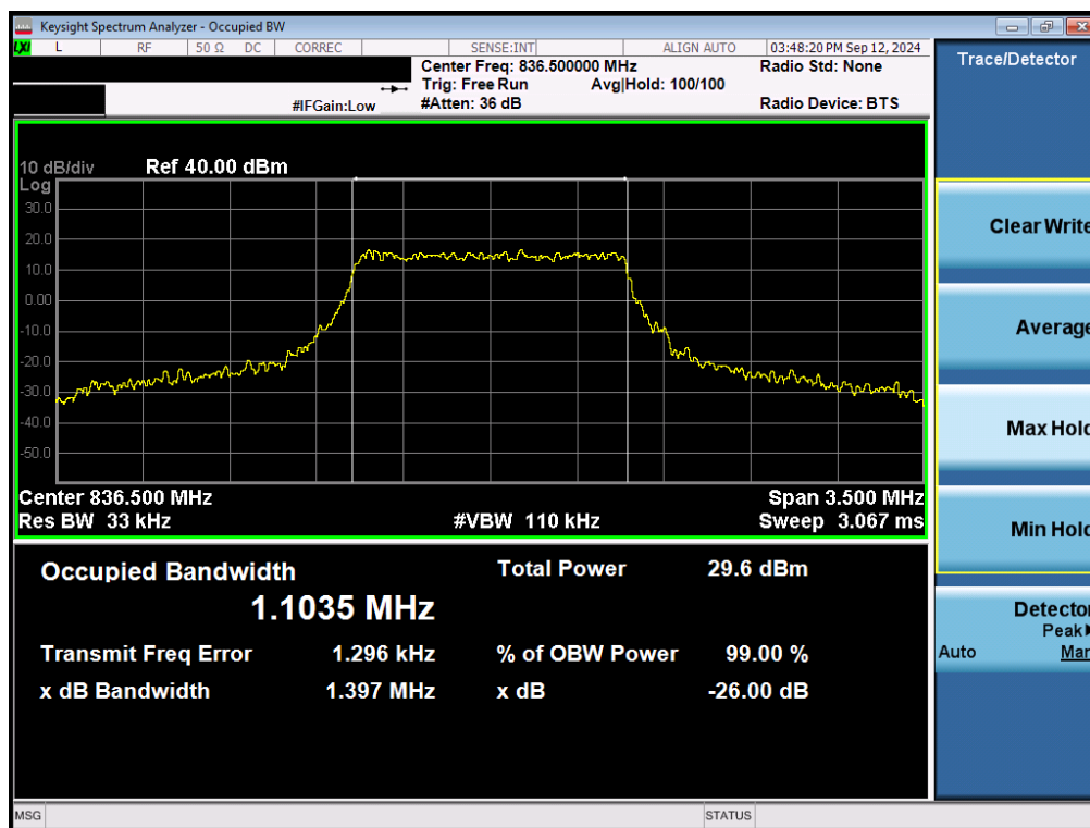
Plot 7-34. Occupied Bandwidth Plot (LTE Band 5 - 1.4MHz QPSK - Full RB - Ant2)
