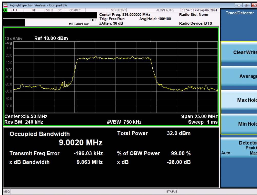
Plot 7-19. Occupied Bandwidth Plot (NR Band n5 - 10MHz \pi/2 BPSK - Full RB - Ant1)
