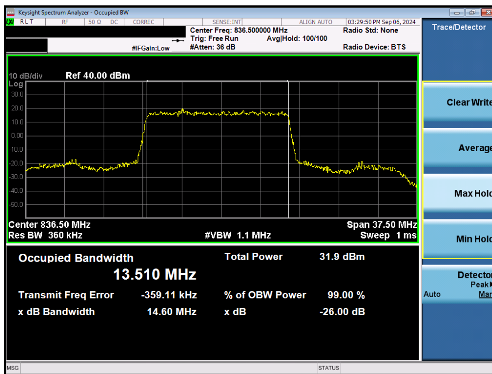
Plot 7-16. Occupied Bandwidth Plot (NR Band n5 - 15MHz \pi/2 BPSK - Full RB - Ant1)
