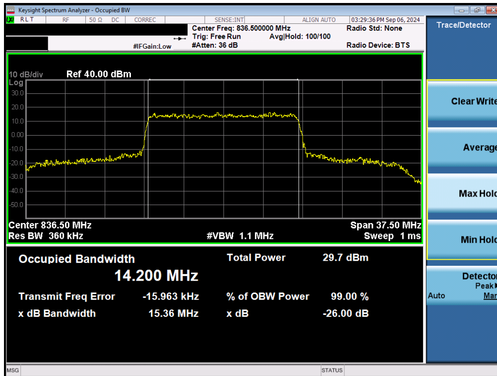
Plot 7-18. Occupied Bandwidth Plot (NR Band n5 - 15MHz 16-QAM - Full RB - Ant1)
