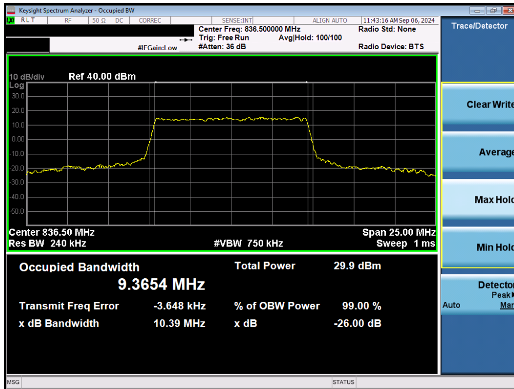
Plot 7-44. Occupied Bandwidth Plot (NR Band n5 - 10MHz 16-QAM - Full RB - Ant2)
