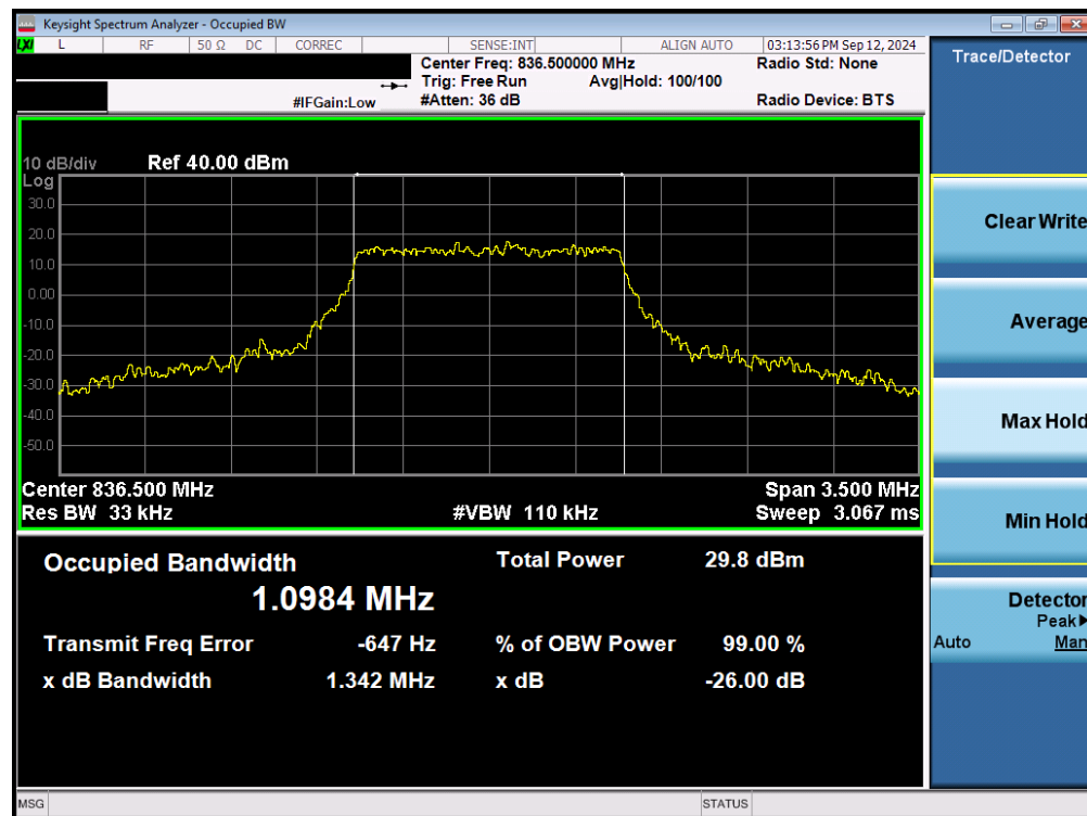
Plot 7-12. Occupied Bandwidth Plot (LTE Band 5 - 1.4MHz 16-QAM - Full RB - Ant1)
