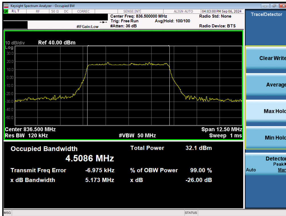
Plot 7-22. Occupied Bandwidth Plot (NR Band n5 - 5MHz \pi/2 BPSK - Full RB - Ant1)
