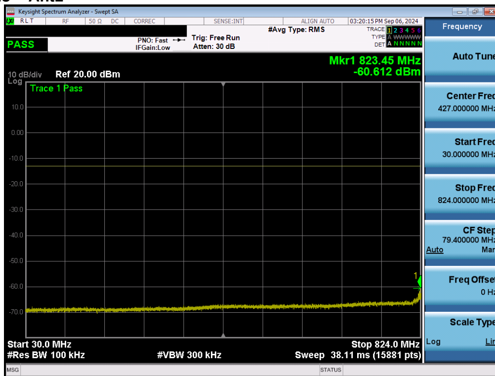
Plot 7-57. Conducted Spurious Plot (NR Band n5 - 20.0MHz - 1 RB - Low Channel - Ant1)
