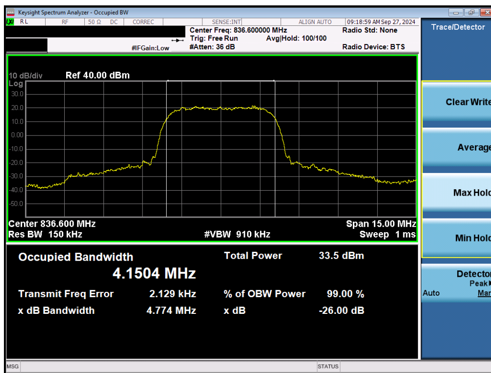
Plot 7-27. Occupied Bandwidth Plot (WCDMA, Ch. 4183 – Ant2)
