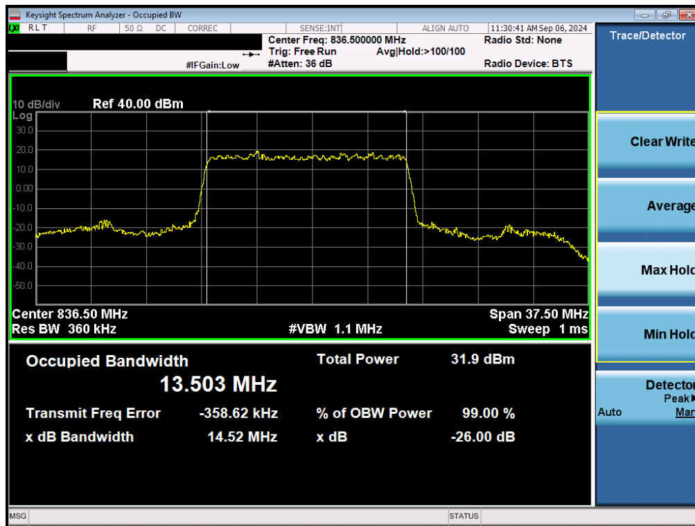
Plot 7-39. Occupied Bandwidth Plot (NR Band n5 - 15MHz \pi/2 BPSK - Full RB - Ant2)
