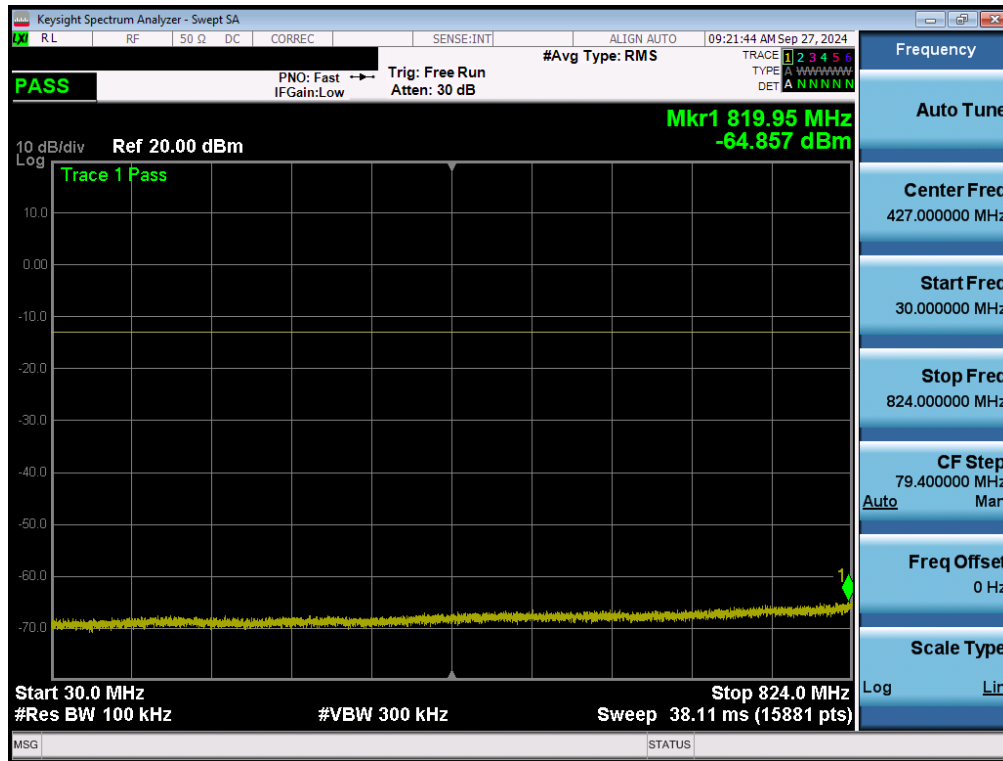
Plot 7-63. Conducted Spurious Plot (WCDMA Ch. 4233 – Ant2)
