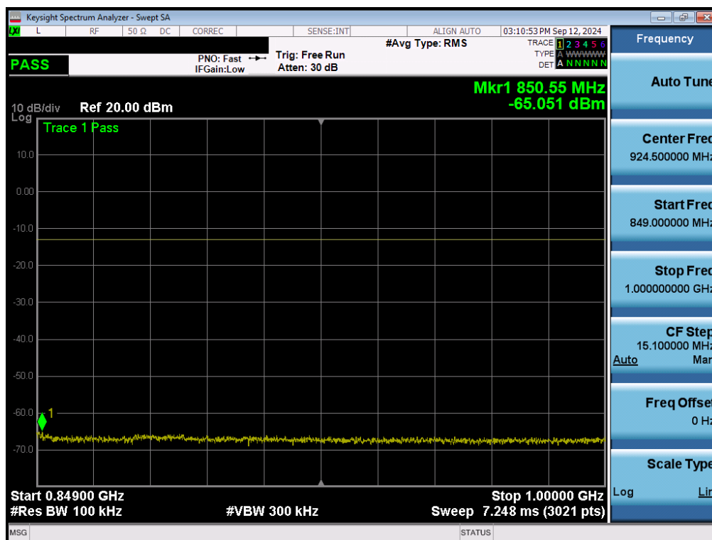
Plot 7-55. Conducted Spurious Plot (LTE Band 5 - 10MHz QPSK - 1 RB - Mid Channel – Ant1)
