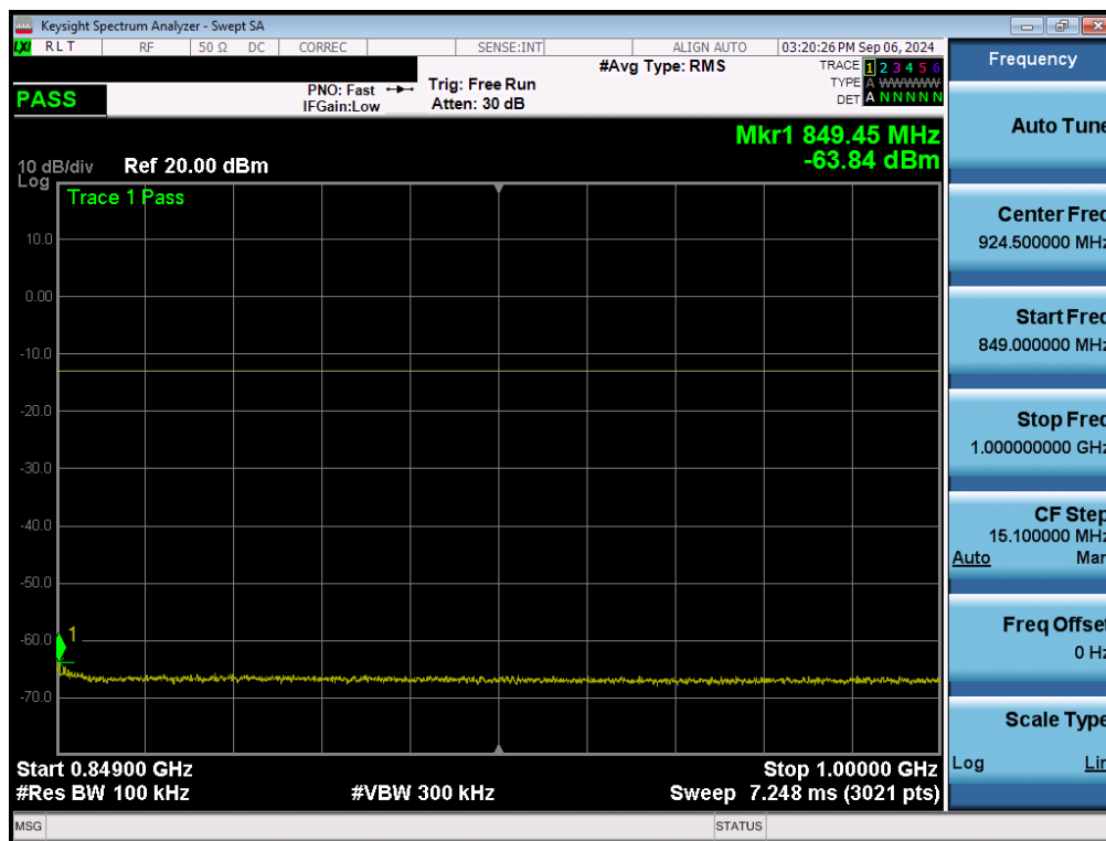
Plot 7-58. Conducted Spurious Plot (NR Band n5 - 20.0MHz - 1 RB - Low Channel - Ant1)
