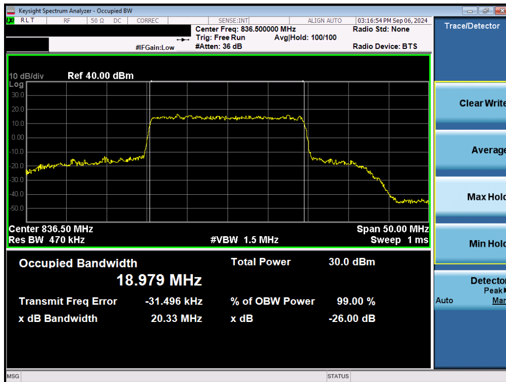
Plot 7-14. Occupied Bandwidth Plot (NR Band n5 - 20MHz QPSK - Full RB - Ant1)
