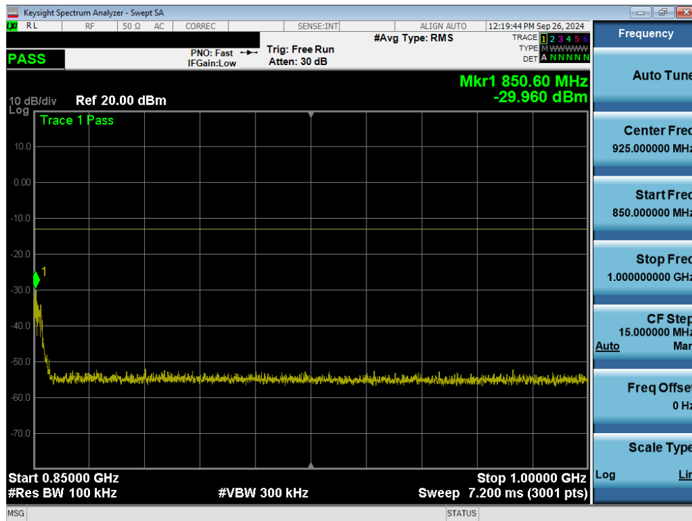
Plot 7-49. Conducted Spurious Plot (GPRS Ch. 251 – Ant1)
