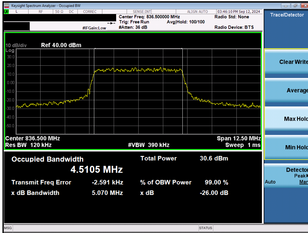
Plot 7-30. Occupied Bandwidth Plot (LTE Band 5 - 5MHz QPSK - Full RB - Ant2)
