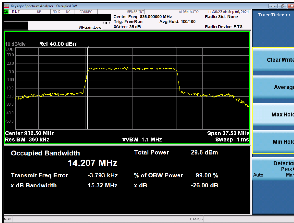
Plot 7-40. Occupied Bandwidth Plot (NR Band n5 - 15MHz QPSK - Full RB - Ant2)
