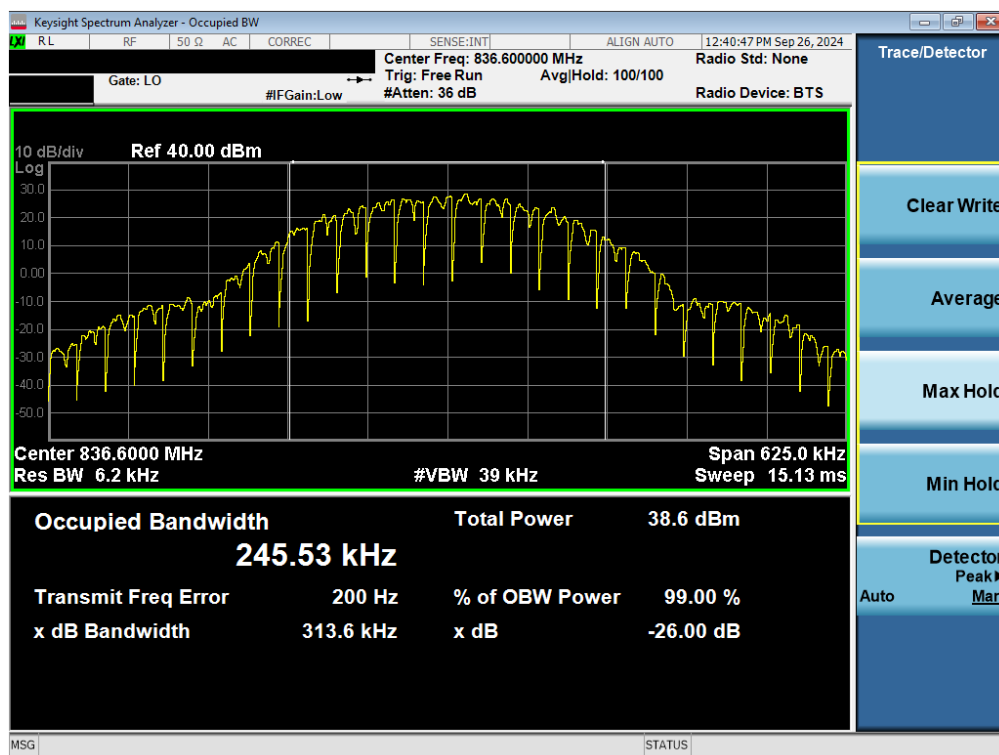
Plot 7-25. Occupied Bandwidth Plot (GPRS, Ch. 190 – Ant2)
