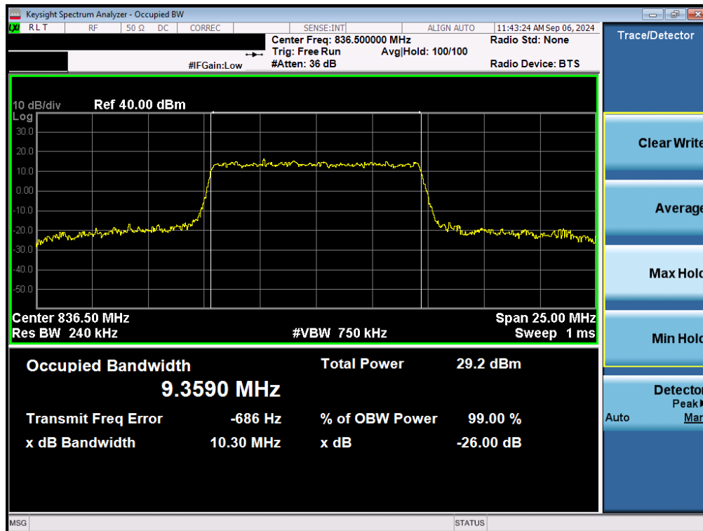
Plot 7-43. Occupied Bandwidth Plot (NR Band n5 - 10MHz QPSK - Full RB - Ant2)
