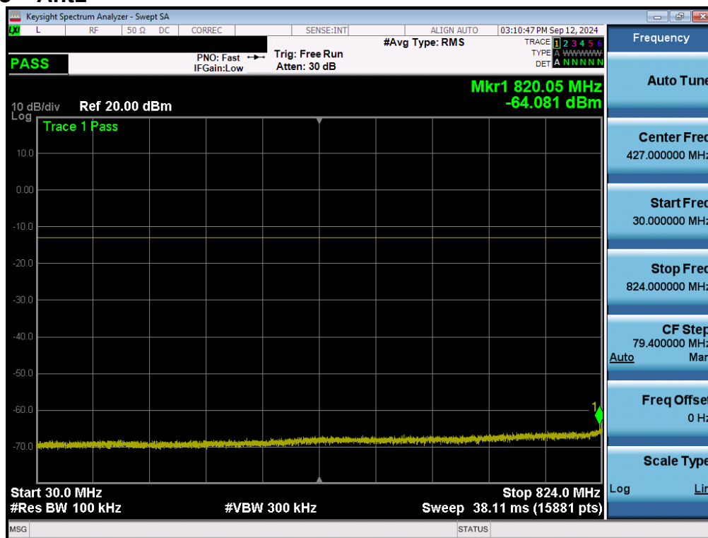
Plot 7-54. Conducted Spurious Plot (LTE Band 5 - 10MHz QPSK - 1 RB - Mid Channel – Ant1)
