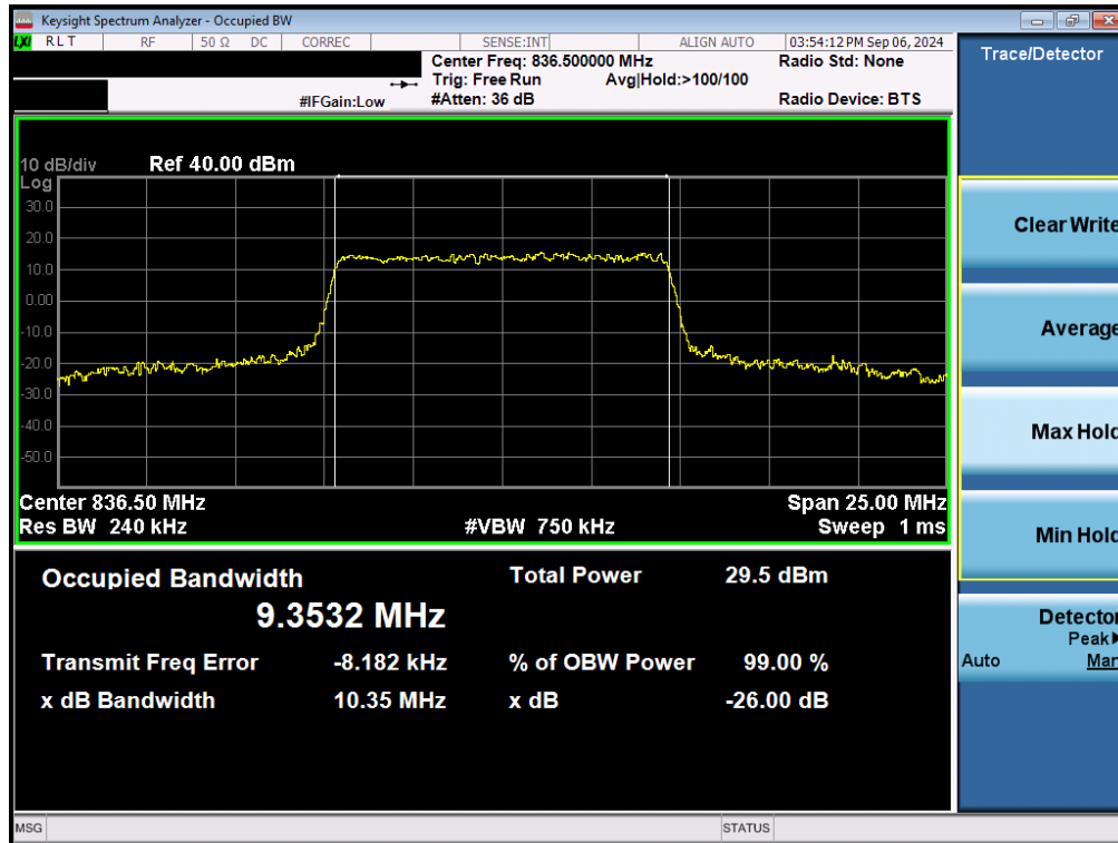
Plot 7-21. Occupied Bandwidth Plot (NR Band n5 - 10MHz 16-QAM - Full RB - Ant1)
