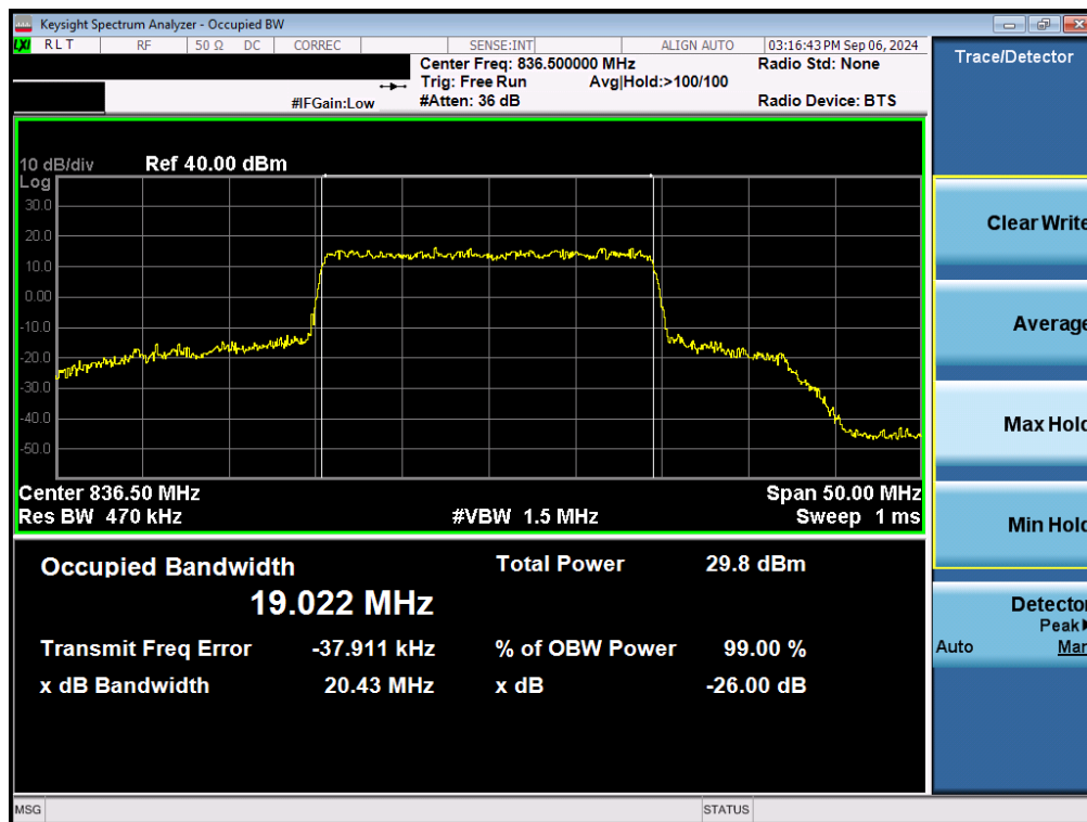
Plot 7-15. Occupied Bandwidth Plot (NR Band n5 - 20MHz 16-QAM - Full RB - Ant1)
