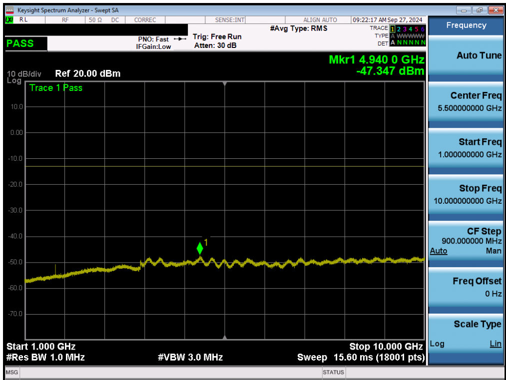
Plot 7-65. Conducted Spurious Plot (WCDMA Ch. 4233 – Ant2)
