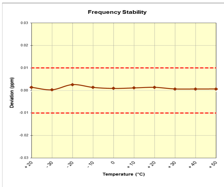
Figure 7-3. Frequency Stability Plot
