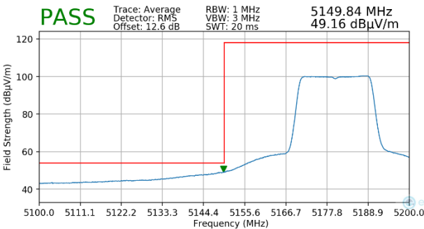
Plot 7-1. Radiated Lower Band Edge Plot MIMO (Average – UNII Band 1)
