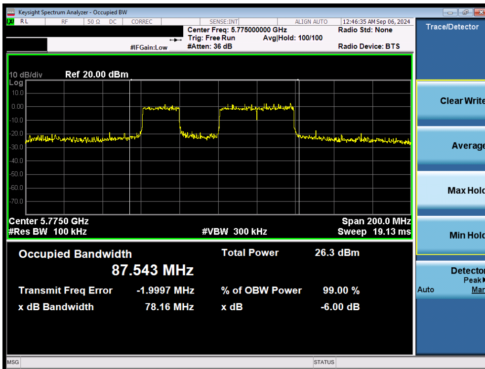
Plot 7-50. 6dB Bandwidth Plot MIMO ANT2 (80MHz 802.11be (20MHz Puncture) (UNII Band 3) – Ch. 155)
