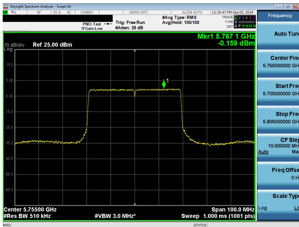
Plot 7-77. Power Spectral Density Plot MIMO ANT1 (40MHz 802.11ax/be (UNII Band 3) – Ch. 151)
