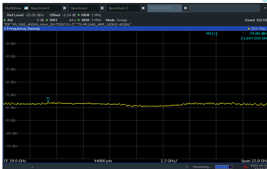
Plot 7-49. Radiated Spurious Pre-Scan 18 – 40 GHz - CH.9
