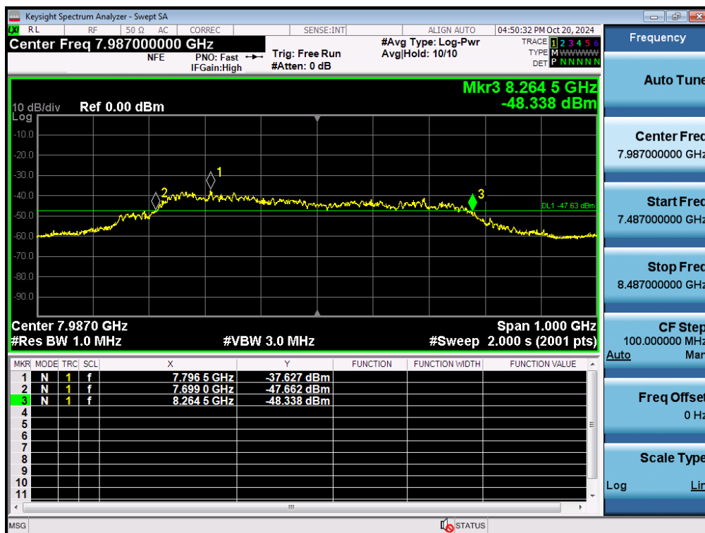
Plot 7-26. 10dBc Bandwidth – CH.9 – SP1 – Preamble 12
