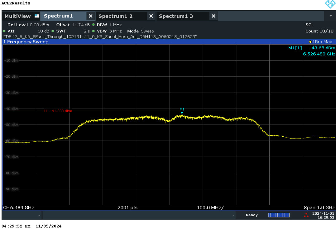
Plot 7-38. UWB Average Power Measurement - CH.5 – HPRF
