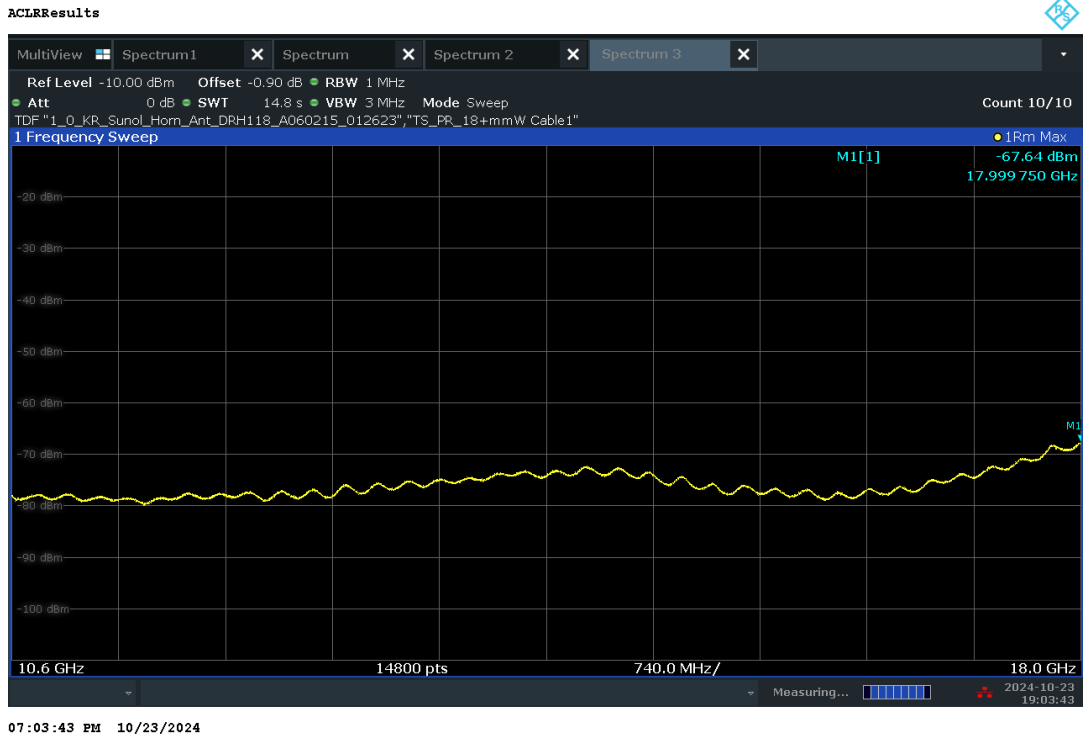
Plot 7-41. Radiated Spurious Pre-Scan 10600 - 18000 MHz - CH.5
