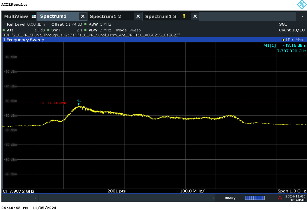
Plot 7-39. UWB Average Power Measurement - CH.9 – HPRF
