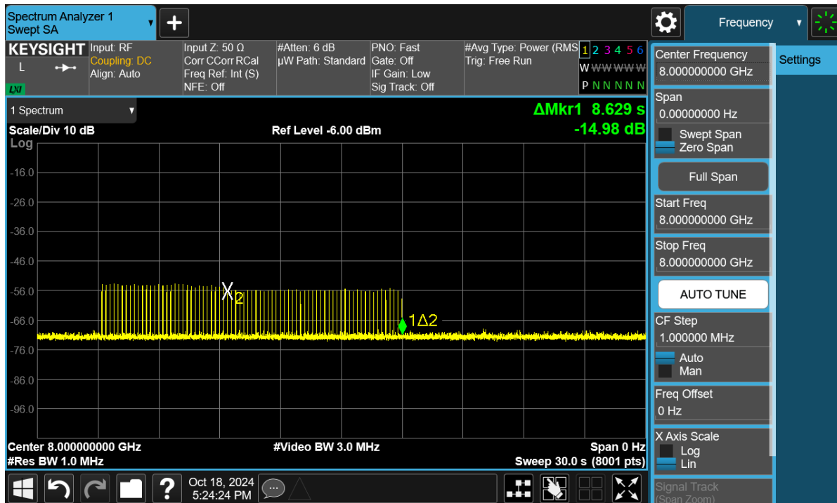
Plot 7-31. Cessation Time Plot
