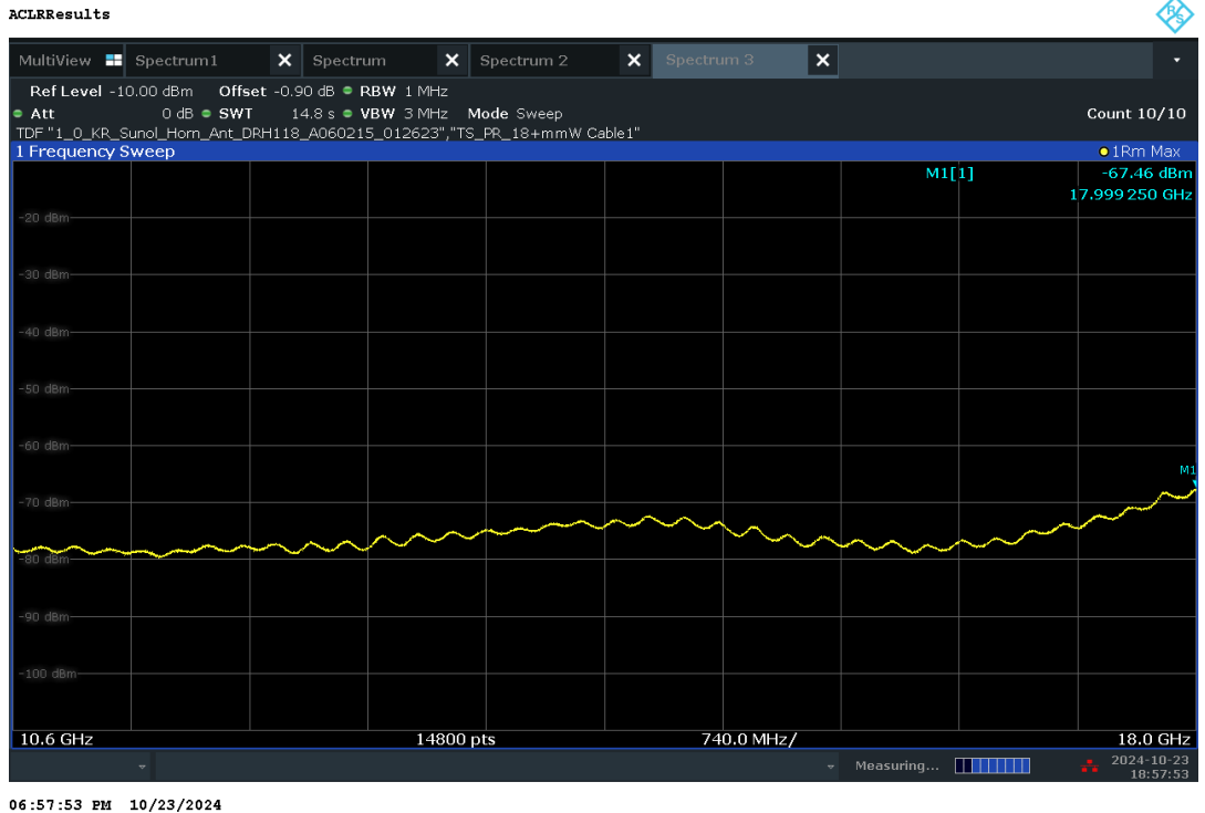
Plot 7-46. Radiated Spurious Pre-Scan 10600 - 18000 MHz - CH.9
