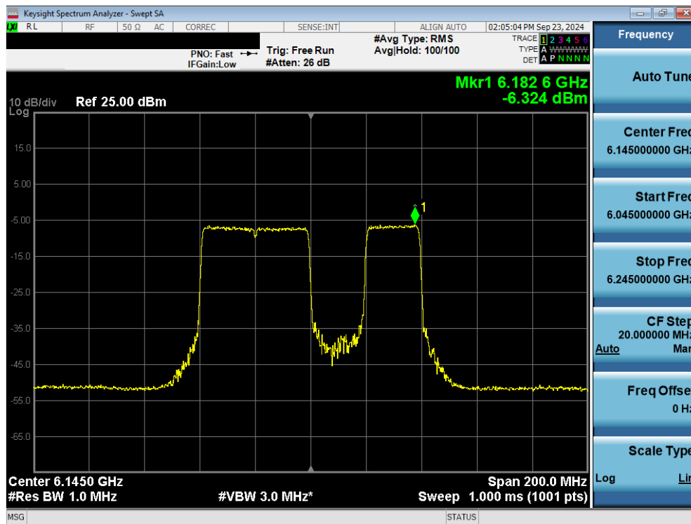
Plot 7-41. Power Spectral Density Plot MIMO ANT2 (80MHz 802.11be (UNII Band 5) – Ch. 39) – 20MHz Punctured - VLP
