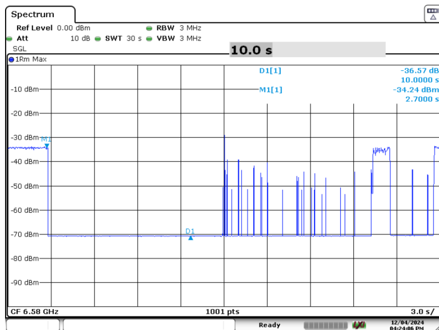
Plot 7-3. Contention Based Protocol Timing Plot (320MHz (UNII Band 5) – Ch. 95 High)
