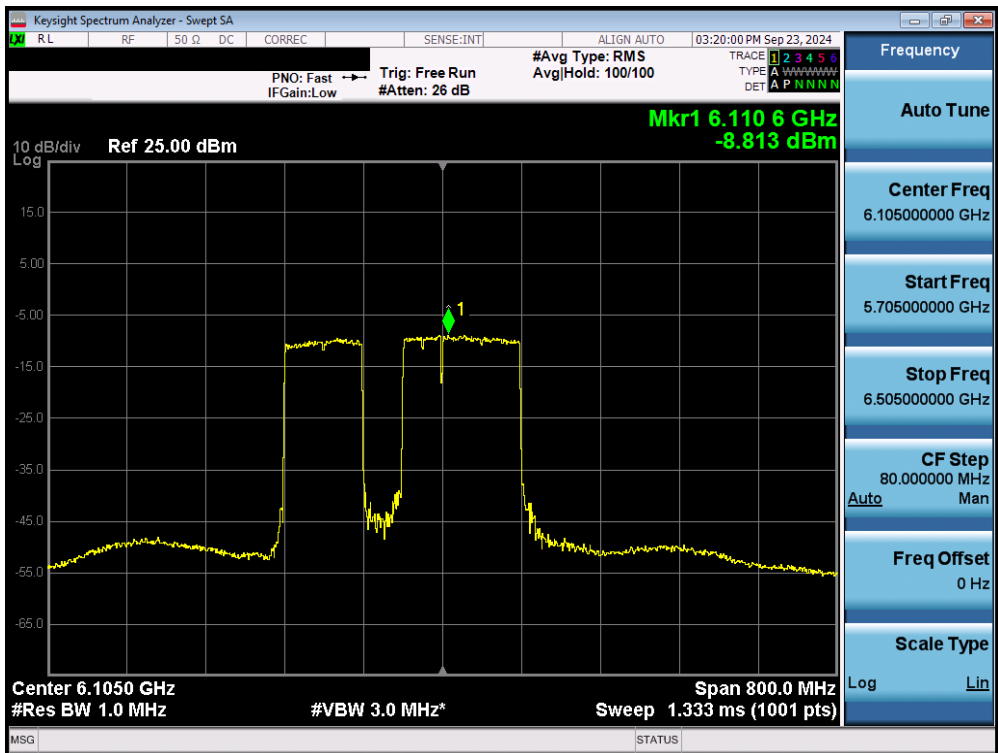
Plot 7-34. Power Spectral Density Plot MIMO ANT1 (320MHz 802.11be (UNII Band 5) – Ch. 31) – 120MHz Punctured - VLP
