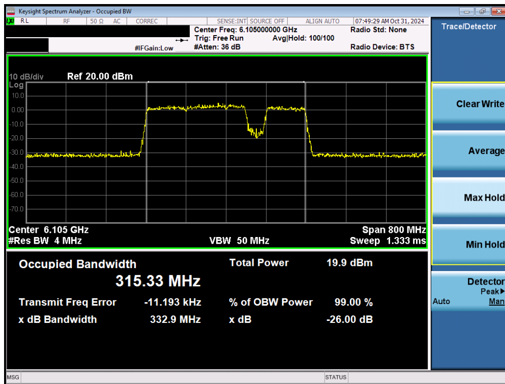
Plot 7-16. 26dB Bandwidth Plot MIMO ANT1 (320MHz 802.11be (UNII Band 5) – Ch. 31) – 40MHz Punctured - VLP
