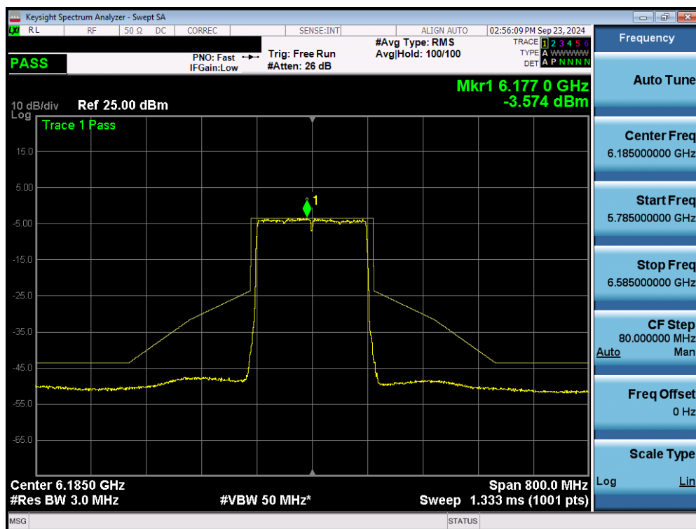
Plot 7-48. In Band Emissions Plot MIMO ANT1 (160MHz 802.11ax/be (UNII Band 5) – Ch. 47) - VLP
