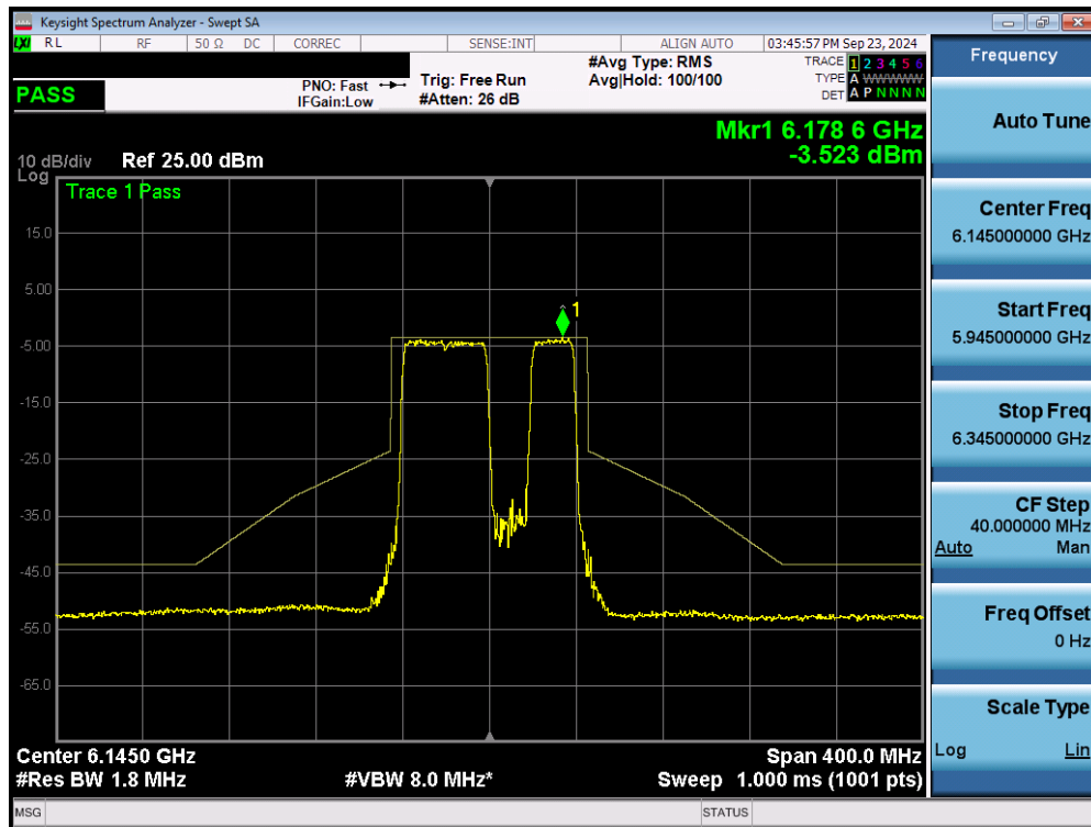
Plot 7-50. In Band Emissions Plot MIMO ANT1 (80MHz 802.11be (UNII Band 5) – Ch. 39) – 20MHz Punctured - VLP
