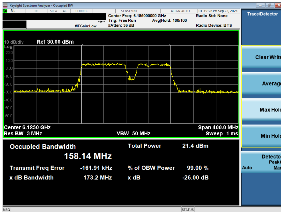
Plot 7-24. 26dB Bandwidth Plot MIMO ANT2 (160MHz 802.11be (UNII Band 5) – Ch. 47) – 20MHz Punctured - VLP
