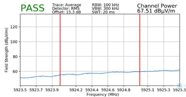
Plot 7-7. Radiated Lower Band Edge Plot MIMO (Average – UNII Band 5)
