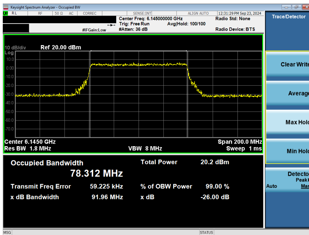
Plot 7-20. 26dB Bandwidth Plot MIMO ANT2 (80MHz 802.11ax/be (UNII Band 5) – Ch. 39) - VLP
