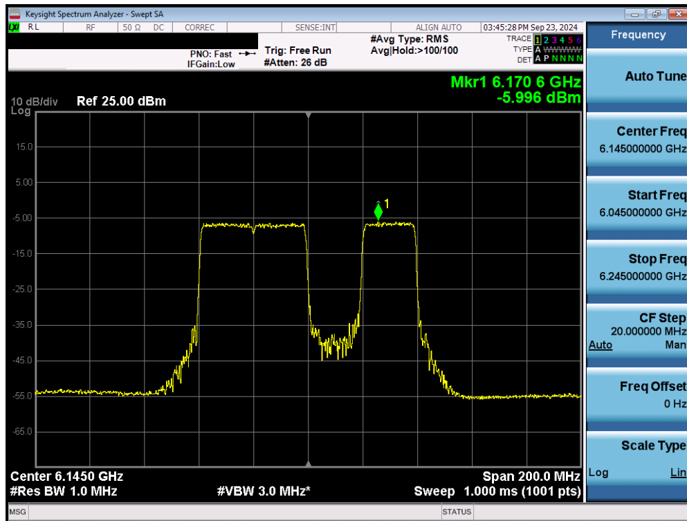
Plot 7-32. Power Spectral Density Plot MIMO ANT1 (80MHz 802.11be (UNII Band 5) – Ch. 39) – 20MHz Punctured - VLP
