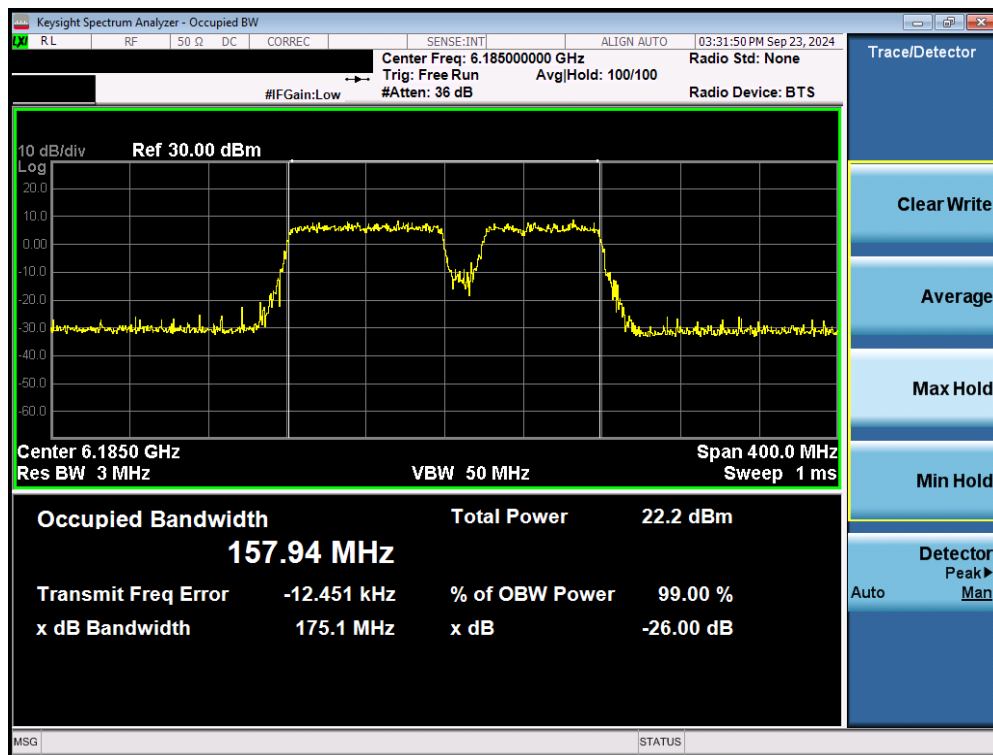
Plot 7-15. 26dB Bandwidth Plot MIMO ANT1 (160MHz 802.11be (UNII Band 5) – Ch. 47) – 20MHz Punctured - VLP
