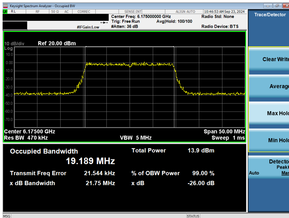
Plot 7-18. 26dB Bandwidth Plot MIMO ANT2 (20MHz 802.11ax/be (UNII Band 5) – Ch. 45) - VLP
