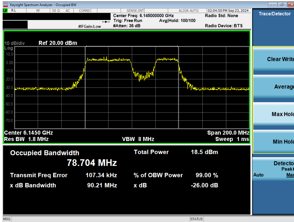
Plot 7-23. 26dB Bandwidth Plot MIMO ANT2 (80MHz 802.11be (UNII Band 5) – Ch. 39) – 20MHz Punctured - VLP
