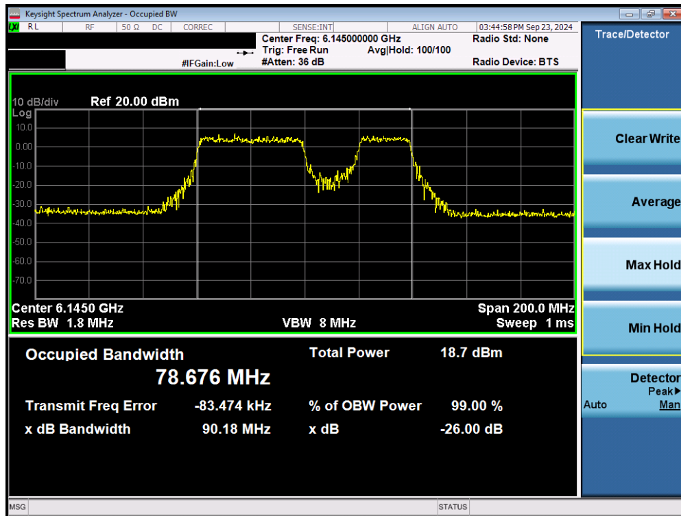
Plot 7-14. 26dB Bandwidth Plot MIMO ANT1 (80MHz 802.11be (UNII Band 5) – Ch. 39) – 20MHz Punctured - VLP
