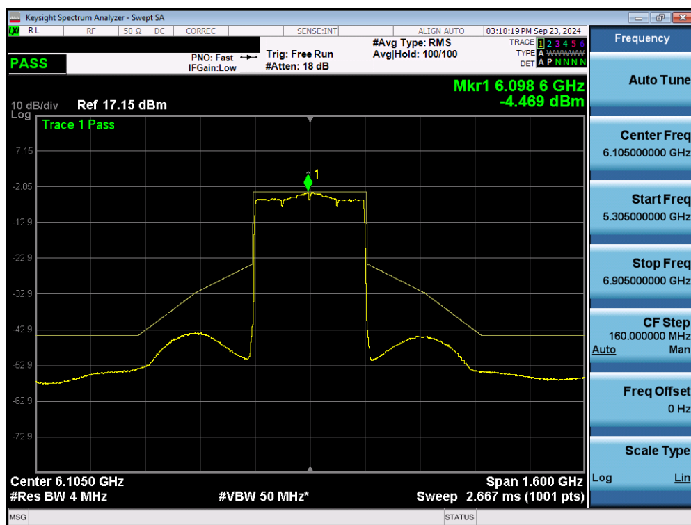
Plot 7-49. In Band Emissions Plot MIMO ANT1 (320MHz 802.11ax/be (UNII Band 5) – Ch. 31) - VLP
