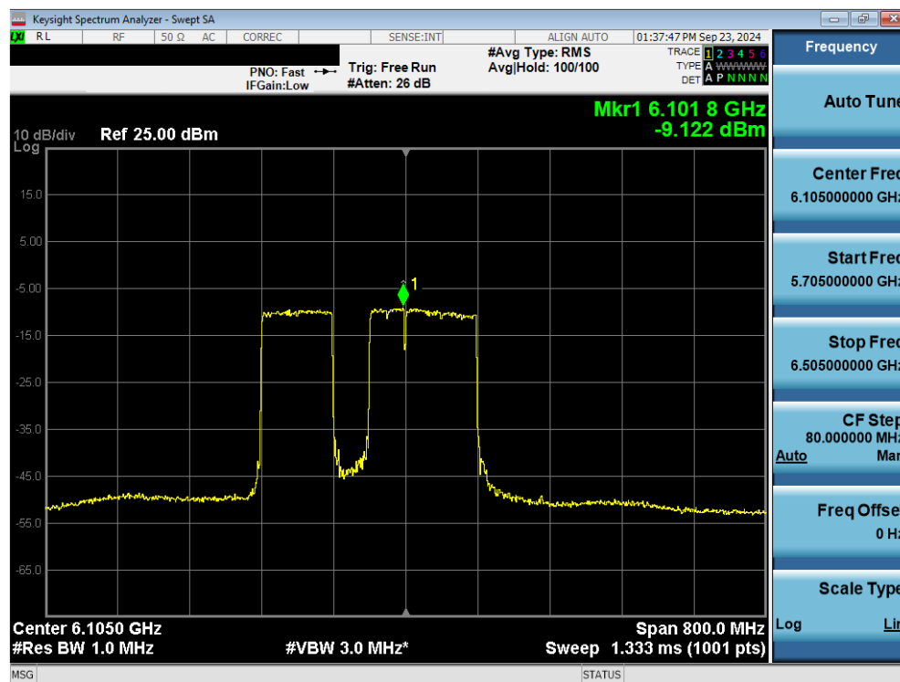
Plot 7-43. Power Spectral Density Plot MIMO ANT2 (320MHz 802.11be (UNII Band 5) – Ch. 31) – 120MHz Punctured – VLP
