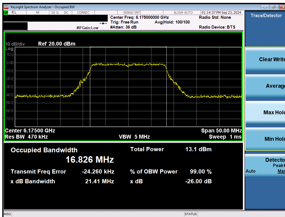
Plot 7-8. 26dB Bandwidth Plot MIMO ANT1 (20MHz 802.11a (UNII Band 5) – Ch. 45) - VLP
