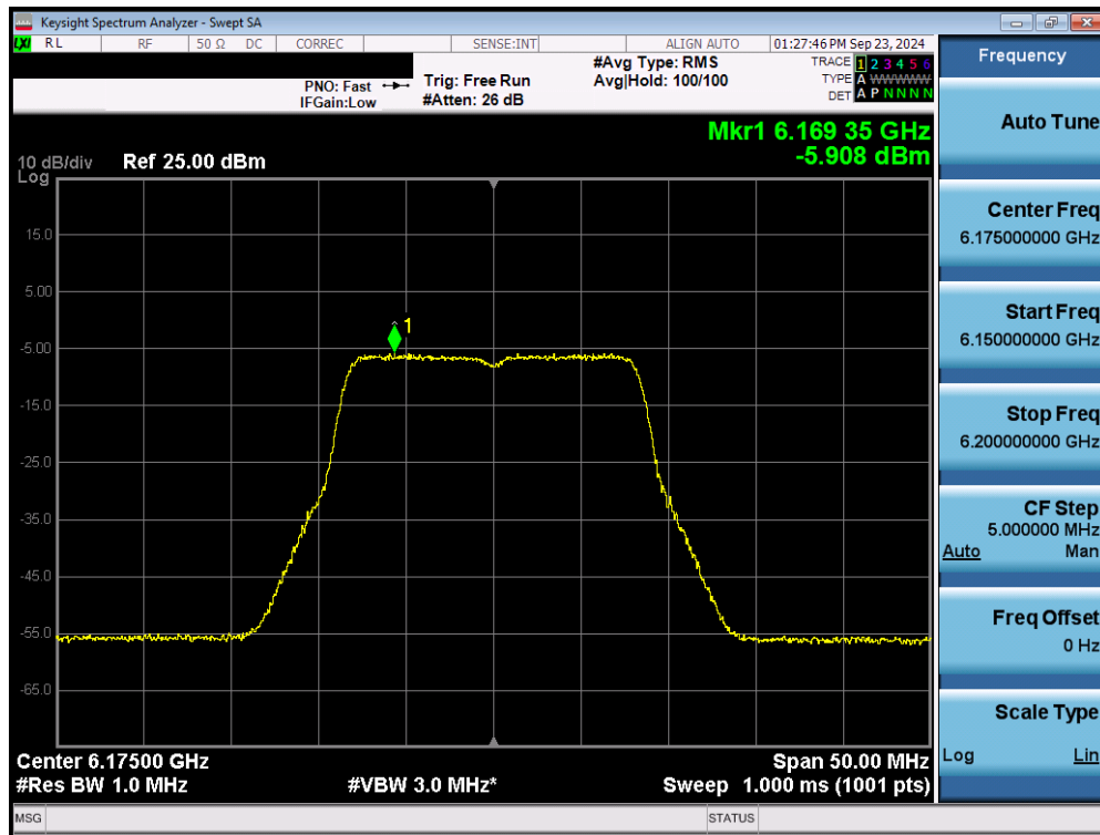
Plot 7-26. Power Spectral Density Plot MIMO ANT1 (20MHz 802.11a (UNII Band 5) – Ch. 45) - VLP
