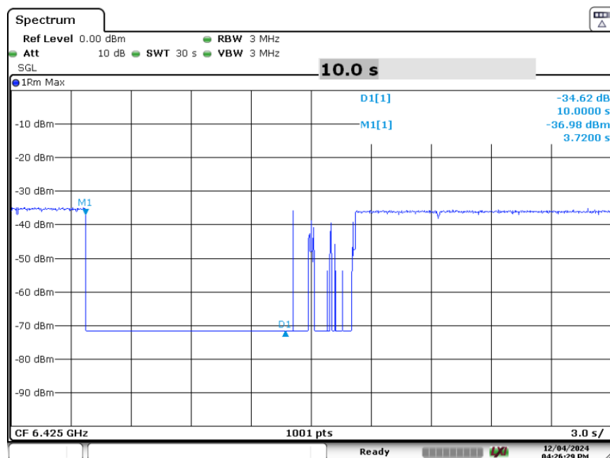
Plot 7-2. Contention Based Protocol Timing Plot (320MHz (UNII Band 5) – Ch. 95 Mid)
