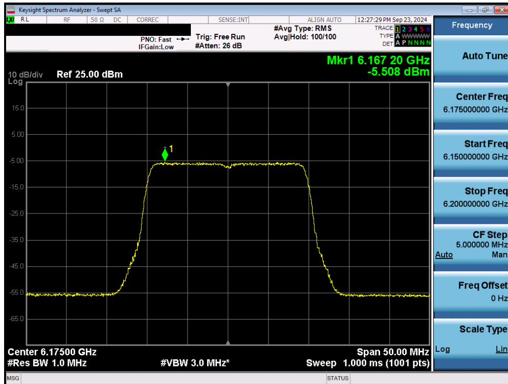
Plot 7-27. Power Spectral Density Plot MIMO ANT1 (20MHz 802.11ax/be (UNII Band 5) – Ch. 45) - VLP
