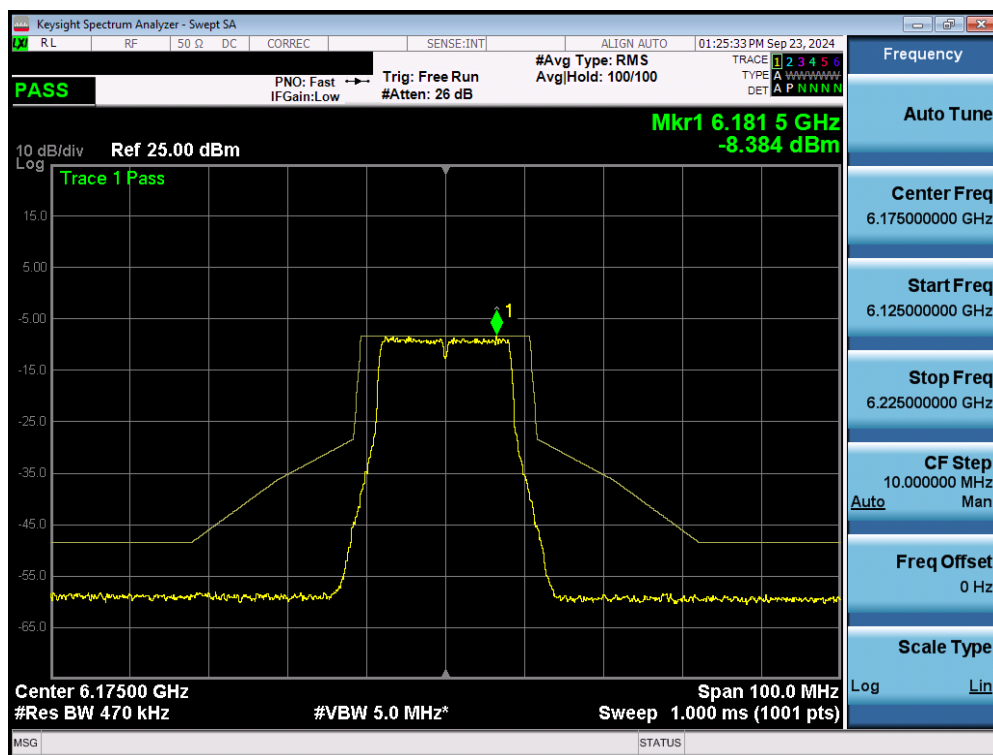
Plot 7-44. In Band Emissions Plot MIMO ANT1 (20MHz 802.11a (UNII Band 5) – Ch. 45) - VLP
