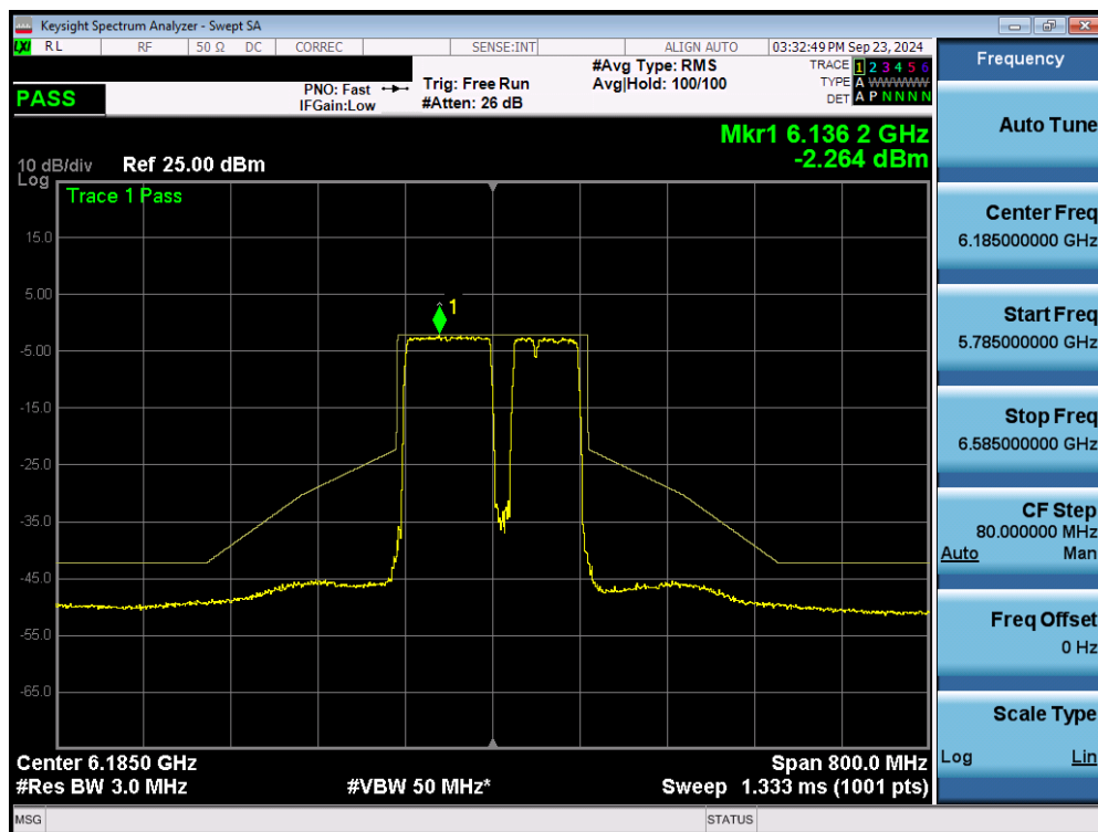
Plot 7-51. In Band Emissions Plot MIMO ANT1 (160MHz 802.11be (UNII Band 5) – Ch. 47) – 20MHz Punctured - VLP
