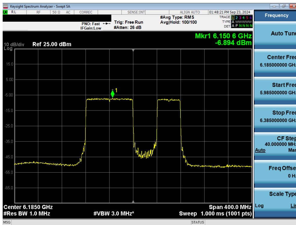
Plot 7-42. Power Spectral Density Plot MIMO ANT2 (160MHz 802.11be (UNII Band 5) – Ch. 47) – 40MHz Punctured - VLP
