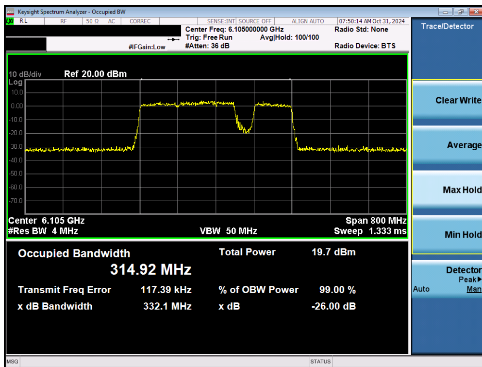
Plot 7-25. 26dB Bandwidth Plot MIMO ANT2 (320MHz 802.11be (UNII Band 5) – Ch. 31) – 40MHz Punctured - VLP
