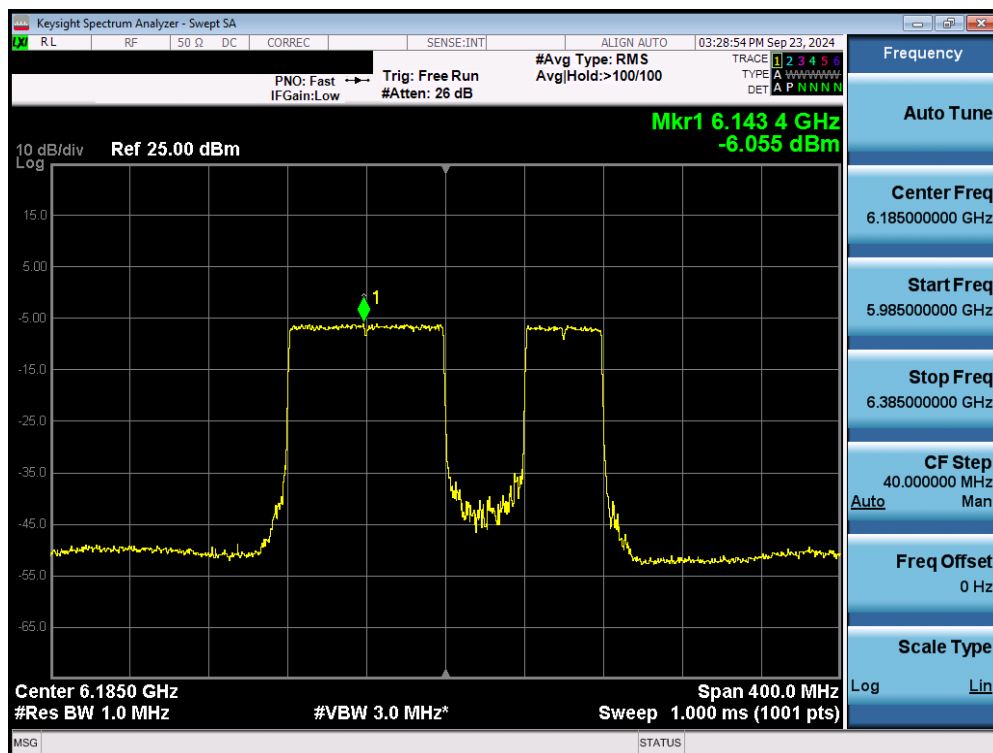
Plot 7-33. Power Spectral Density Plot MIMO ANT1 (160MHz 802.11be (UNII Band 5) – Ch. 47) – 40MHz Punctured - VLP
