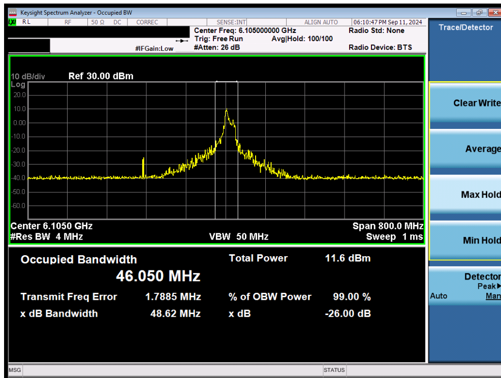
Plot 7-34. 26dB Bandwidth Plot MIMO ANT2 (320MHz 802.11ax/be (26 Tones) (UNII Band 5) – Ch. 31) - LPI
