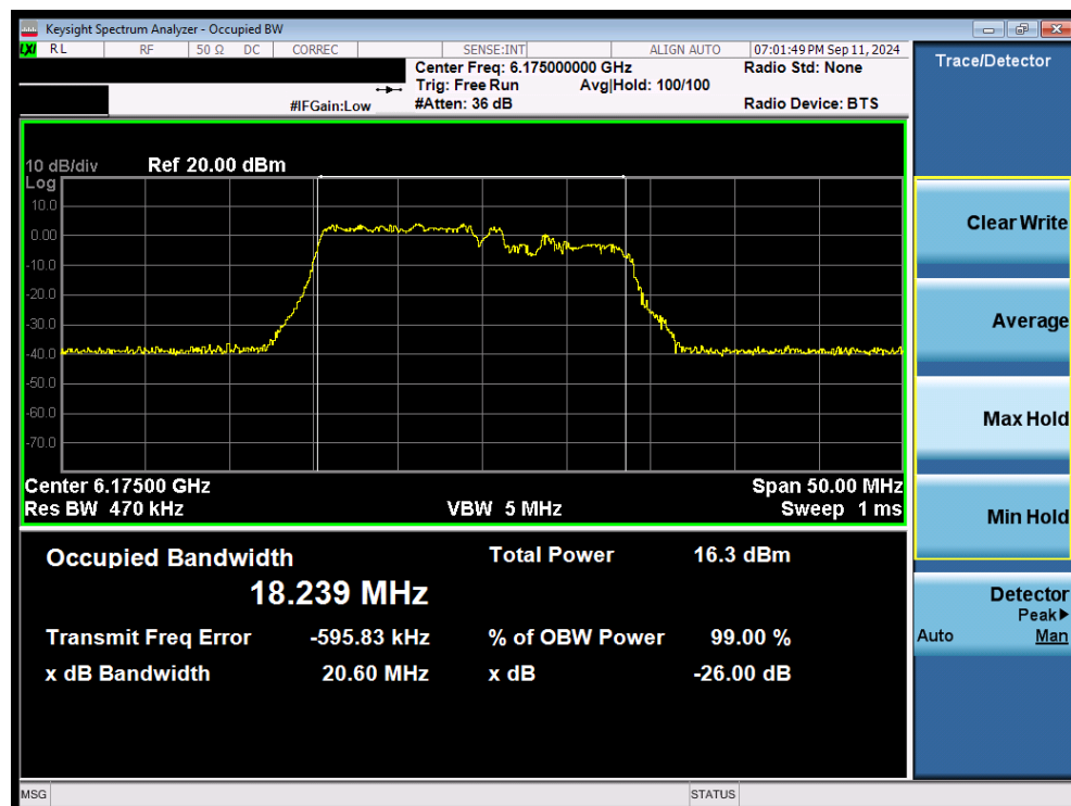
Plot 7-35. 26dB Bandwidth Plot MIMO ANT2 (20MHz 802.11be (106+26 Tones) (UNII Band 5) – Ch. 45) - LPI
