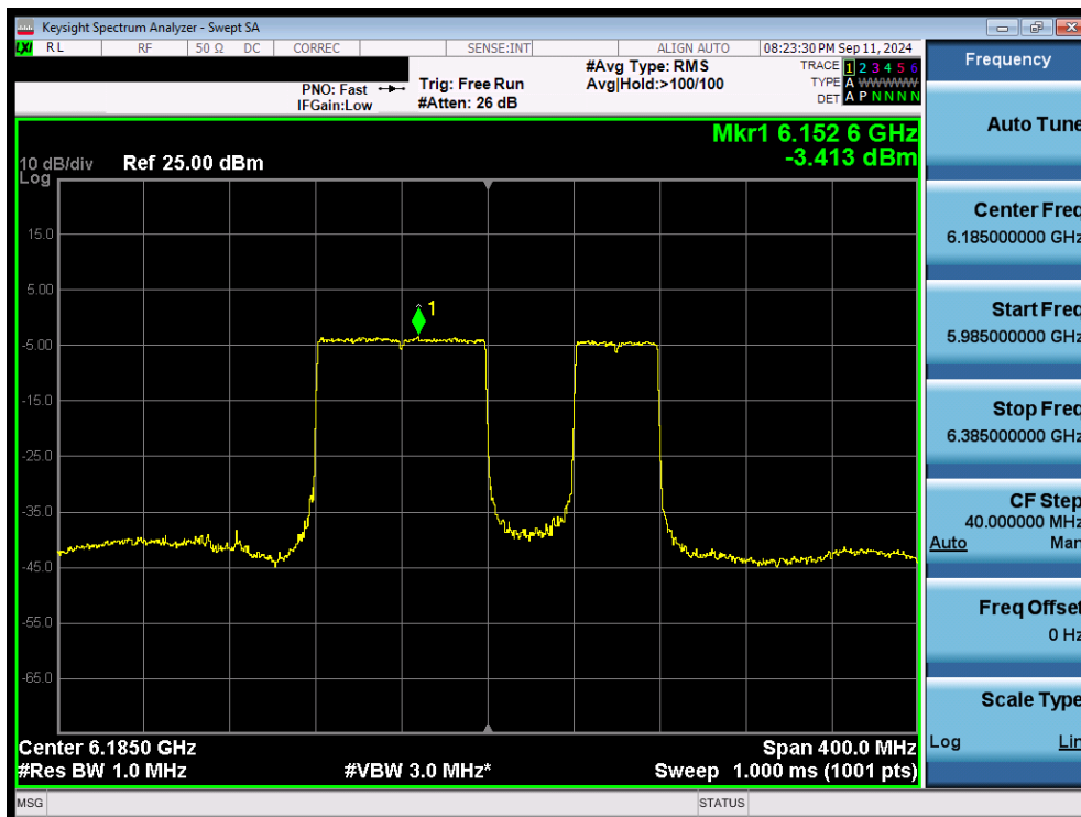
Plot 7-83. Power Spectral Density Plot MIMO ANT2 (160MHz 802.11be (996+484 Tones) (UNII Band 5) – Ch. 47) LPI/SP
