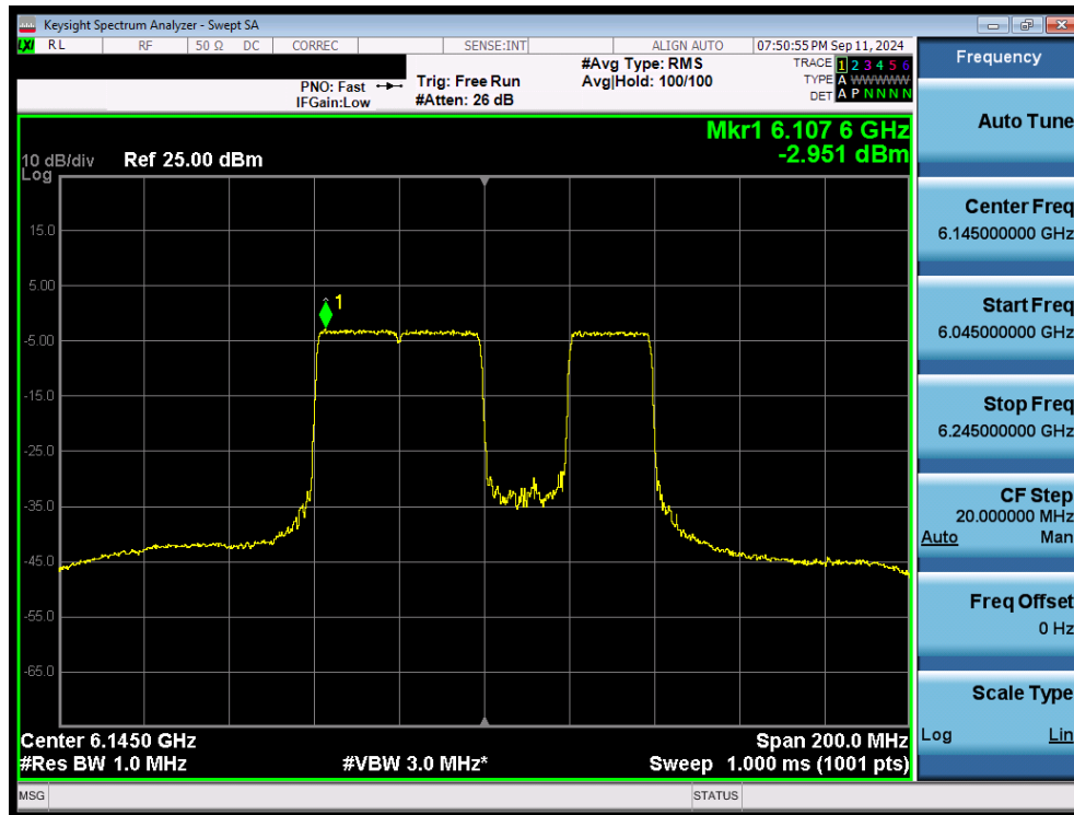
Plot 7-82. Power Spectral Density Plot MIMO ANT2 (80MHz 802.11be (484+242 Tones) (UNII Band 5) – Ch. 39) LPI
