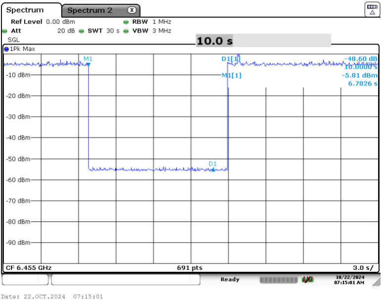
Plot 7-153. Contention Based Protocol Timing Plot (20MHz (UNII Band 6) – Ch. 101)
