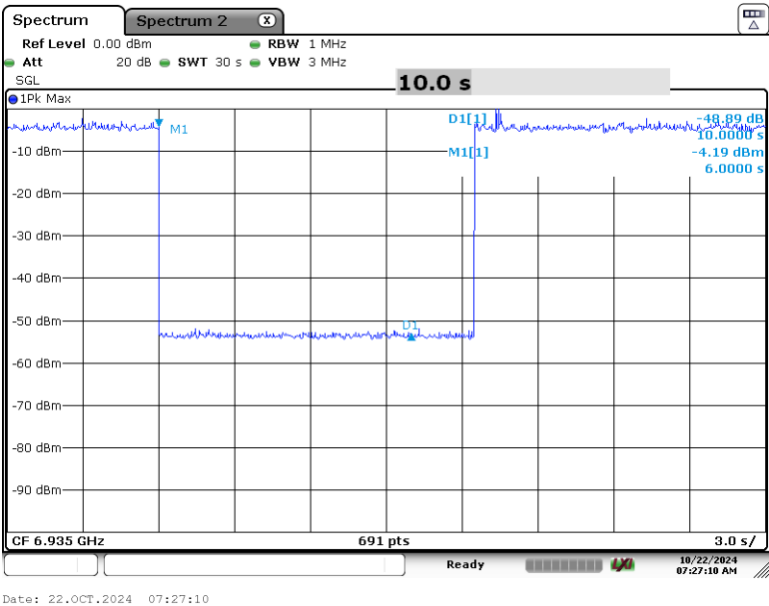
Plot 7-161. Contention Based Protocol Timing Plot (20MHz (UNII Band 8) – Ch. 197)
