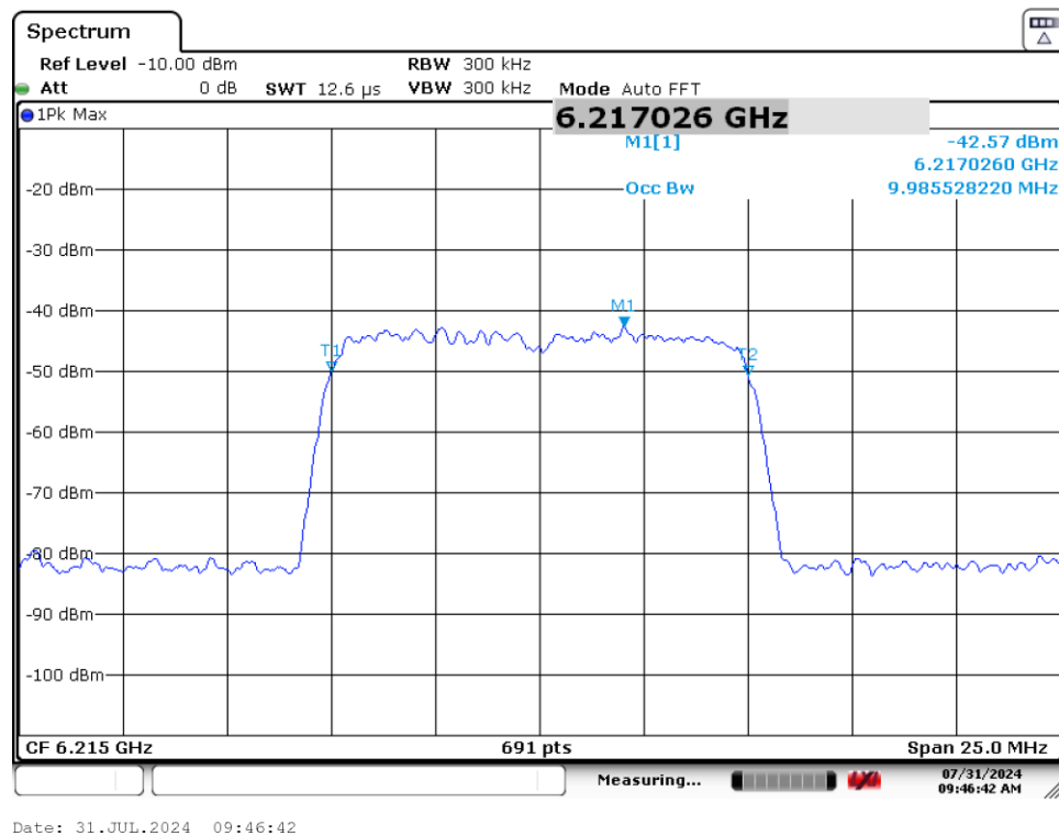
Plot 7-148. AWGN Signal (Demonstration)
