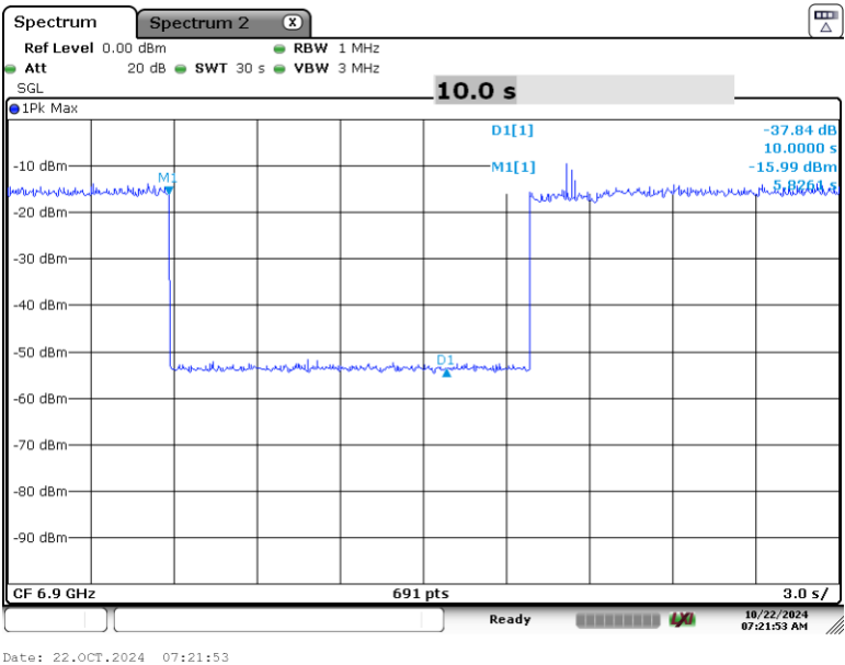
Plot 7-160. Contention Based Protocol Timing Plot (320MHz (UNII Band 7) – Ch. 159 High)
