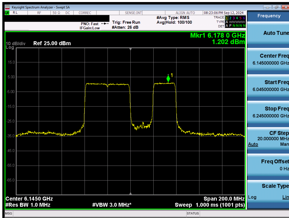
Plot 7-91. Power Spectral Density Plot MIMO ANT2 (80MHz 802.11be (484+242 Tones) (UNII Band 5) – Ch. 39) SP
