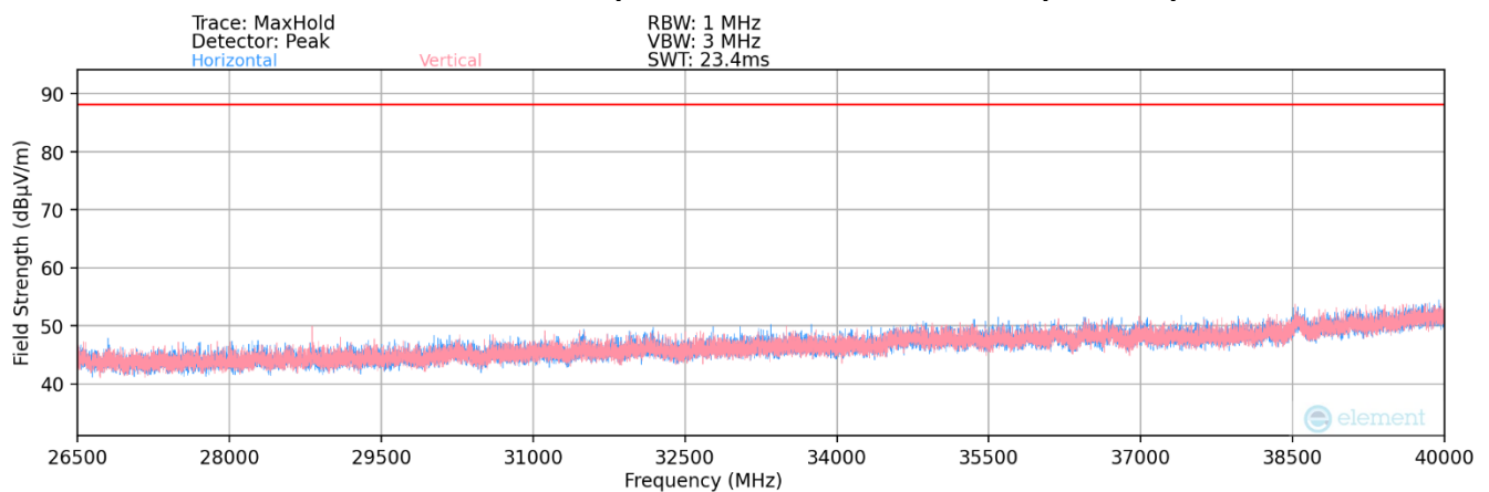
Plot 7-173. Radiated Spurious Plot 26.5GHz - 40GHz (802.11ax)
