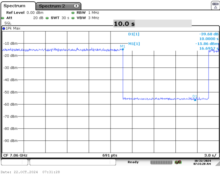
Plot 7-164. Contention Based Protocol Timing Plot (320MHz (UNII Band 8) – Ch. 191 High)
