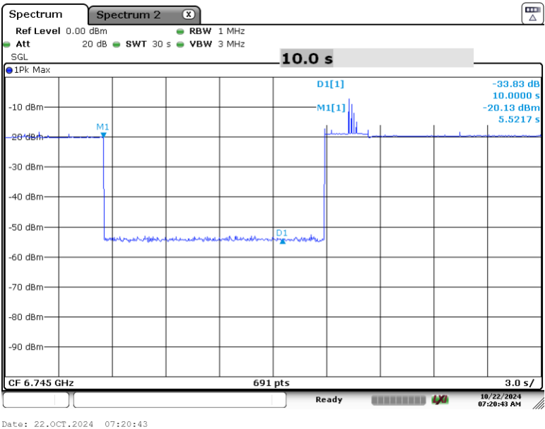
Plot 7-159. Contention Based Protocol Timing Plot (320MHz (UNII Band 7) – Ch. 159 Mid)
