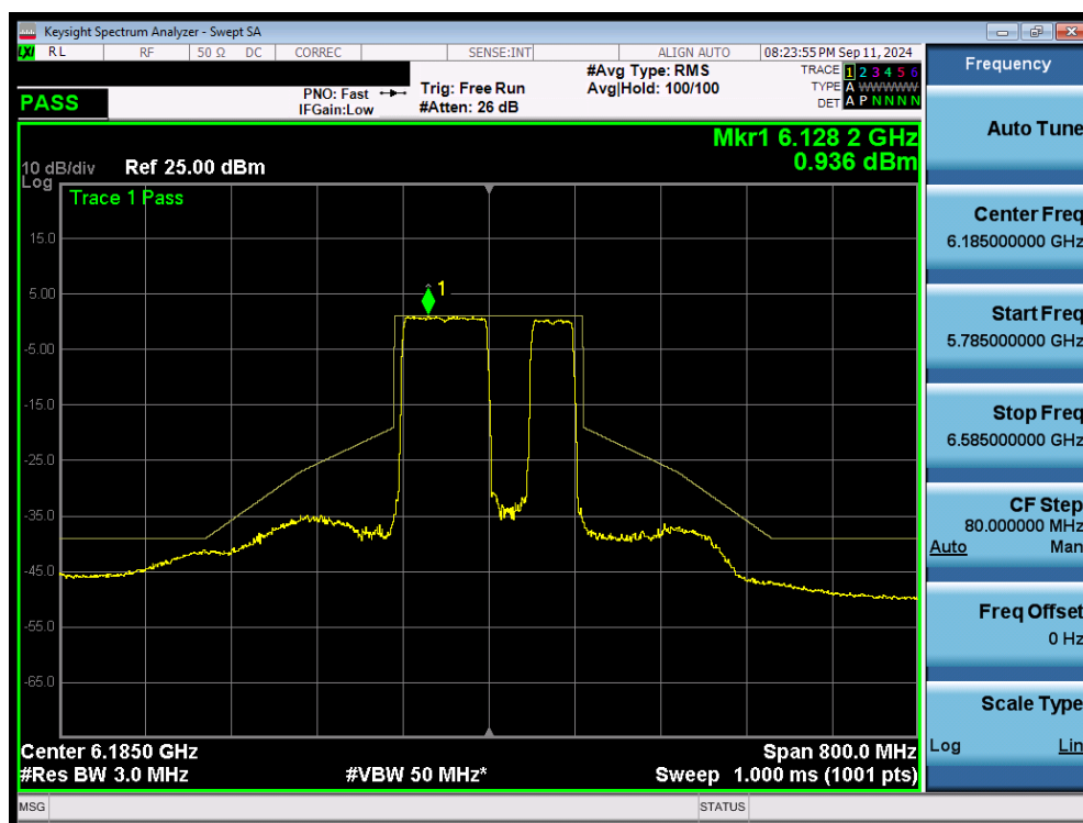
Plot 7-131. In Band Emissions Plot MIMO ANT2 (160MHz 802.11be (996+484 Tones) (UNII Band 5) – Ch. 47) LPI
