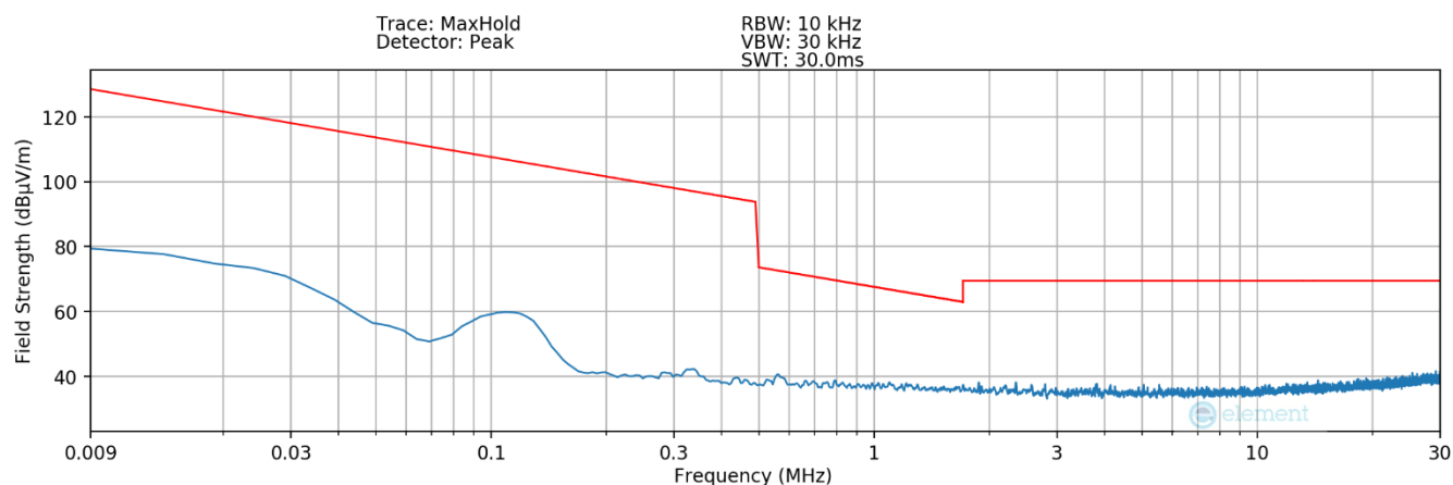
Plot 7-8 Radiated Spurious Plot 9kHz – 30MHz (Pol. Y – Device to Device)
