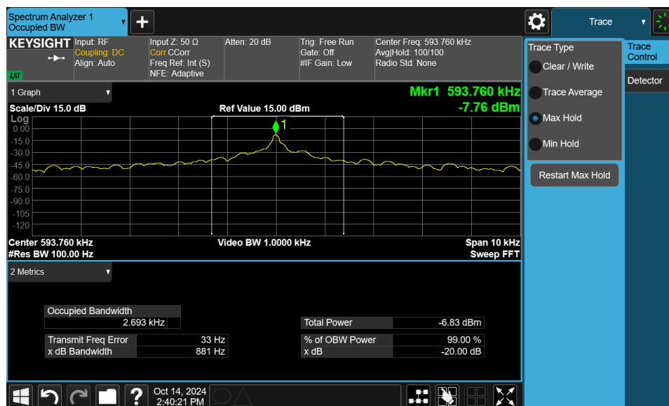
Plot 7-6. Occupied Bandwidth Measurement – Eraser
