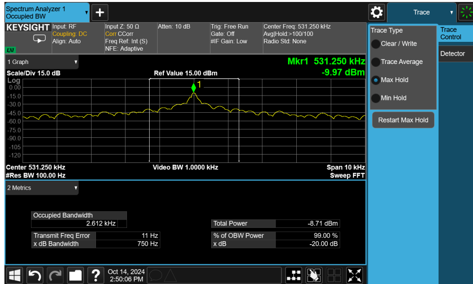
Plot 7-4. Occupied Bandwidth Measurement – Click
