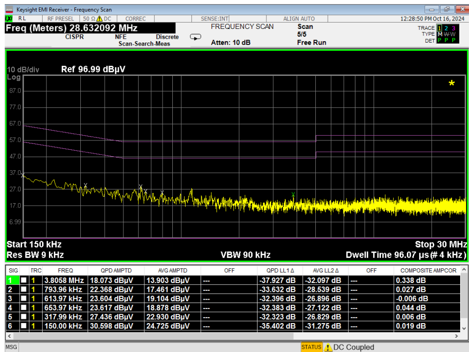
Plot 7-26. Line-Conducted Test Plot (N) – Digitizer (Eraser)
