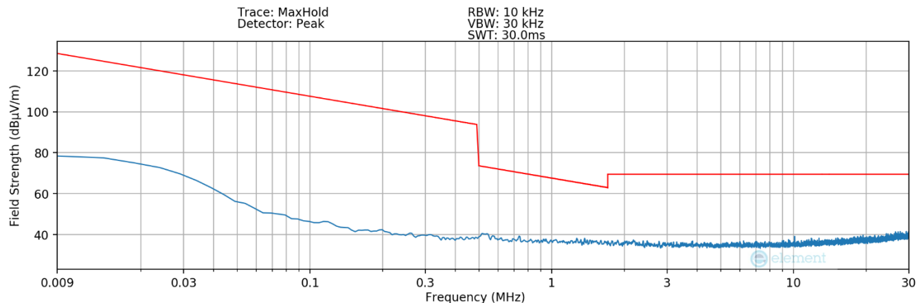
Plot 7-10. Radiated Spurious Plot 9kHz – 30MHz (Pol. X – Digitizer – Click)
