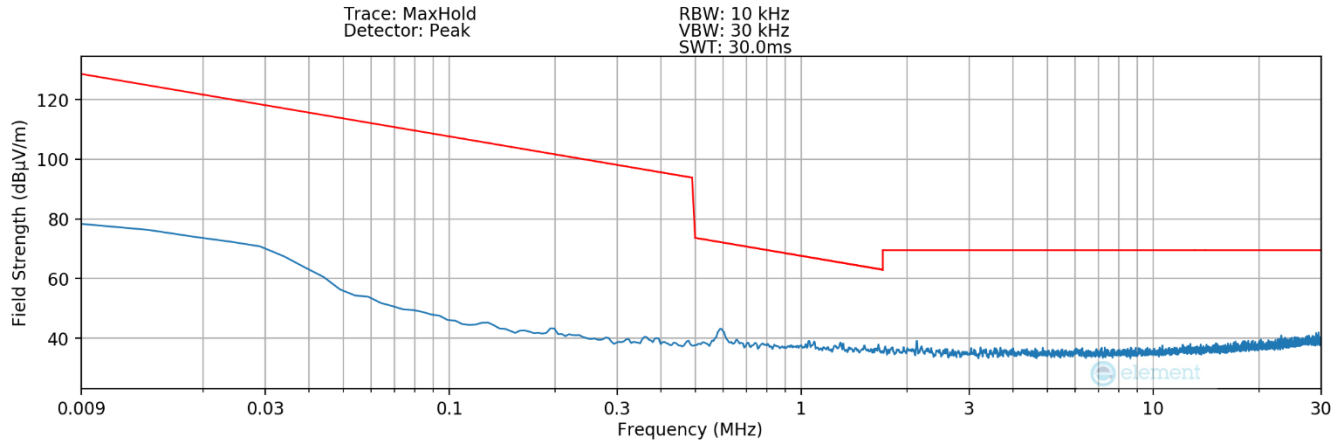
Plot 7-16. Radiated Spurious Plot 9kHz – 30MHz (Pol. X – Digitizer – Eraser)
