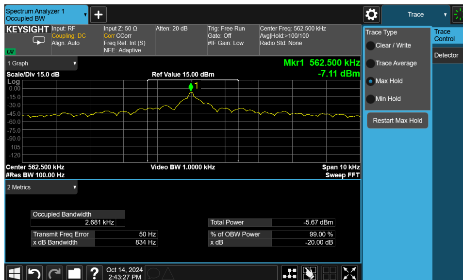
Plot 7-5. Occupied Bandwidth Measurement – Hover
