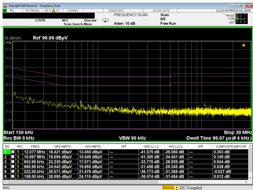
Plot 7-24. Line-Conducted Test Plot (N) – Digitizer (Hover)
