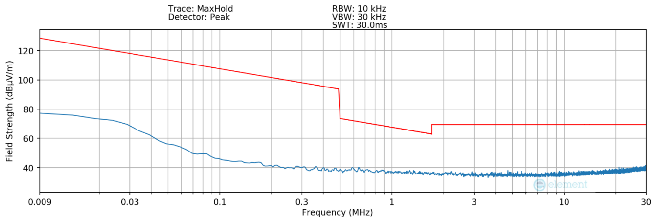
Plot 7-18. Radiated Spurious Plot 9kHz – 30MHz (Pol. Z– Digitizer – Eraser)
