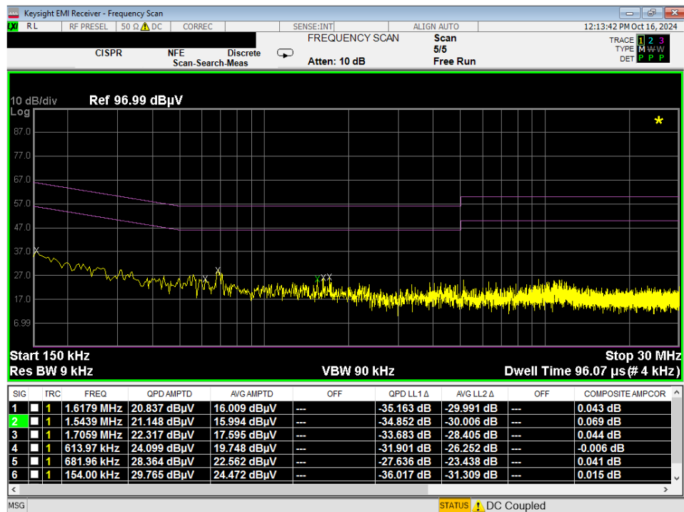
Plot 7-23. Line-Conducted Test Plot (L1) – Digitizer (Hover)
