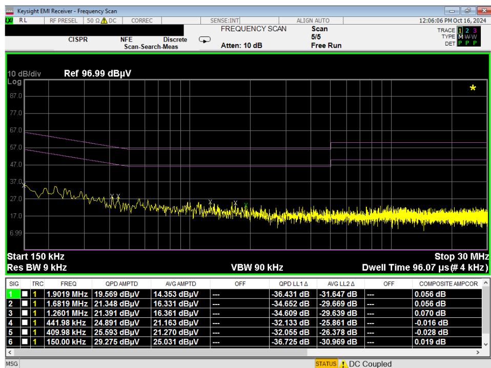
Plot 7-22. Line-Conducted Test Plot (N) – Digitizer (Click)
