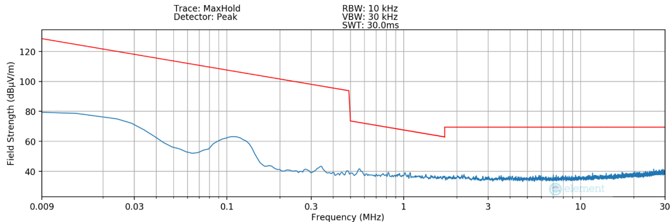
Plot 7-7. Radiated Spurious Plot 9kHz – 30MHz (Pol. X – Device to Device)
