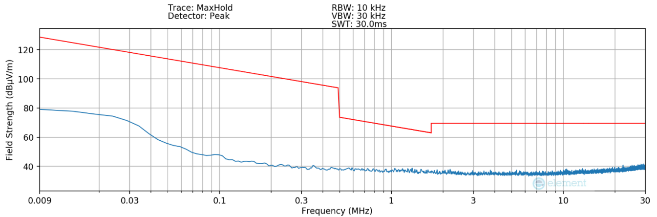
Plot 7-14Radiated Spurious Plot 9kHz – 30MHz (Pol. Y – Digitizer – Hover)
