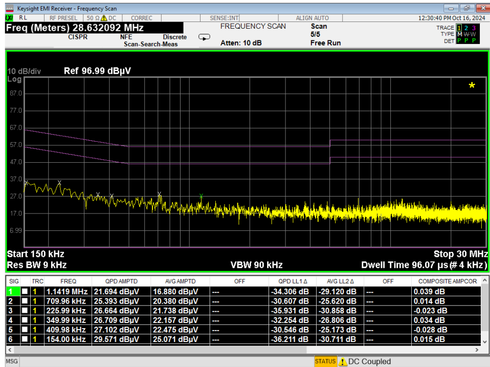
Plot 7-25. Line-Conducted Test Plot (L1) – Digitizer (Eraser)
