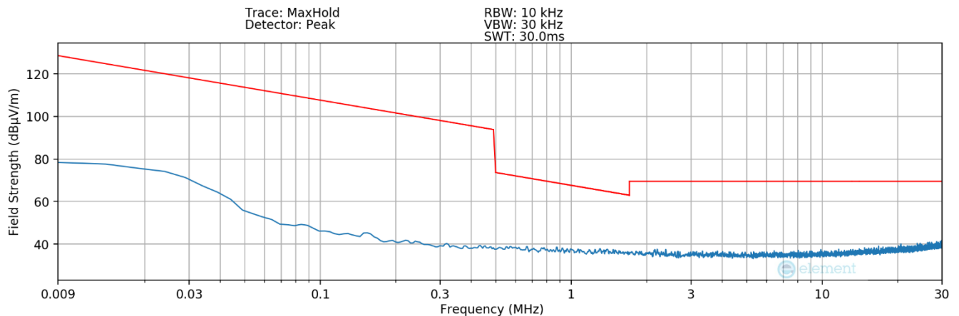
Plot 7-15. Radiated Spurious Plot 9kHz – 30MHz (Pol. Z – Digitizer – Hover)
