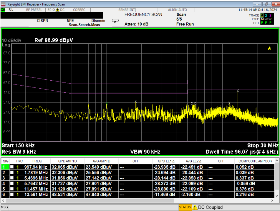
Plot 7-19. Line-Conducted Test Plot (L1) – Device to Device
