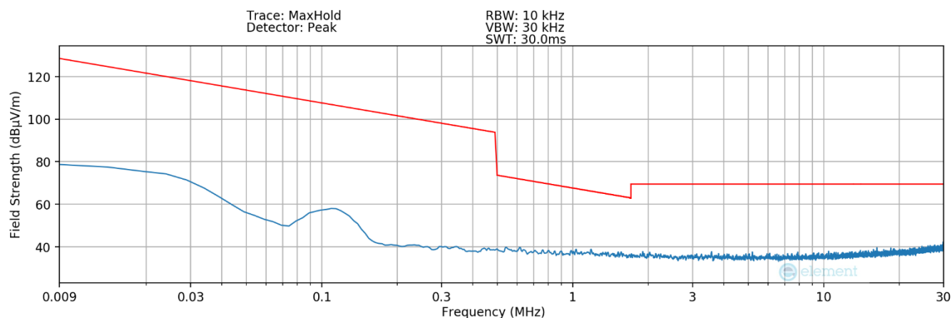
Plot 7-9. Radiated Spurious Plot 9kHz – 30MHz (Pol. Z– Device to Device)
