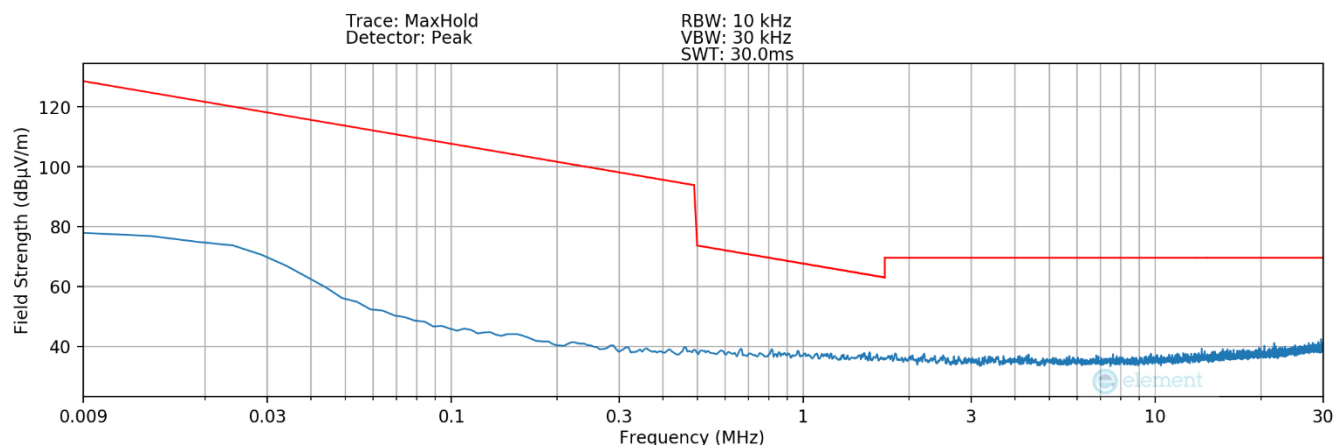
Plot 7-12. Radiated Spurious Plot 9kHz – 30MHz (Pol. Z– Digitizer – Click)
