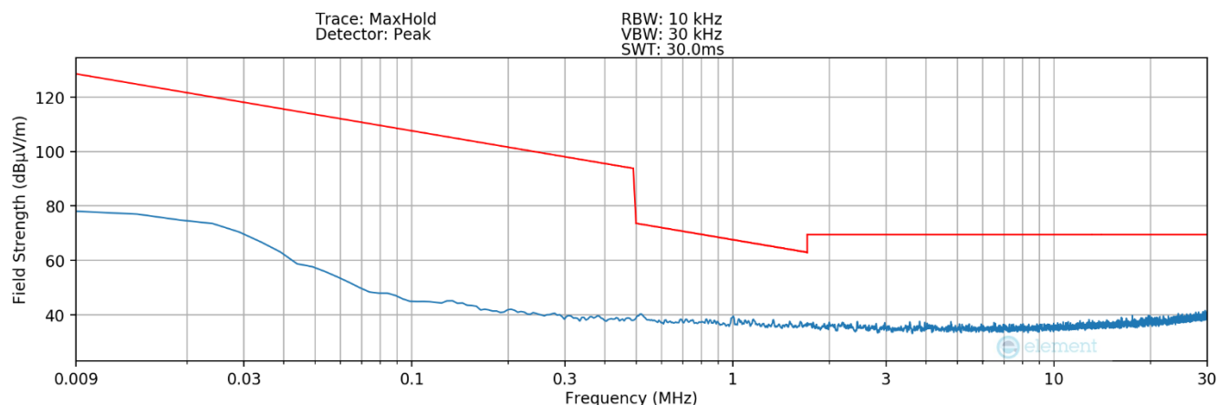
Plot 7-11 Radiated Spurious Plot 9kHz – 30MHz (Pol. Y – Digitizer – Click)
