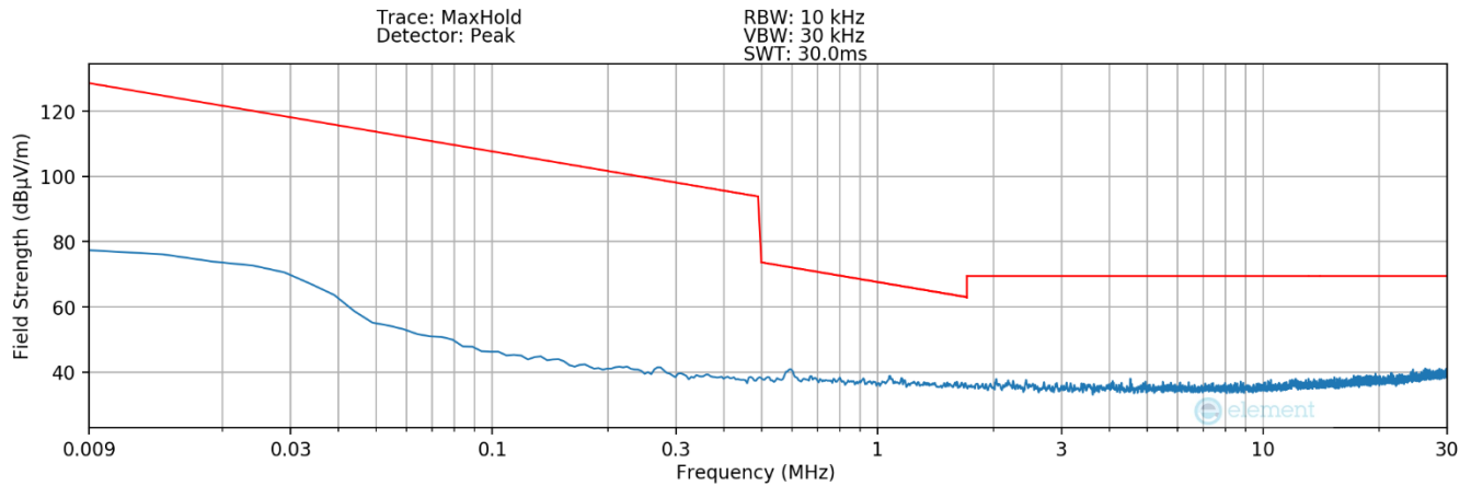
Plot 7-17Radiated Spurious Plot 9kHz – 30MHz (Pol. Y – Digitizer – Eraser)
