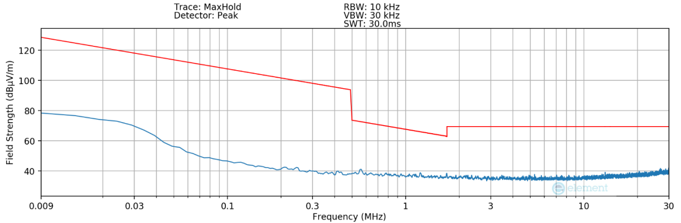
Plot 7-13. Radiated Spurious Plot 9kHz – 30MHz (Pol. X – Digitizer – Hover)
