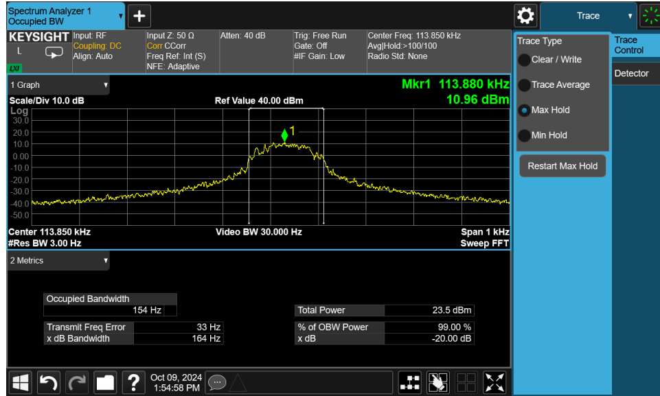
Plot 7-3. Occupied Bandwidth Measurement – Device to Device
