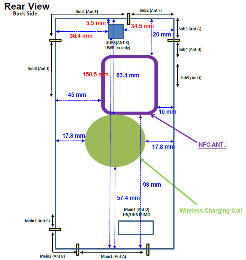
Figure D-2 NFC Antenna Locations
