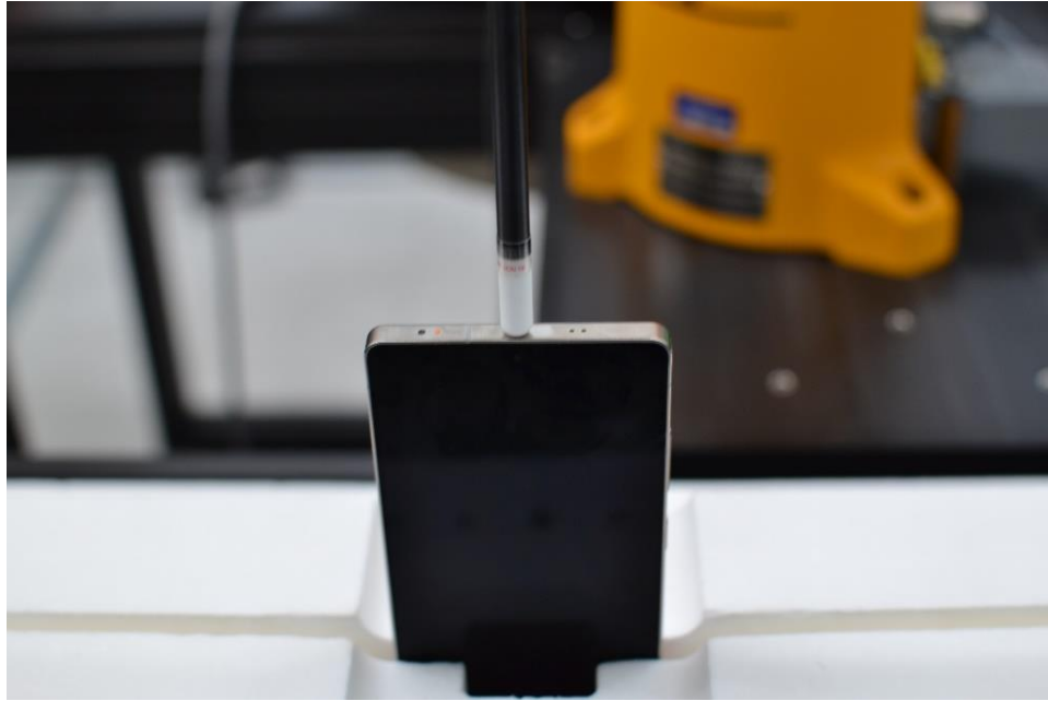
SAR Test Setup Photo 19 – PD, Top Edge at 2mm
