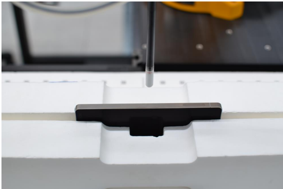
SAR Test Setup Photo 21 – PD, Left Edge at 8.78mm
