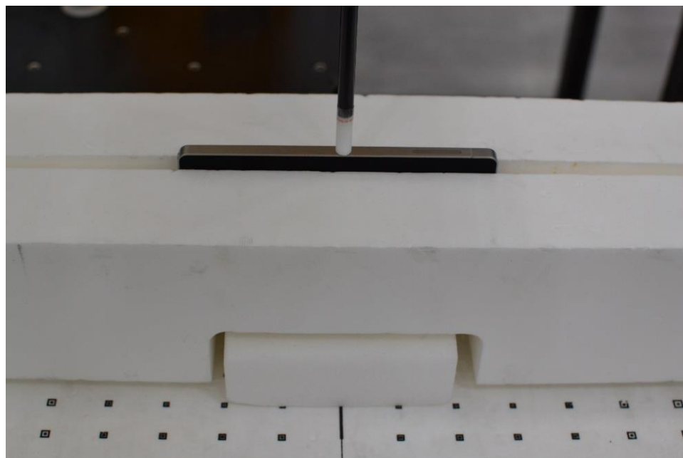
SAR Test Setup Photo 20 – PD, Left Edge at 2mm
