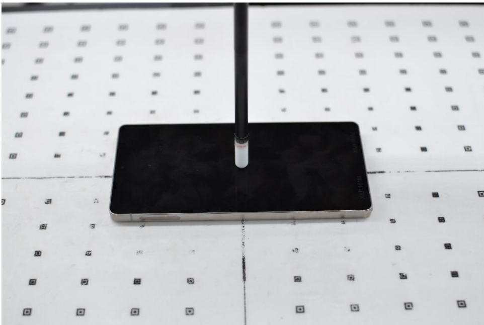
SAR Test Setup Photo 18 – PD, Front Side at 2mm
