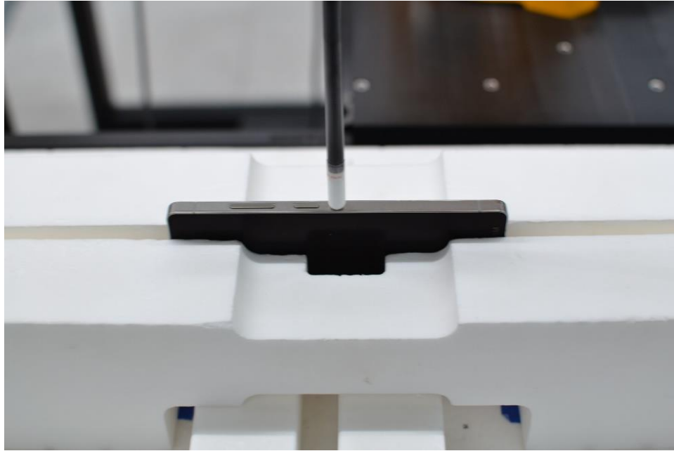
SAR Test Setup Photo 23 – PD, Right Edge at 2mm
