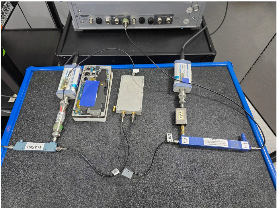
Test Setup Photo 6 – Conducted Test Setup (Figure 5-1c)
