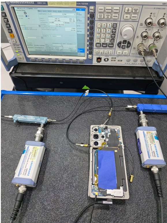
Test Setup Photo 9 – Conducted Test Setup (Figure 5-1e)
