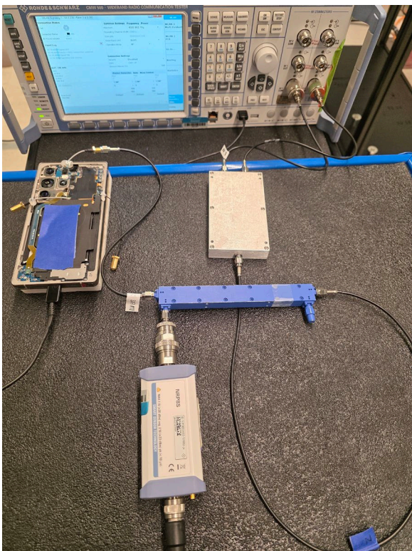
Test Setup Photo 11 – Conducted Test Setup (Figure 5-1g)
