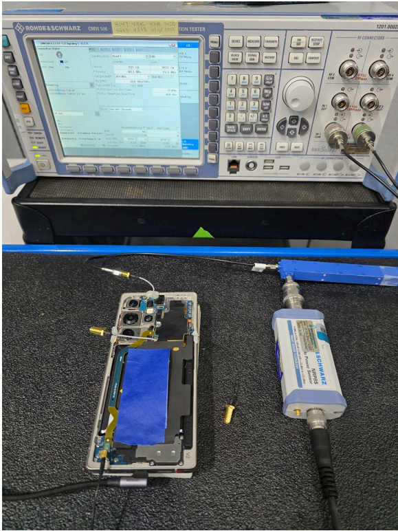
Test Setup Photo 8 – Conducted Test Setup (Figure 5-1d)
