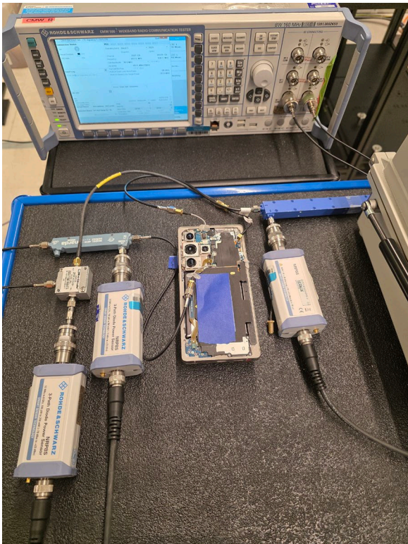
Test Setup Photo 10 – Conducted Test Setup (Figure 5-1f)
