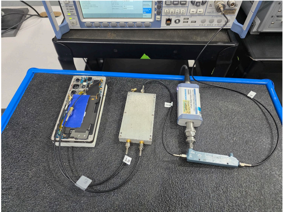
Test Setup Photo 5 – Conducted Test Setup (Figure 5-1b)
