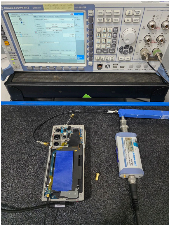
Test Setup Photo 7 – Conducted Test Setup (Figure 5-1d)
