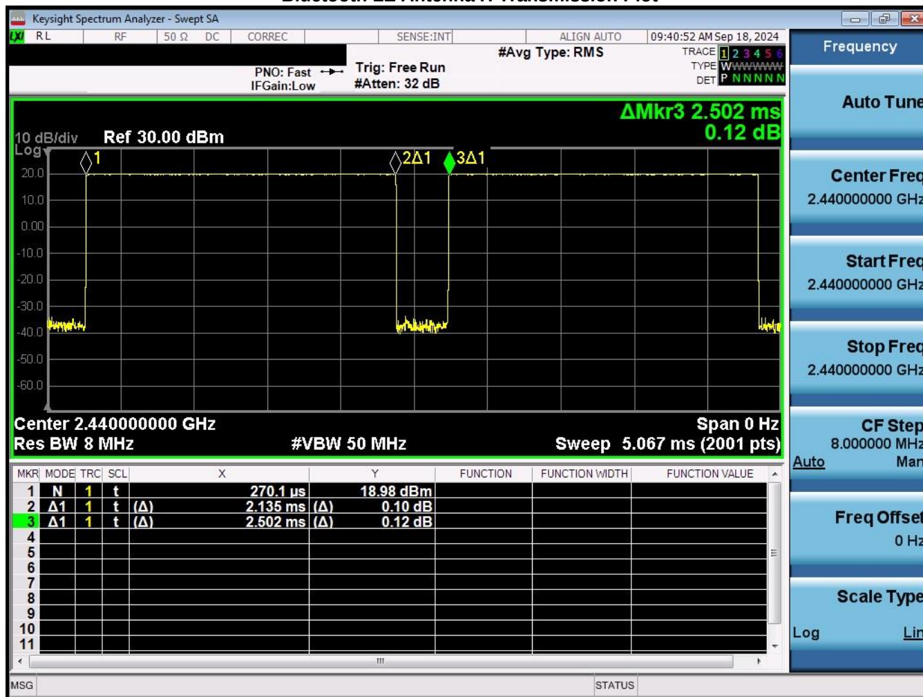
Figure 10-11 Bluetooth LE Antenna H Transmission Plot
