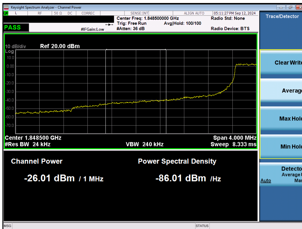
Plot 7-141. Extended Lower Band Edge Plot (LTE Band 25/2 - 3MHz QPSK – Full RB - Ant2)
