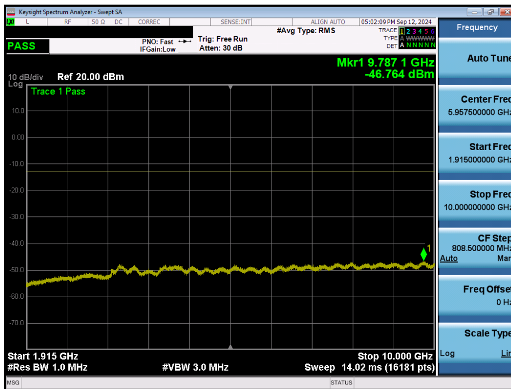
Plot 7-113. Conducted Spurious Plot (LTE Band 25/2 - 20MHz QPSK - 1RB - Low Channel - Ant2)
