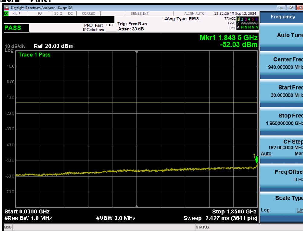
Plot 7-103. Conducted Spurious Plot (NR Band n25/2 -40.0MHz - 1RB - Low Channel - Ant1)
