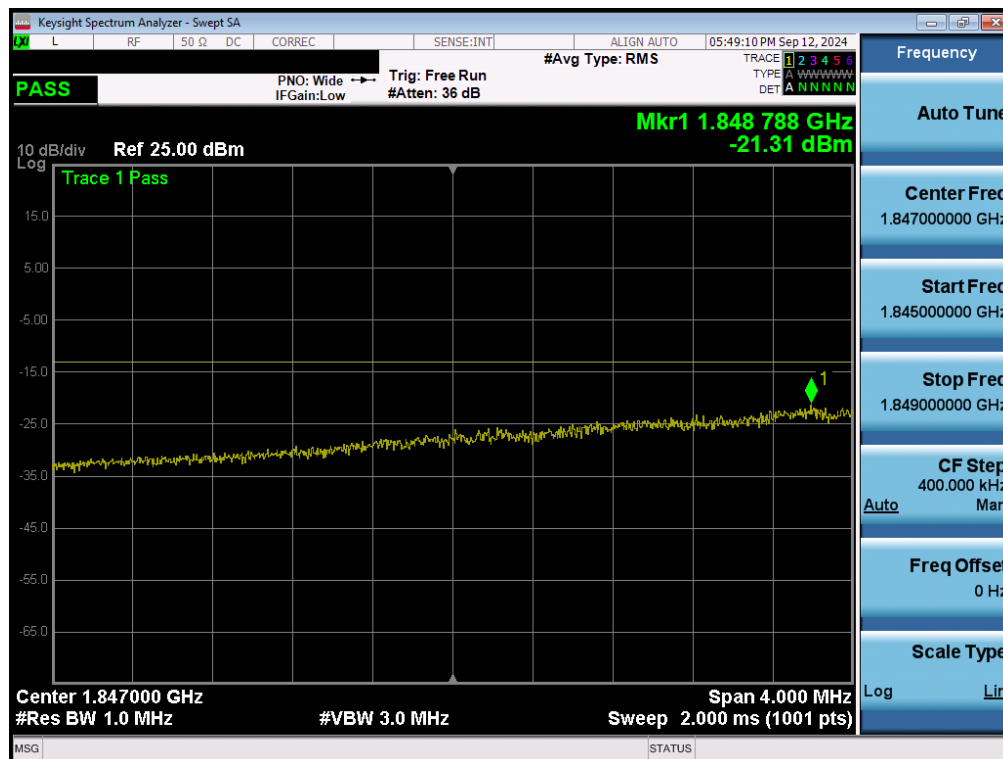
Plot 7-135. Extended Lower Band Edge Plot (LTE Band 25/2 - 10MHz QPSK – Full RB - Ant1)
