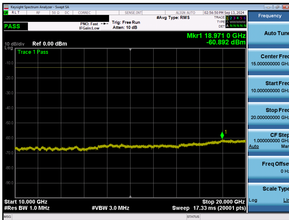
Plot 7-126. Conducted Spurious Plot (NR Band n25/2 - 40.0MHz - 1RB - Mid Channel - Ant2)
