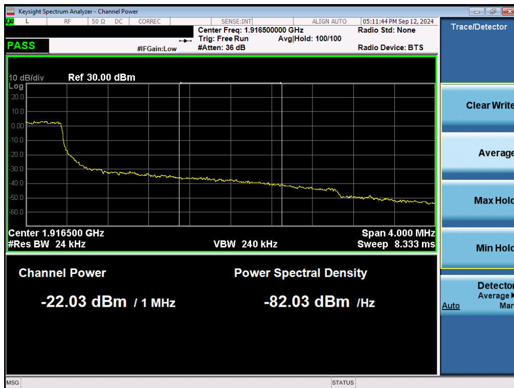
Plot 7-145. Extended Upper Band Edge Plot (LTE Band 25 - 3MHz QPSK – Full RB - Ant2)
