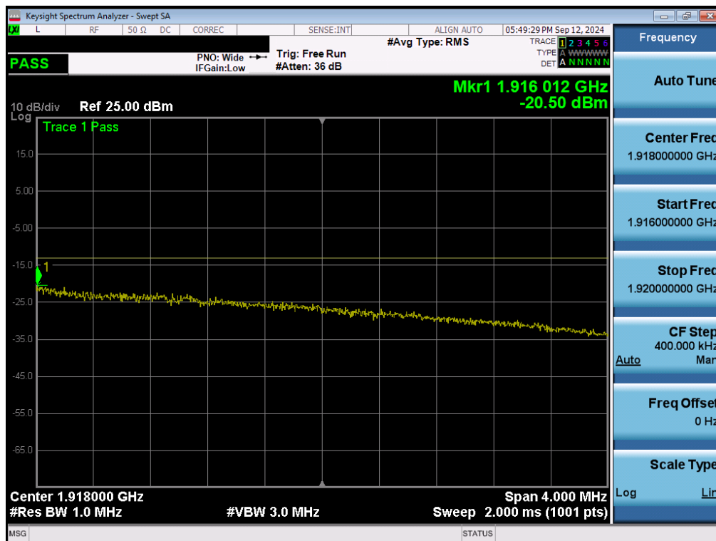
Plot 7-139. Extended Upper Band Edge Plot (LTE Band 25 - 10MHz QPSK - Full RB - Ant1)
