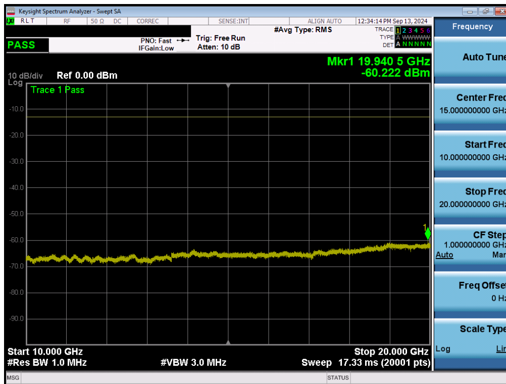
Plot 7-108. Conducted Spurious Plot (NR Band n25/2 - 40.0MHz - 1RB - Mid Channel - Ant1)
