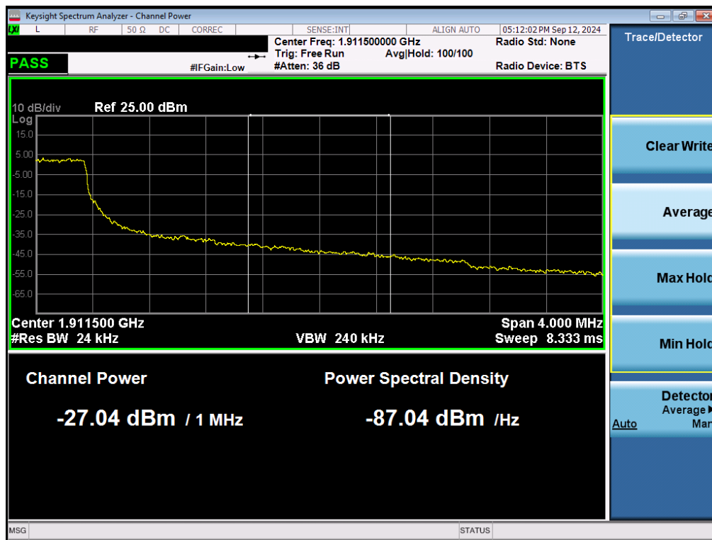
Plot 7-143. Extended Upper Band Edge Plot (LTE Band 2 - 3MHz QPSK – Full RB - Ant2)
