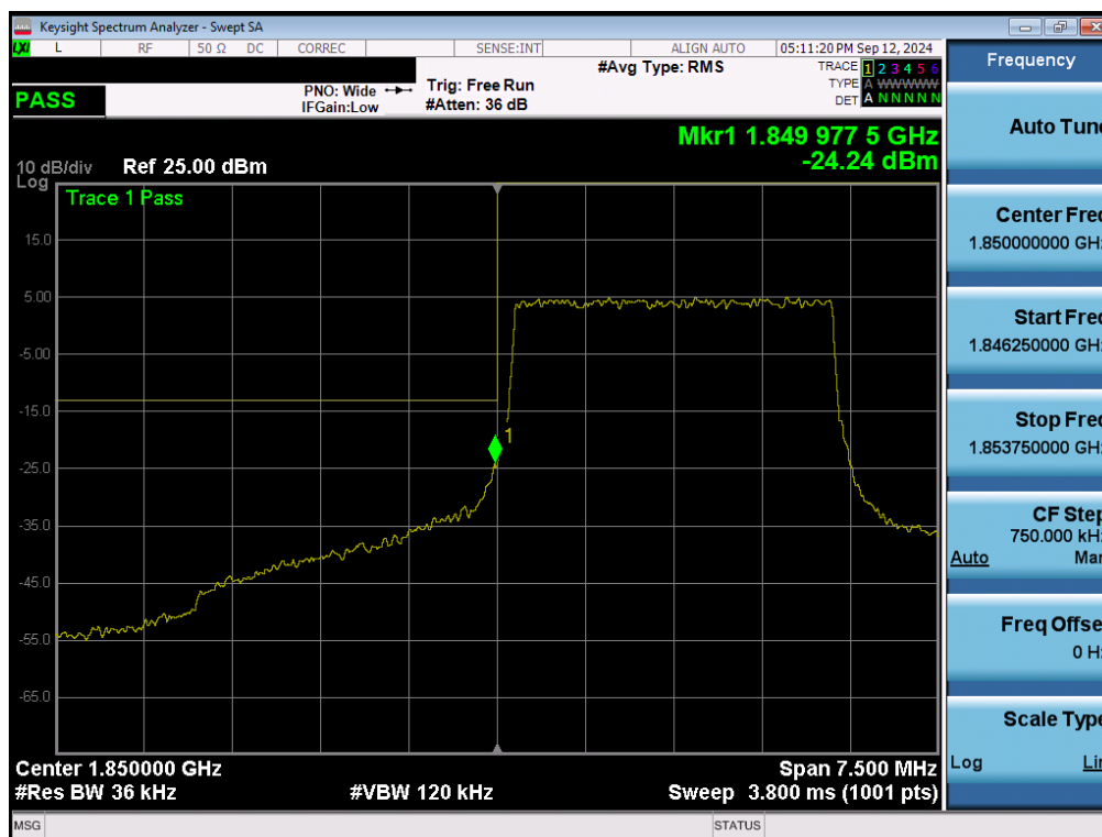
Plot 7-140. Lower Band Edge Plot (LTE Band 25/2 - 3MHz QPSK – Full RB - Ant2)
