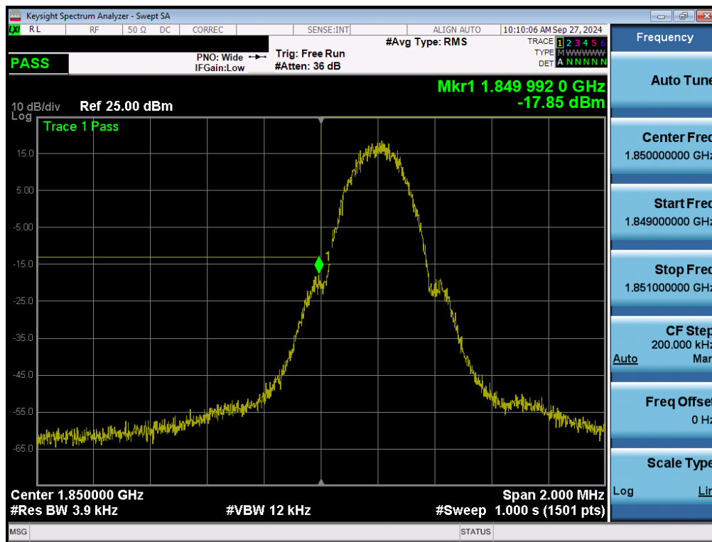
Plot 7-130. Lower Band Edge Plot (GPRS PCS – Ch. 512 - Ant1)
