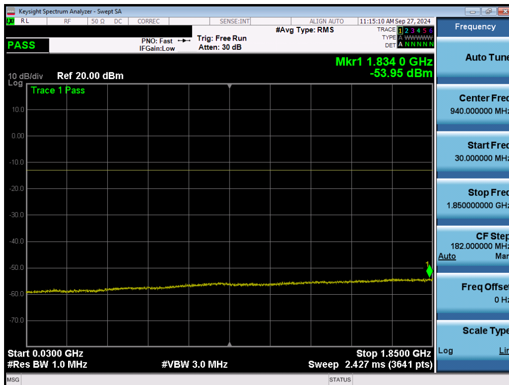
Plot 7-88. Conducted Spurious Plot (WCDMA Ch. 9400 - Ant1)
