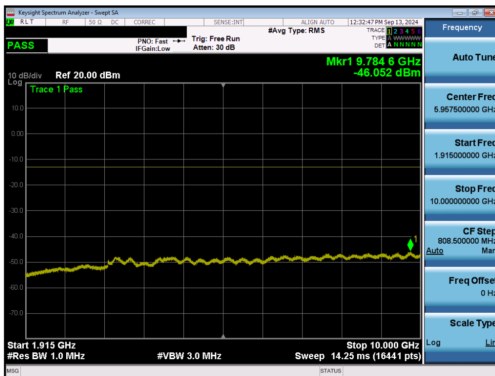
Plot 7-104. Conducted Spurious Plot (NR Band n25/2 - 40.0MHz - 1RB - Low Channel - Ant1)
