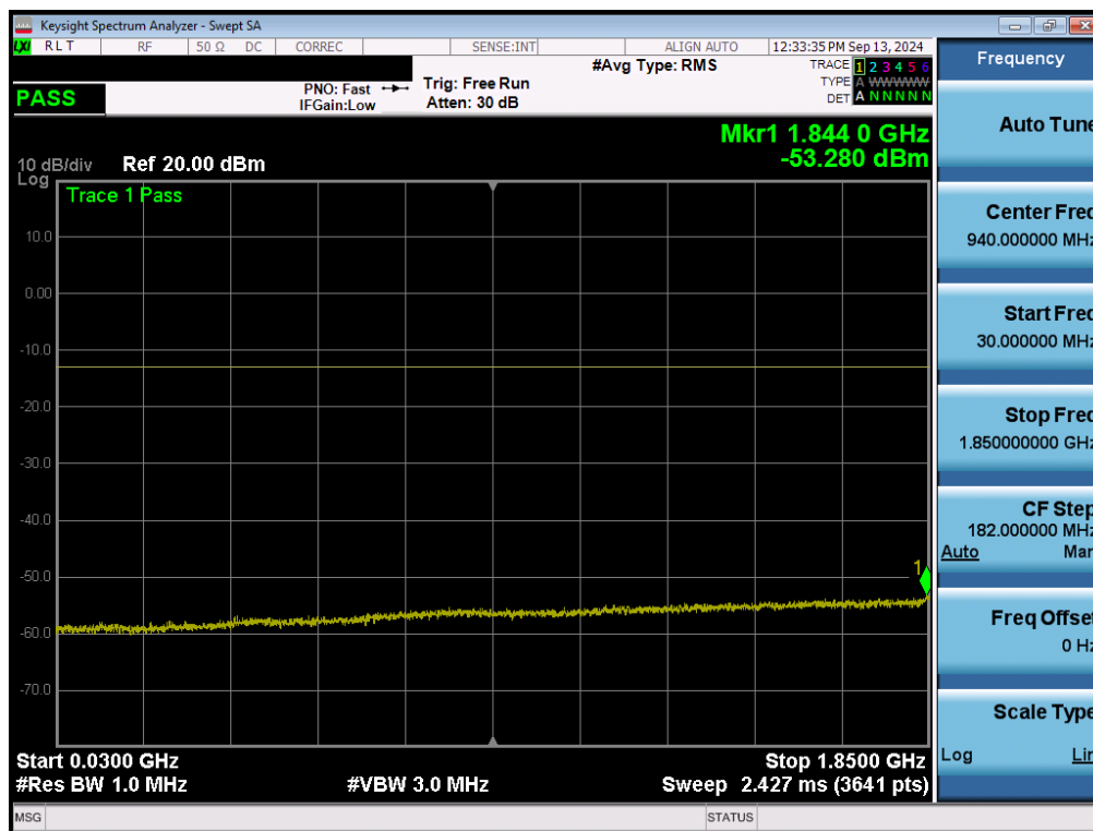
Plot 7-106. Conducted Spurious Plot (NR Band n25/2 - 40.0MHz - 1RB - Mid Channel - Ant1)
