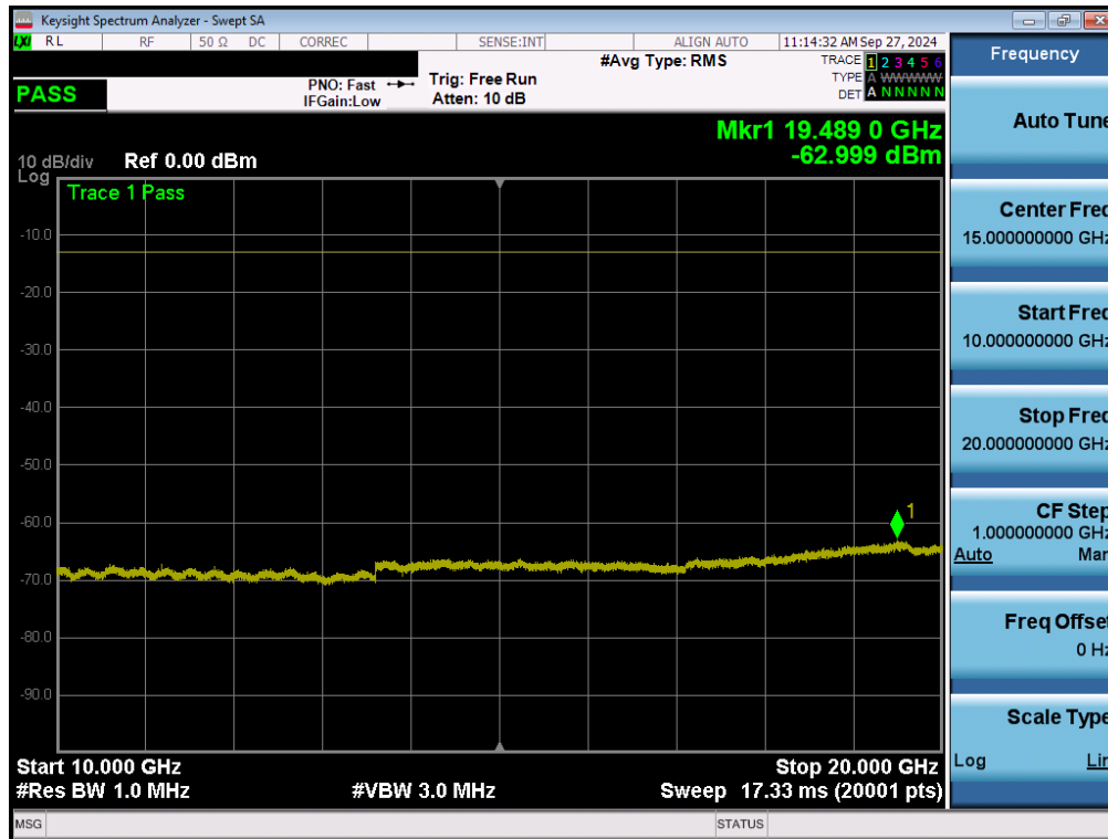
Plot 7-87. Conducted Spurious Plot (WCDMA Ch. 9262 - Ant1)
