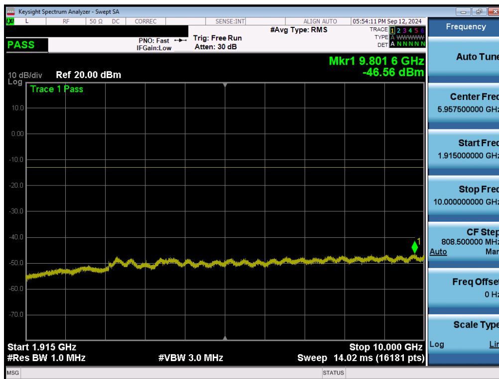
Plot 7-95. Conducted Spurious Plot (LTE Band 25/2 - 20MHz QPSK - 1RB - Low Channel - Ant1)
