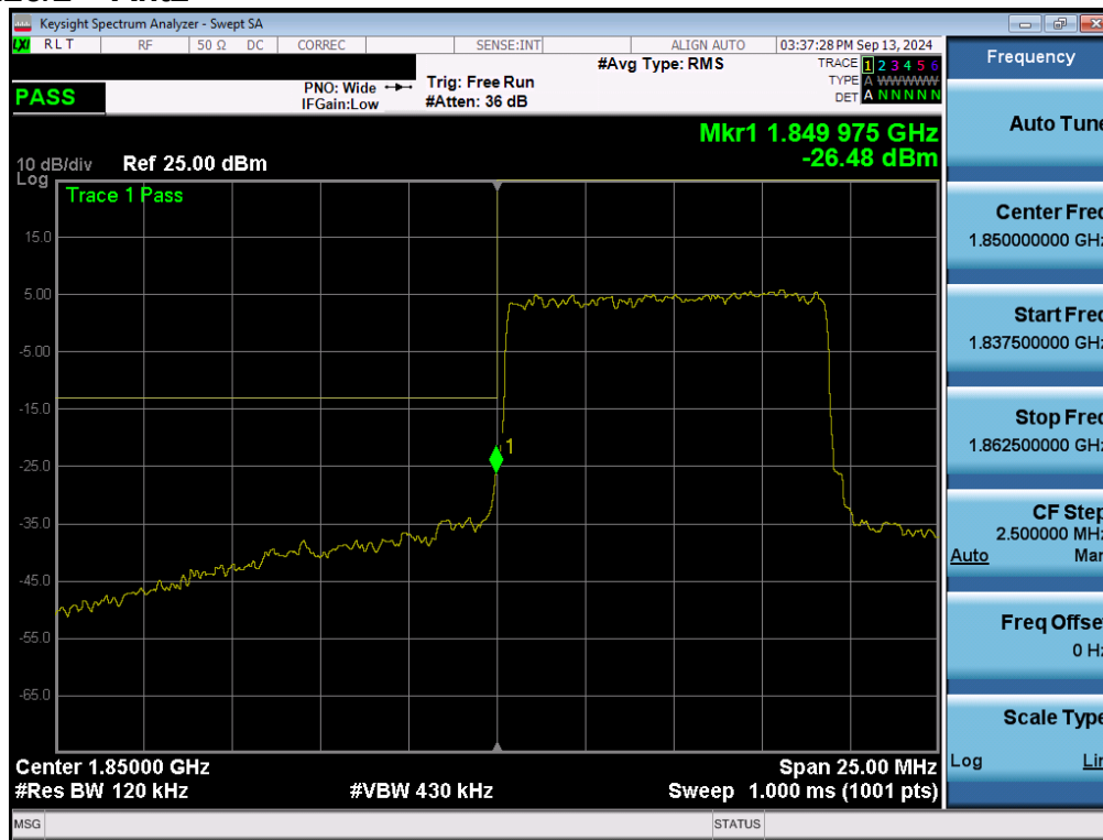
Plot 7-152. Lower Band Edge Plot (NR Band n25/2 - 10MHz QPSK – Full RB - Ant2)
