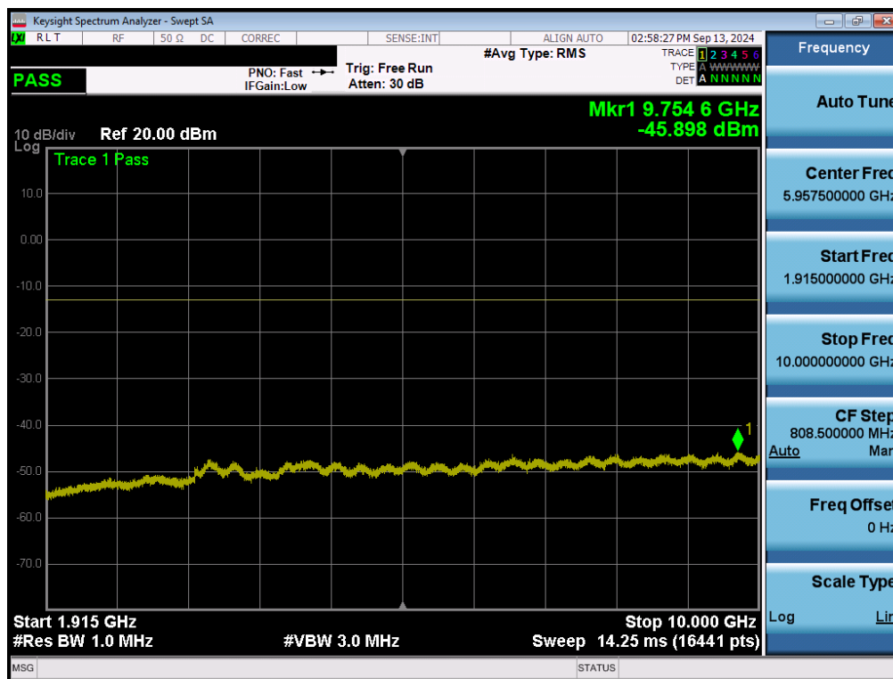
Plot 7-122. Conducted Spurious Plot (NR Band n25/2 - 40.0MHz - 1RB - Low Channel - Ant2)
