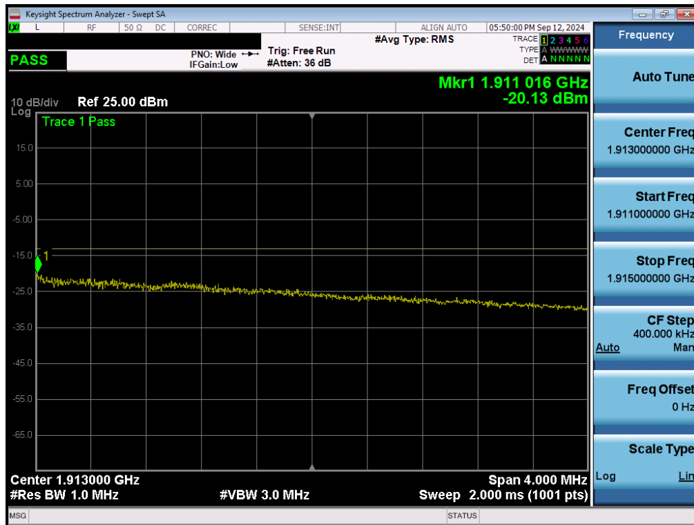
Plot 7-137. Extended Upper Band Edge Plot (LTE Band 2 - 10MHz QPSK – Full RB - Ant1)
