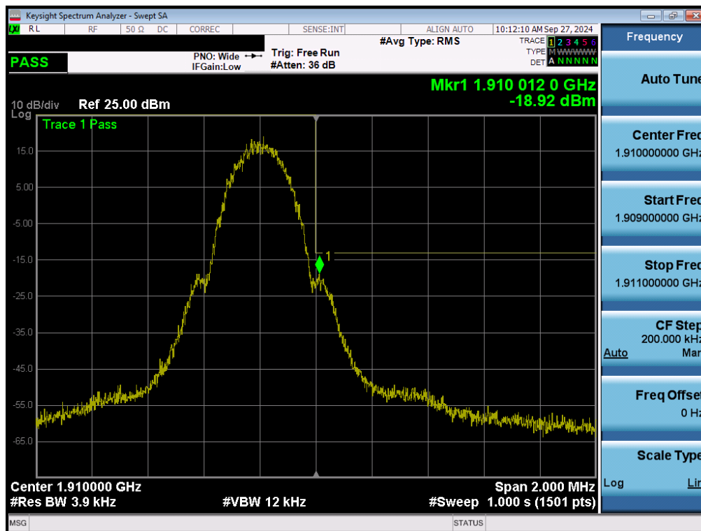
Plot 7-131. Upper Band Edge Plot (GPRS PCS – Ch. 810 - Ant1)
