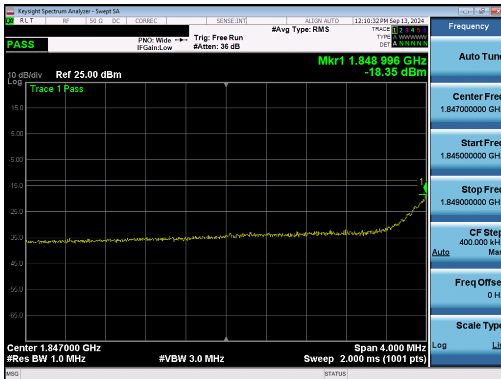
Plot 7-147. Extended Lower Band Edge Plot (NR Band n25/2 - 10MHz QPSK – Full RB - Ant1)
