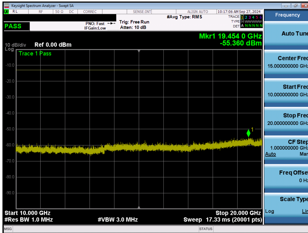
Plot 7-84. Conducted Spurious Plot (GPRS Ch. 810 - Ant1)
