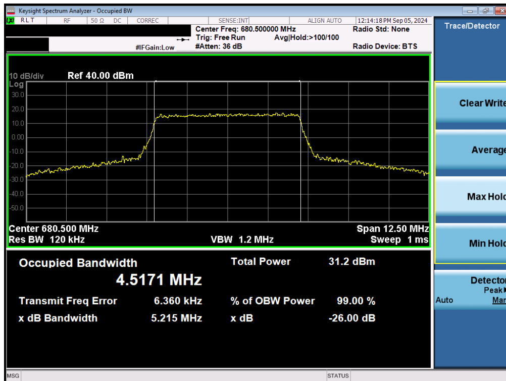
Plot 7-107. Occupied Bandwidth Plot (LTE Band 71 - 5MHz 16-QAM - Full RB – ANT2)
