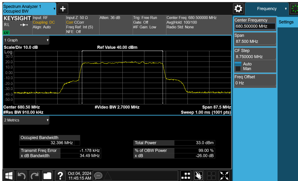
Plot 7-141. Occupied Bandwidth Plot (NR Band n71 - 35MHz DFT-s-OFDM BPSK - Full RB – ANT2)
