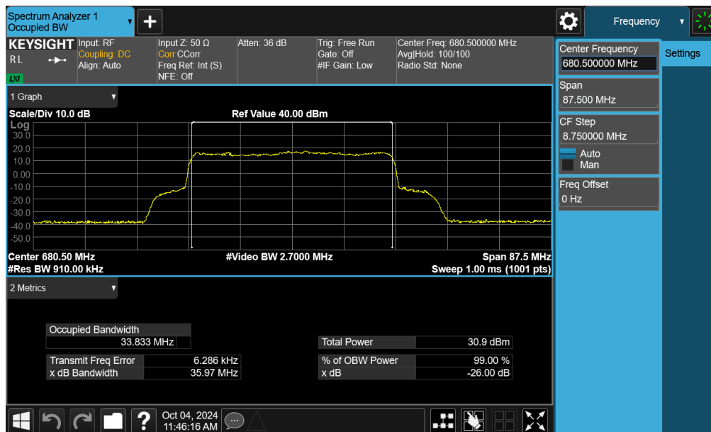
Plot 7-142. Occupied Bandwidth Plot (NR Band n71 - 35MHz CP-OFDM QPSK - Full RB – ANT2)
