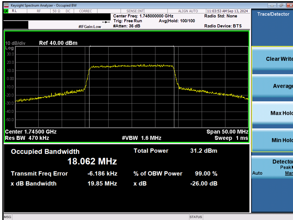
Plot 7-121. Occupied Bandwidth Plot (LTE Band 66/4 - 20MHz 16-QAM - Full RB - ANT2)
