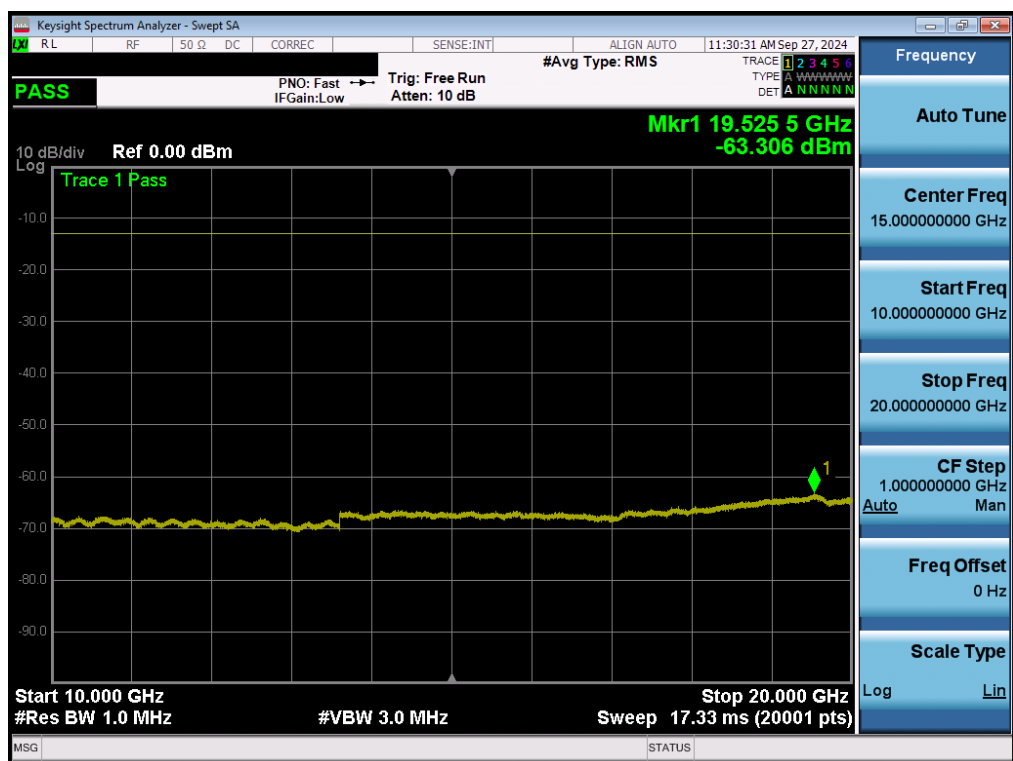
Plot 7-200. Conducted Spurious Plot (WCDMA-AWS - 5MHz QPSK - 1 RB - Low Channel)
