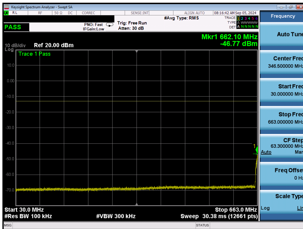
Plot 7-201. Conducted Spurious Plot (LTE Band 71 - 20MHz QPSK - 1 RB - High Channel - ANT1)
