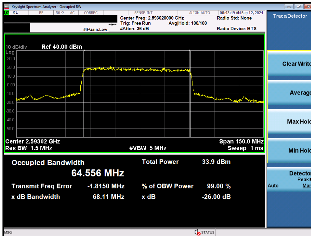
Plot 7-81. Occupied Bandwidth Plot (NR Band n41 - 70MHz 7 \pi /2 BPSK - Full RB - Ant F)
