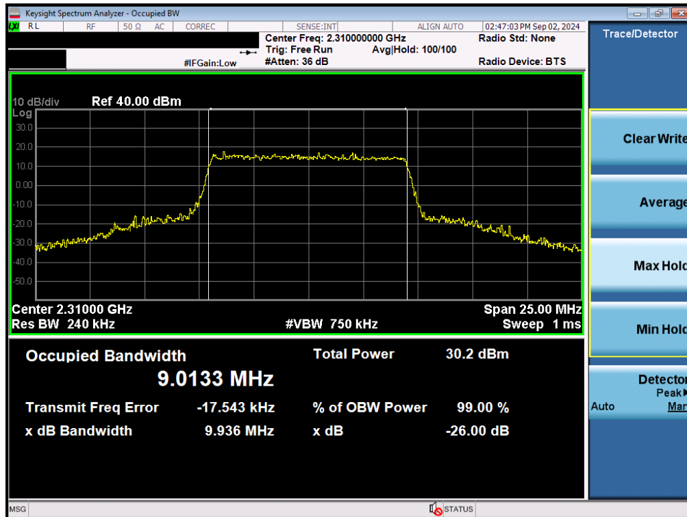
Plot 7-20. Occupied Bandwidth Plot (LTE Band 30 - 10MHz 16-QAM - Full RB - Ant A)
