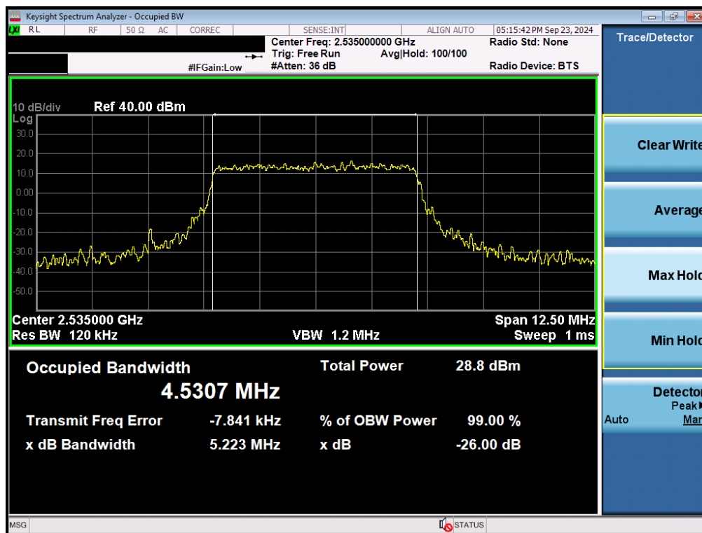
Plot 7-71. Occupied Bandwidth Plot (NR Band n7 - 5MHz 16-QAM - Full RB - Ant F)
