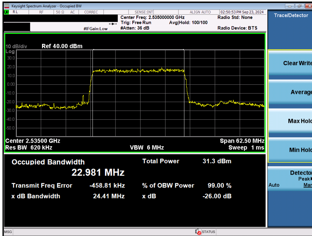
Plot 7-57. Occupied Bandwidth Plot (NR Band n7 - 25MHz \pi/2 BPSK - Full RB - Ant F)
