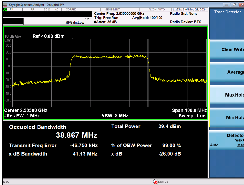
Plot 7-49. Occupied Bandwidth Plot (NR Band n7 - 40MHz QPSK - Full RB - Ant F)
