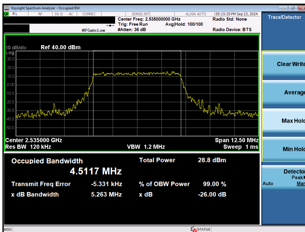
Plot 7-70. Occupied Bandwidth Plot (NR Band n7 - 5MHz QPSK - Full RB - Ant F)
