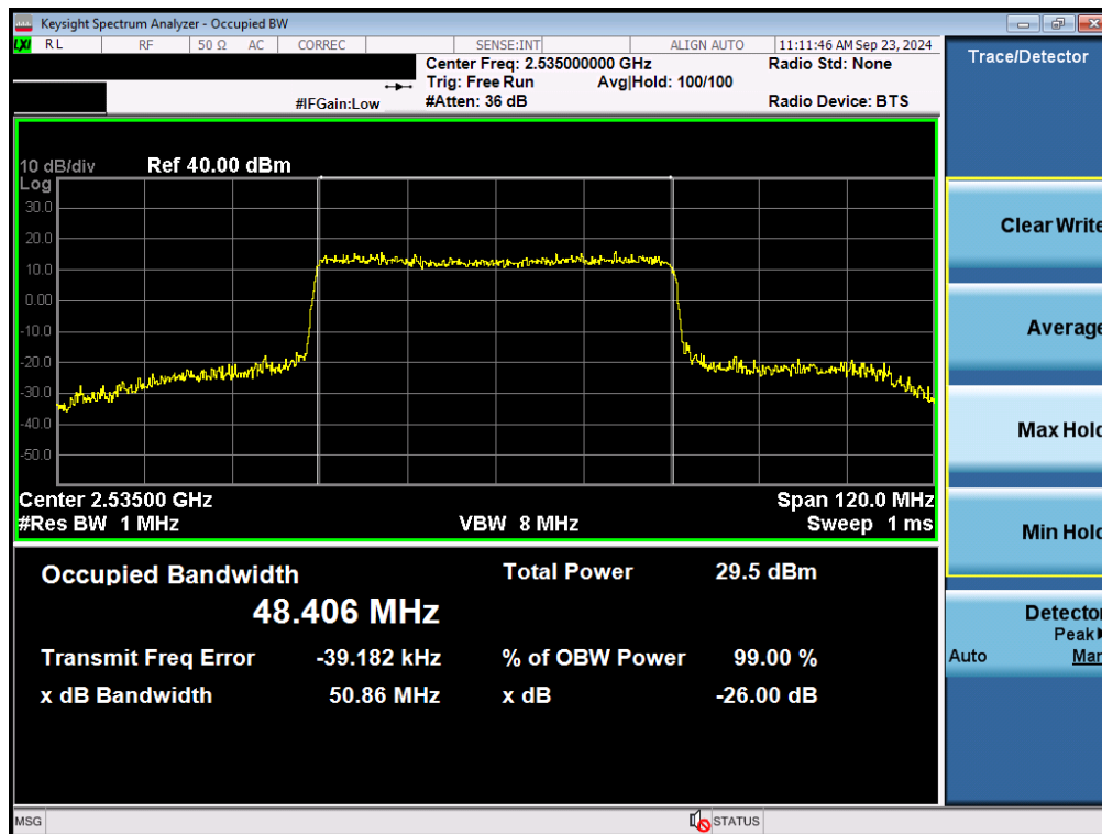
Plot 7-46. Occupied Bandwidth Plot (NR Band n7 - 50MHz QPSK - Full RB - Ant F)
