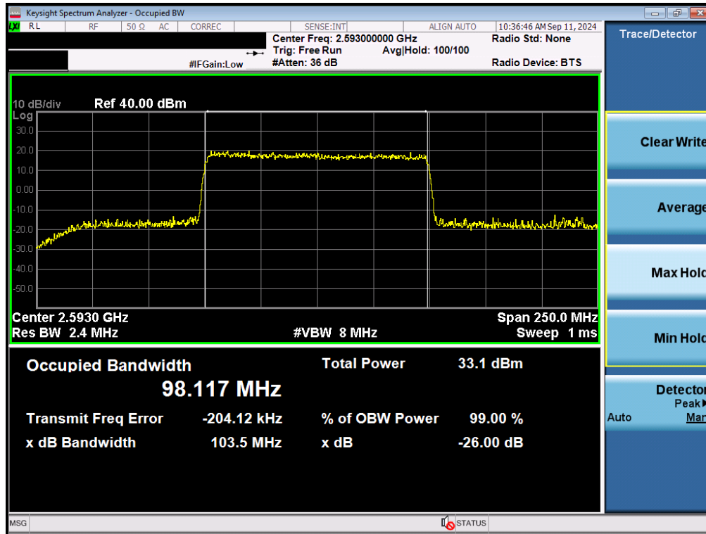
Plot 7-116. Occupied Bandwidth Plot (NR Band n41 - 100MHz 16-QAM - Full RB - Ant B)
