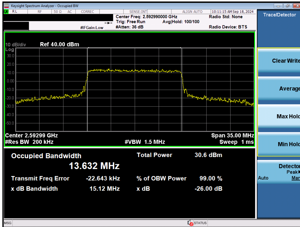
Plot 7-109. Occupied Bandwidth Plot (NR Band n41 - 15MHz QPSK - Full RB - Ant F)
