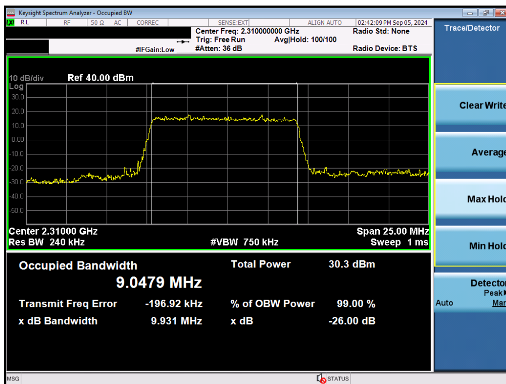
Plot 7-39. Occupied Bandwidth Plot (NR Band n30 - 10MHz \pi/2 BPSK - Full RB - Ant F)
