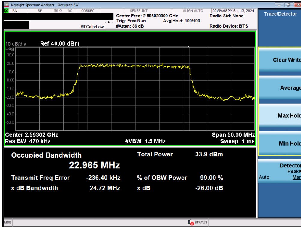
Plot 7-102. Occupied Bandwidth Plot (NR Band n41 - 25MHz \pi/2 BPSK - Full RB - Ant F)
