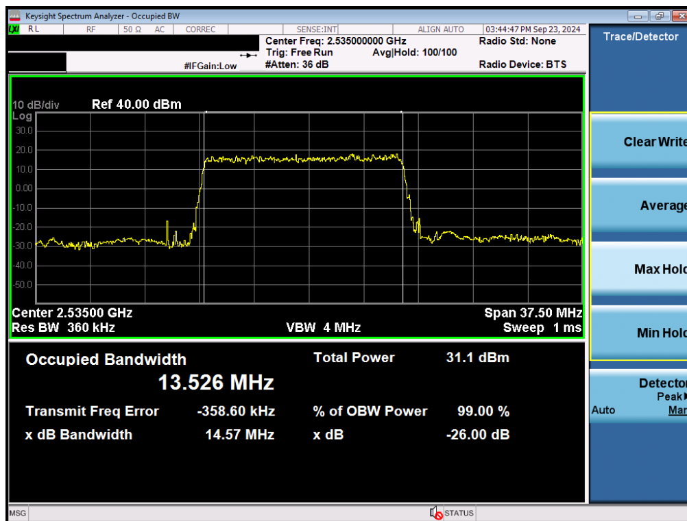
Plot 7-63. Occupied Bandwidth Plot (NR Band n7 - 15MHz \pi/2 BPSK - Full RB - Ant F)
