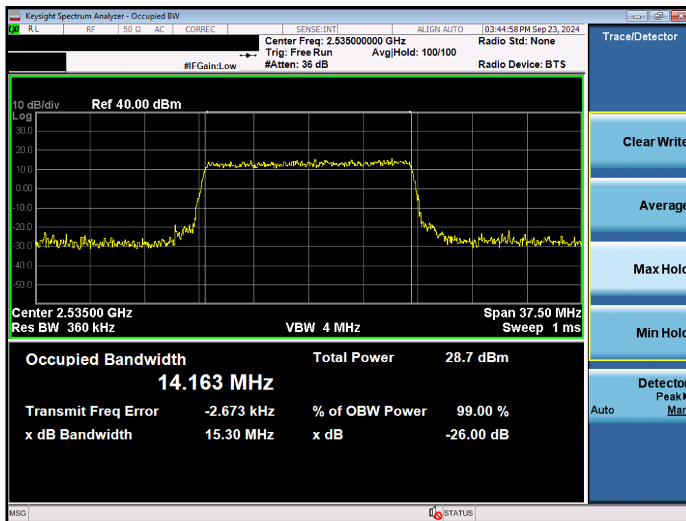
Plot 7-64. Occupied Bandwidth Plot (NR Band n7 - 15MHz QPSK - Full RB - Ant F)
