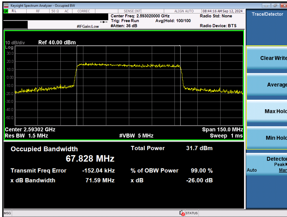
Plot 7-83. Occupied Bandwidth Plot (NR Band n41 - 70MHz 16-QAM - Full RB - Ant F)
