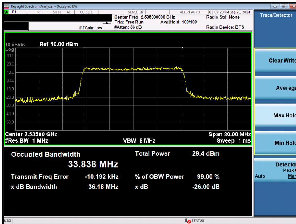
Plot 7-52. Occupied Bandwidth Plot (NR Band n7 - 35MHz QPSK - Full RB - Ant F)
