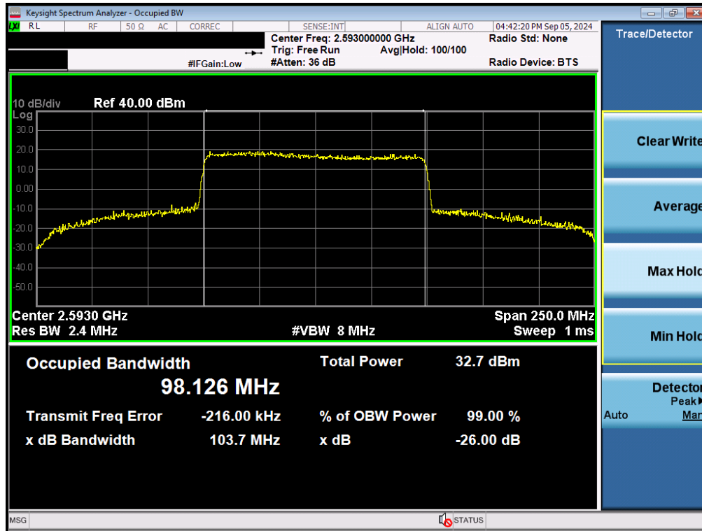
Plot 7-74. Occupied Bandwidth Plot (NR Band n41 - 100MHz 16-QAM - Full RB - Ant F)
