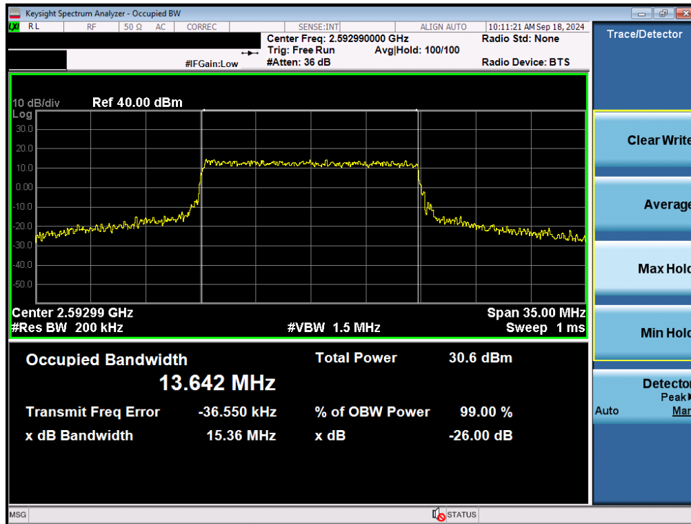
Plot 7-110. Occupied Bandwidth Plot (NR Band n41 - 15MHz 16-QAM - Full RB - Ant F)
