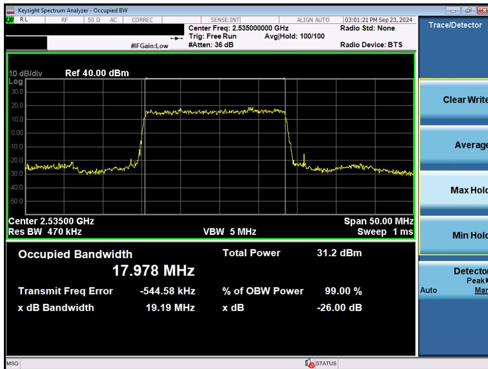
Plot 7-60. Occupied Bandwidth Plot (NR Band n7 - 20MHz \pi/2 BPSK - Full RB - Ant F)
