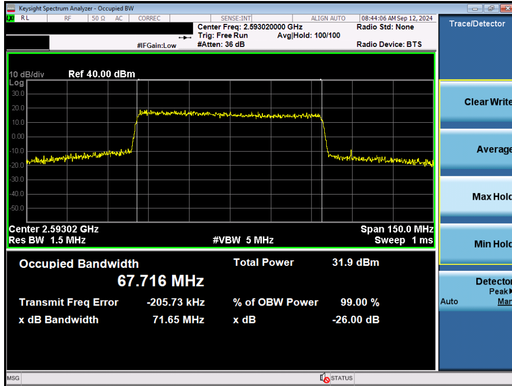
Plot 7-82. Occupied Bandwidth Plot (NR Band n41 - 70MHz QPSK - Full RB - Ant F)
