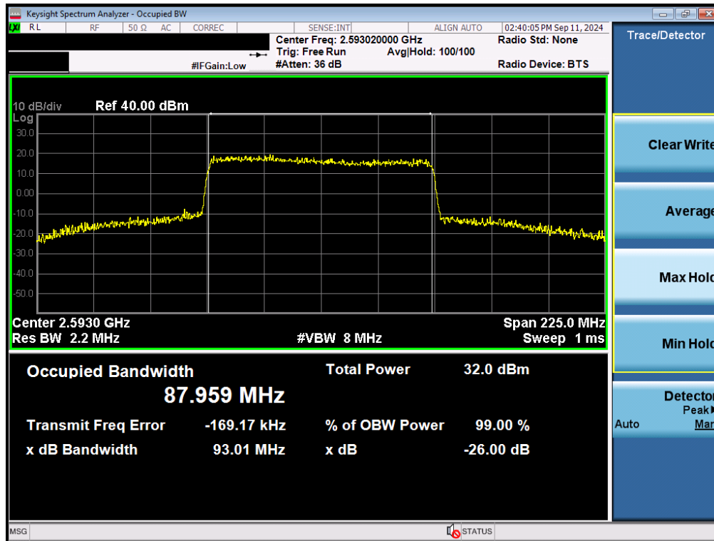
Plot 7-76. Occupied Bandwidth Plot (NR Band n41 - 90MHz QPSK - Full RB - Ant F)
