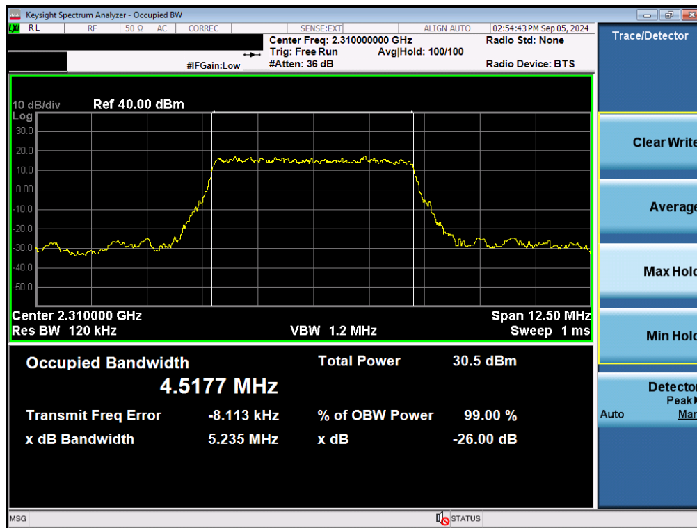
Plot 7-42. Occupied Bandwidth Plot (NR Band n30 - 5MHz \pi/2 BPSK - Full RB - Ant F)
