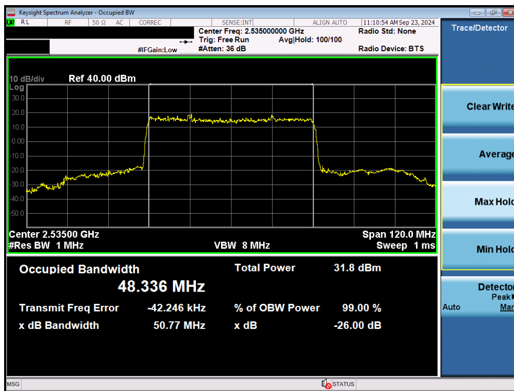
Plot 7-45. Occupied Bandwidth Plot (NR Band n7 - 50MHz \pi/2 BPSK - Full RB - Ant F)
