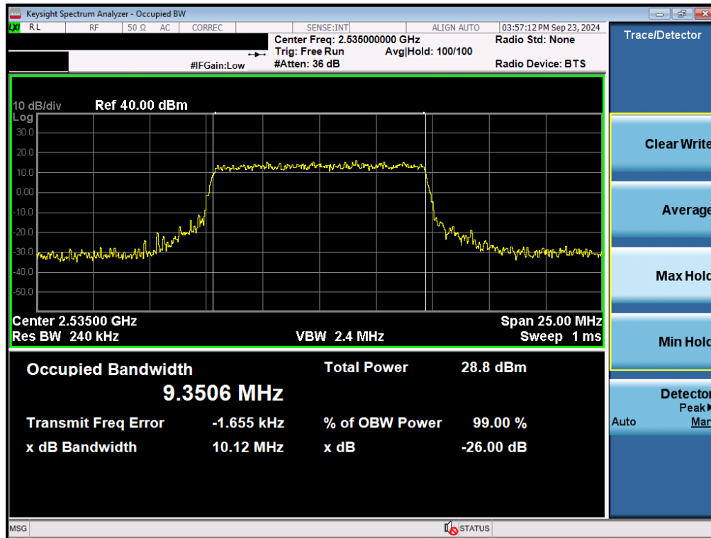
Plot 7-68. Occupied Bandwidth Plot (NR Band n7 - 10MHz 16-QAM - Full RB - Ant F)
