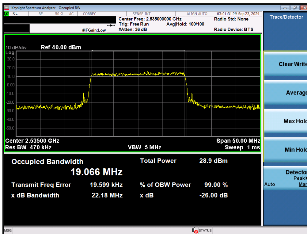
Plot 7-61. Occupied Bandwidth Plot (NR Band n7 - 20MHz QPSK - Full RB - Ant F)
