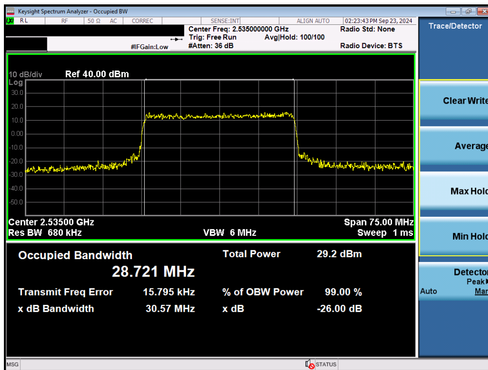
Plot 7-56. Occupied Bandwidth Plot (NR Band n7 - 30MHz 16-QAM - Full RB - Ant F)
