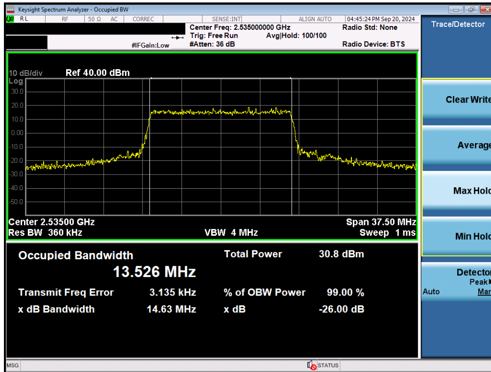
Plot 7-25. Occupied Bandwidth Plot (LTE Band 7 - 15MHz QPSK - Full RB - Ant B)
