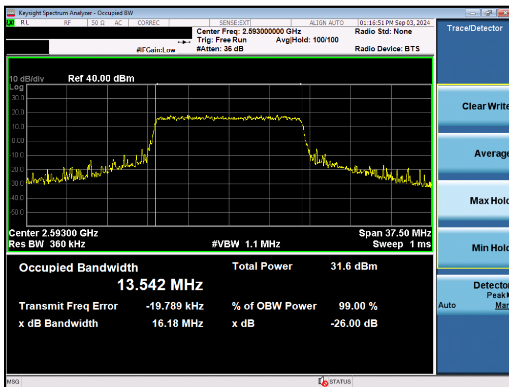
Plot 7-33. Occupied Bandwidth Plot (LTE Band 41(PC3)/38 - 15MHz QPSK - Full RB - Ant B)
