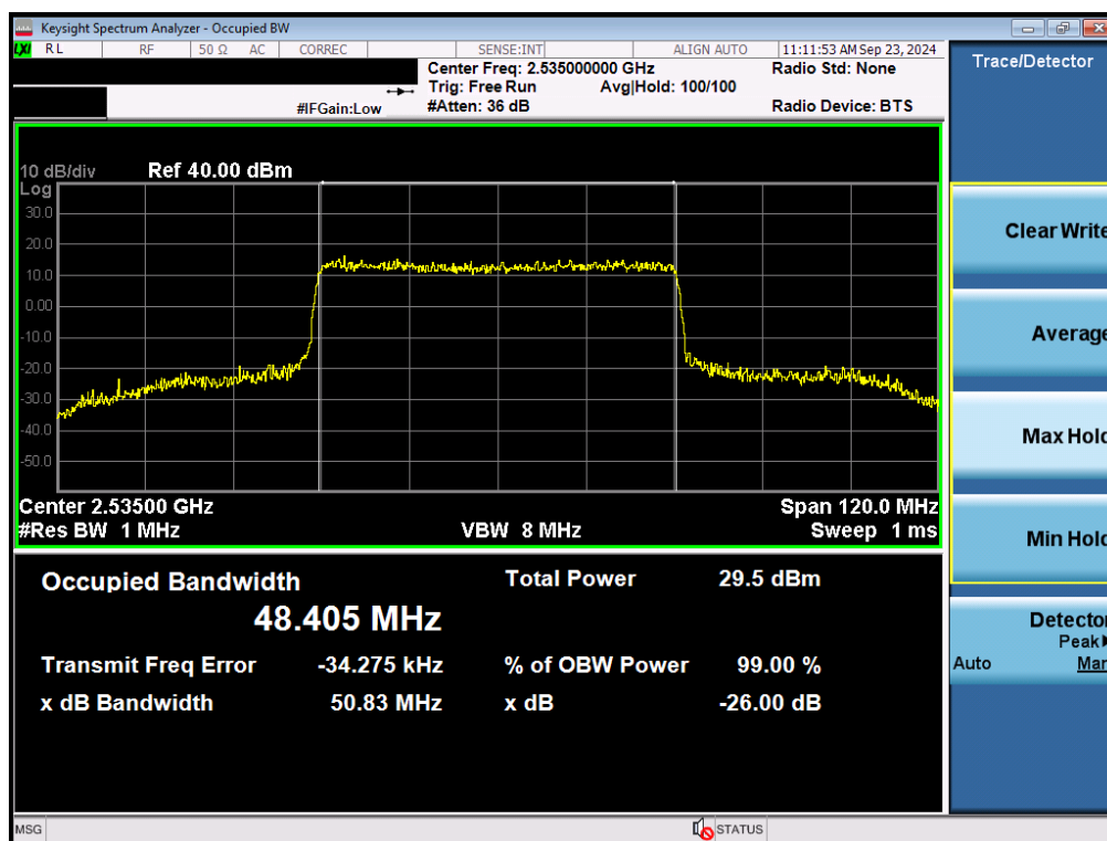
Plot 7-47. Occupied Bandwidth Plot (NR Band n7 - 50MHz 16-QAM - Full RB - Ant F)
