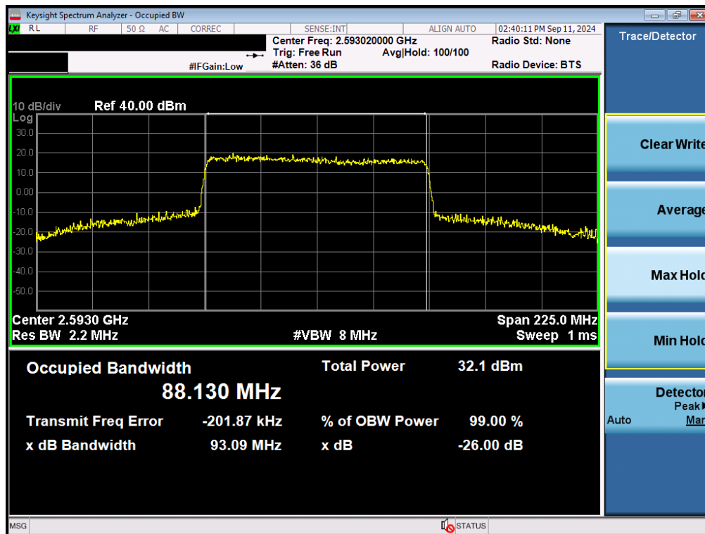
Plot 7-77. Occupied Bandwidth Plot (NR Band n41 - 90MHz 16-QAM - Full RB - Ant F)
