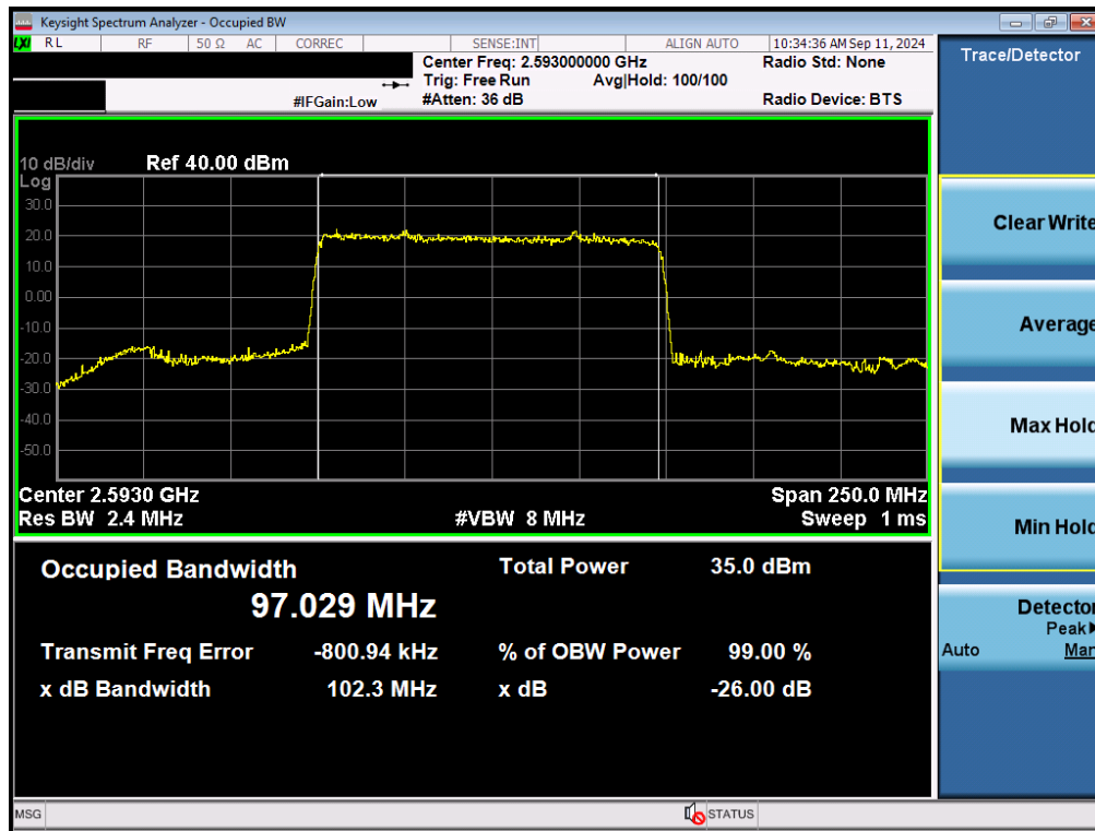
Plot 7-114. Occupied Bandwidth Plot (NR Band n41 - 100MHz \pi/2 BPSK - Full RB - Ant B)
