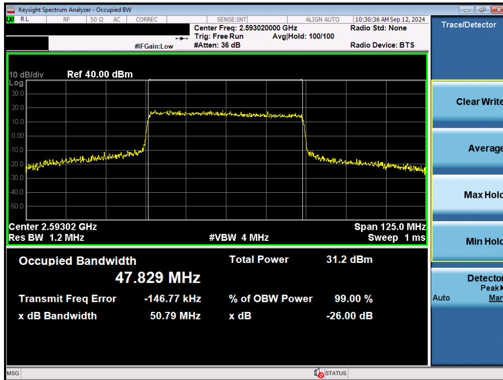
Plot 7-89. Occupied Bandwidth Plot (NR Band n41 - 50MHz 16-QAM - Full RB - Ant F)
