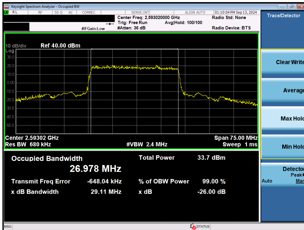
Plot 7-99. Occupied Bandwidth Plot (NR Band n41 - 30MHz \pi/2 BPSK - Full RB - Ant F)
