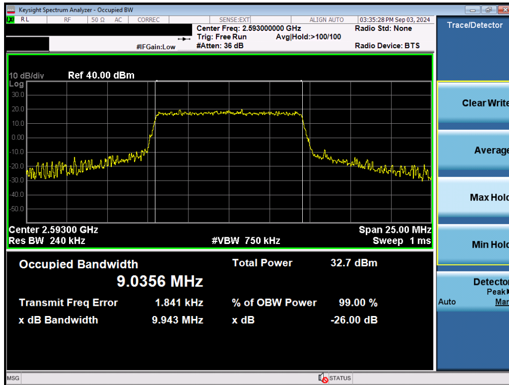
Plot 7-35. Occupied Bandwidth Plot (LTE Band 41(PC3)/38 - 10MHz QPSK - Full RB - Ant B)
