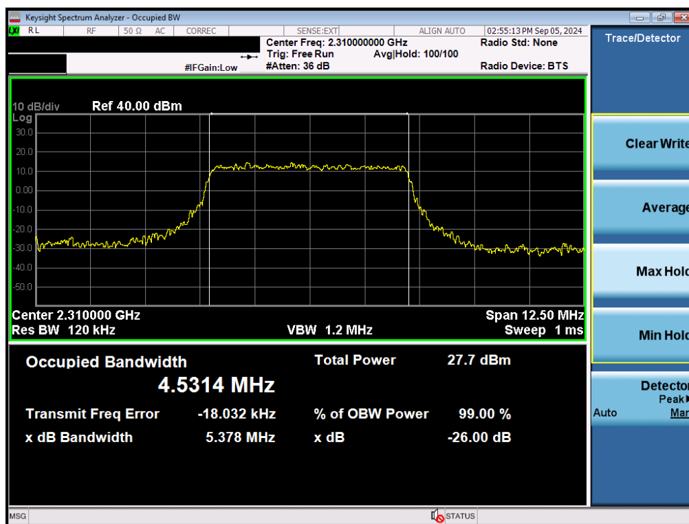
Plot 7-44. Occupied Bandwidth Plot (NR Band n30 - 5MHz 16-QAM - Full RB - Ant F)
