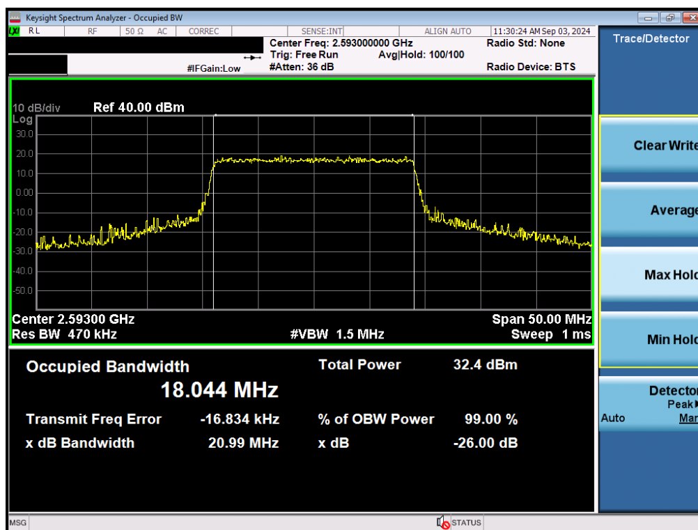
Plot 7-31. Occupied Bandwidth Plot (LTE Band 41(PC3)/38 - 20MHz QPSK - Full RB - Ant B)
