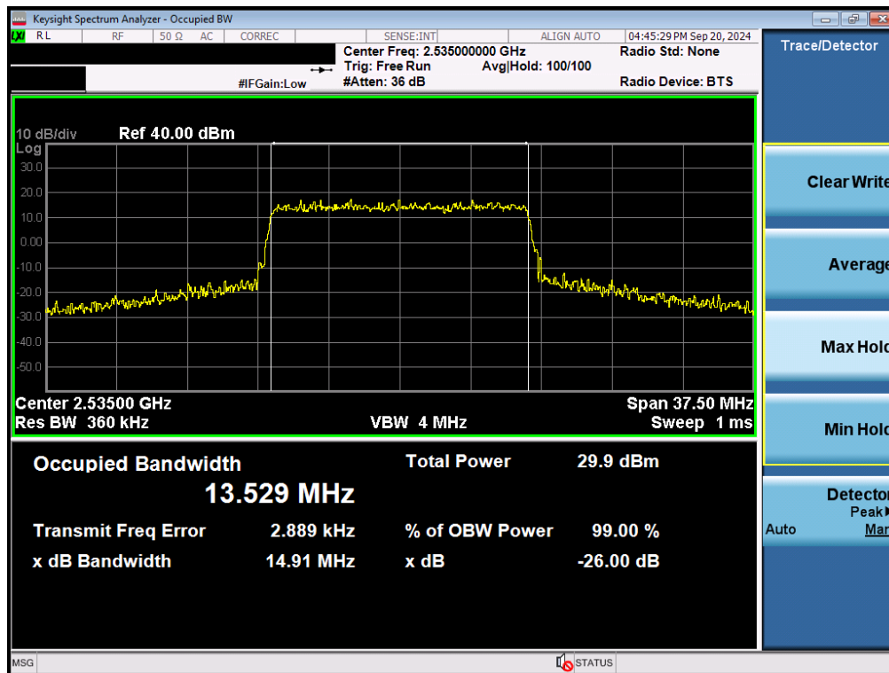
Plot 7-26. Occupied Bandwidth Plot (LTE Band 7 - 15MHz 16-QAM - Full RB - Ant B)
