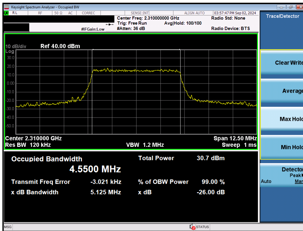
Plot 7-21. Occupied Bandwidth Plot (LTE Band 30 - 5MHz QPSK - Full RB - Ant A)
