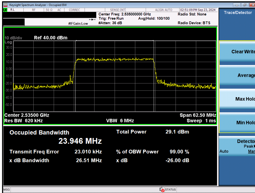
Plot 7-59. Occupied Bandwidth Plot (NR Band n7 - 25MHz 16-QAM - Full RB - Ant F)
