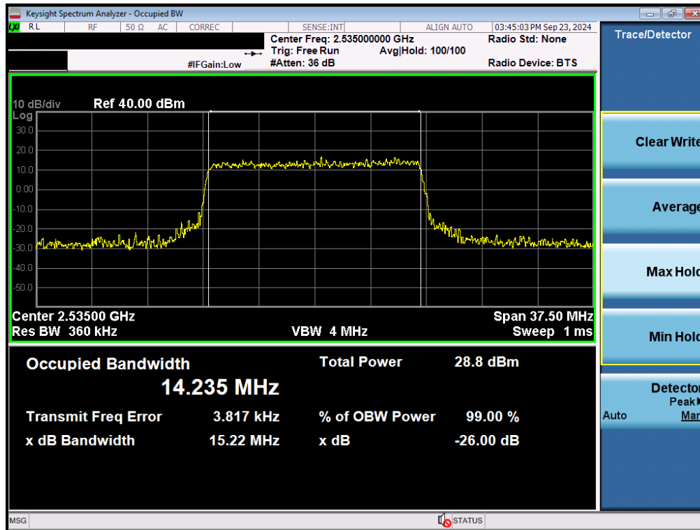
Plot 7-65. Occupied Bandwidth Plot (NR Band n7 - 15MHz 16-QAM - Full RB - Ant F)
