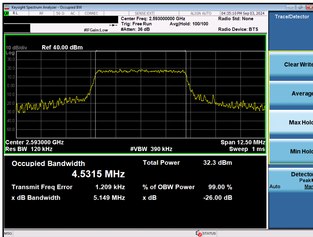
Plot 7-37. Occupied Bandwidth Plot (LTE Band 41(PC3)/38 - 5MHz QPSK - Full RB - Ant B)
