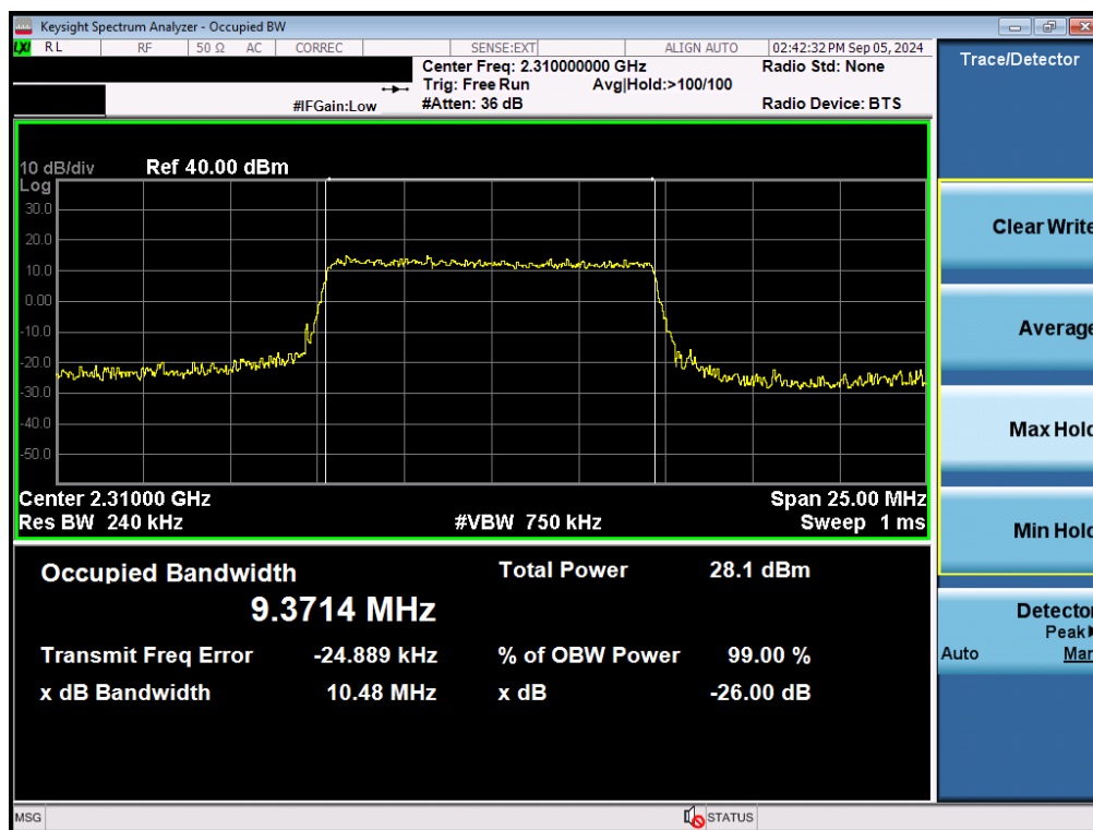
Plot 7-40. Occupied Bandwidth Plot (NR Band n30 - 10MHz QPSK - Full RB - Ant F)
