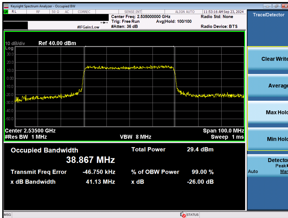
Plot 7-50. Occupied Bandwidth Plot (NR Band n7 - 40MHz 16-QAM - Full RB - Ant F)
