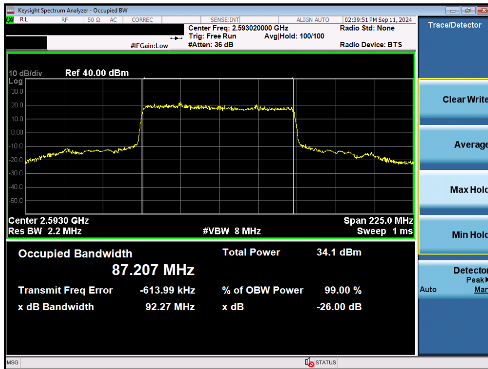
Plot 7-75. Occupied Bandwidth Plot (NR Band n41 - 90MHz \pi/2 BPSK - Full RB - Ant F)
