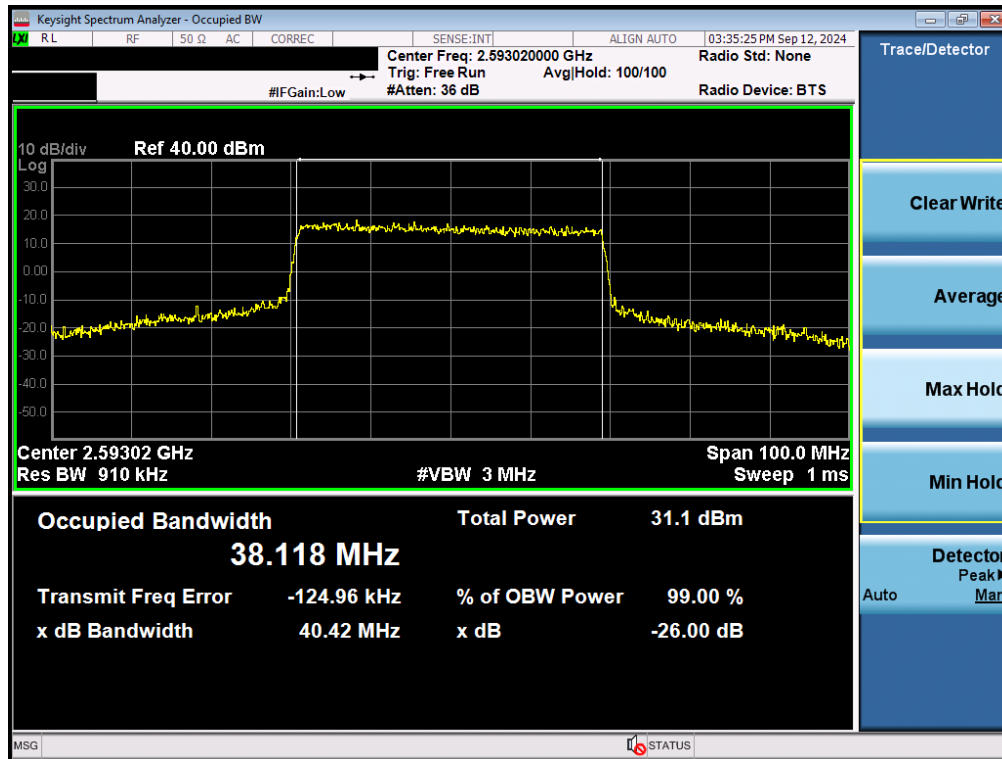
Plot 7-94. Occupied Bandwidth Plot (NR Band n41 - 40MHz QPSK - Full RB - Ant F)
