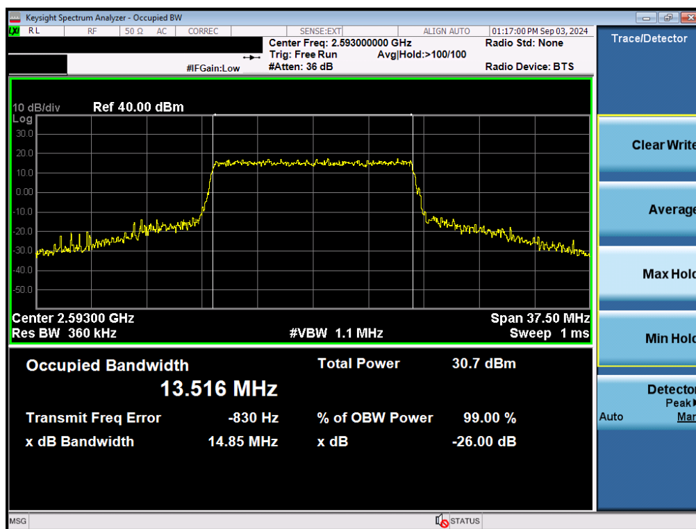
Plot 7-34. Occupied Bandwidth Plot (LTE Band 41(PC3)/38 - 15MHz 16-QAM - Full RB - Ant B)
