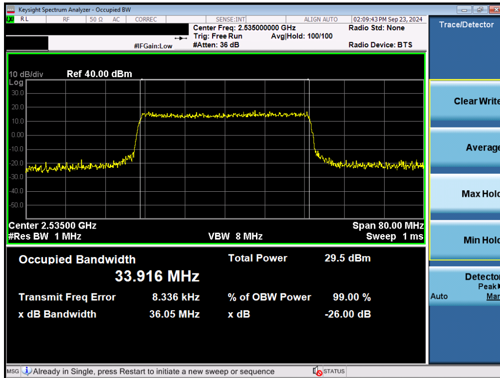
Plot 7-53. Occupied Bandwidth Plot (NR Band n7 - 35MHz 16-QAM - Full RB - Ant F)
