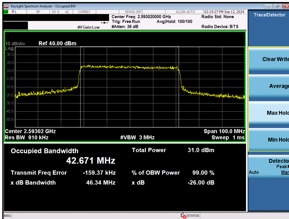
Plot 7-91. Occupied Bandwidth Plot (NR Band n41 - 45MHz QPSK - Full RB - Ant F)
