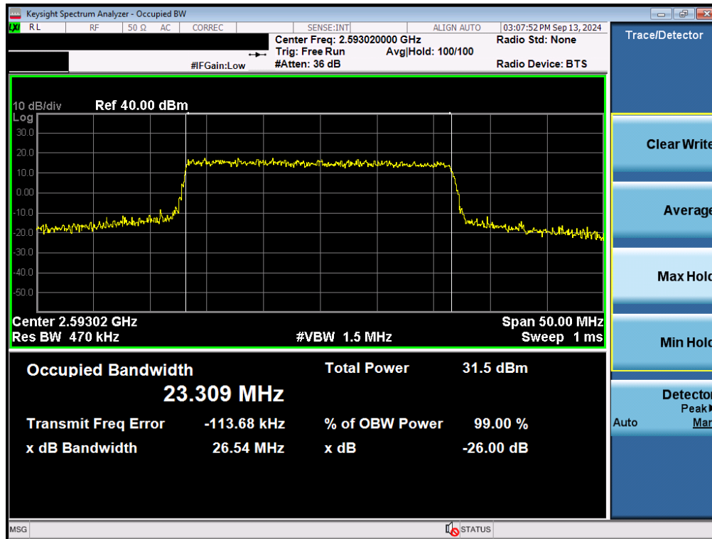
Plot 7-104. Occupied Bandwidth Plot (NR Band n41 - 25MHz 16-QAM - Full RB - Ant F)
