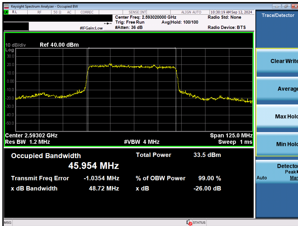
Plot 7-87. Occupied Bandwidth Plot (NR Band n41 - 50MHz \pi/2 BPSK - Full RB - Ant F)
