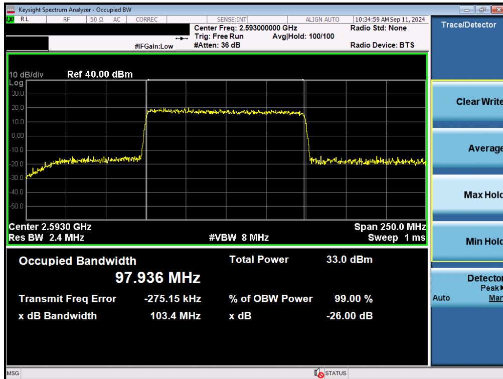
Plot 7-115. Occupied Bandwidth Plot (NR Band n41 - 100MHz QPSK - Full RB - Ant B)
