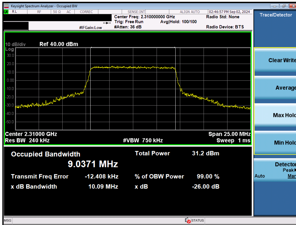
Plot 7-19. Occupied Bandwidth Plot (LTE Band 30 - 10MHz QPSK - Full RB - Ant F – Ant A)
