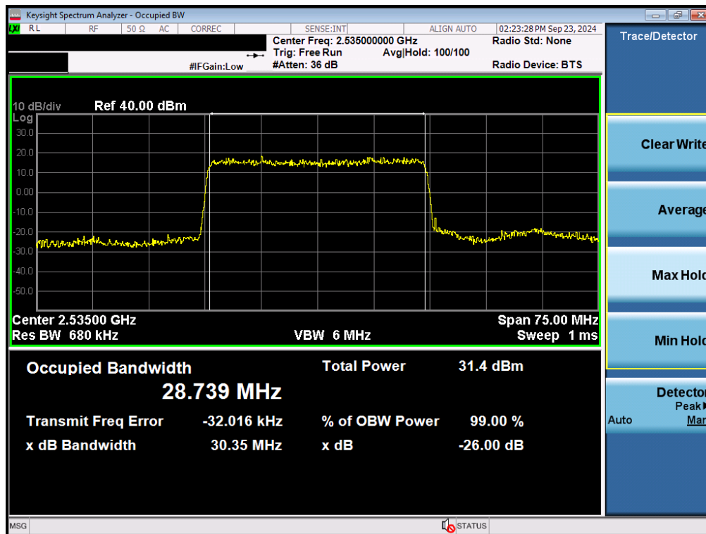
Plot 7-54. Occupied Bandwidth Plot (NR Band n7 - 30MHz \pi/2 BPSK - Full RB - Ant F)
