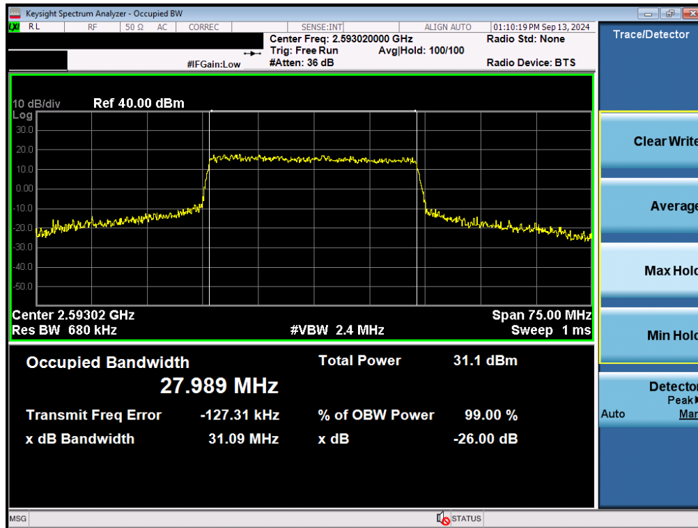
Plot 7-100. Occupied Bandwidth Plot (NR Band n41 - 30MHz QPSK - Full RB - Ant F)
