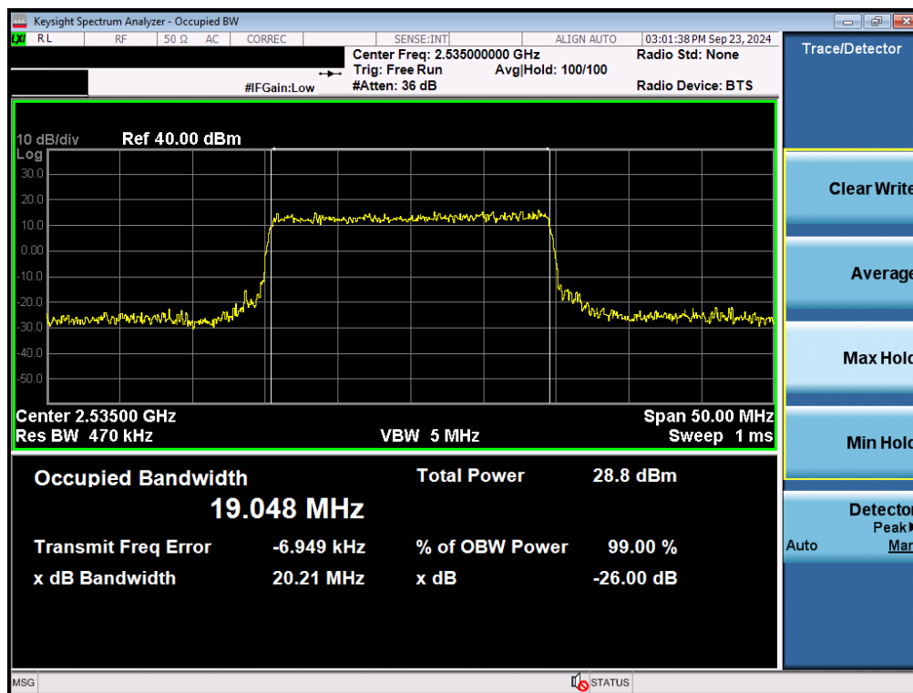
Plot 7-62. Occupied Bandwidth Plot (NR Band n7 - 20MHz 16-QAM - Full RB - Ant F)
