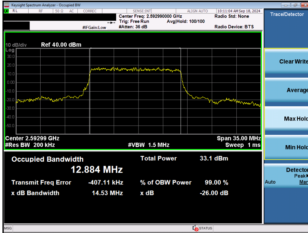
Plot 7-108. Occupied Bandwidth Plot (NR Band n41 - 15MHz \pi/2 BPSK - Full RB - Ant F)
