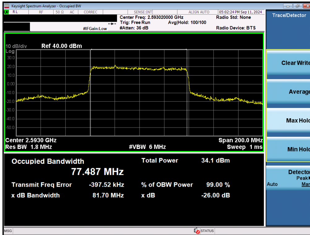
Plot 7-78. Occupied Bandwidth Plot (NR Band n41 - 80MHz \pi/2 BPSK - Full RB - Ant F)
