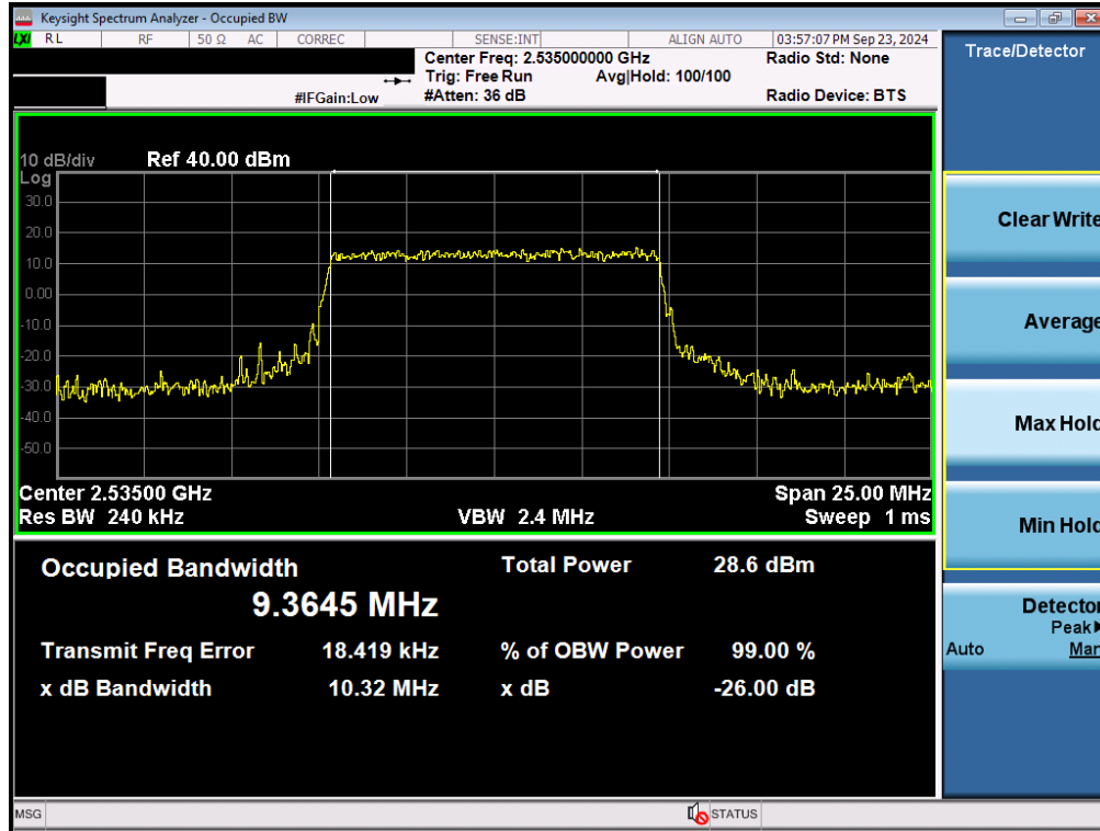
Plot 7-67. Occupied Bandwidth Plot (NR Band n7 - 10MHz QPSK - Full RB - Ant F)
