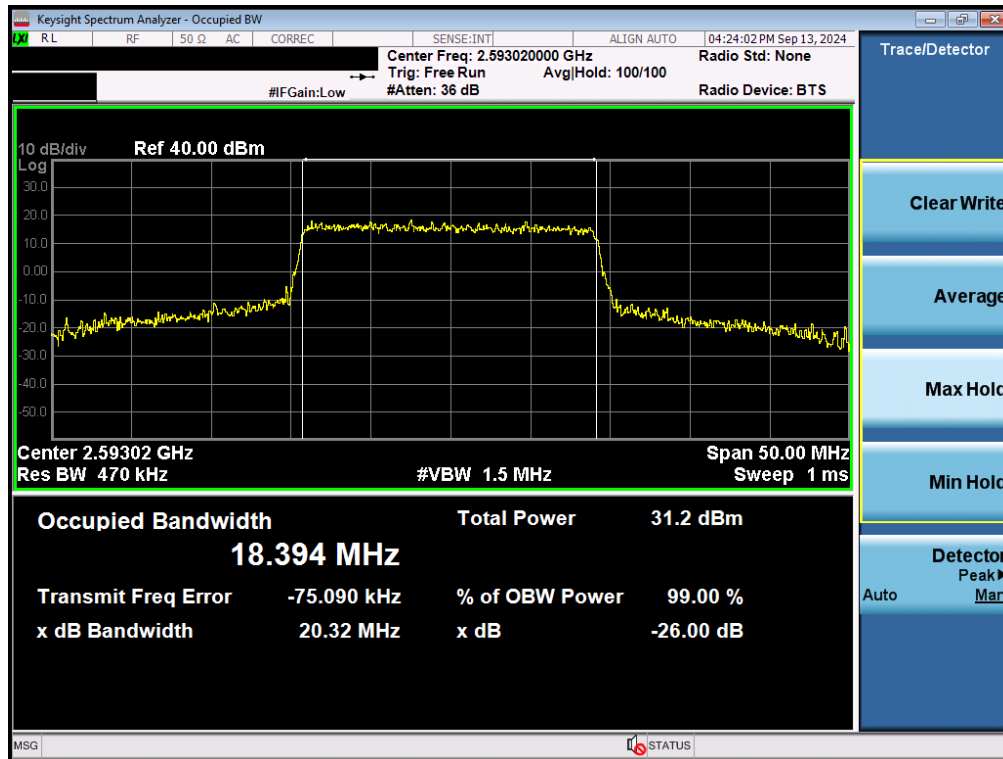
Plot 7-107. Occupied Bandwidth Plot (NR Band n41 - 20MHz 16-QAM - Full RB - Ant F)
