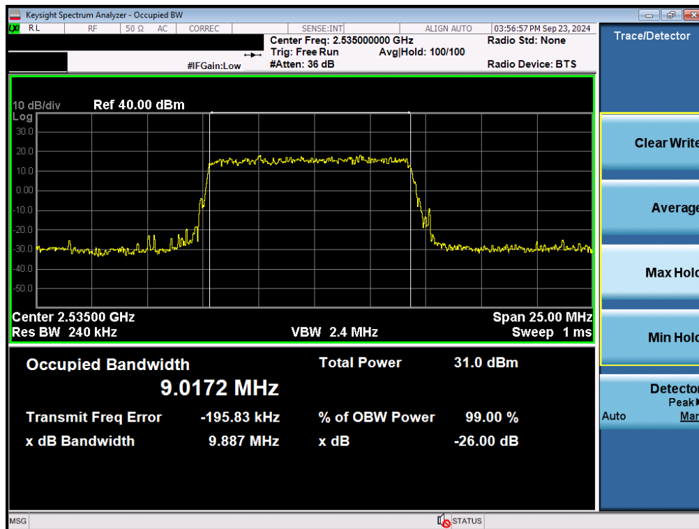
Plot 7-66. Occupied Bandwidth Plot (NR Band n7 - 10MHz \pi/2 BPSK - Full RB - Ant F)
