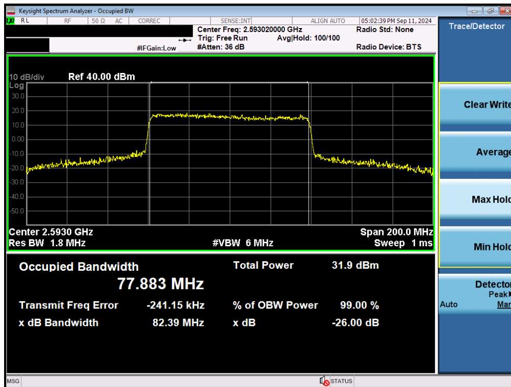
Plot 7-79. Occupied Bandwidth Plot (NR Band n41 - 80MHz QPSK - Full RB - Ant F)
