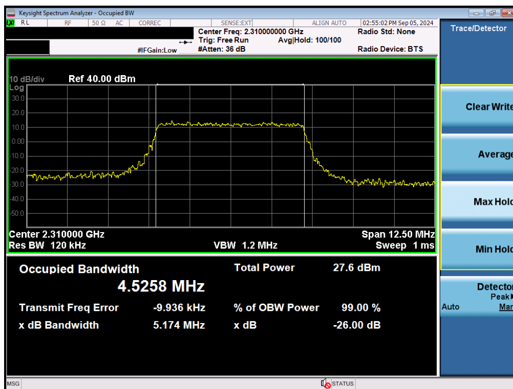
Plot 7-43. Occupied Bandwidth Plot (NR Band n30 - 5MHz QPSK - Full RB - Ant F)
