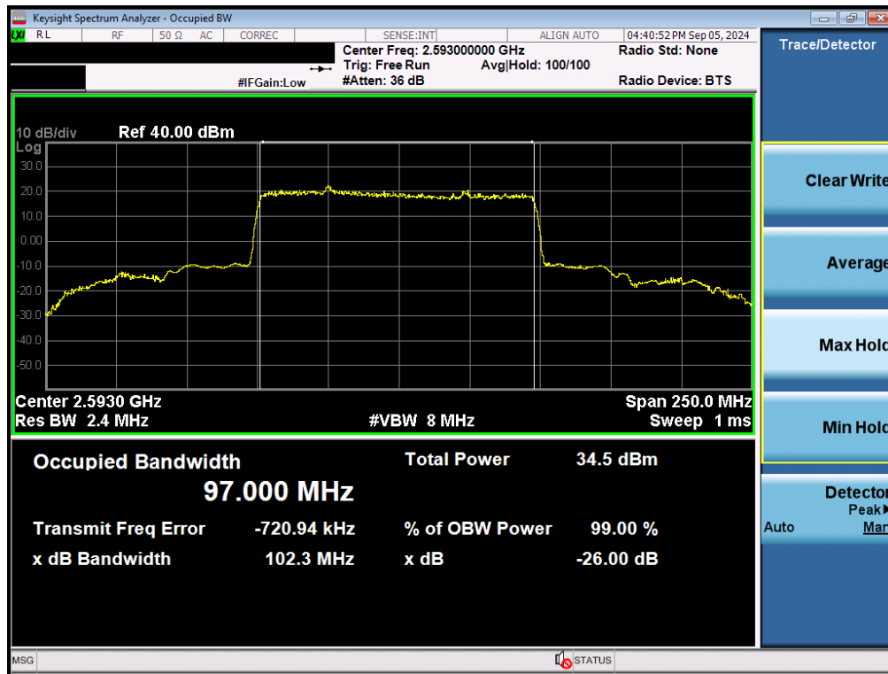
Plot 7-72. Occupied Bandwidth Plot (NR Band n41 - 100MHz \pi/2 BPSK - Full RB - Ant F)
