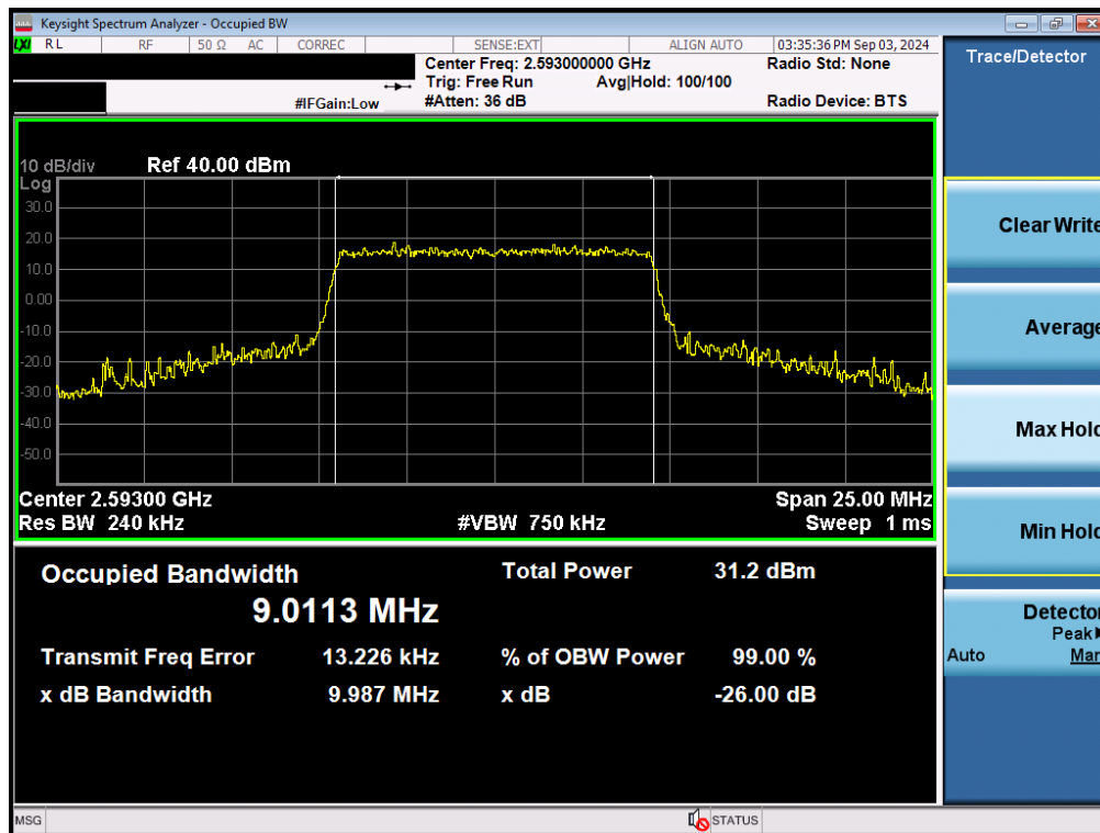
Plot 7-36. Occupied Bandwidth Plot (LTE Band 41(PC3)/38 - 10MHz 16-QAM - Full RB - Ant B)
