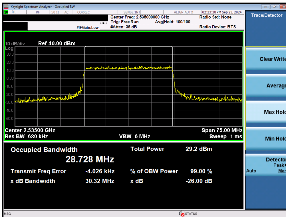
Plot 7-55. Occupied Bandwidth Plot (NR Band n7 - 30MHz QPSK - Full RB - Ant F)
