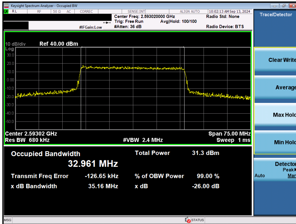
Plot 7-97. Occupied Bandwidth Plot (NR Band n41 - 35MHz QPSK - Full RB - Ant F)
