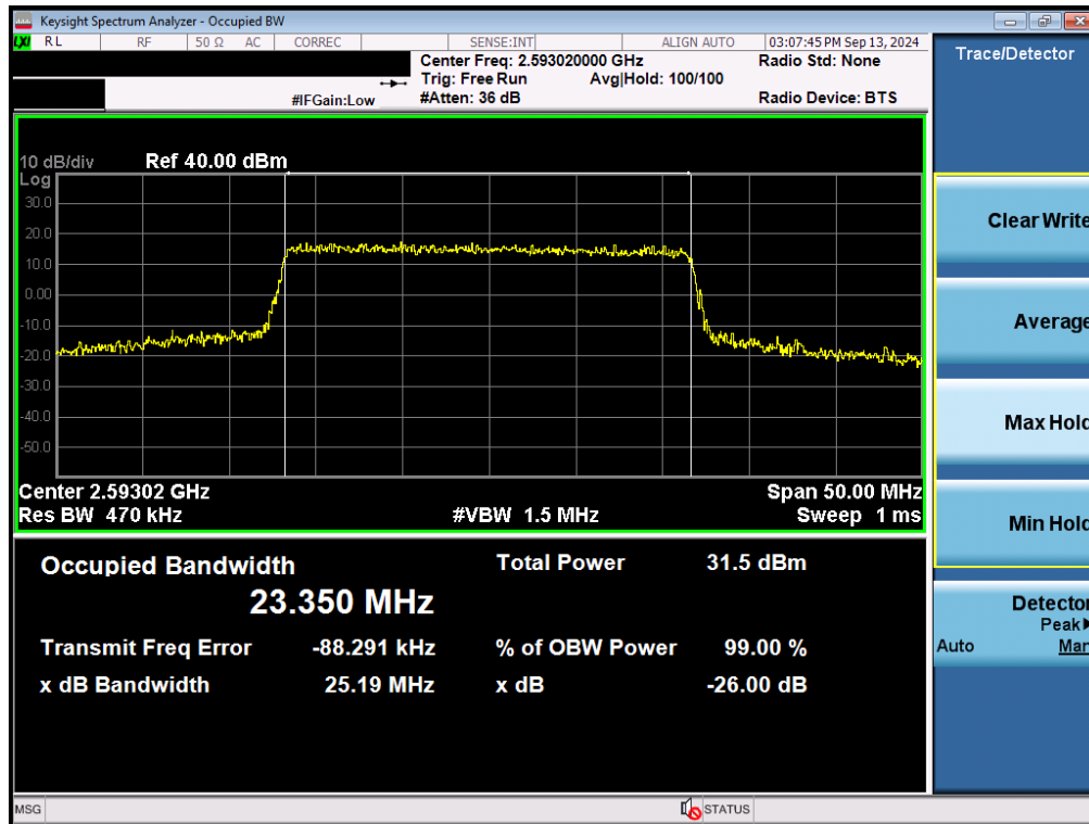
Plot 7-103. Occupied Bandwidth Plot (NR Band n41 - 25MHz QPSK - Full RB - Ant F)
