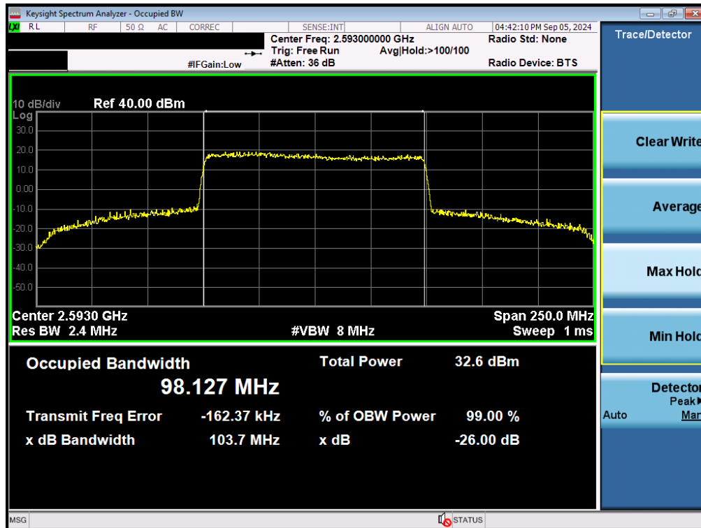
Plot 7-73. Occupied Bandwidth Plot (NR Band n41 - 100MHz QPSK - Full RB - Ant F)
