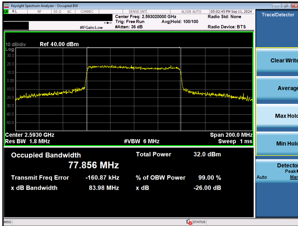
Plot 7-80. Occupied Bandwidth Plot (NR Band n41 - 80MHz 16-QAM - Full RB - Ant F)
