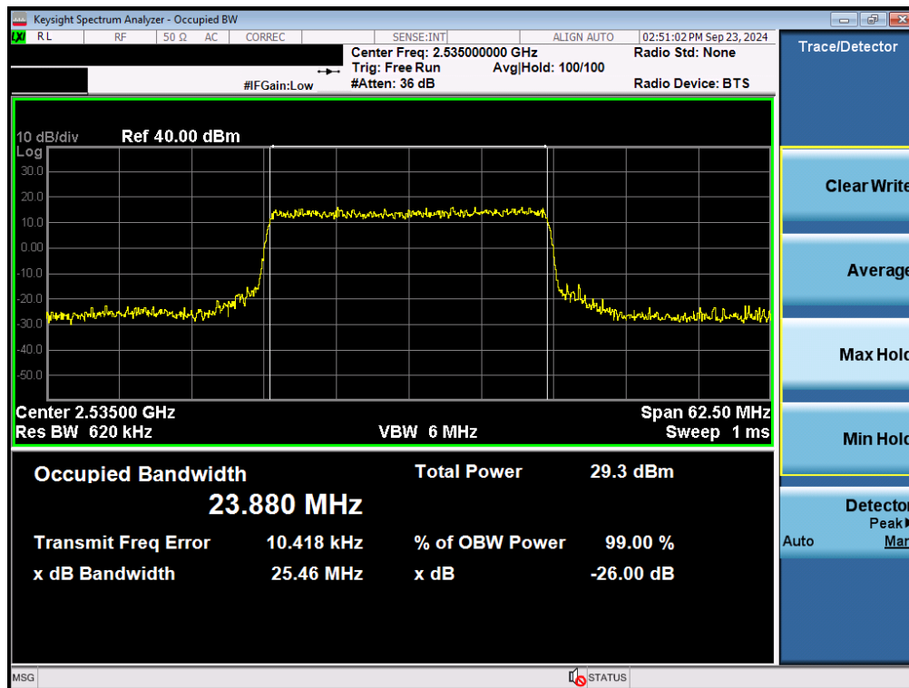
Plot 7-58. Occupied Bandwidth Plot (NR Band n7 - 25MHz QPSK - Full RB - Ant F)
