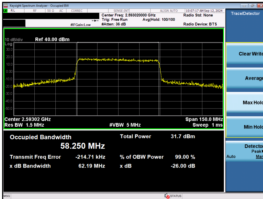
Plot 7-85. Occupied Bandwidth Plot (NR Band n41 - 60MHz QPSK - Full RB - Ant F)
