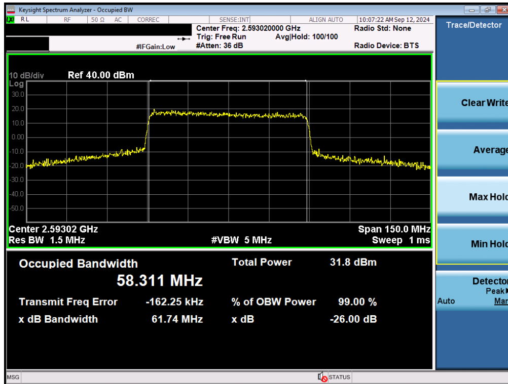
Plot 7-86. Occupied Bandwidth Plot (NR Band n41 - 60MHz 16-QAM - Full RB - Ant F)
