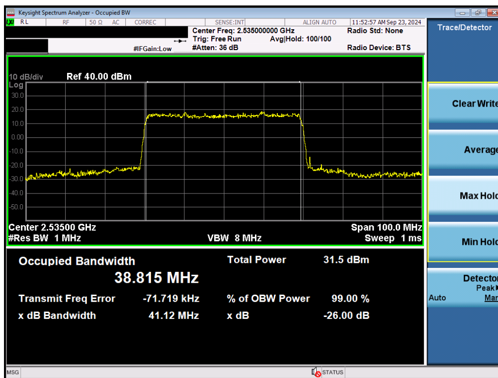
Plot 7-48. Occupied Bandwidth Plot (NR Band n7 - 40MHz \pi/2 BPSK - Full RB - Ant F)
