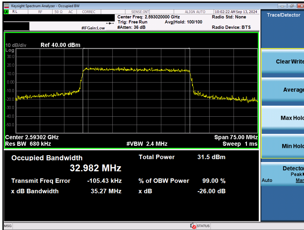
Plot 7-98. Occupied Bandwidth Plot (NR Band n41 - 35MHz 16-QAM - Full RB - Ant F)
