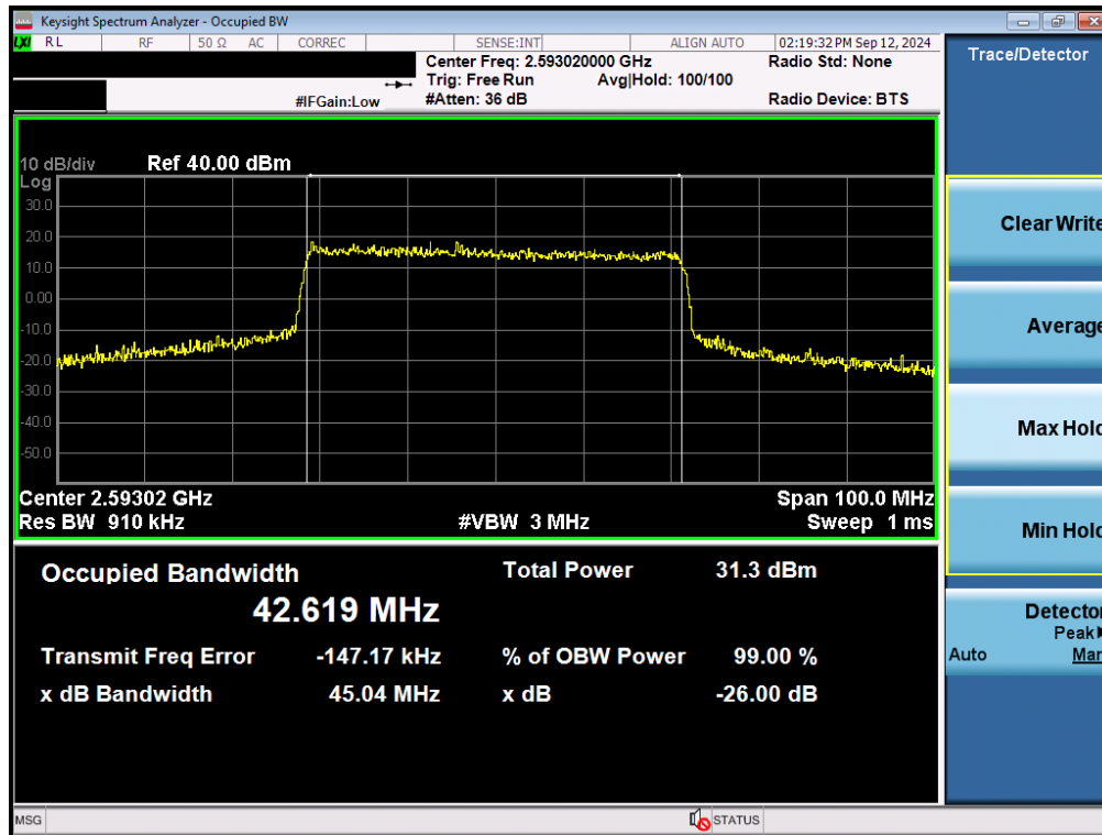
Plot 7-92. Occupied Bandwidth Plot (NR Band n41 - 45MHz 16-QAM - Full RB - Ant F)
