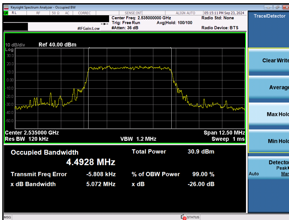
Plot 7-69. Occupied Bandwidth Plot (NR Band n7 - 5MHz \pi/2 BPSK - Full RB - Ant F)
