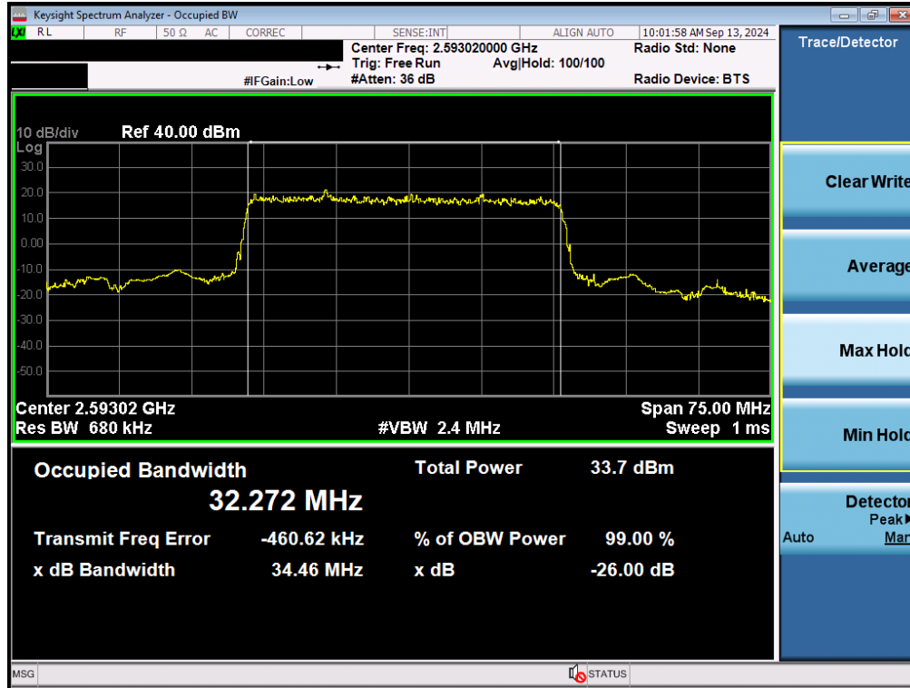
Plot 7-96. Occupied Bandwidth Plot (NR Band n41 - 35MHz \pi/2 BPSK - Full RB - Ant F)
