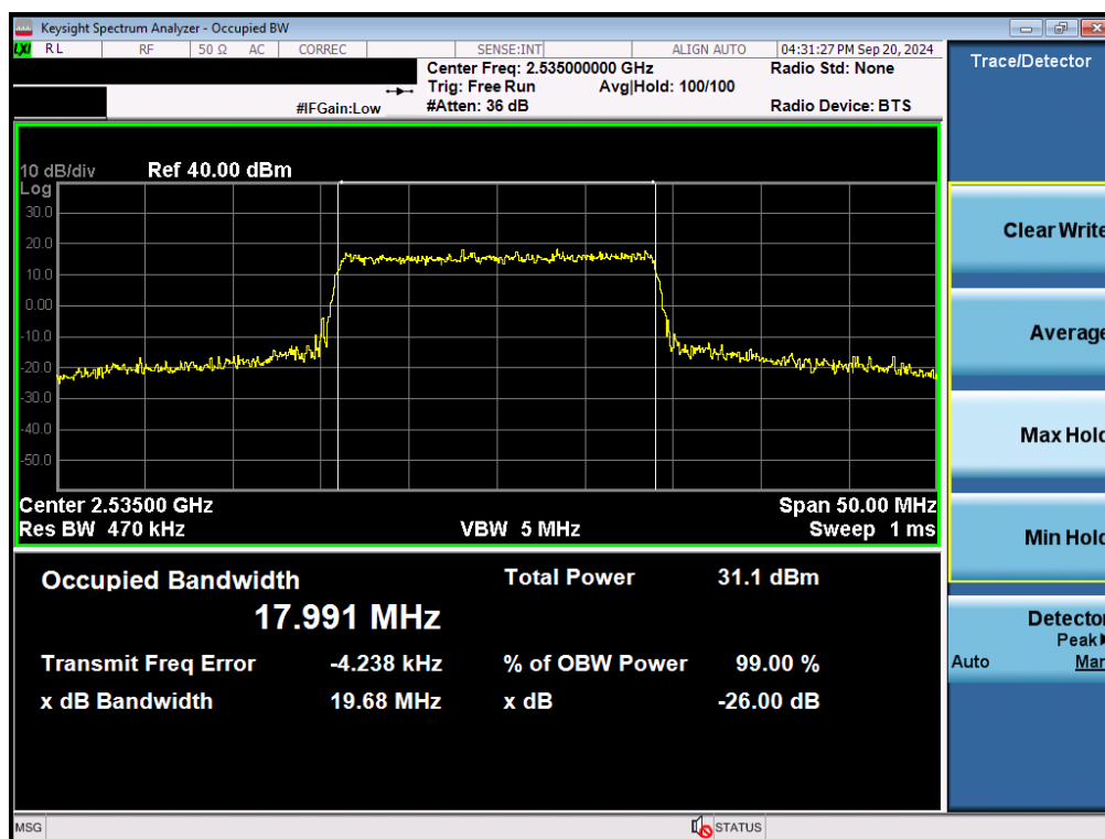
Plot 7-23. Occupied Bandwidth Plot (LTE Band 7 - 20MHz QPSK - Full RB - Ant B)
