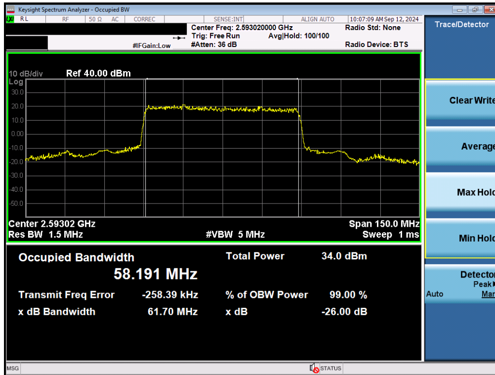
Plot 7-84. Occupied Bandwidth Plot (NR Band n41 - 60MHz \pi/2 BPSK - Full RB - Ant F)
