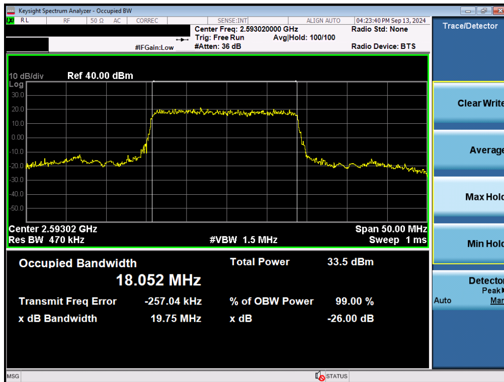
Plot 7-105. Occupied Bandwidth Plot (NR Band n41 - 20MHz \pi/2 BPSK - Full RB - Ant F)
