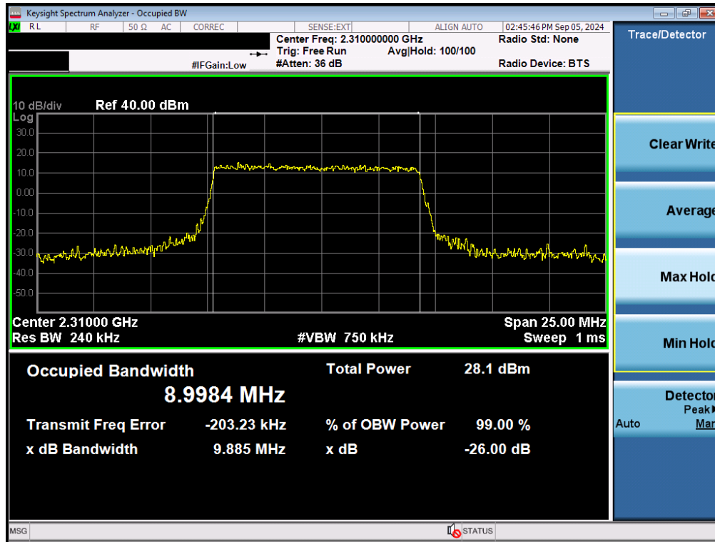
Plot 7-41. Occupied Bandwidth Plot (NR Band n30 - 10MHz 16-QAM - Full RB - Ant F)
