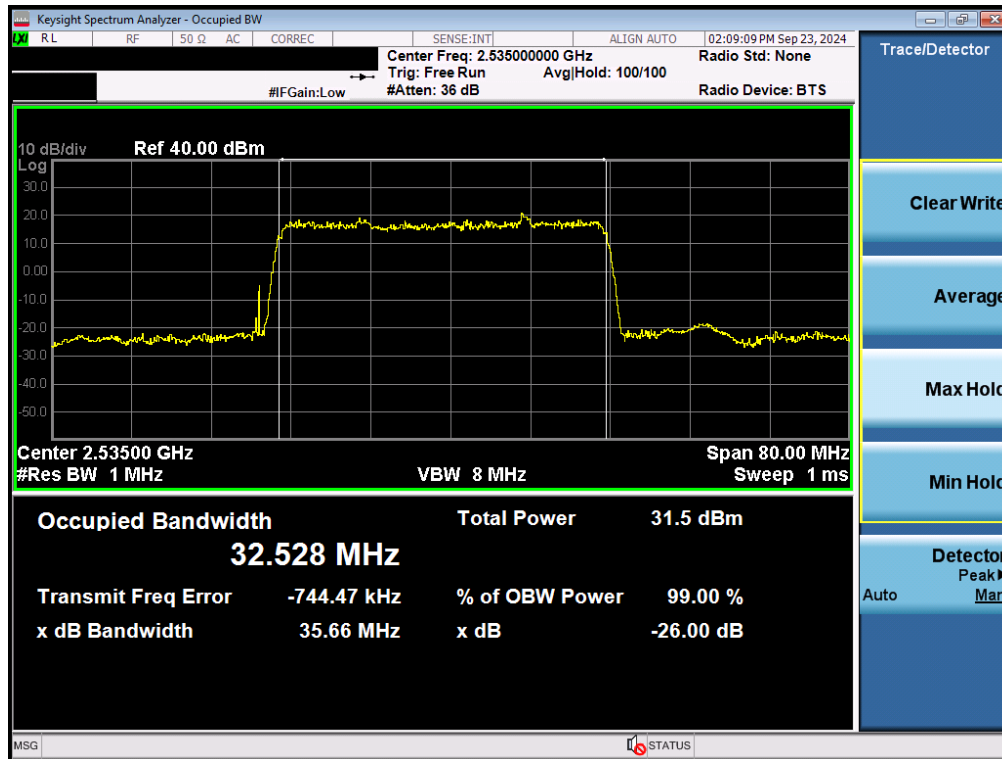
Plot 7-51. Occupied Bandwidth Plot (NR Band n7 - 35MHz \pi/2 BPSK - Full RB - Ant F)
