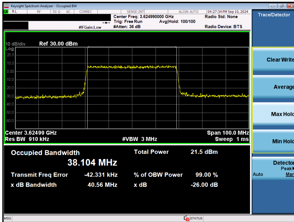
Plot 7-39. Occupied Bandwidth Plot (NR Band n48 - 40MHz QPSK - Full RB Configuration - Ant D)
