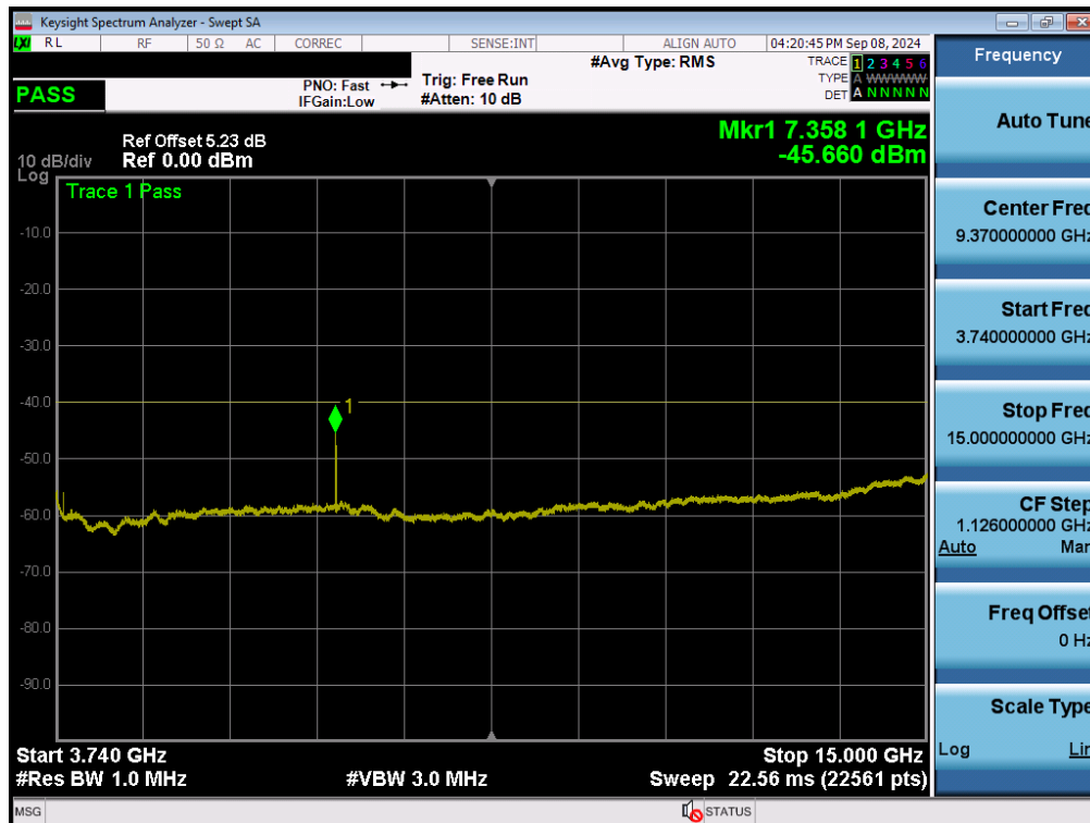
Plot 7-51. Conducted Spurious Plot (NR Band n48 - 40MHz QPSK - High Channel - Ant F)
