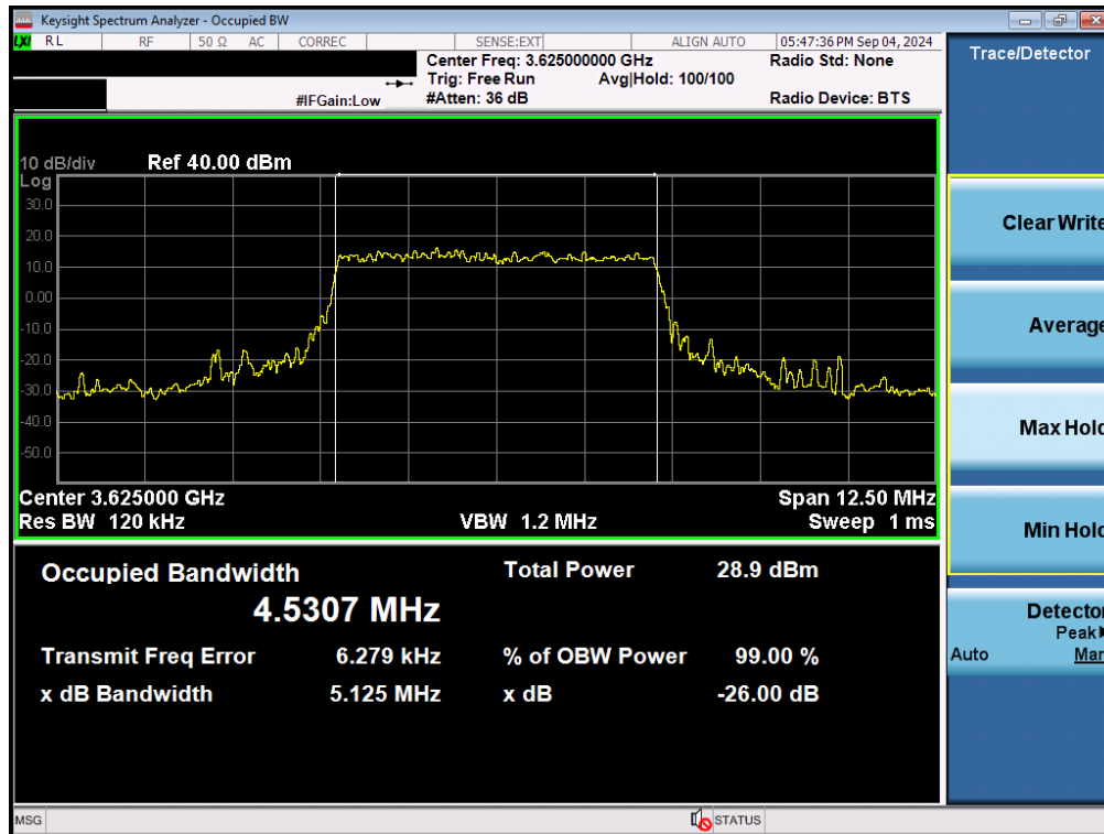
Plot 7-7. Occupied Bandwidth Plot (LTE Band 48 - 5MHz QPSK - Full RB Configuration - Ant F)
