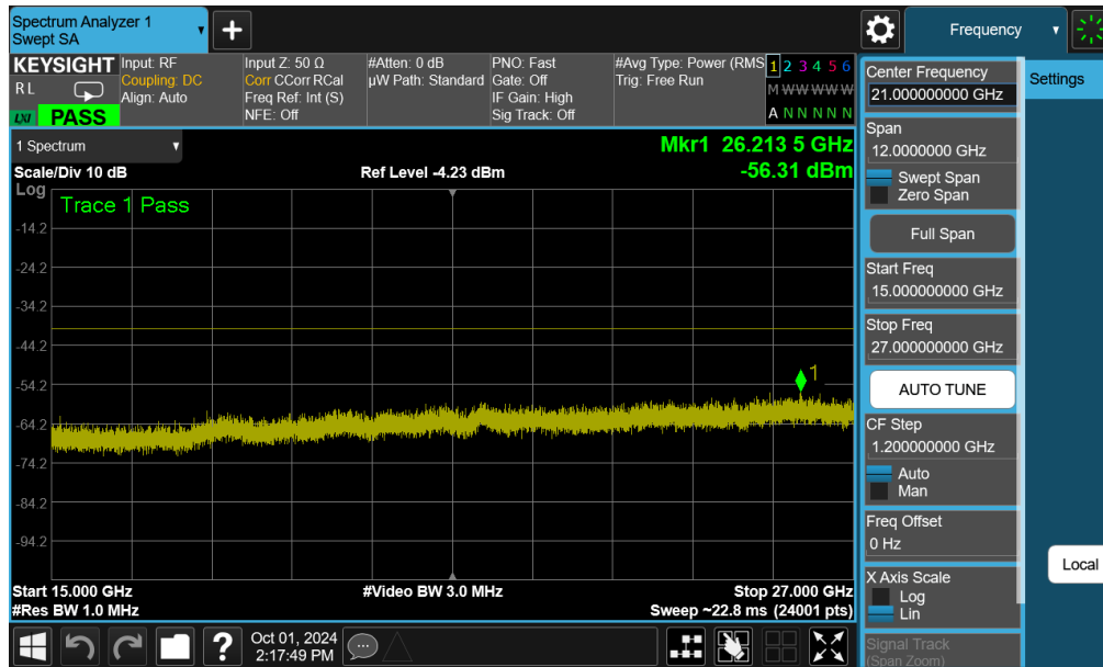
Plot 7-43. Conducted Spurious Plot (LTE Band 48 - 20MHz QPSK - High Channel - Ant F)
