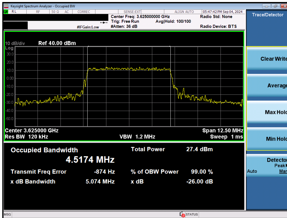
Plot 7-8. Occupied Bandwidth Plot (LTE Band 48 - 5MHz 16-QAM - Full RB Configuration - Ant F)
