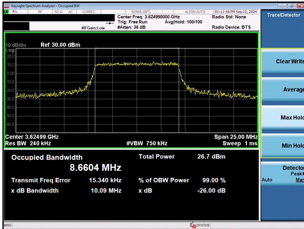
Plot 7-31. Occupied Bandwidth Plot (NR Band n48 - 10MHz 16-QAM - Full RB Configuration - Ant F)
