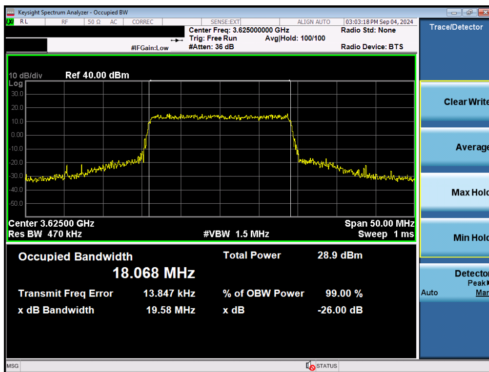
Plot 7-1. Occupied Bandwidth Plot (LTE Band 48 - 20MHz QPSK - Full RB Configuration - Ant F)
