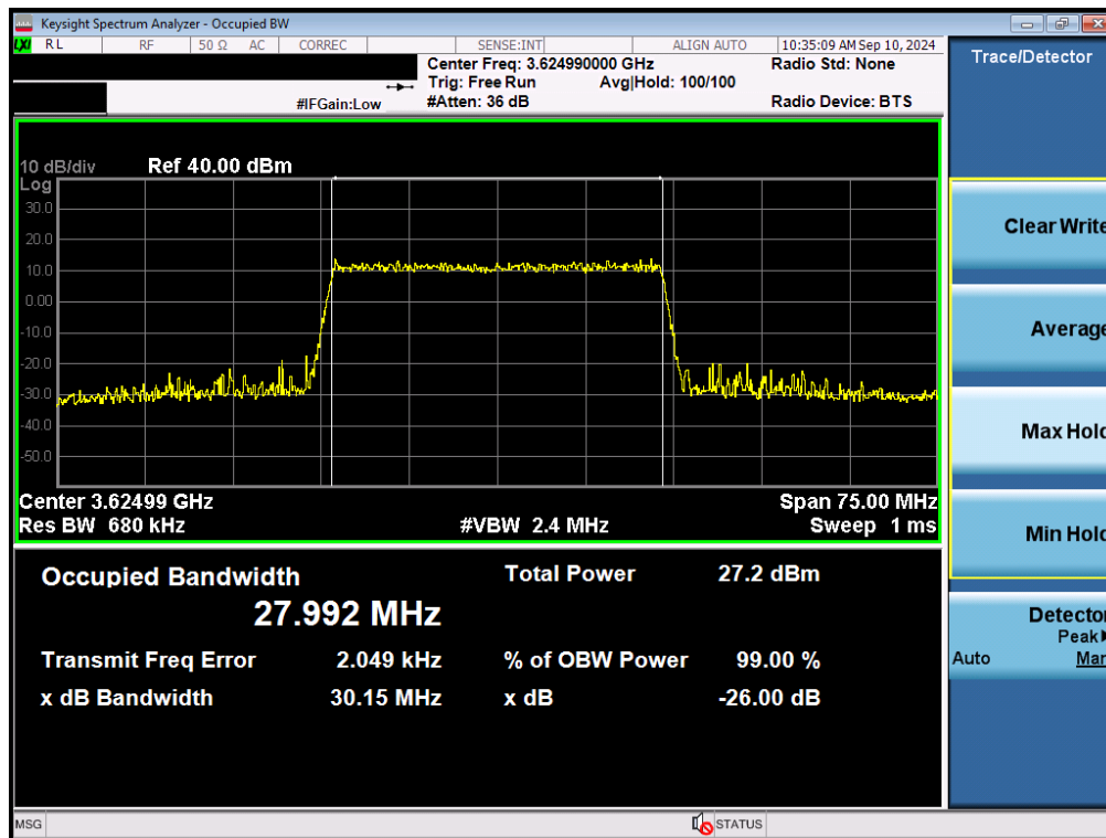
Plot 7-22. Occupied Bandwidth Plot (NR Band n48 - 30MHz 16-QAM - Full RB Configuration - Ant F)
