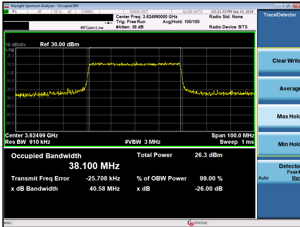
Plot 7-37. Occupied Bandwidth Plot (NR Band n48 - 40MHz 16-QAM - Full RB Configuration - Ant I)
