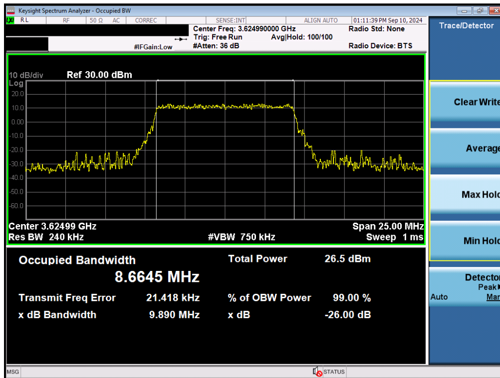
Plot 7-30. Occupied Bandwidth Plot (NR Band n48 - 10MHz QPSK - Full RB Configuration - Ant F)
