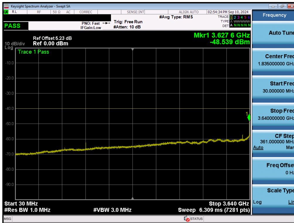
Plot 7-54. Conducted Spurious Plot (NR Band n48 - 40MHz QPSK – High Channel - Ant C)
