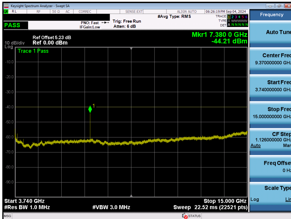
Plot 7-42. Conducted Spurious Plot (LTE Band 48 - 20MHz QPSK - High Channel - Ant F)
