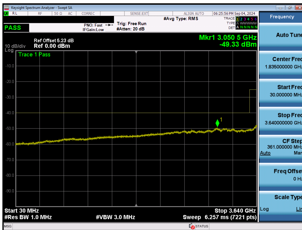
Plot 7-41. Conducted Spurious Plot (LTE Band 48 - 20MHz QPSK - High Channel - Ant F)
