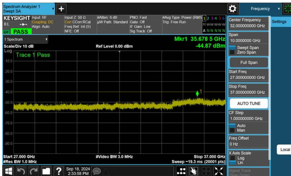
Plot 7-49. Conducted Spurious Plot (ULCA LB48 - 20+20MHz QPSK - Mid Channel - Ant F)
