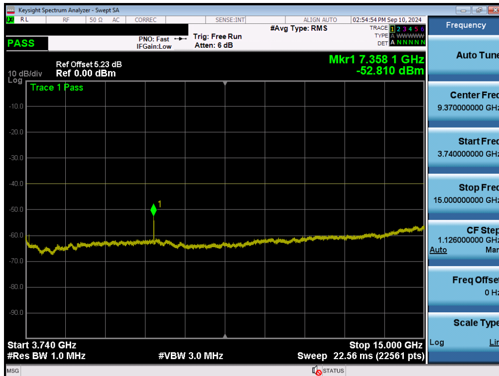
Plot 7-55. Conducted Spurious Plot (NR Band n48 - 40MHz QPSK - High Channel - Ant C)
