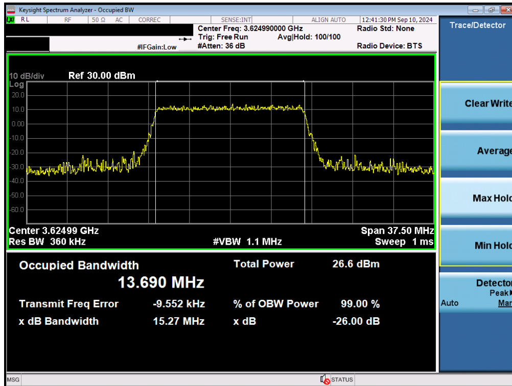
Plot 7-27. Occupied Bandwidth Plot (NR Band n48 - 15MHz QPSK - Full RB Configuration - Ant F)
