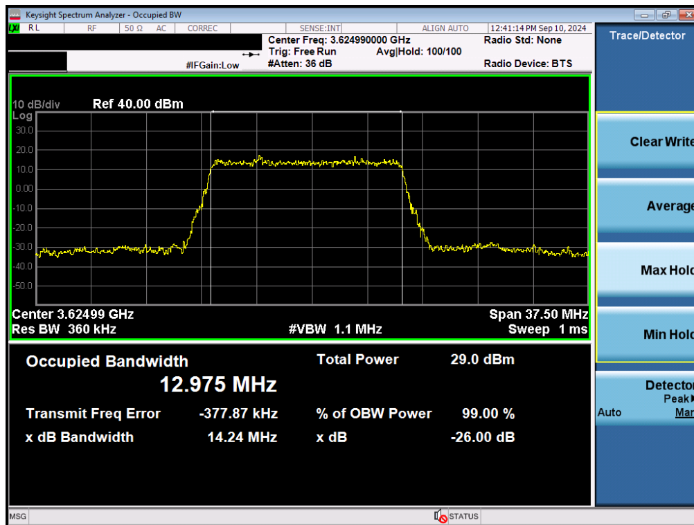
Plot 7-26. Occupied Bandwidth Plot (NR Band n48 - 15MHz \pi/2 BPSK - Full RB Configuration - Ant F)
