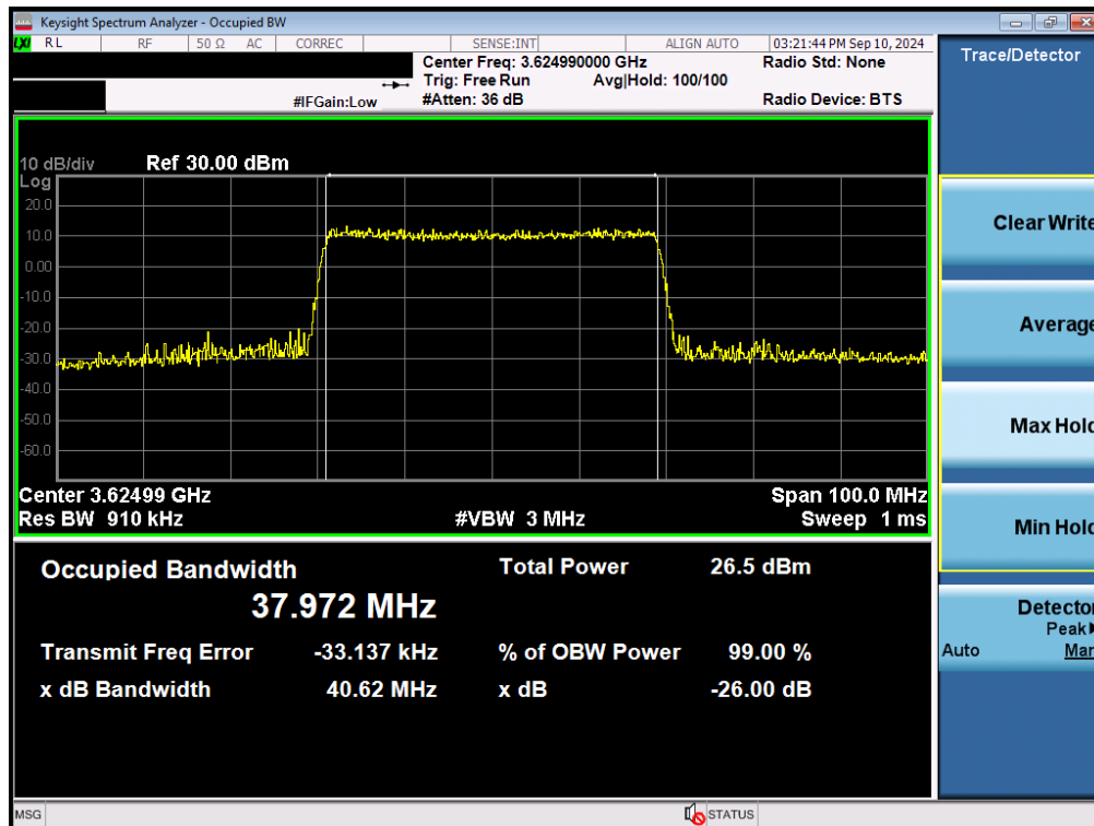
Plot 7-36. Occupied Bandwidth Plot (NR Band n48 - 40MHz QPSK - Full RB Configuration - Ant I)
