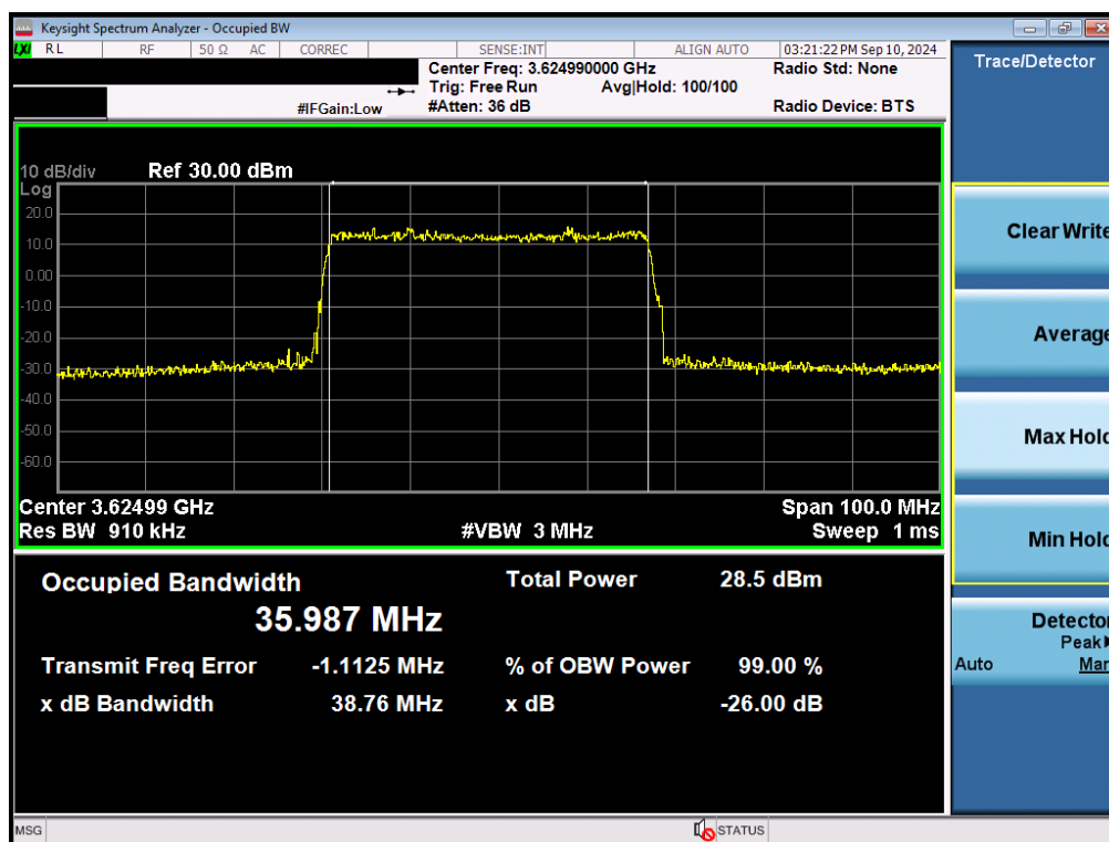
Plot 7-35. Occupied Bandwidth Plot (NR Band n48 - 40MHz \pi/2 BPSK - Full RB Configuration - Ant I)
