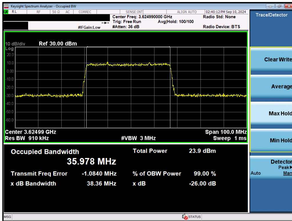
Plot 7-32. Occupied Bandwidth Plot (NR Band n48 - 40MHz \pi/2 BPSK - Full RB Configuration - Ant C)
