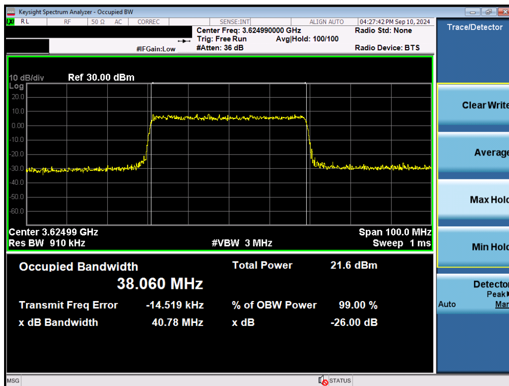
Plot 7-40. Occupied Bandwidth Plot (NR Band n48 - 40MHz 16-QAM - Full RB Configuration - Ant D)
