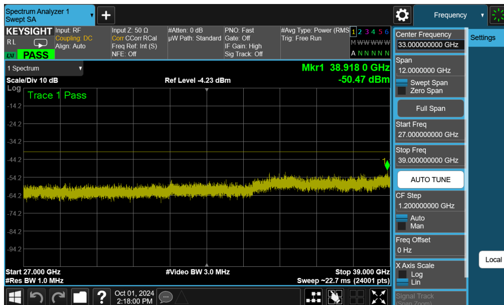
Plot 7-44. Conducted Spurious Plot (LTE Band 48 - 20MHz QPSK - High Channel - Ant F)
