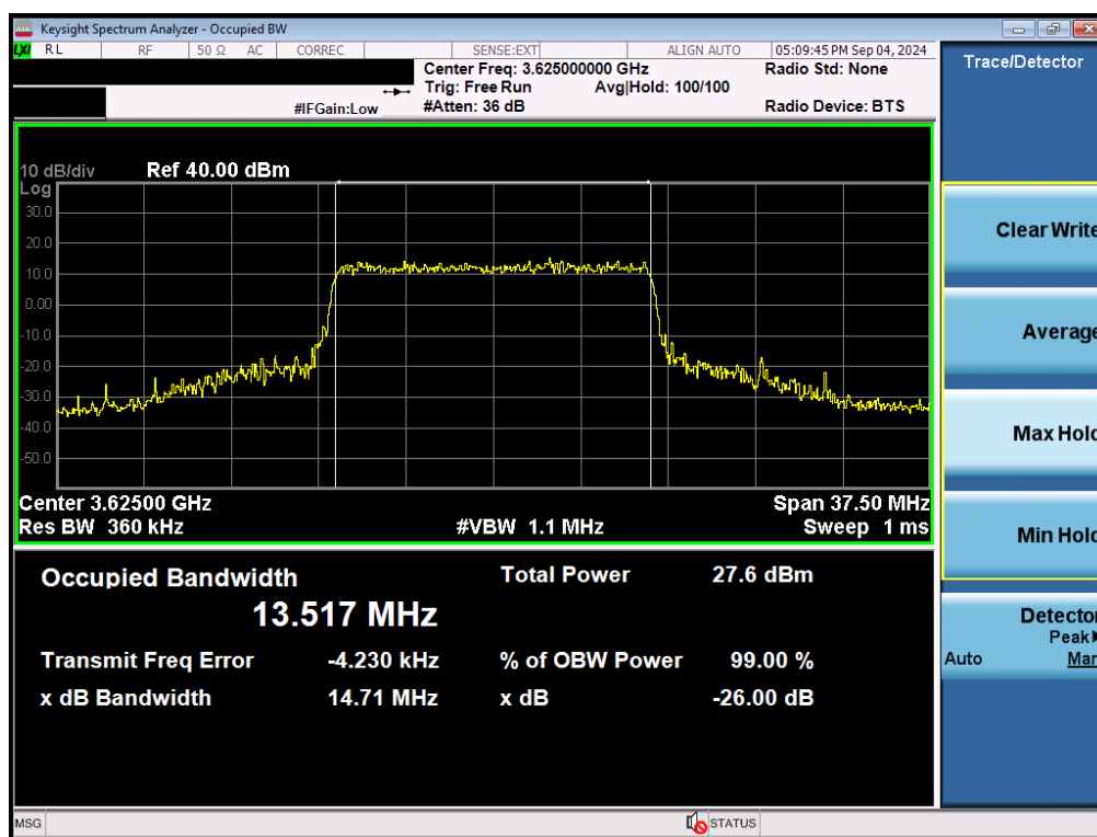
Plot 7-4. Occupied Bandwidth Plot (LTE Band 48 - 15MHz 16-QAM - Full RB Configuration - Ant F)
