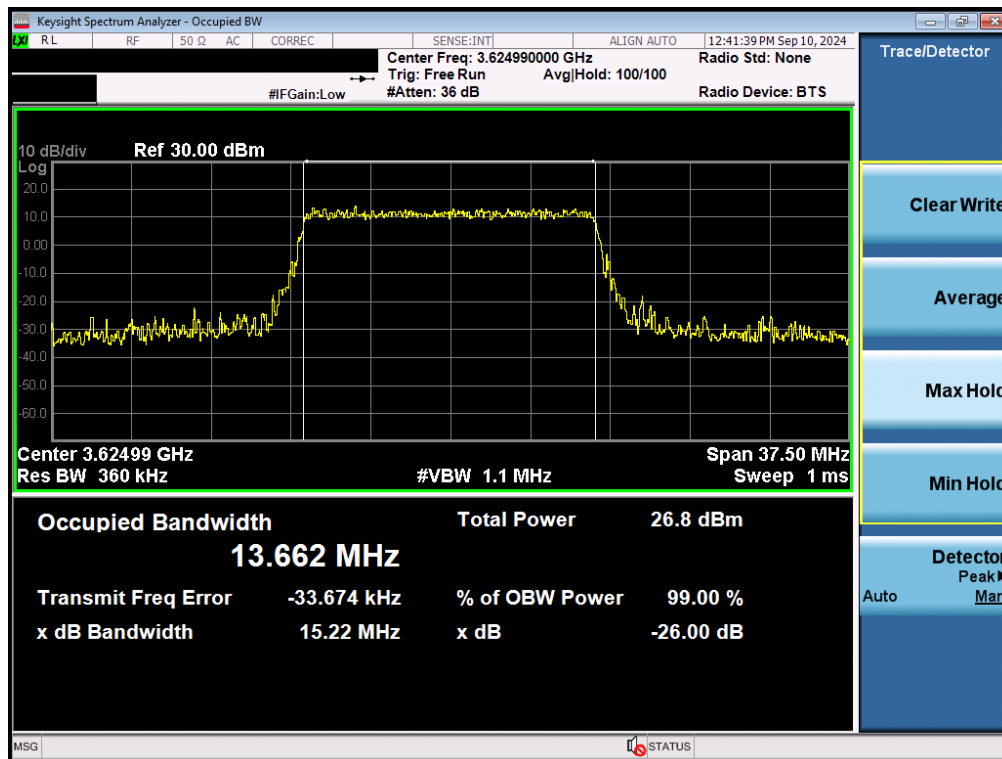
Plot 7-28. Occupied Bandwidth Plot (NR Band n48 - 15MHz 16-QAM - Full RB Configuration - Ant F)
