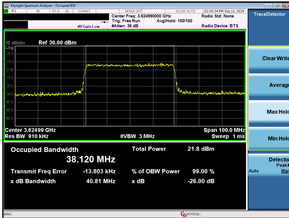
Plot 7-34. Occupied Bandwidth Plot (NR Band n48 - 40MHz 16-QAM - Full RB Configuration - Ant C)
