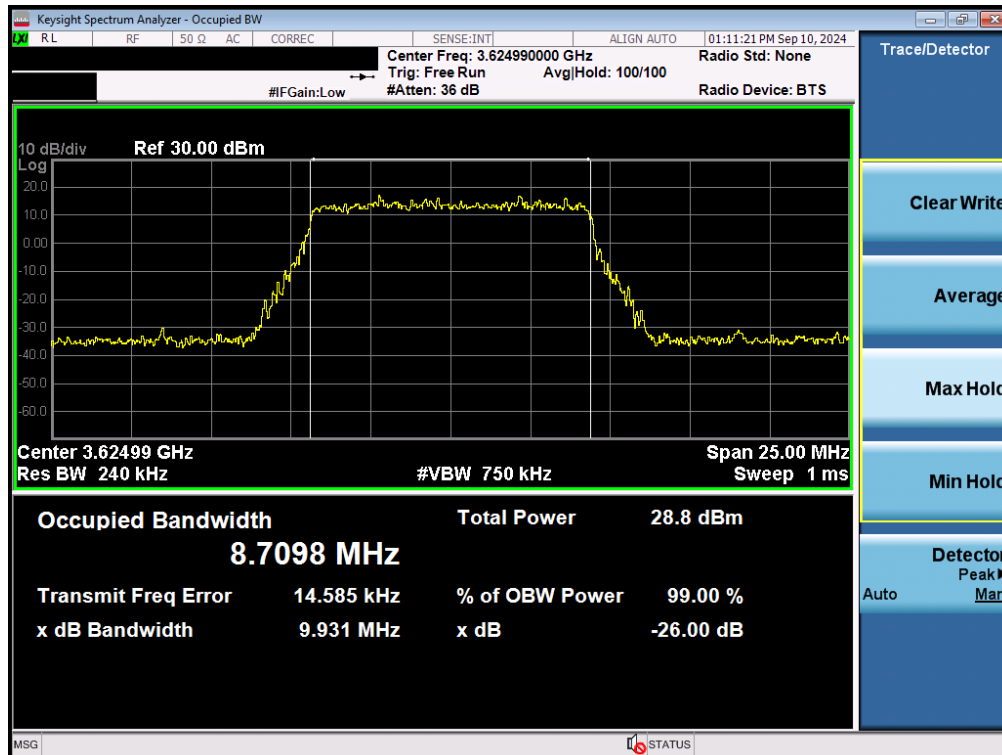
Plot 7-29. Occupied Bandwidth Plot (NR Band n48 - 10MHz \pi/2 BPSK - Full RB Configuration - Ant F)
