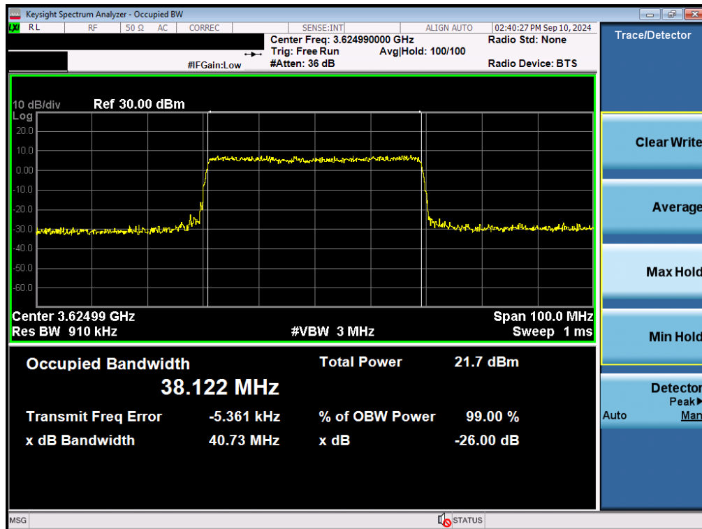
Plot 7-33. Occupied Bandwidth Plot (NR Band n48 - 40MHz QPSK - Full RB Configuration - Ant C)
