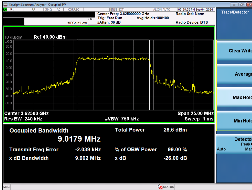
Plot 7-5. Occupied Bandwidth Plot (LTE Band 48 - 10MHz QPSK - Full RB Configuration - Ant F)
