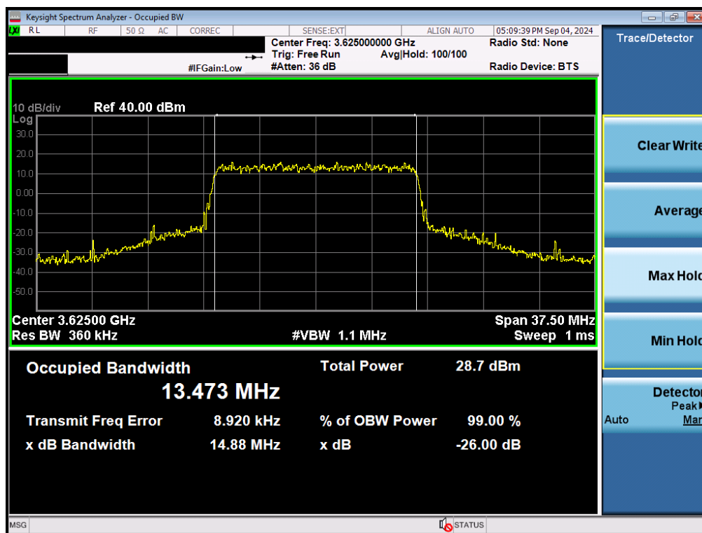
Plot 7-3. Occupied Bandwidth Plot (LTE Band 48 - 15MHz QPSK - Full RB Configuration - Ant F)
