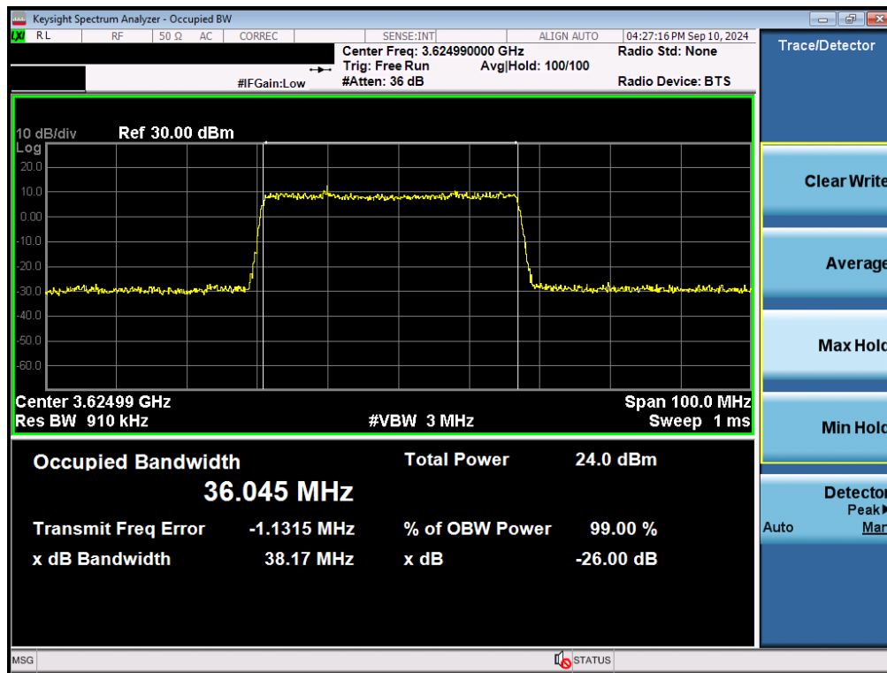
Plot 7-38. Occupied Bandwidth Plot (NR Band n48 - 40MHz \pi/2 BPSK - Full RB Configuration - Ant D)
