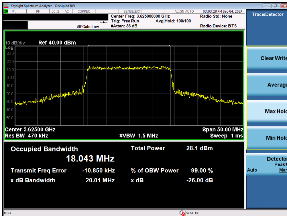
Plot 7-2. Occupied Bandwidth Plot (LTE Band 48 - 20MHz 16-QAM - Full RB Configuration - Ant F)
